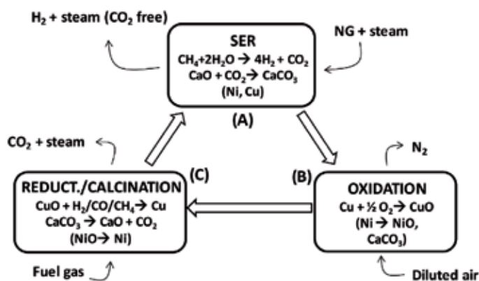
Figure 1. Conceptual scheme of the Ca-Cu looping process.
