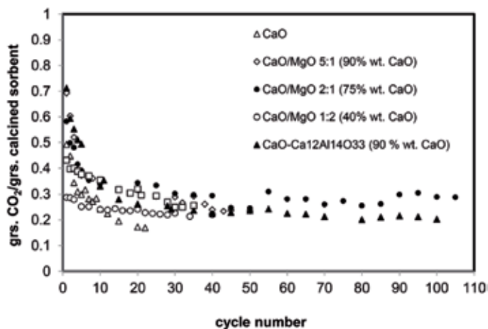
Figure 2. Evolution of CO 2 carrying capacity with the number of cycles for different CaO-based materials (adapted from the information published in [24]). White symbols correspond to materials tested in powder form (<75 μm) and black symbols to materials in particle size cut of 0.6–1 mm.
