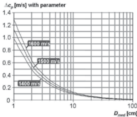
Fig. 5. Dependence of \Delta c_p on D_{med} (formula (6)) for different values of c_p in a measurement area
