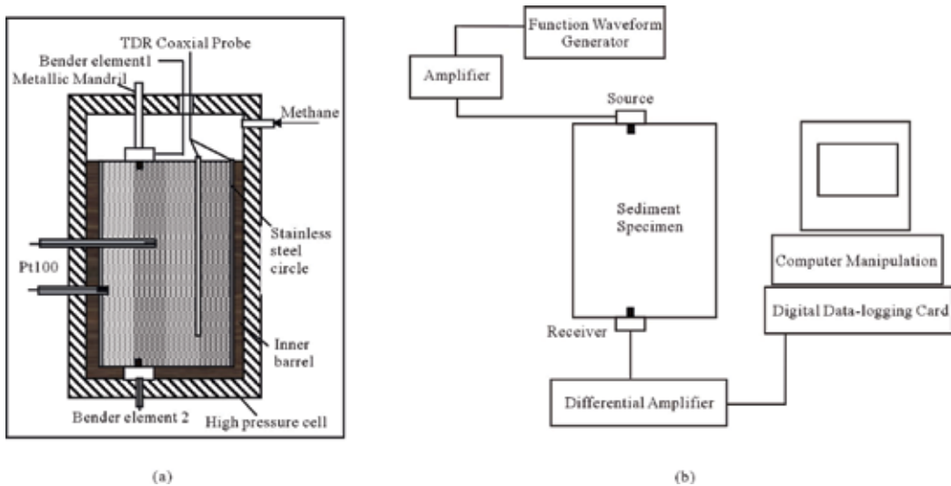
Fig. 11. (a) Schematic map of the high pressure cell for hydrate formation and acoustic measurements; (b) Measuring system of bender elements
