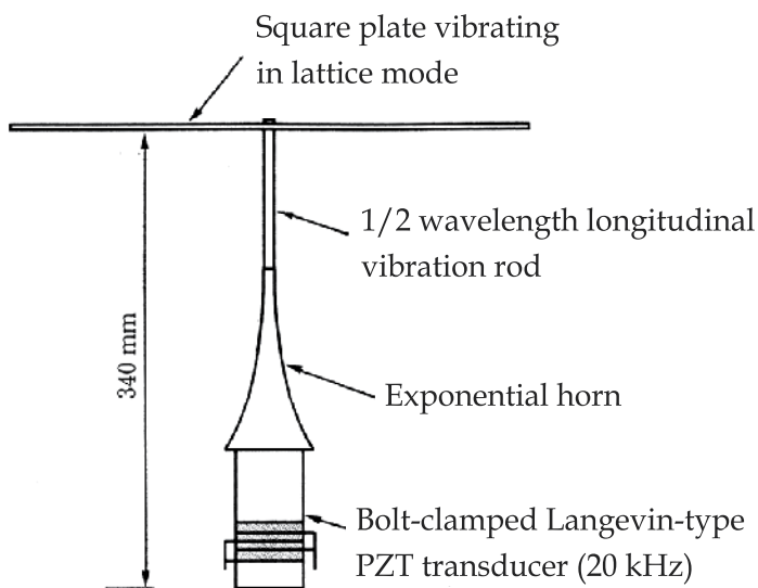
Fig. 1. Schematic diagram of an aerial ultrasonic source.
