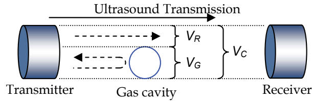
Fig. 2. The simplified ultrasound transmission model
