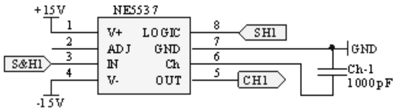
Fig. 11. The sample and hold circuit
