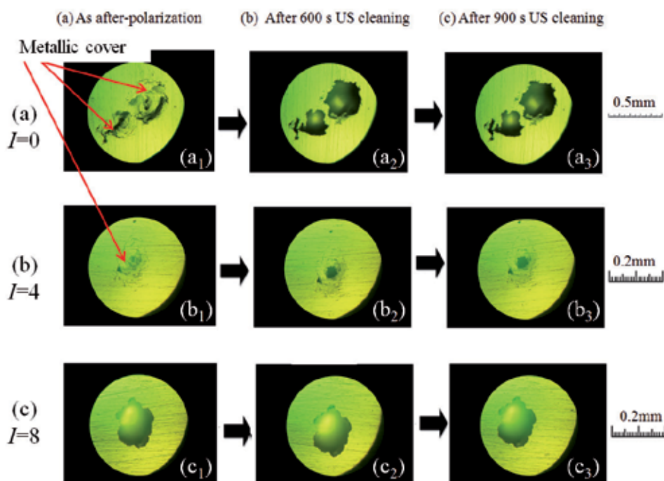
Fig. 21. Surface morphology of specimens after simultaneously holding potential and applying ultrasound at I = 0 (a), I = 4 (b) and I = 8 (c) at frequency of 19.5 kHz. The surfaces a_1 , b_1 and c_1 are cleaned only by running distilled water; a_2 , b_2 , c_2 and a_3 , b_3 , c_3 are further cleaned in distilled water by an ultrasound cleaner for a total time of 600 s and 900 s.
