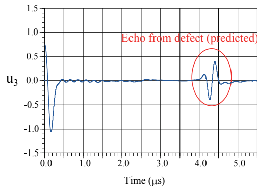
Fig. 21. Predicted echo which is observed at the array transducer.
