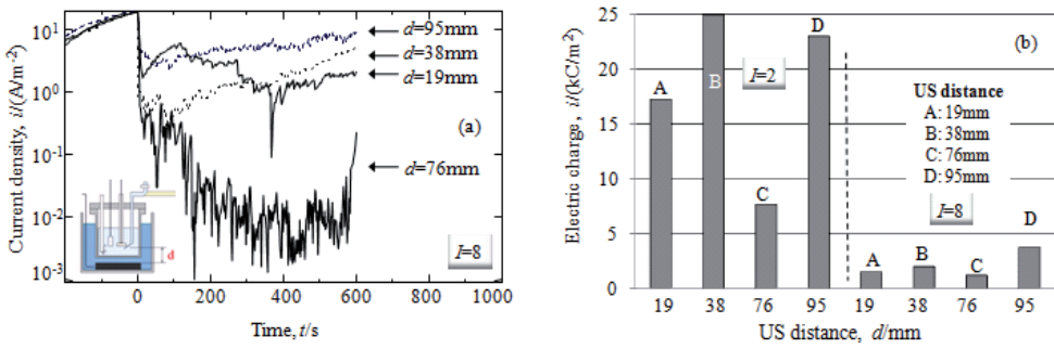
Fig. 14. Pitting current density (a) and accumulated electric charge (b) during the period of simultaneously holding potential and applying ultrasound with different distances at a constant input power of I = 8 or I = 2 . Copyright 2009 Elsevier
