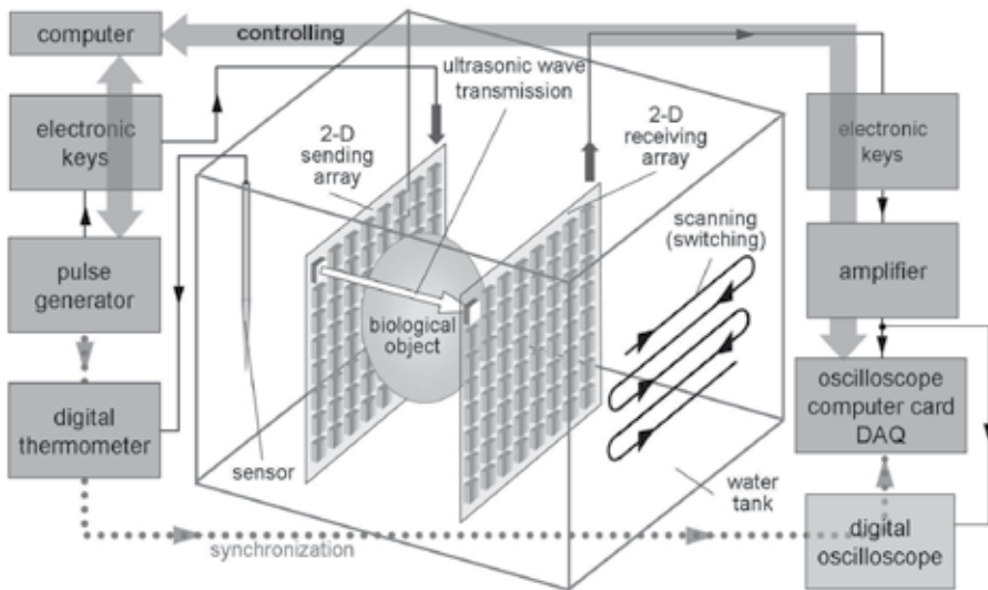
Fig. 21. Block scheme of the laboratory measurement setup for visualization of the distribution of acoustic parameters of biological media internal structure by means of ultrasonic projection method
