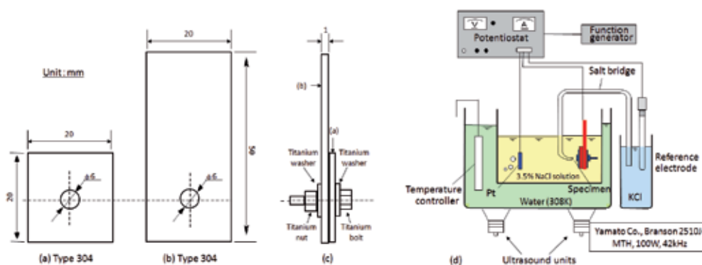
Fig. 5. (a-c) Specimen with crevice and (d) apparatus for polarization test. Copyright 2008 The Japan Institute of Metals
