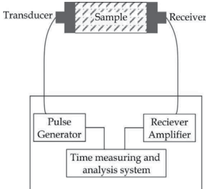
Fig. 1. Pulse velocity test (Malhotra & Carino, 1991)
