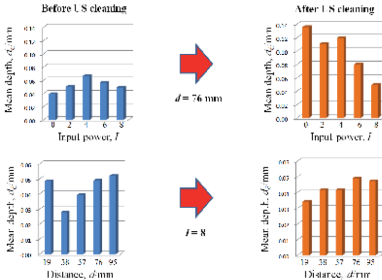
Fig. 22. Mean depth of pits before and after ultrasound cleaning on specimens, which were polarized by simultaneously holding potential and applying ultrasound with frequency of f_1 = 19.5 kHz.
