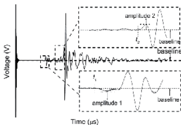
Fig. 2. Ultrasonic waveform measured by flat-plate transducers. Arrival times of the first arrival wave of compressional and shear waves are t_1 and t_2 , respectively. Amplitude 1 and amplitude 2 represent the amplitudes of compressional and shear waves, respectively.
