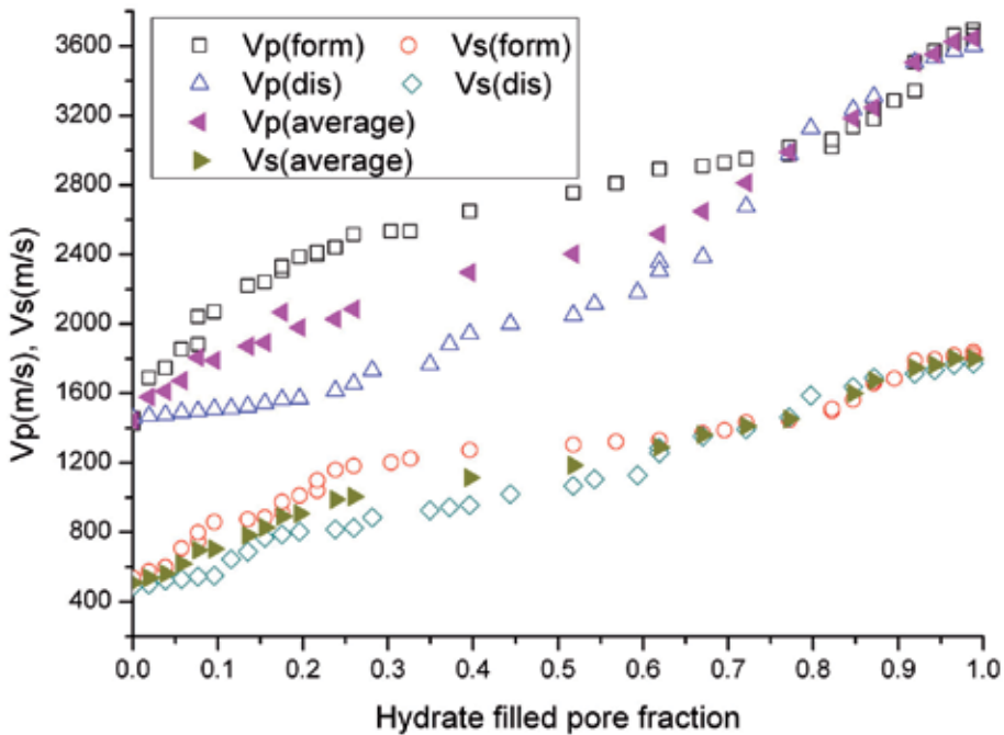
Fig. 19. For unconsolidated sediments: variation in V_p during hydrate formation ( V_p(\text{form}) ) and hydrate dissociation ( V_p(\text{dis}) ), V_s during hydrate formation ( V_s(\text{form}) ) and hydrate dissociation ( V_s(\text{dis}) ), the average V_p of V_p(\text{form}) and V_p(\text{dis}) , and the average V_s of V_s(\text{form}) and V_s(\text{dis}) .
