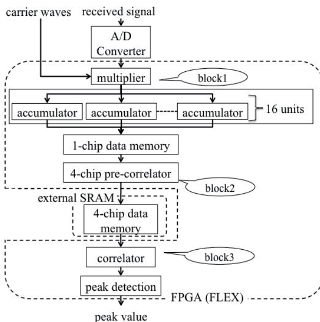
Fig. 6. Hardware layout on the real-time processor
