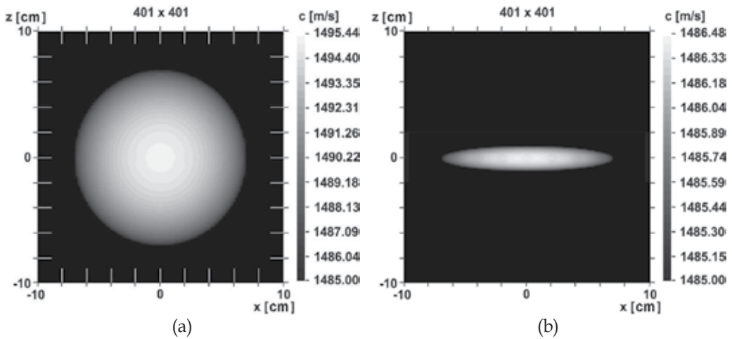
Fig. 7. Ultrasonic projection images of objects shown in Fig.6, obtained on the basis of computer-simulated measurements of mean values of ultrasonic wave propagation velocity: a) object C , b) object D
