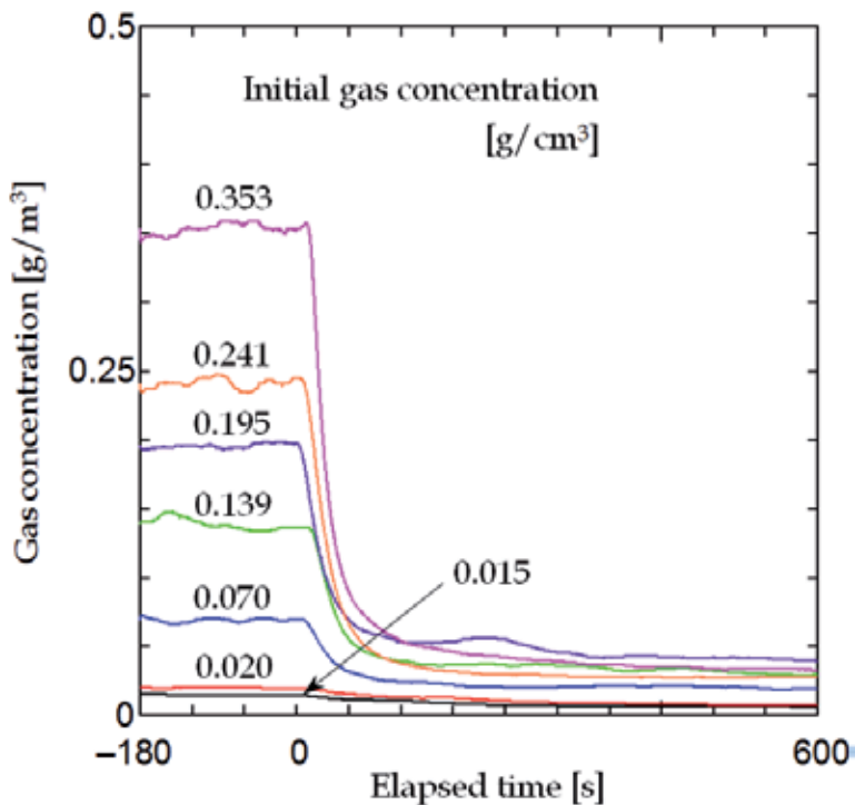
Fig. 21. Relationship between elapsed time and gas concentration. The input electric power is 50 W, the amount of water mist of large particles is 2.78 \text{ cm}^3/\text{s} , the amount of water mist of small particles is 0.27 \text{ cm}^3/\text{s} , and the driving frequency is 19.8 kHz.
