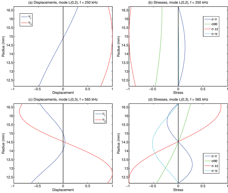
Fig. 8. Displacement and stress profiles for mode L(0,2) at f = 250 kHz (upper row), and mode L(0,3) at f = 565 kHz (bottom row), computed with pcwvform .
