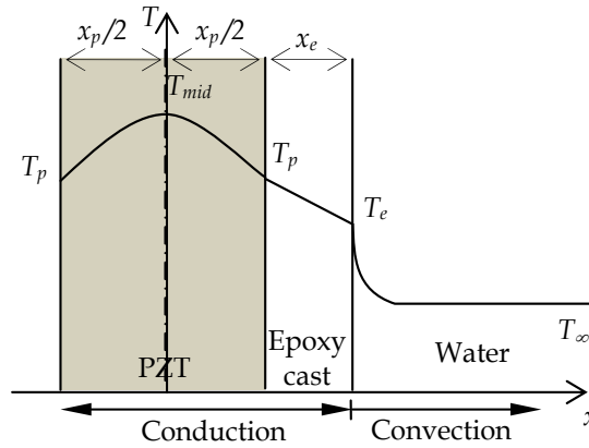
Fig. 16. A schematic diagram of the heat transfer profile. Acoustic transmission is generated by a transducer made from a PZT, through an epoxy cast layer into the water. Temperature gradient in each material outlines their relative heat transmission.
