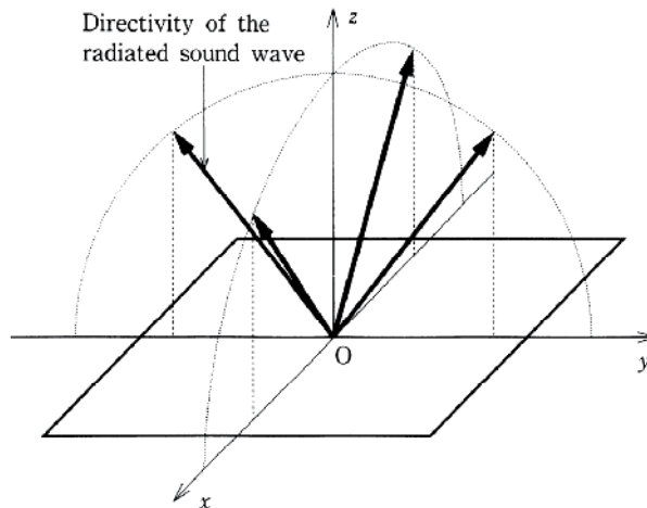
Fig. 10. Outline of the directivity.
