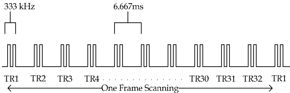
Fig. 7. The burst tones generated by microcontroller
