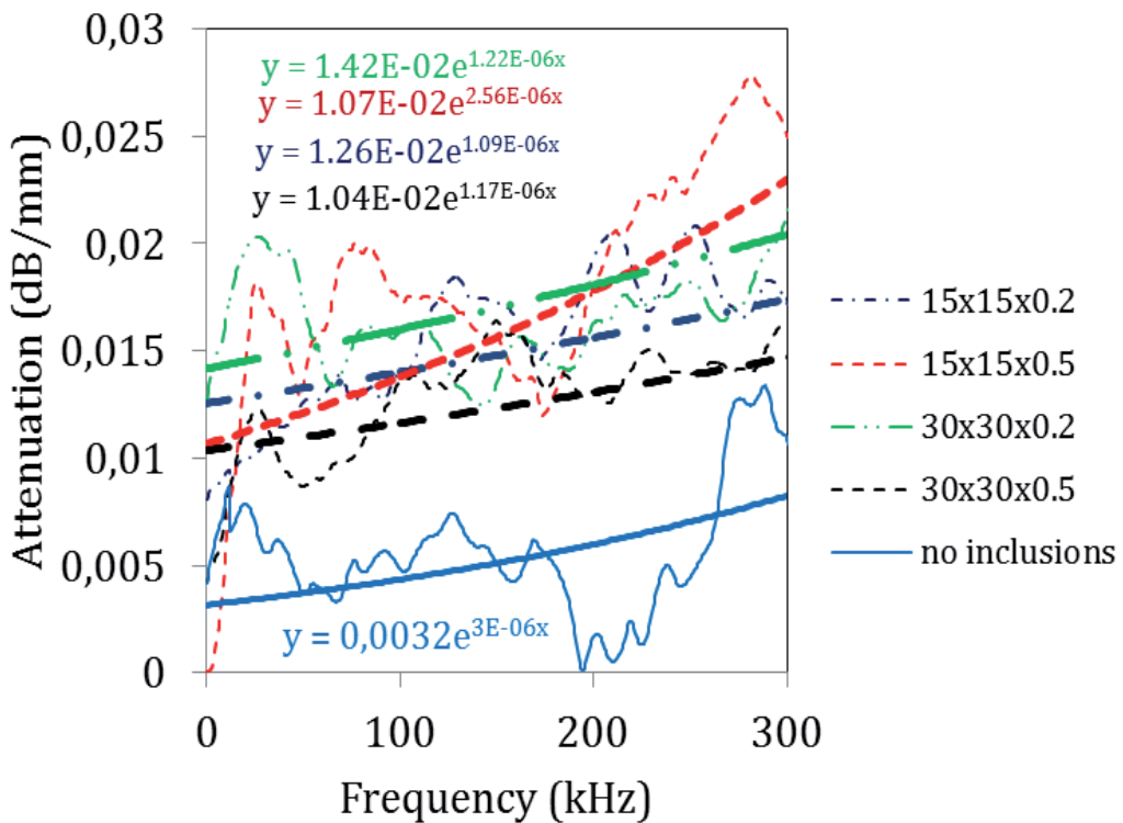
Fig. 7. Attenuation vs. frequency for mortar with different inclusion size and content 5%.
