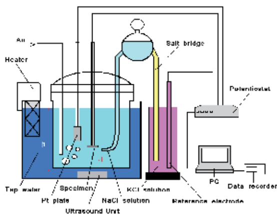
Fig. 11. Apparatus for polarization and applying ultrasound. Copyright 2009 Elsevier
