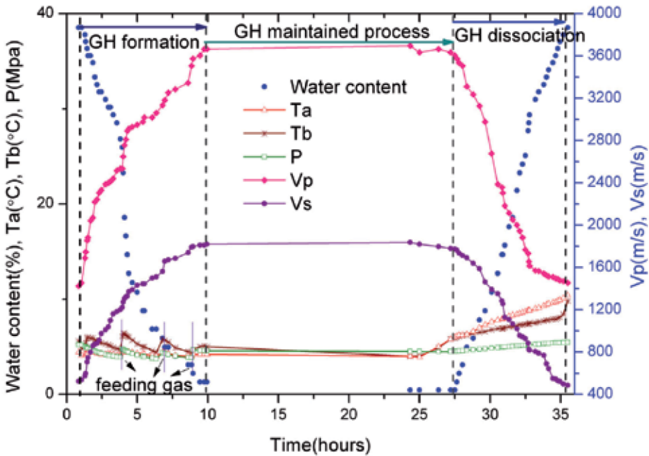
Fig. 18. Changes of parameters during gas hydrate formation and subsequent dissociation
