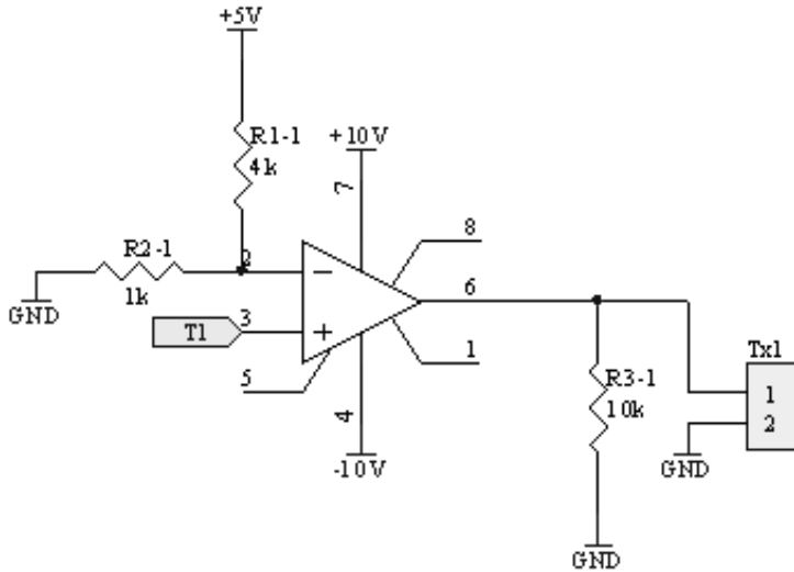
Fig. 8. The signal generator circuit
