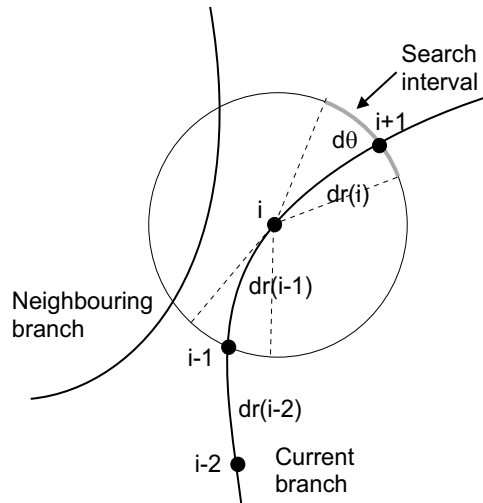
Fig. 4. Illustrates the root tracing algorithm used by PCDISP.
