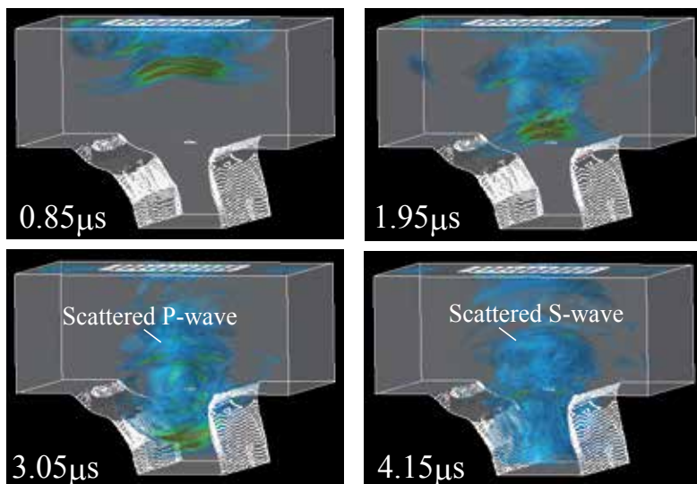
Fig. 19. Snapshots of ultrasonic wave propagation in welded T-joint (isosurface rendering).
