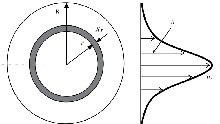
Fig. 4. An elemental disc sectioned laterally from the ultrasonic field. Axis of the transducer passes through the center of the concentric circles. The shaded annulus area, 2\pi r \delta r , is an elemental area through which flow discharges.
