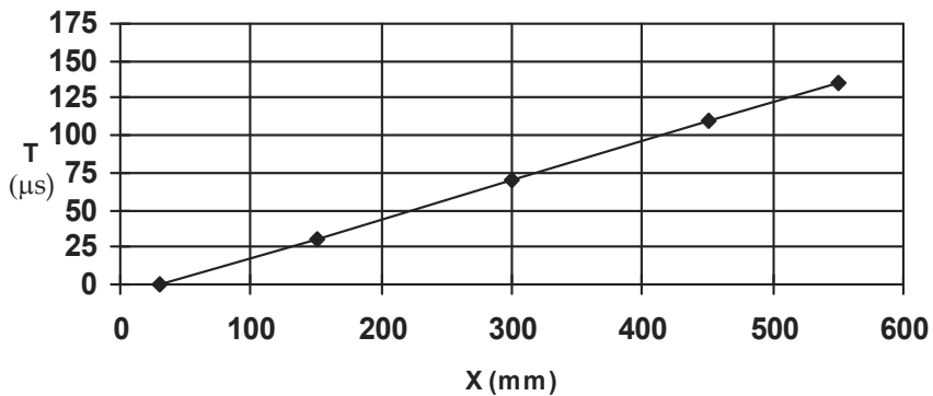
Fig. 4. Pulse velocity determination for homogenous concrete block
