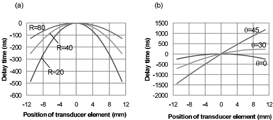
Fig. 6. Delay laws for the linear array transducer; number of element N=16 ; element pitch p = 1.475 mm; velocity c=5900 m/s (carbon steel): (a) normal beams and (b) angled beams with the focal length R=40 mm.
