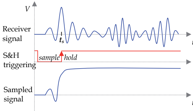
Fig. 10. The sample and hold operation
