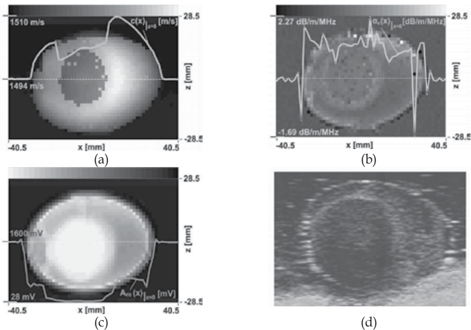
Fig. 10. Ultrasonic projection images of a hard-boiled hen's egg without shell, obtained from the following measurements of mean values: a) ultrasonic wave propagation velocity, b) derivative of the ultrasonic wave amplitude attenuation coefficient on frequency, c) ultrasonic wave pulse amplitude, in comparison to the ultrasonogram of the same egg (d)
