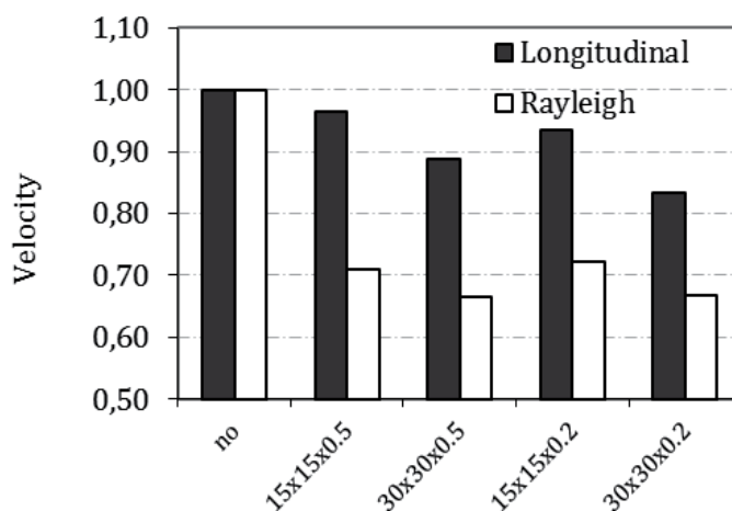
Fig. 3. Wave velocities for different inclusion sizes and constant content (5%).
