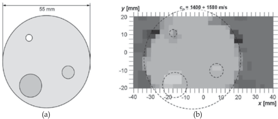
Fig. 22. Lateral projection of the agar phantom AC_Blue : structure (a), image of the distribution of projection values of sound velocity in grey scale (b)
