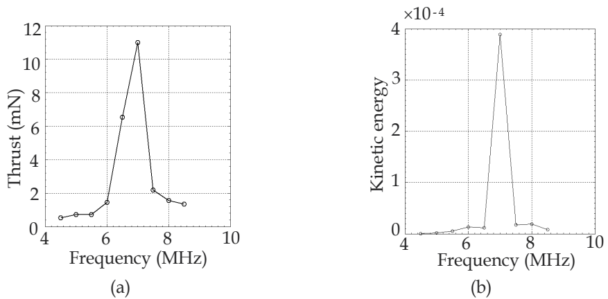
Fig. 9. (a) Measured thrust versus source frequency for sinusoidal waveforms supplied at 59V_{\text{rms}} . (b) Total kinetic energy versus source frequency, from DPIV. The sinusoidal signal is supplied at 54V_{\text{rms}} .
