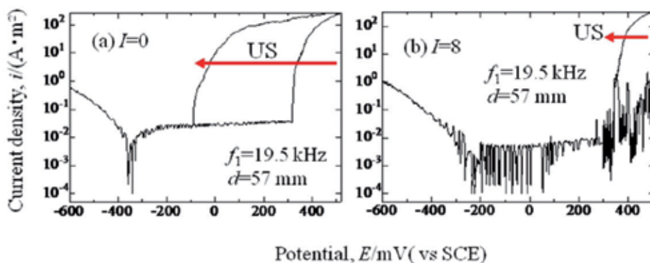
Fig. 23. Polarization curves with reversely sweeping of the potential at 500 mV, simultaneously without or with ultrasound with f_1 = 19.5 kHz at d = 57 mm and I = 8 .
