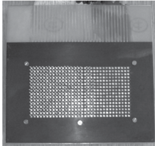
Fig. 15. Photo of the developed 512-element standard matrix for ultrasonic projection examinations
