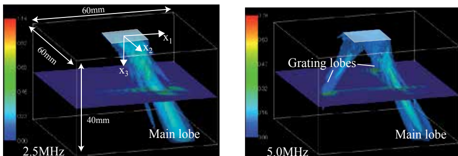
Fig. 11. 3-D wave fields radiated from a matrix array transducer with p_x=p_y=1.0\text{mm} and N \times M=16 \times 16=256 in the case of 2.5\text{MHz} (left side figure) and 5.0\text{MHz} (right side figure).
