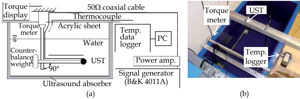
Fig. 17. (a) The experimental setup used to measure the UST temperature and thrust at the same time. Thrust is generated in the normal direction and out of the page. (b) A top view of the UST temperature measurement setup.
