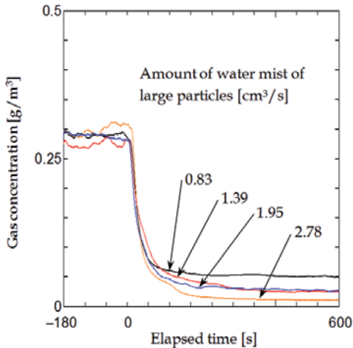
Fig. 19. Relationship between elapsed time and gas concentration. The input electric power is 50 W, the amount of water mist of small particles is 0.27 \text{ cm}^3/\text{s} , and the driving frequency is 19.8 kHz.
