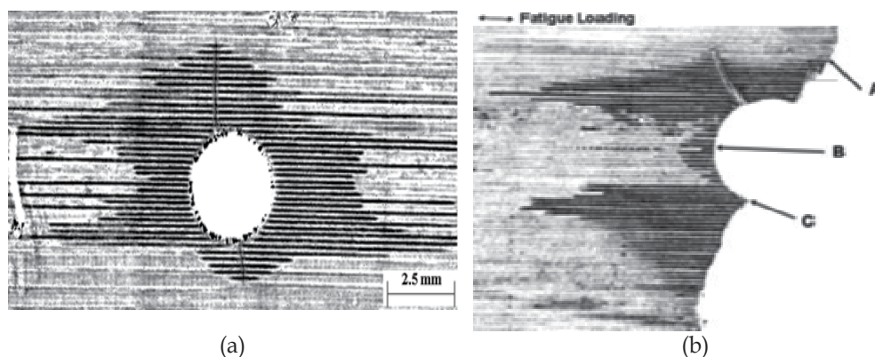
Fig. 10. Ultrasonic microscopy micrographs of (a) Ti-15Mo-3Nb-3Al-0.2Si/SCS-6 composite with [0/90]_S cross-ply lay-up of fibers subjected to 70 hours of isothermal ( 650^\circ\text{C} ) fatigue; (b) Ti-15Mo-3Nb-3Al-0.2Si/SCS-6 composite with unidirectional lay-up of fibers after 1.8 \times 10^5 cycles of isothermal ( 650^\circ\text{C} ) fatigue: A. Point of accelerated crack growth to failure. B. Interfacial degradation due to compressive stresses. C. Interfacial degradation due to tensile stresses.
