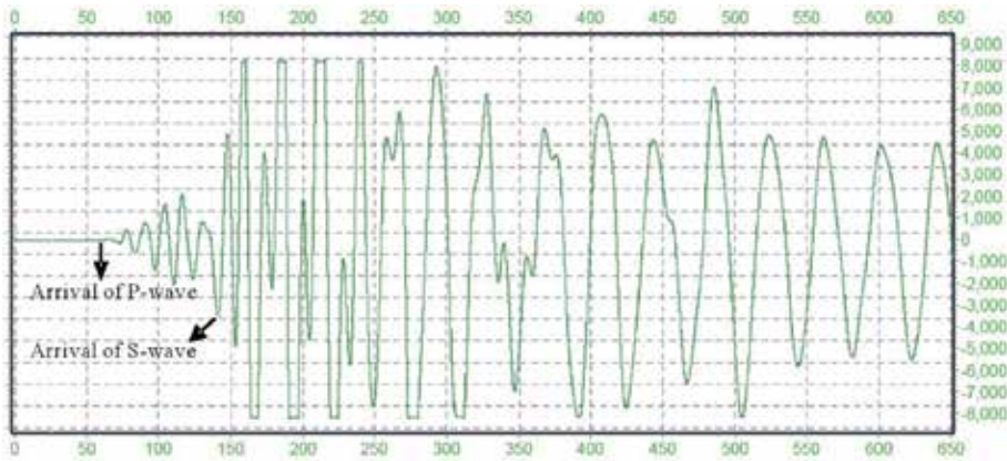
Fig. 13. Waveform of POM-I by bender element transducers
