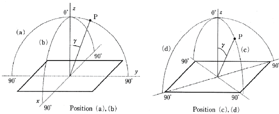
Fig. 8. Measurement positions of directivity.
