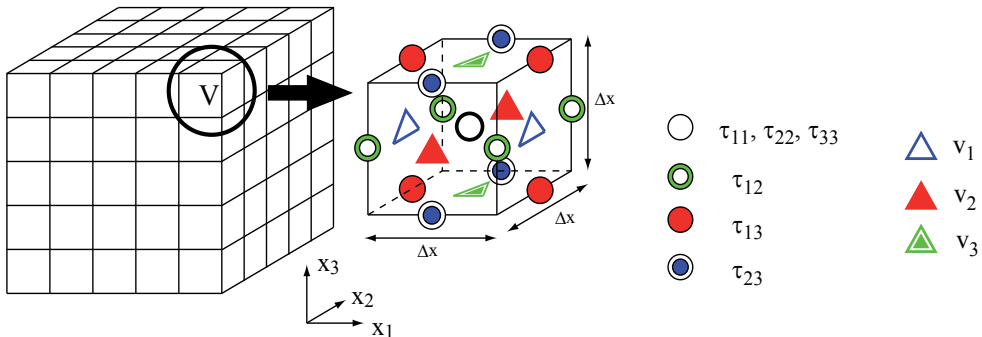
Fig. 15. Finite volume V and grid arrangement in the 3-D FIT.
