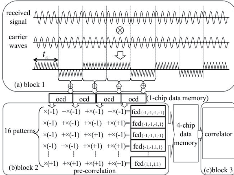
Fig. 7. Work flow of the real-time correlation
