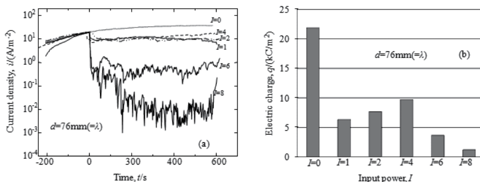
Fig. 12. Pitting current density (a) and accumulated electric charge (b) during the period of simultaneously holding potential and applying ultrasound with different input powers at a constant distance of 76 mm. Copyright 2009 Elsevier
