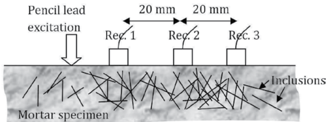
Fig. 1. The experimental setup.
