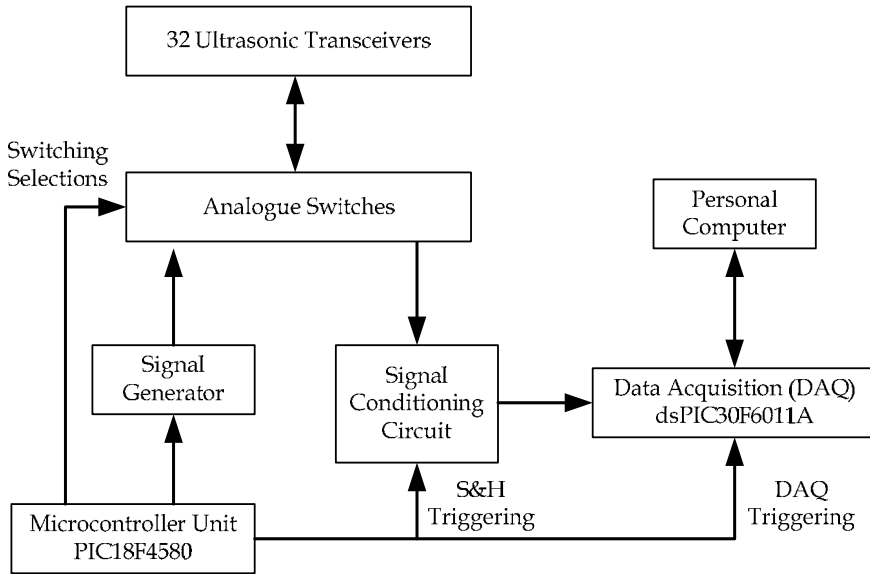
Fig. 6. The ultrasonic system block diagram
