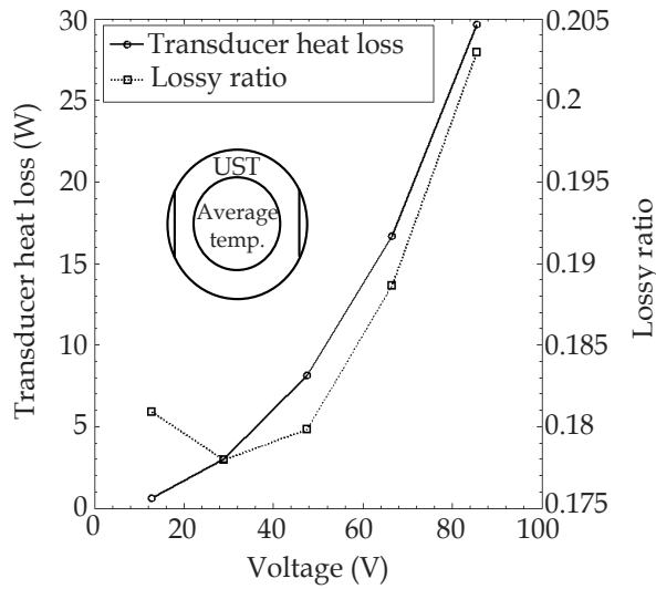
Fig. 20. Superfluous heat loss through the surface of the UST versus output voltage, E_{rms} . An increase in output voltage is generally associated with an increase in heat loss. The minimum of the lossy curve signifies the least heat loss in the system. Higher lossy ratio means more electrical energy is converted into heat losses instead of proportionately thrust.
