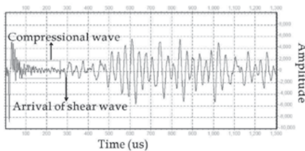
Fig. 8. Waveform of the hydrated unconsolidated sediments measured by bender elements
