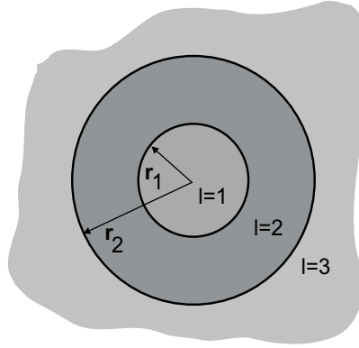
Fig. 1. Example of a three-layer cylindrical waveguide.
