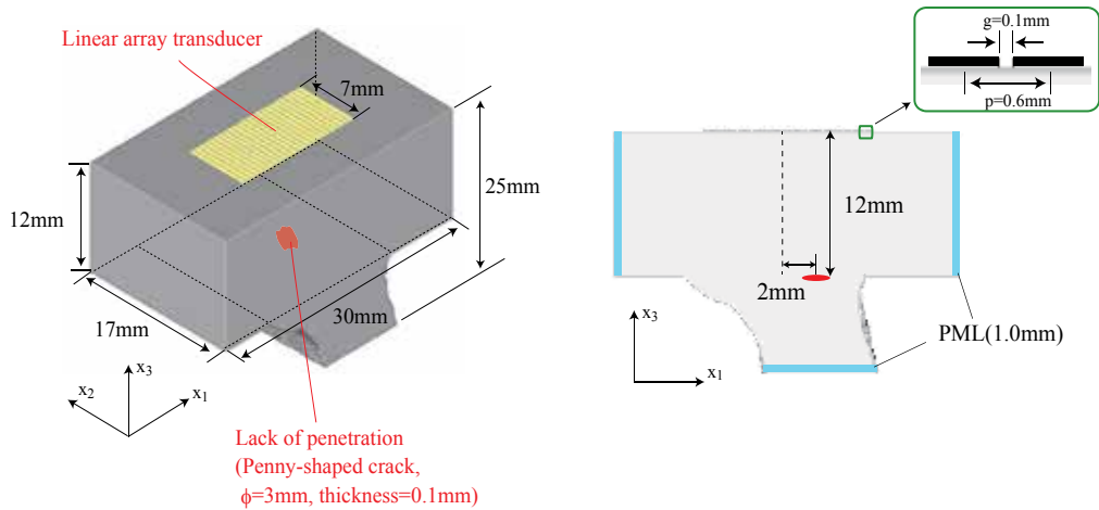
Fig. 18. Numerical model of the welded T-joint including an artificial defect (penny-shaped crack).
