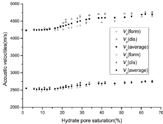
Fig. 7. Variation in V_p during hydrate formation ( V_p(\text{form}) ) and hydrate dissociation ( V_p(\text{dis}) ), V_s during hydrate formation ( V_s(\text{form}) ) and hydrate dissociation ( V_s(\text{dis}) ), the average V_p of V_p(\text{form}) and V_p(\text{dis}) , and the average V_s of V_s(\text{form}) and V_s(\text{dis}) .
