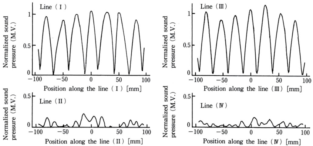
Fig. 6. Distributions of the sound pressure near the vibrating plate. Lines (I) - (IV) are indicated in Fig.4.
