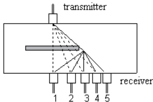
Fig. 8. The cause of time delay of pulses.
