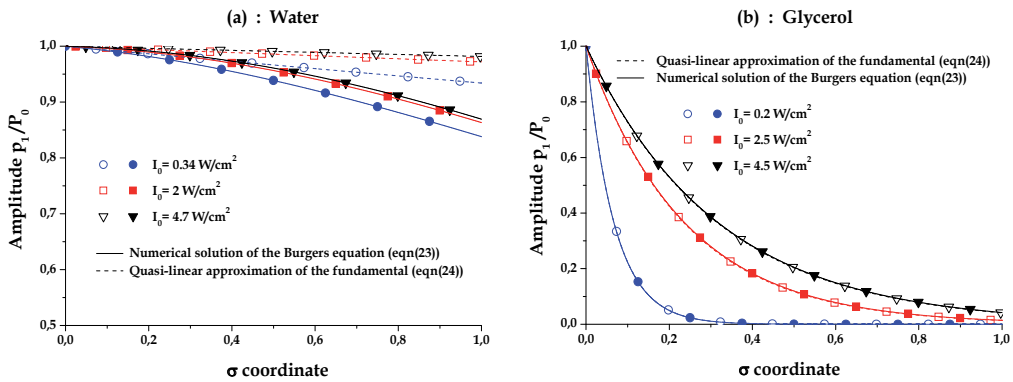
Fig. 1. Pressure amplitude p_1/P_0 versus the \sigma coordinate.
