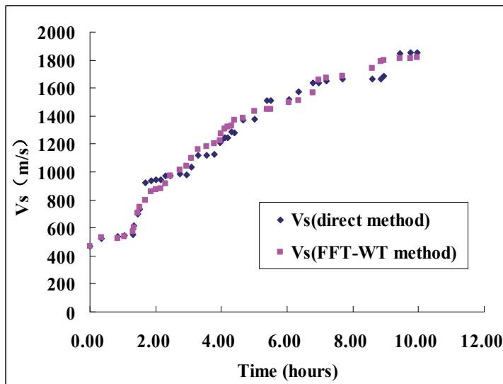
Fig. 17. Comparison of V_s determined by the direct method and the FFT-WT method
