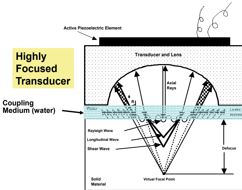
Fig. 8. Principle of ultrasonic microscopy.
