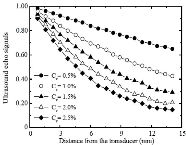
Fig. 2. Signal attenuation function of the distance from the ultrasonic transducer and the volumetric concentration of particle, d_p = 0.7 mm
