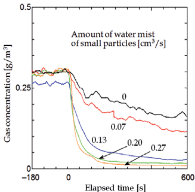
Fig. 17. Relationship between elapsed time and gas concentration. The input electric power is 50 W, the amount of water mist of large particles is 2.78 cm 3 /s, and the driving frequency is 19.8 kHz.
