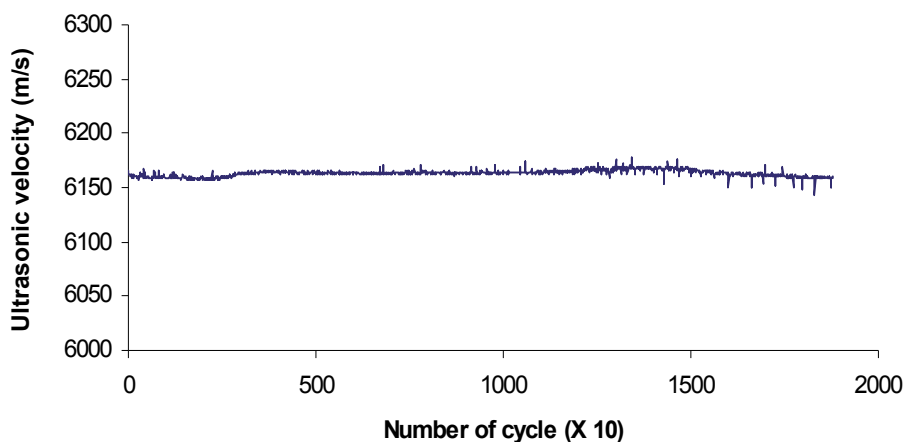
Fig. 15. Variation of longitudinal wave velocity with fatigue life
