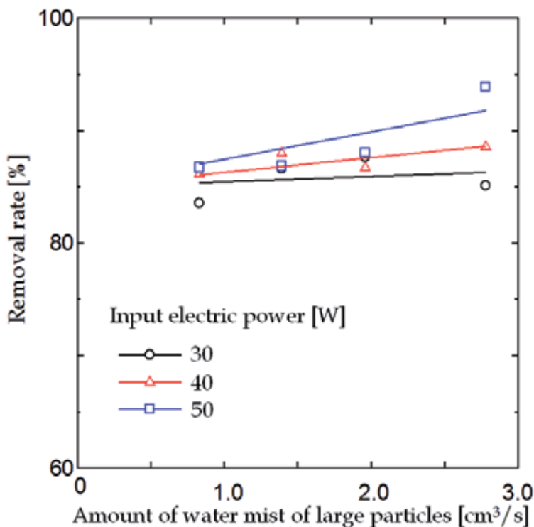
Fig. 20. Relationship between amount of water mist of large particles and removal rate. The Amount of water mist of small particles is 0.27 \text{ cm}^3/\text{s} , and the driving frequency is 19.8 kHz.
