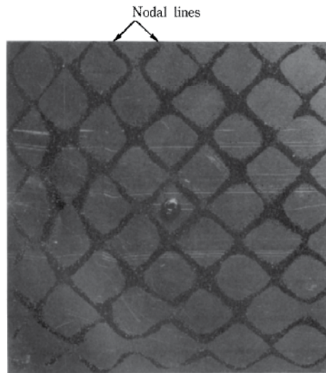
Fig. 3. Chladni sand figure showing nodal pattern of the square vibrating plate.
