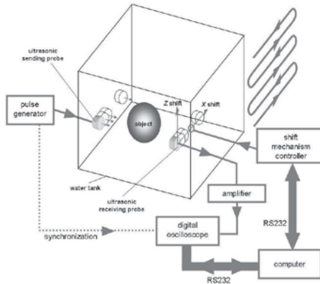
Fig. 9. Block scheme of the measurement setup for biological media structure imaging by means of the ultrasonic projection method using one-element ultrasonic probes
