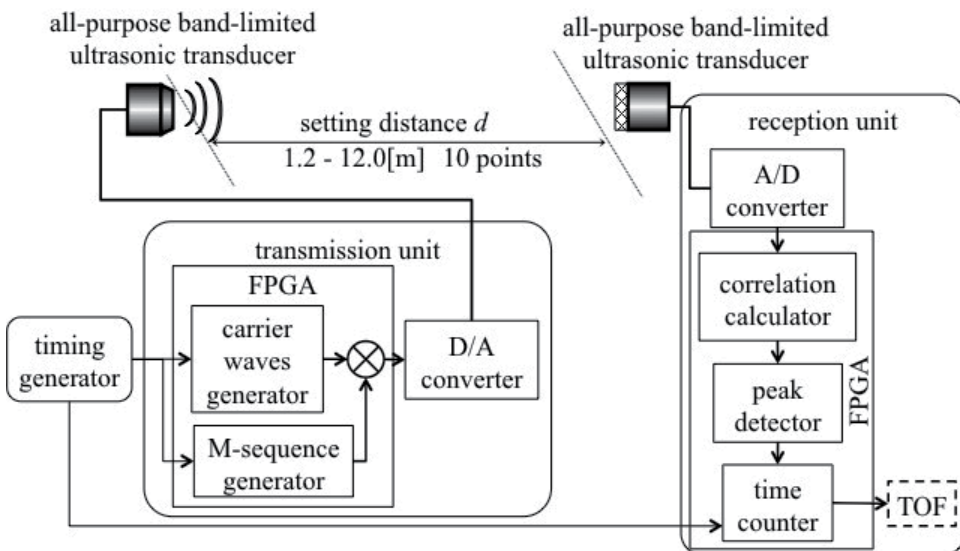
Fig. 3. System architecture for TOF measurement using SS ultrasonic signals
