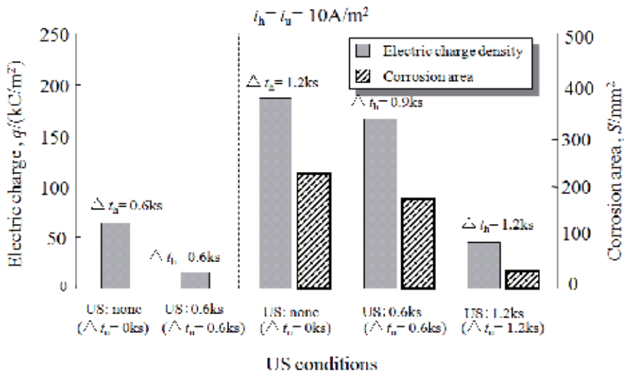
Fig. 8. Electric charge during the holding of potential without and with ultrasound ( i_h = i_u = 10 \text{ A/m}^2 ). Copyright 2008 The Japan Institute of Metals
