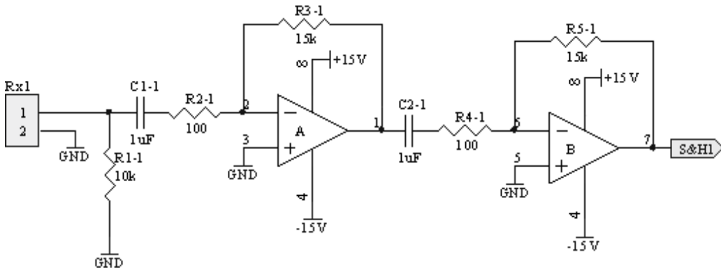
Fig. 9. The signal conditioning circuit
