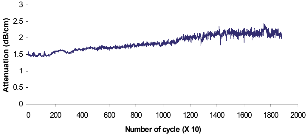
Fig. 16. Variation of ultrasonic attenuation with fatigue life
