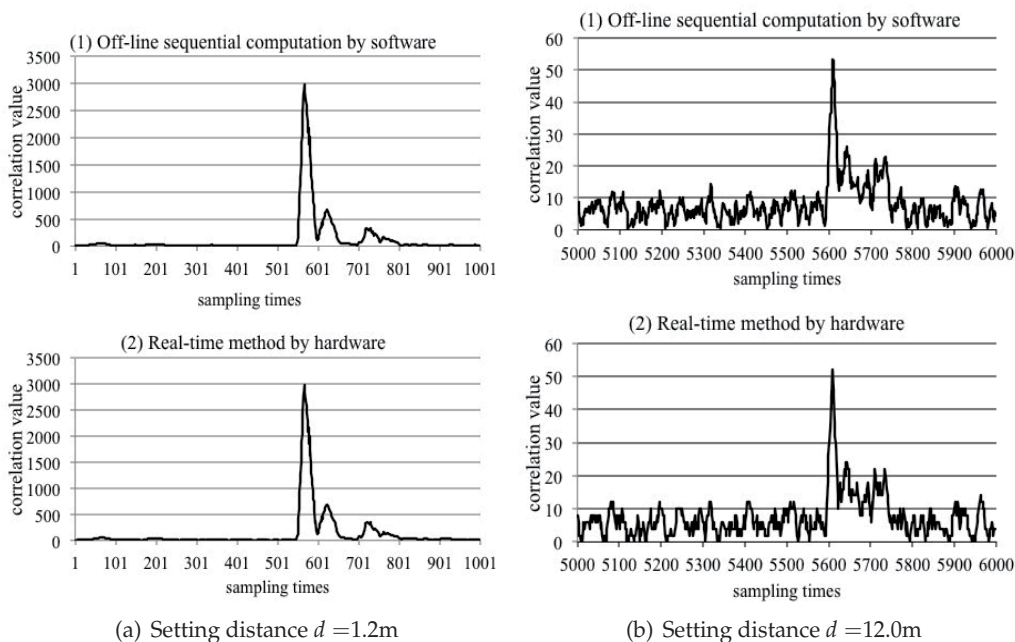
Fig. 10. Difference between off-line sequential computation using software and the real-time method using the SPCM hardware
