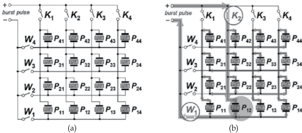
Fig. 16. Diagram of connections of transducers in a passive matrix (a) and a phenomenon of crosstalk formation (b)
