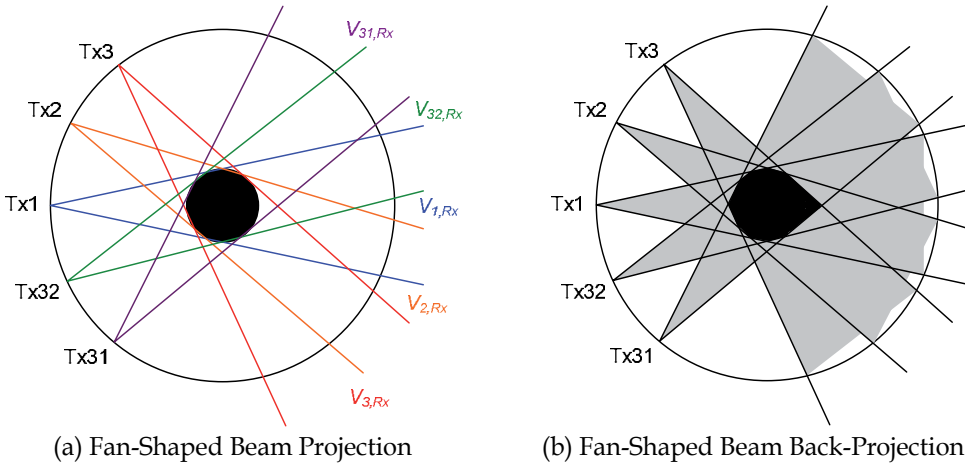
Fig. 14. The fan-shaped beam back-projection
