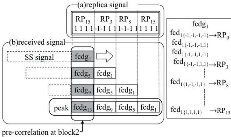
Fig. 9. Selection of 4-chip data using replica signals in block 3
