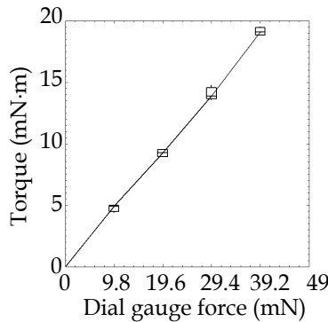
Fig. 7. Calibration of the test rig. Each of the four points shown is an average of four separate force applications using a sensitive dial gauge.
