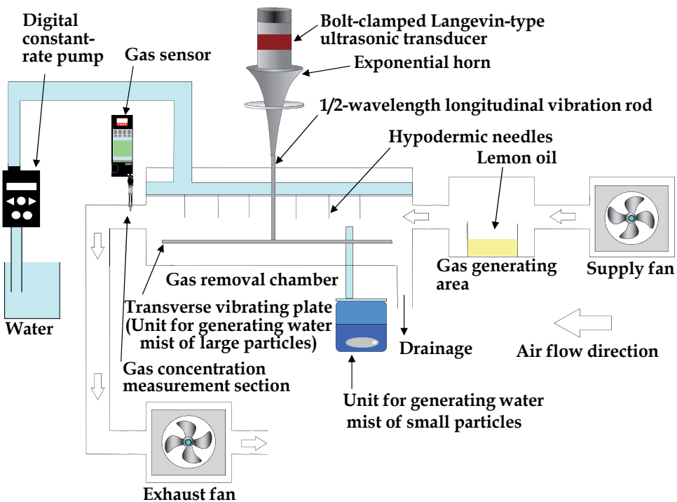
Fig. 12. Schematic of gas removal apparatus.
