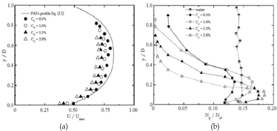
Fig. 8. Effect of the particle volumetric concentration on: a) the velocity profiles; b) the local concentration profiles for d_p=0.27 mm and Re=44600 .
