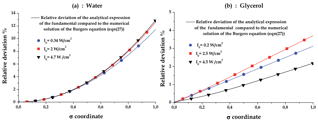
Fig. 3. Relative deviation of the analytical expression of the fundamental compared to the numerical solution of the Burgers’ equation versus the \sigma coordinate.
