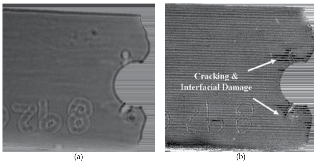
Fig. 9. The role of coupling medium in ultrasonic microscopy; using (a) water as coupling medium for imaging damage in Ti-24Al-11Nb/SCS-6 composite subjected to TMF, (b) methanol as coupling medium for imaging the same specimen.
