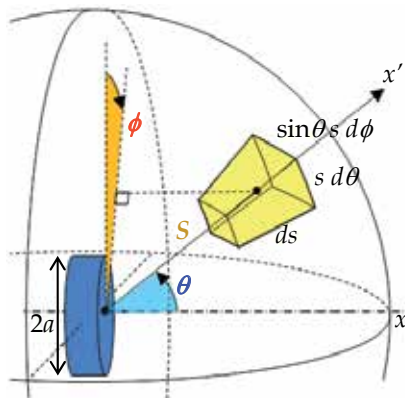
Fig. 2. An elemental control volume in the far-field; the elevation angle, azimuth angle and distance from the center of transducer are \theta , \phi , and s respectively.
