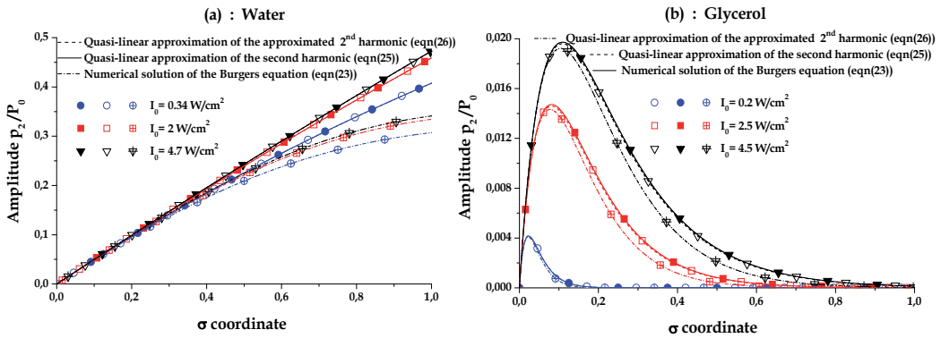
Fig. 2. Pressure amplitude p_2/P_0 versus the \sigma coordinate.
