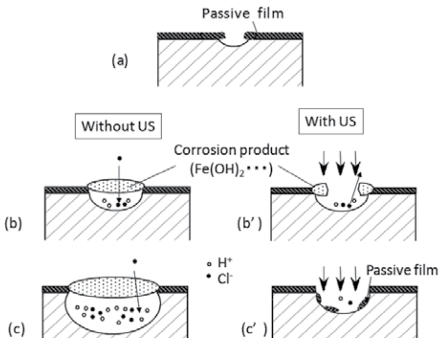
Fig. 4. Decrease in growth of corrosion pits by ultrasound. Copyright 2007 The Japan Institute of Metals
