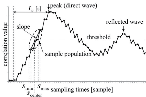
Fig. 5. A method for peak detection
