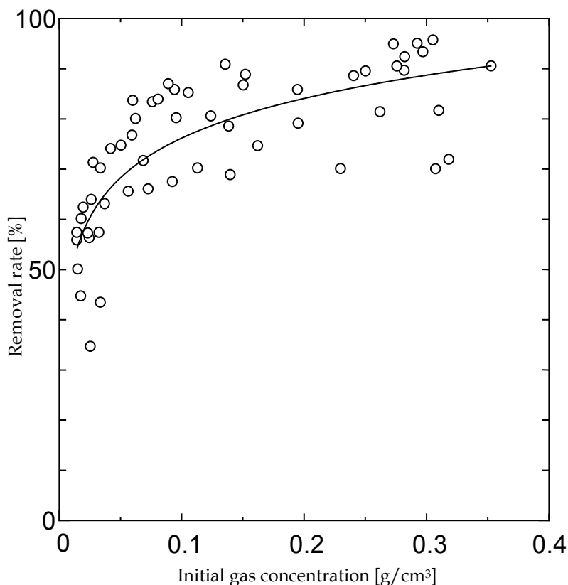
Fig. 22. Relationship between initial gas concentration and removal rate. The input electric power is 50 W, the amount of water mist of large particles is 2.78 cm 3 /s, the amount of water mist of small particles is 0.27 cm 3 /s, and driving frequency is 19.8 kHz.
