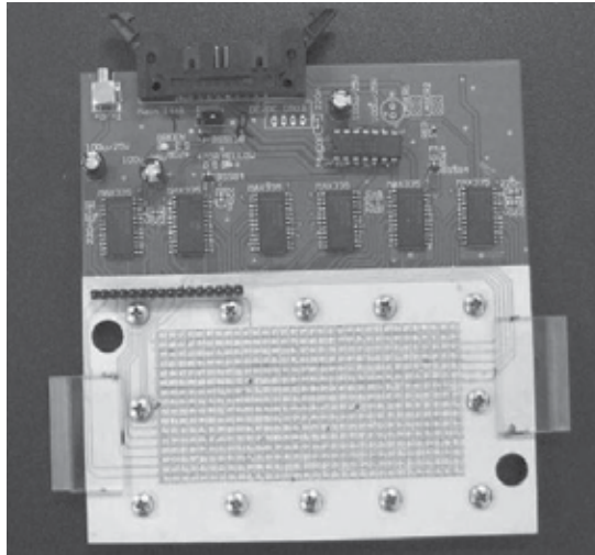
Fig. 17. The view of the developed 512-element ultrasonic passive matrix
