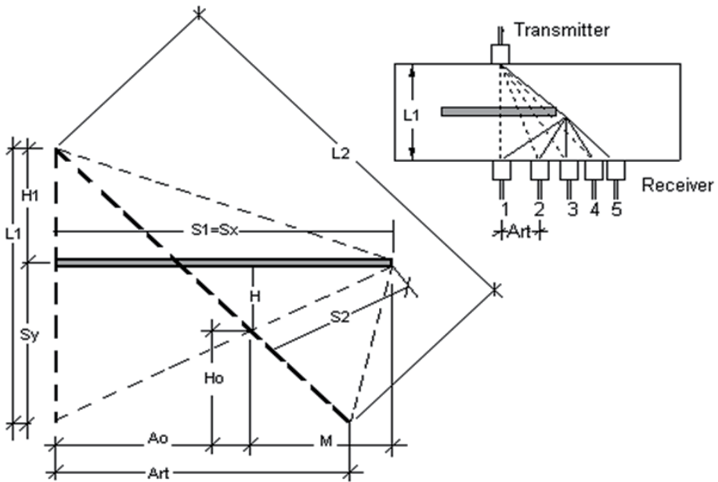
Fig. 13. Pulses travel paths for both receiver positions.
