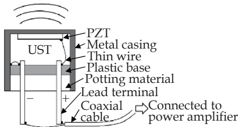
Fig. 5. Construction of the UST (adapted from Murata Manufacturing Co. Ltd).
