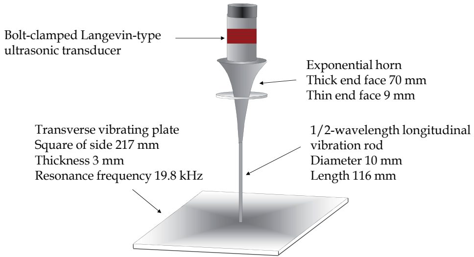
Fig. 13. Schematic of ultrasonic transducer.
