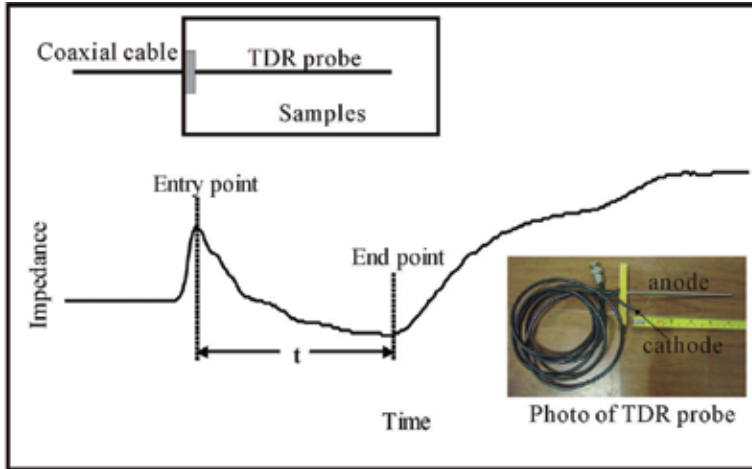
Fig. 3. TDR waveform of low-salty sediments with traditional TDR probe
