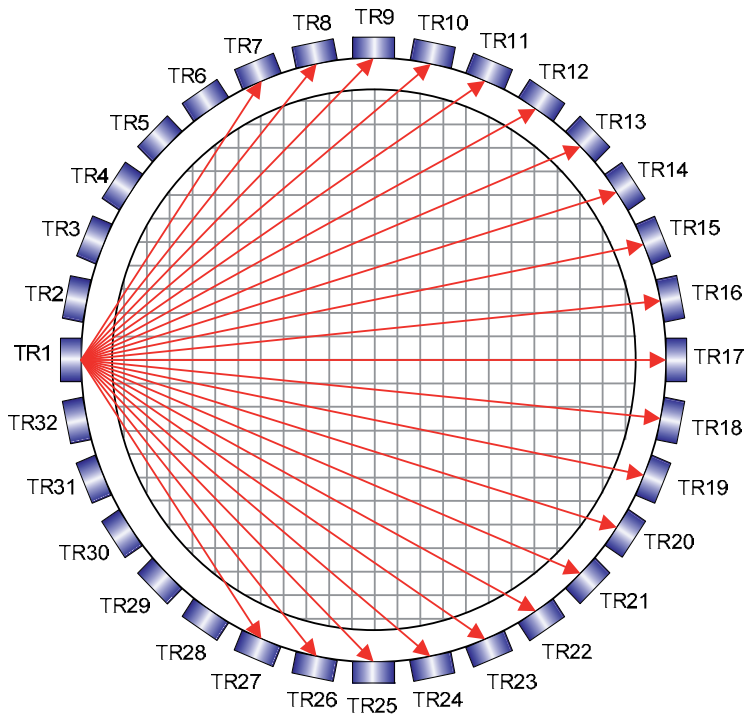
Fig. 3. Ultrasonic transceiver sensor array
