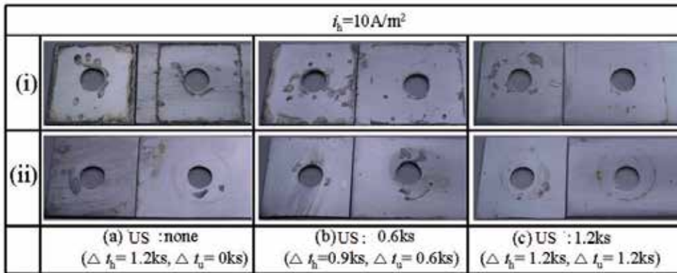
Fig. 7. Specimen surfaces after polarization without and with ultrasound ( i_h = i_u = 10 \text{ A/m}^2 ). Copyright 2008 The Japan Institute of Metals
