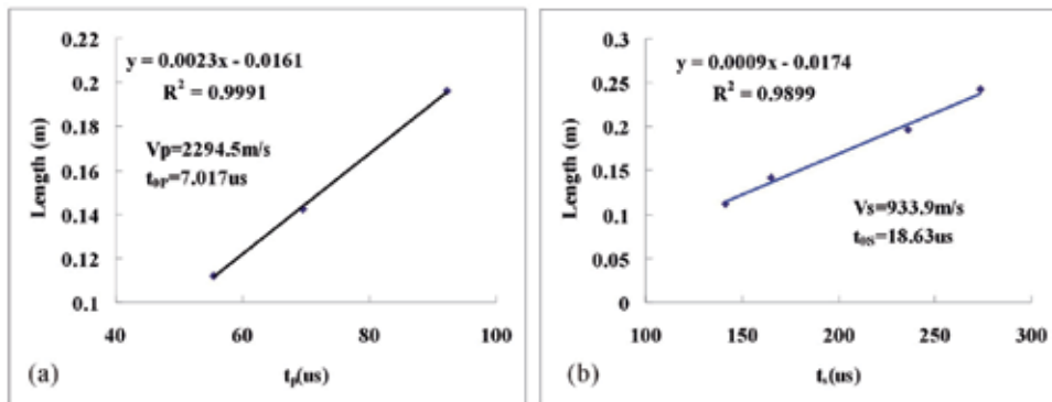
Fig. 14. Calibrating results of the new bender elements
