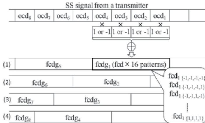
Fig. 8. Production of 4-chip data from 1-chip data
