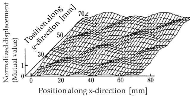
Fig. 5. Distribution of the vibration displacement.
