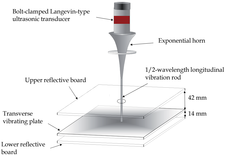
Fig. 14. Positions of reflective boards.
