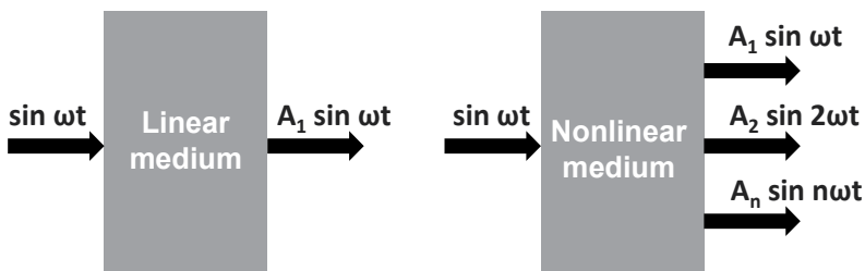
Fig. 11. Linear and nonlinear wave propagation in solid materials.
