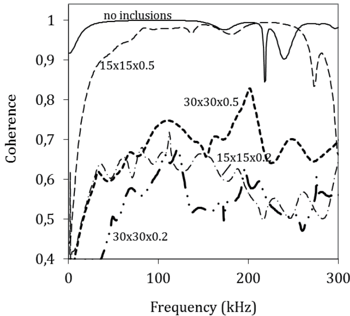
Fig. 5. Coherence function for different size of inclusions and content 5% by vol.
