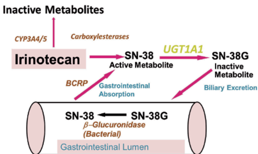
Fig. 2. Irinotecan Metabolism
