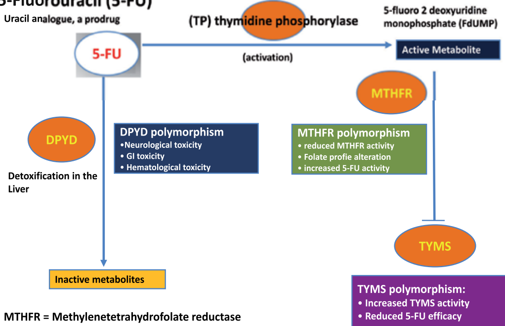
Fig. 1. 5-Fluorouracil metabolism
