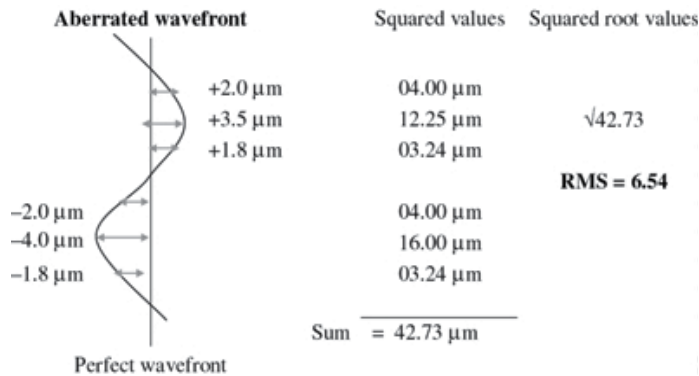
Fig. 7. Graphical representation of root mean squared wavefront error (9).
