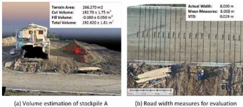
Figure 3. GoogleEarthWork features demonstration: (a) earth volume survey from automated 3D reconstruction and (b) relative positioning accuracy evaluation.
