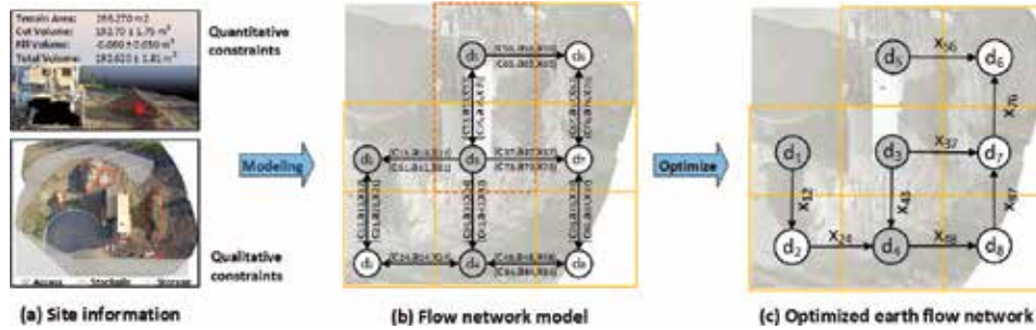
Figure 6. Flow network model for earthwork optimization and state presentation in GoogleEarthWork. (a) Typical constraints on a construction site, (b) quantitative constraints and qualitative constraints modeled as attributes and network structure, respectively, and (c) optimized earth flow network used to represent the state of the system.
