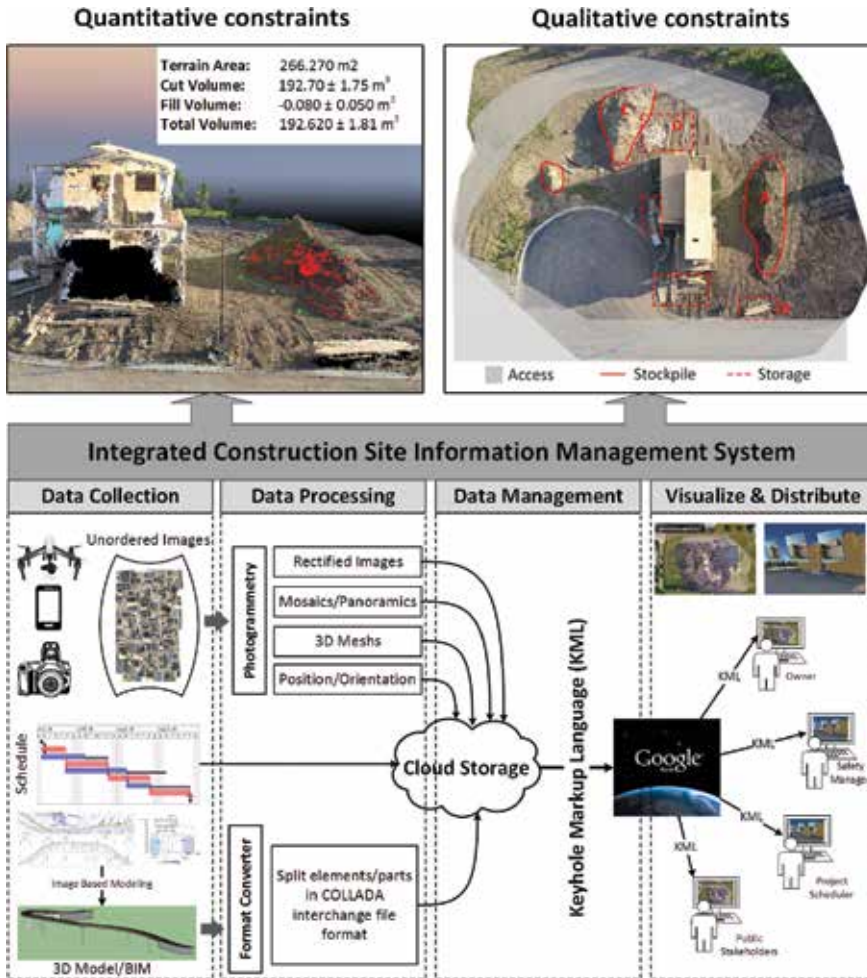
Figure 1. GoogleEarth Work for earthwork construction planning.
