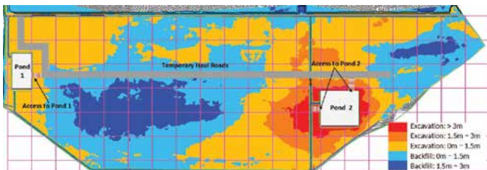
Figure 8. Rough grading construction site: drawing and layouts.
