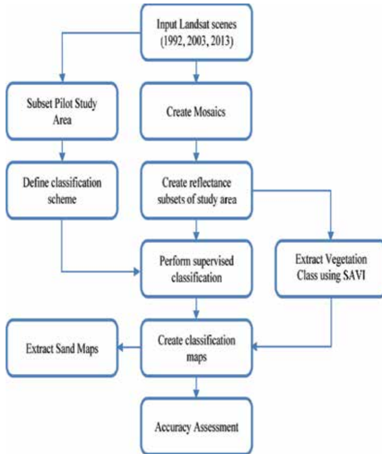
Figure 6. Sand mapping methodology flowchart.
