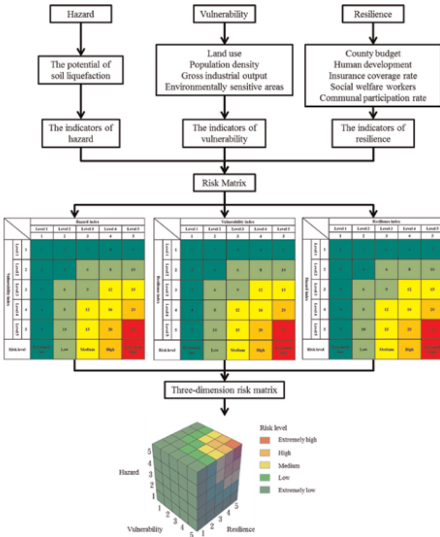
Figure 8. Procedure of the risk level analysis.
