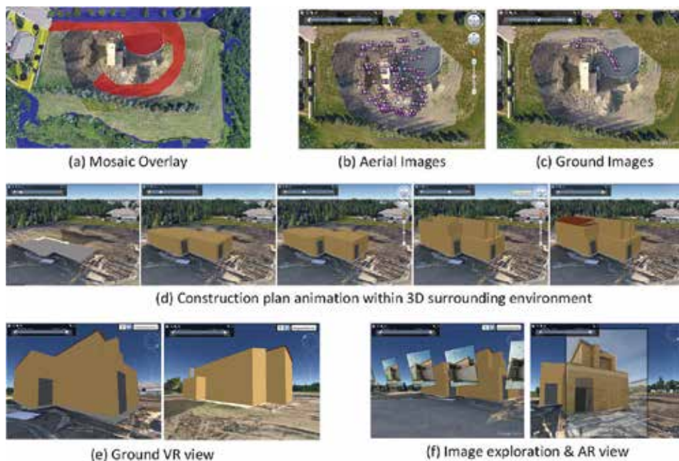
Figure 2. Integrated project data management and visualization.
