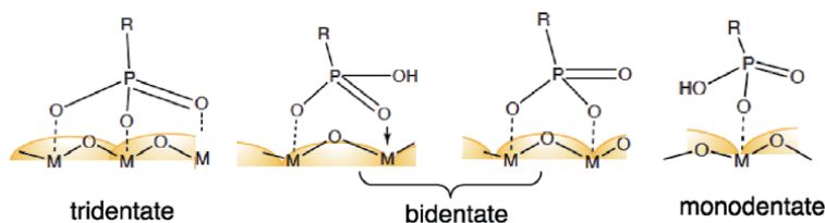
Figure 9. Proposed surface binding modes of phosphonic acid groups on a metal oxide ( MO_x ) surface ( M = \text{metal} ) [30].
