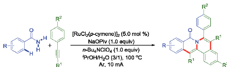
Figure 38. Ruthenium(II)-catalyzed synthesis of polycyclic Isoquinolinones.
