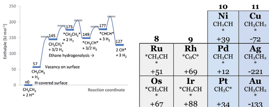
Figure 4. Calculated reaction enthalpies for the elementary steps in the hydrogenolysis of ethane on a Ru(001) surface (593 K, left) and intermediates with the lowest activation free-energy barrier relative to ^*CH-CH^* bond activation (right) [49]. Energies are relative to a surface covered with chemisorbed hydrogen ( H^* ); * denotes coordination to the ruthenium surface.
