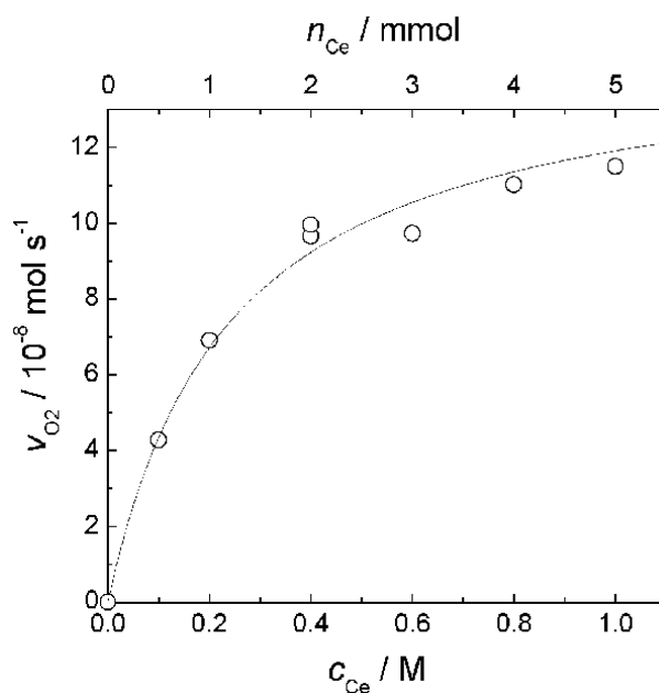
Figure 13. Plots of v_{O_2} versus the Ce^{IV} concentration ( c_{Ce}/\text{M} ) in chemical water oxidation experiments using 0.2 mM 4EtO (5.0 ml water) at 25^\circ\text{C} . the solid line is the simulated curve based on a Michaelis–Menten-like kinetic equation. (reproduced with permission from ref. [39]. Copyright 2011 the Royal Society of Chemistry).
