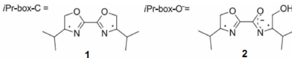
Figure 7. Oxazoline ligands [31].
