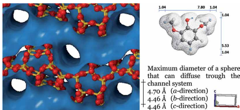
Figure 11. Comparison of the characteristic dimensions of syringol (top right) and the three-dimensional MFI pore system of zeolite ZSM-5, here viewed down the b -direction (left; not to scale; red, oxygen atoms; orange, silicon atoms), and maximum diameter of a sphere that can diffuse through the channel system (bottom right).
