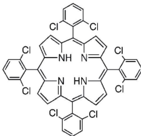
Figure 2. Meso-Tetrakis(2,6-dichlorophenyl)porphyrin (TDCPP).
