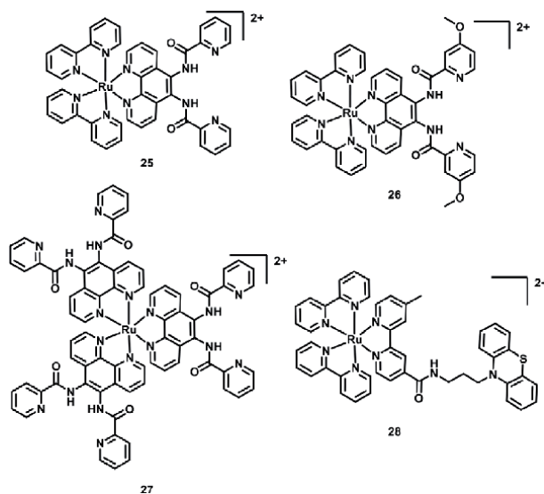
Figure 10. Chemical drawing of probes 25–28 .
