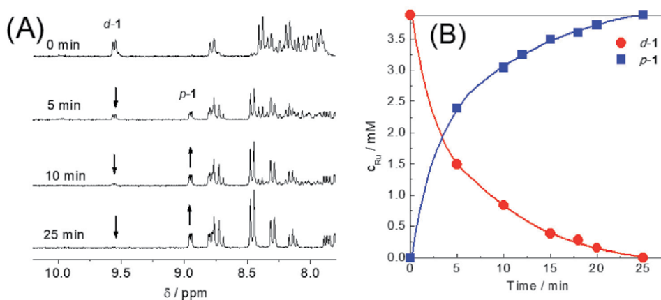
Figure 2. (A) Time course of 1 H NMR spectral changes during the photoisomerization of d -1 in D 2 O with 180 \text{ mW cm}^{-2} visible light irradiation ( \lambda > 420 \text{ nm} ). (B) Kinetic profiles of d -1 (red circle) and of p -1 (blue square). (Reproduced with permission of American Chemical Society from ref. [21]).
