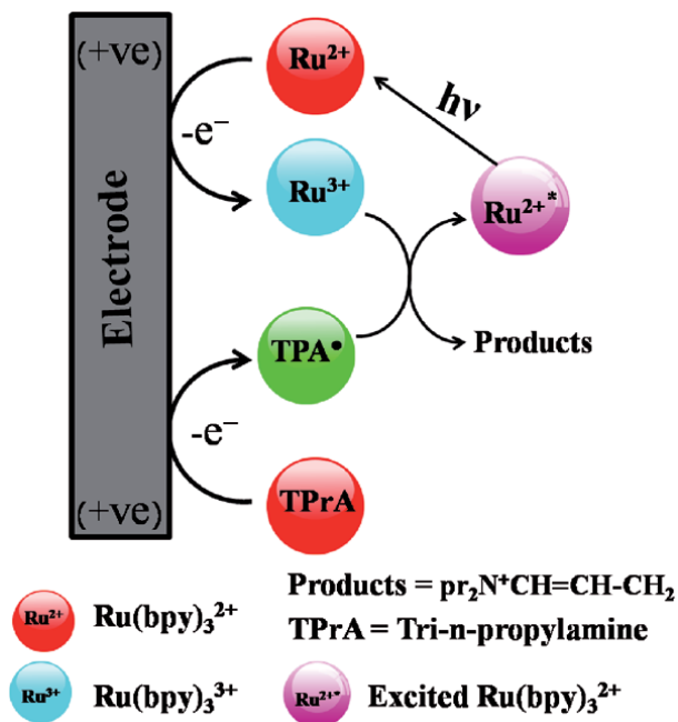
Figure 2. The schematic illustration of oxidative-reduction mechanism of Ru(bpy)_3^{2+} molecule and TPrA.
