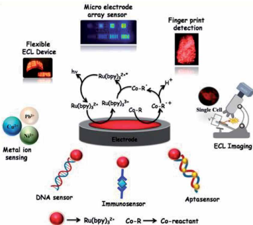
Figure 4. Schematic illustration of ECL based applications using \text{Ru}(\text{bpy})_3^{2+} as a active probe.
