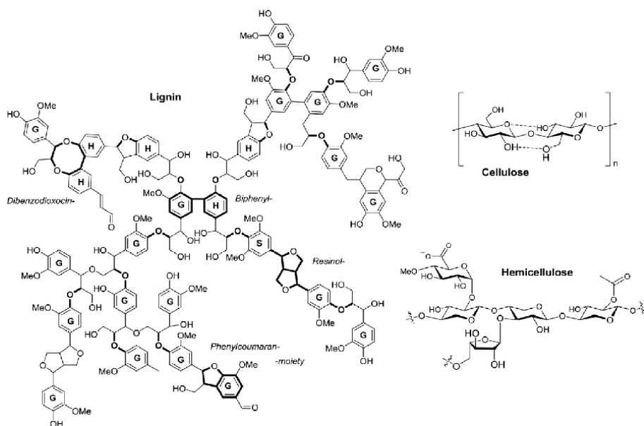
Figure 8. Chemical structure of important biomass fractions, lignin (left), cellulose with 1,4-glycosidic linkages and selected hydrogen bonds (right, top) and the common molecular motif of hemicellulose (right, bottom). For the structure of lignin, the characteristic aromatic p -hydroxyphenyl ( H ), guaiacyl ( G ) and syringyl ( S ) moieties as well as aromatic ether linkages (- O -), dibenzodioxocin, biphenyl, resinol, and phenylcoumaran linkages [109, 127] were marked.
