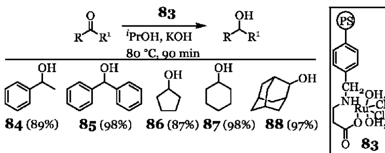
Figure 21. Heterogeneous TH of ketone.
