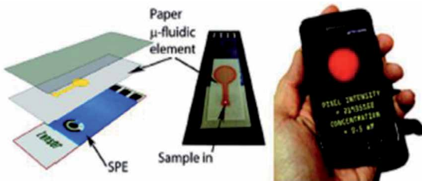
Figure 13. Schematic diagram of a paper-based microfluidic ECL sensor. Using inkjet-printed paper fluidic substrates and screen-printed electrodes, this ECL sensor can be read with mobile phone cameras. Copyright © 2011, American Chemical Society.
