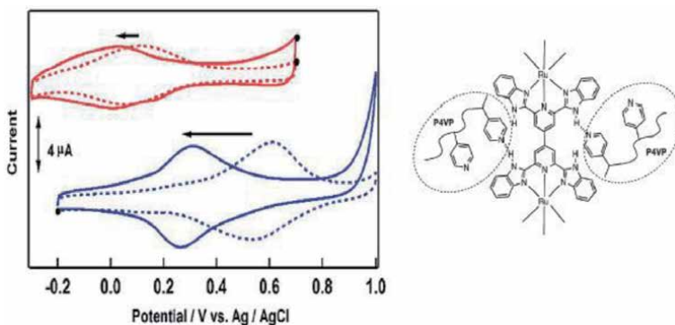
Figure 28. Cyclic voltammograms of ITO|(16) 3 /P4VP (blue solid lines) and ITO|(17) 3 /P4VP films (red solid lines), together with those of ITO|(16) 3 (blue dotted lines) and ITO|(17) 3 films (red dotted lines), in 0.1 M NaClO 4 aqueous solution, as well as a schematic illustration of the hydrogen-bonding interactions between the Ru complex 16 and the P4VP polymer [83].
