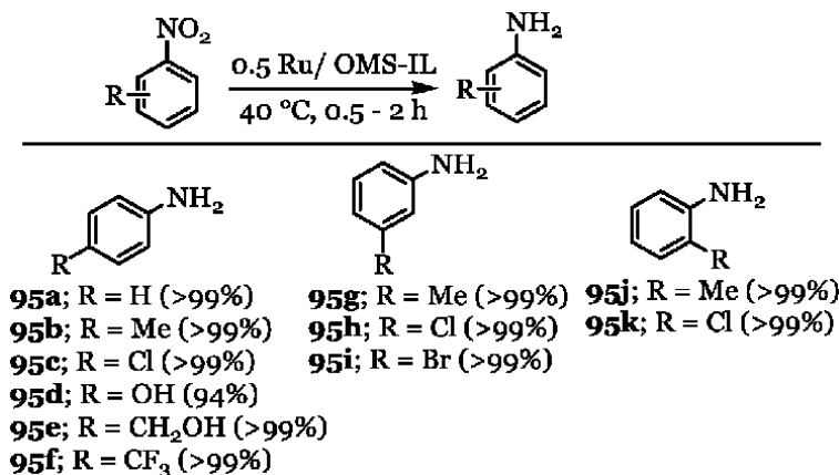
Figure 25. Reduction of nitro arenes via ruthenium-catalyzed TH.
