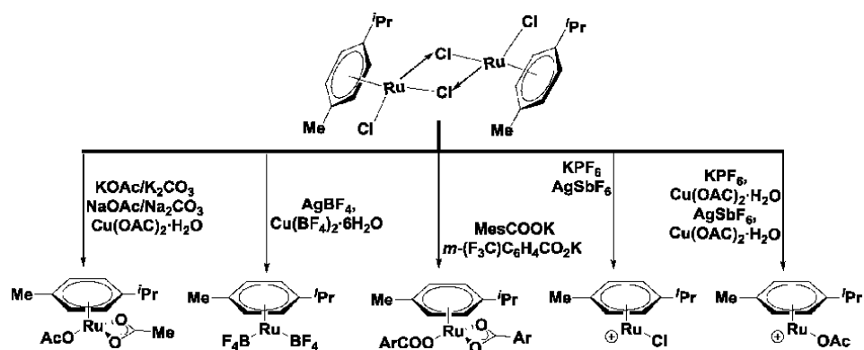
Figure 1. In Situ generated active Ru(II) complex.
