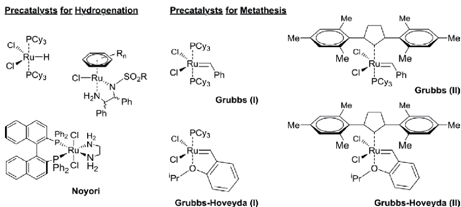
Figure 5. Examples of molecular ruthenium complexes that are used in homogeneously catalyzed hydrogenation and metathesis reactions.
