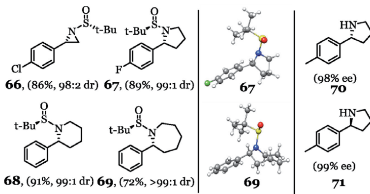
Figure 17. Asymmetric transfer hydrogenation examples of selected N -protected aziridine ( 66 ), pyrrolidine ( 67 ), piperidines ( 68 ) and azepane ( 69 ) and X-ray crystal structures of 67 , 69 (from ref. [21]) as well as structure of free pyrrolidines ( 70 , 71 ).
