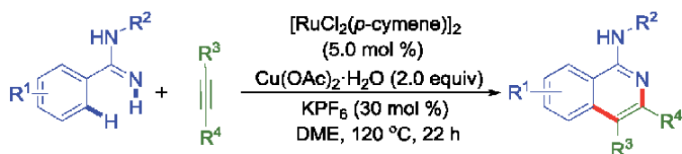
Figure 27. Ru(II)-Catalyzed synthesis of 1-Aminoisoquinolines derivatives.
