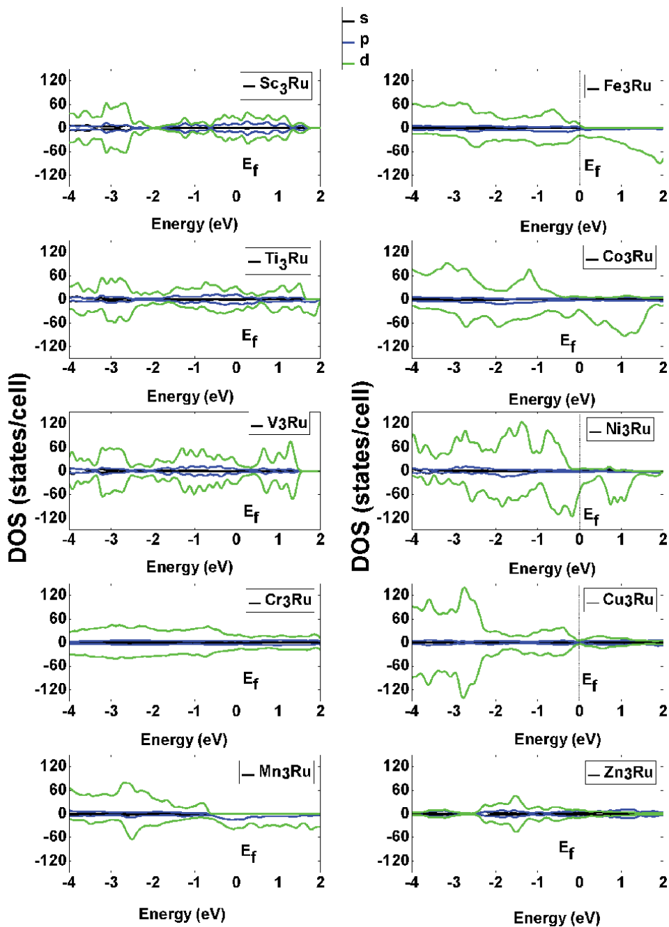
Figure 5. Partial density of states of binary X_3Ru ( X = Sc, Ti, V, Cr, Mn, Fe, Co, Ni, Cu and Zn ). The Fermi energy is taken as zero energy, indicated with the vertical dotted line.
