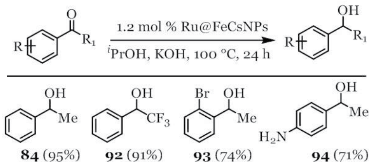
Figure 23. Ru@FeCSNPs catalyzed TH of acetophenone.
