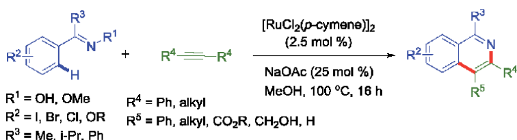
Figure 8. Ruthenium(II)-catalyzed synthesis of substituted Isoquinolines.
