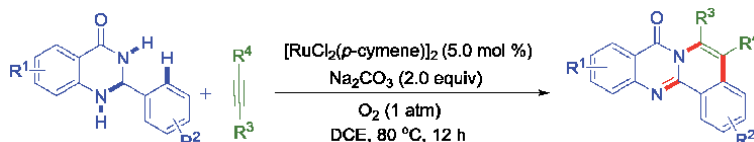
Figure 35. Ruthenium(II)-catalyzed external oxidant FreeSynthesis of tetracyclic Heteroarenes.
