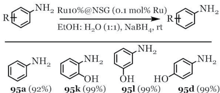
Figure 26. Ru10%@NSG catalyzed reduction of nitroarenes.
