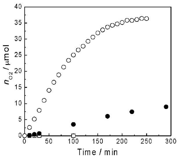
Figure 12. Time courses of the amount ( n_{O_2}/\text{Mol} ) of O_2 evolved in chemical water oxidation experiments in an aqueous solution at 25^\circ\text{C} using a Ce^{IV} oxidant. c_{Ce} = 0.1 \text{ M} (0.5 mmol); complexes, 20 \mu\text{M} (0.1 \mu\text{mol} ); \text{pH} = 1.0 ; liquid volume, 5.0 ml. (○) 4EtO , (●) 4H and (□) without complex. (reproduced with permission from ref. [39]. Copyright 2011 the Royal Society of Chemistry).
