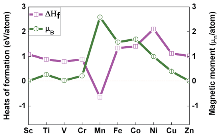
Figure 4. A comparison of the calculated heats of formation (eV/atom) and magnetic moment ( \mu_B /atom) of \text{X}_3\text{Ru} ( \text{X} = \text{Sc}, \text{Ti}, \text{V}, \text{Cr}, \text{Mn}, \text{Fe}, \text{Ni}, \text{Co}, \text{Cu} and \text{Zn} ) alloys.
