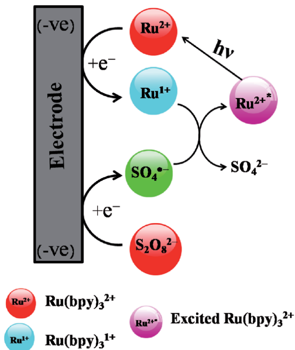
Figure 3. The scheme of reductive-oxidation mechanism of Ru(bpy)_3^{2+} molecule and persulfate.
