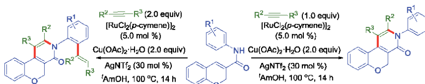
Figure 36. Ruthenium catalyzed synthesis of Benzopyran-fused 2-pyridones.
