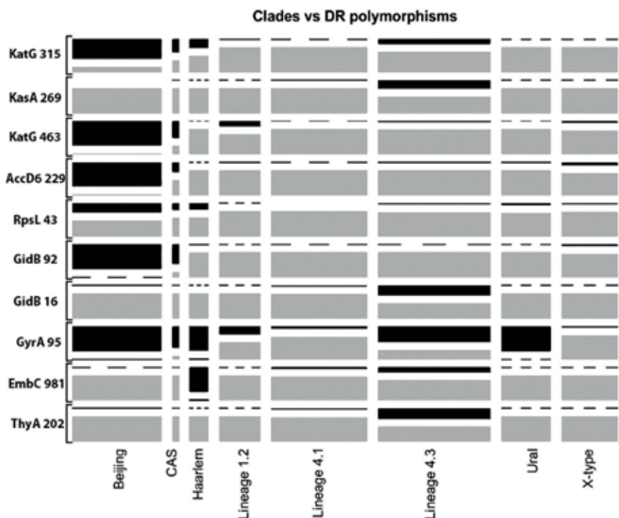
Figure 1. Mosaic plot representing the contingency table for the presence (black) or absence (gray) of each DR polymorphism for each of the 10 loci and the clade for the specimens in the GMTV dataset. The size of the rectangle represents the number of sequences in the category. A dotted line indicates that there were no specimens in that category. Clades with 10 or fewer representatives were omitted.
