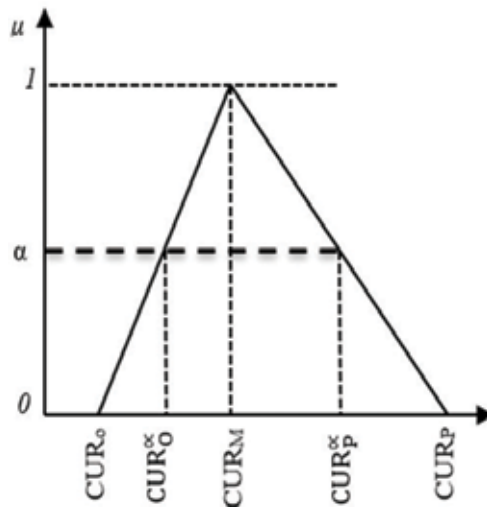
Figure 4. Triangular fuzzy number with \alpha -cut.
