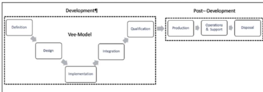
Figure 4. Generic system engineering process Vee-model.
