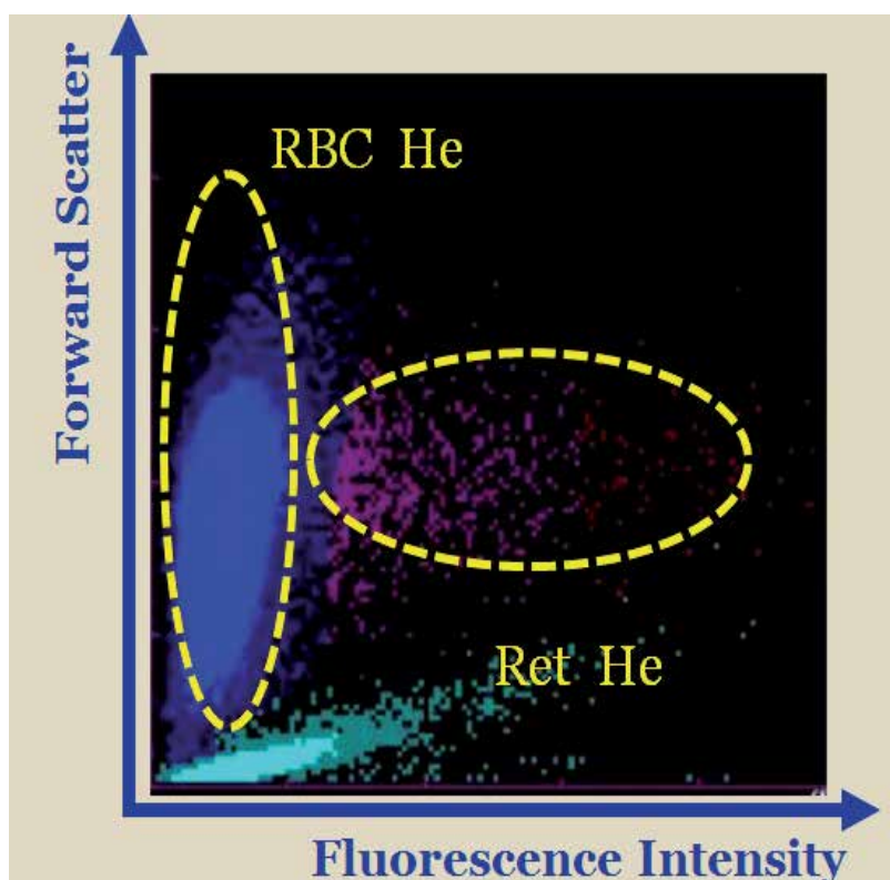
Fig. 4. In the reticulocyte channel blood cells are stained by a polymethine dye, specific for RNA/DNA, and analysed by flow cytometry using a semiconductor laser. A bi-dimensional distribution of forward scattered light and fluorescence is presented as a scattergram, indicating mature red cells and reticulocytes. Forward scatter correlates with erythrocyte and reticulocyte hemoglobin content (RBC He, Ret He).
