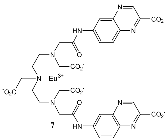
Fig. 2. Eu-DTPA-Quinoline Complex.
