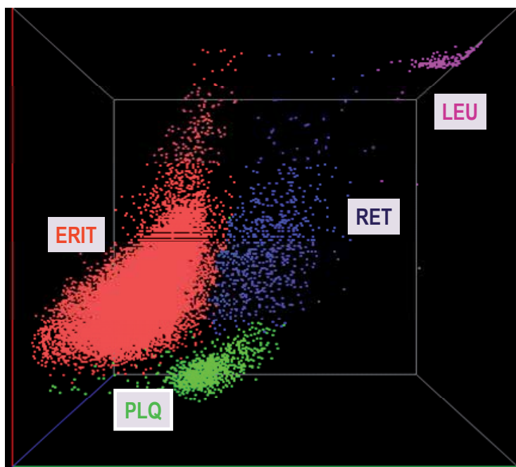
Fig. 6. the Beckman -Coulter cube in which the cells are classified according to the volume, conductivity and laser scatter signals. ERIT , erythrocytes; PLQ, platelets; RET, reticulocytes; LEU, leucocytes.
