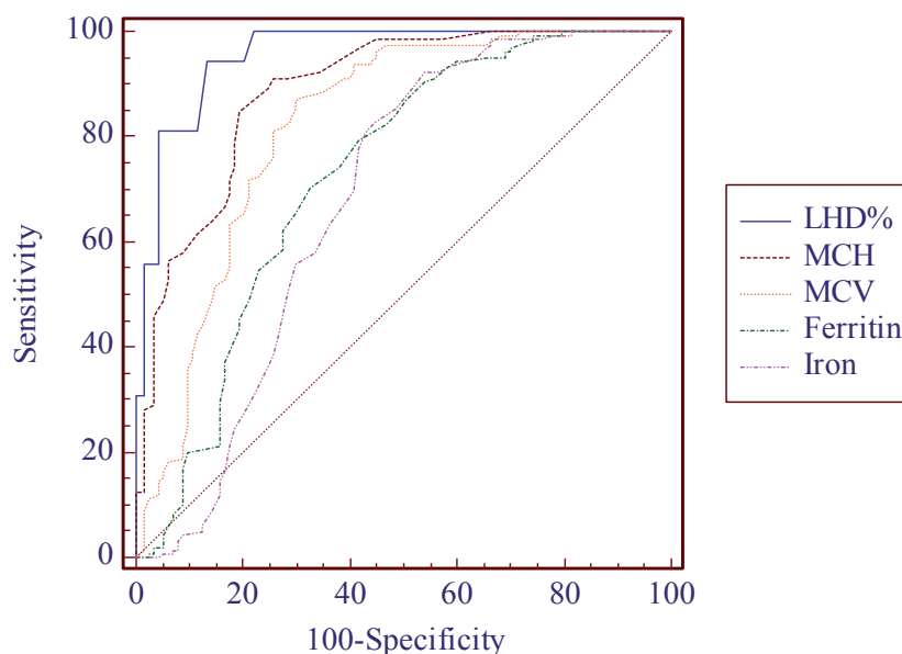
Fig. 9. Receiver operating characteristic (ROC) curve analysis for LHD% and Biochemical parameters and classical erythrocyte indices in the diagnosis of iron deficiency, defined by %Hypo >5%. LHD% Ares under curve (AUC) 0.954; mean cell hemoglobin (MCH), AUC 0.89; mean cell volume, (MCV), AUC 0.822; serum ferritin, AUC 0.722; serum iron, AUC 0.683.
