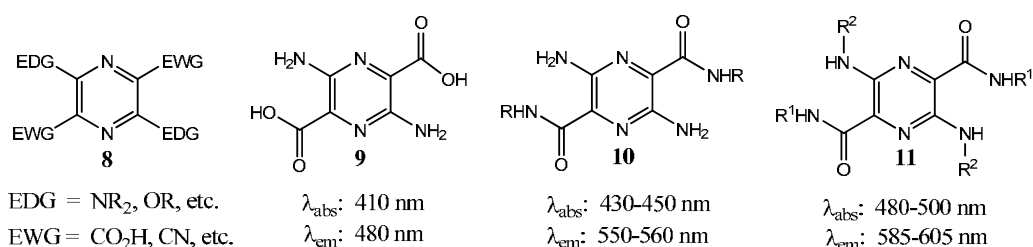
Fig. 3. Pyrazine Derivatives.
