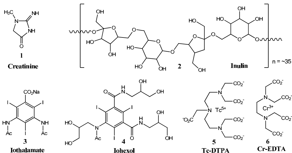
Fig. 1. Structures of Currently Known Exogenous GFR Markers.
