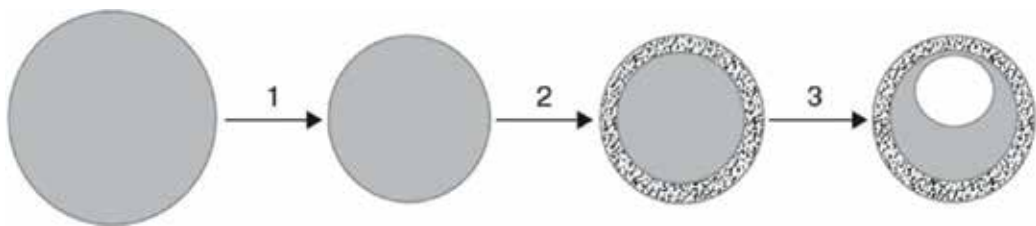
Figure 6. Schematic representation of droplet morphological changes during spray drying. Adapted from [2].
