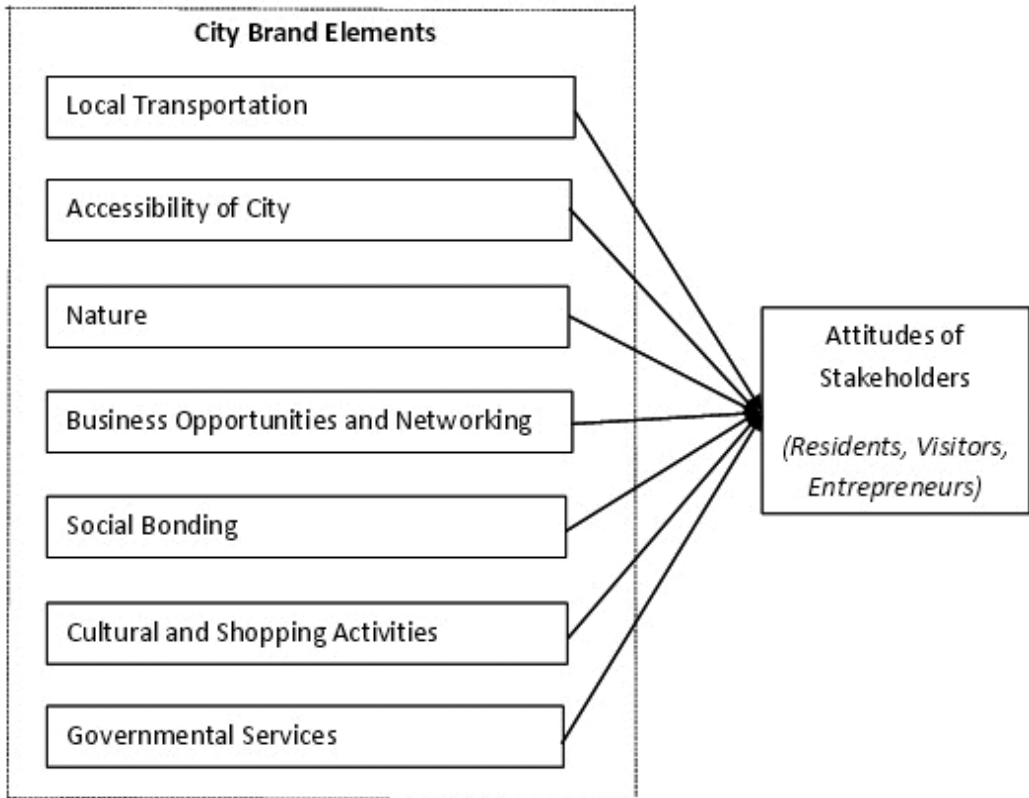
Figure 2. Research model.
