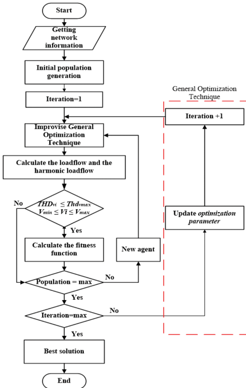
Figure 5. Flowchart of the general optimization technique for determining optimal placement and sizing of DG in a distribution system.
