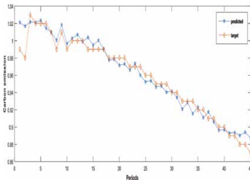
Figure 3. Visual inspection from the predicted and actual CO 2 emission [29].
