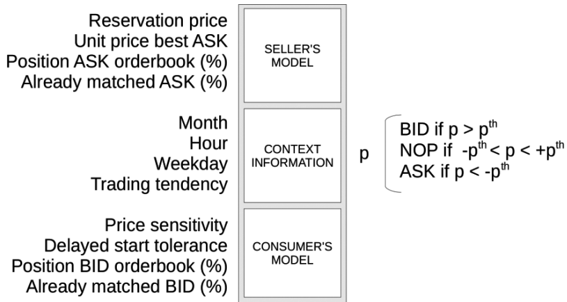
Figure 7. The introduced controller.
