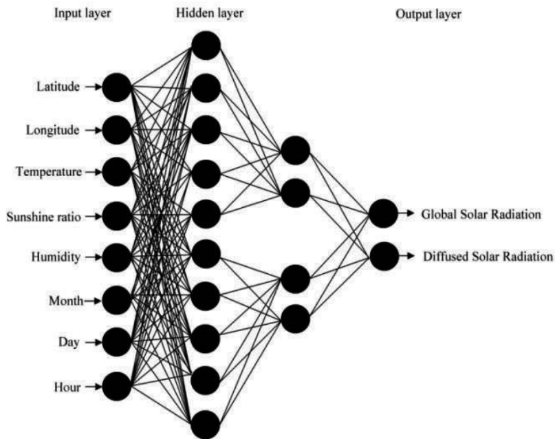
Figure 4. Topology of the GRNN used to model the global solar radiation.
