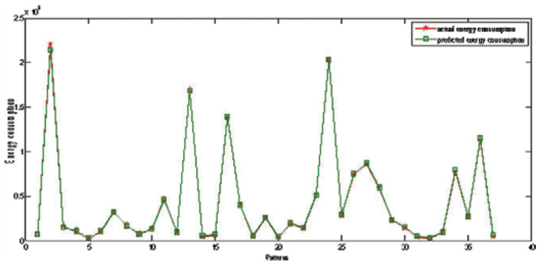
Figure 10. Visual inspection to the ANN prediction [32].
