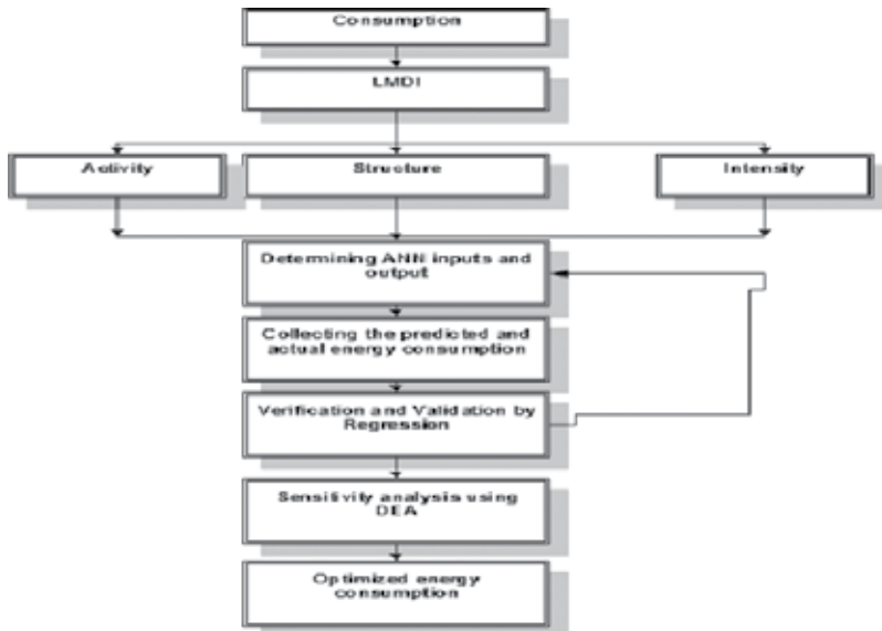
Figure 1. Hybrid structure for energy potential analysis.
