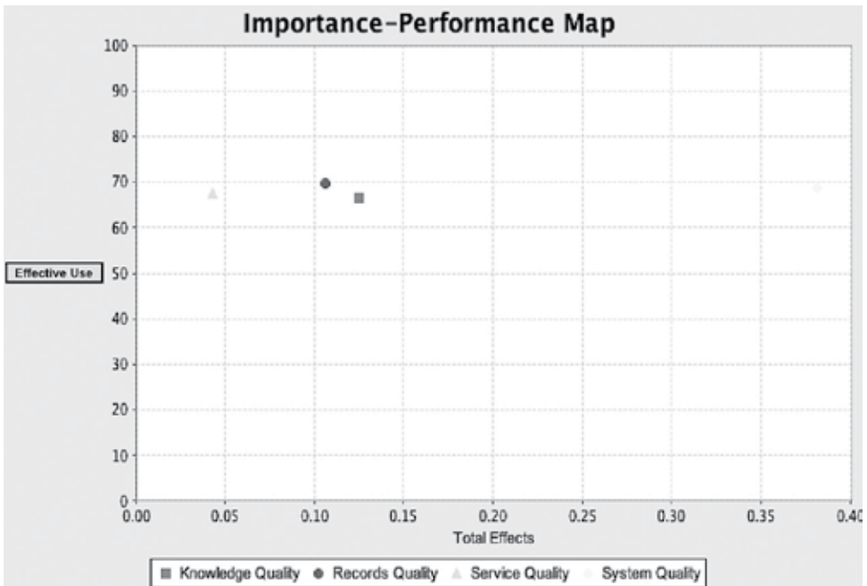
Figure 1. IPMA for effective use at construct level.
