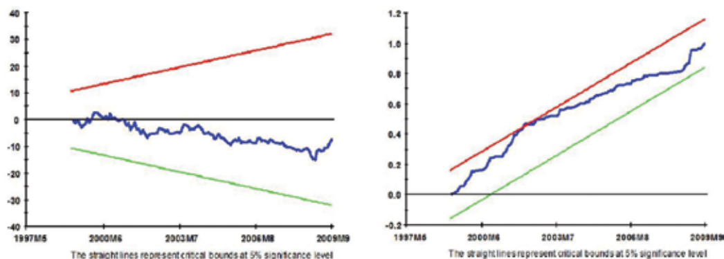
Figure 1. Diagnostic tests of CUSUM and CUSUMSQ.
