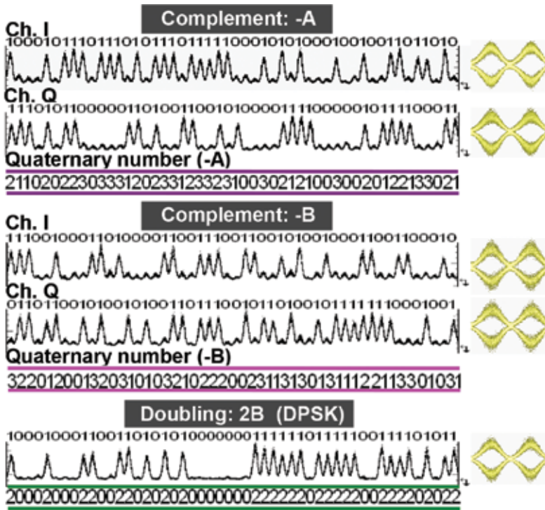
Figure 7. Demodulated waveforms and balanced eyes for 50-Gbaud quaternary complement and doubling using 100-Gbit/s (D)QPSK signals.
