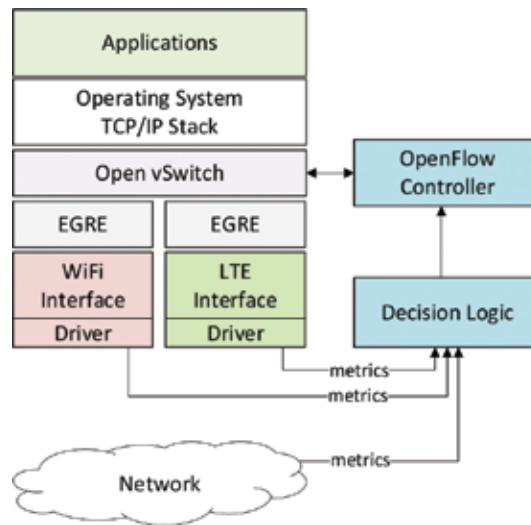
Figure 2. Proposed testbed topology for multi-RAT HetNets.
