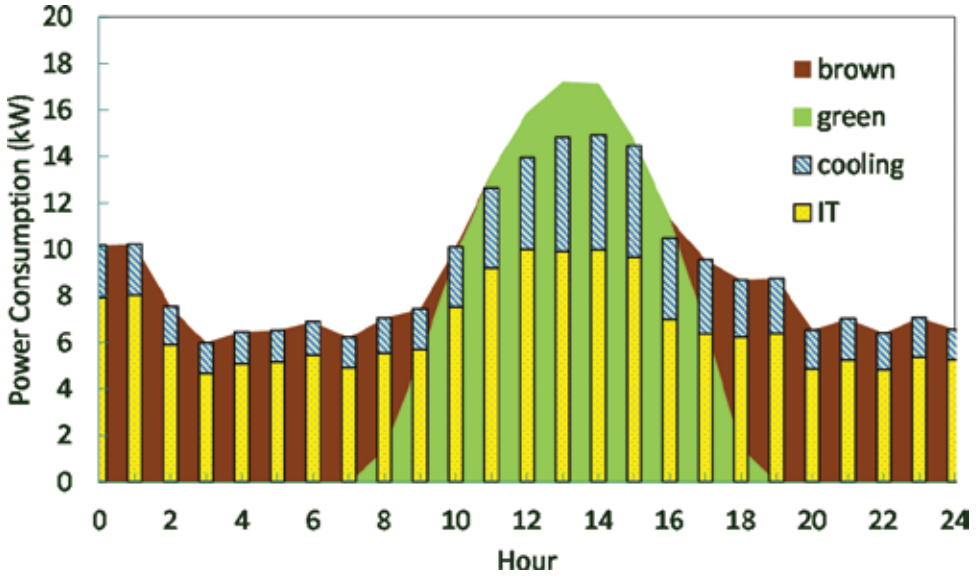
Figure 8. Power consumption details under JOP strategy.
