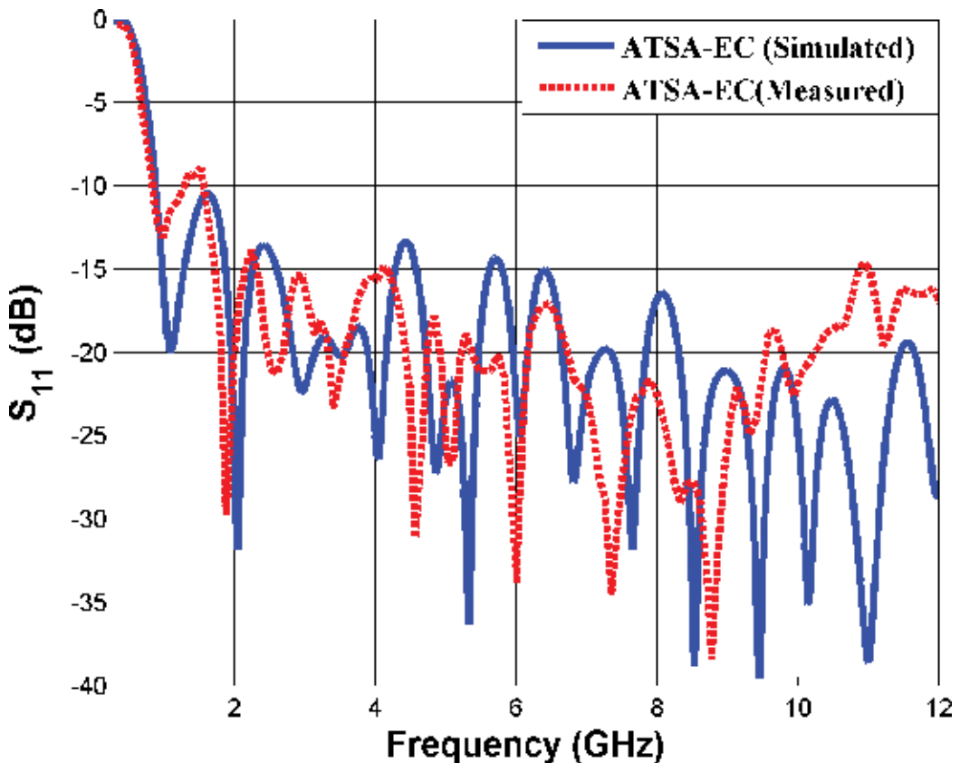
Figure 4. Measured return loss characteristics of fabricated ATSA-EC [34].
