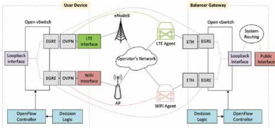
Figure 3. Overall architecture of prototype implementation.
