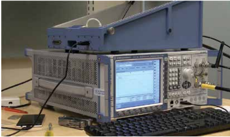
Figure 1. Setup with Rohde and Schwartz CMW500.
