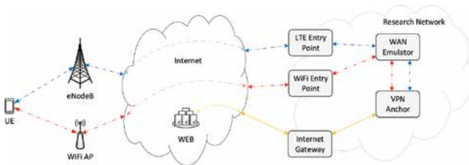
Figure 5. Setup with WAN emulation node.
