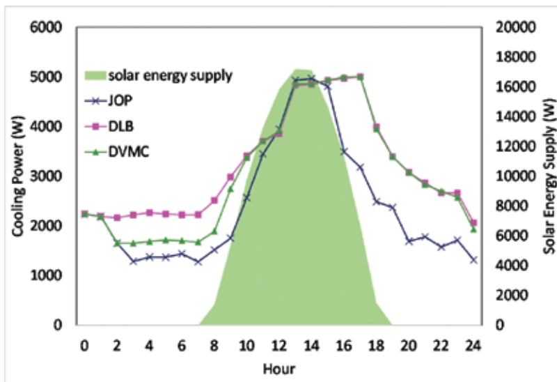
Figure 10. Cooling energy consumption under three different strategies.
