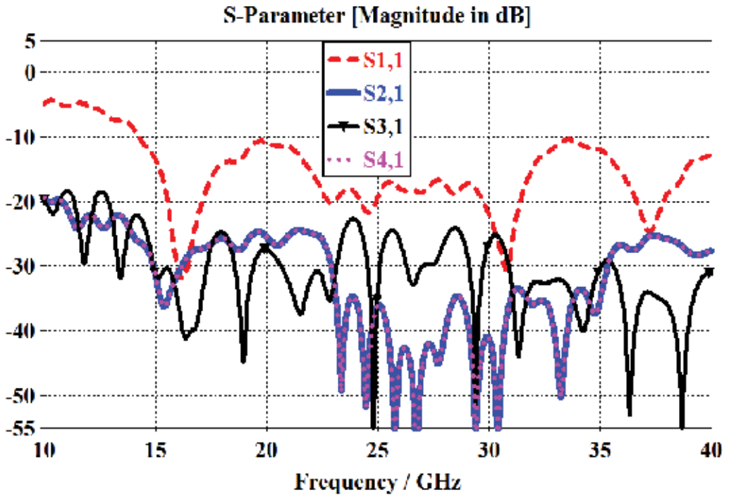
Figure 12. S-parameters of four-element beam-switched antenna system [38].
