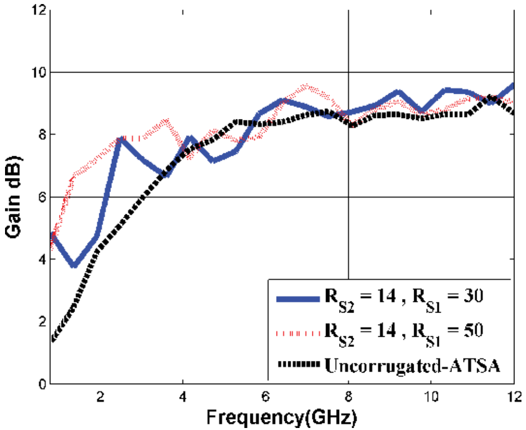
Figure 5. Simulated gain characteristics of ATSA at different edge corrugation values [34].
