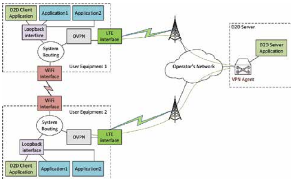
Figure 7. Prototype setup for D2D architecture.
