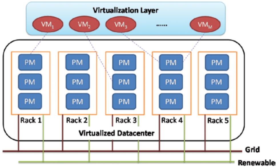
Figure 2. Virtualized datacenter.
