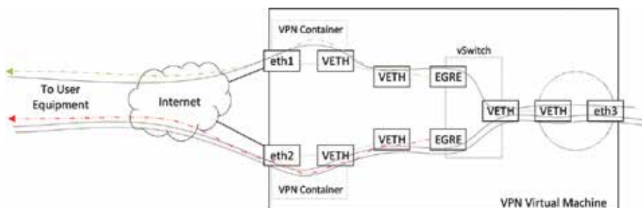
Figure 4. Detailed network architecture of VPN server.
