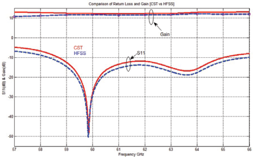
Figure 15. S-parameters and gain of proposed ACMPA.
