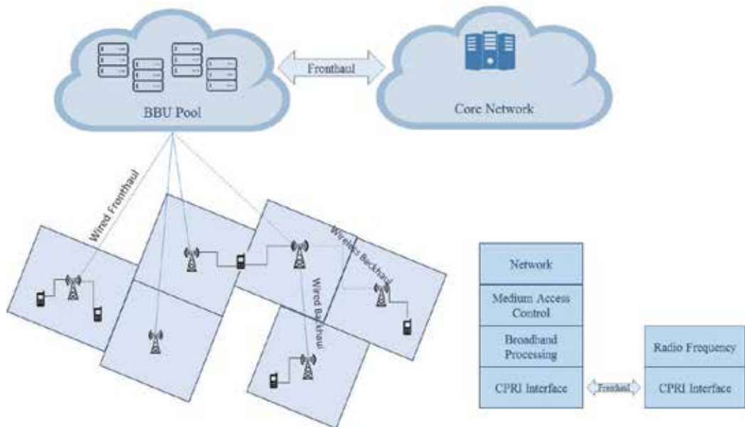
Figure 1. Architecture for general C-RAN system.
