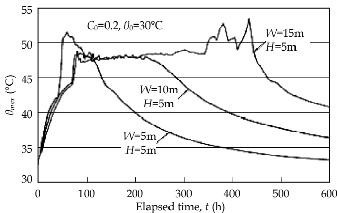
Fig. 19. Numerical simulation results of the maximum temperature transition in coal stock with three different aspect ratios
