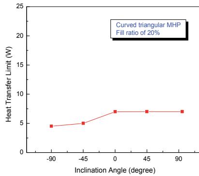
Fig. 9. Thermal performance by inclination angle
