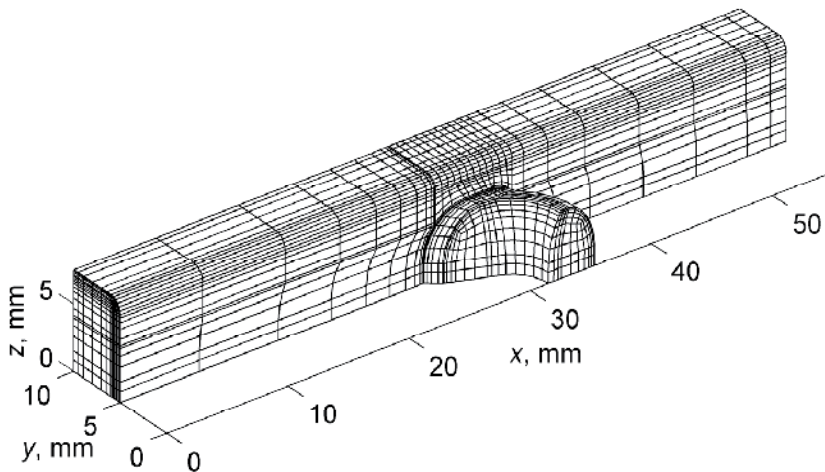
Fig. 19. Model of an electromagnetic railgun.
