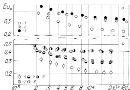
Fig. 26. Aerodynamic drag of bundles of partially finned tubes at \Theta > 0 . a) staggered bundles; b) in-line bundles; 1) geometry 6a; 2) geometry 8b; 3) geometry 8c; 4) geometry 10d; 5) geometry 12e; 6) geometry 13e; 7) geometry 14f; 8) geometry 15f (the geometry numbers correspond to Table 8)
