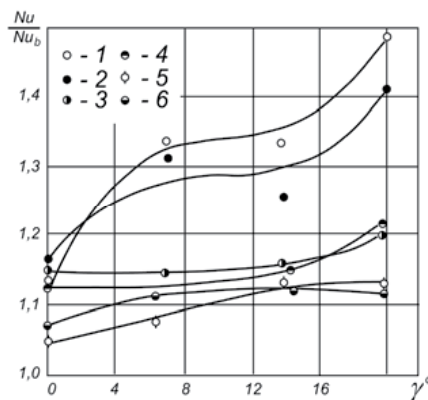
Fig. 16. Enhancement of heat transfer as a function of convergence angle \gamma at Re = 1.3 \cdot 10^4 . \sigma_1 = 3.21 ; \sigma_2 : 1) 1.29; 2) 1.55; 3) 1.79; 4) 2.02; \sigma_1 = 2.05 ; \sigma_2 : 5) 1.79; 6) 2.02
