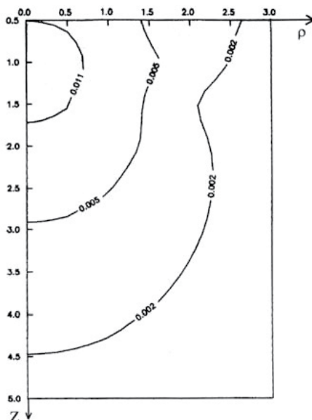
Fig. 16. Isolines of dimensionless major stresses \sigma_1^* = \sigma_T / \sigma_0 for features of materials from Table 3 (Yevtushenko et al., 2009).
