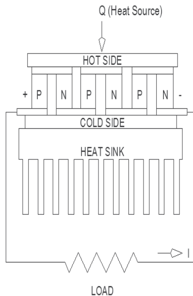
Fig. 3. Schematic of a thermoelectric power generator
