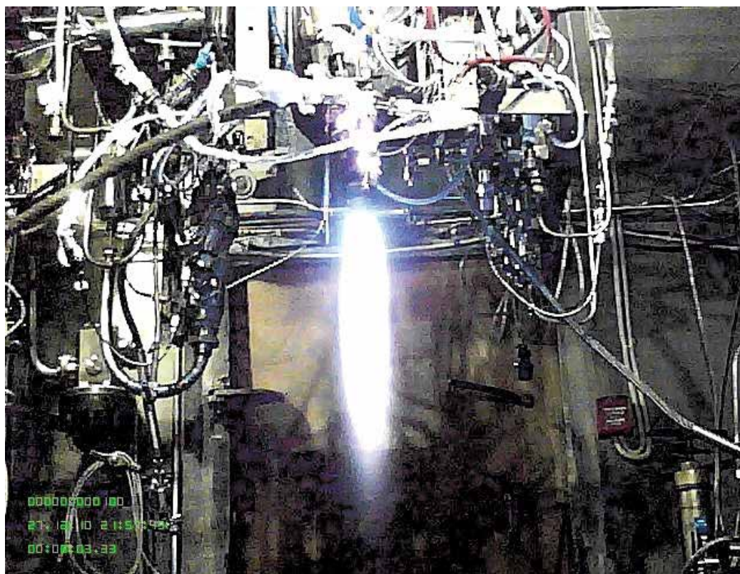
Fig. 16. Photo of working thruster.
