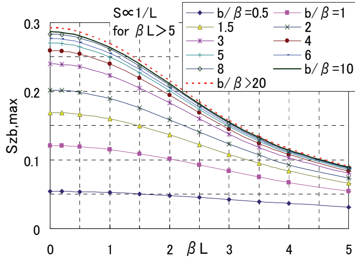
Fig. 8. The maximum bending stress
