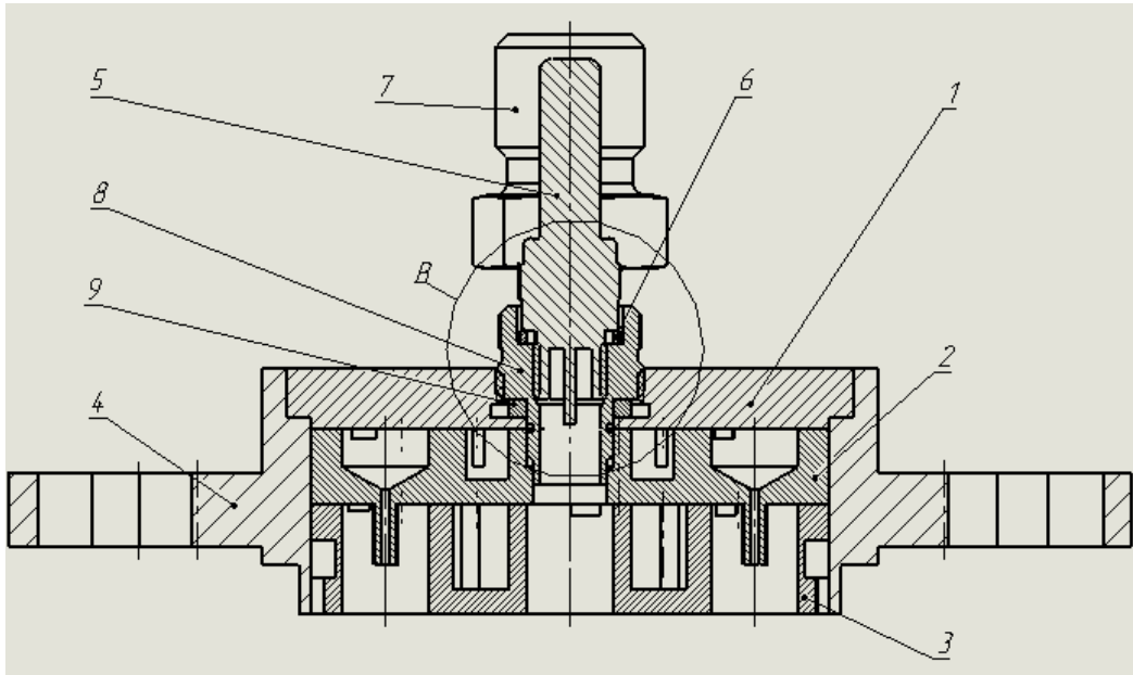
Fig. 10. Drawing of mixing head. 1.top of head, 2.plate of fuel, 3.plate of oxygen,4.flange, 5.candle of ignition, 6. compression of candle, 7.connecting pipes for components, 8.bush of candle, 9.compression of the bush.
