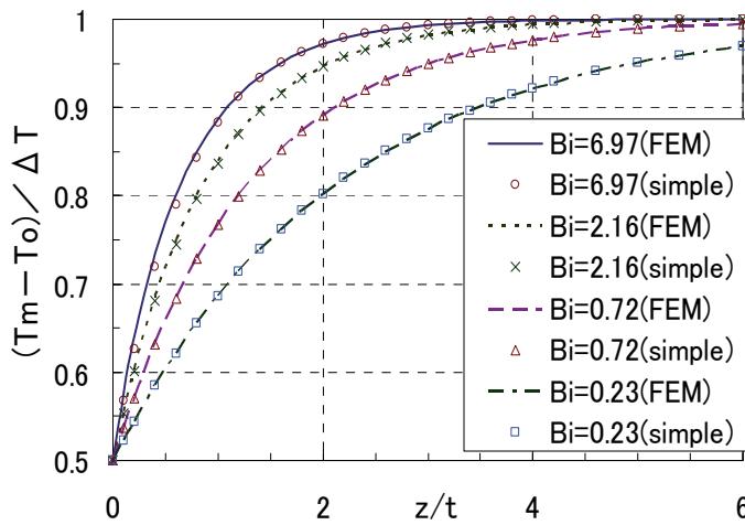
Fig. 4. Vessel temperatures for step-shaped fluid temperature
