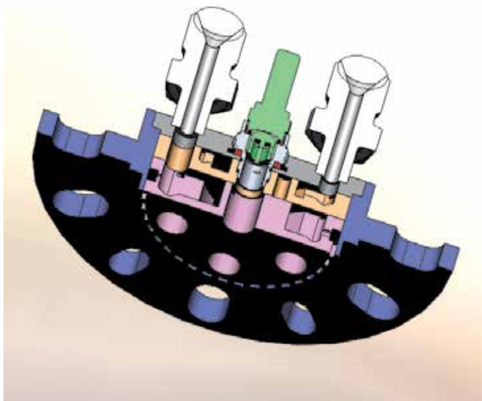
Fig. 11. Model of mixing head.
