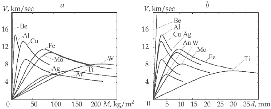
Fig. 6. Ultimate velocities vs. sheet mass ( a ) and vs. sheet thickness ( b ), for L = 1 m
