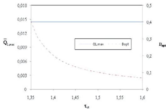
Fig. 17. Maximum heat exchanger, Q_{L,max} to reached a refrigerated space temperature set point temperature ( \tau_H=1.3 and \tau_L=0.97 ).
