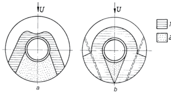
Fig. 18. Transformation of the dimensions of typical regions on the surface of a finned tube in the inward part of a bundle with \sigma_1/\sigma_2 > 2 with fin bent to provide for flow convergence. (a) an ordinary (basic) fin, and (b) bent fin. 1) region of intensive secondary circulating flows; 2) the trailing vortex zone
