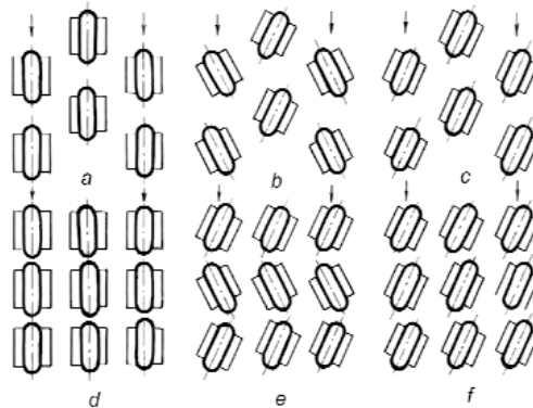
Fig. 24. Geometric arrangements of configured tubes within the bundles: (a) through (c) staggered bundles; (d) through (f) in-line bundles
