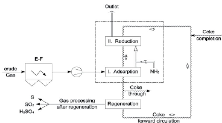
Fig. 19. Diagram of the Bergbau-Forschung process.
