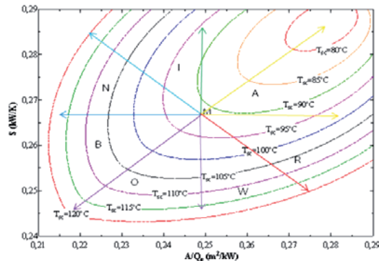
Fig. 3. Entropy rate versus the inverse specific cooling load.
