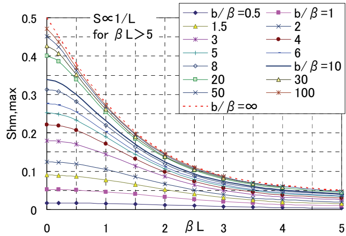
Fig. 10. The maximum membrane stress
