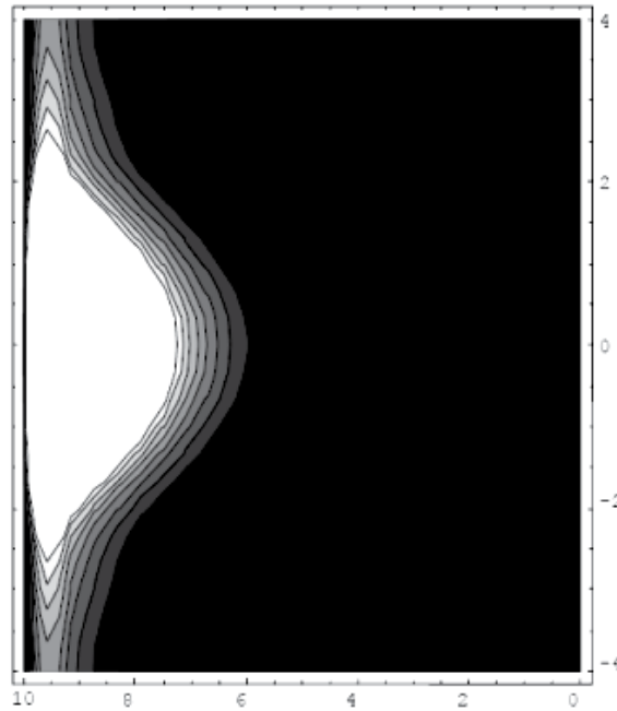
Fig. 4. The temperature field in water produced by a 10 MeV electron beam, when the “steady-state” is achieved.
