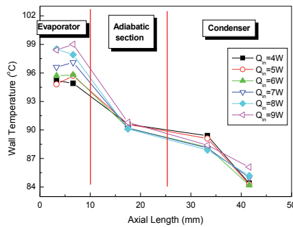
Fig. 8. Wall temperature distribution along the longitudinal axis of the MHP at T_v = 90 °C
