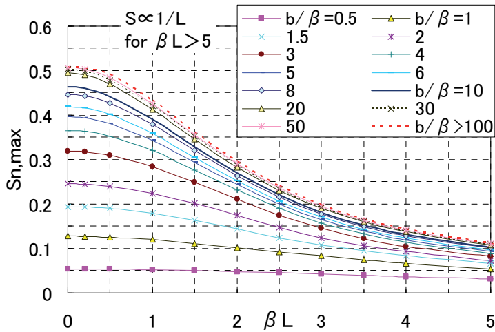
Fig. 12. The maximum stress intensity
