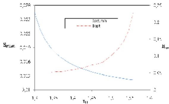
Fig. 15. The effect of dimensionless collector stagnation temperature, \tau_{st} , on minimum entropy set point temperature and optimal collector size ( \tau_{st}=1.6 ).
