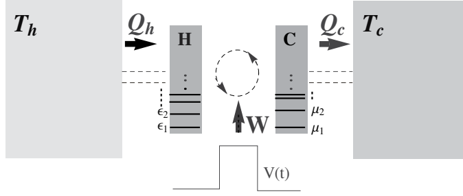
Fig. 1. The heat pump model. The few-level systems H and C operate between two baths at temperatures T_c and T_h T_c < T_h . During the first step of operation the two systems interact together either spontaneously or driven by a work-source at the cost of work W . During this stage couplings with the thermal baths is neglected (thermal isolation). In the second step the systems H and C do not interact with each other and freely relaxes to their equilibrium states (2) under action of the corresponding thermal bath.
