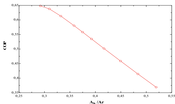
Fig. 4. Effect of the areas distribution on the COP
