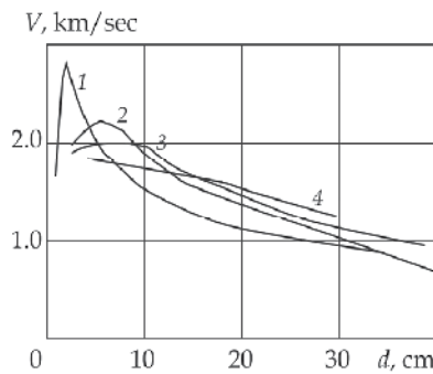
Fig. 17. Copper and titanium alloy composed armature. The curves 2 to 4 correspond to N = 4, 6, 10.
