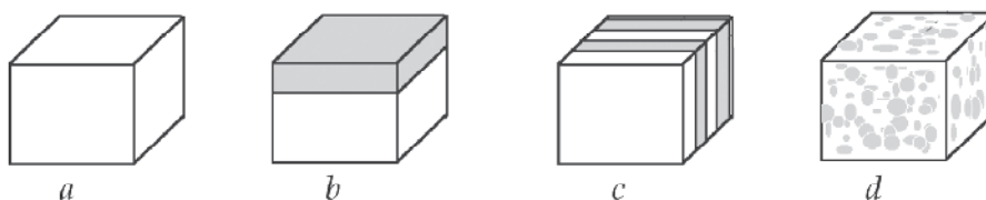
Fig. 2. Electrode structures. a ) homogeneous electrode, b ) coated electrode, c ) multilayer electrode with vertical layers, d ) composite electrode consisting of a mixture of powders.
