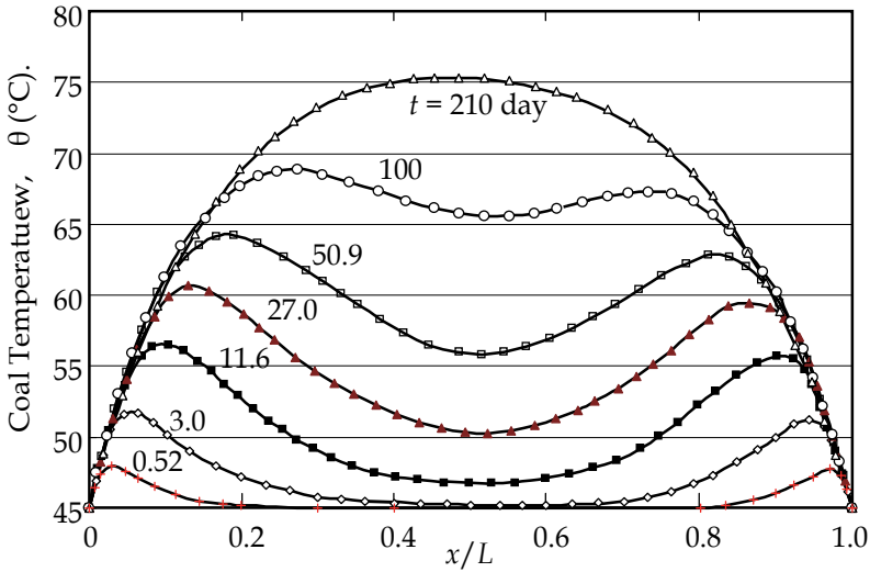
Fig. 11. Transition of temperature distribution of coal seam ( L=5\text{m} , Initial temperature, \theta(0) = \theta(L) = 45^\circ\text{C} , outer oxygen concentration, C(0) = C(L) = 0.20 , permeability K_0=50\text{ md} = 4.9 \times 10^{-14}\text{ m}^2 , D=7.1 \times 10^{-6}\text{ m}^2/\text{s} )
