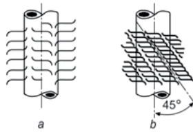
Fig. 1. Tubes with cut fins (Taranyan et al., 1972; Kuntysch & Iokhvedov, 1968; Iokhvedov et al., 1975)
