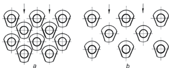
Fig. 20. Comparison of configurations of bundles with \sigma_1 = 3.21 , \sigma_2 = 1.55 ( \sigma_1/\sigma_2 = 2.08 ) (b) and with \sigma_1 = 2.64 , \sigma_2 = 1.29 ( \sigma_1/\sigma_2 = 2.06 ) (a)
