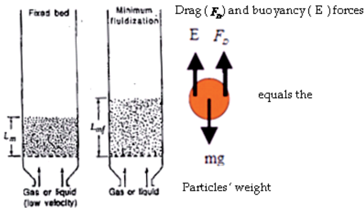
Fig. 8. Fixed and a fluidized bed of particles at a minimum fluidization velocity - adapted from (Kunii & Levenspiel, 1991).
