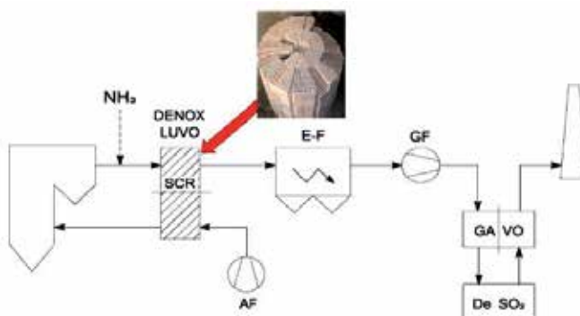
Fig. 8. "High dust" system with DENOX LUVO.
