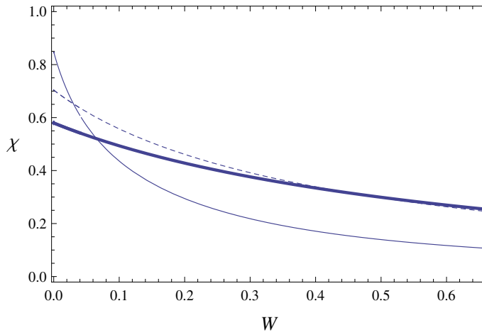
Fig. 3. The efficiency \chi versus work W for \theta \equiv T_c/T_h = 0.5 and n = 2 (normal curve), n = 10 (dashed curve) and n = 30 (thick curve).
