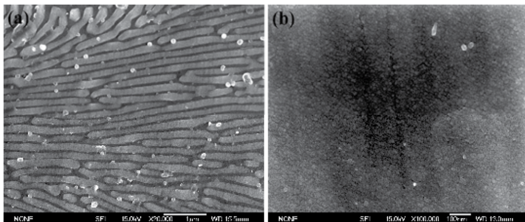
Fig. 1. SEM images of the \text{ZrW}_2\text{O}_8 block synthesized by LRS with 500 W laser power at 3 mm/s scan speed: (a) surface; (b) cross section.
