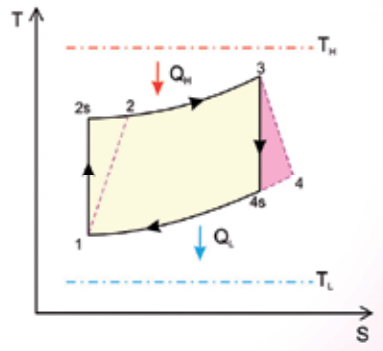
Fig. 3. A Brayton cycle with internal and external irreversibilities.
