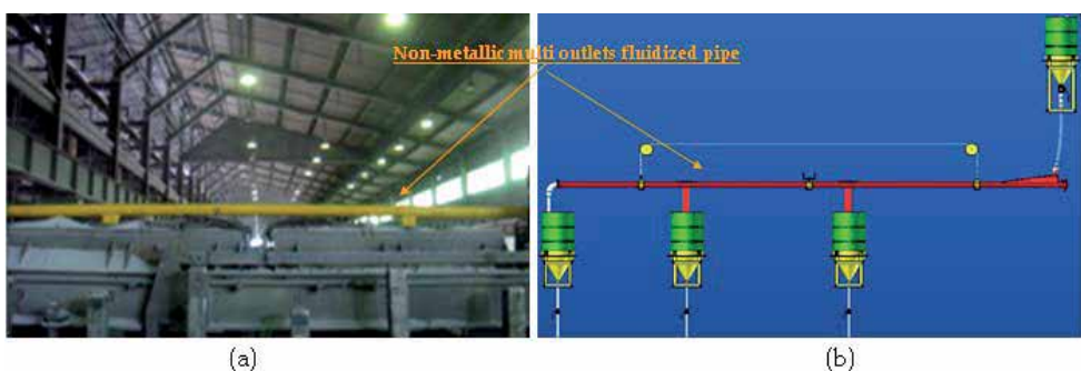
Fig. 21. a) The nonmetallic fluidized pipe during tests in electrolytic aluminum cell; b) Sketch of the nonmetallic fluidized pipe for performance test at the fluidization laboratory.
