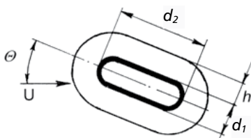
Fig. 5. Geometric characteristics of a plane-oval finned tube
