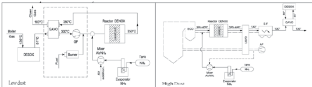
Fig. 12. DENOX installation
