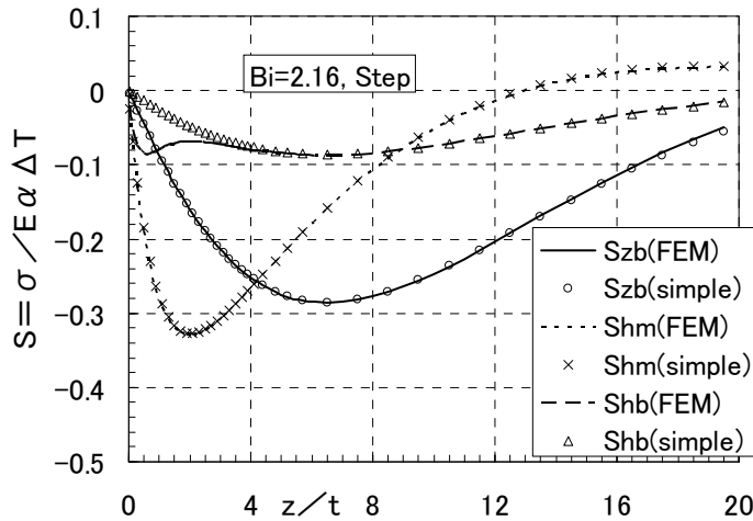
Fig. 5. Thermal stresses for step-shaped fluid temperature
