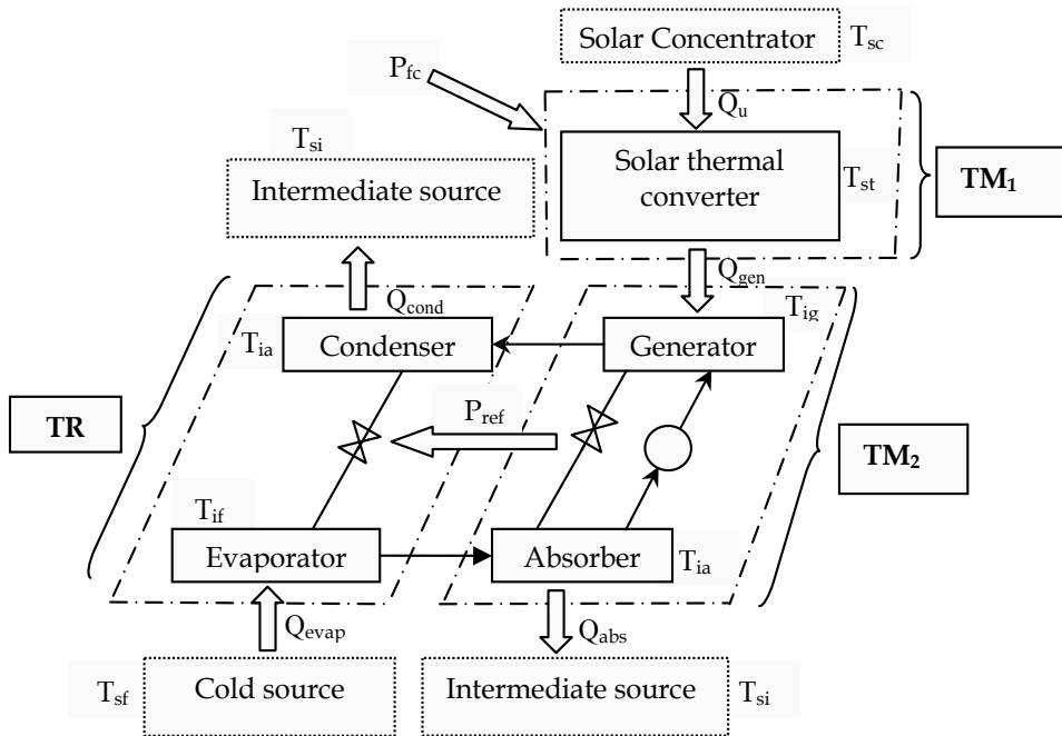
Fig. 1. Working principle and decomposition of a solar absorption refrigerator cycle Under the constraints:
