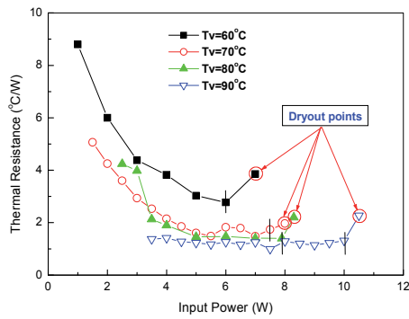
Fig. 12. Thermal performance by the operating temperature
