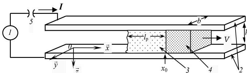
Fig. 1. Schematic diagram of the plasma-armature launcher of solids. 1 - power supply, 2 - electrodes, 3 - plasma armature, 4 -projectile, 5 - switch.
