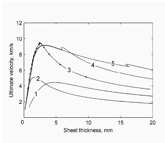
Fig. 8. Ultimate velocity versus sheet thickness for L = 0.1 m.
