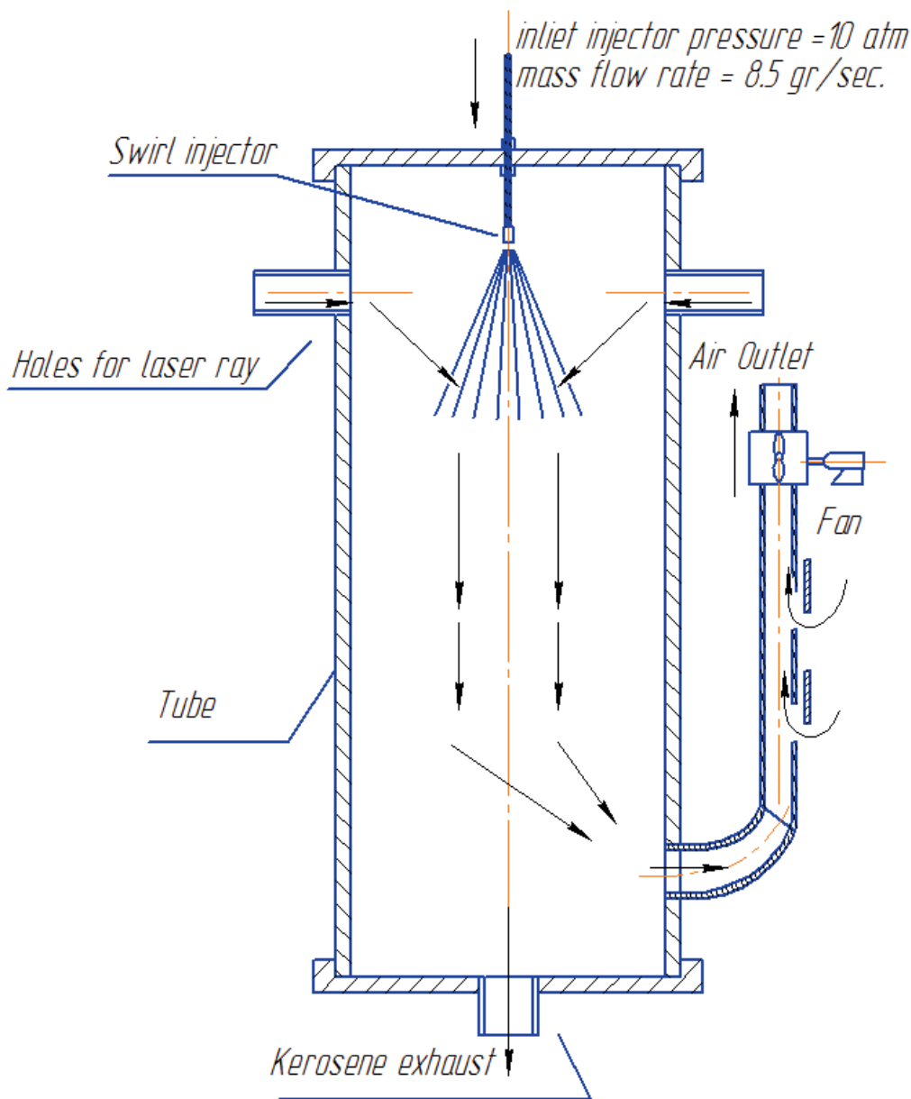
Fig. 2. Scheme of drops-trap.
