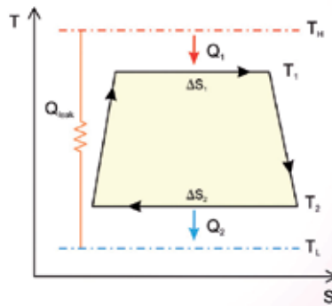
Fig. 1. A Carnot cycle with heat leak, finite rate heat transfer and internal dissipations of the working fluid.
