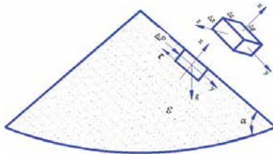
Fig. 10. Force balance acting on an elemental pecked bed block of alumina flowing to repose.
