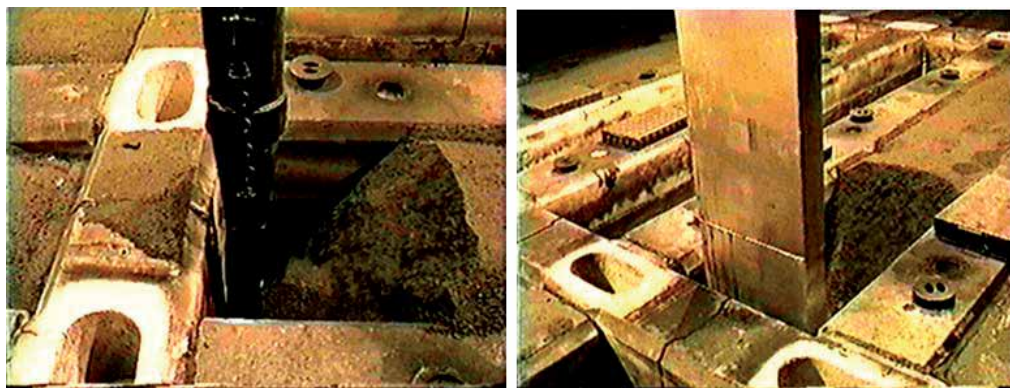
Fig. 14. Albras bake furnace coke suction system before and after modifications – source: Albras Alumínio Brasileiro SA.
