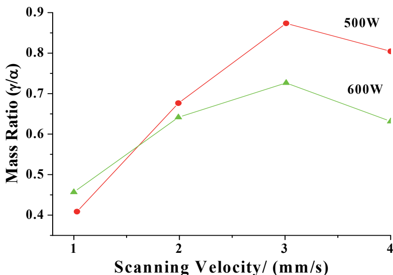
Fig. 5. The mass ratio of the \gamma to \alpha phase at different scan speeds.
