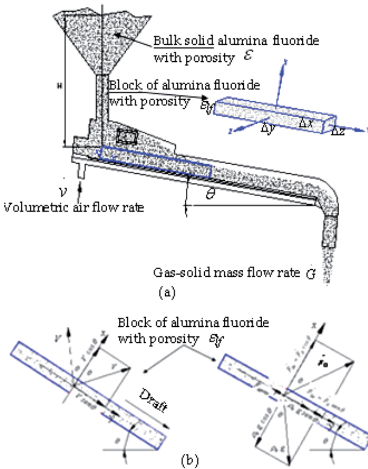
Fig. 11. (a) Elemental block of alumina in an air-fluidized conveyor inclined of an angle \theta , (b) in the left: elemental block alumina being fluidized by the components of superficial air velocity V , in the right: balance of forces per unit of volume acting on the elemental block of alumina.
