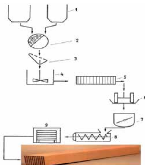
Fig. 2. Schematic diagram of production of monolithic carriers. 1-Raw material dispensers, 2-Grinder, 3-Sieve, 4-Tank with agitator, 5-Press, 6-Crusher, 7-Agitator, 8-Belt press, 9-Dryer.
