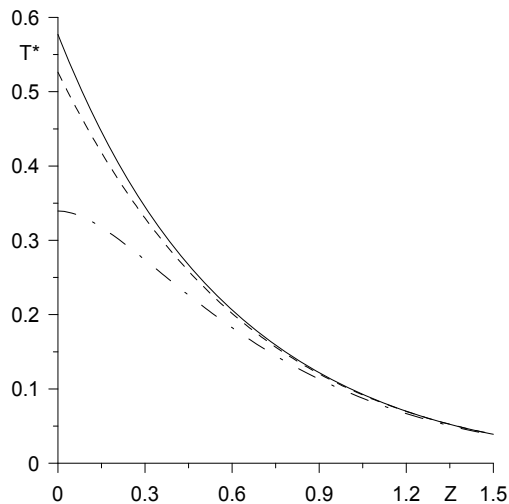
Fig. 5. Evolution of dimensionless temperature T^* along symmetry axis \rho = 0 at \tau_s = 0.6 (Yevtushenko et al., 2009).
