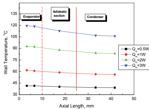
Fig. 14. Temperature distributions along FPMHP with fill ratio of 25% with the axial length for rectangular
