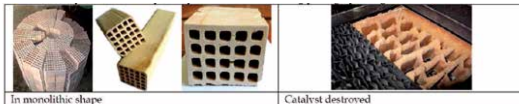
Fig. 14. View of a catalyst SCR.
