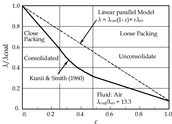
Fig. 5. Effective thermal conductivity vs. porosity of coal stock in the air evaluated by Kunii & Smith's equation(1960) (a case for \lambda_{coal}/\lambda_{air} = 13.3 )
