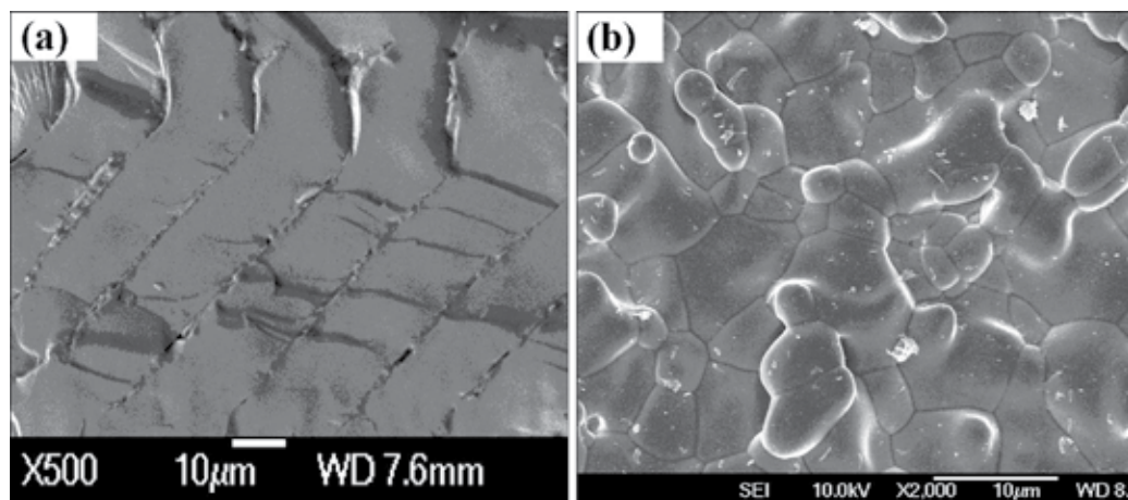
Fig. 6. SEM images of the LSGM samples prepared by (a) LRS and (b) solid state reactions at 1600\text{ }^{\circ}\text{C} .
