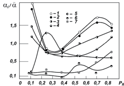
Fig. 6. Distribution of the relative heat transfer coefficient over the height of type 1 fin ( h/d = 0.932 ) located in the first (along the gas flow) row. Re = 2 \cdot 10^4 . \varphi , °: 1) 0; 2) 30; 3) 60; 4) 90; 5) 120; 6) 150; 7) 180
