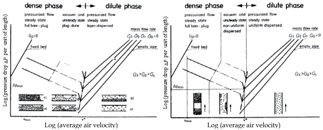
Fig. 7. Conveying conditions showing the changes in solids loading; left: State diagram horizontal flow, right: State diagram vertical flow - source: (Klinzing et al, 1997).
