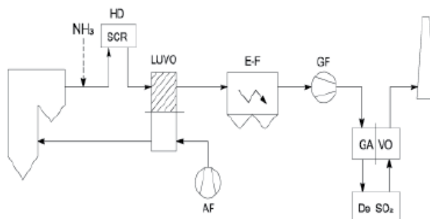
Fig. 7. "High dust" system with desulphurisation and denitrification.
