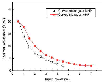
Fig. 11. Performance comparison by cross-section type
