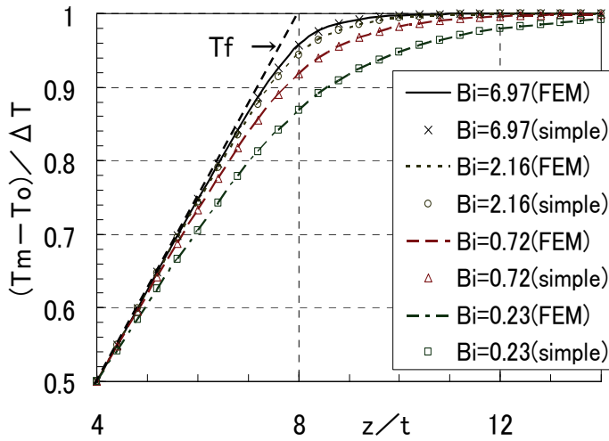
Fig. 6. Vessel temperatures for ramp-shaped fluid temperature
