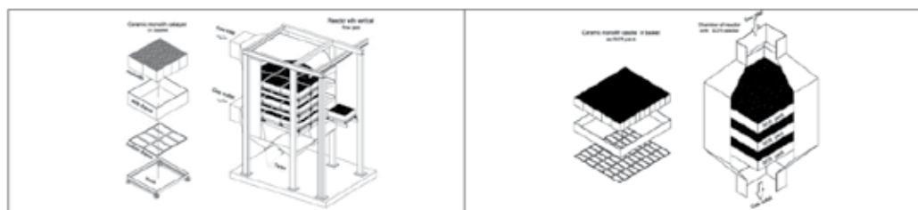
Fig. 16. Diagram of the SCR reactor (right - the element and package of ceramic catalysts)
