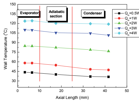
Fig. 7. Wall temperature distribution along the longitudinal axis by thermal loads
