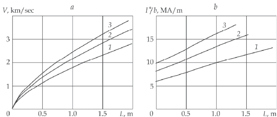
Fig. 3. Velocity (a) and critical current density (b) vs. plasma piston position in the railgun channel for copper electrodes. The numbers 1, 2, and 3 correspond to plasma length equal 5, 10, 15 cm.
