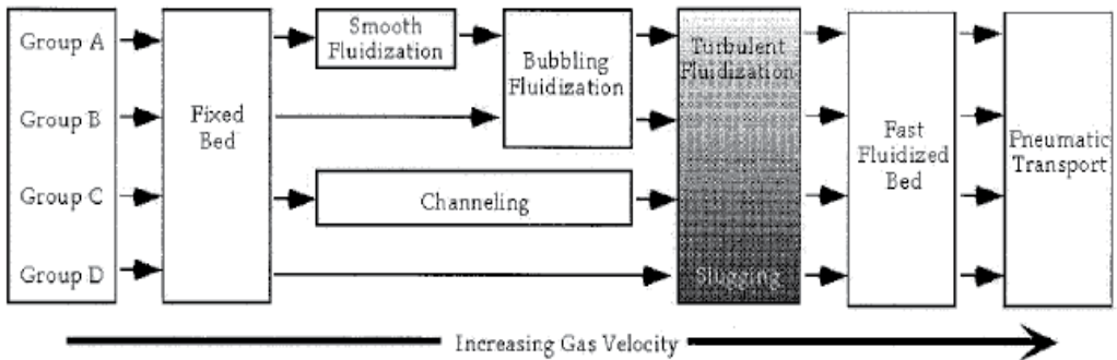
Fig. 5. Flow regime map for various powders.
