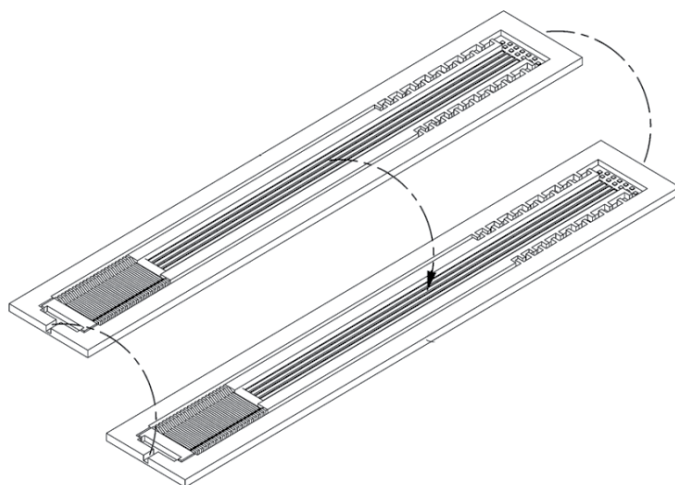
Fig. 26. Micro CPL considering commercialization
