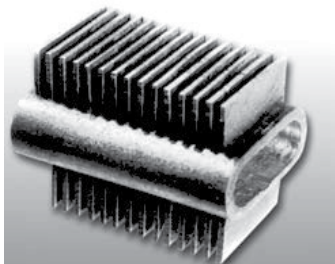
Fig. 23. Partially finned flattened oval tubes
