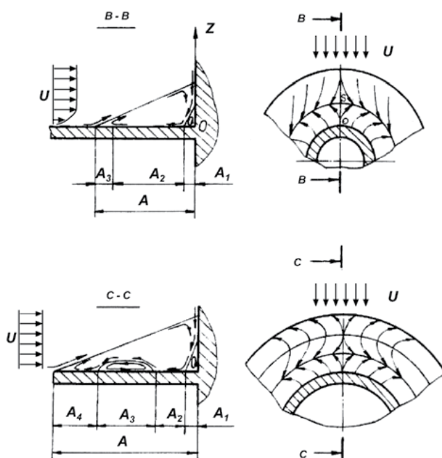
Fig. 7. Patterns of flow upstream of the windward part of the finned tube. a) At high h/d ; b) at low h/d ; A zone of secondary circulation flows; A_1 and A_3 zones of separation of the boundary layer from the surface; A_2 and A_4 reattachment regions
