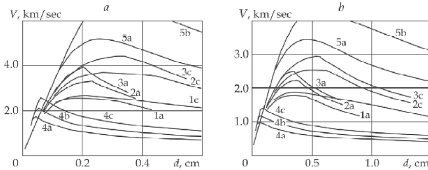
Fig. 14. The dependences of the ultimate velocity for aluminum (a) armatures and tungsten (b) multilayer armatures.
