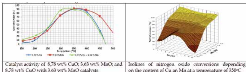
Fig. 7. Catalyst activity
