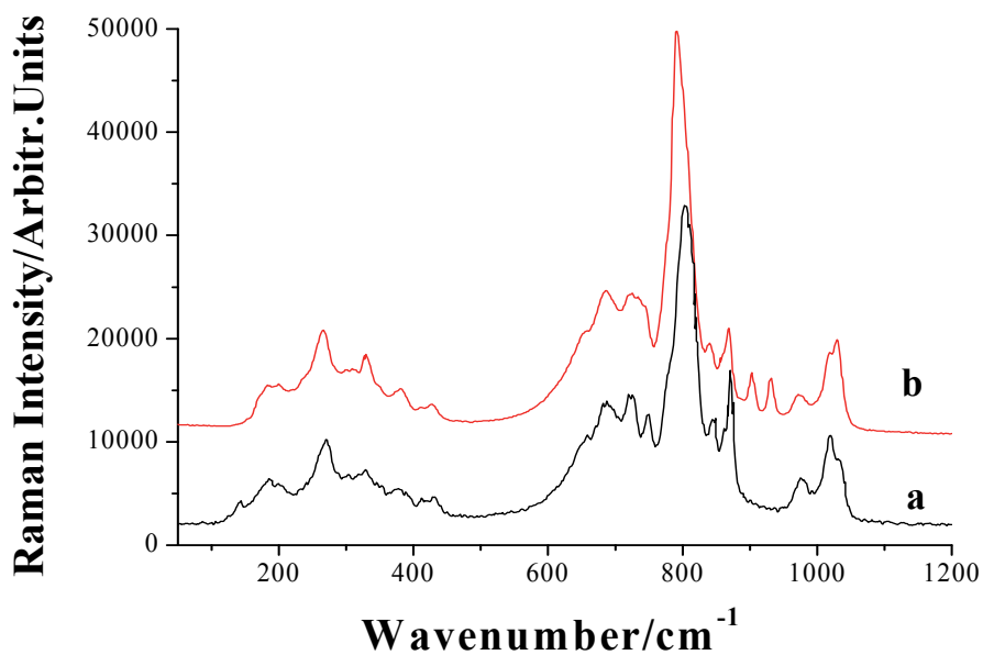
Fig. 3. Raman spectra of \text{ZrW}_2\text{O}_8 synthesized with 500 W laser power and 3 mm/s scan speed cooled (a) in air and (b) in water.
