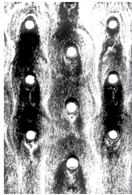
Fig. 14. Flow pattern in the finned tube bundle with S_1/S_2 = 3.0 ( Re = 5.3 \cdot 10^4 ) (Pis'mennyi, 1991)
