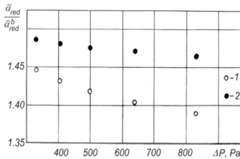
Fig. 22. Ratio of surface-averaged reduced heat transfer coefficients of the enhanced and basis bundles at the same values of drag and \sigma_2 = 1.29 ; \sigma_1 : 1) 3.21; 2) 2.64
