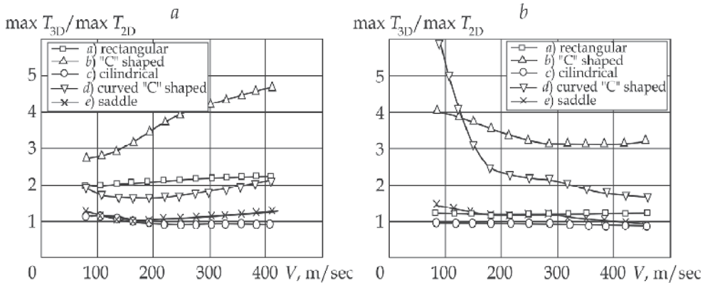
Fig. 21. Ratio of the maximum armature temperatures obtained by 3D and 2D calculations versus Cu (a) and Al (b) armature velocity
