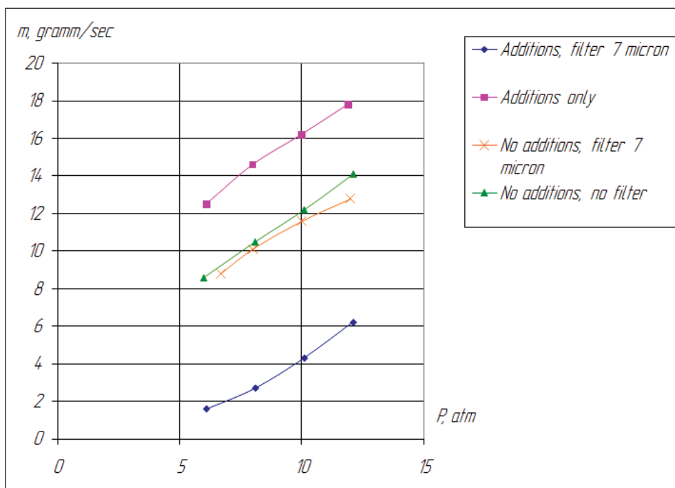
Fig. 9. Feeding pressure/mass flow rate dependency.
