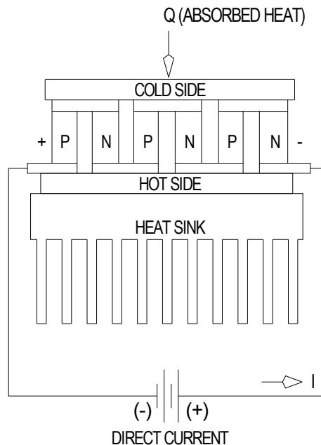
Fig. 2. Schematic of a Peltier effect (thermoelectric cooling device)
