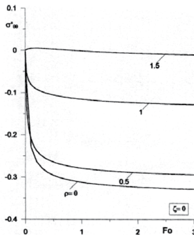
Fig. 13. Evolution of dimensionless peripheral stresses \sigma_{\theta\theta}^* on the irradiated surface of the body \zeta = 0 for Bi = 0.01 and for different values of dimensionless radial variable \rho (Rozniakowski et al., 2003).
