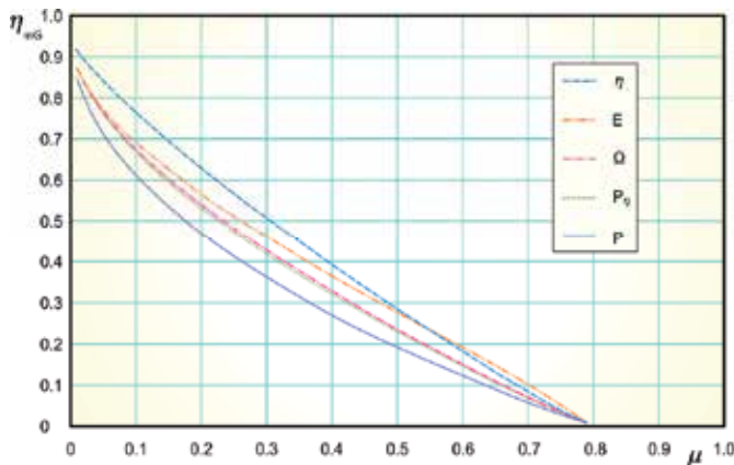
Fig. 5. Behaviors of \eta_{mp} , \eta_{max} , \eta_{mE} , \eta_{mp\eta} , \eta_{m\Omega} , with respect to \mu if I = 1.235 and L = 0.01 .
