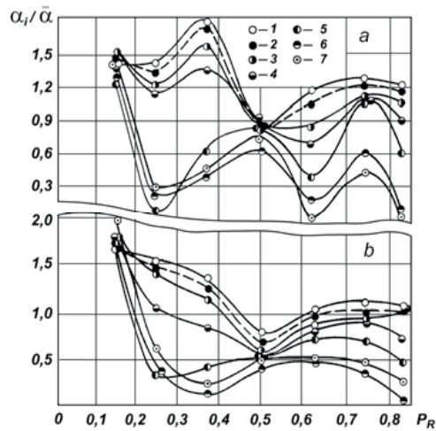
Fig. 8. Distribution of the relative heat transfer coefficient over the height of type 2 fin ( h/d = 0.357 ) located in the first (in the direction of gas flow) row. Re: a) 1 \cdot 10^4 ; b) 2 \cdot 10^4 . \varphi , °: 1) 0; 2) 30; 3) 60; 4) 90; 5) 120; 6) 150; 7) 180
