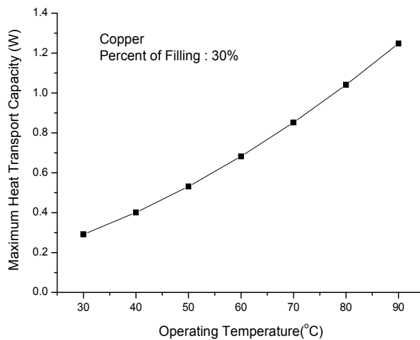
Fig. 1. Maximum heat transport capacity according to operating temperatures
