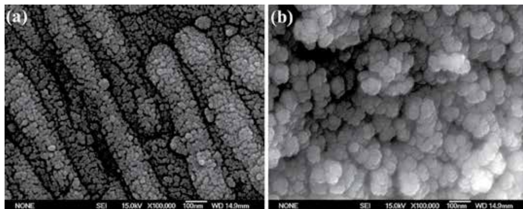
Fig. 4. SEM images of the \text{ZrW}_2\text{O}_8 block synthesized by LRS and cooled in water.
