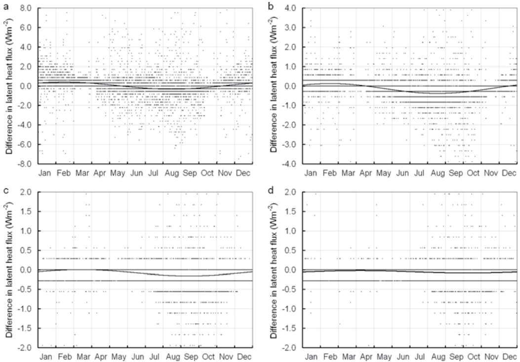
Fig. 6. Latent heat flux of the no-groundwater profile subtracted from those of profiles with groundwater at a) 0.5 m depth b) 1 m depth c) 2 m depth d) 3 m depth. Solid lines are first harmonics.
