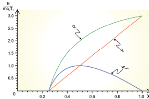
Fig. 6. Heat and work qualitative behavior for \mu=0.25 .
