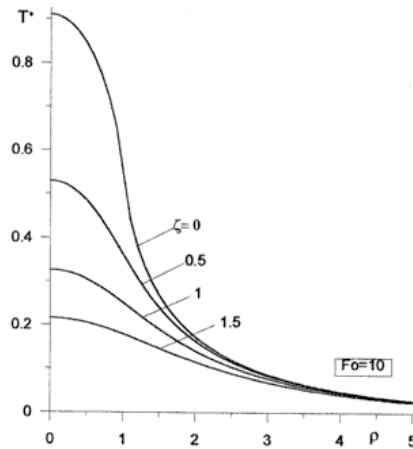
Fig. 10. Distribution of dimensionless stationary temperature T^* along the dimensionless radial variable \rho for Bi = 0.01 , \tau = 10 and for different values of dimensionless variable \zeta (Rozniakowski et al., 2003).
