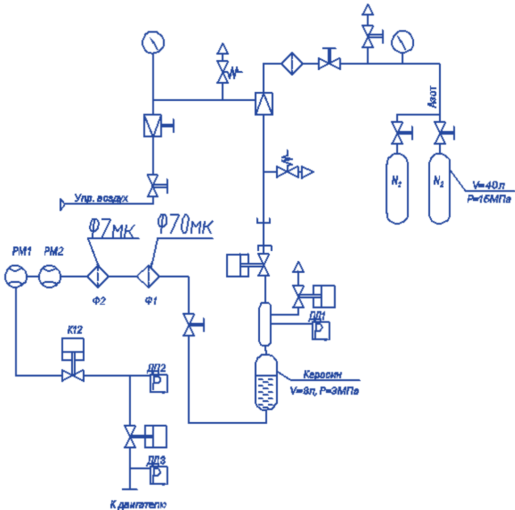
Fig. 1. Kerosene feeding system.
