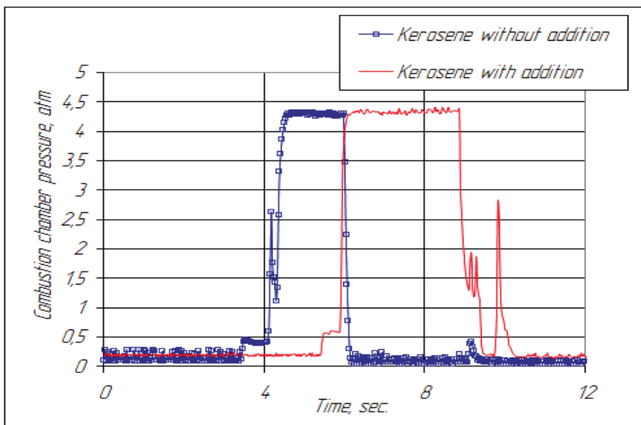
Fig. 17. Combustion chamber pressure.
