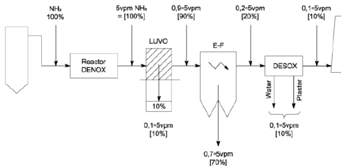
Fig. 13. \text{NH}_3 balance at SCR - "HD"
