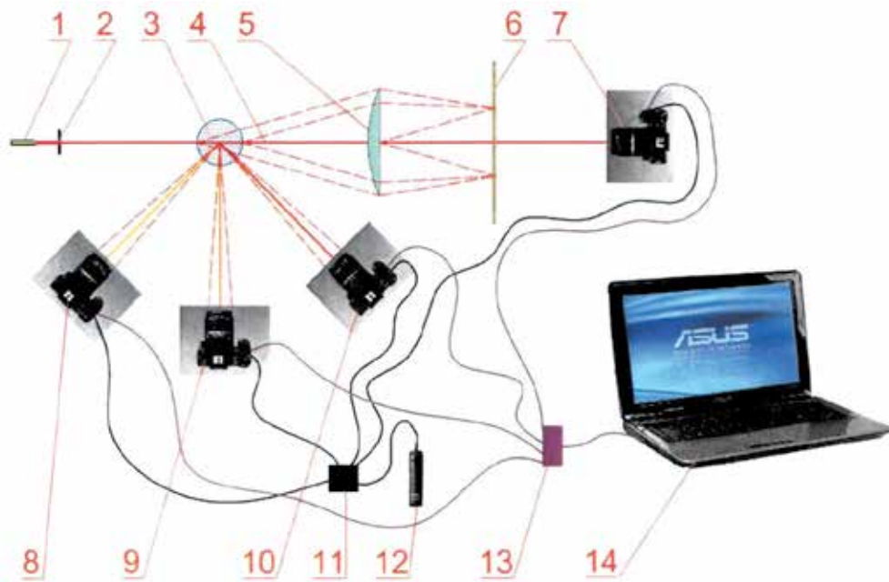
Fig. 6. Principle scheme of system for measurement distribution drops at sizes.
