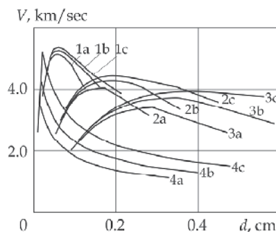
Fig. 16. Shaped aluminum armature. Curves 1 to 3 correspond to f=1, 0.5, 0.3 . Curves 4 are for homogeneous armature.
