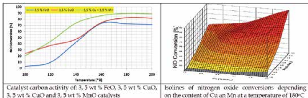
Fig. 21. Carbon based catalyst activity
