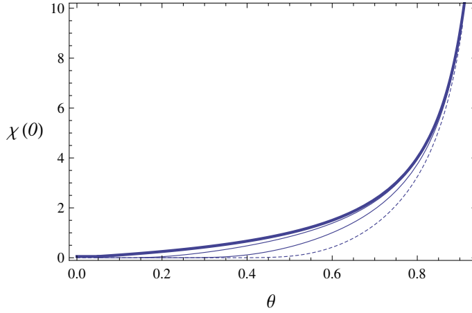
Fig. 4. The maximal efficiency \chi(0) = \chi(W = 0) given by (??) versus \theta = T_c/T_h for n = 2 (top normal curve), n = 101 (bottom normal curve), and n = 10^5 (dotted curve). Thick curve: the efficiency \theta/(1 - \theta) .
