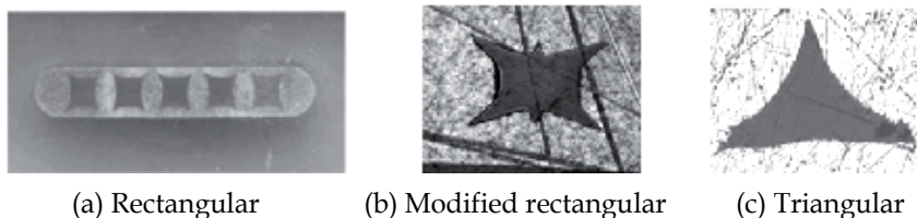
Fig. 5. Cross sections of the FPMHPs
