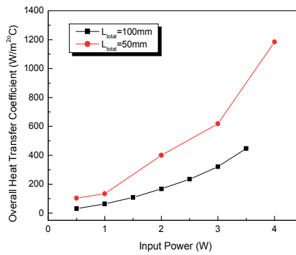
Fig. 10. Overall heat transfer coefficient by total length
