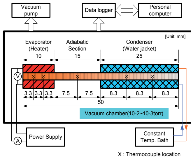
Fig. 6. Experimental apparatus
