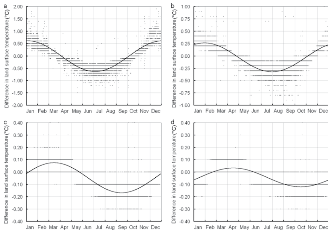
Fig. 3. Land surface temperature of the no-groundwater profile subtracted from those of profiles with groundwater at a) 0.5 m depth b) 1 m depth c) 2 m depth d) 3 m depth. Solid lines are first harmonics.
