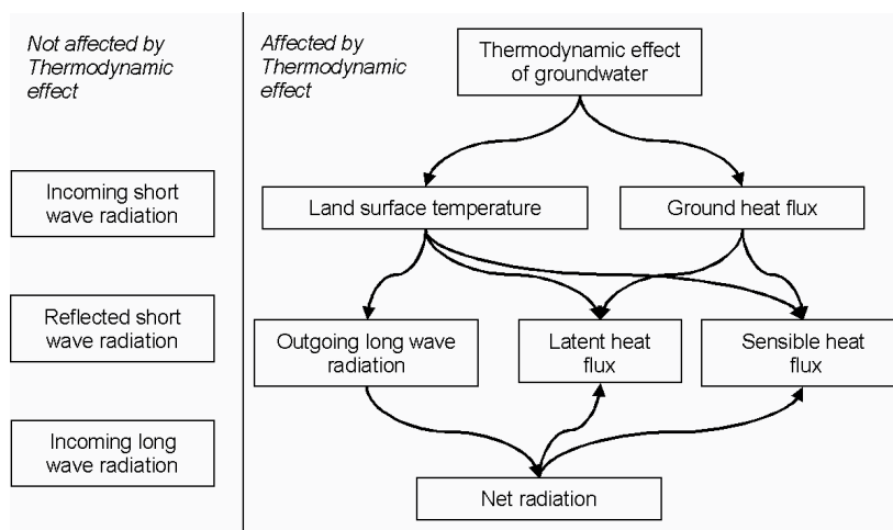
Fig. 9. Schematic description of groundwater thermodynamic effect on land surface temperature and the different components of surface energy balance.
