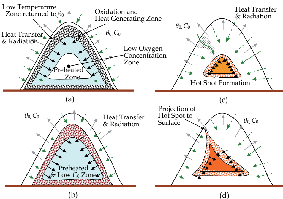
Fig. 2. Schematic process showing spontaneous combustion of large amount of coal stock, (a), (b) and (c): Hot spot forming process with accumulating heat and shrinking zone of oxidation and preheating zone, (d): Projection growth of hot spot toward to stock surface through high permeable path
