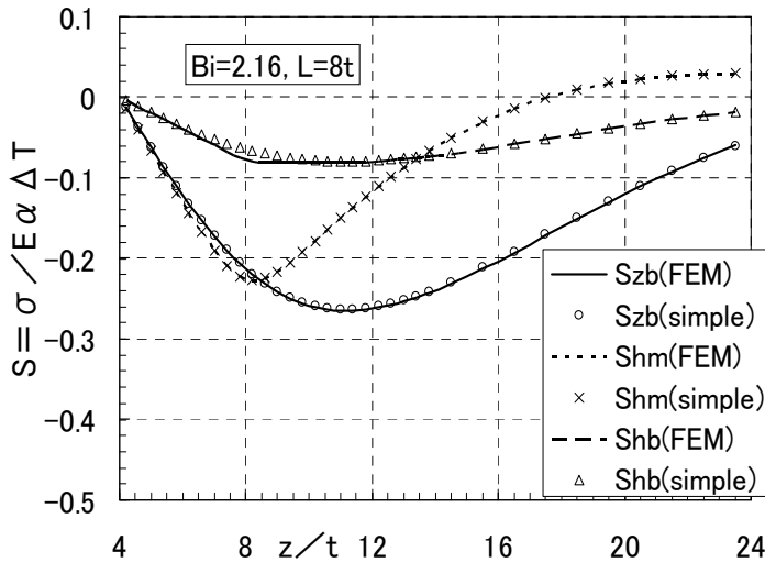
Fig. 7. Thermal stresses for ramp-shaped fluid temperature
