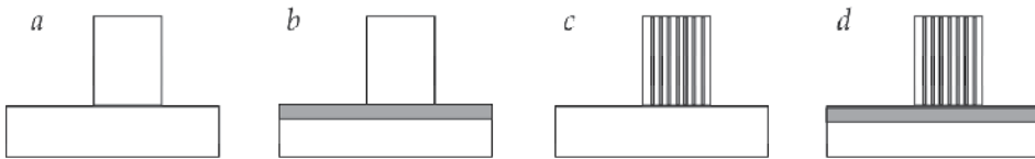
Fig. 10. Configuration of calculation regions. Homogeneous armature and rails (a), homogeneous armature and rails with a resistive layer (b), multilayer armature and homogeneous rails (c), and multilayer armature and rails with a resistive layer (d).
