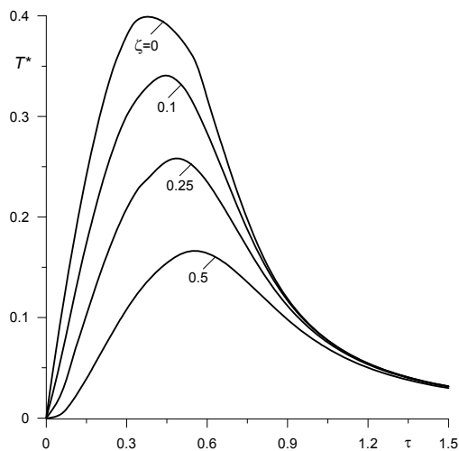
Fig. 18. Evolution of dimensionless temperature T^* along symmetry axis \rho = 0 for different values of dimensionless variable \zeta (Yevtushenko & Matysiak, 2005).
