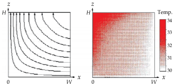
a) Flow stream line in right half b) Temperature distribution in right half,
