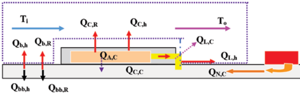
Figure 9. Schematic diagram for airflow channel.
