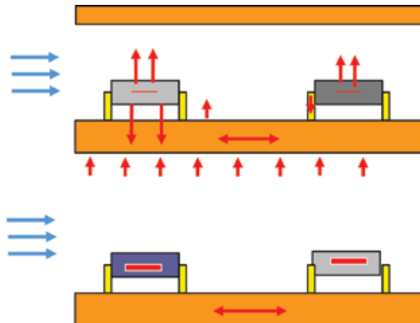
Figure 3. Heat transfer mechanism between each PWB.
