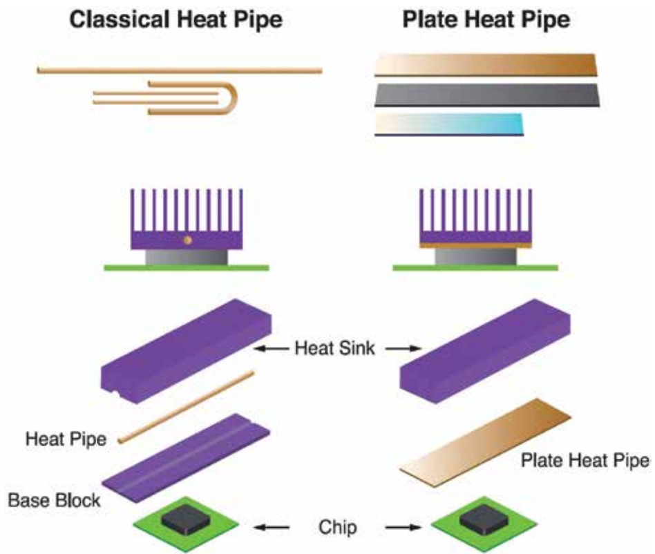
Figure 15. Use of tubular heat pipe and flat-plate heat pipe.
