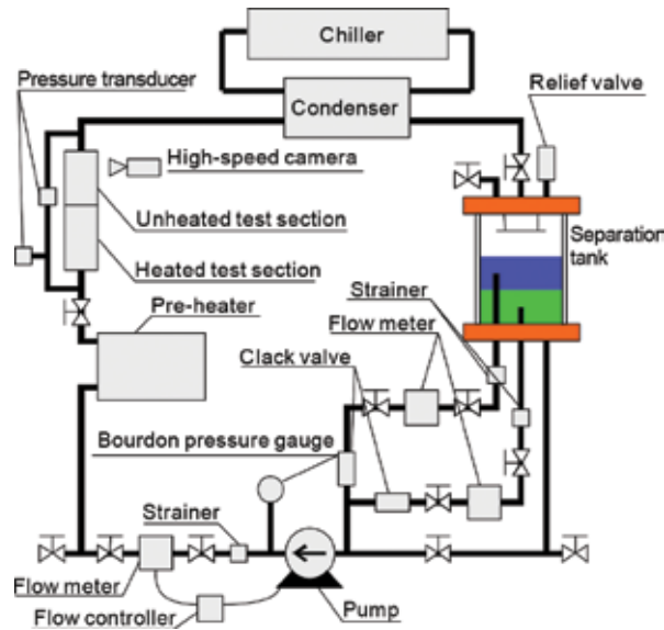
Figure 11. Outline of test section [21].
