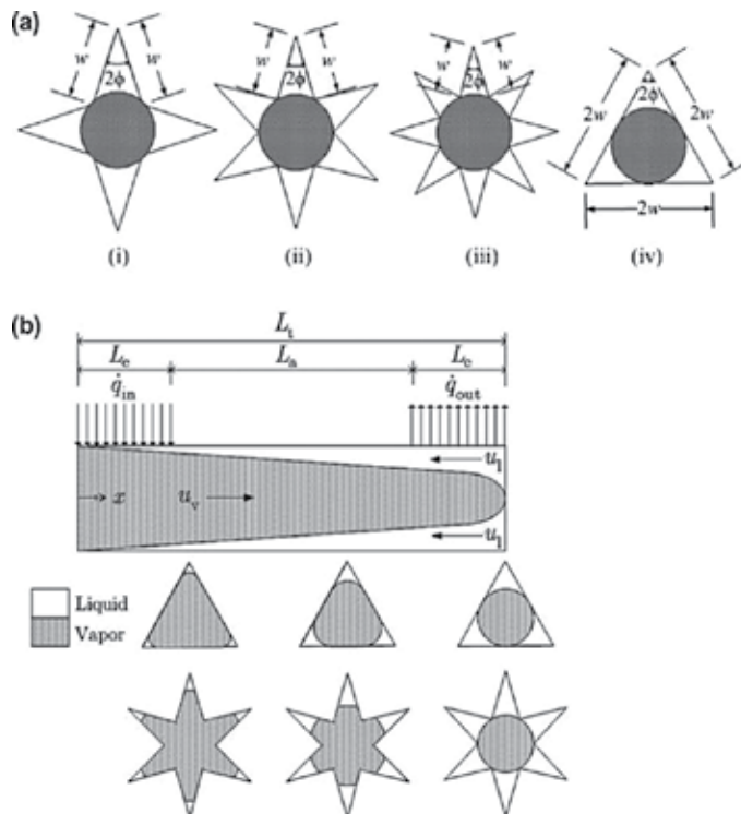
Figure 7. (a) Geometry of different cross-sectional shapes of micro-heat pipe: (i) square star groove, (ii) hexagonal star groove, (iii) octagonal star groove, and (iv) equilateral triangle. (b) Schematic diagram of optimally charged equilateral triangular and star-groove micro-heat pipes [29].
