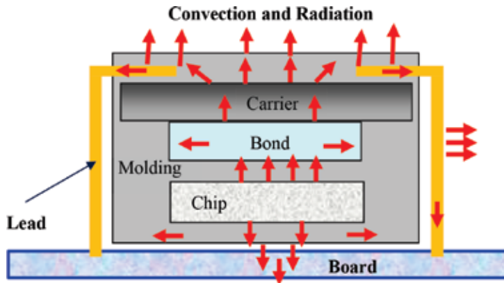
Figure 1. Heat transfer mechanism process of the chip for the upper part.
