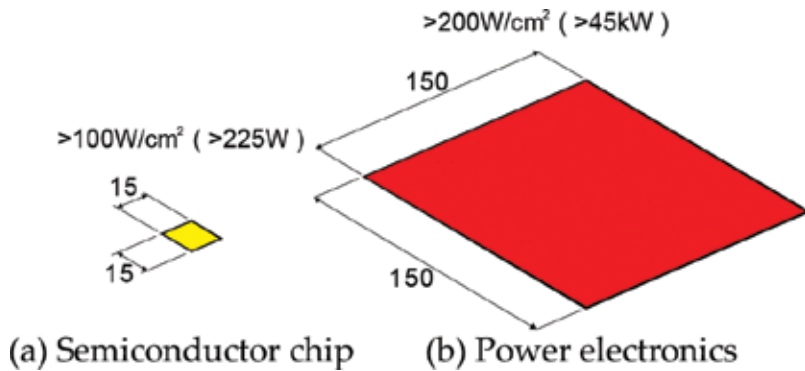
Figure 1. Difference in the size and heat flux level of semiconductors as a target of cooling.
