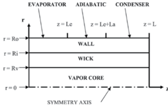
Figure 9. Coordinate system of the heat pipe [38].
