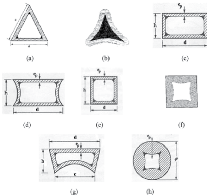
Figure 2. Cross-sections of individual micro-grooved heat pipes: (a, b) triangular section; (c, d) rectangular section; (e, f) square section; (g) trapezoidal section; (h) circular section [10].
