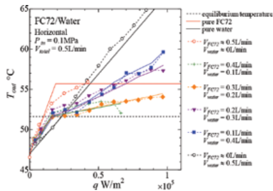
Figure 15. Outlet fluid temperature versus heat flux.
