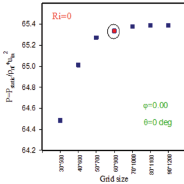
(B) Pressure drop
