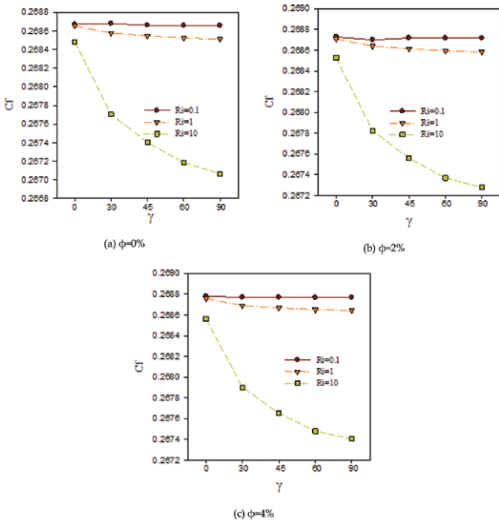
Figure 10. Average friction factor on microchannel's top wall. (A) \phi=0\% ; (B) \phi=2\% ; (C) \phi=4\% .
