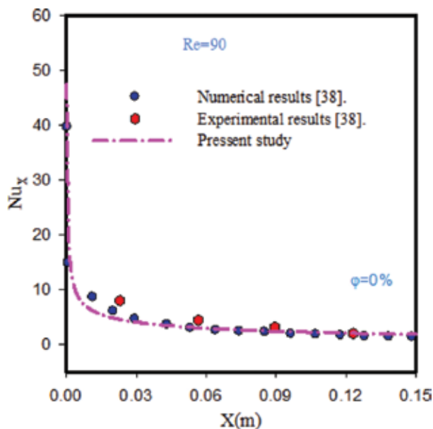
Figure 2. Local Nusselt number variation—comparison with the work of Salman et al. [38].
