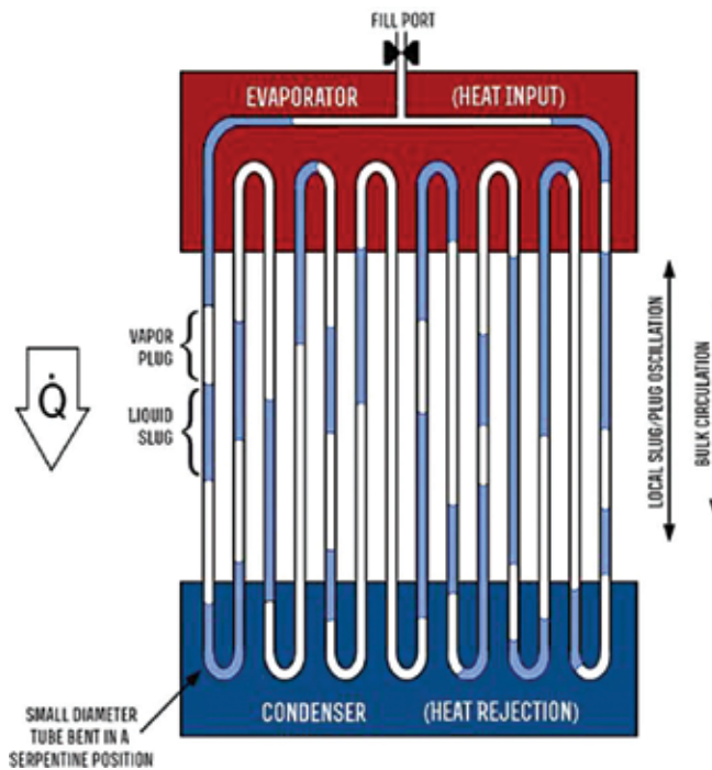
Figure 8. Schematic of an oscillating heat pipe [33].
