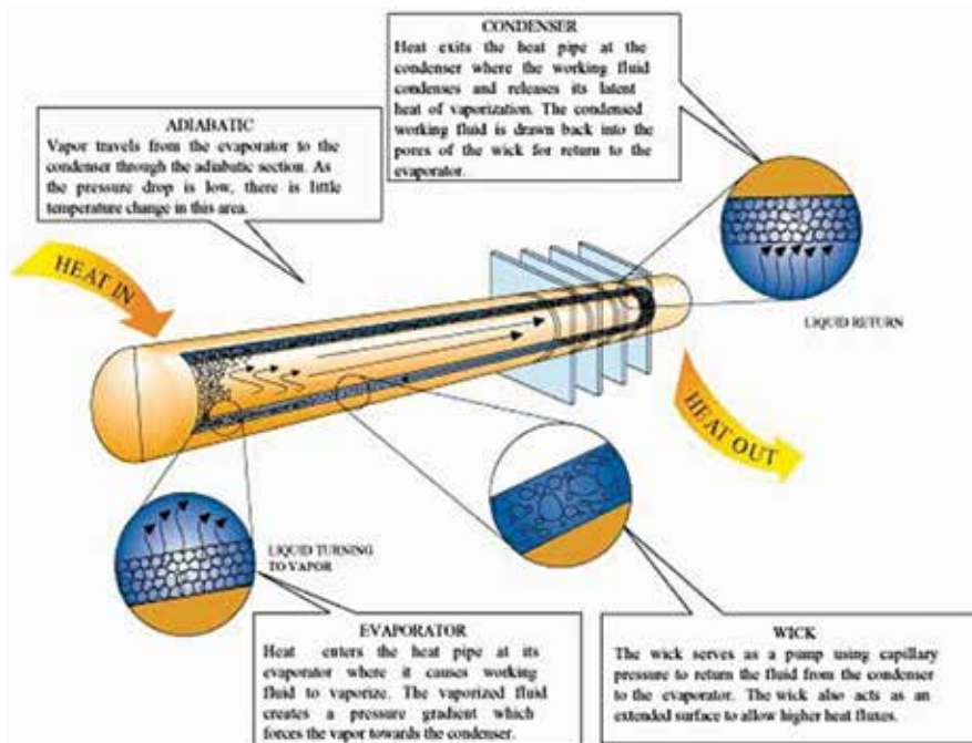
Figure 1. Heat pipe operation [10].
