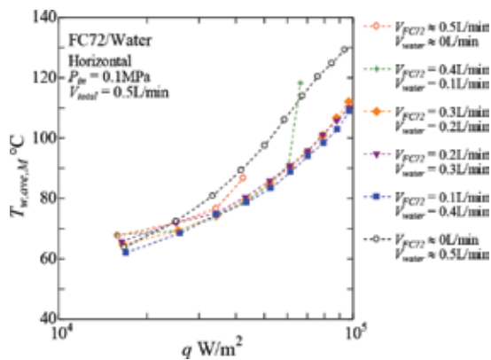
Figure 17. Wall temperature versus heat flux at midstream.
