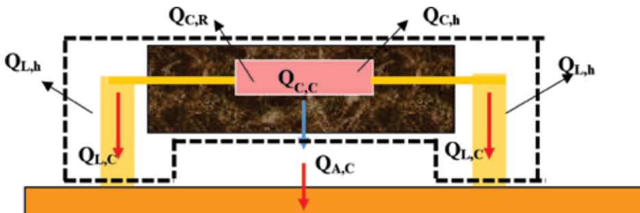
Figure 6. Heat transfer diagram outside the chip.
