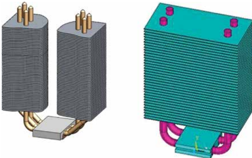
Figure 13. Finned U-shape heat pipe for desktop computer cooling [53, 54]. (a) Finned U-shape multi-heat pipe [53]. (b) Finned U-shape twin heat pipe [54].
