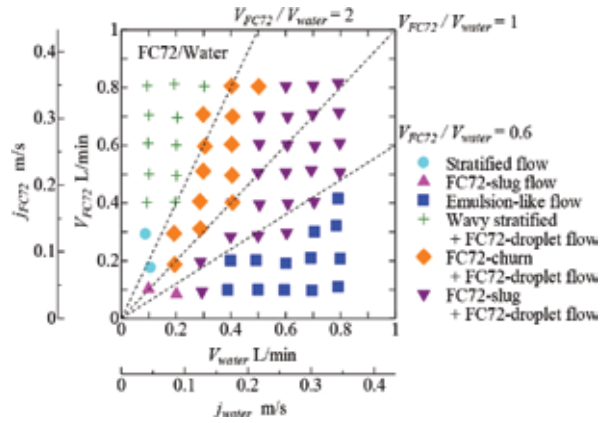
Figure 14. Flow pattern map for FC72/water. [21]
