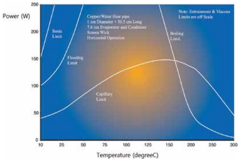
Figure 7. Performance limitations with respect to the temperature.
