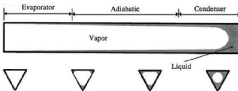
Figure 3. Schematic diagram of a micro-heat pipe with triangular cross-section.
