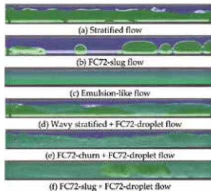
Figure 13. Typical flow patterns of FC72/water [21].
