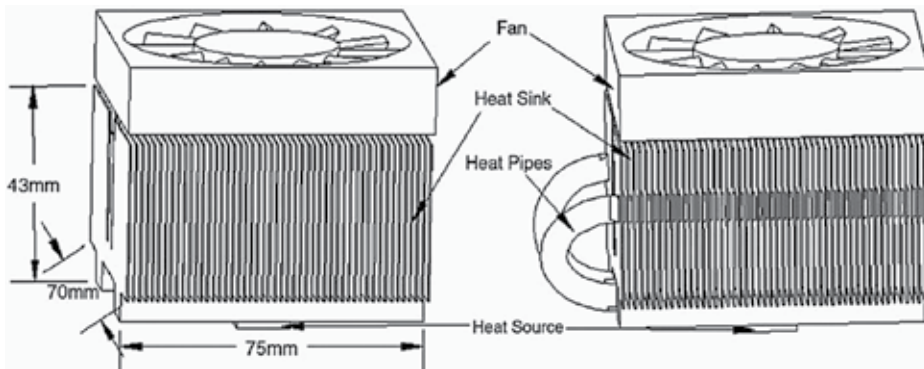
Figure 12. Heat sink without and with embedded heat pipes [50].
