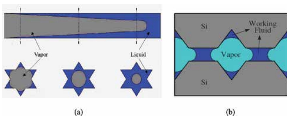
Figure 7. Schematic diagram of star grooves MHP (a) and rhombus grooves MHP (b) [37].
