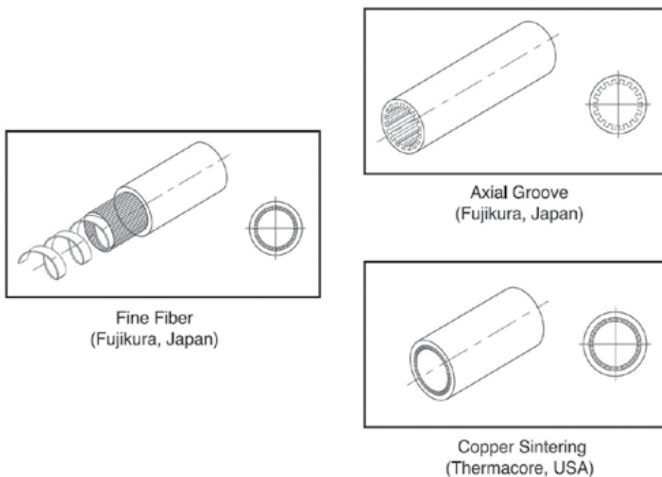
Figure 5. Typical wick structures.
