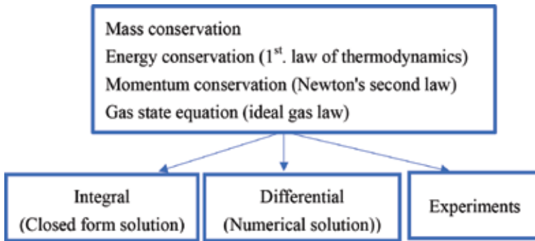
Figure 5. Three methods for solving heat-dissipated problems.
