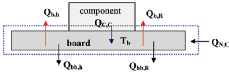
Figure 10. Schematic of chip on board.
