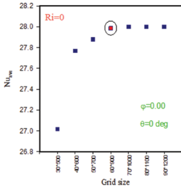
(A) Average Nusselt number
