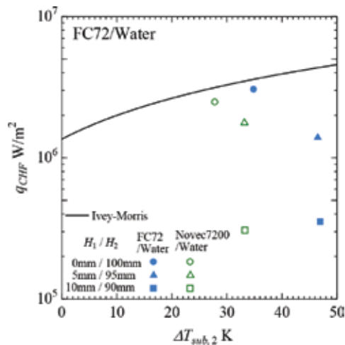
Figure 9. The comparison of CHF data with predicted values for subcooled boiling of less-volatile liquid.
