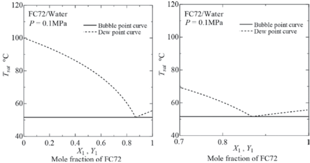
Figure 3. Phase equilibrium diagram of FC72/water mixture.
