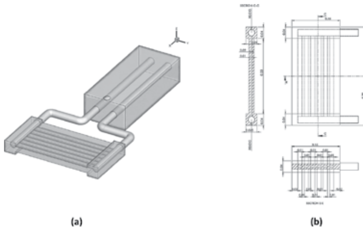
Figure 6. (a) 3D geometry of the cooling loops and (b) key dimensions.
