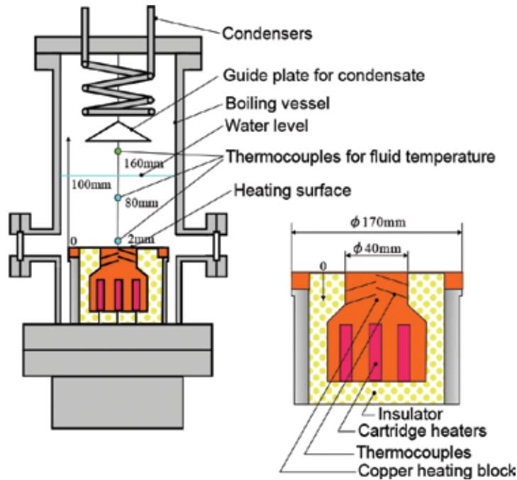
Figure 5. Outline of pool boiling experimental apparatus.
