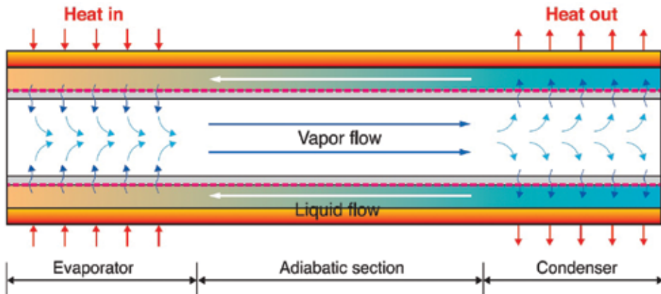
Figure 4. Working principle of heat pipe.
