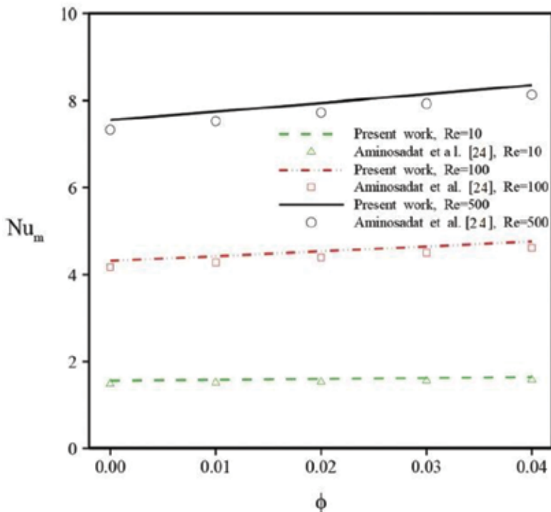
Figure 3. Averaged Nusselt number from present work versus that of Aminossadati et al. [24] for different values of Re and \phi .
