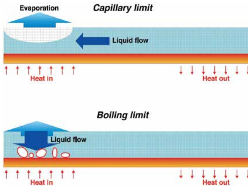
Figure 8. Capillary limit and boiling limit.
