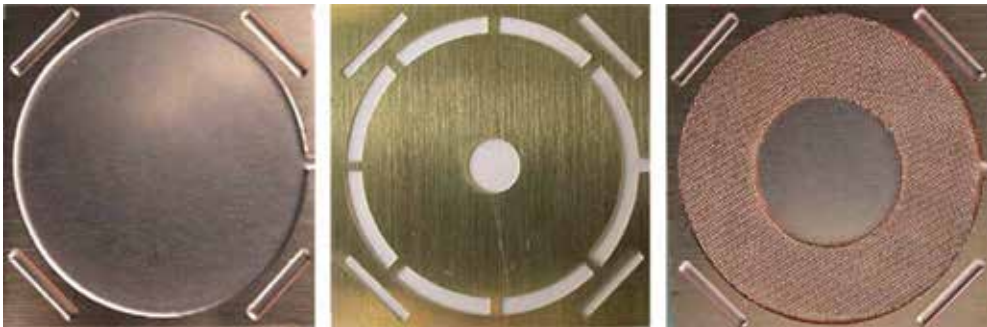
Figure 12. The diagram about the structures of each layer of a copper-screen-styled micro-heat pipe heat spreader: gas phase (left); partition panel (central); liquid phase (right) [59].
