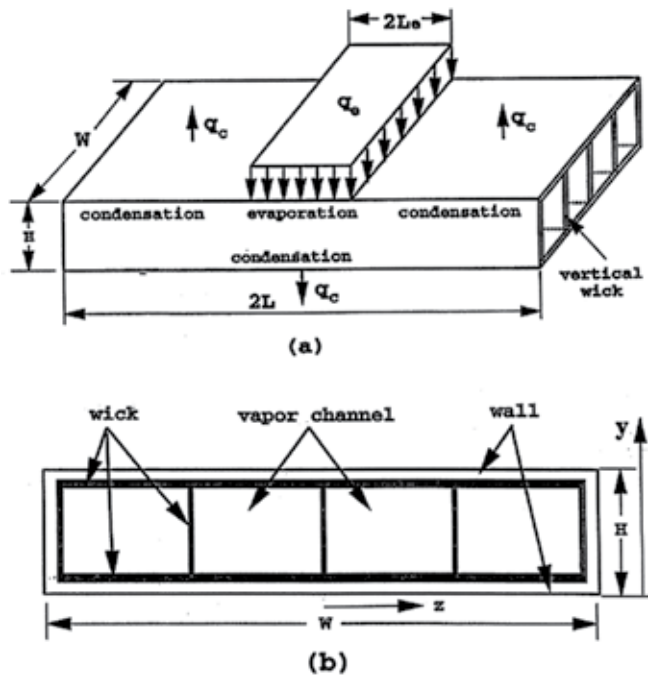
Figure 6. Schematic of the flat plate heat pipe: (a) geometry of the heat pipe and (b) cross-sectional view of the heat pipe [27].
