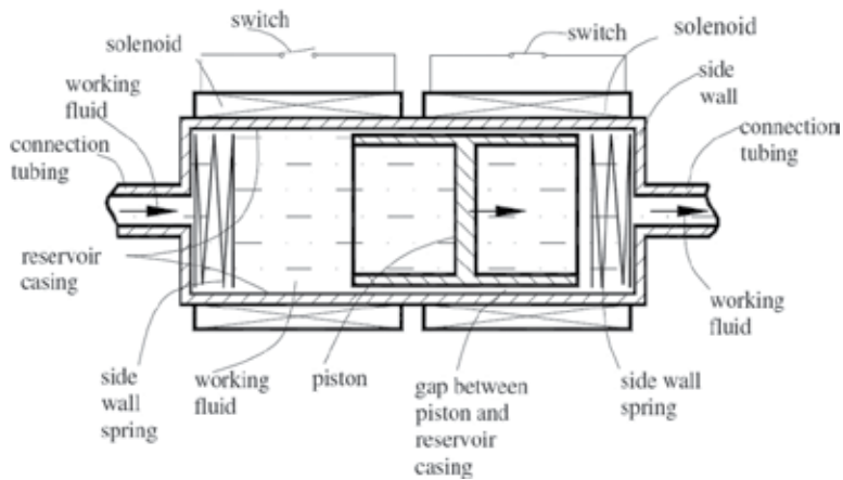
Figure 3. Schematic of a solenoid driver integrated with the liquid reservoir [12].
