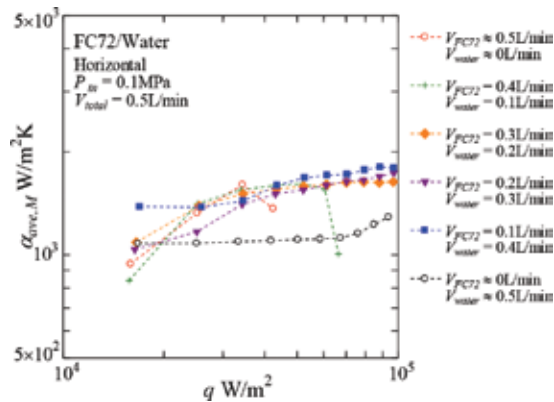
Figure 16. Heat transfer coefficient versus heat flux at midstream.
