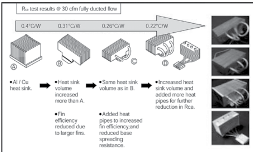
Figure 10. Heat pipe heat sink solution for cooling desktop PCs [47].
