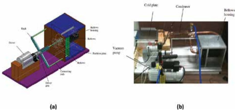
Figure 2. (a) Configuration of the designed bellows/driver assembly. (b) A photo of the assembled bellows-type heat loop being evacuated [9].
