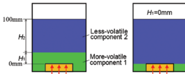
Figure 6. Condition representing volume ratio of immiscible liquids [9].
