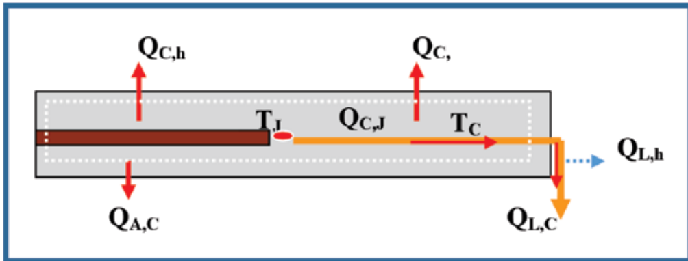
Figure 8. Junction temperature and heat transfer diagram inside the chip.
