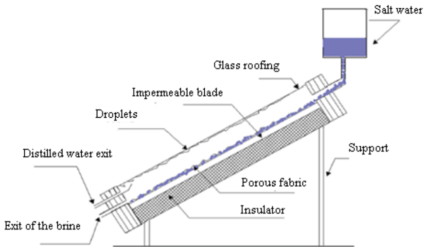
Fig. 4. Solar distiller with wick
