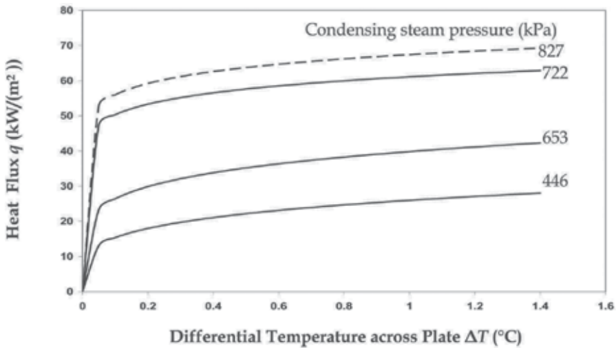
Fig. 5. Heat flux across the plate corresponding to different \Delta T . Forced convection in saturated pool boiling. R is the optimal corresponding value (Figures 4). Smooth curves were calculated using Equations 12 to 14. Dashed line is a projection to desired operating pressure using Equations 15 to 19. (Lara & Holtzapple, 2010)
