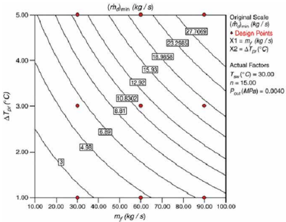
Fig. 7. Contour of minimum distilled water for N=15 , T_{sw}=30^\circ\text{C} , P_{out}=0.004\text{MPa}
