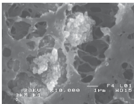
Fig. 8. SEM images of deposits formed inside the large pores (3-5 \mu\text{m} of diameter)
