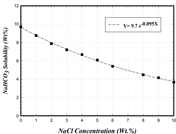
Fig. 5.3. Effect of \text{NaCl} on the solubility of \text{NaHCO}_3 at 25 °C
