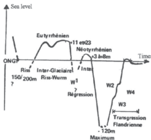
Fig. 13. Fluctuations of sea level in the Pleistocene period (Bonifay et al., 1974).
