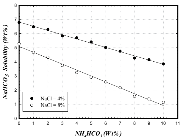
Fig. 5.4. Effect of NH_4HCO_3 on the solubility of NaHCO_3 at 25 °C
