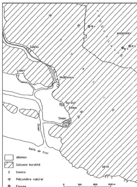
Fig. 16. Outflow area of Kras aquifer (Krivic, 1982).
