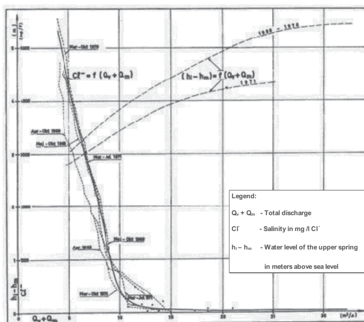
Fig. 6. Almyros Irakliou spring in Greece. Relation between discharge, water level and salinity (Ré, 1968, published in Breznik, 1973).
