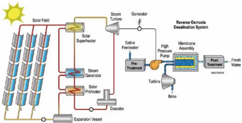
Fig. 17. Parabolic trough coupled with seawater RO desalination unit (modified from Bechtel Power)
