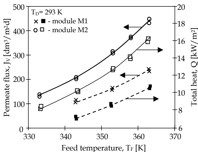
Fig. 5. Effect of feed inlet temperature and mode of membrane arrangement (M1 - parallel, irregular, M2 - braided membranes) on permeate flux and heat transfer in DCMD
