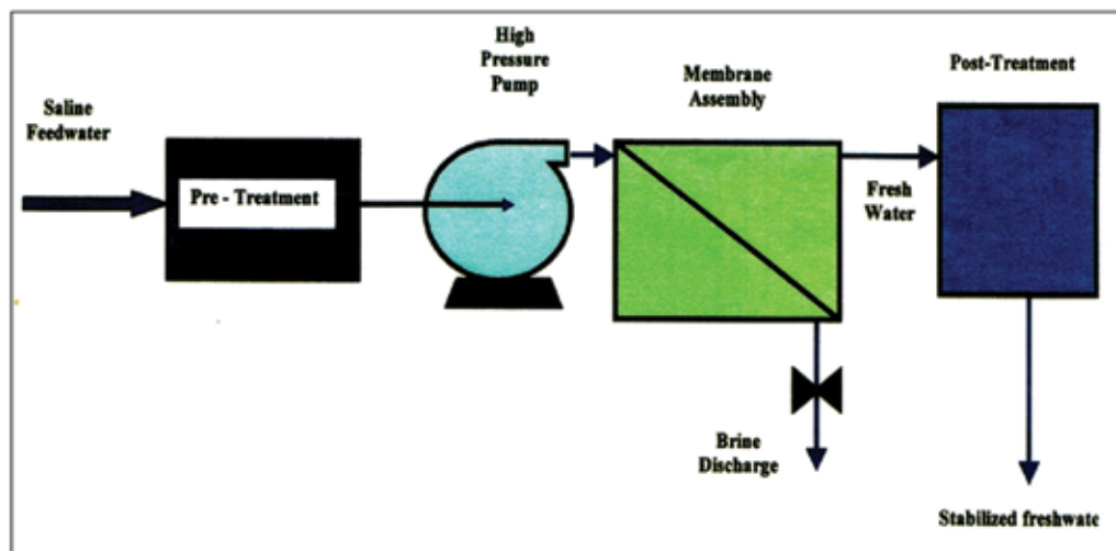
Fig. 2. Flow diagram of RO desalination process
