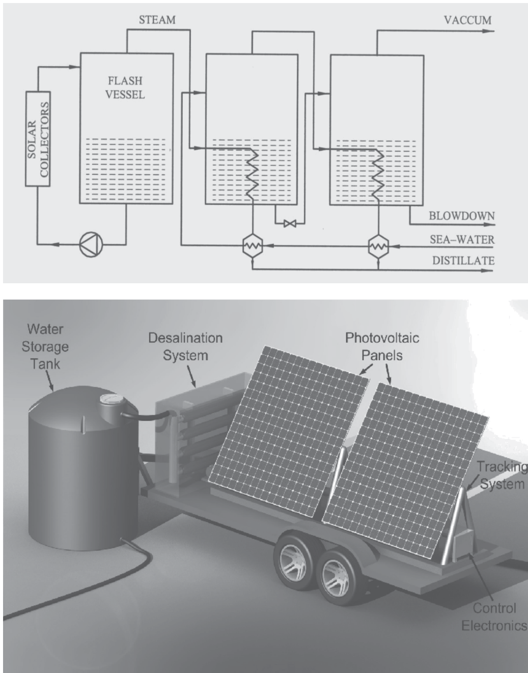
Fig. 9. a. (Top) Schematic of a multiple effect boiler (MEB) (Kalogirou (2005). 9b. (Bottom) A simple mobile solar powered reverse osmosis system (Dubowsky, 2010).
