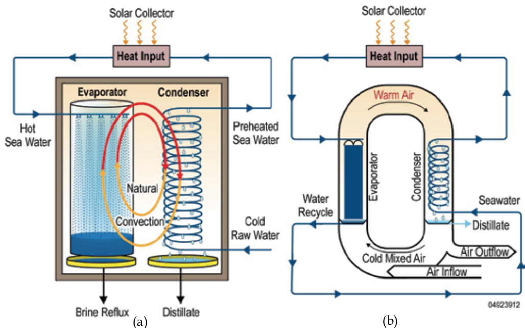
Fig. 12. Humidification-dehumidification systems: (a) open-water closed-air cycle, and (b) open-air closed-water cycle (modified from [64]).
