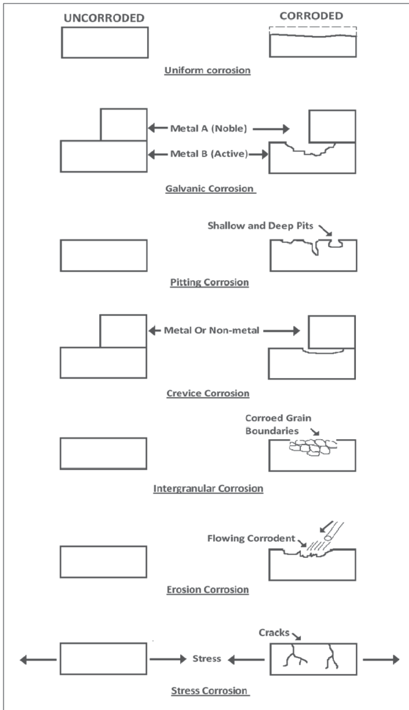
Fig. 3. Types of corrosion in desalination plants.
