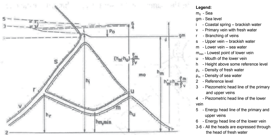
Fig. 5. Scheme of veins in the conduit type karst aquifer of a coastal spring (Breznik, 1973).
