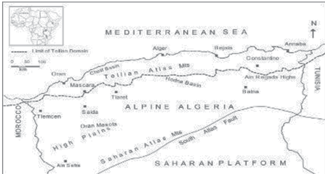
Fig. 5. a. Geological units of Northern Algeria (Mahmoudi et al., 2010; Kedaid, 2007)
