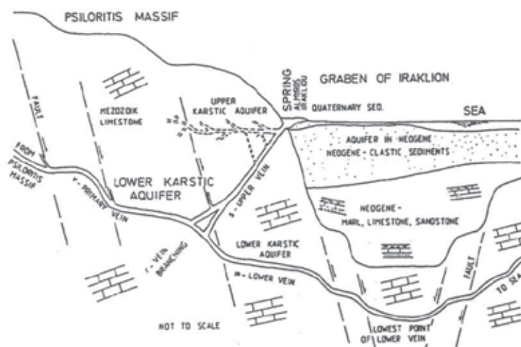
Fig. 23. Almyros Irakliou brackish spring. Main aquifers of the Psiloritis and Keri massifs and of the Irakliou graben (Breznik, 1984; 1998).
