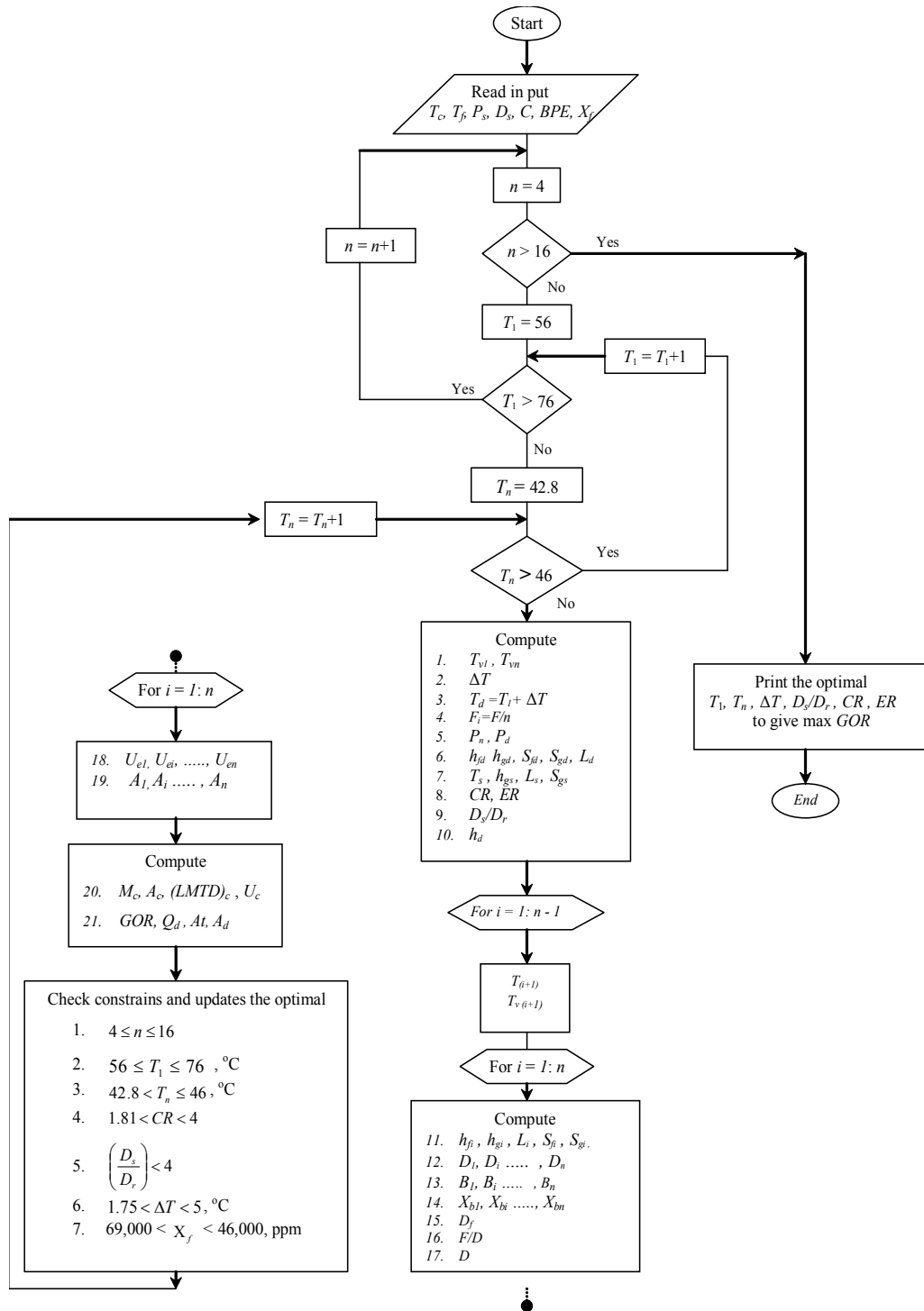
Fig. 16. Solution algorithm of the optimization problem.
