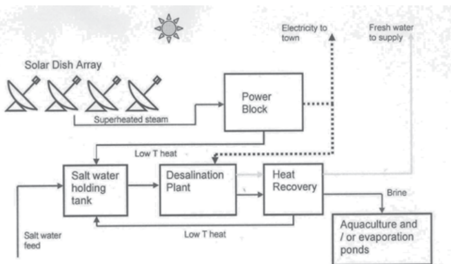
Fig. 3. Combined dish based solar thermal power generation and RO desalination (Burgess and Lovegrove, 2005)
