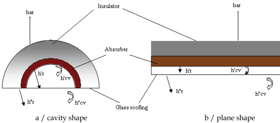
Fig. 14. Protected absorber (greenhouse effect).
