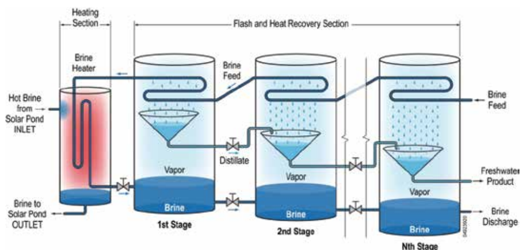
Fig. 14. MSF desalination unit operated by solar pond.
