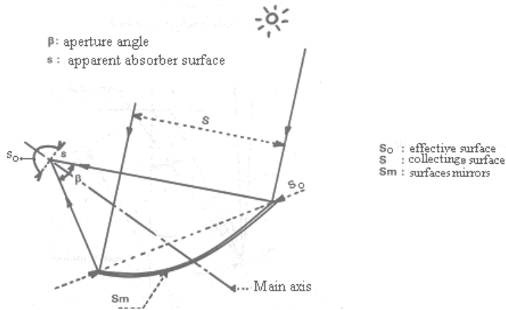
Fig. 12'. Diagram of a mirror concentrator
