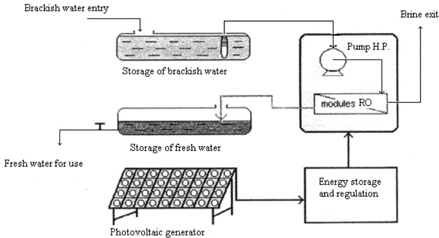
Fig. 9. Reverse osmosis desalination process
