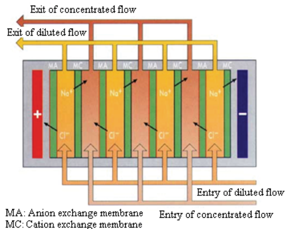
Fig. 8. Electro dialysis desalination process
