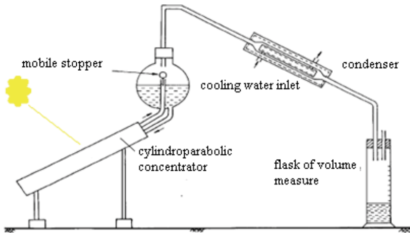
Fig. 2. Solar distiller with cylindroparabolic concentrator
