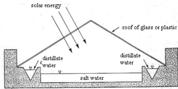
Fig. 1. Solar distillation by greenhouse effect.
