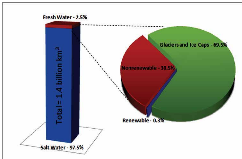
Fig. 1. Distribution of world water
