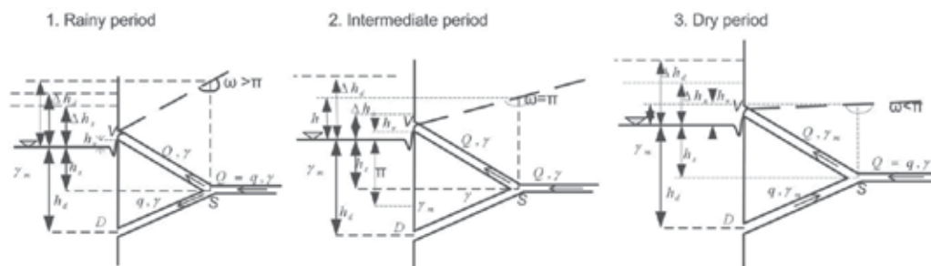
Fig. 1. Outflows of the Gurdić spring in the southern Adriatic (Gjurašin, 1943).
