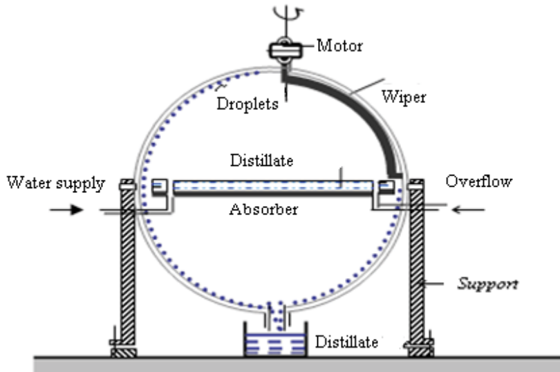
Fig. 3. Spherical solar distiller with sweeping
