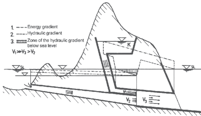
Fig. 10. "Sea water mill" on Kefalonia Island in Greece (Glanz, 1965).
