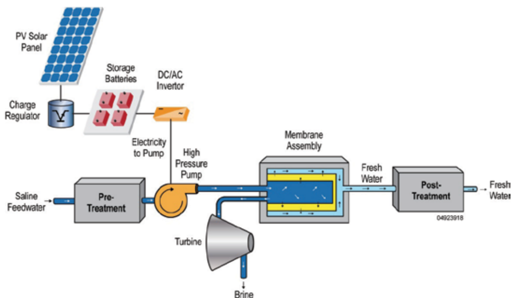
Fig. 19. Schematic of a PV/RO system.
