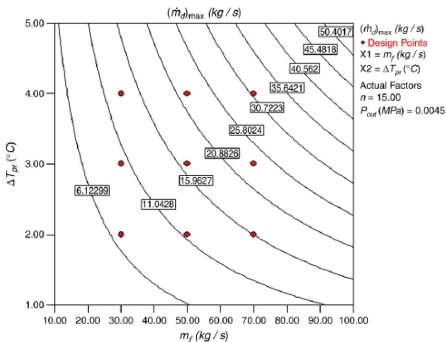
Fig. 10. Contour of maximum distilled water for N=15 , P_{out}=0.0045 MPa
