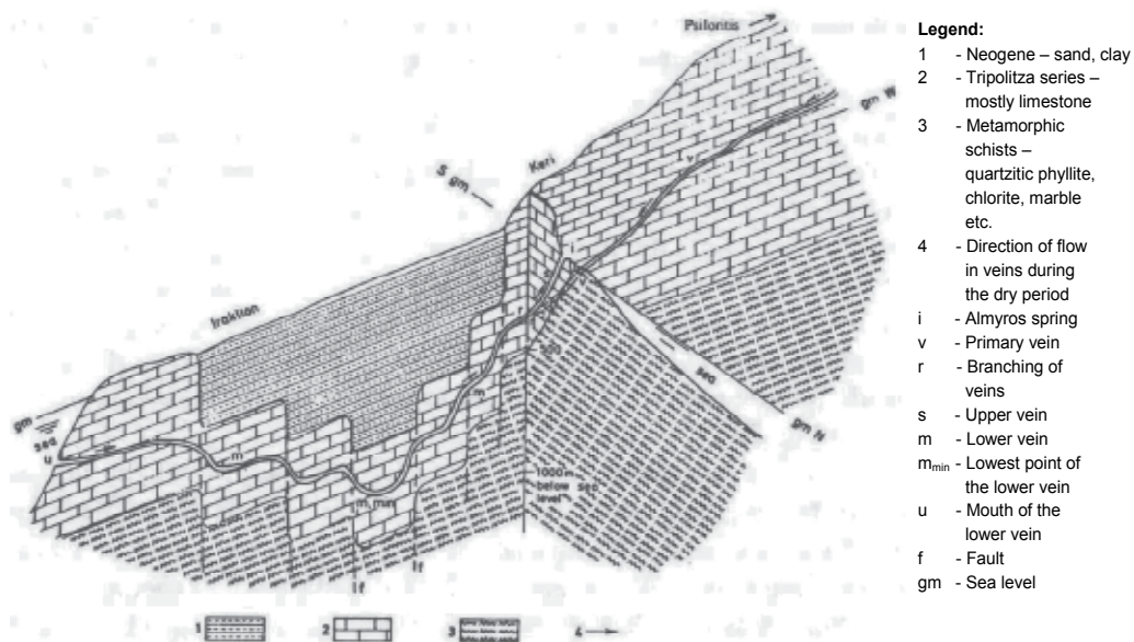
Fig. 22. Almyros Irakliou spring in Greece. Schematic geological block diagram with the supposed disposition of the spring veins in the conduit-flow karstic aquifer (Breznik, 1978).
