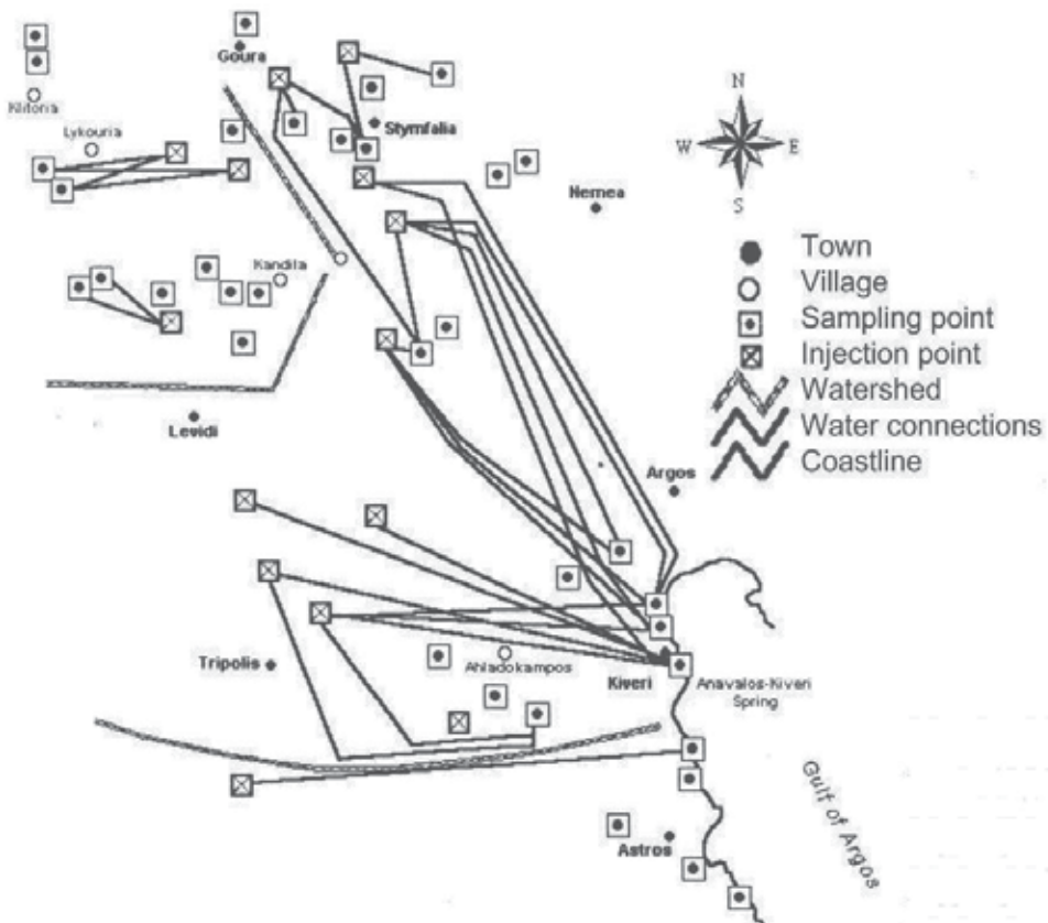
Fig. 19. Underground water connections of the Peloponnese, found by tracing experiments (Gospodarič & Leibungut, 1986).
