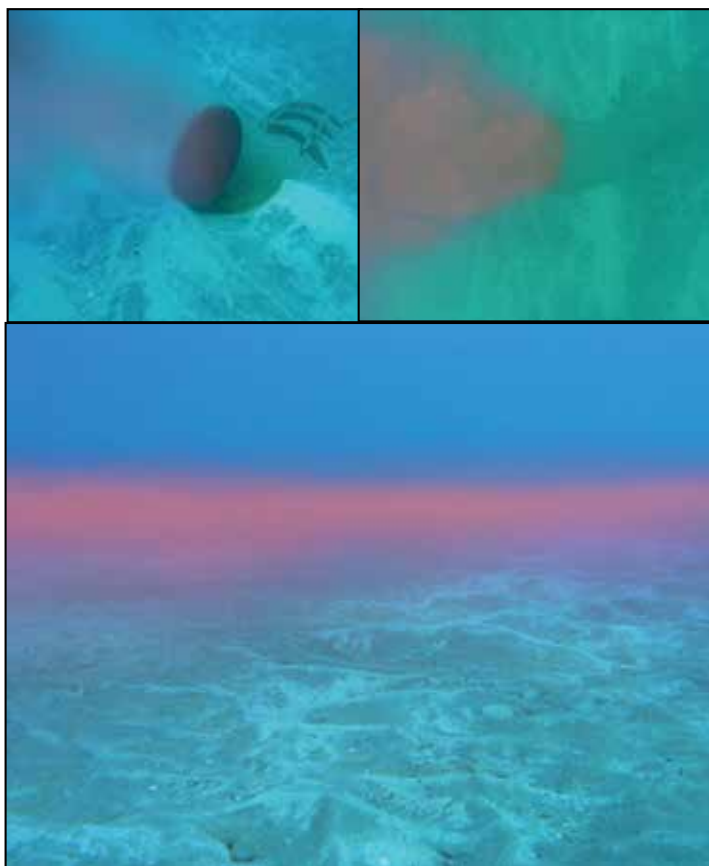
Fig. 2. Pictures from an ad hoc brine discharge dyed by rhodamine in Maspalomas beach. Near (upper panel) and Far field (lower panel) regions can be observed.
