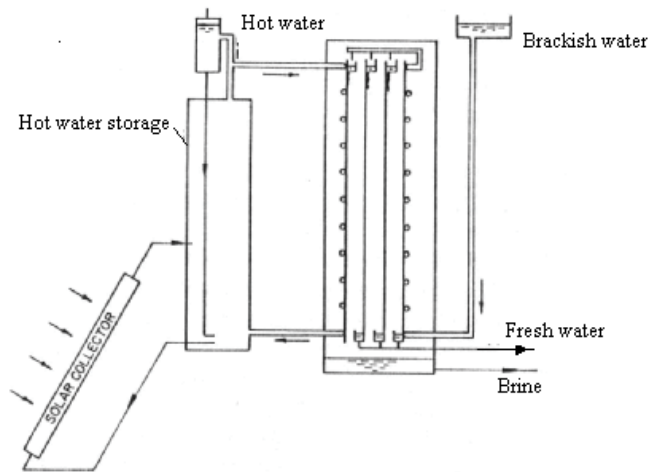
Fig. 7. Multiple effects solar distillation.
