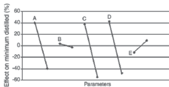
Fig. 3. Response of first DOE for minimum distilled water
