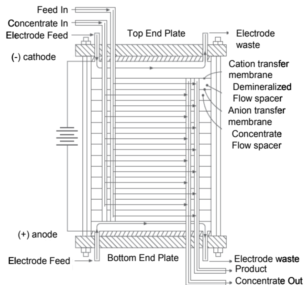
Fig. 2. Stack description (Ionics Inc., 1984)
