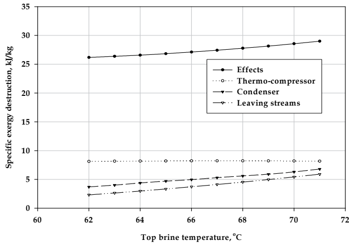
Fig. 10. The effect of top brine temperature on the specific exergy destruction in different components of Al-Jubail ME-TVC unit.
