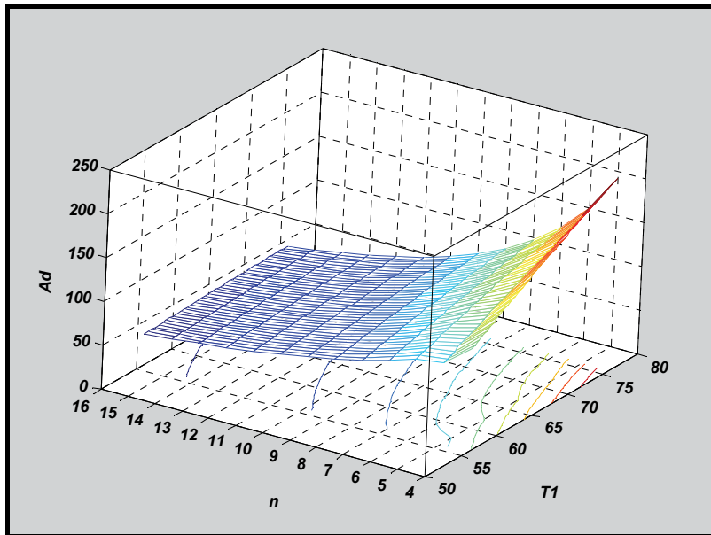
Fig. 18. The impact of top brine temperature and the number of effects on the specific energy consumption.
