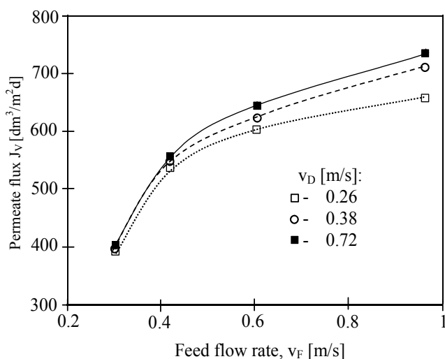
Fig. 4. The effect of the flow rate of streams in a module with braided membranes (module M1) on the permeate flux. T_F = 353 K, T_D = 293 K
