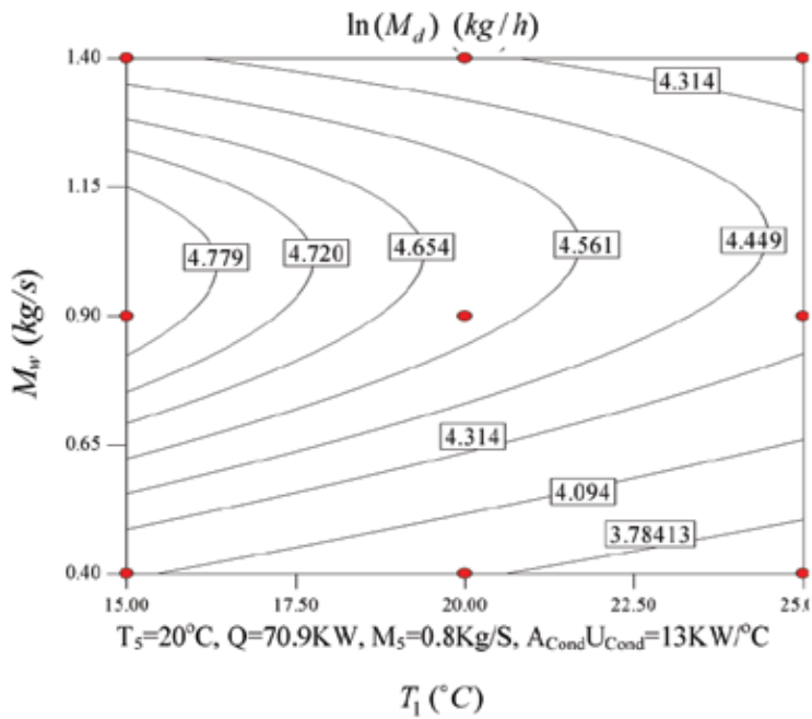
Fig. 16. Contour of the inlet water temperature and its mass flow rate on the fresh water production.
