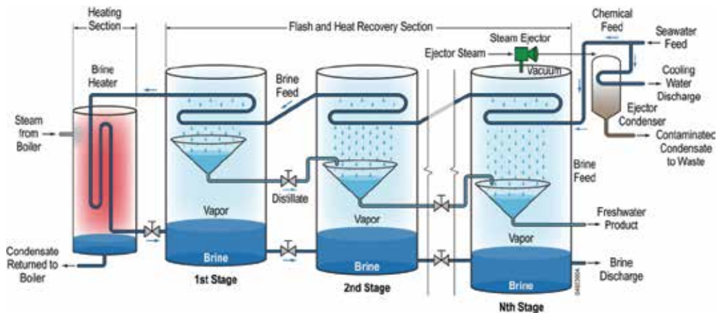
Fig. 4. Diagram of typical MSF unit (modified from [7])
