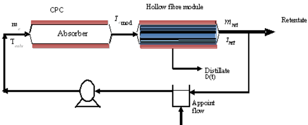
Fig. 10. Diagram of the desalination unit
