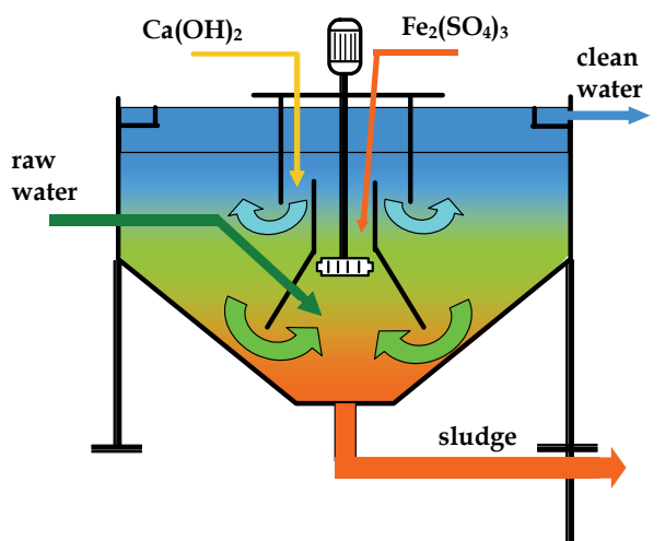
Fig. 12. Water treatment using the contact clarifiers (accelerator)
