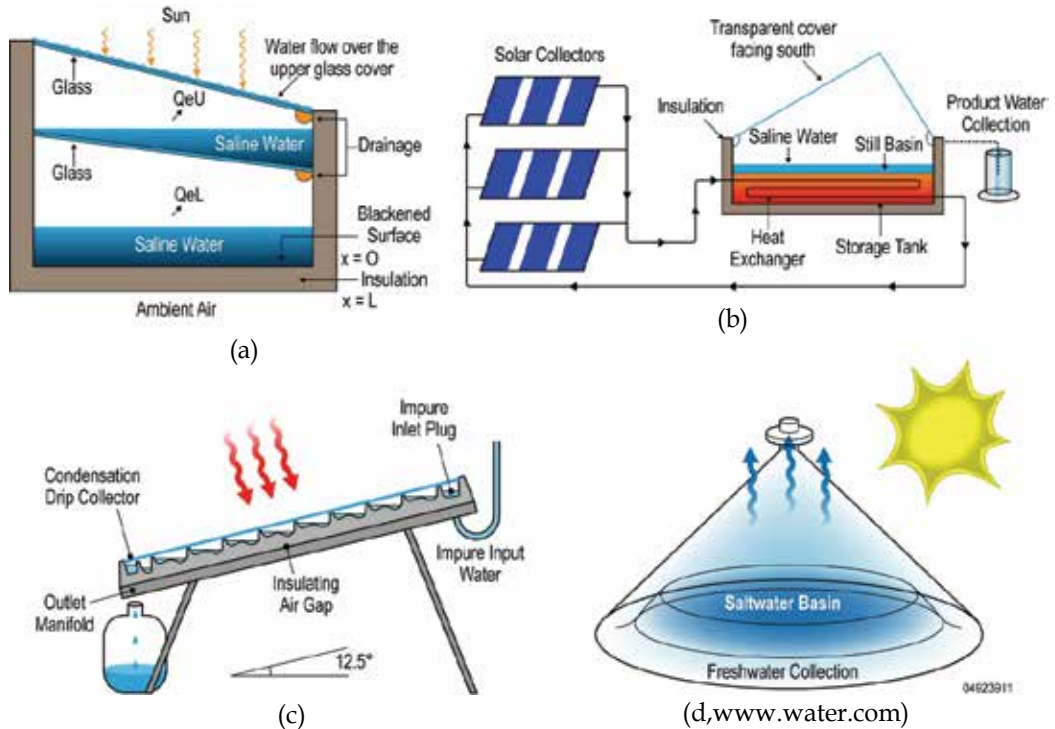
Fig. 11. Diagrams of various solar stills: (a) double-basin solar still, (b) single-basin solar still coupled with flat plate collector, (c) multi-steps tilted solar still, (d) micro-solar solar still.
