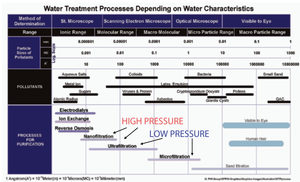
Fig. 4. Water Treatment Spectrum
