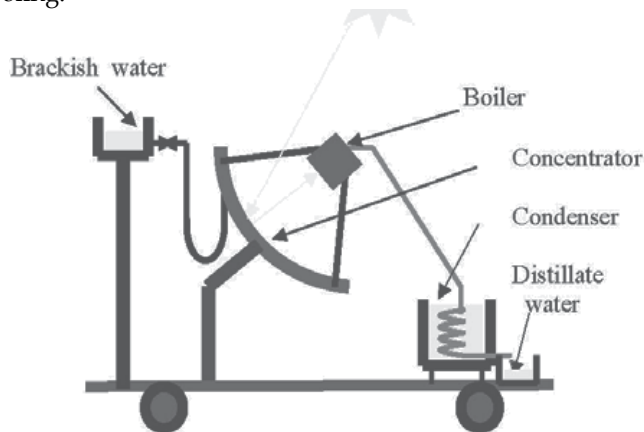
Fig. 15. Experimental device.
