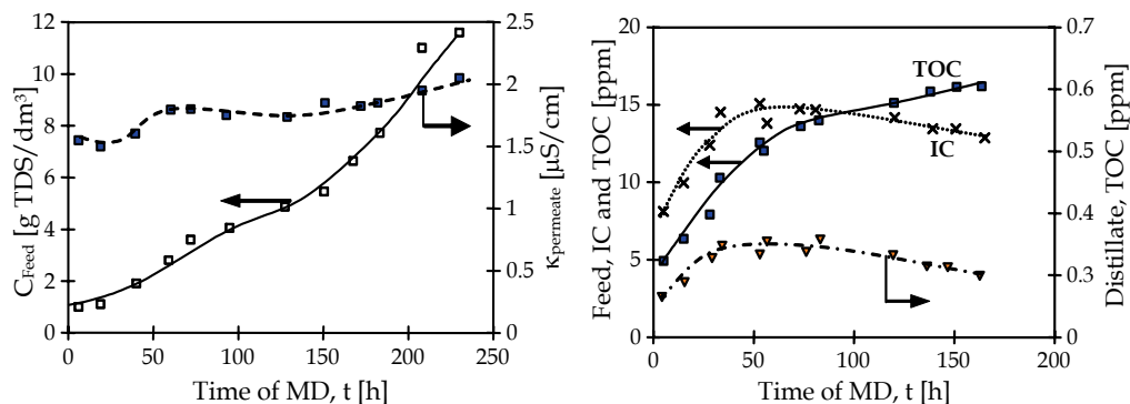
Fig. 16. Desalination of surface water by MD process
