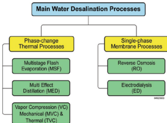
Fig. 3. Main desalination technologies.
