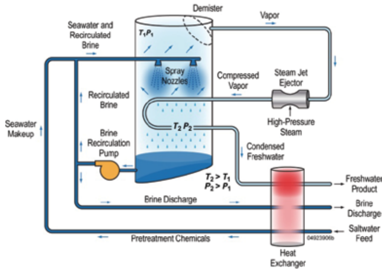
Fig. 6b. Diagram of a thermal vapor-compression plant (modified from [7])
