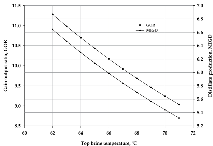
Fig. 6. The effect of top brine temperature on the distillate production and gain output ratio.
