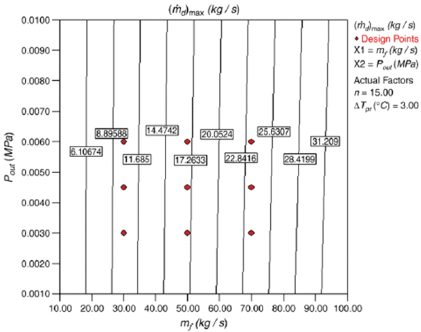
Fig. 9. Contour of maximum distilled water for N=15 , \Delta T_{pr}=3^{\circ} C
