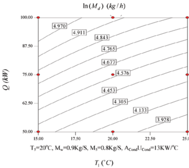
Fig. 15. Contour of feed water temperature and the given total heat flux of the cycle on the fresh water production.
