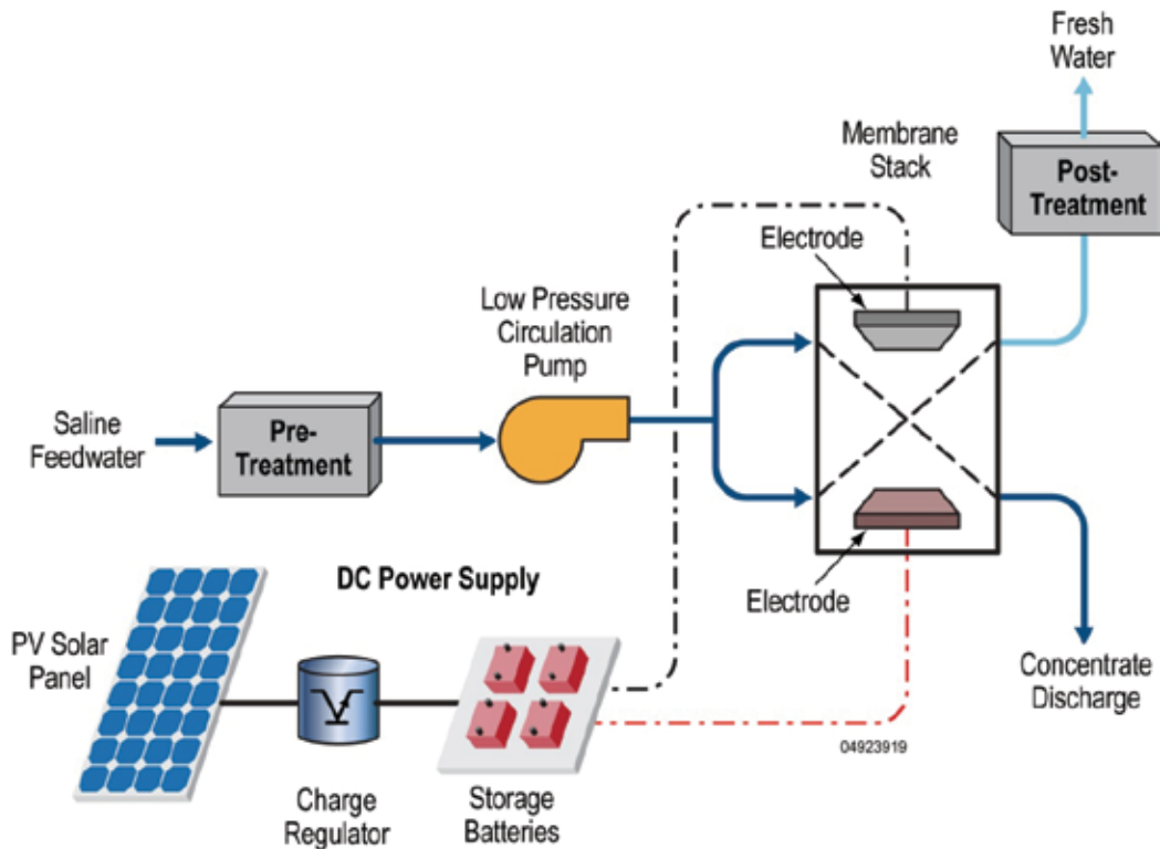
Fig. 20. Shows a schematic diagram of a PV-powered ED system.
