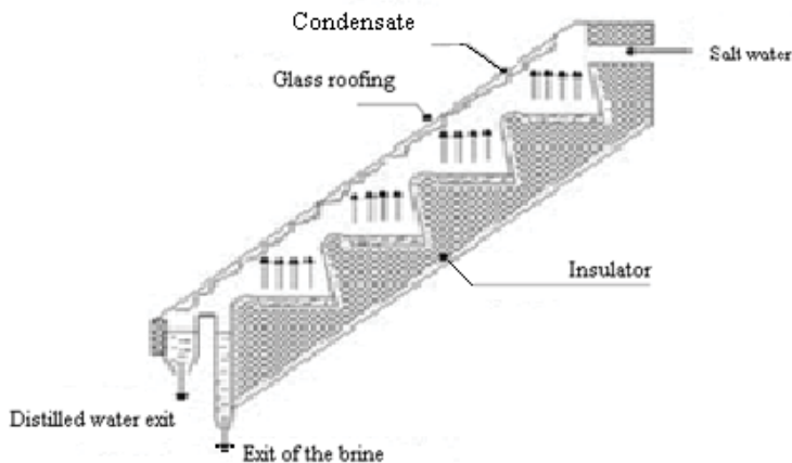
Fig. 5. Solar distiller with cascade
