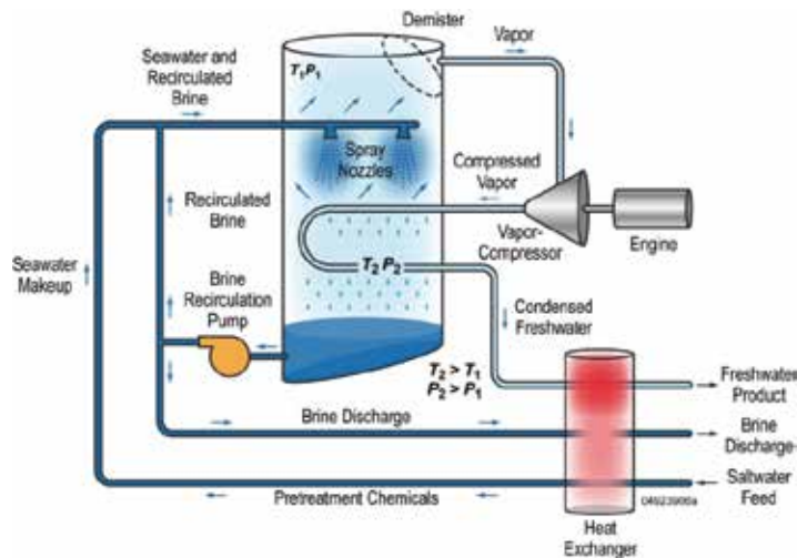
Fig. 6a. Diagram of a mechanical vapor-compression plant.
