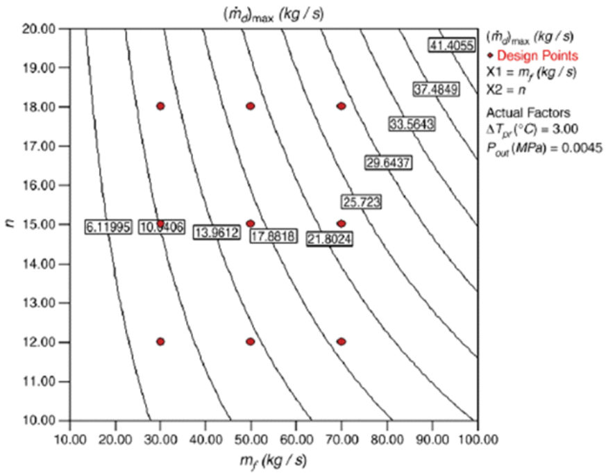
Fig. 8. Contour of maximum distilled water for T_{sw}=30^{\circ} C, \Delta T_{pr}=3^{\circ} C, P_{out}=0.004 MPa
