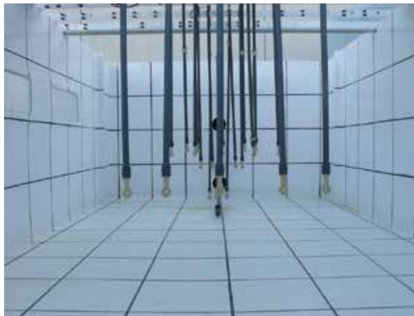
Fig. 5. Tank and gauges for brine discharge physical experiments.
