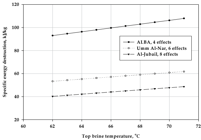
Fig. 9. The effect of top brine temperature on the specific exergy destruction for different units.
