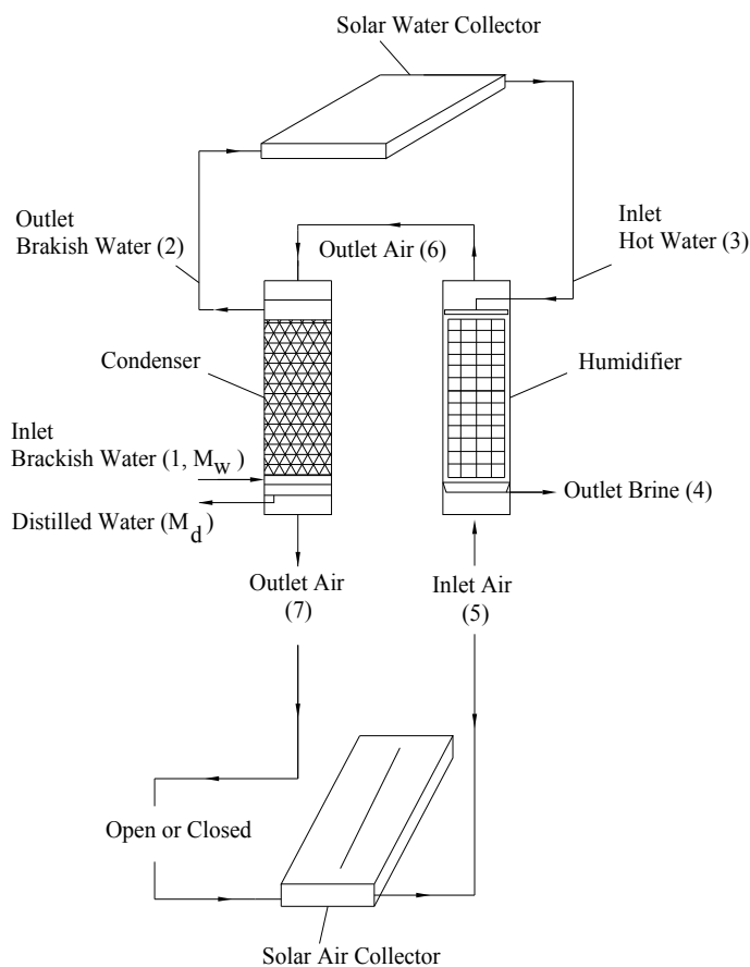
Fig. 11. Schematic of SDHD plant
