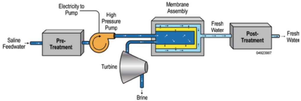
Fig. 7. Major subsystems in a reverse-osmosis system.
