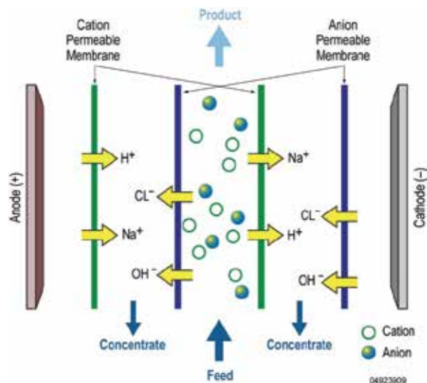
Fig. 8. Ion exchange in electrodialysis unit.
