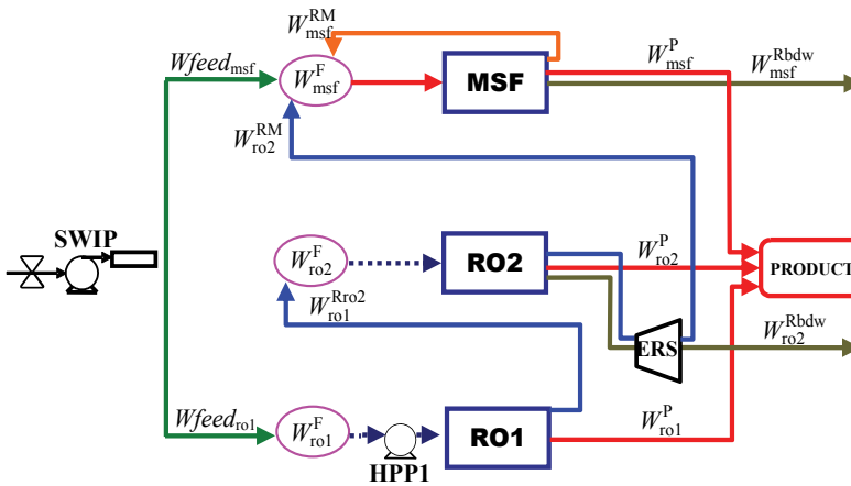
Fig. 6. Scheme of the optimal design for seawater salinities between 39000 and 45000 ppm
