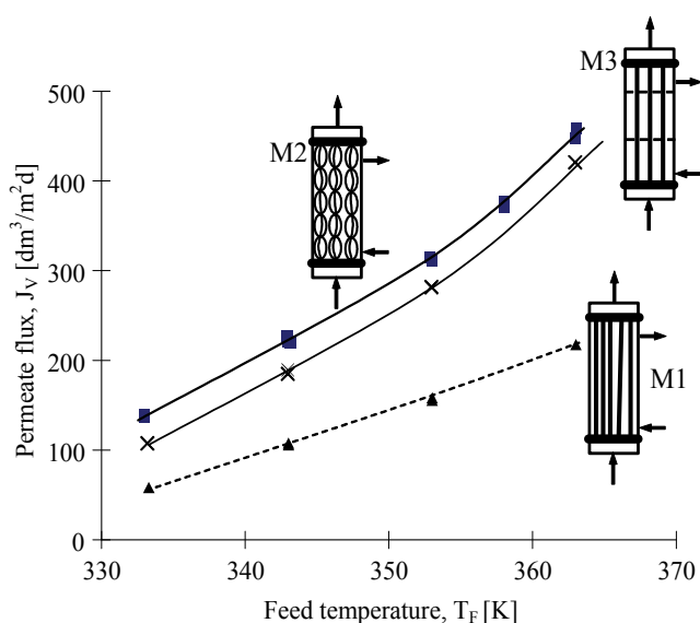
Fig. 3. The influence of feed temperature and the mode of membrane arrangement in a capillary module on the permeate flux. M1 - bundle of parallel membranes; M2 - braided capillaries; and M3 - capillaries mounted inside mesh of sieve baffles
