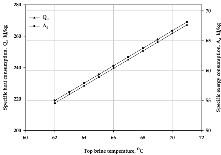
Fig. 7. The effect of top brine temperature on the specific heat consumption and specific exergy consumption.
