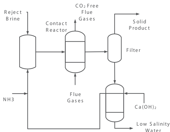
Fig. 5.5. A schematic diagram of a reject brine management process
