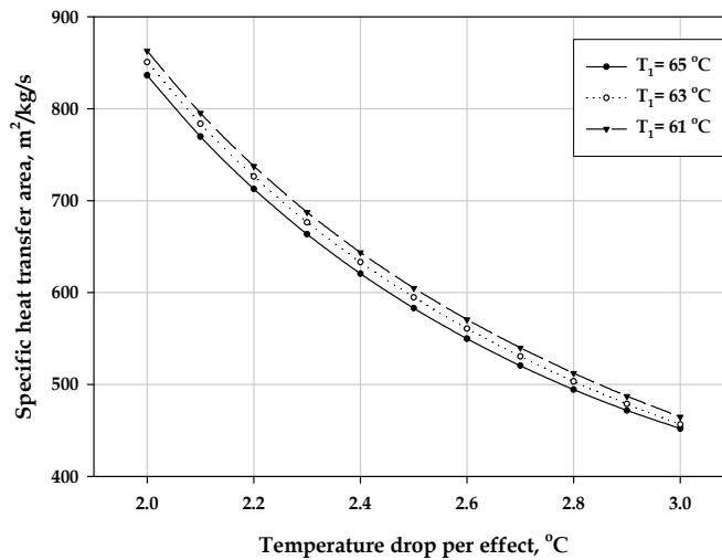
Fig. 8. The effect of temperature drop per effect on the specific heat transfer area.
