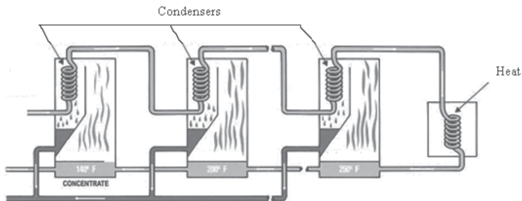
Fig. 6. Multi stage flash distiller
