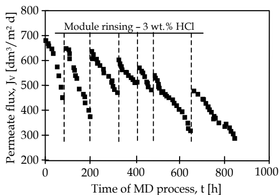
Fig. 9. Changes of the permeate flux during MD process of tap water
