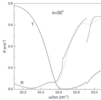
Fig. 9. Reflectivity and transmissivity versus frequency for a fixed angle of incidence of 30^\circ . After Bai, et. al. 2007.
