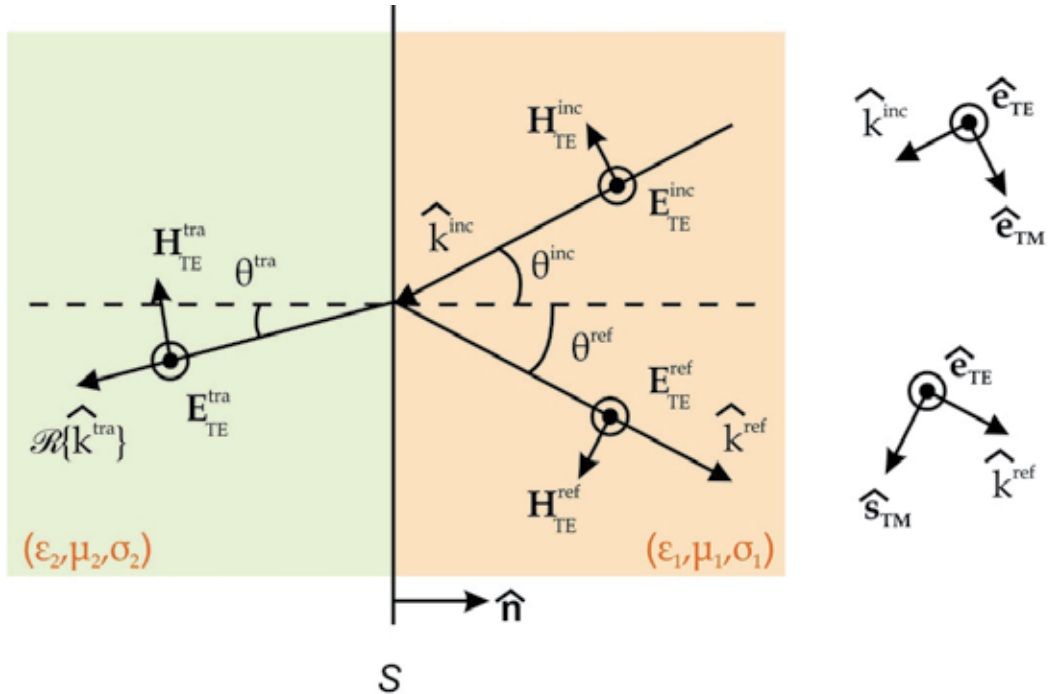
Fig. 2. Field decomposition. TE component.
