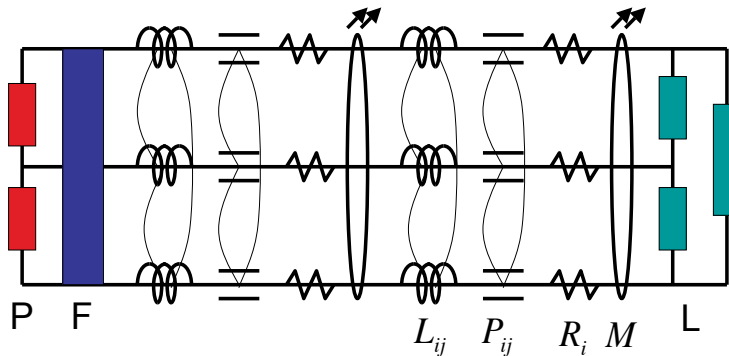
Fig. 1. A symmetrized electric circuit for the use of the normal mode decoupled from the common and antenna modes. Around the third line (middle line) two power supplies P , the filtering element F are placed in the left end and the electric loads L are placed in the right end. The connecting three-conductor transmission lines have the properties of self and mutual inductances L_{ij} denoted by coil, self and mutual coefficients of potential P_{ij} denoted by short parallel lines, resistance R_i and antenna mode coefficient M . The three-conductor transmission lines are coupled each other and their performance follows a coupled integro-differential equation with these coefficients.
