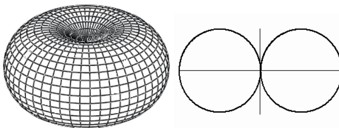
Fig. 3. Directivity diagram of the Hertzian dipole, the isotropic medium ( \epsilon = \epsilon_1 = 1 )
