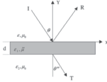
Fig. 8. Geometry and coordinate system for nonlinear reflection and transmission of an AF film with thickness d . R the reflection off and T the transmission through the film.
