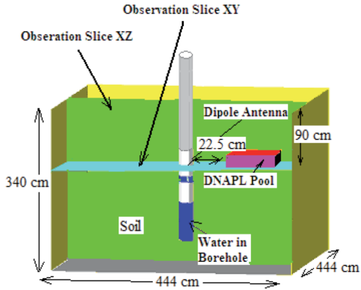
Fig. 7. Schematic representation of the borehole dipole antenna geometry and DNAPL pool ( 45 \times 45 \text{ cm} \times 15 \text{ cm} ).
