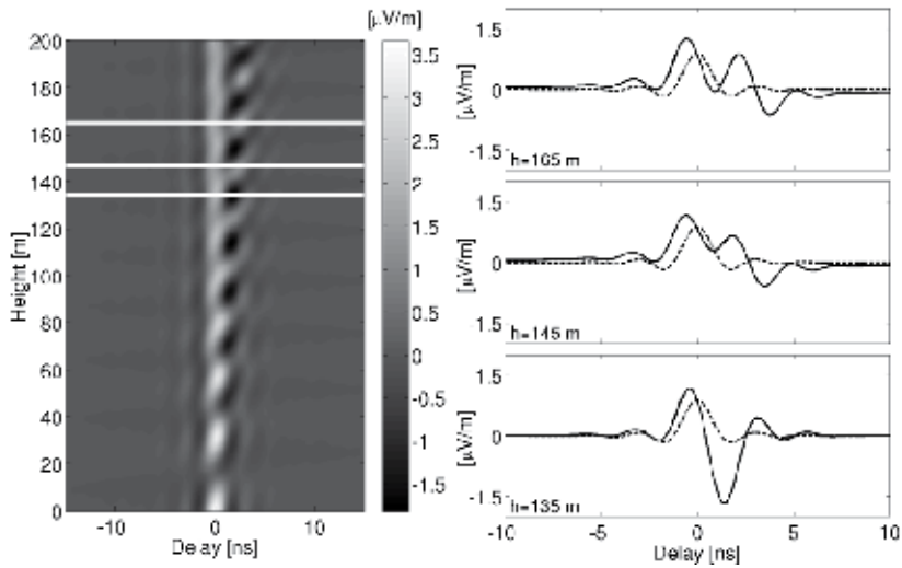
Fig. 16. Impulse response panel (left). The image on the right shows the channel response to the transmitted Nyquist wavelet at three height values, sketched as a white line in the panel on the left.
