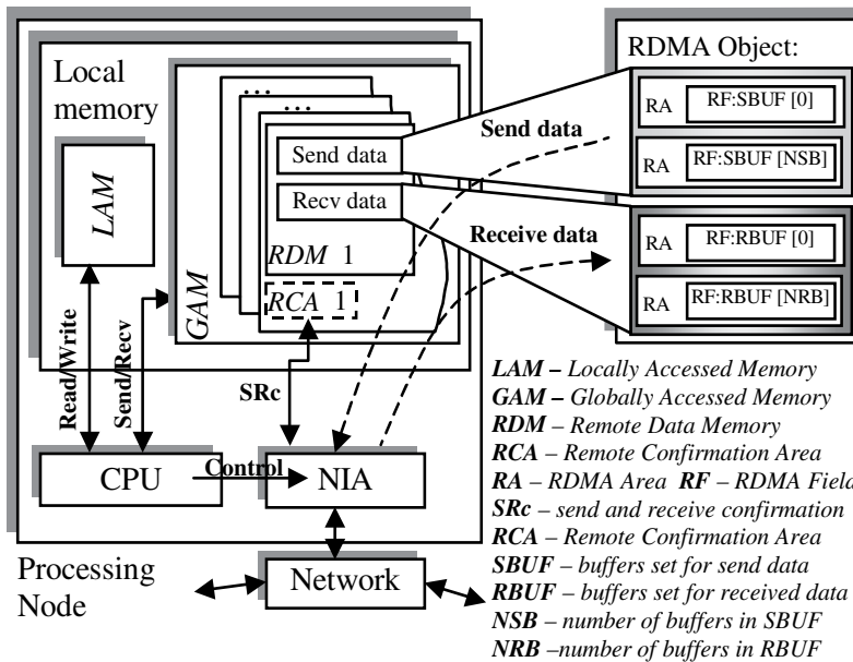
Fig. 7. Memory Structure in Rotating-Buffers Method (For One processing Node on the HITACHI SR2201 supercomputer).
