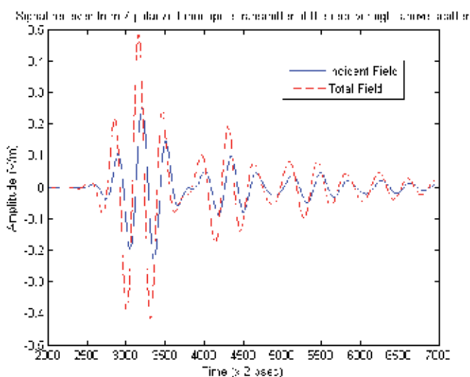
Fig. 6. Z-component of total and incident electric fields due to the monopole antenna, received at a receiver located right above the DNAPL pool.
