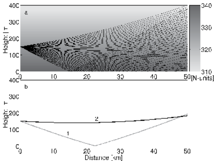
Fig. 13. Ray pattern (top) and wavefronts (bottom)
