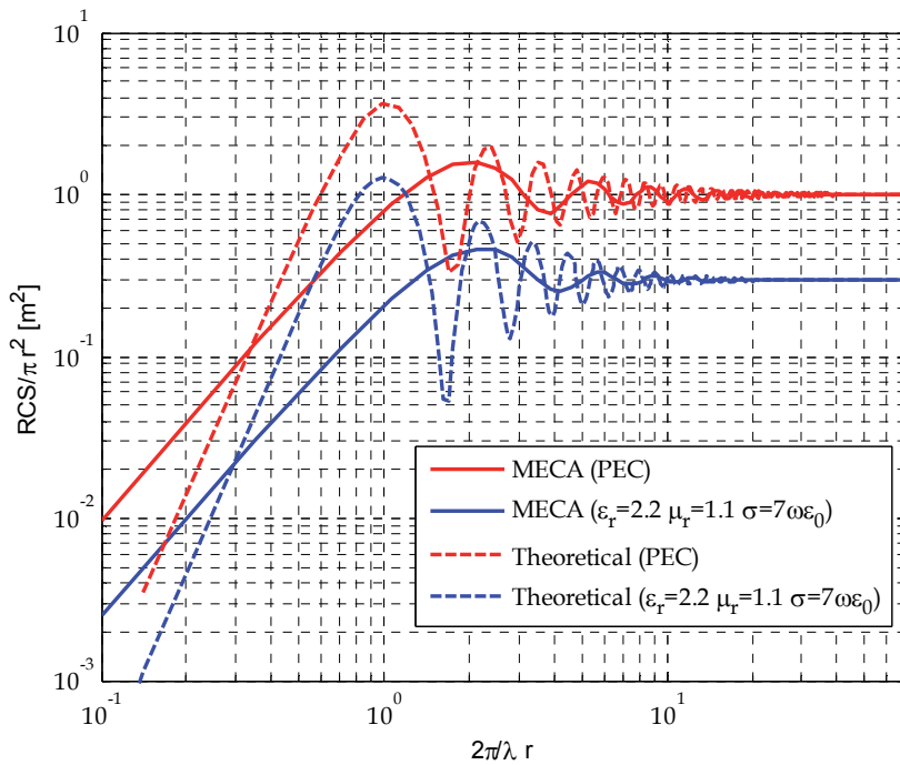
Fig. 5. Monostatic RCS of a sphere. PEC and lossy characterization ( \epsilon_r = 2.2 , \mu_r = 1.1 , \sigma = 7\omega\epsilon_0 ).
