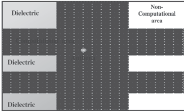
Fig. 1. Model of the 2 Dimensional FDTD Simulation.
