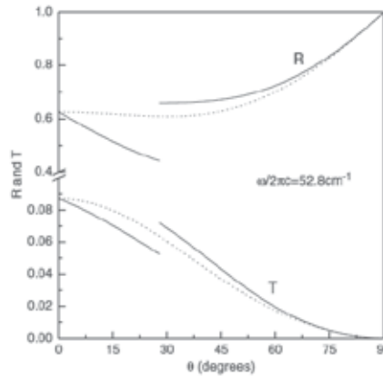
Fig. 10. Reflectivity and transmissivity versus angle of incidence for the frequency fixed at 52.8 \text{ cm}^{-1} . After Bai, et. al. 2007.
