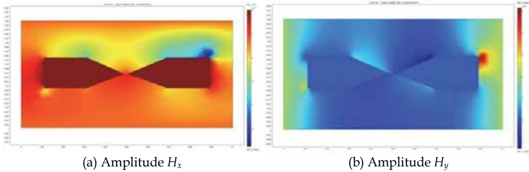
Fig. 15. Amplitude H_x and H_y of the magnetic field strength
