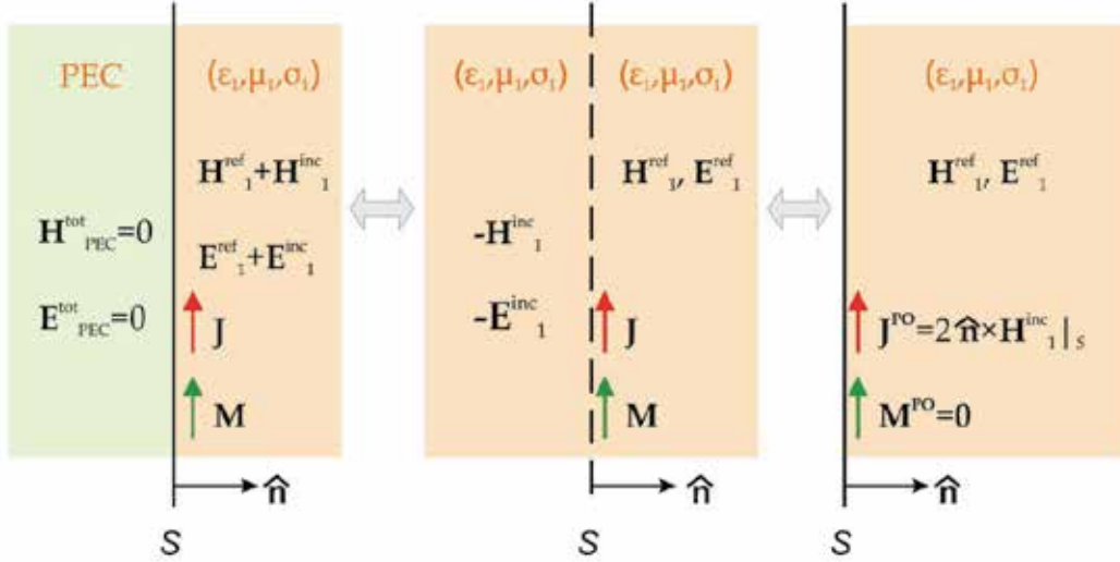
Fig. 1. Equivalence principle and Physical Optics approximation.
