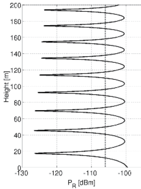
Fig. 15. Received Power vertical profile (solid line) and direct arrival (dotted line)
