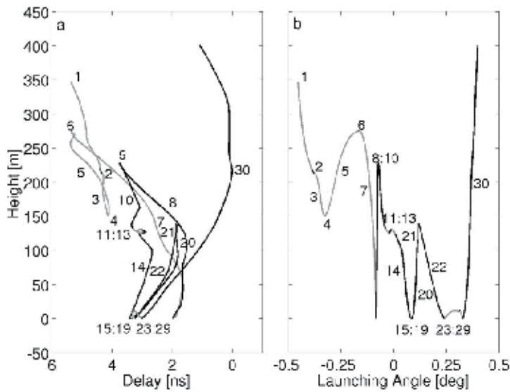
Fig. 7. Wavefronts time delay dispersion (a) and launching angle distribution (b)
