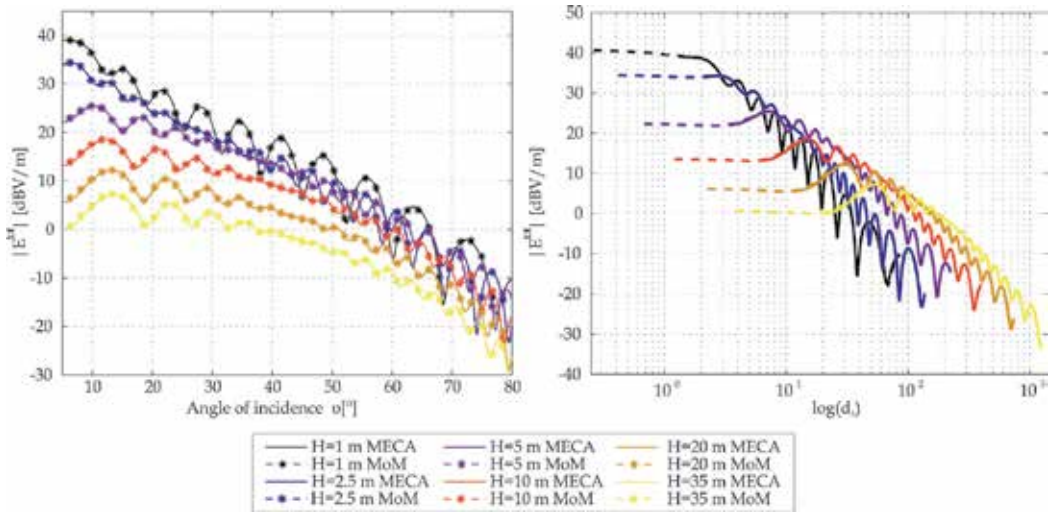
Fig. 7. Magnitude of the total electric field for the electrically large surface configuration. On the left, the results have been represented as a function of the angle \nu and on the right, as a function of the logarithm of the distance in wavelengths. MECA and MoM show a great coincidence.
