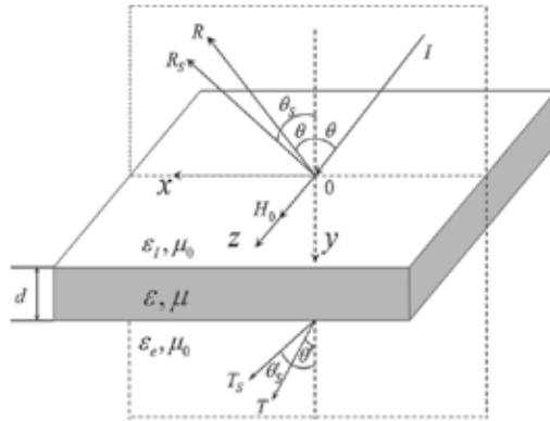
Fig. 11. Geometry and coordinate system.
