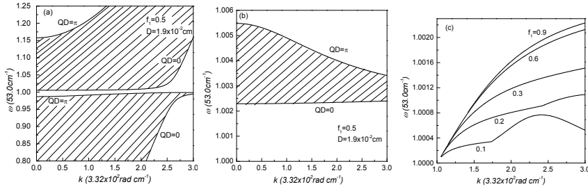
Fig. 4. Frequency spectrum of the polaritons of the FeF 2 /ZnF 2 superlattice. (a) shows the top and bottom bands, and (b) presents the middle band. The surface mode is illustrated in (c). f_1 denotes the ratio of the FeF 2 in one period of the superlattice. After Wang & Li, 2005.
