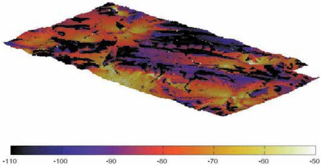
Fig. 10. Power density in dBW/m 2 for the rural scenario with MECA. The electromagnetic field levels have been evaluated for a penetrable characterization of the terrain given by \epsilon_r = 3 , \mu_r = 1 , \sigma = 0.001 S/m .
