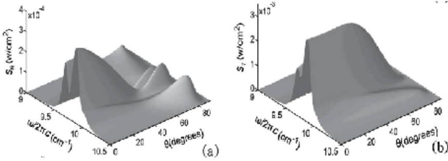
Fig. 12. SH outputs of a single AF film ( \text{MnF}_2 film), S_R and S_T versus the incident angle and frequency. After Zhou & Wang, 2008.
