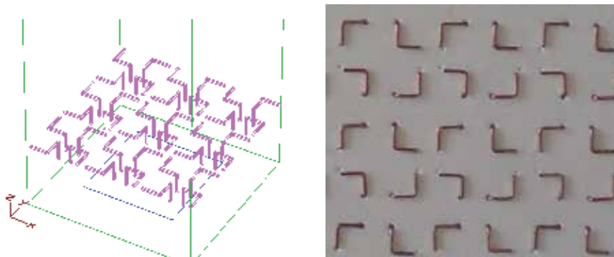
Fig. 3. Detailed view of a periodical lattice of cranks with the same handedness produced from 0.68 mm diameter and 15 mm length copper wire by bending in three segments by two 90 degrees angles. One of the segments is introduced perpendicularly into the host medium, polyurethane foam with a relative permittivity close to one. The backside of the medium is completely free of metal. Right: photograph of the lattice (García-Collado et al., 2010). Left: MEFIsTo™ model in which we may see the geometry of the cranks
