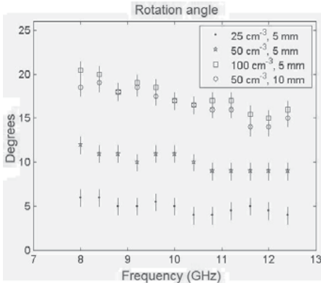
Fig. 9. Rotation angle produced by a random distribution of helices (Fig. 1) in a host, for different helix densities ( 25 \text{ cm}^{-3} , 50 \text{ cm}^{-3} , 100 \text{ cm}^{-3} ) and sample thickness (5 mm, 10 mm).
