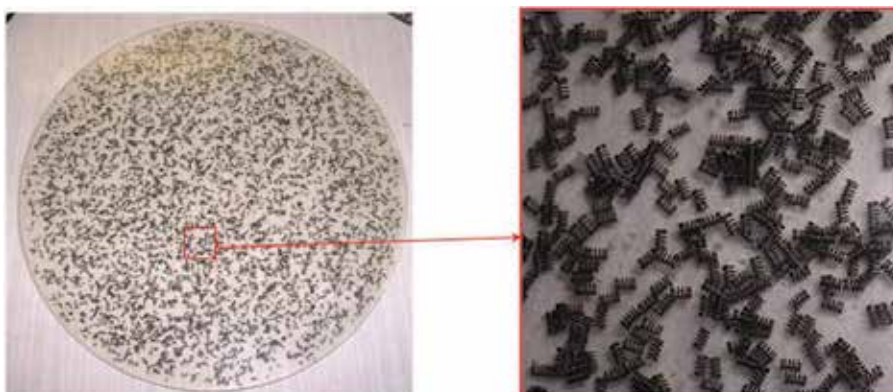
Fig. 1. Helix-based artificial chiral material. The sample is a 30 cm diameter disk fabricated by dispersion of six-turn stainless-steel helices in an epoxy resin with a low curing temperature. The helices are 2 mm height and 1.2 mm outer diameter.
