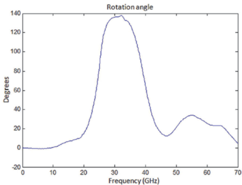
Fig. 16. Rotation of the polarization plane for a plane wave normally incident over a condensed array of cranks like represented in Fig. 14, normalizing between 0^\circ and 180^\circ
