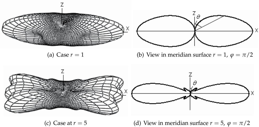
Fig. 6. Directivity diagram, the axis of magnetic dipole ( z ) is perpendicular to axis of a crystal at \varepsilon_1/\varepsilon = 15 .
