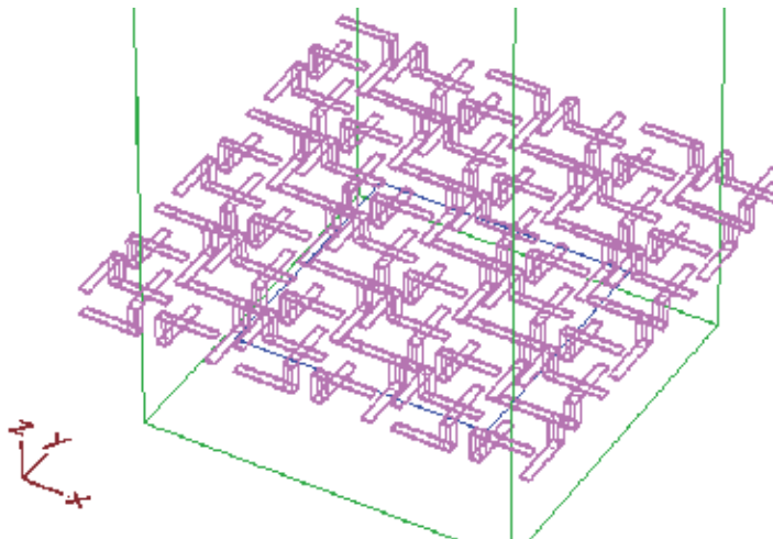
Fig. 14. MEFiSTo™ model of a condensed array of cranks. Each crank is composed by two arms, 3mm long, one in each side of the board (1.5 mm of thickness), plus a via connecting both.
