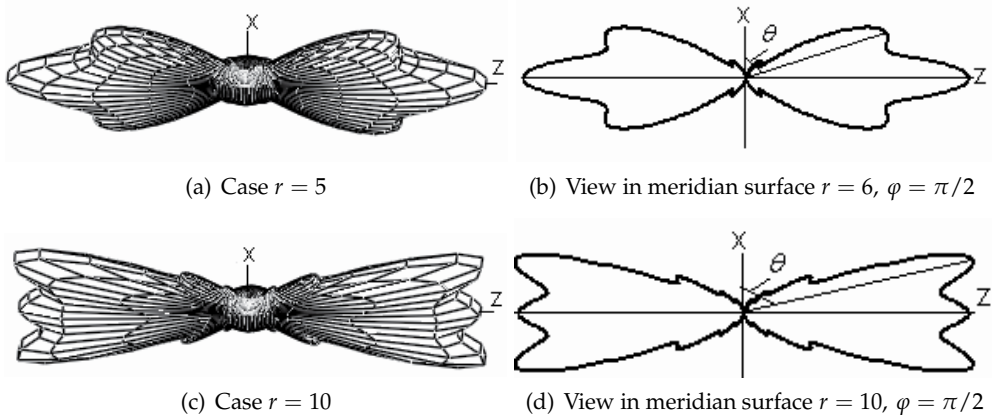
Fig. 12. Directivity diagram. The axis of magnetic dipole is perpendicular to z , \mu_1/\mu = 15
