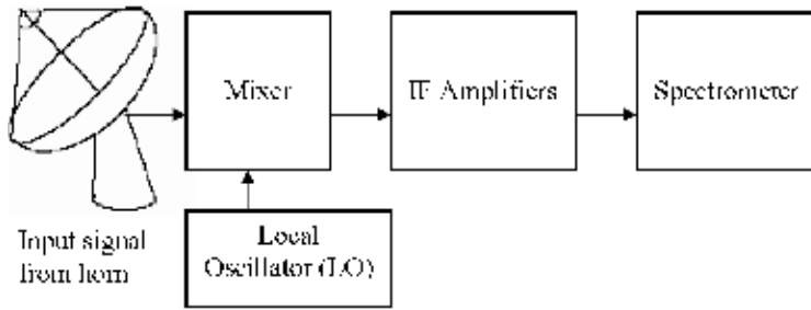
Fig. 1. Block diagram of a heterodyne receiver.
