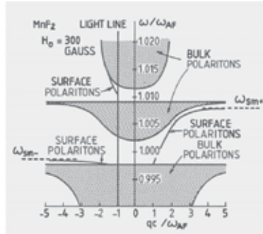
Fig. 2. Surface polariton dispersion curves and bulk continua on the \text{MnF}_2 in the geometry with an applied external field. After Camley & Mills, 1982
