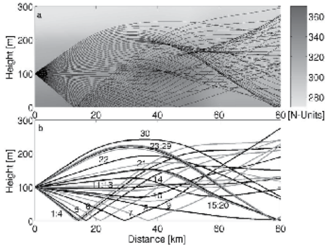
Fig. 6. Ray pattern (top) and wavefronts (bottom)
