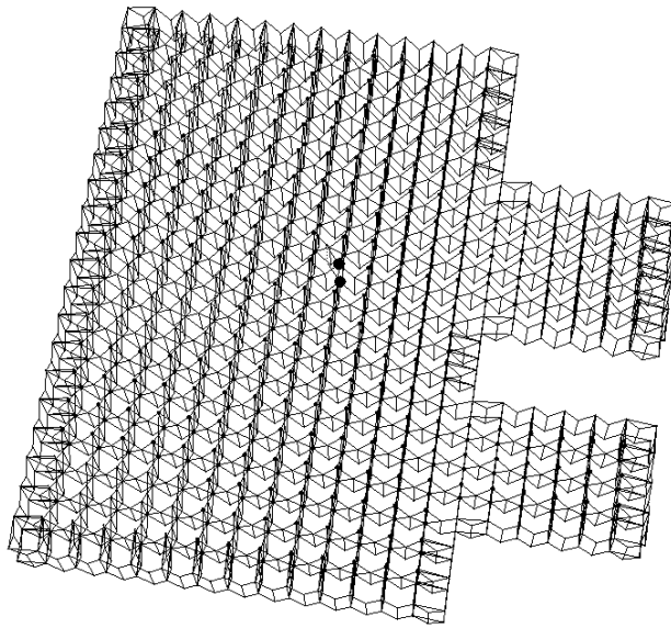
Fig. 3. Data Flow Graph for Two Iterations of the FDTD Problem for Irregular Computational Area.
