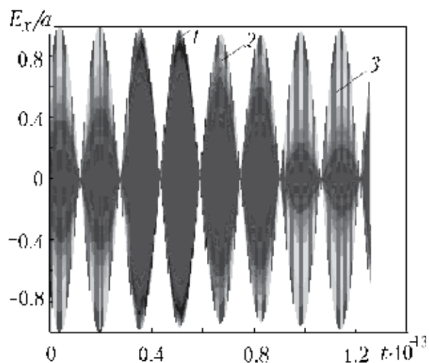
Fig. 5. Time change in the electric-field strength at a distance of 1 (1), 5 (2), and 10 \mu\text{m} (3) from the surface of the medium. t , sec.
