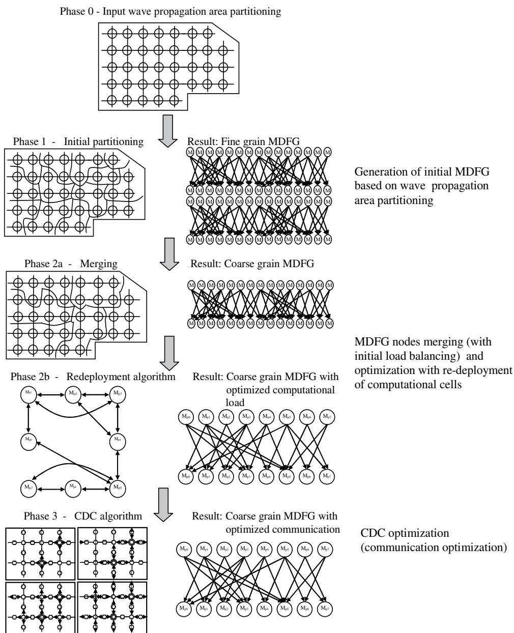
Fig. 12. RCDC Hierarchical Algorithm Scheme.
