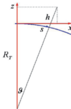
Fig. 3. The two reference systems: cartographic coordinates (s,h) and absolute ones (x,z) .
