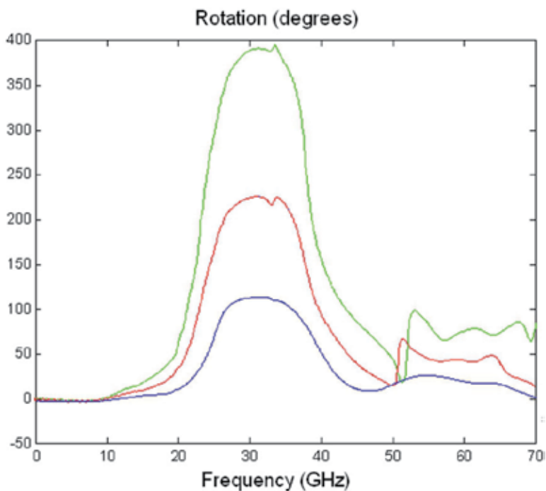
Fig. 17. Rotation of the polarization angle for a wave linearly polarized, incident over a condensed distribution of cranks like shown in Fig. 14, for one (blue line), two (red) or three (green) parallel boards. [Reprinted from Barba et al. (2009) © 2009 IEEE]
