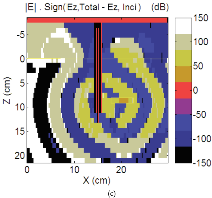
Fig. 5. Electric field [\text{Sign}(E_{z,\text{Total}} - E_{z,\text{Incident}})] \times 20 \log_{10}(|E| \text{ or } |\vec{E}_x \hat{i} + E_z \hat{k}|) , on the depth slice (XZ-plane) at time t = 3.6 nsec (the extent of the DNAPL pool and soil-air interface are marked in yellow): a) Incident image, b) Total image, and c) Scattered image.
