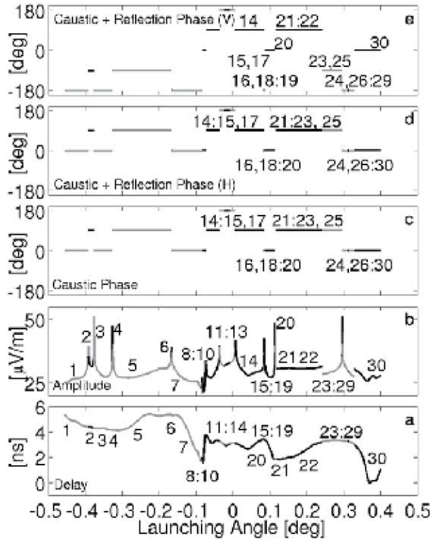
Fig. 9. Green's function attributes for the field calculation: from bottom to top: delay (a), amplitude (b), caustic phase (c), caustic + reflection phase (H polarization), caustic + reflection phase (V polarization)
