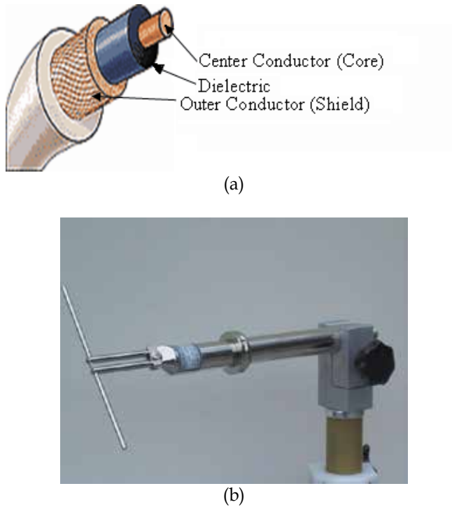
Fig. 2. Antennae: (a) Monopole antenna derived from a coaxial cable by removing a part of outer conductor, (b) a UHF-Half-Wave Dipole (Wikipedia, 2011).
