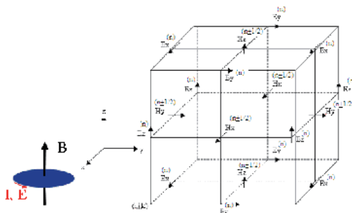
Fig. 1. 3D interlocking FDTD cell (Yee cell, 1966).
