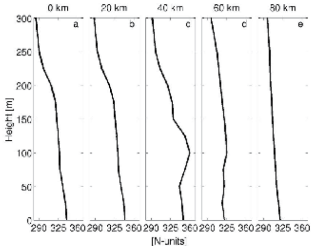
Fig. 5. Vertical profile at 5 chosen range distances.
