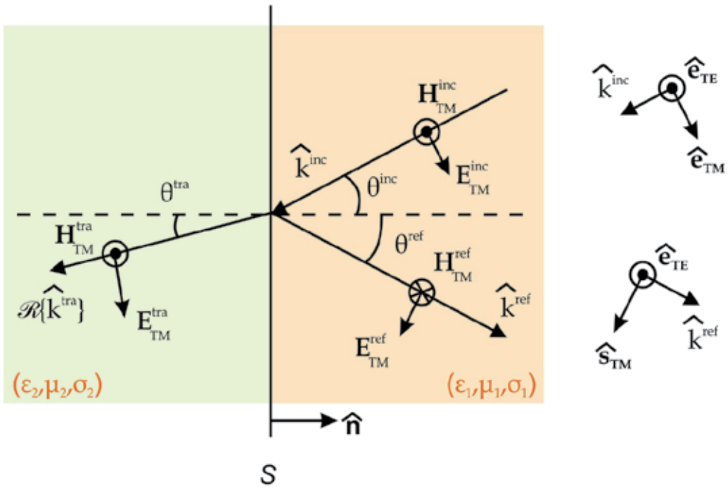
Fig. 3. Field decomposition. TM component.
