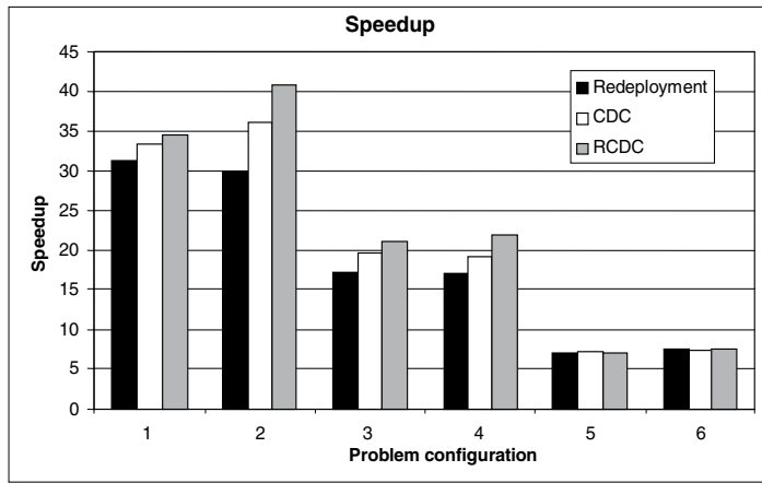
Fig. 13. Comparison of the Parallel Simulation Speedup for Redeployment, CDC and RCDC Algorithms.
