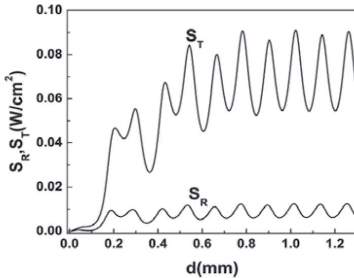
Fig. 15. SH outputs of SiO 2 /MnF 2 /air. S_R and S_T versus the film thickness for \omega = 9.84 \text{ cm}^{-1} and \theta = 41.3^\circ . After Zhou & Wang, 2008.
