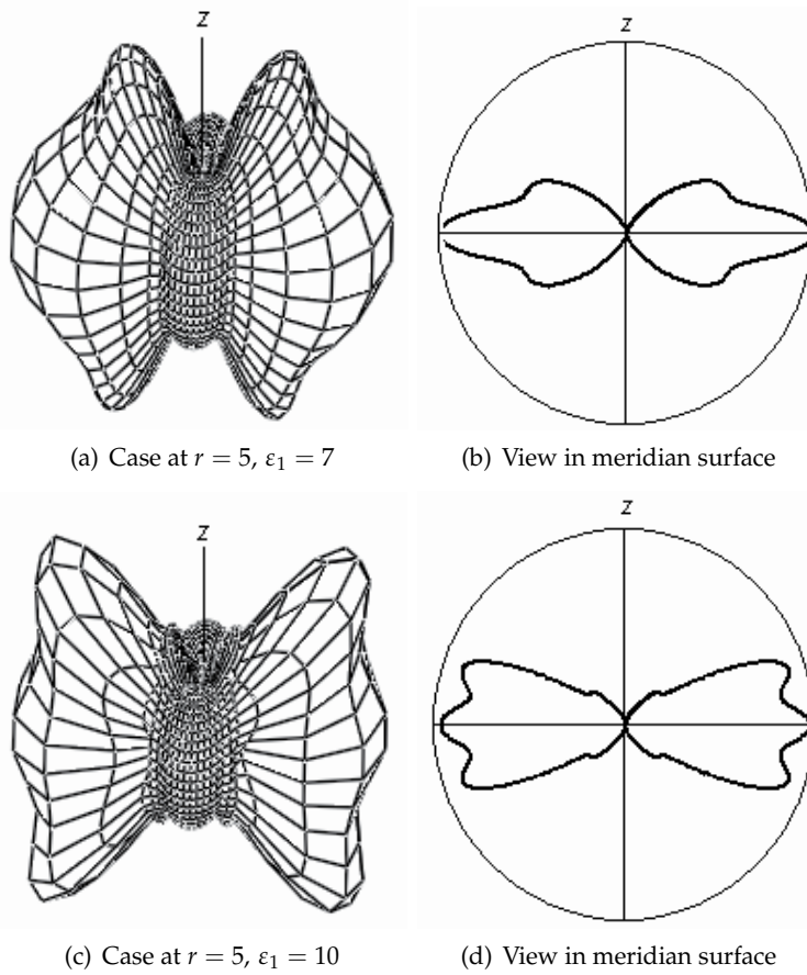
Fig. 2. Directivity diagram, the axis of dipole ( z ) is perpendicular to axis of a crystal
