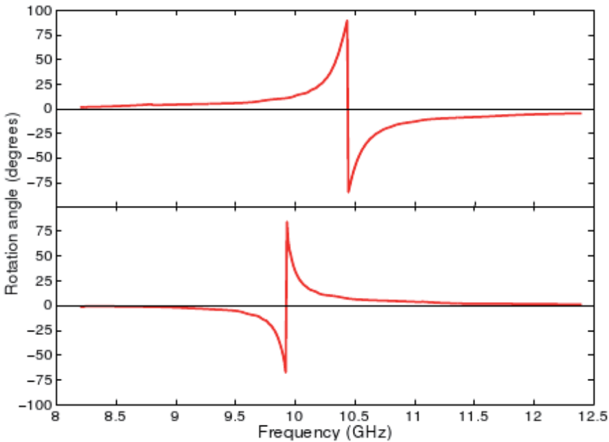
Fig. 12. Two examples of the rotation angle produced by a periodical lattice of metallic cranks formed by three equal size segments (5 mm) cranks for left-handed cranks with a separation of 6.9 mm (up) and right-handed cranks with a separation of 9.1 mm (down). [Reprinted from García-Collado et al. (2010) © 2010 IEEE]
