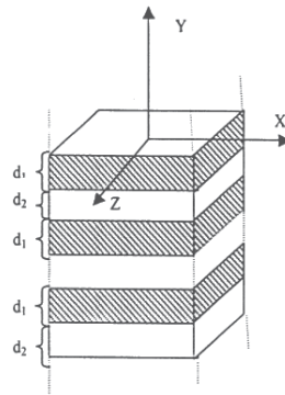
Fig. 3. The structure of AF superlattice and selected coordinate system.
