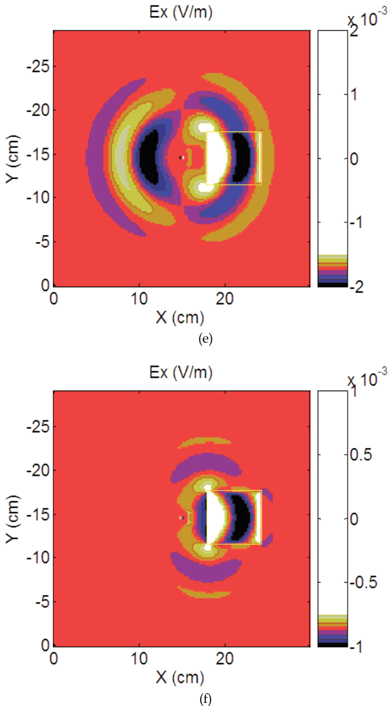
Fig. 4. Electric field simulated on the cross-sectional slice (XY-plane) at t = 3.6 nsec (the extent of the DNAPL pool is marked by a yellow box): Z-component of the electric field: a) Incident, b) Total, and c) Scattered; and X-component of the electric field: d) Incident, e) Total, and f) Scattered.
