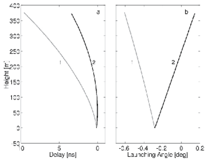
Fig. 14. Wavefronts time delay dispersion (a) and launching angle distribution (b)
