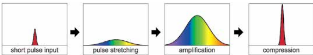
Fig. 6. Basic CPA scheme: ultrashort seed pulse is stretched, amplified, and recompressed.
