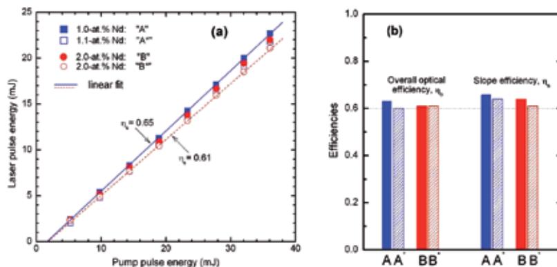
Fig. 11. Characteristics of laser emission in free-generation regime (i.e. without Cr 4+ :YAG): (a) Laser pulse energy versus pump pulse energy; (b) Overall optical efficiency ( \eta_0 ) and slope efficiency ( \eta_s ) for the available pump pulse energy of 36.1 mJ.
