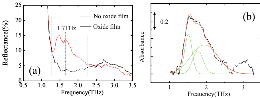
Fig. 14. THz spectra of copper surface covered with oxide and without oxides at room temperature.
