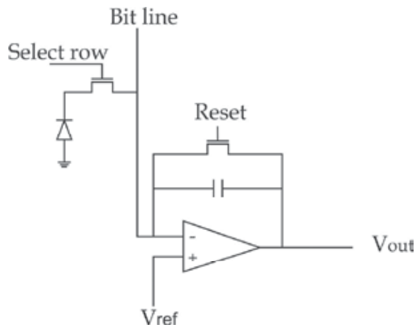
Fig. 10. A schematic of a passive pixel sensor
