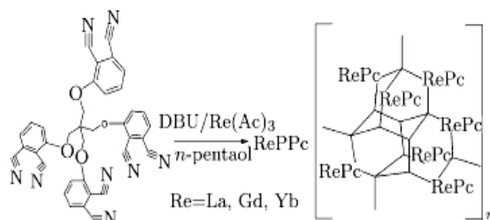
Scheme 3. Structures and synthesis route of rare earth polymeric phthalocyanines
