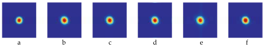
Fig. 13. The image at the output of the a) laser resonator, b) achromatic doublet, c) graded index fiber, d) optical part of the CMOS, e) electrical part of the CMOS, f) filtered image
