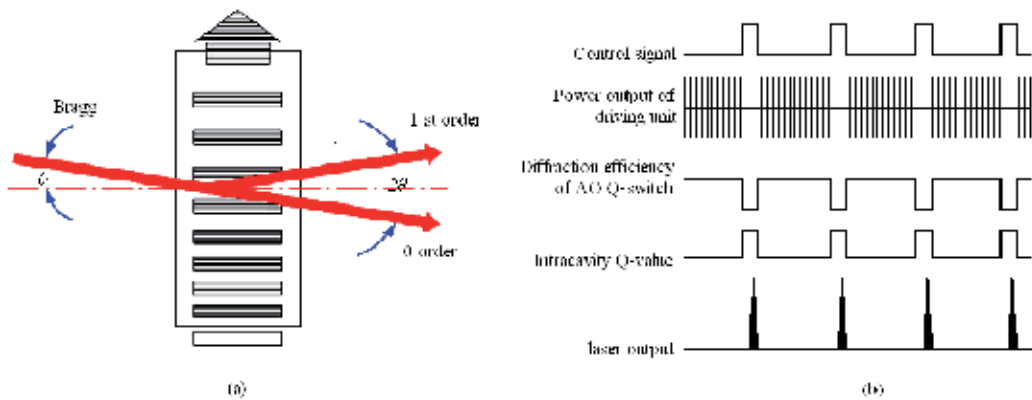
Fig. 1. The scheme of Q-switch
