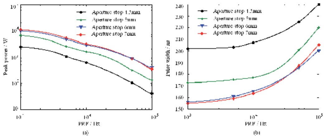
Fig. 11. Peak power (a), pulse width (b) of the CO 2 laser as a function of apertures stop
