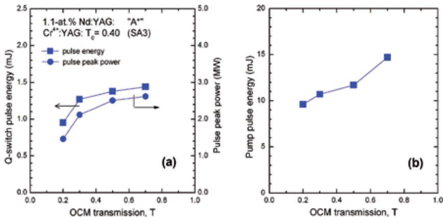
Fig. 15. (a) Q-switched laser pulse energy and peak power versus OCM transmission for the 1.1-at.% Nd:YAG ceramics and the Cr 4+ :YAG ceramics with T_0=0.40 . The resonator length was 11 mm. (b) Energy of the pump pulse is shown.
