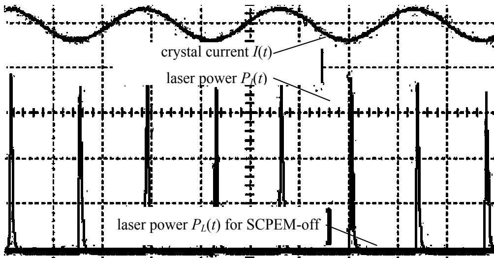
Fig. 13. Pulse sequence of a SCPEM-Q-switched Nd:YAG-laser: pulse frequency 190.2kHz, average power 2.1W, peak power 70W, pulse width 333ns. Crystal current I(t) (upper graph) and laser powers P_l(t) for SCPEM-on and SCPEM-off (with 2.8W cw-power)
