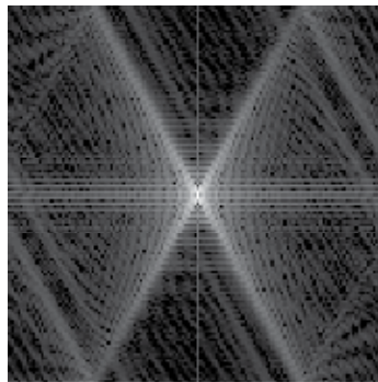
Fig. 6. The log of PSF for the apochromat
