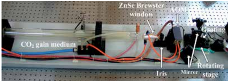
Fig. 16. Tunable acousto-optically Q-switch CO 2 laser
