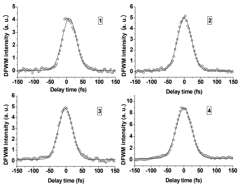
Fig. 2. Temporal profiles of DFWM signal of the diarylethene-phthalocyanine dyads 1-4
