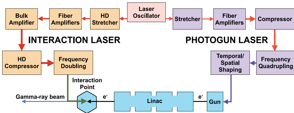
Fig. 5. Block diagram of the LLNL MEGa-ray Compton source with details of the laser systems.
