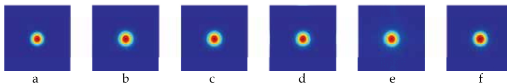
Fig. 14. The image at the output of the a) laser resonator, b) apochromat, c) self phase modulation fiber, d) optical part of the CMOS, e) electrical part of the CMOS, f) filtered image
