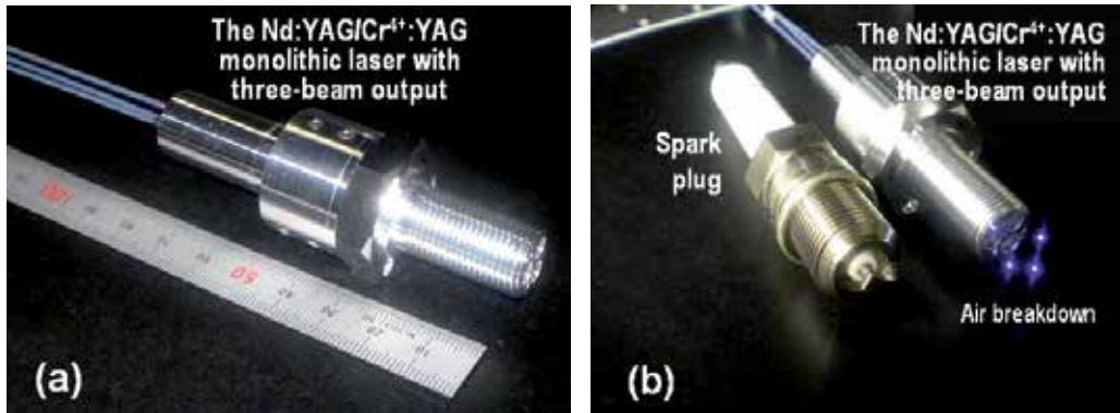
Fig. 23. (a) The passively Q-switched Nd:YAG/Cr+:YAG micro-laser with three-beam output is shown. (b) Air breakdown in three points is realized.
