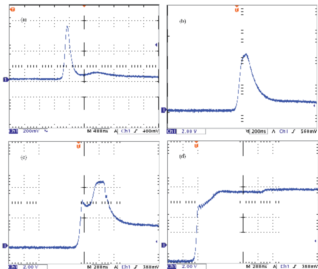
Fig. 18. Experimental results of PC-10.6 detector irradiated by pulse laser: (a) Normal working, (b) Disturbance phenomenon, (c) Saturation phenomenon, (d) Saturation completely
