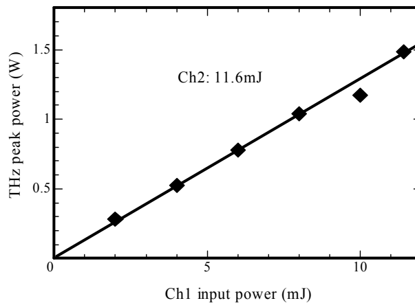
Fig. 4. Generated THz-wave power as a function of the pump beam (Ch1) energy/pulse in the 10-mm-long GaP crystal using a Cr:F source system. The signal beam (Ch2) energy/pulse was 11.6 mJ.
