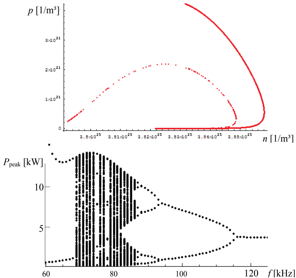
Fig. 11. Numerical analysis of a SCPEM-Q-switched Yb:YAG-slab laser Poincare-map of photon density p vs. inversion density n for chaotic operation (top) Bifurcation diagram: Peak powers P_{peak} vs. SCPEM-frequency f (bottom)
