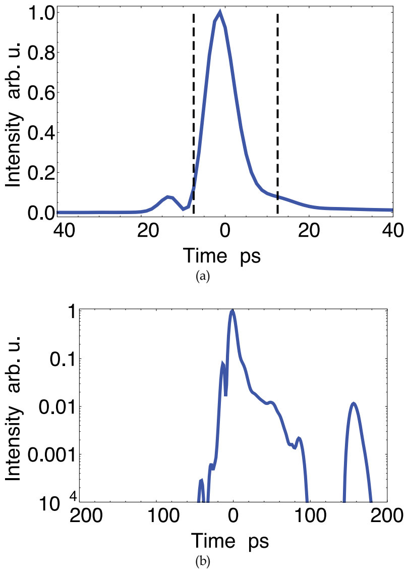
Fig. 18. Temporal pulse intensity obtained by analyzing a numerically processed FROG spectrogram on the linear scale (a) and log scale (b). FWHM of the pulse duration is 8.3 ps, and 84% of the energy is contained in the 20 ps bin (dashed box).
