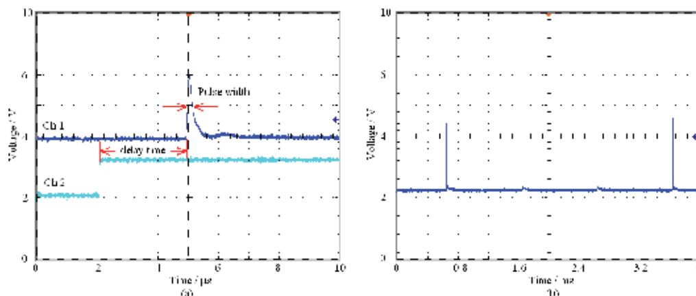
Fig. 13. Output waveforms of CO 2 laser at 1 kHz
