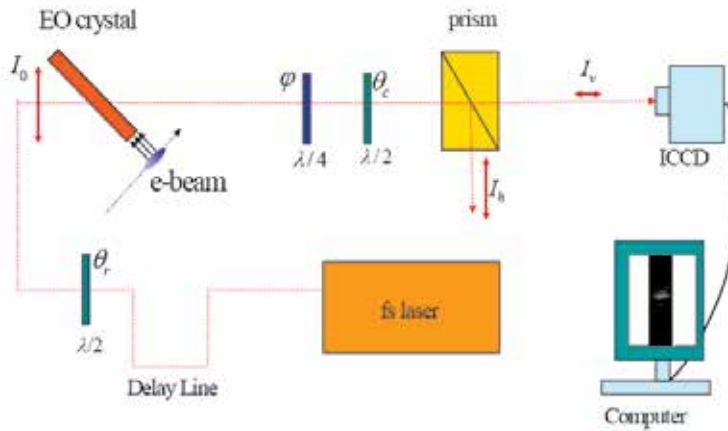
Fig. 3. Layout of the EO sampling experiment of electron beam in TEO setup at FLASH in DESY.
