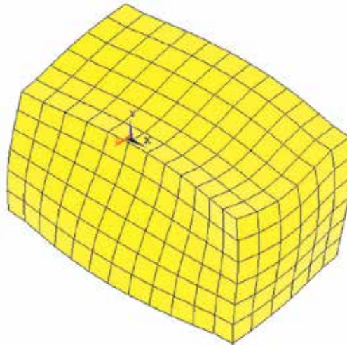
Fig. 6. ANSYS-simulation: yz-shear-eigenmode with 122.85 kHz of a y-excited BBO-crystal with dimensions 8.6 x 4.05 x 4.5mm
