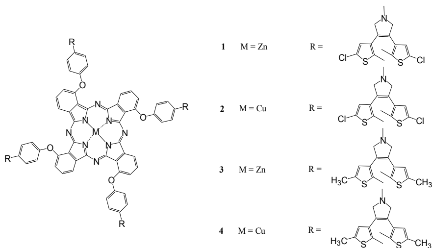
Fig. 1. Structures of diarylethene-phthalocyanine dyads 1-4
