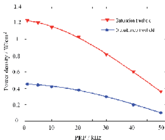
Fig. 22. Variations of detector threshold with pulse repetition frequency
