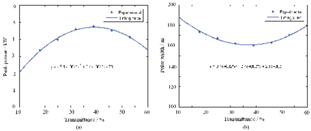
Fig. 10. The fitting curves of peak power (a) and the pulse width (b) versus transmittance of the output mirror
