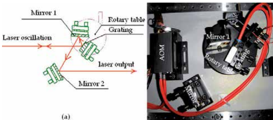
Fig. 14. Device of grating tuning. (a) The schematic, (b) The Photoshop
