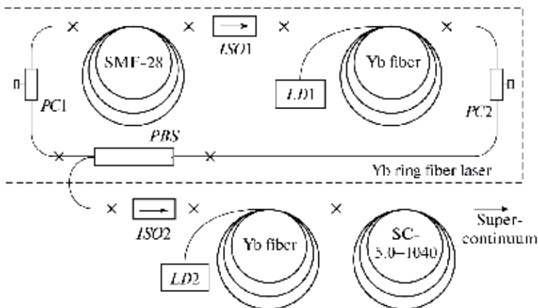
Fig. 6. Schematic layout of the all-fibre SC generator: LD1, LD2 – pumping laser diodes, PC1, PC2 – fibre polarisation controllers, ISO1, ISO2 – polarisation-insensitive optical isolators, and PBS – fibre polarisation beam splitter.
