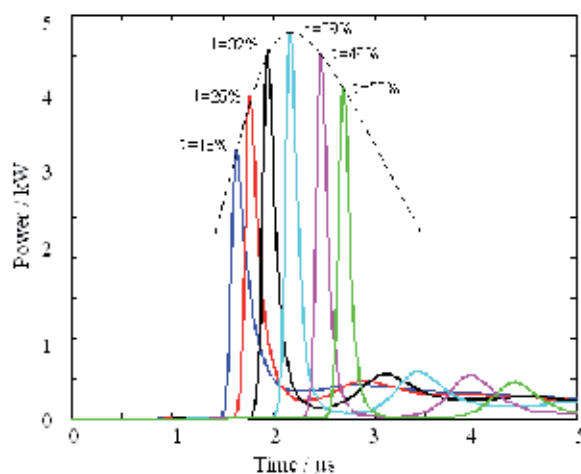
Fig. 9. Output power of the laser versus time at different transmittance
