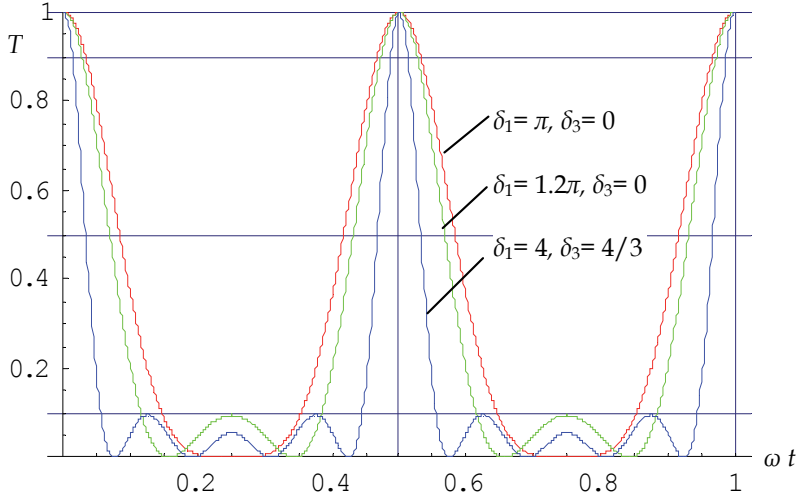
Fig. 7. Transmission curves of a dual mode SCPEM with \delta_1 = \pi , \delta_3 = 0 ; \delta_1 = 1.2\pi , \delta_3 = 0 ; and \delta_1 = 4 , \delta_3 = 4/3 .
