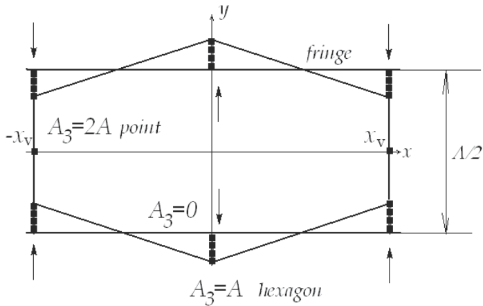
Fig. 7. The location of optical vortices within one cell of the pattern for different values of A_3 . Note that every pair of vortices is displaced along vertical line.
