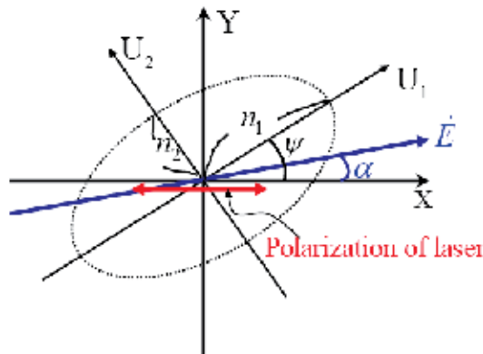
Fig. 2. The index ellipse is shown with the principal axis U_1 and U_2 . a represents the angle between the crystal axis X and the applied electric field E . The \psi is the angle between the principal axis and the crystal axis. The probe laser is linearly polarized as parallel to the X axis.
