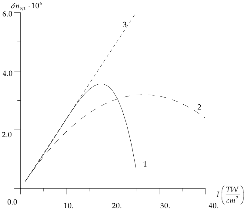
Fig. 2. Nonlinear additive to the index of refraction of air as a function of intensity 1- four-term approximation, 2- two-term approximation, 3- one-term approximation.
