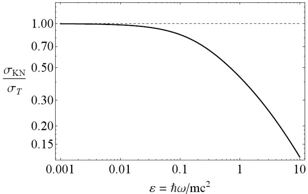
Fig. 1. Plot of the Klein-Nishina expression for the Compton scattering cross section. For small values of \varepsilon , the Compton cross section approaches the Thomson limit. At large values of \varepsilon , the Compton cross section approaches the asymptotic solution \sigma_{KN} \sim \frac{3}{8} \frac{\sigma_T}{\varepsilon} (\ln 2\varepsilon + \frac{1}{2}) .
