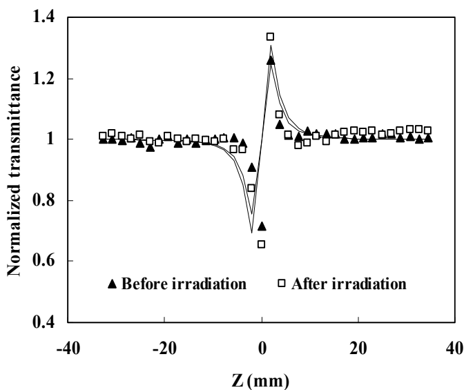
Fig. 5. Normalized transmission for the closed aperture of Z-scan measurement
