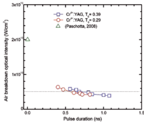
Fig. 16. Optical intensity of a laser pulse with ns duration that induced air breakdown.
