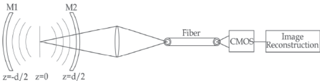
Fig. 1. A schematic of the image capture system
