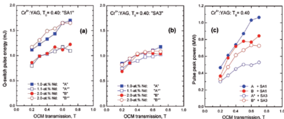
Fig. 12. Q-switched pulse energy versus OCM transmission obtained with Nd:YAG gain media and a Cr 4+ :YAG SA of T_0 = 0.40 : (a) The single-crystal Cr 4+ :YAG (SA1); (b) The poly-crystalline Cr 4+ :YAG (SA3) ceramics; (c) Laser pulse peak power is shown.
