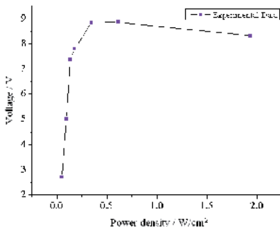
Fig. 21. The response curve of PV-10.6 detector irradiated by pulse laser
