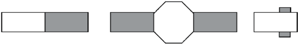
Fig. 1. Different shapes of classical photo-elastic modulators. The actuators are shown grey.
