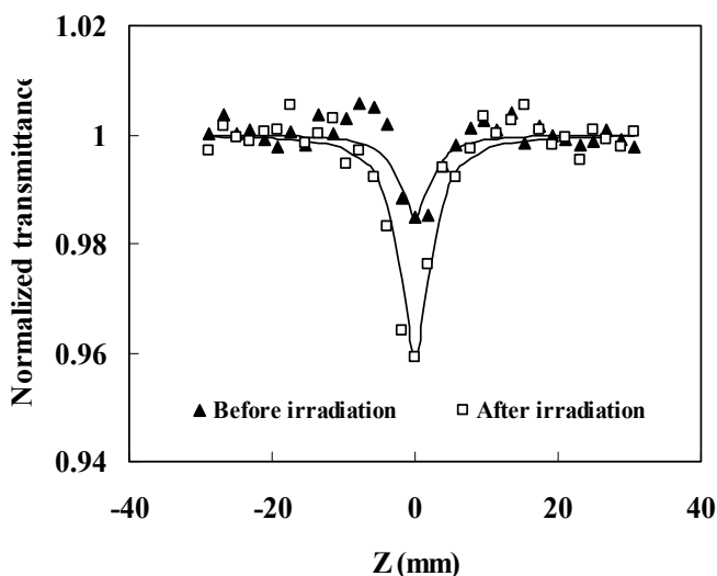
Fig. 4. Normalized transmission without aperture at 532 nm (open aperture) as a function of distance along the lens axis. The filled triangles and open squares are measured data for before irradiation and after irradiation of azo-phthalocyanine, respectively. Each point corresponds to the average of 5 pulses. The solid line is the theoretical fit.
