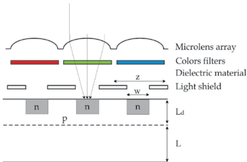
Fig. 7. The view of the simplified pixel cross section
