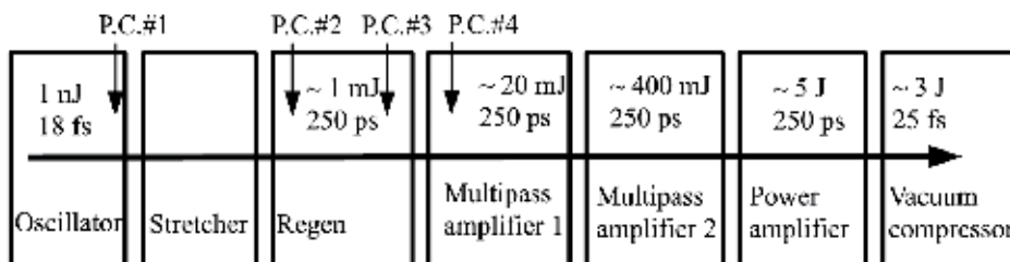
Fig. 1. Architecture of a high intensity laser system. P.C. indicates the position of the Pockels cells in the laser system. Typical output energy and pulse duration (FWHM) are indicated at each location.
