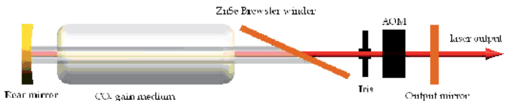
Fig. 2. Schematic diagram of acousto-optically Q-switch CO 2 laser
