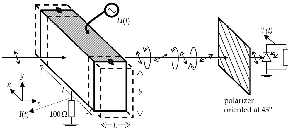
Fig. 2. Single Crystal Photo-Elastic Modulator made of a 3m-crystal (Bammer, 2009).
