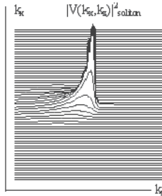
Fig. 9. Plot of the side projection |V(k_x, k_z)|^2 of the spectrum of a Lorentzian profile V(x, y, z) = 1/[1 + x^2 + y^2 + (z + ia)^2 + a^2] , a = 2 increasing towards the small k_z wave-numbers (compare with Fig. 8).
