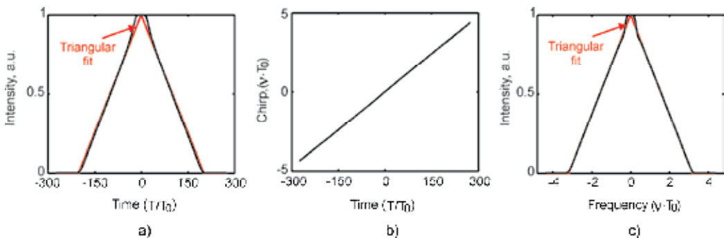
Fig. 15. Normalized pulse temporal intensity ( M = 0.037 ) – (a), spectrum ( M = 0.018 ) – (c) and chirp (b) in the steady-state regime produced from initial secant pulse ( N = 10, \xi = 10 ). Red curves show corresponding triangular fits.
