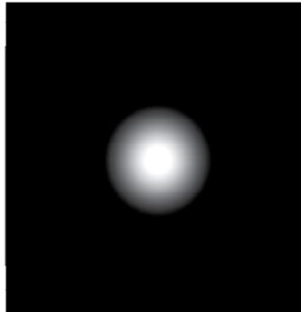
Fig. 2. The fundamental Hermite Gaussian mode TEM_{00}
