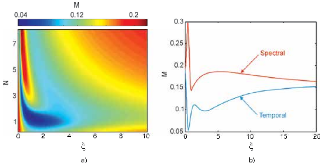
Fig. 2. a) Evolution of the misfit parameter M versus N and \xi in the case of initial secant pulse shape. b) Evolution of the misfit parameter M versus \xi for the temporal and spectral pulse shapes ( N = 2 ).
