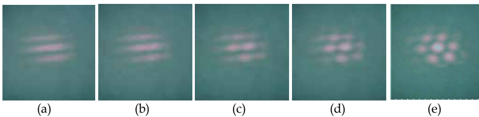
Fig. 14. Intensity patterns for interference of three laser beams with progressive change of amplitude of one of interfering waves. Here we go from (a) two beams ( A_3=0 ) to (e) complete three beams ( A_3=A ) interference.
