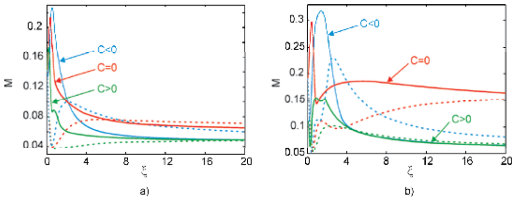
Fig. 4. Evolution of the misfit parameter M versus \xi for the temporal and spectral pulse shapes ( N = 2 ) in the case of initial pulse with initial positive chirp, negative and unchirped. The absolute value of initial chirp parameter here is 0.5. a) - initial Gaussian pulse; b) - initial secant pulse. Dotted lines denote temporal curves; solid lines - spectral curves.
