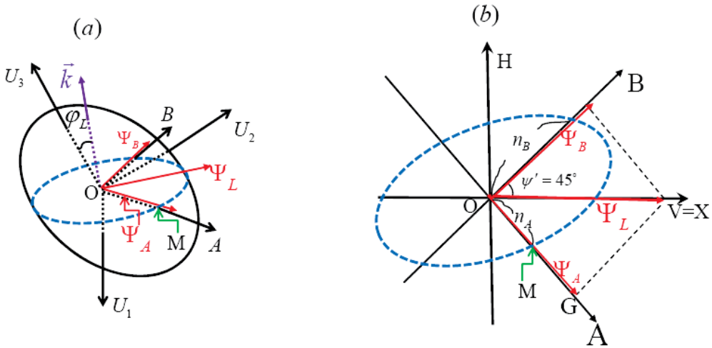
Fig. 5. (a) The index ellipsoid is shown with the principal axes U_1, U_2 , and U_3 . (b) The 2D configuration for the decomposition of the laser polarization vector \Psi_L . A and B axes make 45^\circ with respect to the polarization vector \Psi_L . H and V axes are the horizontal and vertical axes in the AB plane. The polarization vector \Psi_L is fixed as parallel to the X axis. n_A and n_B are the refractive indices along A and B axes, respectively.
