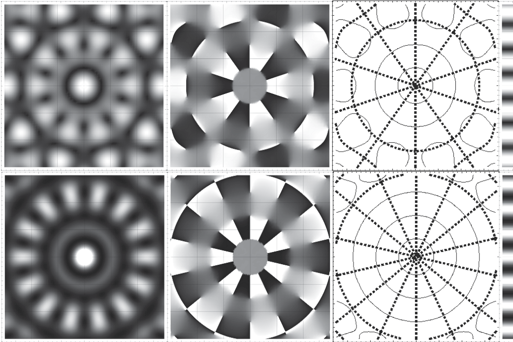
Fig. 10. Numerical calculations of the interference pattern of five plane waves (top) and of seven plane waves (bottom). Intensity distribution is shown in the first column, the phase distribution is shown in the second column and the plot of lines \text{Re}=0 (solid line) and \text{Im}=0 (dashed line) (third column). Angles between wave vectors are equal. The amplitudes of interfering waves are equal. The scale is related to the period of the two-waves interference as shown on the side.
