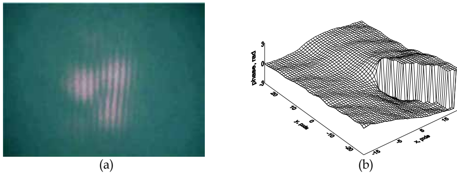
Fig. 13. The experimental observation of one vortex formation: (a) with the reference beam, one can see the bifurcation of the single black fringe into two fringes, (b) the phase distribution in radians, transverse coordinates are in pixels. ).
