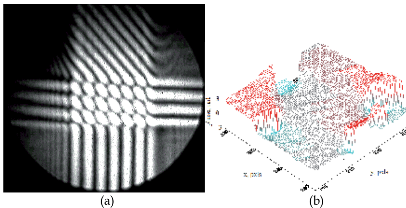
Fig. 12. (a) Experimental pattern of intensity distribution of the total field of three plane waves (center) and patterns of two plane waves (up, down, sides). The vortices reveal in vertices as black pots. To simplify the comparison with the numerical calculations of Fig.3, parts of each wave were closed. The diffraction effect is seen on the edges of screens. (b) the phase distribution in of one hexagonal cell of (a).
