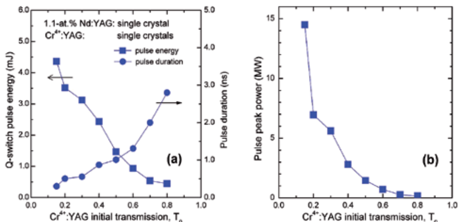
Fig. 8. Characteristics of Q-switched pulses yielded by the Nd:YAG-Cr 4+ :YAG laser shown in Fig. 7, versus initial transmission T_0 of Cr 4+ :YAG: a) Energy and duration; b) Peak power.
