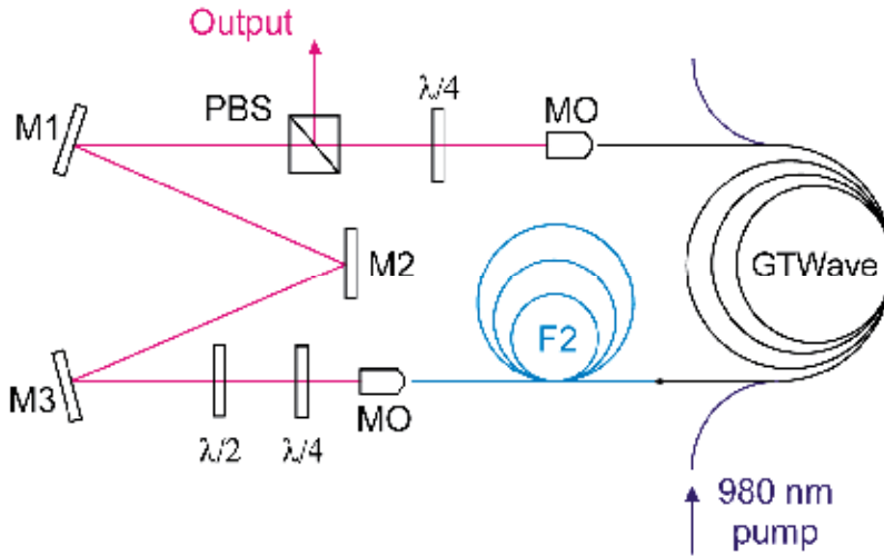
Fig. 3. Schematic of extra-long mode-locked fibre laser: F2 – All-wave fibre, length of 2,6 km.
