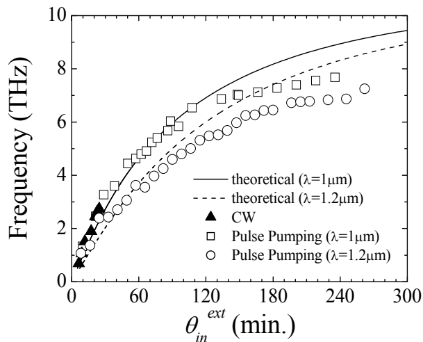
Fig. 2. The relationship between \theta_{in}^{ext} and the THz-wave frequency at which the maximum output power was obtained in CW and pulse pumping. The solid line represents the calculated relationship described in more detail within the text.
