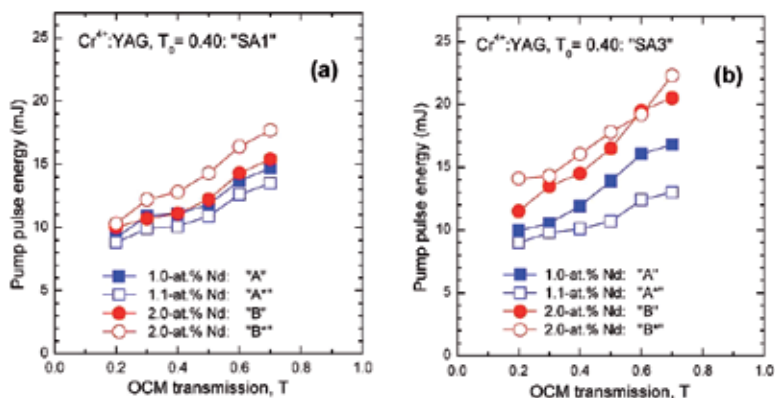
Fig. 13. Pump pulse energy necessary for laser emission with: (a) The single-crystal \text{Cr}^{4+}:\text{YAG} (SA1); (b) The poly-crystalline \text{Cr}^{4+}:\text{YAG} (SA3) ceramics.
