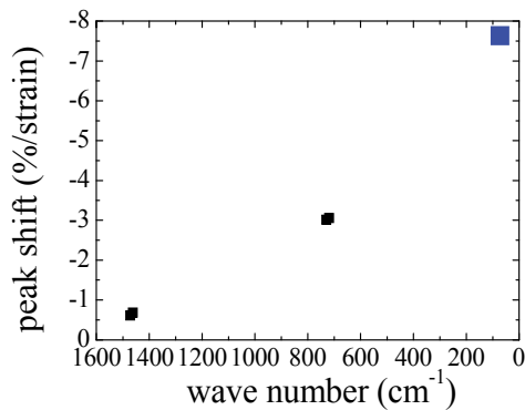
Fig. 10. The relation between peak shift rate and peak position of the B_{1u} band during uniaxial deformation.
