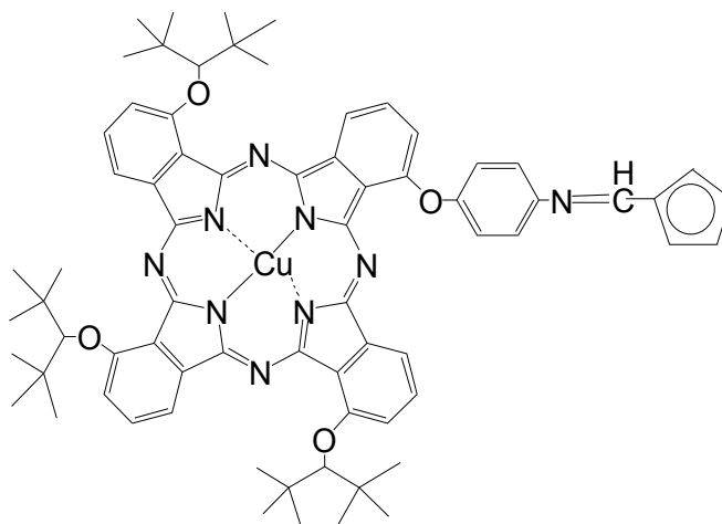
Fig. 7. Structure of novel copper phthalocyanine-ferrocene dyad
