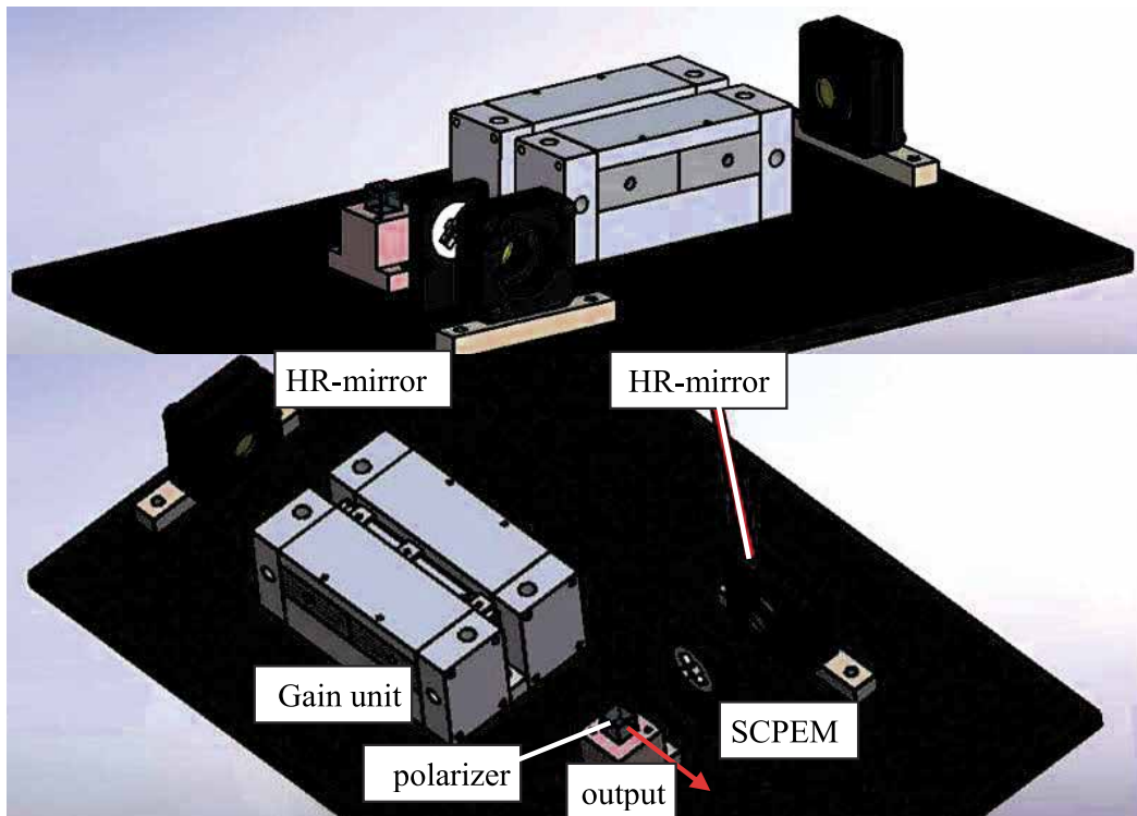
Fig. 12. Nd:YAG-laser for SCPEM-Q-switching
