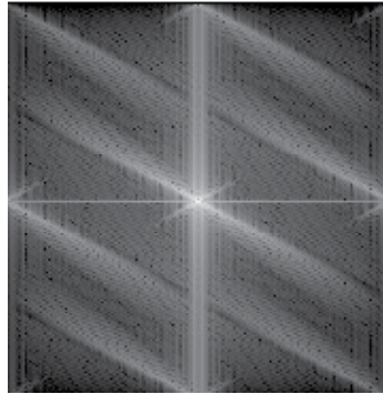
Fig. 5. The log of the PSF for the achromatic doublet
