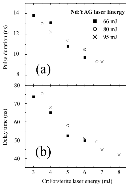
Fig. 5. Cr:Forsterite laser characteristics of the pulse duration (a) and delay time (b) at Cr:Forsterite laser energy of 3–8 mJ. The cavity length was fixed to 20 cm. Nd:YAG laser power was changed to 66 mJ, 80 mJ, and 95 mJ.
