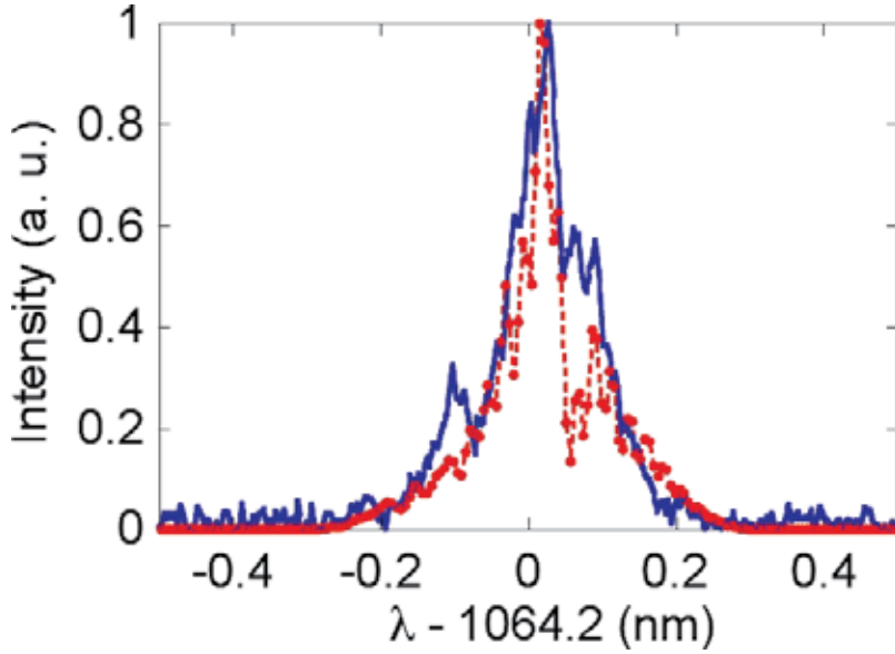
Fig. 19. Pulse spectrum from FROG (red dots) and spectrometer (solid line) measurements.
