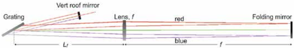
Fig. 7. Grating and lens based stretcher is folded with a flat mirror. The distance from the grating to the focal length of the lens determine the sign and magnitude of the chirp.
