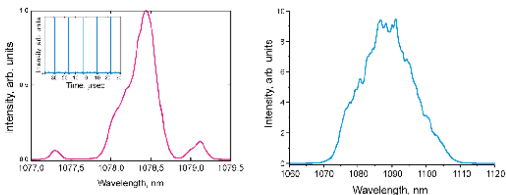
Fig. 5. Optical spectra of the ultra-long mode-locked Yb-doped fibre laser. On the left: spectrum in the case of single 3-ns pulses generation, inset: real-time oscilloscope trace of single pulse train; on the right: spectrum in the case of multiple nanosecond pulse train generation.
