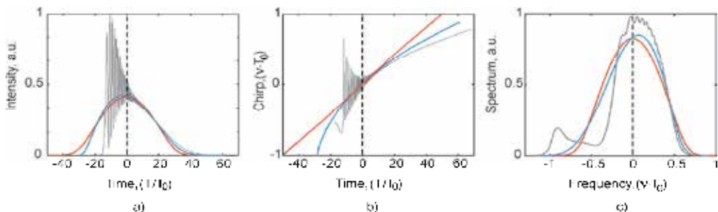
Fig. 6. Pulse evolution in the steady-state under the TOD impact ( N = 2 , \xi = 8 ). (a) - Pulse temporal profile. (b) - Chirp. (c) - Spectrum. Color indicates the relative magnitude of TOD: red curve - without TOD; blue curve - L'_D / L_D = 7.3 ; gray curve - L'_D / L_D = 3.3 .
