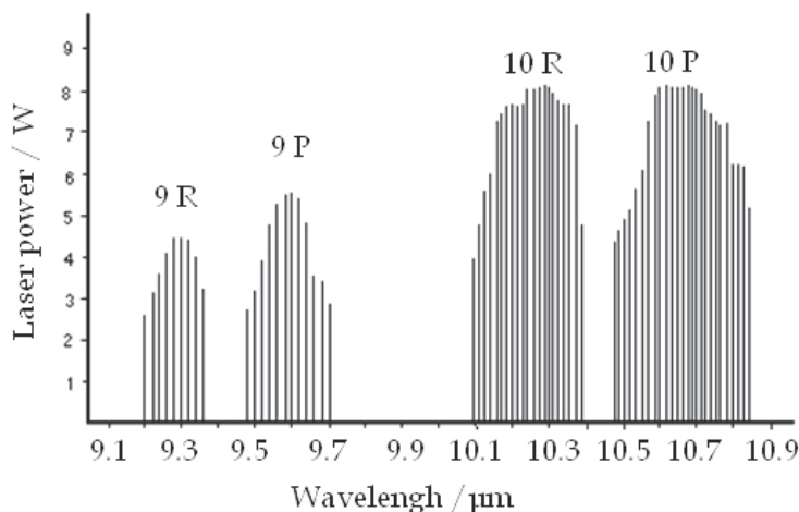
Fig. 15. Laser Spectral Lines
