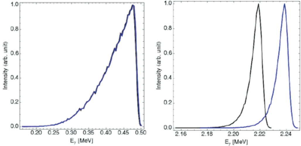
Fig. 4. Gamma-ray spectra in the case of Compton scattering (black) and Thomson scattering (blue). Left: T-REX source parameters (laser: 20 ps FWHM pulse duration, 532 nm wavelength, 34 \mu\text{m} rms spot size, 150 mJ; electron beam: 116 MeV, 40 \mu\text{m} rms spot size, 20 ps FWHM bunch length, 0.5 nC beam charge, 6 mm.mrad normalized emittance). Right: future Compton source parameters (laser 10 ps FWHM pulse duration, 532 nm wavelength, 12 \mu\text{m} rms spot size, 150 mJ; electron beam: 250 MeV, 15 \mu\text{m} rms spot size, 10 ps FWHM bunch length, 0.25 nC beam charge, 1 mm.mrad normalized emittance).
