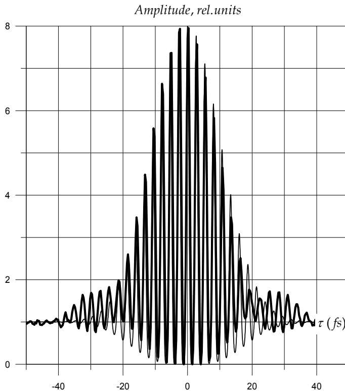
Fig. 7. Output signal of interferometric intensity autocorrelator for a transform limited wave packet. The bold and fine curves are for the experiment and the calculation using Eq. (24) for L = 1 , respectively.
