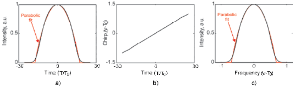
Fig. 5. Normalized pulse temporal intensity - (a), spectrum - (c) and chirp (b) in the steady-state regime produced from initial Gaussian pulse with positive chirp ( N = 2 , \xi = 4 , C = 1 ). Red curves show corresponding parabolic fits.
