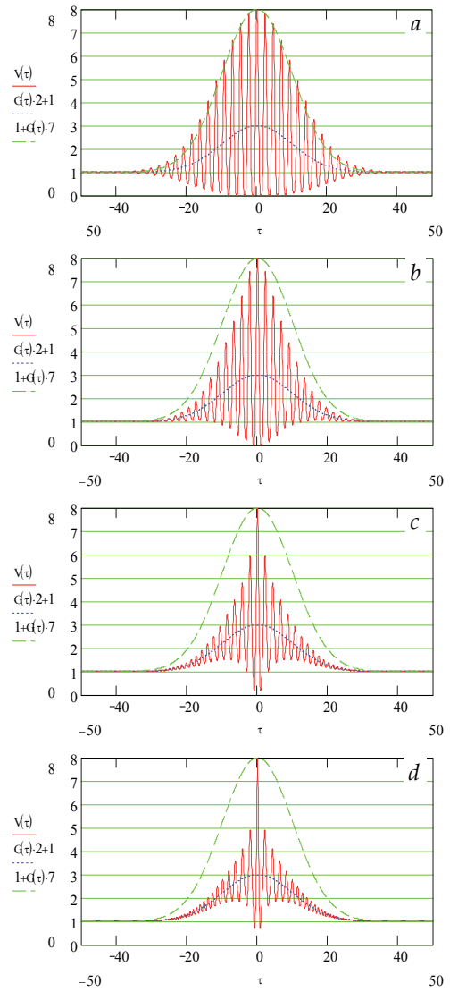
Fig. 6. Profile of the signal V(\tau) for K = 1 (a), K = 5 (b), K = 20 (c), and K = 50 (d) in the case of a pulse of duration \tau_0 = 10\text{fs} with cubic phase modulation.
