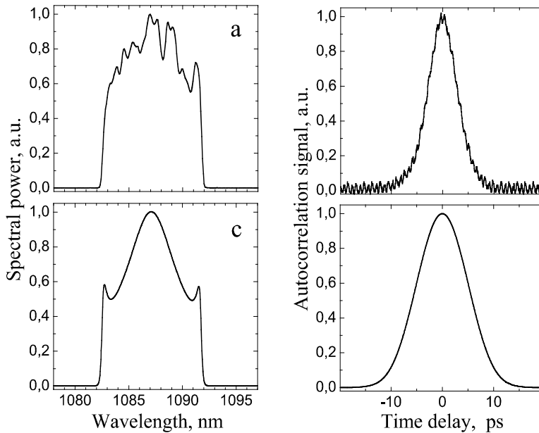
Fig. 9. Stable single-pulse generation: a, b - experimental results; c, d - simulations; a, c - spectra; b, d - ACFs.
