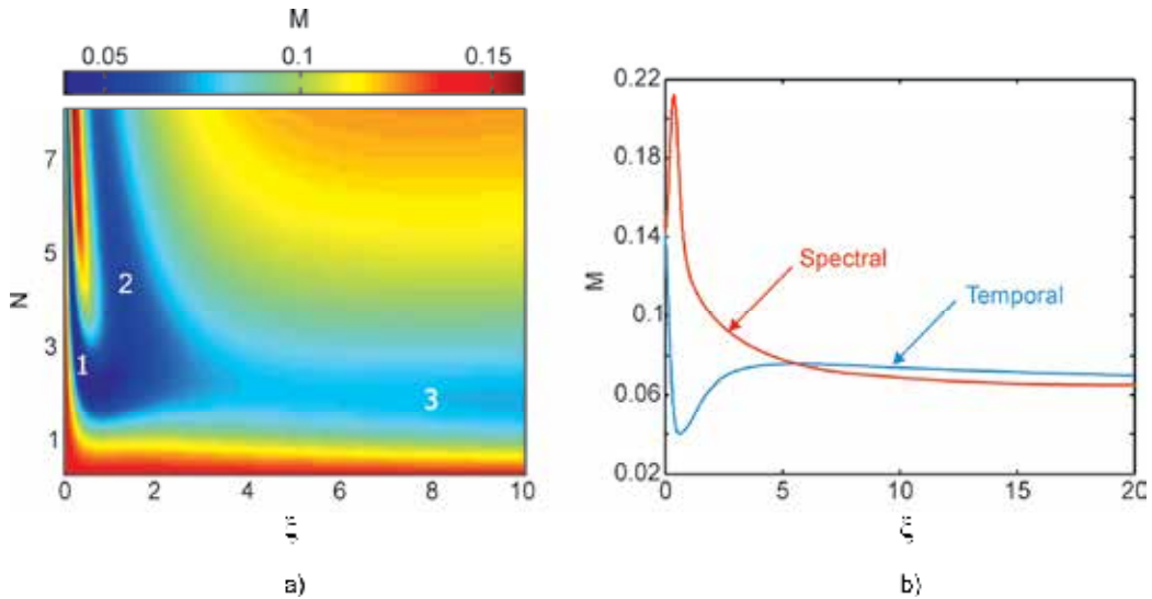
Fig. 1. a) Evolution of the misfit parameter M versus N and \xi in the case of initial Gaussian pulse shape. Numbers at the figure denote three specific areas described in the text. b) Evolution of the misfit parameter M versus \xi for the temporal and spectral pulse shapes ( N = 2 ).
