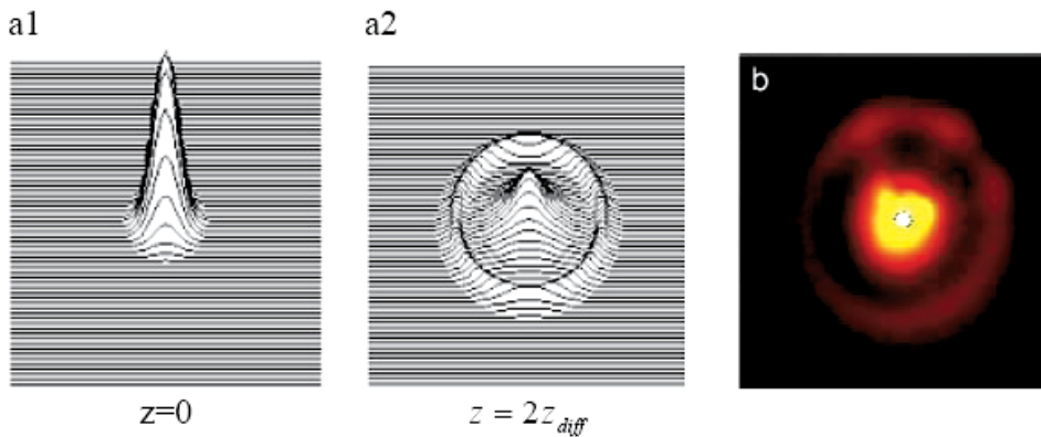
Fig. 4. Nonlinear evolution of the waist (intensity) projection |A(x,y)|^2 of a 400 fs initial Gaussian pulse (a1) at \lambda = 800 \text{ nm} , with spot r_0 = 120 \mu\text{m} , and longitudinal spatial pulse duration z_0 = v_{gr}t_0 \cong 120 \mu\text{m} at a distance z = 2z_{diff} (a2), obtained by numerical simulation of the 3D+1 nonlinear AE equation (20). The power is above the critical for self-focusing P = 2P_{kr} . Typical self-focal zone (core) surrounded by Newton's ring is obtained. (b) Comparison with the experimental result presented in (12).
