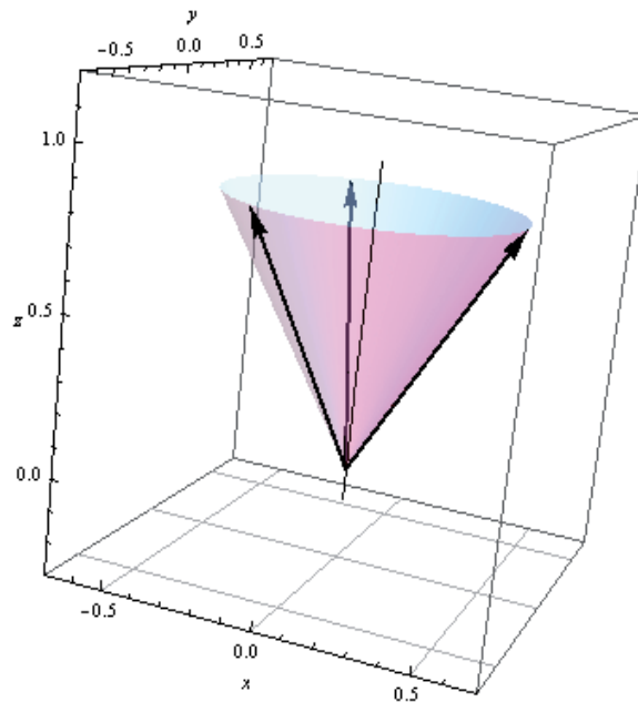
Fig. 2. The direction of wave vectors for three plane waves interfering at symmetric angles of \psi=2\pi/3 radians and azimuth \theta=\pi/10 radians.
