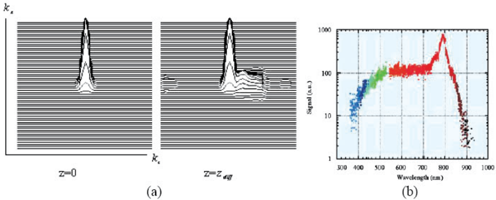
Fig. 6. (a) Fourier spectrum of the same side ( x, z ) projection of the intensity |A(k_x, k_z)|^2 as in Fig.5. At one diffraction length the pulse enlarges asymmetrically forwards the short wavelengths (high k_z wave-numbers), (b) a spectral form observed also in the experiments (12).
