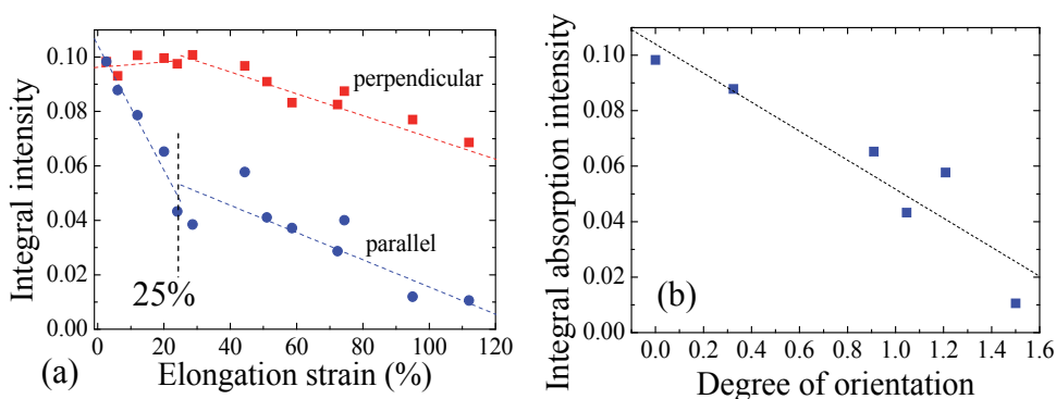
Fig. 8. (a) The integrated absorption intensities of the B_{1u} band as a function of the degree of elongation strain. Incident THz wave was polarized parallel (●) and perpendicular (■) to the axial direction of the deformation. (b) THz absorption intensity vs. degree of orientation. THz wave electric polarization direction is perpendicular to the deformation direction. Degree of orientation was evaluated by XRD measurements.
