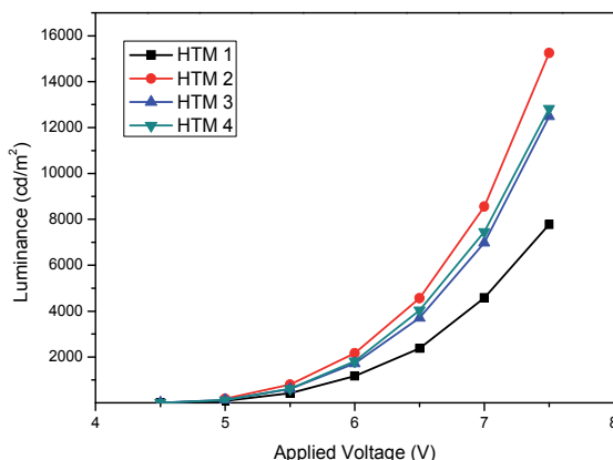
Fig. 6. Luminance-applied voltage characteristics of devices III-VI.
