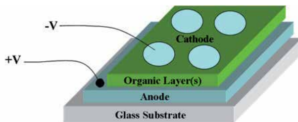
Fig. 3. The device structure of an OLED
