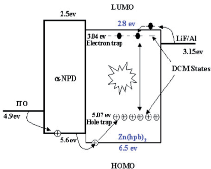
Fig. 22. Energy level diagram for the \text{Zn(hpb)}_2 /DCM system.
