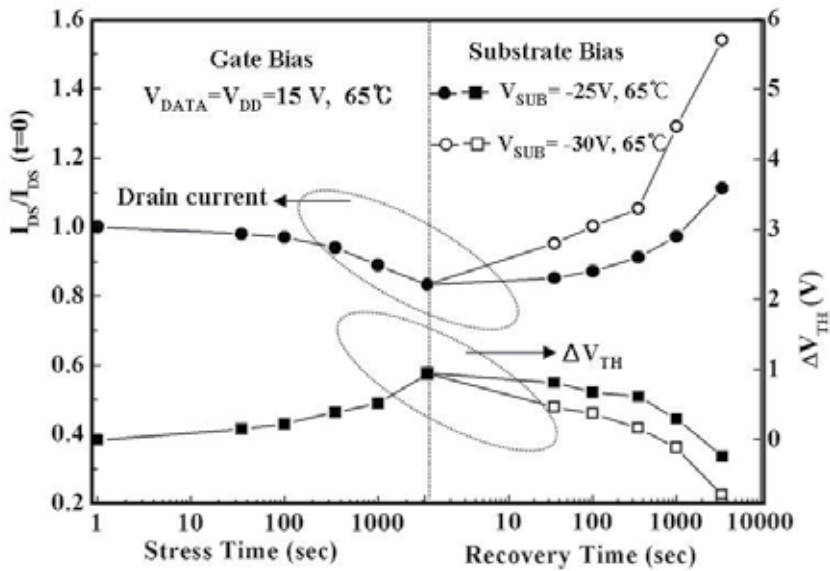
Fig. 20. Drain current and threshold voltage transition of a driving TFT as a function of stress and recovery time. V_{\text{DATA}} = V_{\text{DD}} = 15\text{V} is applied to the driving TFT at 65^\circ\text{C} for stress time and V_{\text{SUB}} = -25 and -30\text{ V} is applied to metal foil substrate at 65^\circ\text{C} for recovery time.
