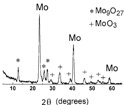
Fig. 15. XRD patterns of an annealed Mo-substrate showing, beside Mo structure, there are two structures of Mo oxides, namely MoO 3 and Mo 9 O 27
