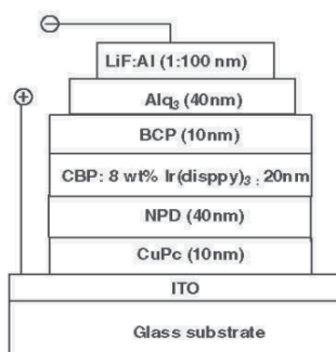
Fig. 10. The device structure of Ir(disppy) 3 or Ir(ppy) 3 based PHOLEDs.
