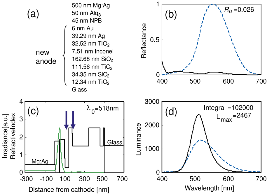
Fig. 8. (a) OLED design; (b) calculated reflectance (solid line) with the photopic curve (dash line) and the value of the luminous reflectance R_D ; (c) refractive index profile (step) and irradiance profile inside the OLED, with the arrows showing the metal layers, and the emitting layer marked in black.
