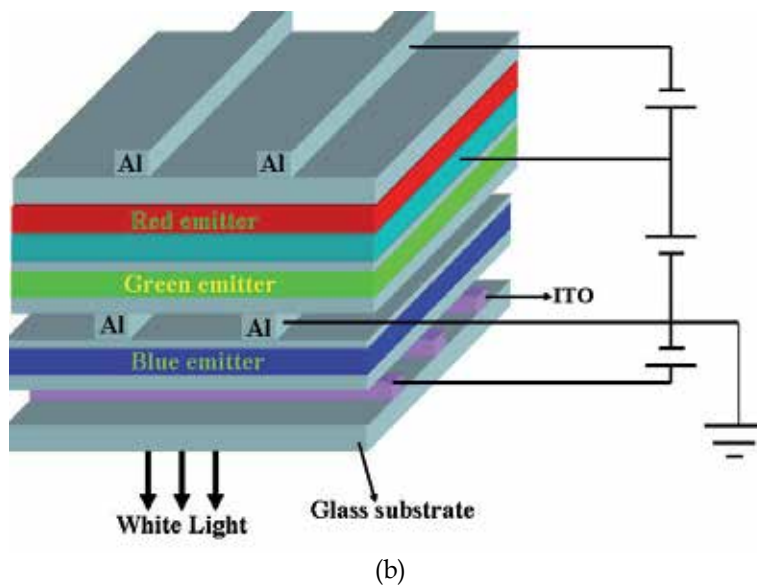
Fig. 8. Schematic diagram of (a) horizontally and (b) vertically stacked OLED.
