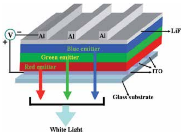
Fig. 7. Schematic diagram of multilayer white OLED
