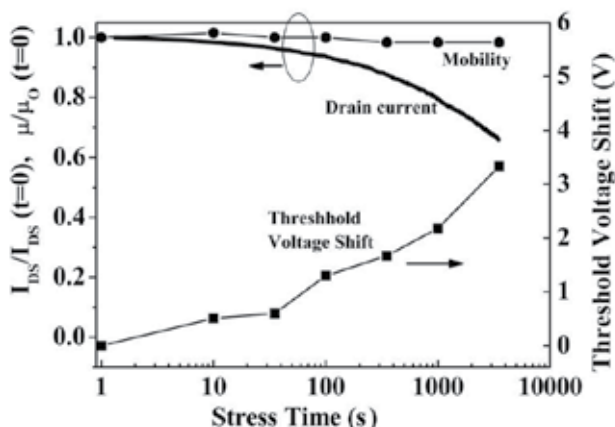
Fig. 13. Drain current, mobility, and threshold voltage transition of a-Si:H TFT under a bias-temperature-stress measurement ( V_{GS}=V_{DS}=15 V, 65 °C). The current drop is attributed to the threshold voltage shift in a-Si:H TFT.
