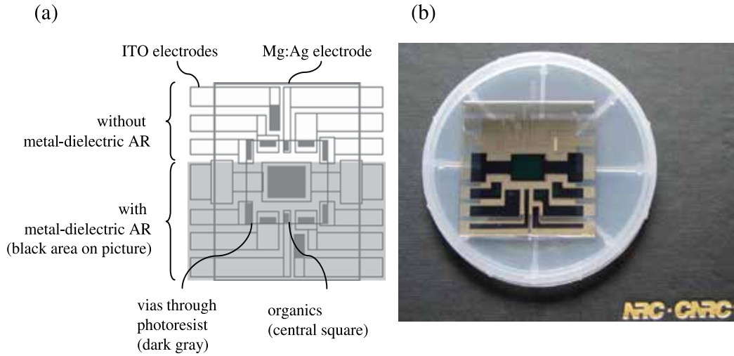
Fig. 9. (a) Schematic bottom view of multi-segment OLED device with and without metal-dielectric AR. (b) Picture of such a device after fabrication. This device corresponds to the design presented in Figure 8.
