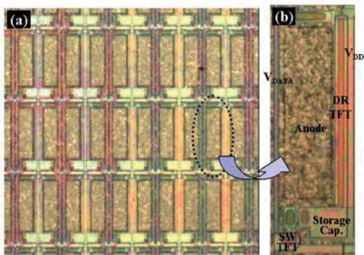
Fig. 19. (a) a-Si:H TFT array fabricated on a metal foil substrate (b) magnification of one pixel including 2-transistor and 1-capacitor.
