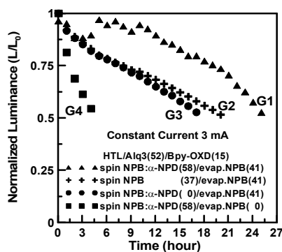
Fig. 10. The lifetime of flexible OLEDs with different HTL structures, and the devices were packaged by evaporating m-MTDATA 500 nm on the device surface
