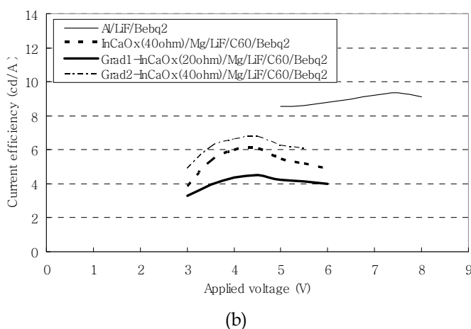
Fig. 27. The performances of OLEDs with ICO and gradient doped ICO; (a) current density-voltage and (b) current efficiency-voltage.
