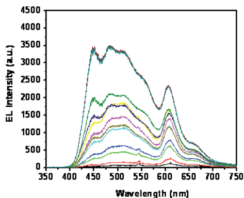
Fig. 14 EL spectrum of WOLED at different bias voltage (6 to 12 V).
