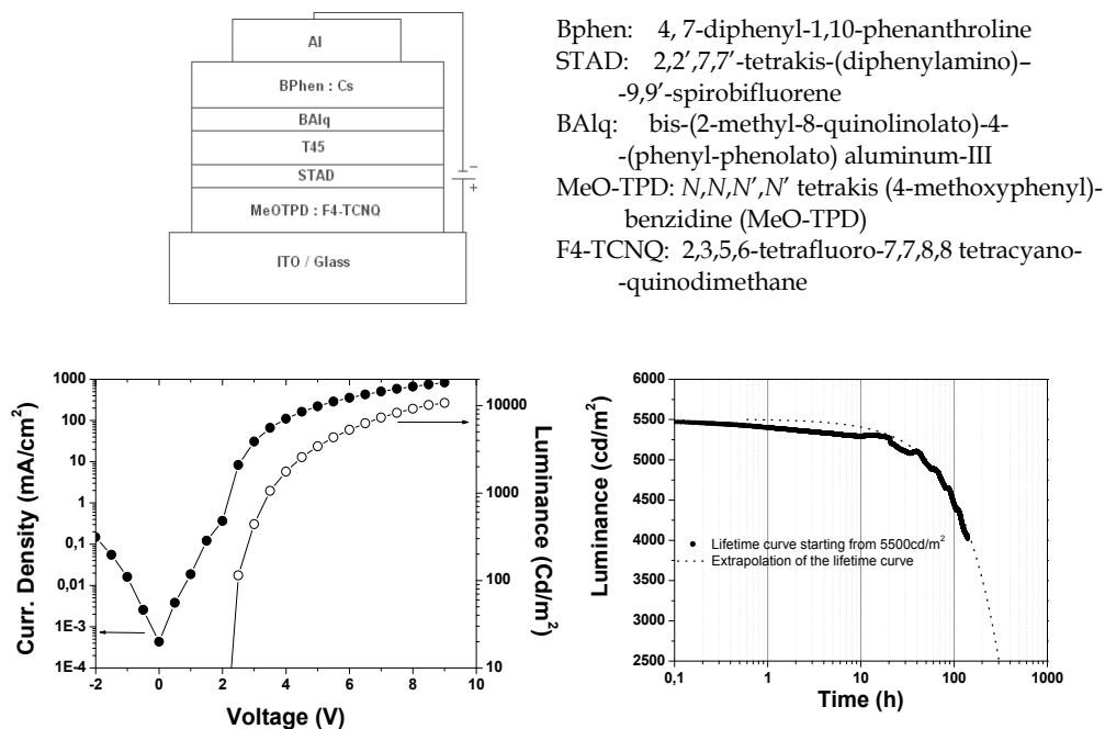
Fig. 10. Top: device structure. Bottom: (A) Luminance-Current Density vs. Voltage (left); Luminance decay time for a starting value of 5500Cd/m 2 at fixed current density (right).
