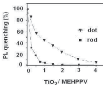
Fig. 3. MEH-PPV luminescence quenching vs. \text{TiO}_2 /polymer volume ratio at \lambda = 480 nm (Petrella et al., 2004)
