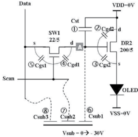
Fig. 15. Pixel circuit considering parasitic capacitances and substrate capacitances. The size of switching and driving TFT is 22/5 \mu\text{m} and 200/5 \mu\text{m} , respectively. Node A means the floating gate electrode of the driving TFT.
