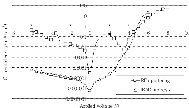
Fig. 24. Current density-voltage curves of ITO-deposited OLED with RF sputtering and ITO-deposited with IBAD thermal process at 85°C.
