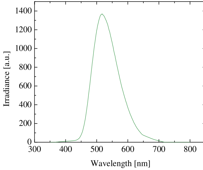
Fig. 2. Emission spectrum of Alq 3 . The curve was taken as representing I_0 inside the OLED emitting layer.
