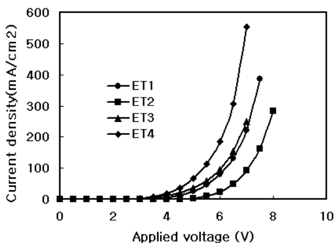
Fig. 12. Voltage-Current curve of ADN series ETMs
