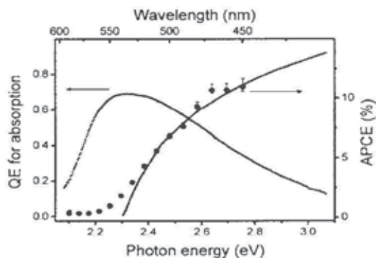
Fig. 7. Comparison of APCE curves obtained experimentally (solid circles) and theoretically (solid line) for 50-nm-thick MEH-PPV (Burlakov et al., 2005)
