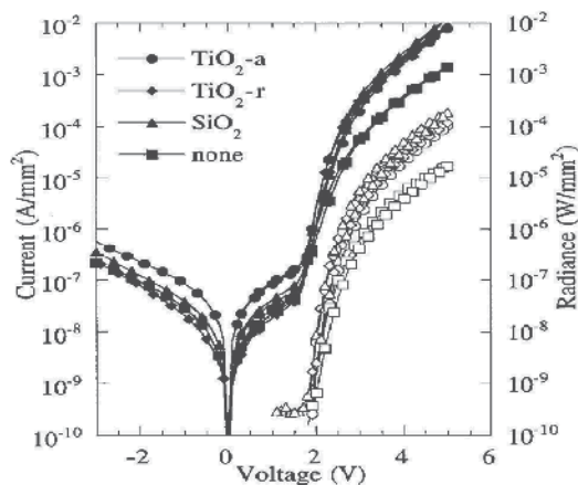
Fig. 8. Current-voltage and radiance-voltage curves for 1:1 \text{TiO}_2 (anatase)/MEH-PPV (circles), 1:1 \text{TiO}_2 (rutile)/MEH-PPV (diamonds), 1:1 \text{SiO}_2 /MEH-PPV (triangles), and for MEH-PPV film with no nanoparticles (squares). Close symbols are for current. Open symbols are for radiance. 1\text{W}/\text{mm}^2 = 7.3 \times 10^7 \text{ cds}/\text{m}^2 (Carter et al., 1997)
