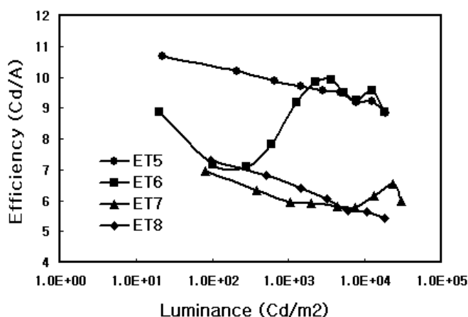
Fig. 15. Luminance-Current efficiency curve of Phenanthroline series ETMs
