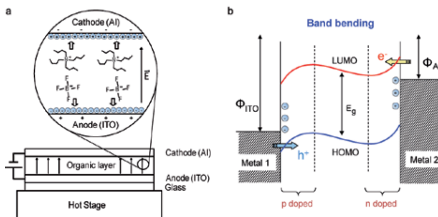
Fig. 1. (a) Architecture of the devices showing the fabrication of the device with the simultaneous electrical and thermal treatments. (b) Schematic energy levels of the device after the simultaneous treatments.
