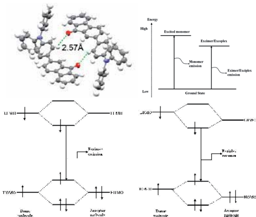
Fig. 15. Schematic diagram showing the formation of excimer/excimer in organic molecule and light emission from excimer/excimer molecule is red shifted from the excited monomer emission.
