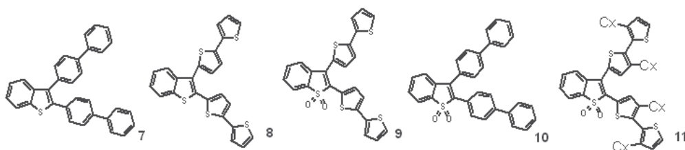
Scheme 5. Molecular structure of V-shaped oligothiophene-S,S-dioxides 7-11. Cx = Cyclohexyl.
