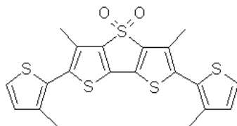
3,5-Dimethyl-2,3'-bis(3-methylthiophene)-dithieno[3,2-b;2',3'-d]thiophene-4,4-dioxide (DTTOMe4)
