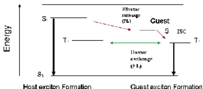
Fig. 13. Energy transfer mechanism for \text{Zn(hpb)}_2 doped with phosphorescent dopant Ir(btp) _2 acac in electroluminescence process.
