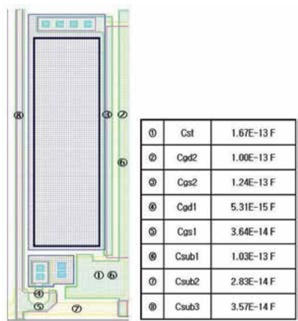
Fig. 16. Lay-out of one pixel and simulation parameters to get the voltage at the floating gate electrode by the substrate bias
