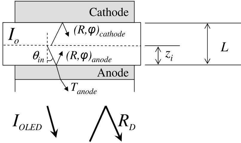
Fig. 1. Schematic view of an OLED showing its Fabry-Perot-like structure and the parameters used in Eq. 3.
