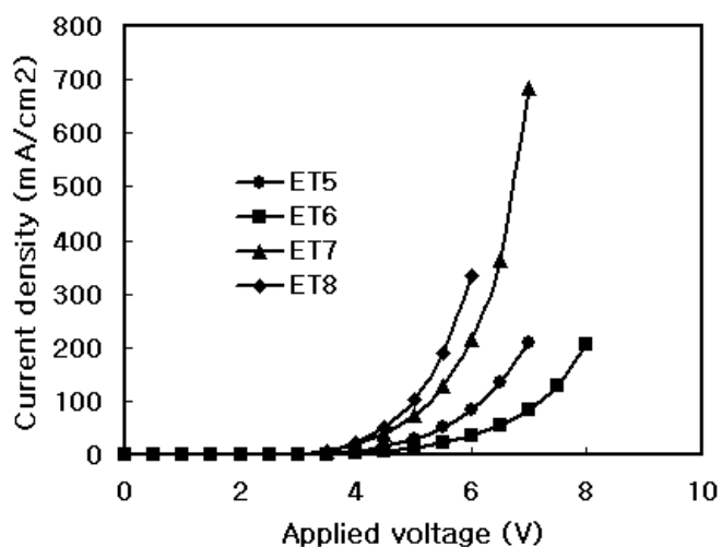
Fig. 14. Voltage-Current curve of Phenanthroline series ETMs
