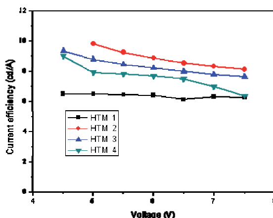
Fig. 7. Current efficiency-applied voltage characteristics of devices III-VI.
