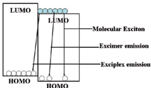
Fig. 16. Formation of excimer and exciplexes
