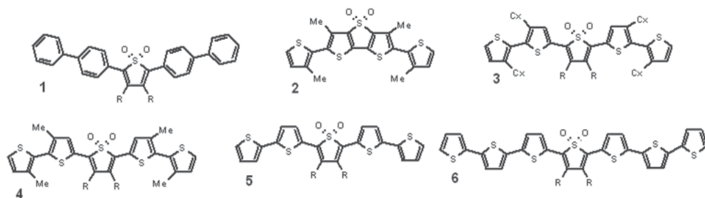
Scheme 4. Molecular structure of linear oligothiophene-S,S-dioxides 1-6. R = Hexyl; Me = Methyl; Cx = Cyclohexyl.
