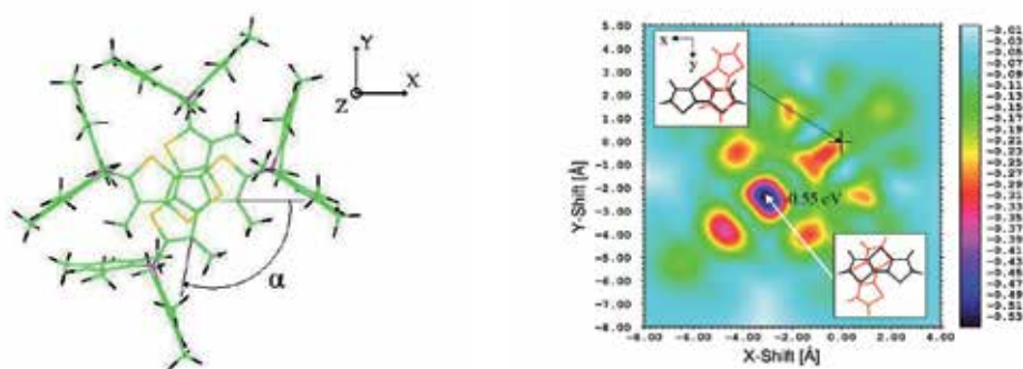
Fig. 8. Molecular structure of two interacting molecules forming a cross-like dimer (left) and (right) Intermediate neglect of differential overlap/single configuration interaction (INDO/SCI) excitation-energy shifts due to intermolecular interactions. The scale on the right corresponds to calculated excitation energy shifts.
