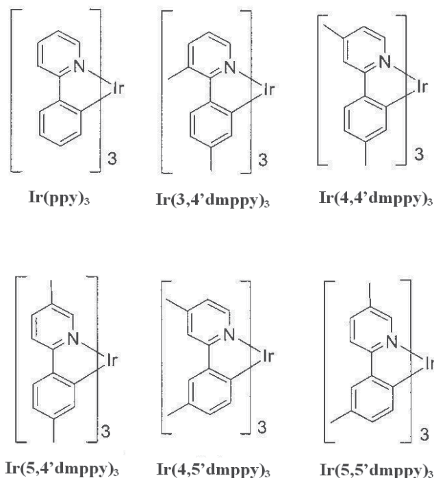
Fig. 1. The molecular structures of methyl substituted \text{Ir}(\text{dmppy})_3 derivatives.
