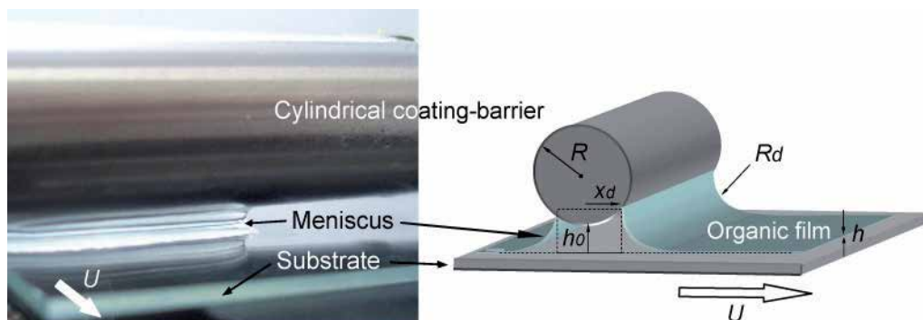
Fig. 9. A photograph (left) with schematic illustration (right) of the premetered horizontal-dip (H-dip) coating process described herein: a cylindrical coating barrier (SUS steel) with a diameter R , a gap height h_0 , and a carrying speed U . (Park & Han, 2009)
