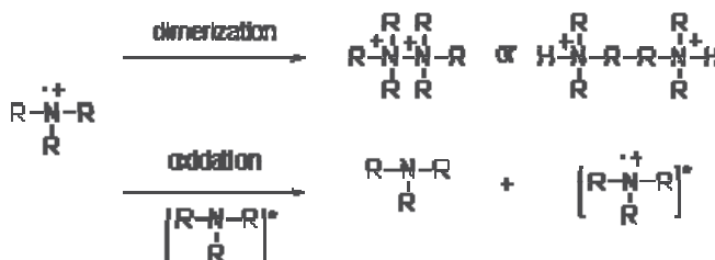
Scheme 2. Dimerization vs oxidation reaction
