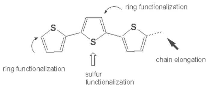
Scheme 1. Functionalization modalities in oligothiophenes
