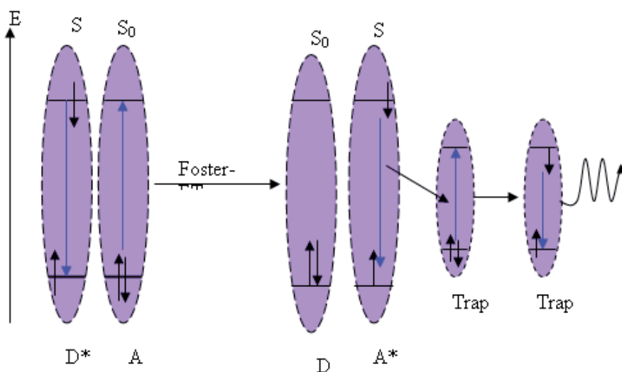
Fig. 20. Simplified scheme of resonant energy Förster energy transfer between a donor (D) and an acceptor (A). Right side shows energy transfer to a trap which is lower in its singlet energy.
