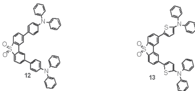
Scheme 6. Molecular structure of branched oligomers 12 and 13.
