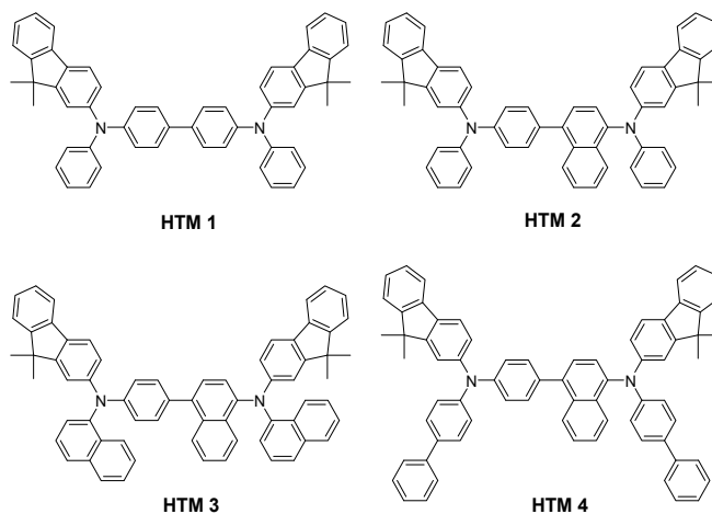
Fig. 2. Hole-transporting materials
