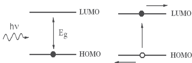
Fig. 1. Formation of “electron-hole pair” induced by an excitation from an external energy source (Klabunde, 2001)
