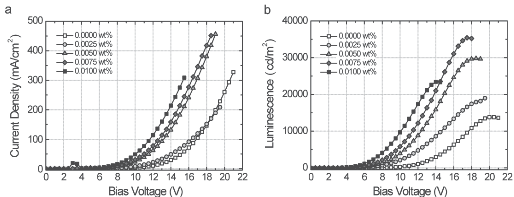
Fig. 8. Characteristics of J-V (a) and L-V (b) for the single-layered ionic p-i-n PHOLEDs with various concentrations of doped salt of \text{Bu}_4\text{NBF}_4 . (Park et al., 2008)
