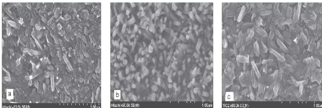
Fig. 17. FE-SEM pictures of annealed titanium surfaces: (a) 700 °C for 1 h (TC1), (b) 700°C for 1.5 h (TC2) and (c) 700°C for 2 h (TC3). The thickness of nc-TiO 2 layers is of 100 nm, 200 nm and 150 nm, respectively for TC1, TC2 and TC3 samples
