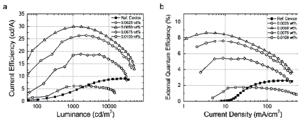
Fig. 5. Current efficiency ( \eta_c ) vs. luminance (a) and external quantum efficiency ( \eta_{\text{ext}} ) vs. current density (b) of the single-layered \text{Ir}(\text{ppy})_3 sample devices (open symbols) with various concentrations of \text{Bu}_4\text{NBF}_4 and reference device (closed square). (Oh et al., 2007)
