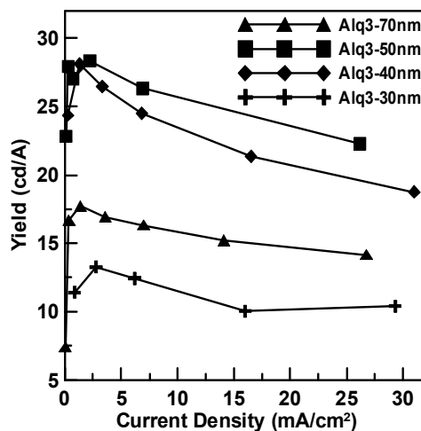
Fig. 3. Luminance efficiency-current density curves for different thicknesses of ETL
