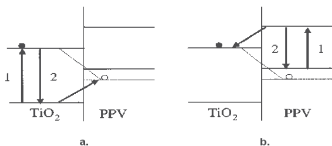
Fig. 6. Schematic diagram of the various excitation, charge transfer, and decay pathways available in a conjugated polymer nanocrystal composite (Salafsky, 1999)
