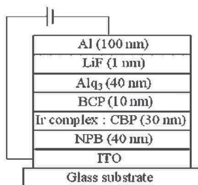
Fig. 13. The device structure of PHOLEDs based on Ir complex, Ir(chpy) 3 or Ir(mchpy) 3 .
