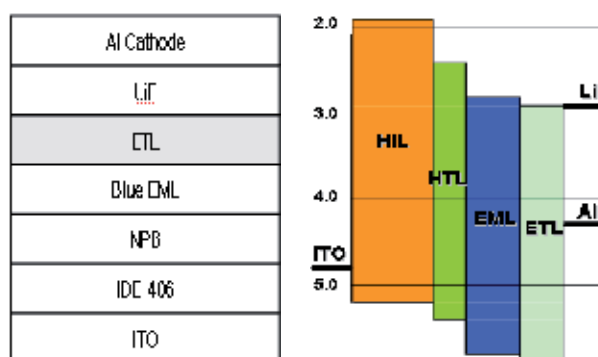
Fig. 11. Blue OLED structure and Energy diagram
