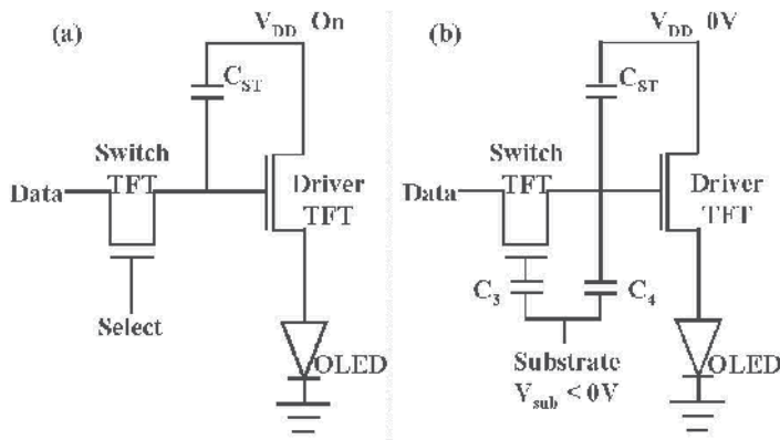
Fig. 14. Two-transistor and one-capacitor pixel circuits for AMOLED: (a) the operating circuit and (b) the recovery circuit during idle time ( V_{SUB} < 0 V, V_{DD} = 0 V)
