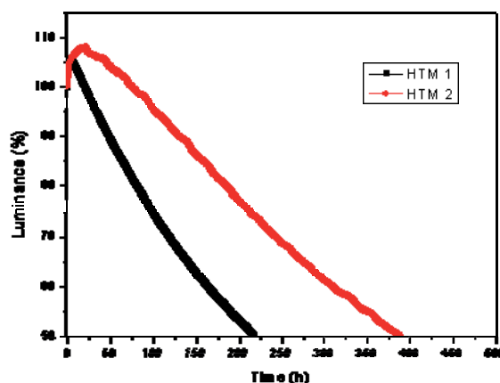
Fig. 8. The life-time characteristics of the two devices at 100mA/cm 2 ; device III (■), device IV (●)
