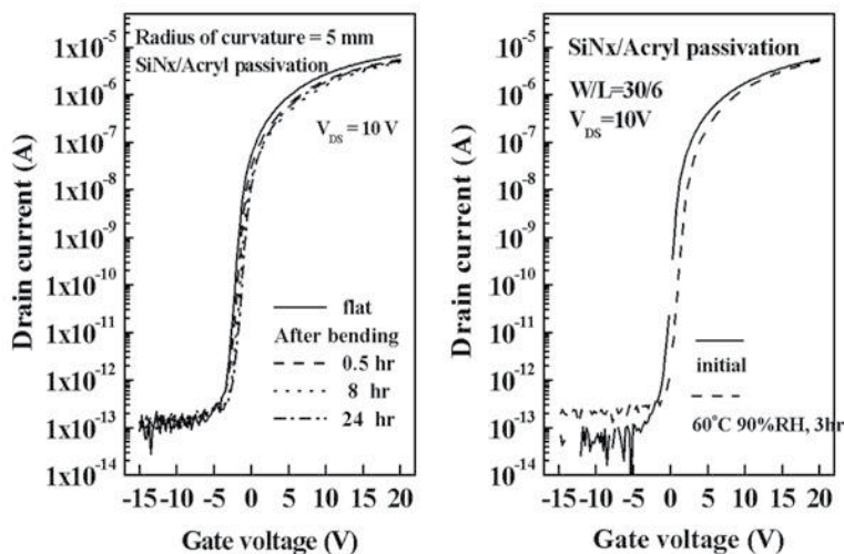
Fig. 11. Transfer characteristics for the hybrid passivation TFT as bending duration time. The radius of curvature R is 5 mm (left). Transfer characteristics for the hybrid passivation TFT stored at 60°C and 90 % RH for 3 hour (right)
