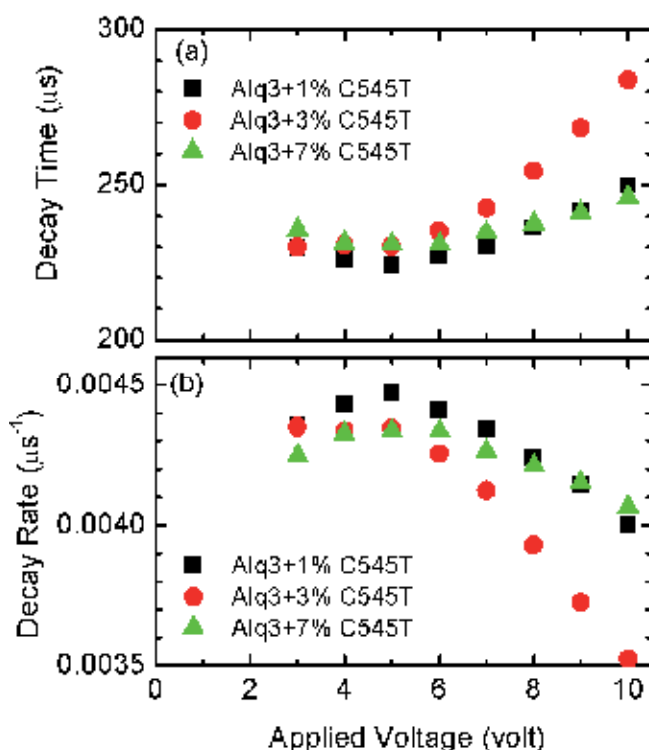
Fig. 7. (a) Decay times as well as (b) decay rates as a function of applied voltage for the three doped samples.
