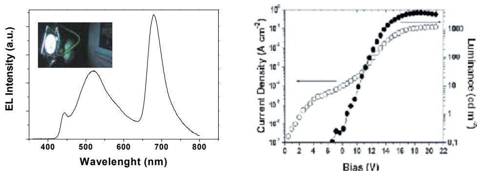
Fig. 9. EL spectrum of device with d_{LiF} \approx 5 nm (left) (inset: image of a large area device); Luminance-current density-voltage characteristics (right).
