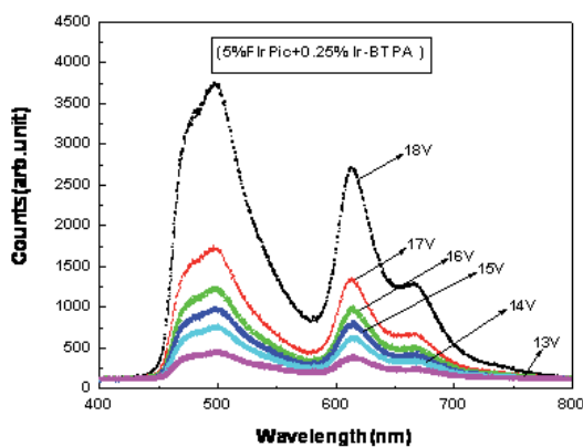
Fig. 12. Electroluminescence spectrum of WOLED at different applied voltages
