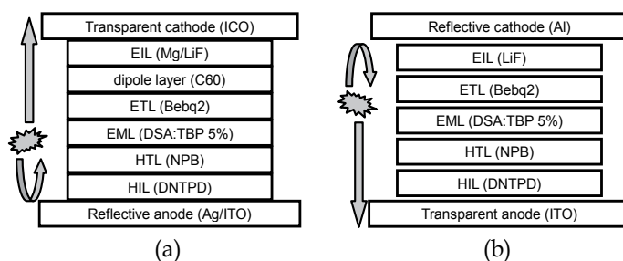
Fig. 25. Schematic device structures of (a) TEOLED with transparent cathode and (b) conventional OLED.
