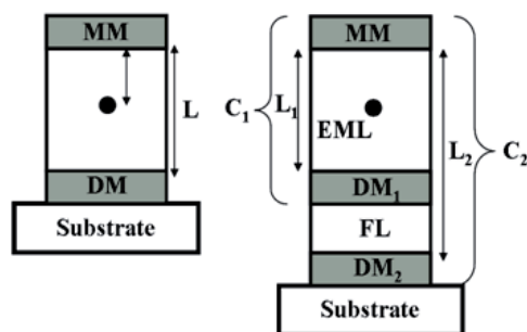
Fig. 18. Concept of (a) usual cavity and (b) multiwavelength resonant cavity (MWRC).
