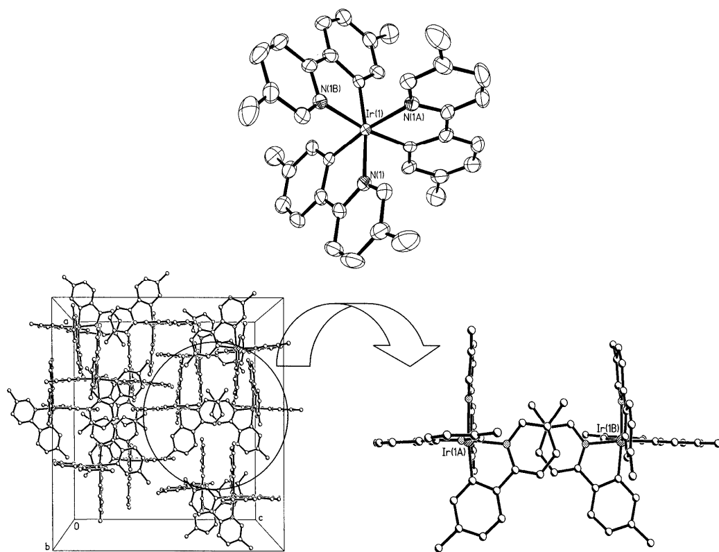
Fig 3. Top: Molecular structure of \text{Ir}(\text{4,5'-dmppy})_3 with atom labeling schemes and 50% thermal ellipsoids; all hydrogen atoms have been omitted for clarity; bottom: crystal packing diagram between two adjacent molecules of \text{Ir}(\text{4,5'-dmppy})_3 showing the intermolecular interaction in the solid state.
