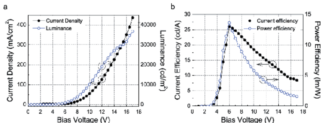
Fig. 12. (a) J - V and L - V characteristics of the ionic p - i - n PHOLED made using the H-dipping process. (b) \eta_c - V and \eta_p - V characteristics of the studied PHOLED.
