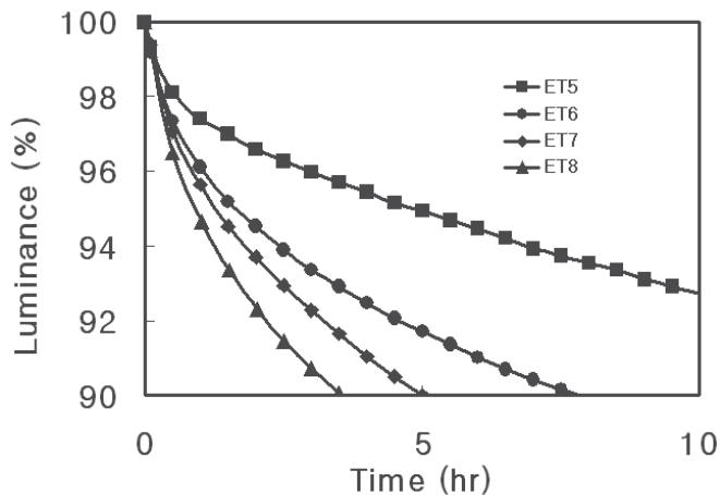
Fig. 19. Initial luminance decrease tendency of devices with Phenanthroline series ETMs at 100 \text{ mA/cm}^2 relatively rapid degradation appearance.
