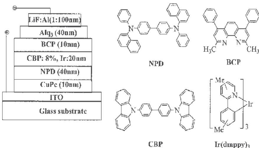
Fig. 5. Device structure and molecular structures of the materials used in the device.
