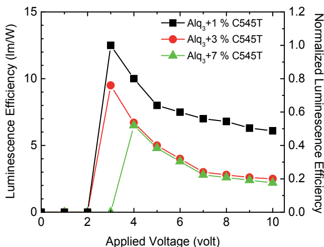
Fig. 8. Luminescence efficiency and normalized quantum efficiency as a function of applied voltage for the three doped samples.
