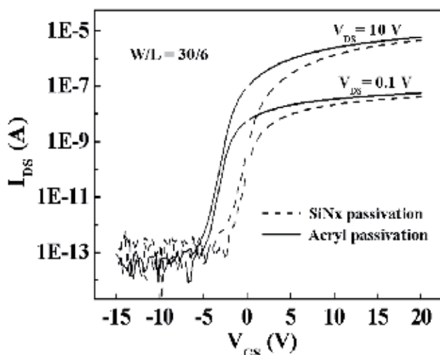
Fig. 5. Transfer characteristics of a-Si:H TFTs as passivation materials: SiNx and acrylic polymer. The size of TFT is W = 30 \mu\text{m} and L = 6 \mu\text{m} .
