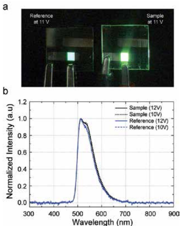
Fig. 6. Upper: A photograph of the operating sample device (right) and reference device (left). Lower: Normalized EL spectra for the operating sample device and reference device. (Park et al., 2008)
