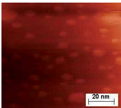
Fig. 10. AFM of a PEDOT+nc- \text{TiO}_2 composite film with embedding of 20 wt.% \text{TiO}_2 nanoparticles
