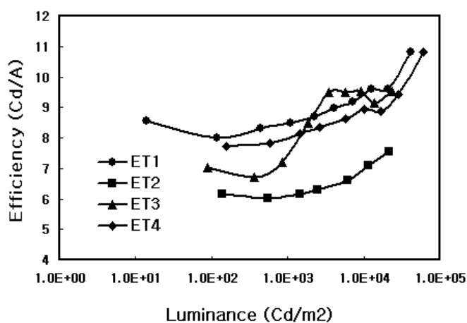
Fig. 13. Luminance-Current efficiency curve of ADN series ETMs
