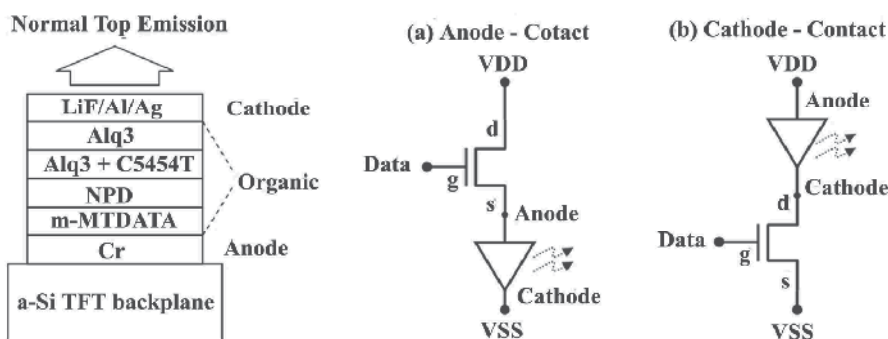
Fig. 21. Structure and circuit implementation of normal top-emission AMOLED (TOLED) pixel: (a) anode-contact with a-Si:H TFT (ACTOLED) and (b) cathode-contact with a-Si:H TFT (CCTOLED)
