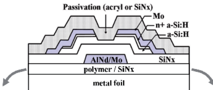
Fig. 6. Cross section of an inverted staggered type TFT fabricated on a flexible metal substrate. The arrows indicate the bending direction.
