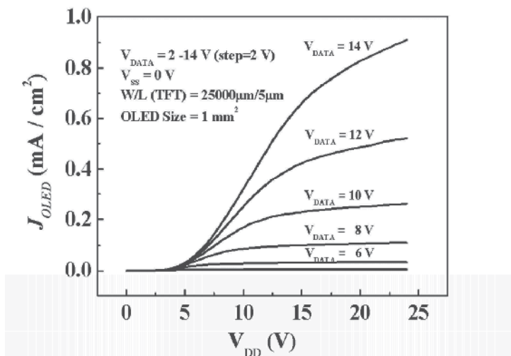
Fig. 25. Current density of the OLED as a function of V_{DD} and V_{DATA}
