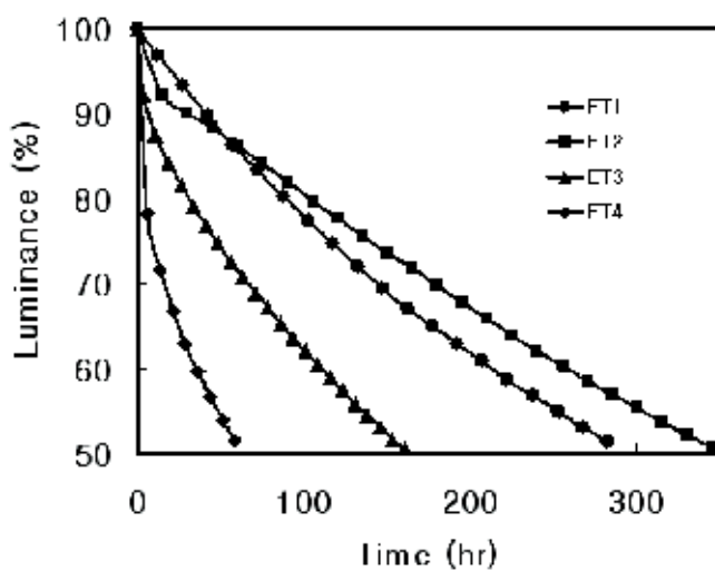
Fig. 16. Life time (half-life) tendency of devices with ADN series ETMs at 100mA/cm 2
