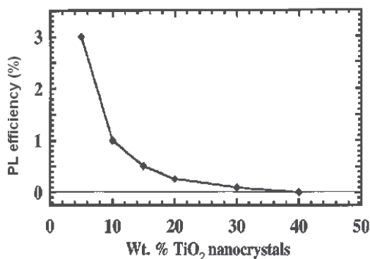
Fig. 5. Absolute photoluminescence (PL) efficiency of PPV: \text{TiO}_2 composites as a function of wt% \text{TiO}_2 nanocrystals (Salafsky, 1999)
