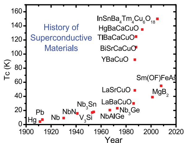
Fig. 1. Survey diagram for superconductive materials. InSnBa_4Tm_4Cu_6O_{18+} is a multiphase superconductor with a possible superconductivity at 150 K (Patent No.: US60/809,267) and T_c of this family is up to about 250 K in 2010.
