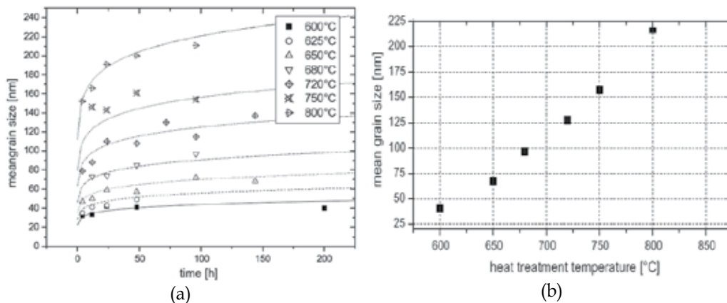
Fig. 2. (a) The change in average grain size with the increase in annealing time at different temperatures is shown. (b) The increase in average grain size with temperature after fixed annealing time of 100 h is shown (Müller & Schneider, 2008).
