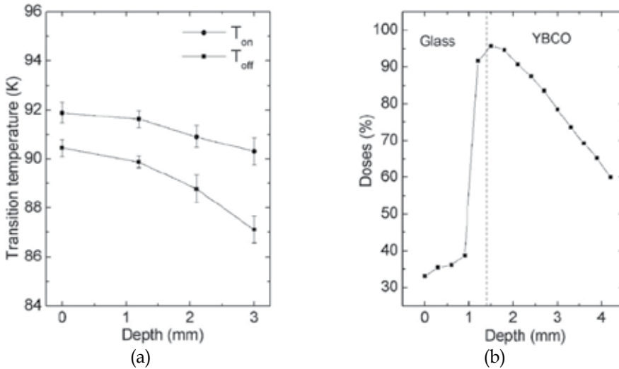
Fig. 13. (a) In-depth T_c profile in a ^{137}\text{Cs} gamma irradiated YBCO sample, T_c measurements were performed through step by step sample polishing. (b) Energy deposition distribution calculated for a model irradiation experiment by means of the EGS-4 code (Leyva et al., 2002a).
