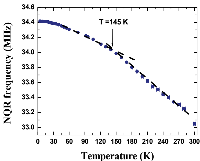
Fig. 6. The temperature dependence of ^{123}\text{Sb} NQR frequency \nu_{Q1} (transition \pm 1/2 \leftrightarrow \pm 3/2 ) for \text{Ag}_5\text{SbS}_4 . Arrow points to the positions of the change of slope in the \nu_{Q1}(T) dependence at 145 K, curves are guides for eyes. For details, see text.
