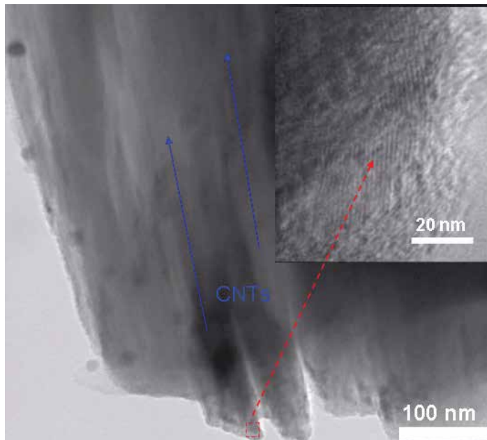
Fig. 4. TEM images of CNT doped \text{MgB}_2 show straightened CNTs in the same processing direction in the \text{MgB}_2 matrix. The inset is a high resolution image of a CNT (Dou et al., 2006)
