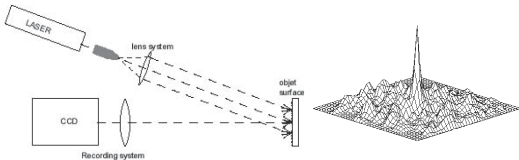
Fig. 2. (a) Digital Speckle Photography recording setup. (b) Plot of a 2D cross correlation function.
