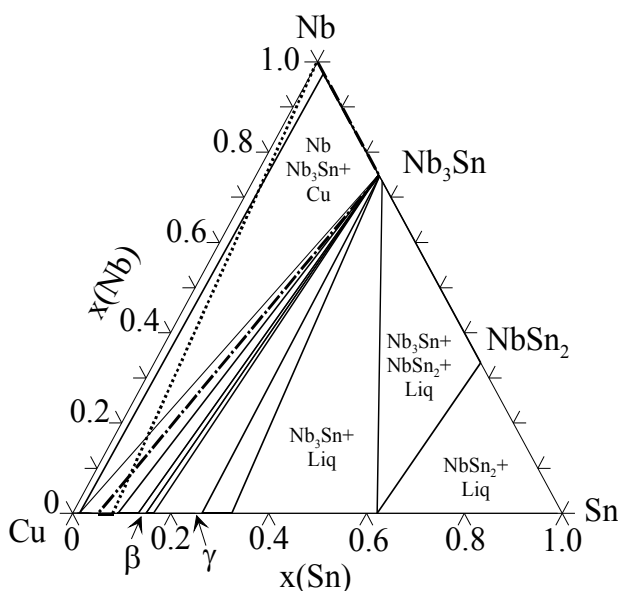
Fig. 15. Calculated Cu-Nb-Sn isothermal section at 700 °C. Dotted line is the contact-line (C.L.) between the end-members and the dashed-dotted line shows the diffusion path.
