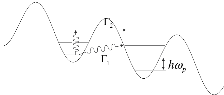
Fig. 10. A schematic of the enhanced macroscopic quantum tunneling in a single Josephson junction due to photon excitation. In each potential valley, the quantum states may form a harmonic oscillator ladder with a spacing of \hbar \omega_p . The absorption of photon energy may lead to an inter-valley resonant tunneling \Gamma_1 , and a tunneling followed by an inner-valley excitation, \Gamma_2 . The enhancement in macroscopic quantum tunneling results in a reduction of junction critical current.
