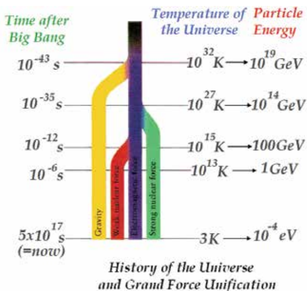
Fig. 13. The schematic representation of the history of the Universe and Grand force unification ( http://ircamera.as.arizona.edu/NatSci102/NatSci102/lectures/eraplanck.htm ).
