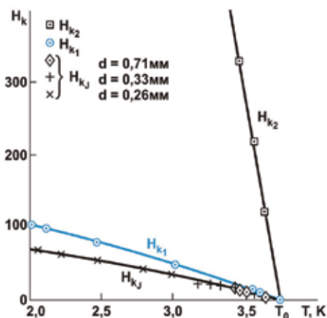
Fig. 14. Temperature dependents of H_{c1} , H_{c2} , H_c for single crystal Pb+66,7at.%Tl (Rjabinin & Shubnikow, 1935a).
