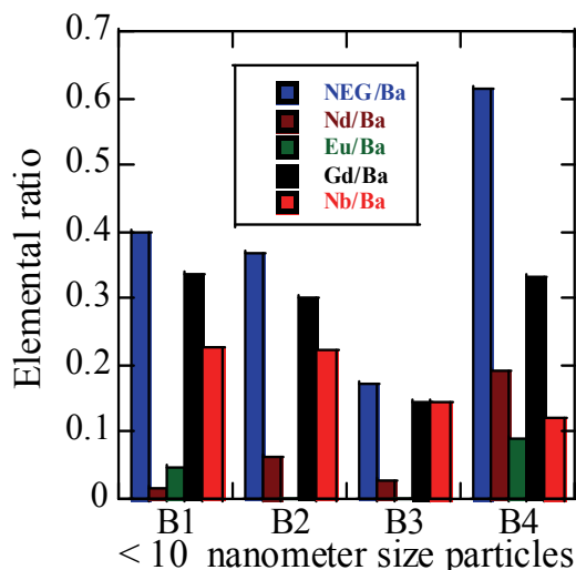
Fig. 17. The elemental content in the new nanoparticles in the material from Fig. 16. Note the significant amount of Nb in all nanoparticles.
