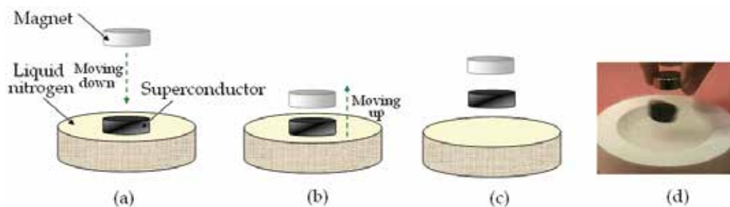
Fig. 10. The schematic representation and the photography of the magnetic suspension effect of the superconductors. (a)- The magnet moves down to the superconductor which is cooled in the liquid nitrogen (b),(c)- When the magnet is lifted up, the superconductor holds its magnetic lines and follows the magnet ( www.images.com/articles/superconductors/superconduction-suspension-effect.html ) (d)- The photography of the magnetic suspension effect of the superconductor. (Web site of the Superconductivity Laboratory of the University of Oslo, http://www.fys.uio.no/super/levitation/ )
