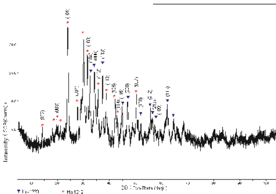
Fig. 7. XRD Pattern and (hkl) planes (Miller indices) of the optimally doped sample in 50 minutes counting. * indicates Hg-1212 and ▼ indicates Hg-1223 phases, respectively.
