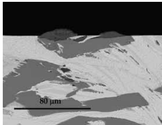
Fig. 18. SEM micrograph showing the decomposition of the (\text{Sr,Ca})\text{CuO}_2 phase due to the reaction with moisture.
