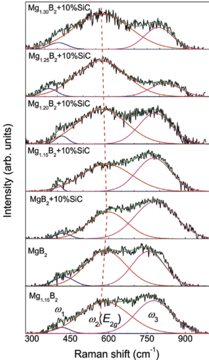
Fig. 12. (Color online) Ambient Raman spectra of MgB 2 , Mg 1.15 B 2 , and Mg x B 2 +10 wt % SiC ( x = 1.00, 1.15, 1.20, 1.25, and 1.30 ) fitted with three peaks: \omega_1 , \omega_2 , and \omega_3 . The dashed line indicates the vibration of the E_{2g} mode ( \omega_2 ) in different samples (Li et al., 2009a)
