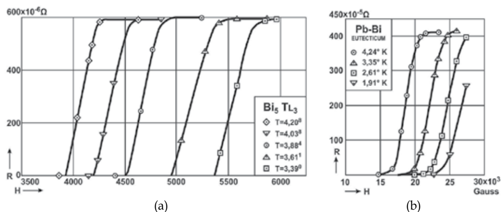
Fig. 6. Variation of electrical resistance of cylindrical specimens of superconducting alloys Bi-Tl (After De Haas & Voogd, 1929), Pb-Bi (After De Haas & Voogd, 1930) in transverse magnetic field at various temperatures.
