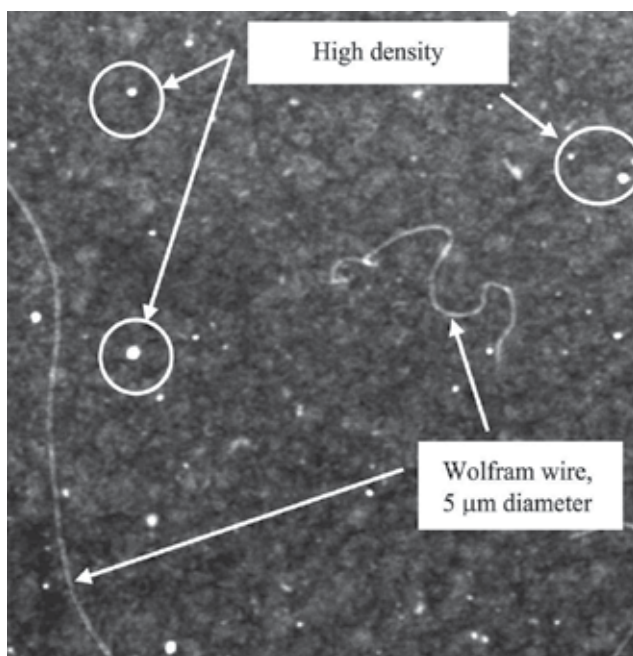
Fig. 12. Digital radiography of a MgB 2 sample and a W-wire.
