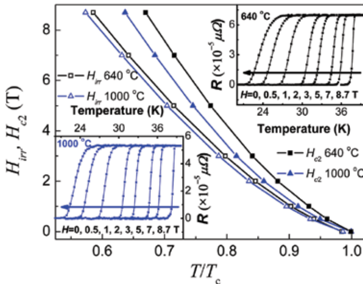
Fig. 8. The effects of sintering temperature on H_{c2} and H_{irr} of 10 wt%, \sim 15 nm SiC doped MgB 2 (Soltanian et al., 2005). The insets show the resistance as a function of temperature at different magnetic fields for samples sintered at 640 °C (upper right) and 1000 °C (lower left)
