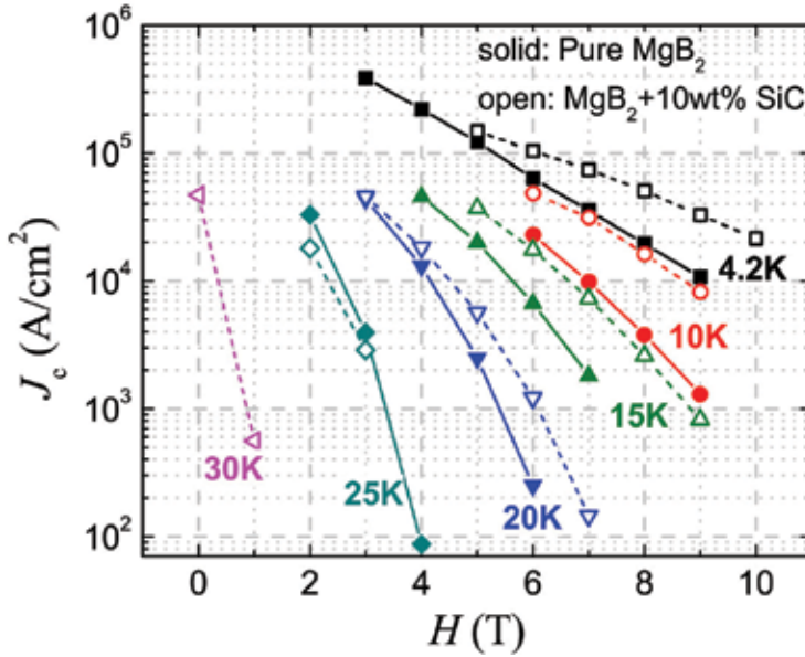
Fig. 7. Comparison of J_c of pure MgB 2 with that of a nanosized SiC doped sample at different temperatures (Dou et al., 2002b; Shcherbakova et al., 2006)
