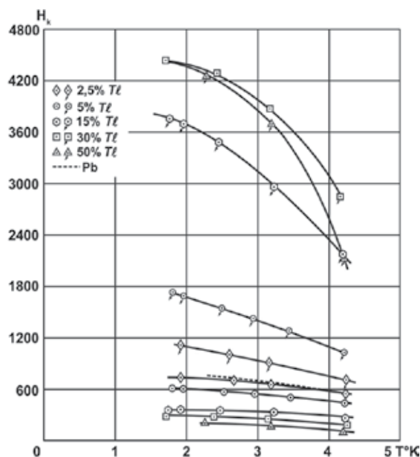
Fig. 20. Temperature dependence of H_{c1} and H_{c2} for single-crystals alloys Pb-Tl of the said concentrations and H_c for pure lead (After Schubnikow et al., 1936).
