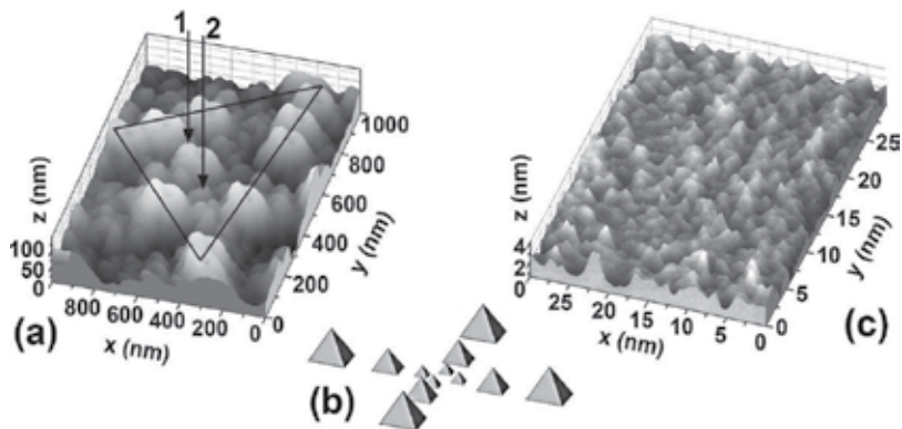
Fig. 5. (a) - STM image of the ultra-shallow boron diffusion profile prepared at the diffusion temperature of 800^\circ\text{C} into the Si (100) wafer covered previously by medium oxide overlayer X||[001] , Y||[010] , Z||[100] . Solid triangle and arrows that are labeled as 1 and 2 exhibit the microdefects with dimensions 740 nm, 225 nm and 68 nm, respectively, which are evidence of their fractal self-assembly. (b) - The model of the self-assembled microcavity system formed by the microdefects of the fractal type on the Si (100) surface. (c) - STM image of the ultra-shallow boron diffusion profile prepared at diffusion temperature of 900^\circ\text{C} into the Si (100) wafer covered previously by medium oxide overlayer. X||[001] , Y||[010] , Z||[100] .
