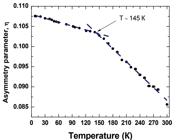
Fig. 8. The temperature dependence of asymmetry parameter, \eta , for \text{Ag}_5\text{SbS}_4 . Arrow points to the positions of the change of slope in this dependence at 145 K, curves are guides for eyes. For details, see text.
