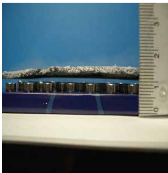
Fig. 8. The photograph of Meissner effect of the sample used in Fig. 7(b)
