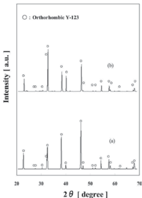
Fig. 3. X-ray diffraction patterns of the sheet samples prepared from the slurry with various PVA concentrations: (a) 0 and (b) 1 wt%.
