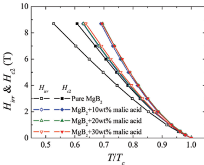
Fig. 16. H_{irr} and H_{c2} variations with doping content of malic acid in \text{MgB}_2 (Kim et al., 2006b)
