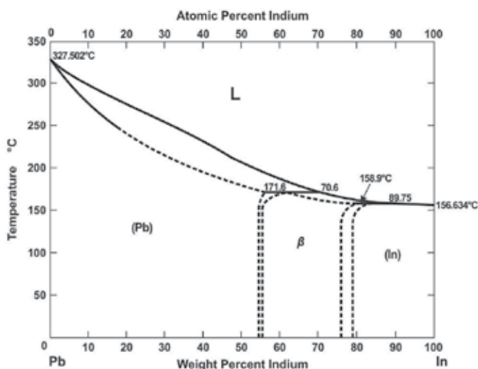
Fig. 15. Binary phase diagrams of the alloy Pb-In (After Massalski, 1987).
