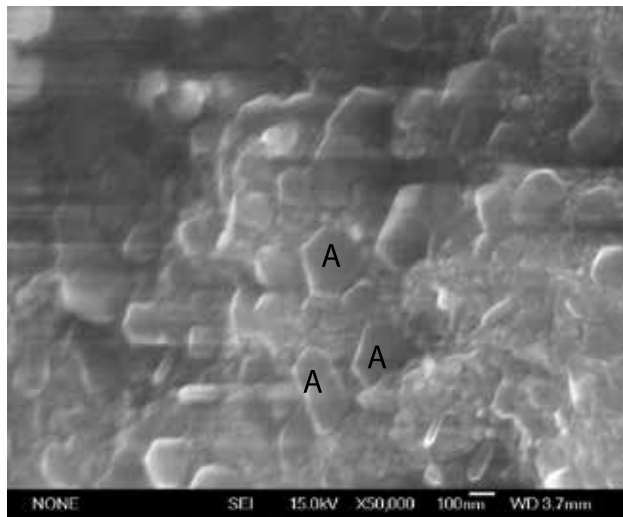
Fig. 6. (Zhang et al., 2009) Image of scanning electronic microscopy (SEM) of the superconducting MgB 2 -MgO composite. Examples of MgB 2 crystal grains were labelled by the letter "A".
