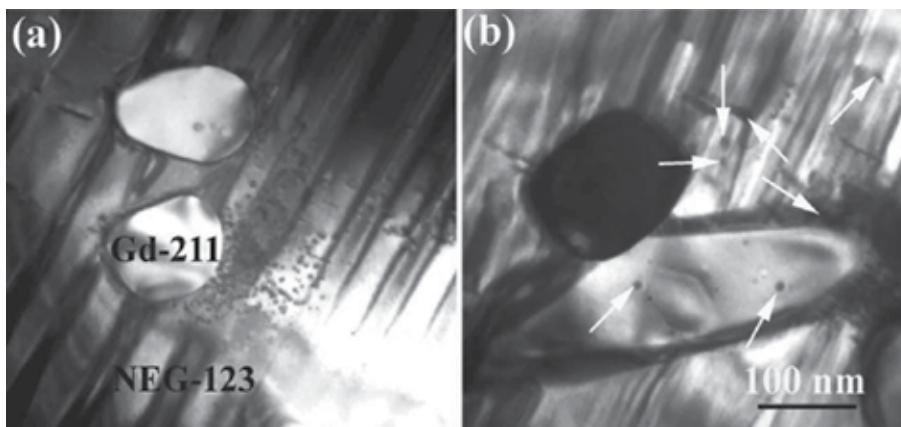
Fig. 13. Transmission electron micrograph of NEG-123 sample with 35 mol% Gd-211 (the initial average particle size 70 nm) and 0.1 mol% \text{MoO}_3 the arrows point to some of the smallest nanoparticles, of size below 10 nm.
