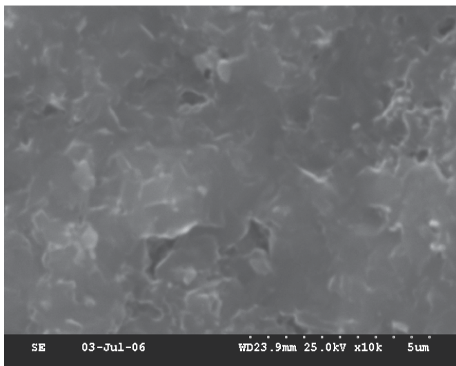
Fig. 13. Polycrystalline \text{MgB}_2 sample ( \times 10,000 ).
