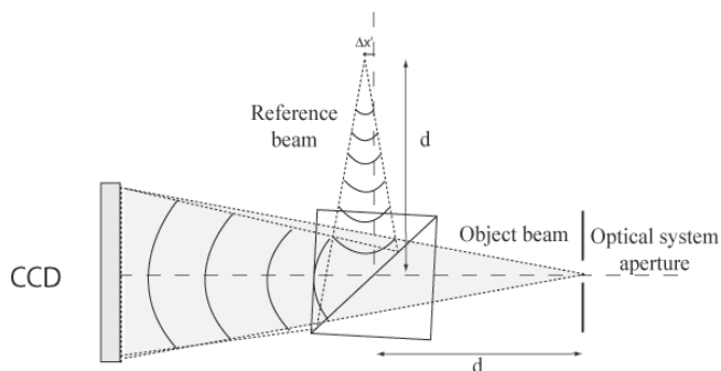
Fig. 4. Experimental setup used for introducing SPS in a DSPI system.
