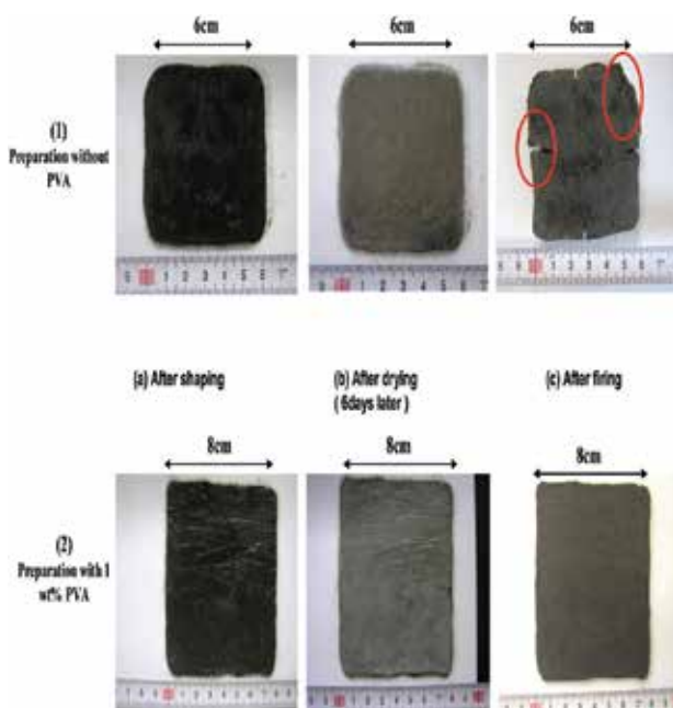
Fig. 2. The effect of PVA on the shaping of sample. Photographs of the samples prepared from the slurry containing (1) 0 and (2) 1 wt% PVA at (a) after shaping, (b) after drying (6 days later) and (c) after firing.
