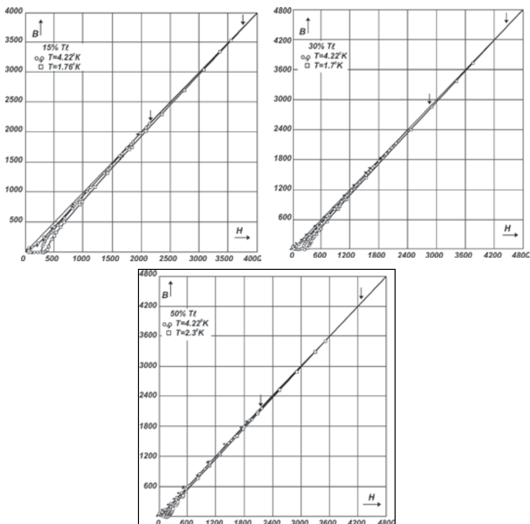
Fig. 18. The induction curve of long cylinders of single-crystals of alloys: Pb+15wt% Tl; Pb+30wt% Tl; Pb+50wt% Tl (After Schubnikow et al., 1936).
