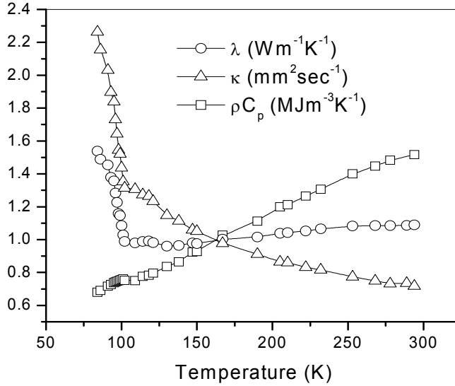
Fig. 6. Variation in thermal transport properties with temperature for the sample
