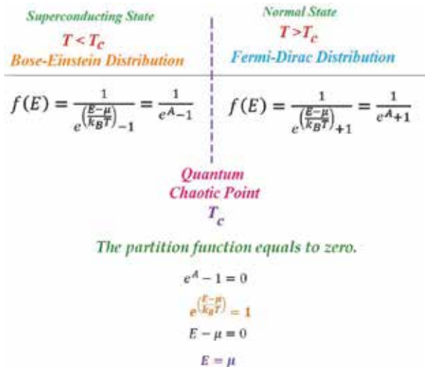
Fig. 5. The representative illustration of the distribution function at the vicinity of the critical Meissner temperature T_c . At the Meissner transition temperature, the partition function equals to zero that results in the equality of the chemical potential to the total energy of the system.
