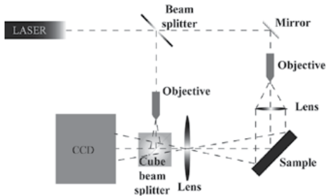
Fig. 3. Digital Speckle Interferometry setup
