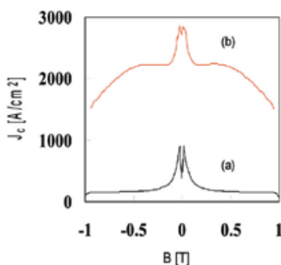
Fig. 10. The dependence of current density on magnetic flux density. Sample (a) was prepared with \text{YBa}_2\text{Cu}_3\text{O}_{7-x} powder made by conventional sintering method. Sample (b) was prepared with \text{YBa}_2\text{Cu}_3\text{O}_{7-x} powder made by MPMQ method.
