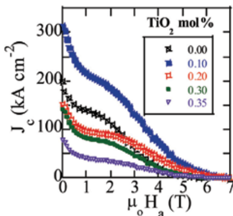
Fig. 7. Field dependence of the super-current density in NEG-123 samples with the same, 35 mol% content of Gd-211 (70 nm) but various contents of TiO_2 . All the samples were measured at T = 77 K with H_{||c} -axis. The current density increased in the whole field range up to the 0.1 mol% content of TiO_2 and decreased thereafter. Note the relatively high critical current density of 320 kA/cm 2 at self-field and 77 K, achieved with 0.1 mol% TiO_2 .
