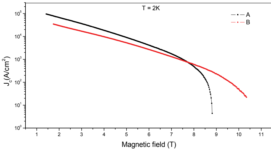
Fig. 6. J_c as a function of field. J_c for B is lower at low field but higher at high field .
