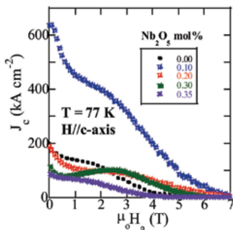
Fig. 14. Field dependence of the super-current density in NEG-123 samples with the same, 35 mol% content of Gd-211 (70 nm) but various contents of Nb 2 O 5 . All the samples were measured at T = 77 K with H \parallel c -axis. The current density increased in the whole field range up to the 0.1 mol% content of Nb 2 O 5 and decreased thereafter. Note the critical current density of 640 kA/cm 2 at self-field and 77 K, achieved with 0.1 mol% Nb 2 O 5 .
