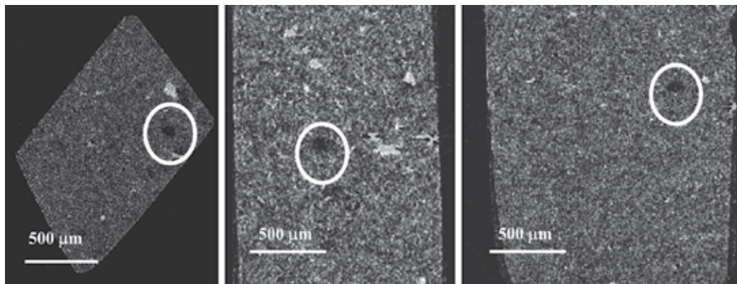
Fig. 11. Transversal, sagittal and longitudinal cross-sections revealing low density region; low density region size (inside circles) is of about 130 \mu\text{m} .
