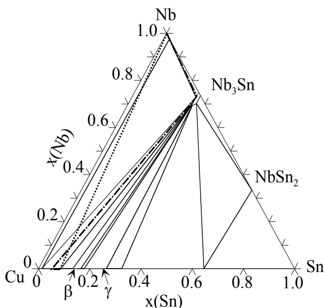
Fig. 16. Calculated Cu-Nb-Sn isothermal section at 700 °C, with 10 at-% Cu solubility induced to Nb 3 Sn. Dotted line is the contact-line (C.L.) between the end-members and the dashed-dotted line shows the diffusion path.
