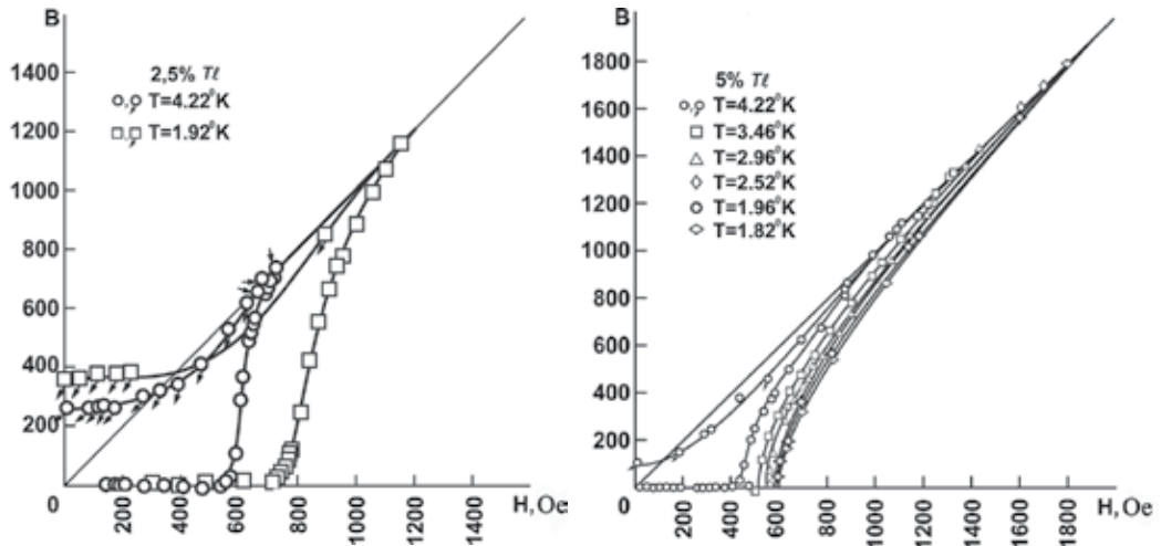
Fig. 17. The induction curve of long cylinders of single-crystals of alloys Pb+2,5wt% Tl; Pb+5wt% Tl (After Schubnikow et al., 1936).
