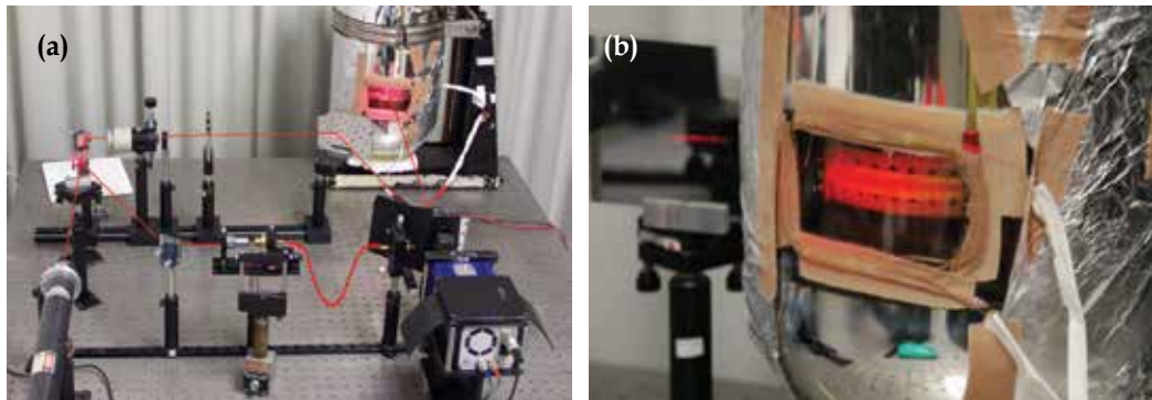
Fig. 5. (a) Experimental arrangement used to apply DSPI in cryogenic conditions. (b) Detail of the modification performed for placing the sample close to the dewar window in order to take measurements with the sample immersed in liquid nitrogen.
