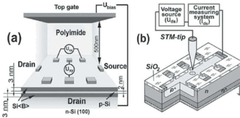
Fig. 8. (a) Schematic diagram of the devices that demonstrates a perspective view of the p-type Si-QW confined by the \delta -barriers heavily doped with boron on the n-type Si (100) surface. The top gate is able to control the sheet density of holes and the Rashba SOI value. The depletion regions indicate the Hall geometry of leads. (b) Planar field-effect silicon transistor structure with the STM tip, which is based on an ultra-shallow p + -diffusion profile prepared in the Hall geometry. The circle dashed line exhibits the point STM contact region.
