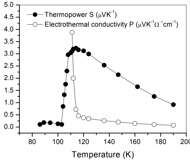
Fig. 9. Variation of thermoelectrical power ( S ) and electrothermal conductivity ( P ) with temperature for the sample
