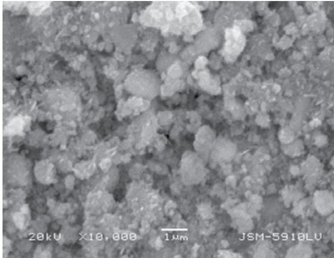
Fig. 10. The optimally oxygen doped Hg-1223 sample with rectangular shape. The SEM output has been taken at 20 kV and JSM-5910 LV ( T_c=140 K, t=1.098 μm)
