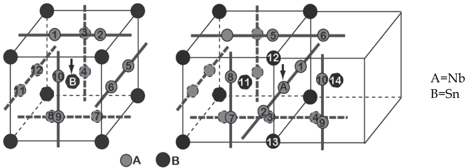
Fig. 9. A15 crystal structure is shown with the nearest neighbors of Nb and Sn.
