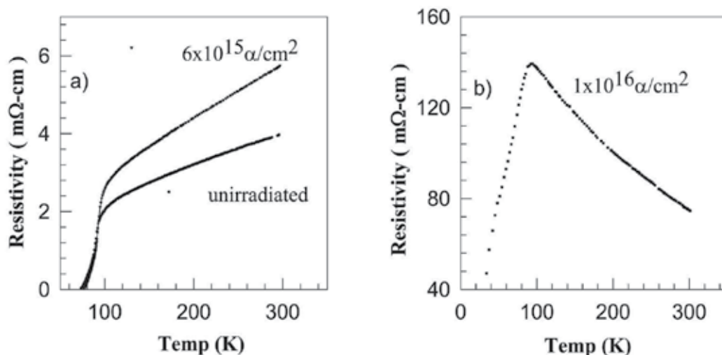
Fig. 3. (a) Resistivity of unirradiated, 6x10 15 α/cm 2 and (b) highest dose (1x10 16 α/cm 2 ) of polycrystalline of Bi-2212 as a function of temperature.
