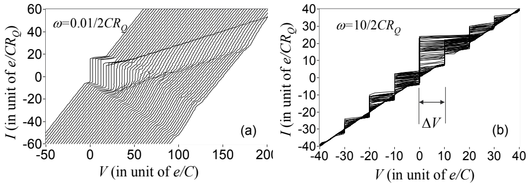
Fig. 2. The calculated current-voltage ( IV ) characteristics of an RC-shunted junction under the ac current driving of various amplitudes at a low frequency (a) and a high frequency (b). Note that the curves in (a) are shifted for clarity. With high frequency driving, the junction exhibits a mode-locking for superconducting phase at certain voltages with an equal spacing \Delta V = \hbar\omega/2e .
