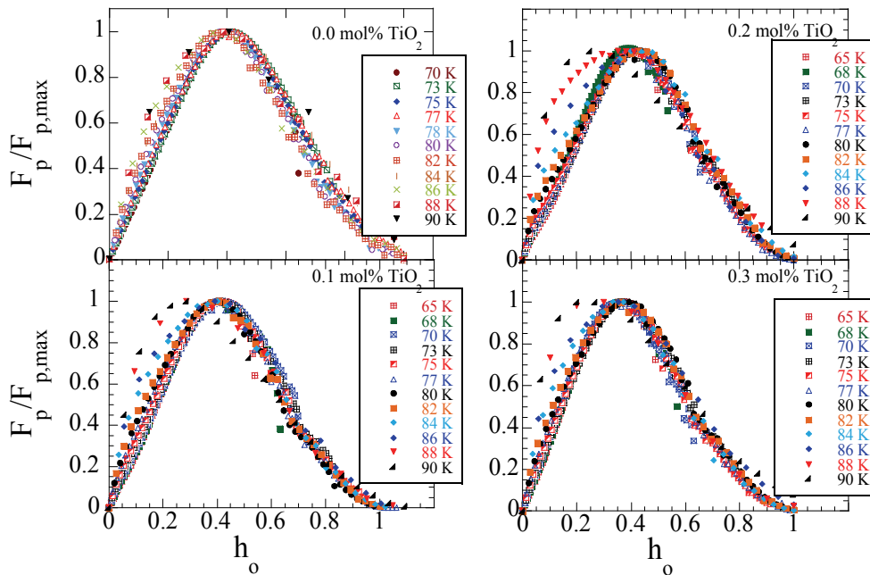
Fig. 10. Normalized pinning force density f=F_p/F_{p,max} as a function of reduced field h=B/B_{irr} of NEG-123 samples with the same, 35 mol%, content of Gd-211 (70 nm) but various contents of TiO 2 , for temperatures from 65 to 90 K.
