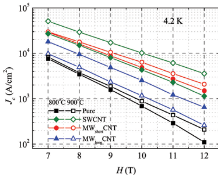
Fig. 5. Transport critical current at 4.2 K at fields up to 12 T for different CNT doped wires produced at sintering temperatures of 800 and 900 °C (Kim et al., 2006a)
