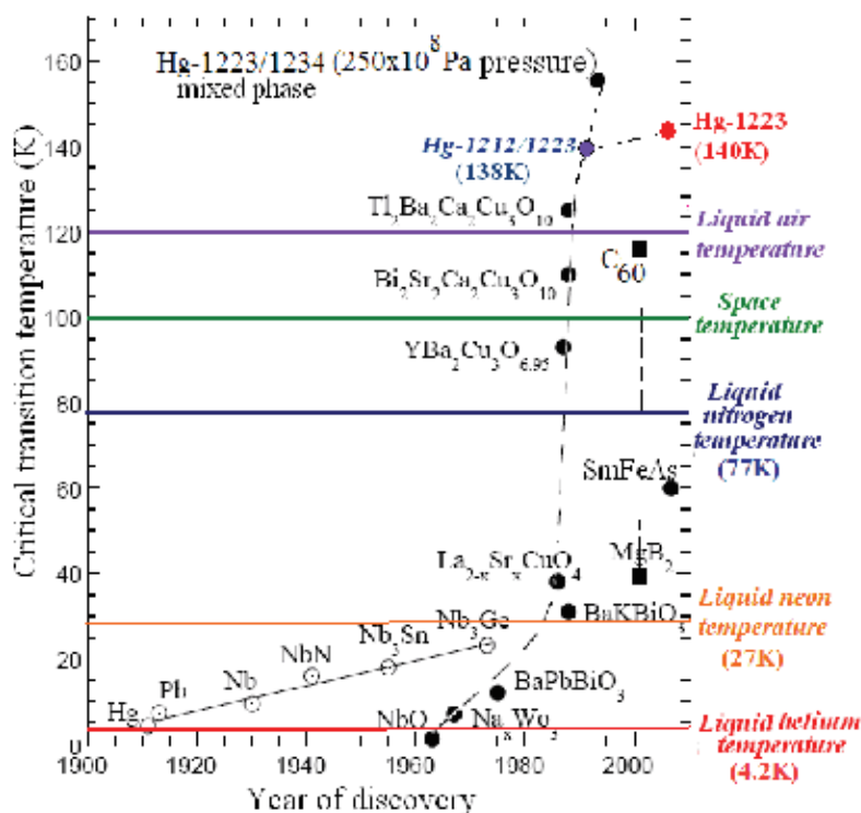
Fig. 1. Illustration of the years of discovery of some superconducting materials and their critical transition temperatures.
