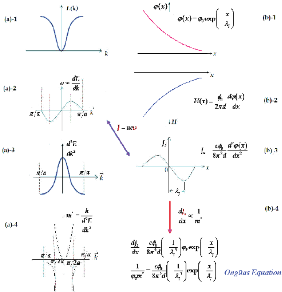
Fig. 3. The derivation procedure of the effective mass equation of the quasi-particles in the condensed matter physics and the mercury cuprates are given in (a)-1,2,3,4 and (b)-1,2,3,4, respectively. (b)-1 The phase versus length graphic for the low magnetic fields in the Josephson junction. (b)-2 The distance dependence of the magnetic field in the Josephson junction. (b)-3 The super current in the Josephson junction versus distance graph. (b)-4 The effective mass equation of the quasi-particles has been derived from the relation of the supercurrent density versus distance.
