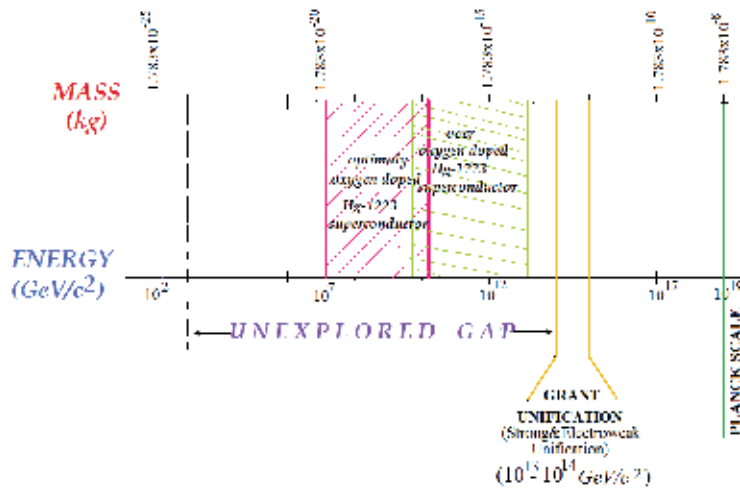
Fig. 9. The representative illustration of the net effective mass values for the optimally and over oxygen doped mercury cuprates in the hierarchic GeV/c^2 energy scale of high energy physics.
