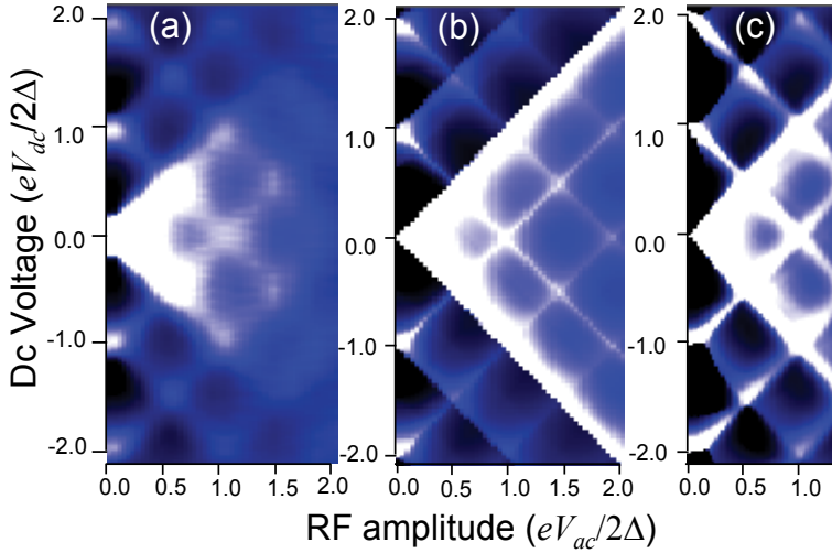
Fig. 5. The intensity plots of the dynamical conductance as a function of dc bias voltage V_{dc} and microwave amplitude V_{ac} of a long array(a) and a short array(c). According to the model described in text, the conductance peaks evolve into a “mesh” structure with the same period in V_{dc} and in V_{ac} of 2\Delta/e . Adopted from(Liou, Kuo et al. 2008)
