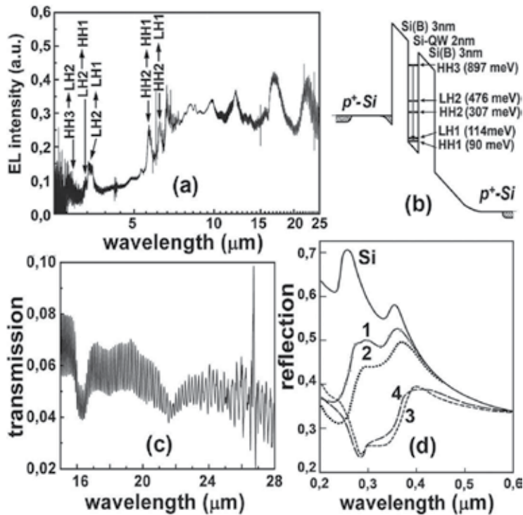
Fig. 3. Electroluminescence spectrum (a) that defines the energies of two-dimensional subbands of heavy and light holes in the p-type Si-QW confined by the \delta - barriers heavily doped with boron on the n-type Si (100) surface (b). T=300\text{K} . (c) Transmission spectrum that reveals both the local phonon mode, \lambda = 16.4 \mu\text{m} , and the superconductor gap, \lambda = 26.9 \mu\text{m} , manifestation. (d) The reflection spectra from the n - type Si (100) surface and from the ultra-shallow boron diffusion profiles prepared on the n - type Si (100) surface that consist of the \delta - barriers confining the ultra-narrow Si-QW. The curves 1-4 are related to the \delta - barriers with different concentration of boron. The values of the concentration boron in different samples are characterized by the following ratio: curve 1 - 0.2, 2 - 0.3, 3 - 0.35, 4 - 0.4. The concentration of boron in the sample characterized by the fourth curve is equal to 5 \cdot 10^{21} \text{ cm}^{-3} . T=300\text{K} .
