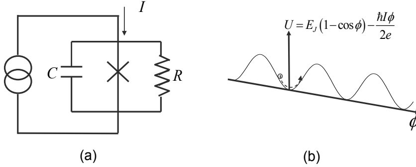
Fig. 1. (a) The model circuit of the resistively( R ) and capacitively( C ) shunted junction. (b) The phase dynamics in a junction under a dc current bias can be modeled with a particle of a mass C moving in a tilted washboard potential.
