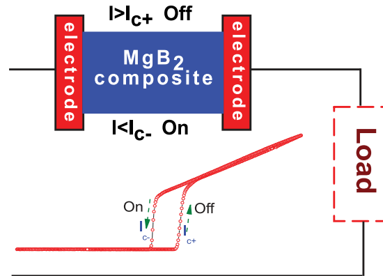
Fig. 13. Diagram for realizing the resistive type SFCL by the superconducting MgB 2 -MgO composite.
