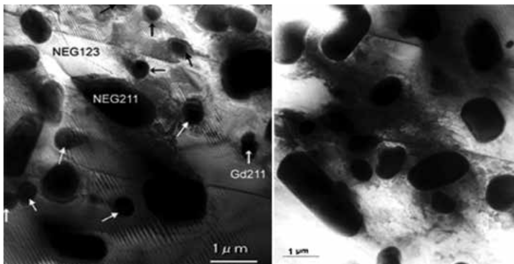
Fig. 2. Transmission electron micrograph of NEG123 with 30 mol% NEG-211 and 0.5 mol% Pt. Note the fine 211 inclusions dispersed in the matrix, which mainly comprise Gd in the rare earth site.
