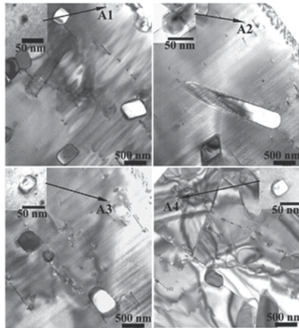
Fig. 5. Transmission electron micrographs of (\text{Nd,Eu,Gd})\text{Ba}_2\text{Cu}_3\text{O}_y samples with 30 mol% Gd-211 (average particle size was 70 nm); Insets show the new Zr-rich pinning medium in a higher magnification.
