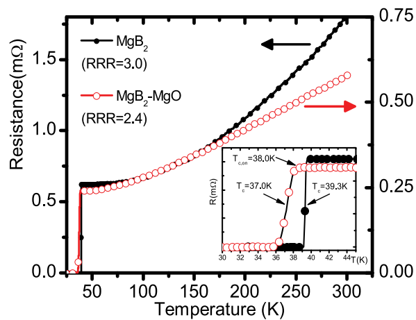
Fig. 7. (Zhang et al., 2010) Resistance vs temperature (R-T) curves of superconducting MgB 2 -MgO composite and pure MgB 2 bulk. The inset shows their R-T curves in the vicinity of N-S transition.
