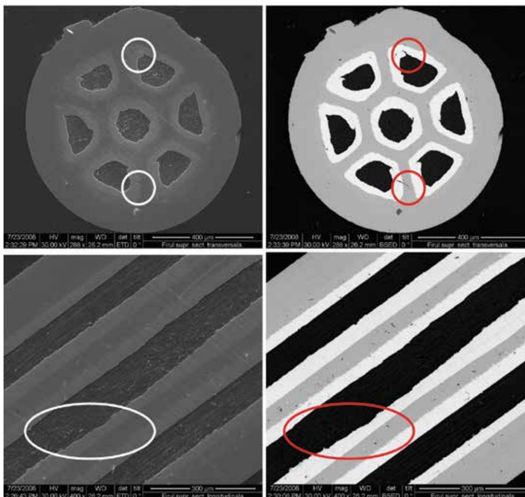
Fig. 7. SEM images of the polished Hypertech MgB 2 wires (7 sub elements): upper panels - transversal SE and BSE modes; bottom panels - longitudinal SE and BSE modes. Defects are identified by the circles. The outer diameter of the wire is 0.83 mm.
