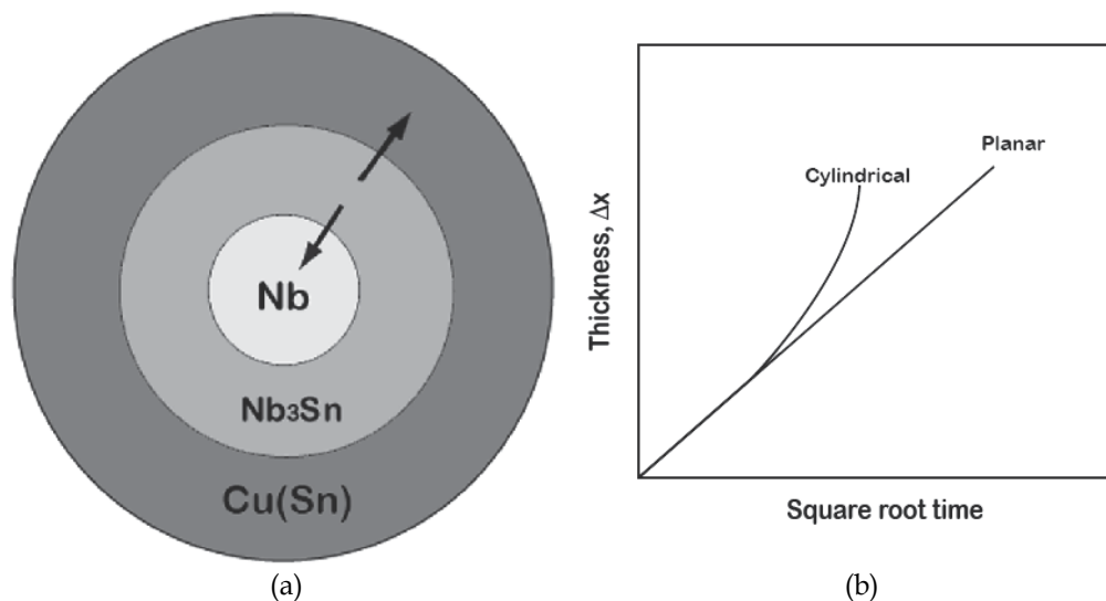
Fig. 7. (a) The growth of Nb 3 Sn product phase in the sample with cylindrical geometry is shown. Arrows indicate the movement of the interfaces following which interfacial area changes. (b) The change in layer with square root of time in the case of sample with planar and cylindrical geometry is shown. Growth rate with planar interface will follow parabolic law in the case of diffusion controlled process; however, it will deviate in the case of growth in a sample with cylindrical geometry (van Loo, 1990).
