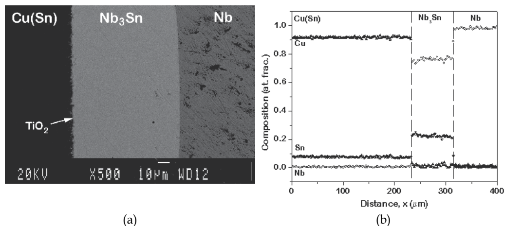
Fig. 8. (a) The growth of the Nb 3 Sn phase and (b) corresponding composition profile are shown in a diffusion couple of Cu(8at.%Sn)/Nb at 775 °C annealed for 330 h (Kumar & Paul, 2009).
