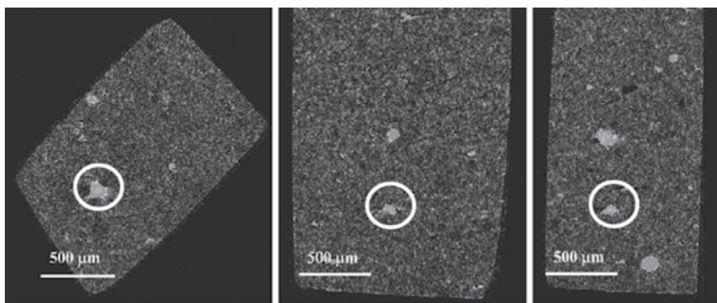
Fig. 9. Transversal, sagittal and longitudinal cross-sections revealing high density regions; high density region size (inside circles) is of about 160 μm.
