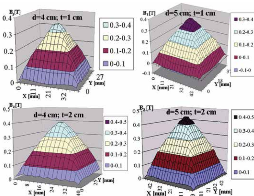
Fig. 18. The calculated trapped field distribution in the sample NEG-123 + 30 mol% Gd-211 (70 nm in size), melt processed in Ar-1% O 2 at liquid oxygen temperature (90.2 K). Dimensions and thicknesses of the sample were assumed 40&50 mm and 10&20 mm, respectively. The high trapped field of 0.45 T was achieved in the remnant state at 90.2 K.
