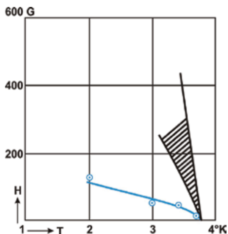
Fig. 11. Temperature dependence of the incipient penetration of magnetic field into the superconducting alloy Pb+64.8wt%Tl. The hatched region denotes the region of gradual flux penetration in magnetic field according to the electrical resistance measurement data (After De Haas & Casimir-Jonker, 1935a).
