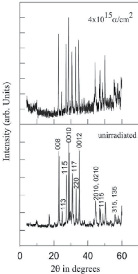
Fig. 1. XRD pattern of unirradiated and 4 \times 10^{15} \alpha/\text{cm}^2 polycrystalline of Bi-2212.
