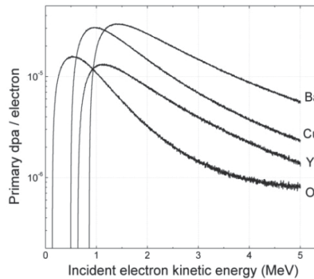
Fig. 4. Monte Carlo simulation of ES processes inducing Primary Knock-On Atomic Displacements in \text{YBa}_2\text{Cu}_3\text{O}_{7.5} depending on electron initial energy at a given discrete event.
