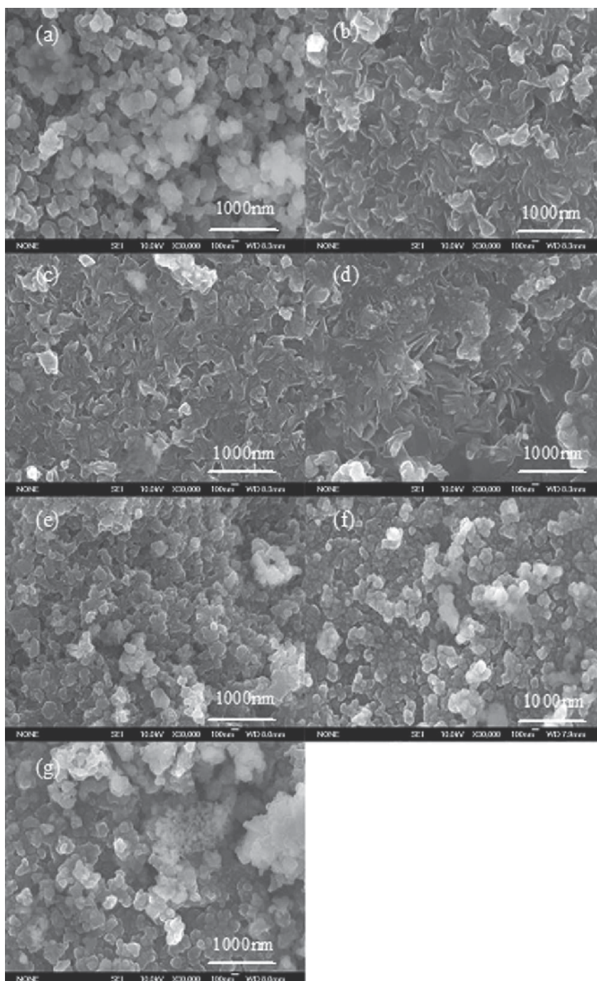
Fig. 11. SEM images of \text{MgB}_2 (a), \text{Mg}_{1.15}\text{B}_2 (b), \text{MgB}_2 +10 wt % SiC (c), \text{Mg}_{1.15}\text{B}_2 +10 wt % SiC (d), \text{Mg}_{1.20}\text{B}_2 +10 wt % SiC (e), \text{Mg}_{1.25}\text{B}_2 +10 wt % SiC (f), and \text{Mg}_{1.30}\text{B}_2 +10 wt % SiC (g) (Li et al., 2009a)
