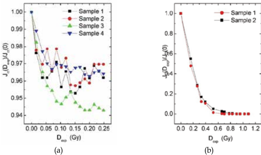
Fig. 16. Dependence of the superconducting critical current dependence on the ^{57}\text{Co} gamma ray exposition doses at different target temperatures: (a) 80 K, (b) 300 K.
