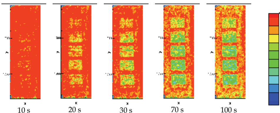
Fig. 22. 2D correlation maps of the as-grown sample with different machined regions at different instants. The reference corresponds to the sample surface at t=1800 s.
