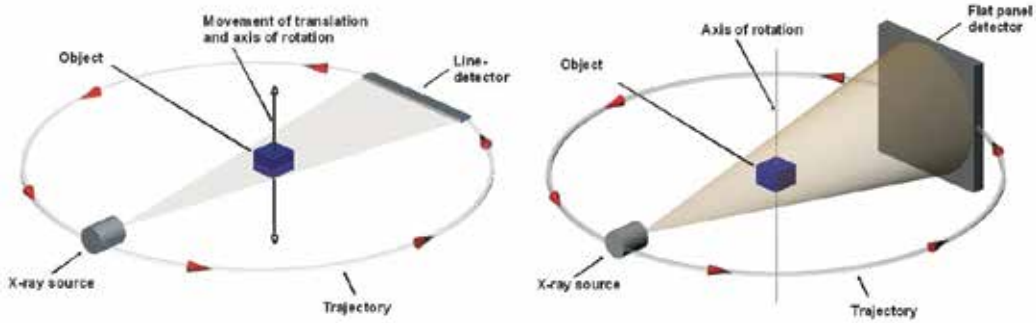
Fig. 1. Fan beam (left) versus cone beam (right) tomography configurations.
