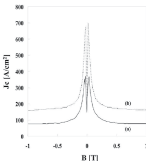
Fig. 6. Dependence of current density on magnetic flux density. The samples were prepared from the slurry with various PVA concentrations: (a) 0 and (b) 1 wt%. Measurement was performed at 77 K.
