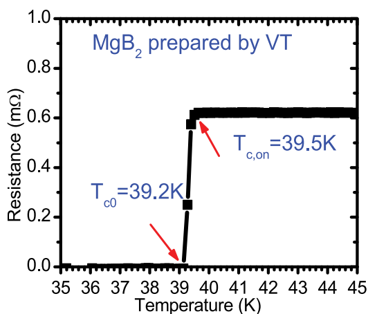
Fig. 4. The temperature dependence of resistance of superconducting \text{MgB}_2 sample synthesized by the vacuum technique in the vicinity of transition temperature.
