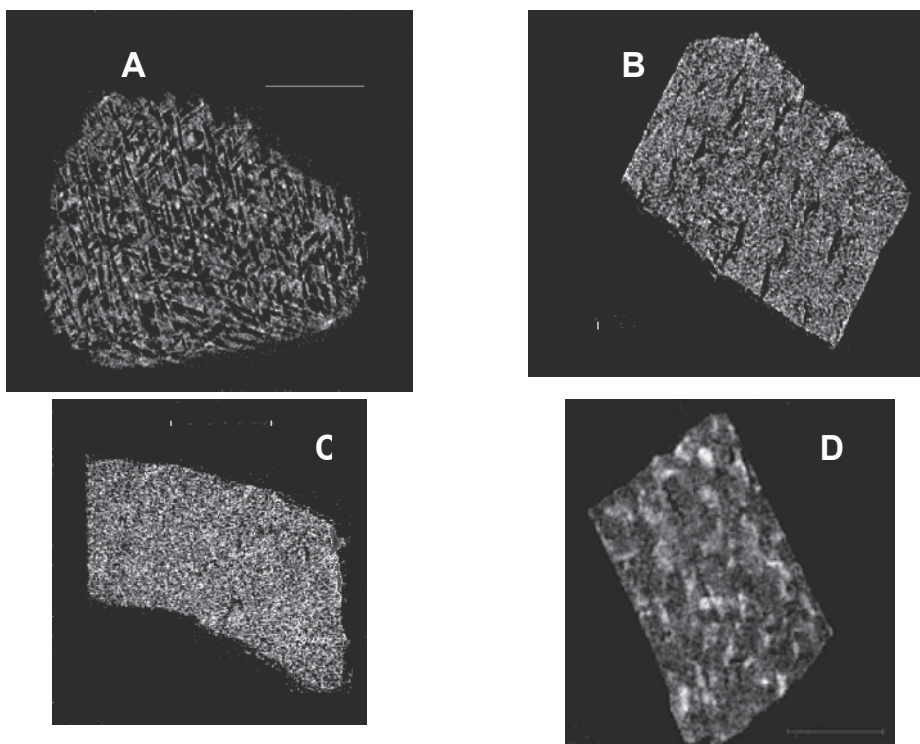
Fig. 5. Representative XRT images of the heat treated bulk samples A-D (Table 1). Images were taken for a voltage of 40 kV and a current of 100 \mu A. Scale bar is 100 \mu m.
