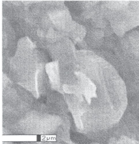
Fig. 11. The optimally oxygen doped uncut (virgin) Hg-1223 sample. The SEM output has been taken at 20 kV, ESD X350. ( T_c=136 K, t=1.5 μm) (Onbaşlı et al, 1998).
