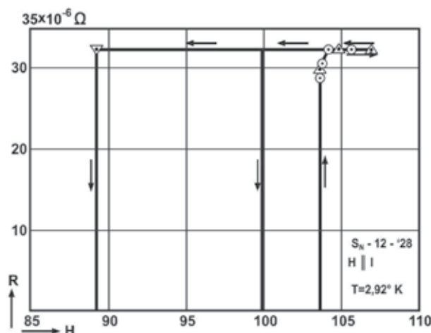
Fig. 3. Sudden change of electrical resistance of wire sample of single crystal tin at T < T_c , as caused by longitudinal magnetic field (After De Haas & Voogd, 1931a).
