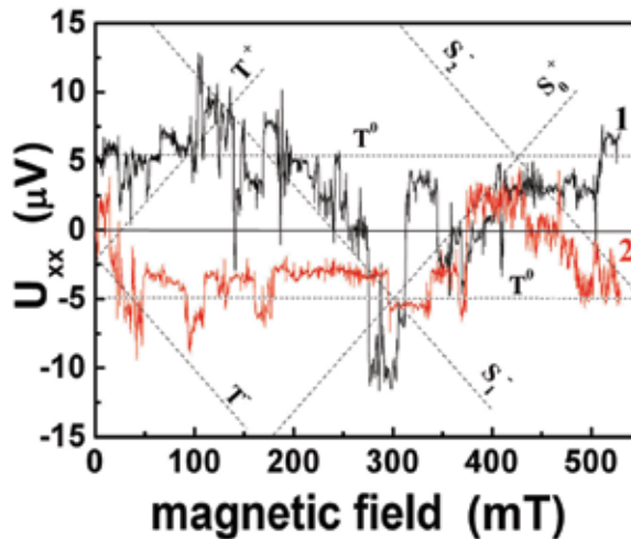
Fig. 13. U_{xx} vs the value of the magnetic field applied perpendicularly to the plane of the p-type Si-QW confined by the \delta -barriers on the n-type Si (100) surface. I_{ds}=10 nA. T=77 K. Curves 1 and 2 measured for opposite orientations of a magnetic field reveal the sign of U_{xx} that corresponds to the diamagnetic response of the superconductor \delta -barriers.
