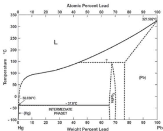
Fig. 8. Binary phase diagrams of the alloy Hg-Pb (After Massalski, 1987).
