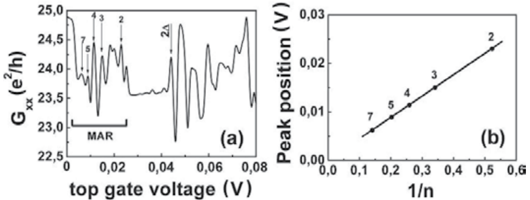
Fig. 20. (a) Multiple Andreev reflections (MAR) that are observed in the longitudinal conductance of the sandwich structure, \delta -barrier - p-type Si-QW - \delta -barrier, on the n-type Si (100) surface by varying the top gate voltage applied within frameworks of the Hall geometry (see Fig. 8a). I_{ds}=10 nA. T=77 K. The MAR peak positions are marked at V_n = 2\Delta/ne with values n indicated. (b) Plot of the MAR peak position versus the inverse index 1/n .
