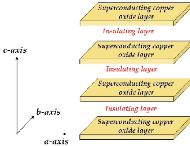
Fig. 2. The schematic representation of the intrinsic Josephson structure in the layered high temperature superconductors.
