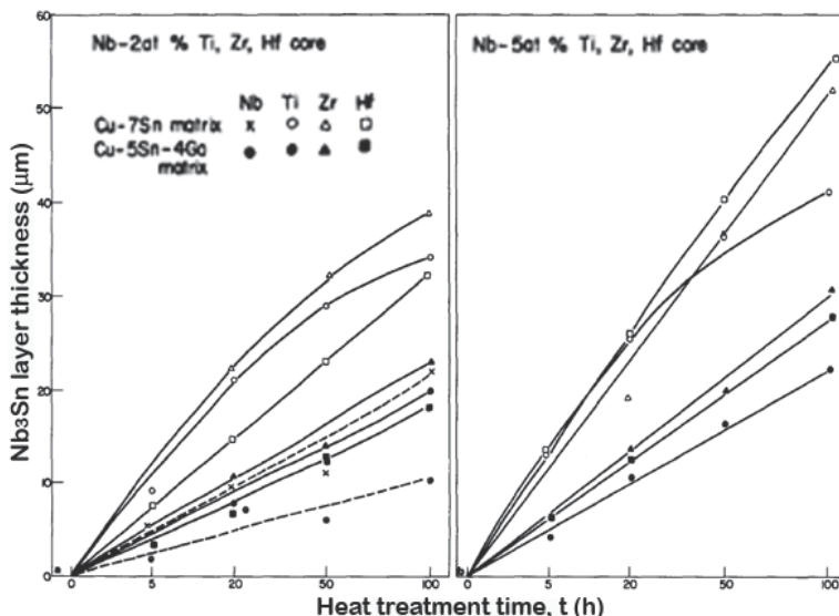
Fig. 18. The increase in layer thickness with the increase in annealing time at 800 °C is shown. (a) Nb-2at.%Ti, Zr and Hf core (b) Nb-5at.%Ti, Zr and Hf core (Takeuchi et al., 1981).
