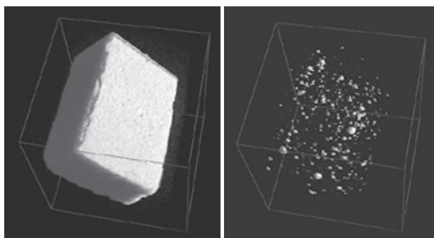
Fig. 10. 3-D reconstruction (left) and the distribution of the high density regions inside the volume of the sample of about 0.8 mm 3 .
