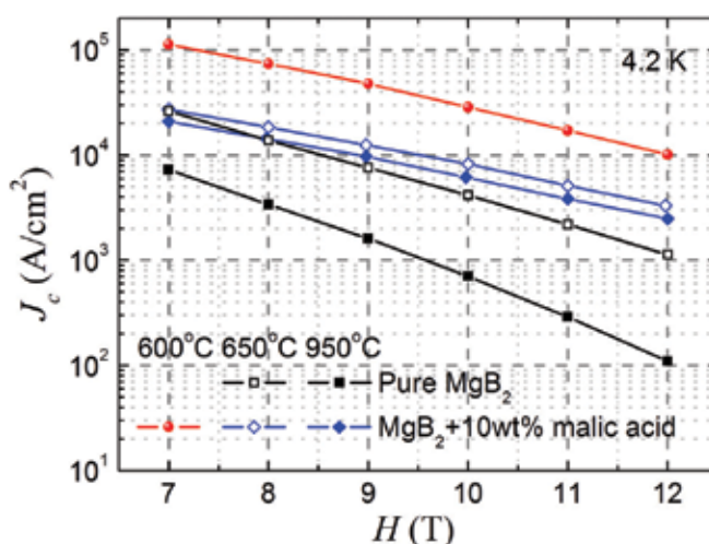
Fig. 14. Sintering temperature effects on the J_c performance of MgB 2 doped with malic acid (Kim et al., 2008)
