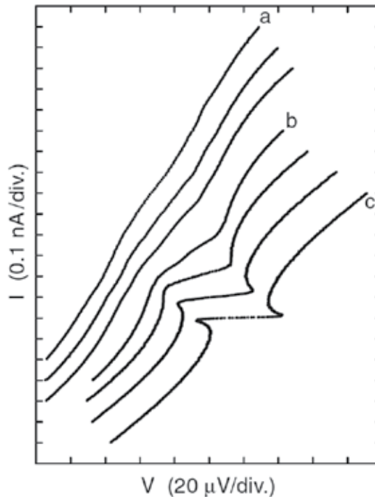
Fig. 8. The IV curves of the single junction in tunable environment of different impedances. From top left to bottom right, the environment impedance increases. Origin of each curve is offset for clarity. Adopted from (Watanabe & Haviland 2001)
