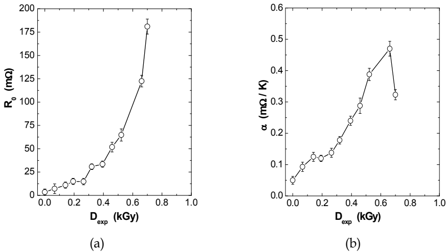
Fig. 17. Exposition dose dependence of (a) residual resistivity R_0 in ( \text{m}\Omega ) and (b) thermal electrical resistivity coefficient \alpha ( \text{m}\Omega\text{K}^{-1} ) of ^{57}\text{Co} irradiated YBCO ceramic samples at room temperature.
