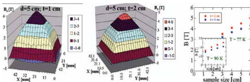
Fig. 19. The calculated trapped field distribution in the sample NEG-123 + 30 mol% Gd-211 (70 nm in size), melt processed in Ar-1% O 2 , calculated for the liquid nitrogen temperature. Dimensions and thicknesses of the sample were assumed 50 mm and 10&20 mm, respectively. Trapped field as high as 4.5 T was achieved in the remnant state at 77.3 K. The summary for the sample size vs trapped field at 77 K and 90 K in the remnant state is in the right figure.
