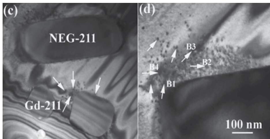
Fig. 16. Transmission electron micrograph of NEG-123 sample with 35 mol% Gd-211 (the initial average particle size 70 nm) and 0.1 mol% \text{Nb}_2\text{O}_5 the arrows point to some of the smallest, Nb-based, nanoparticles.
