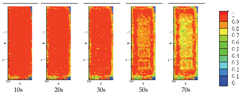
Fig. 23. 2D correlation maps of the annealed sample with different machined regions at different instants. The reference is the sample surface at t=0s .
