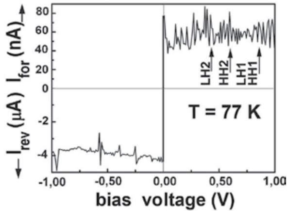
Fig. 14. I - V characteristic that demonstrates the modulation of the critical current with the forward and reverse bias applied to the p-type Si-QW confined by the \delta -barriers on the n-type Si (100) surface.
