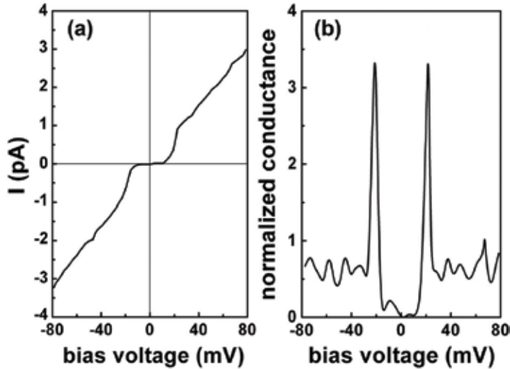
Fig. 12. The I - U (a) and dI/dV(V) (b) characteristics found by the current-voltage measurements (a) and using the STM point contact technique (b), which identify the superconductor energy gap in the nanostructured \delta -barriers heavily doped with boron that confine the p-type Si-QW on the n-type Si (100) surface. (a) - 77 K; (b) - 4.2 K.
