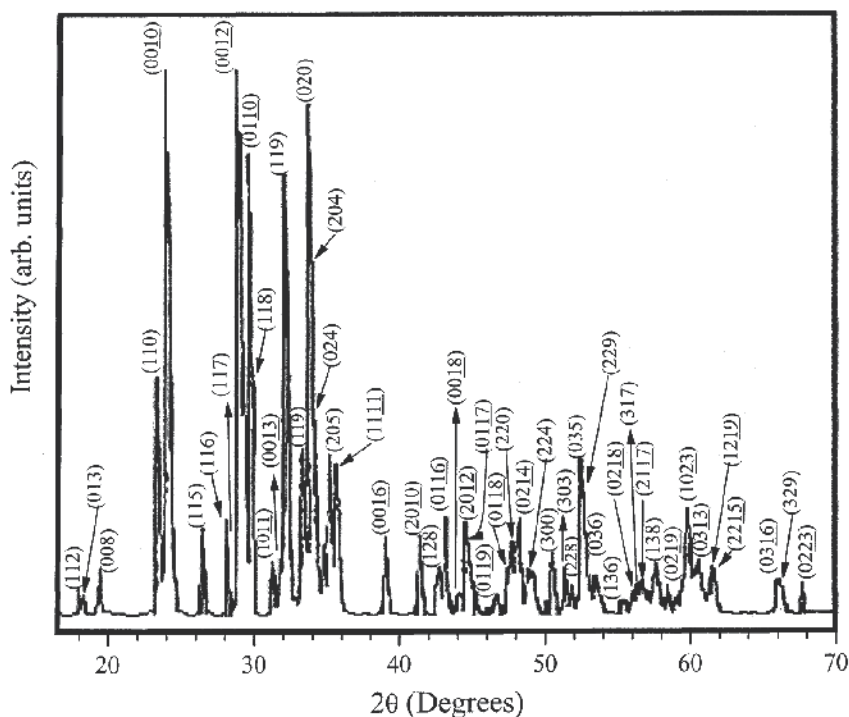
Fig. 5. Indexed x-ray diffraction pattern of the sample after the final sintering at room temperature
