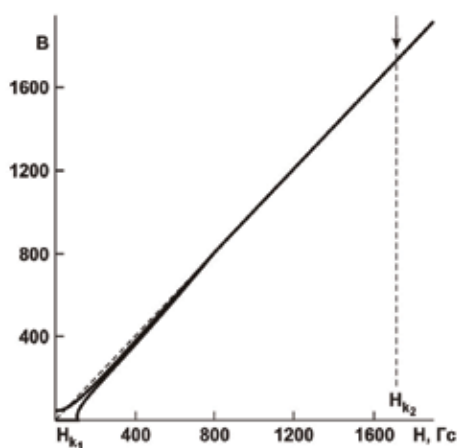
Fig. 13. B-H curve of long cylindrical sample of single crystal Pb+66,7at.%Tl in longitudinal field (Rjabinin & Shubnikow, 1935b).
