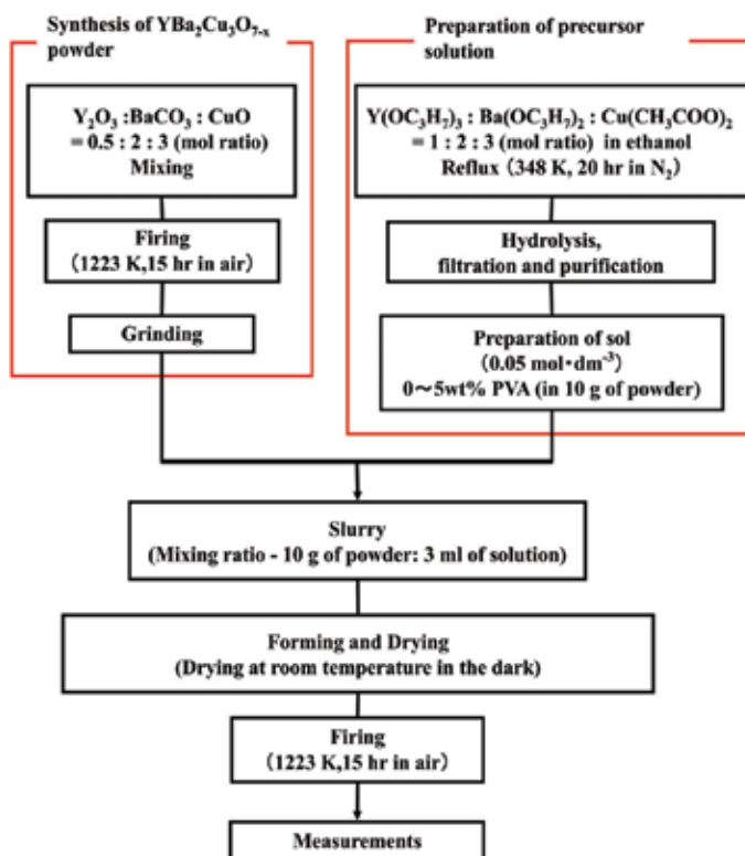
Fig. 1. Preparation procedure for \text{YBa}_2\text{Cu}_3\text{O}_{7-x} slurry and bulk sample.
