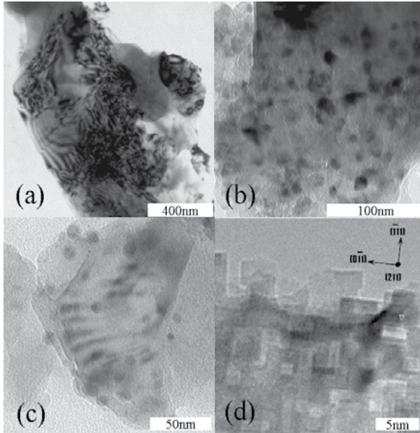
Fig. 10. TEM images of SiC-doped MgB 2 showing the high density of dislocations (a), inclusions larger than 10 nm (b), inclusions smaller than 10 nm (c), and HRTEM image of the nanodomain structure (d) (Dou et al., 2003a; Li et al., 2003)
