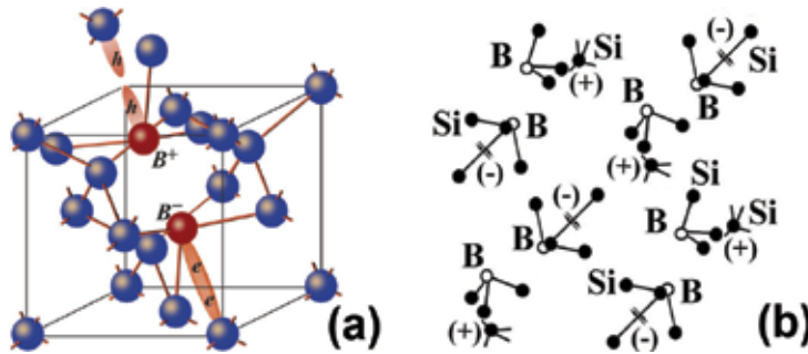
Fig. 7. (a) Model for the elastic reconstruction of a shallow boron acceptor which is accompanied by the formation of the trigonal dipole ( B^+ - B^- ) centers as a result of the negative-U reaction: 2B^0 \rightarrow B^+ + B^- . (b) A series of the dipole negative-U centers of boron located between the undoped microdefects that seem to be a basis of nanostructured \delta -barriers confining the Si-QW.
