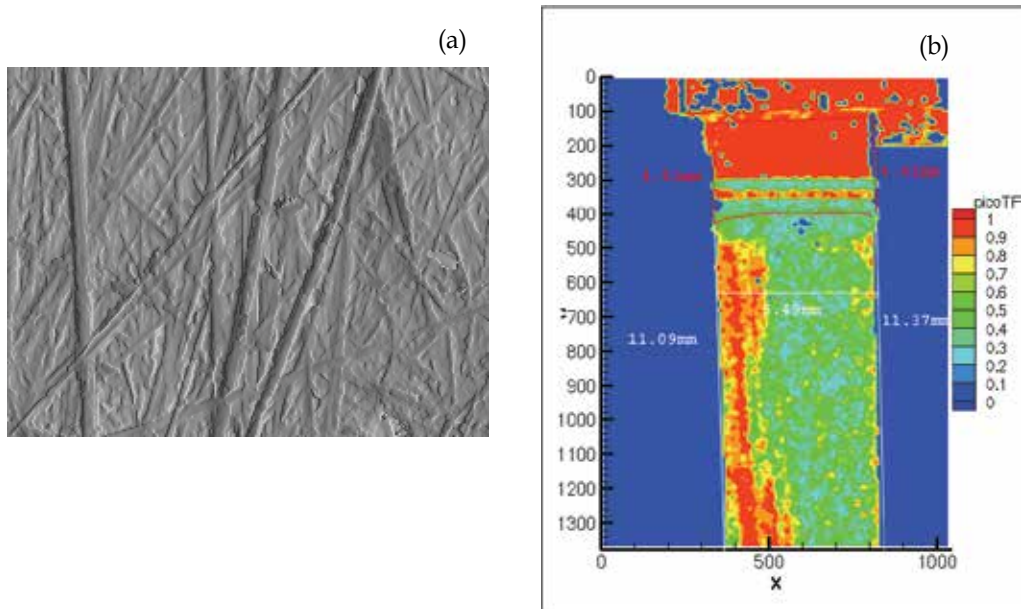
Fig. 14. (a) Confocal image of the Fe surface ( 255 \times 190 \mu\text{m}^2 ) before starting the deposition process. (b) 2D correlation map obtained in a Fe sample after being immersed in a 0.1 M \text{Cu}(\text{NO}_3)_2 solution for 1 h.
