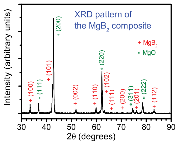
Fig. 5. X-ray diffraction pattern of superconducting MgB 2 -MgO composite. Only diffraction peaks of MgB 2 and MgO phases were detected. The mass ratio of MgB 2 to MgO in the sample was calculated to 1:2.6.
