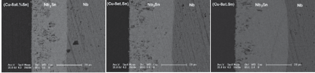
Fig. 11. Different layer thickness in the same diffusion couple annealed at 775 °C for 150 hrs at different locations is shown (Kumar and Paul, 2009).
