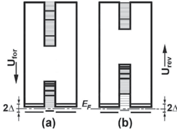
Fig. 15. The one-electron band scheme of the p-type Si-QW confined by the \delta -barriers on the n-type Si (100) surface under forward (a) and reverse (b) bias, which depicts the superconducting gap, 2\Delta , as well as the two-dimensional subbands of holes and the levels that result from the hole interference between the \delta -barriers (a) and the Coulomb charging effects in the Si-QW filled with holes (b).
