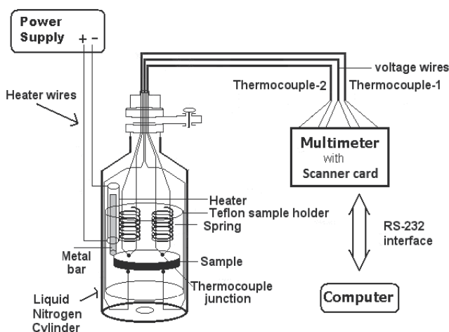
Fig. 2. Block diagram of the apparatus developed for thermoelectric power measurements. Scanner card is used with the multimeter for simultaneous measurements at different points as shown. RS-232 is the standard serial interface of the computer
