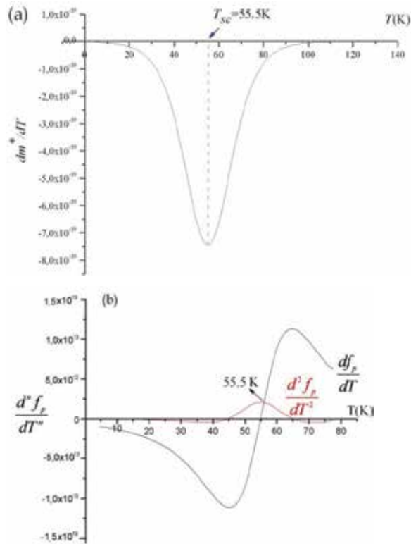
Fig. 11. (a)- The first derivative of the net effective mass with respect to temperature (time). (b)- The plasma frequency shifts from microwave to infrared at the T_{SC} . (Özdemir et al., 2006).
