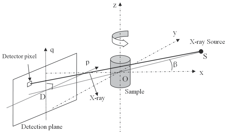
Fig. 2. Feldkamp algorithm cone-beam geometry
