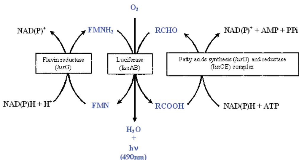
Fig. 1. Bioluminescence reaction (adapted from Sung & Lee, 2004 and Tu & Mager, 1995)
