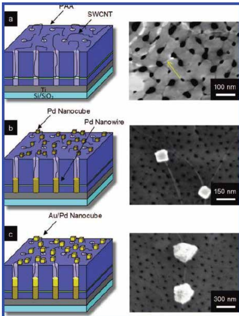
Fig. 4. Tilted cross-sectional schematics with corresponding SEM images portraying sequential fabrication process steps: (a) SWCNTs grown from the pores of the PAA via MPCVD, (b) electrodeposition of Pd to form Pd nanowires in pores and Pd nanocubes on SWCNTs and (c) electrodeposition to coat the existing Pd nanocubes with a thin layer of Au (Claussen et al., 2009).
