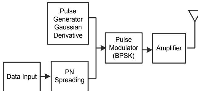
Fig. 3. UWB transmitter block diagram
