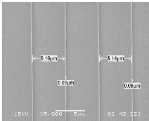
Fig. 12. The SEM image of the silicon nanowires.
