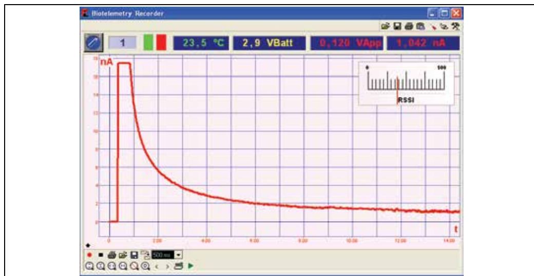
Fig. 7. Simple graphic user interface of the data-acquisition software running on the PC.
