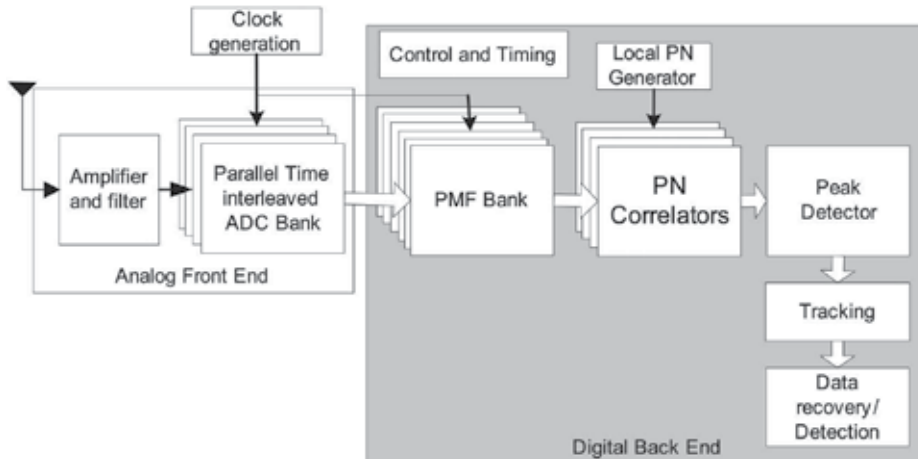
Fig. 4. UWB receiver block diagram
