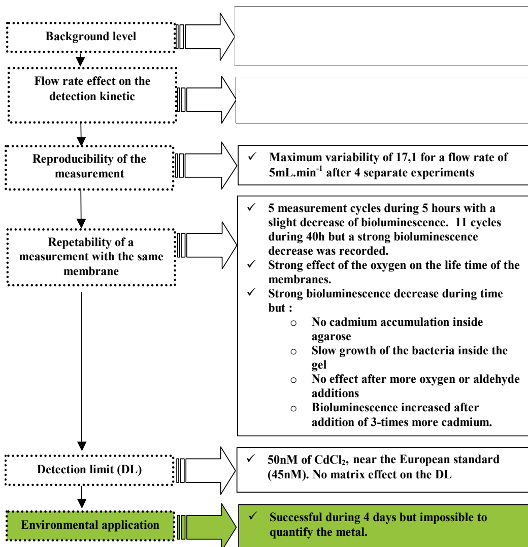
Fig. 16. Summary of the main results obtained in this study with the E.coli DH1 pBzntlux immobilized in the Lumisens 2 biosensor.
