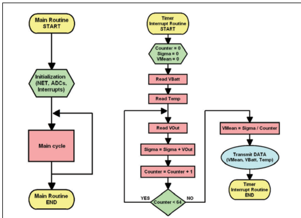
Fig. 5. Firmware running on the implantable biotelemetric device.
