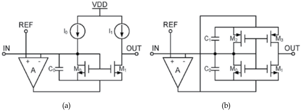
Fig. 4. Conventional current-mode amplifier topologies.
