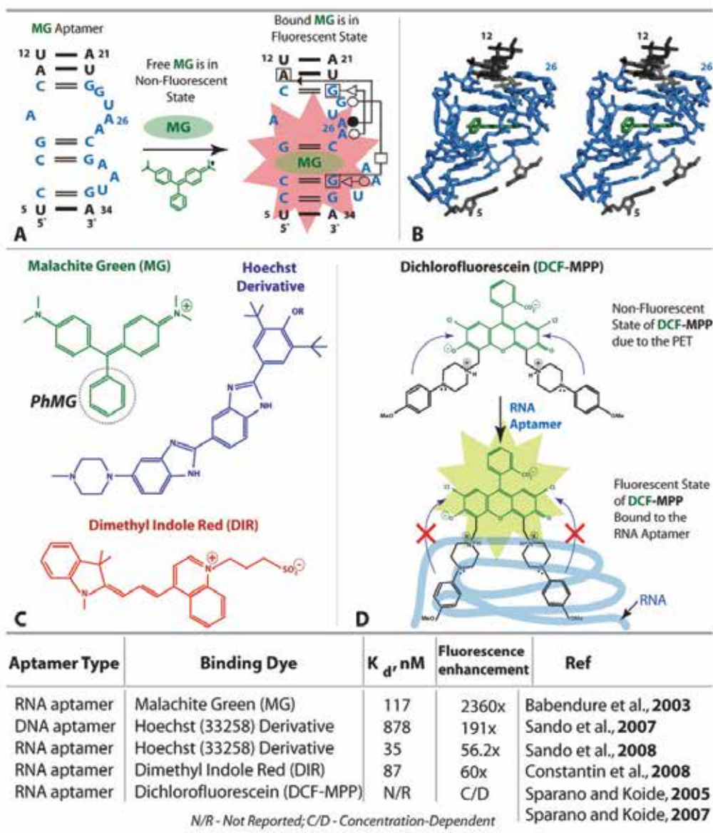
Fig. 2. Light-up dye/apptamer pairs and their properties. A. Malachite Green (MG) aptamer 3D structure with basepairs annotated with Leontis-Westhof nomenclature. Watson-Crick Edges are shown in circles, Hoogsteen Edges in squares, and the Sugar Edges in triangles (Leontis & Westhof, 2001). Hollow symbols indicate trans basepairs and filled symbols, cis basepairs. Boxes indicate nucleotides pairing with more than one base. B. 3D stereo view of the X-ray structure of the MG aptamer binding to tetramethylrosamine (PDB file: 1f1t). Nucleotides are colored to match the annotated 3D structure. C. Several examples of fluorogenic dyes for which nucleic acid aptamers have been obtained to create “light-up” pairs. In case of MG, phenyl ring (PhMG) mentioned in text is circled. D. Schematic
