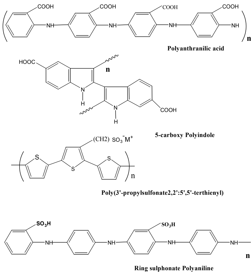
Fig. 2. Electronic structure of self doped conducting polymers
