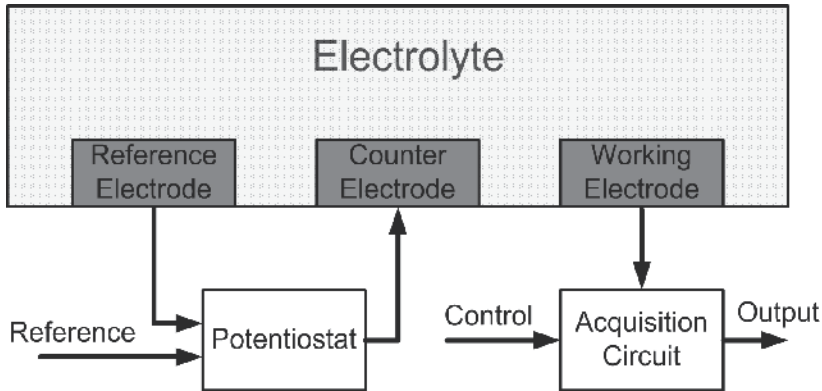
Fig. 2. Interfacing circuits in the CMOS IBS.
