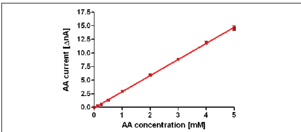
Fig. 11. Ascorbic acid microsensor in-vitro calibration.
