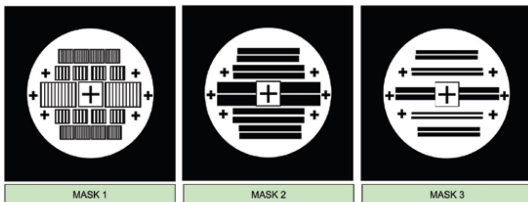
Fig. 4. Mask design for Nanowire fabrication
