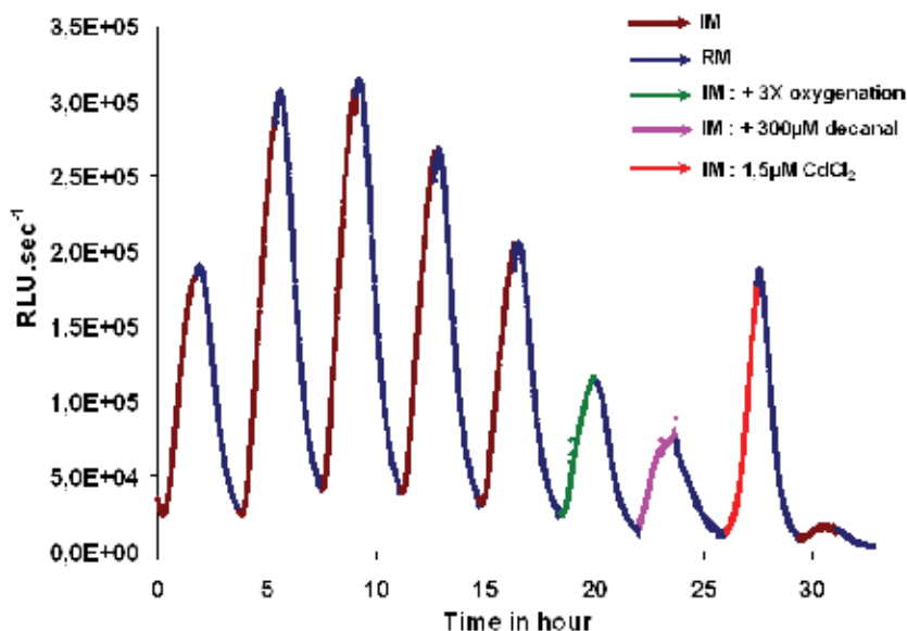
Fig. 13. Parameters influencing the repeatability of the cadmium detection by Lumisens2 biosensor using E.coli DH1 pBzntlux. IM: Induction Medium; RM: Regeneration Medium. Experimental conditions were as described in Fig 7 with constant oxygenation of the feeding media.
