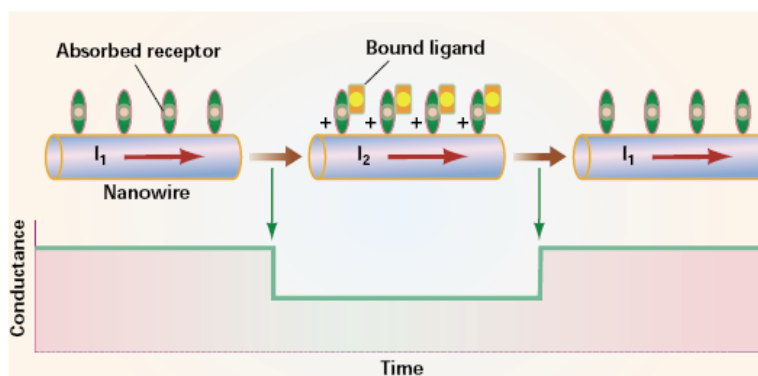
Fig. 2. Operation principle of nanowire filled with DNA [7].
