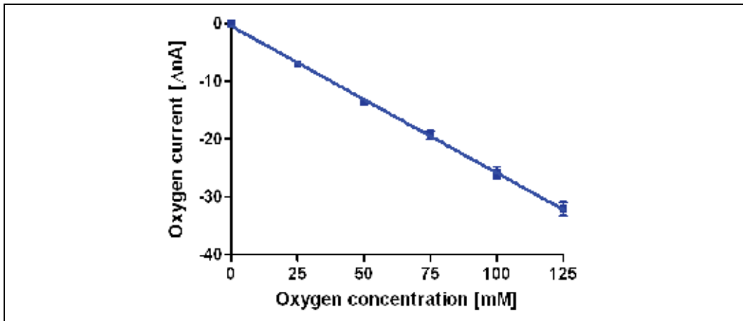
Fig. 9. Oxygen microsensor in-vitro calibration.
