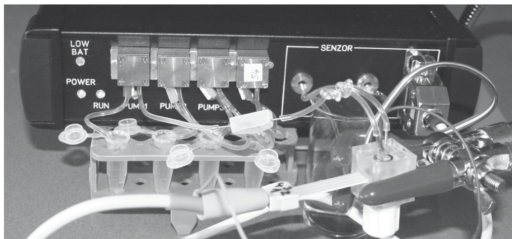
Fig. 5. The amperometric immunosensor detector ImmunoSMART. In the left part of the front panel, four miniature peristaltic pumps are connected to minitubes with bioreagents. The flow-through cell fixed in the holder contains the exchangeable screen-printed immunosensor.
