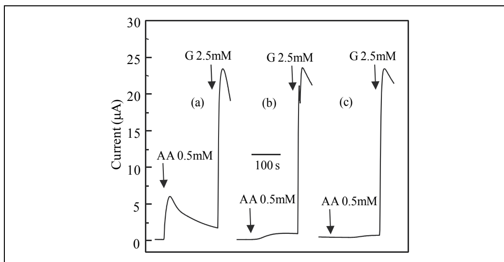
Fig. 10. Amperometric response to 0.5 mM ascorbic acid (AA) and 2.5 mM glucose (G). Acetonitrile plasma polymer coating on the immobilized enzyme: (a) no PP overcoating (GO x /CNT/PP/Au), (b) 10 nm PP overcoat, (10 nm PP/GO x /CNT/PP/Au), and (c) 20 nm PP overcoat (20 nm PP/GO x /CNT/PP/Au). The polarized potential was +0.8 V vs. Ag/AgCl. The electrolyte was a pH 7.4 20 mM phosphate buffer solution.
