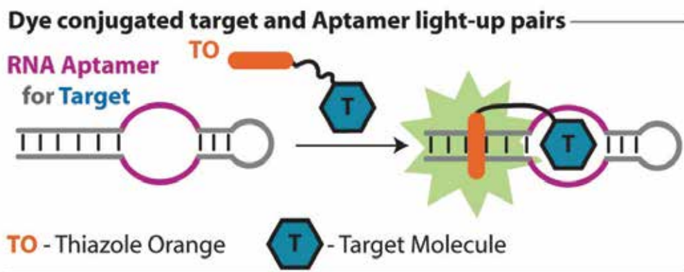
Fig. 3. Stojanovic's strategy for RNA detection. Thiazole Orange (TO), a fluorescent intercalator, is conjugated to a small molecule (blue hexagon). RNA aptamer (pink region) specific for its target binds the small molecule and forces TO binding to double-stranded region at the specific location.
