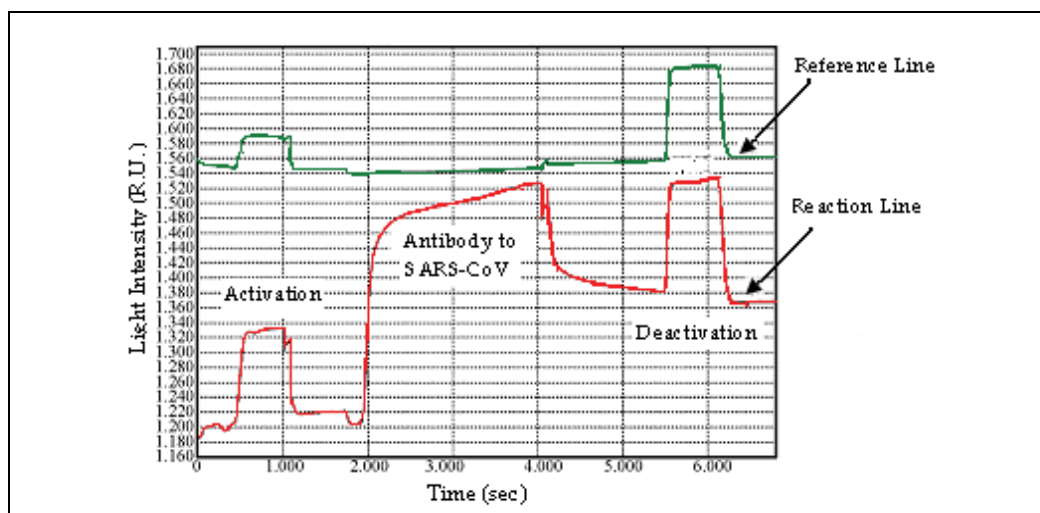
Fig. 4. Signal recording of immobilizing antibodies directly The green line is a reference curve. The red line is a reaction curve.
