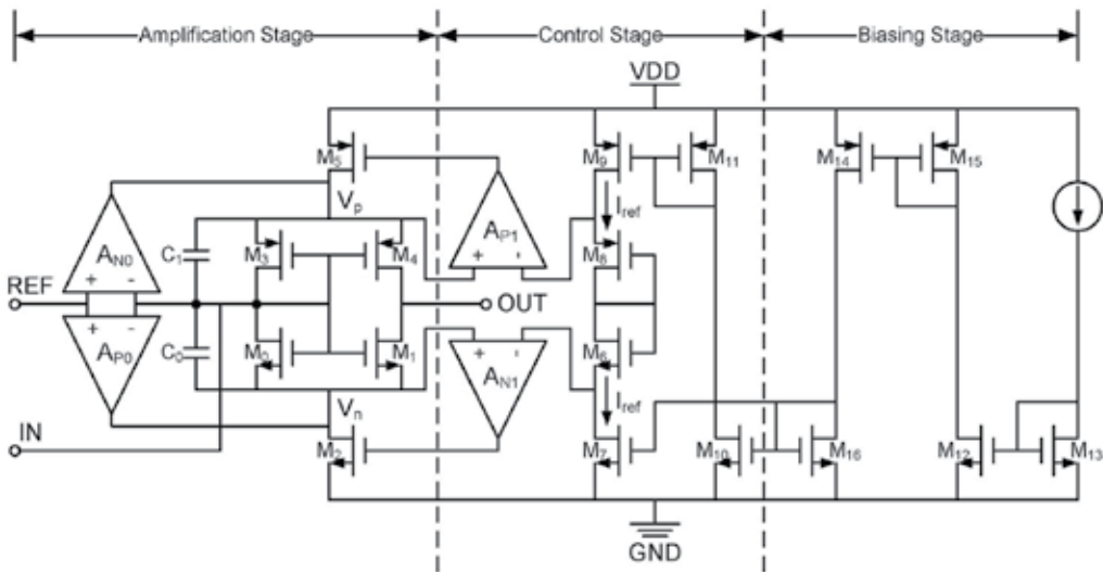
Fig. 5. Circuit schematic of the ULCA.
