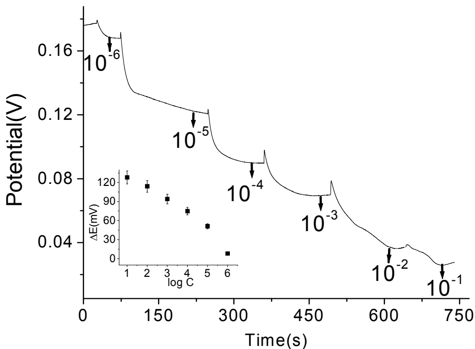
Fig. 6. Potentiometric response of the biosensor (Urease (20 \mu l) /PIIn-PVC/Pt) to increasing urea concentration ( 10^{-6} - 10^{-1} )M. 1 mM Tris-HCl buffer (pH 7.0) calibration curve (Inset)
