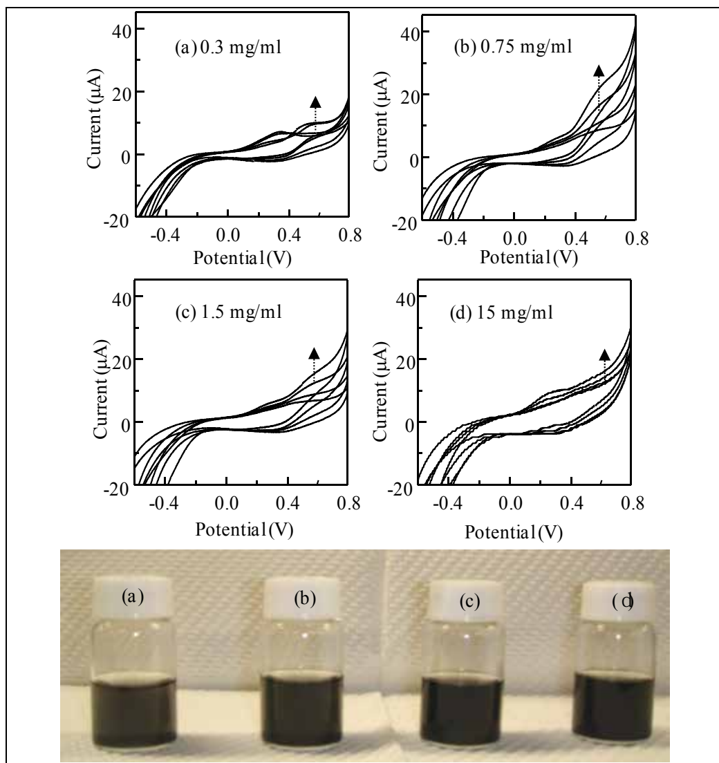
Fig. 6. Cyclic voltammograms of the fabricated amperometric glucose sensor using GO x , CNTs, and PP (PP/GO x /CNT/PP/Au) as a function of the CNT concentration used for casting the CNT layer. CNT concentrations: (a) 0.3, (b) 0.75, (c) 1.5, and (d) 15 mg mL -1 . Arrow directions indicate the glucose concentration increments at 0, 2.5, 14, and 48 mM. Conditions: 20 mM phosphate buffer; pH=7.4; 20 °C; scan rate, 50 mV s -1 ; electrode area (geometric), 25 mm 2 . Photograph: Vials of CNT dispersions after 4 h.
