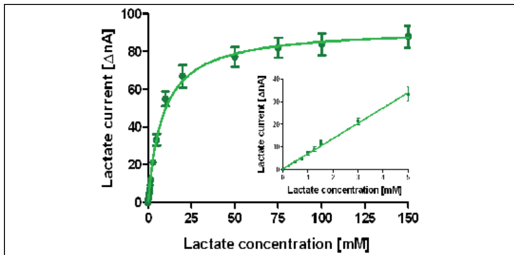
Fig. 15. In-vitro calibration of lactate biosensor (see text).
