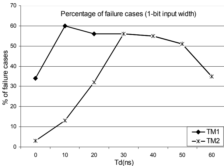
Fig. 8. Percentage failure cases for translation methods (TMs)
