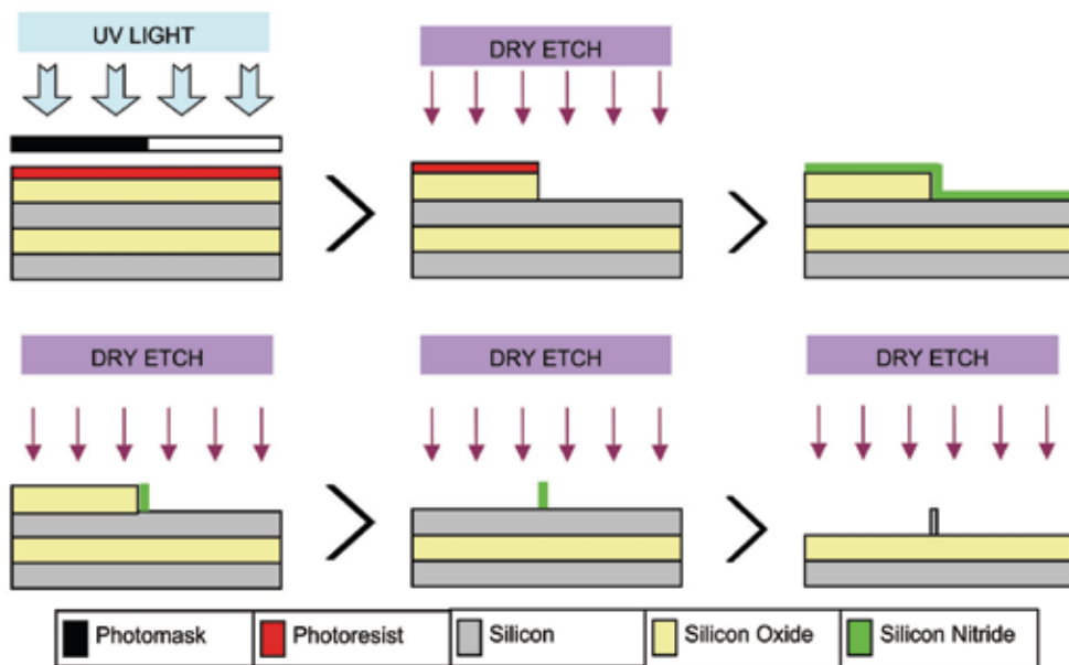
Fig. 5. Layer by layer alignment and patterning method.
