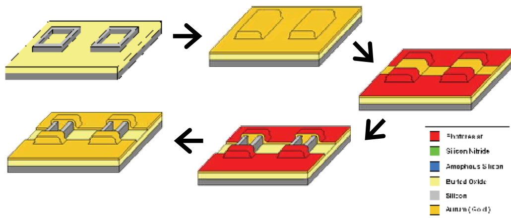
Fig. 6. Process flow of gold pad.
