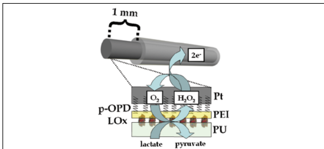
Fig. 14. Schematic representation of the lactate biosensor used in this study.
