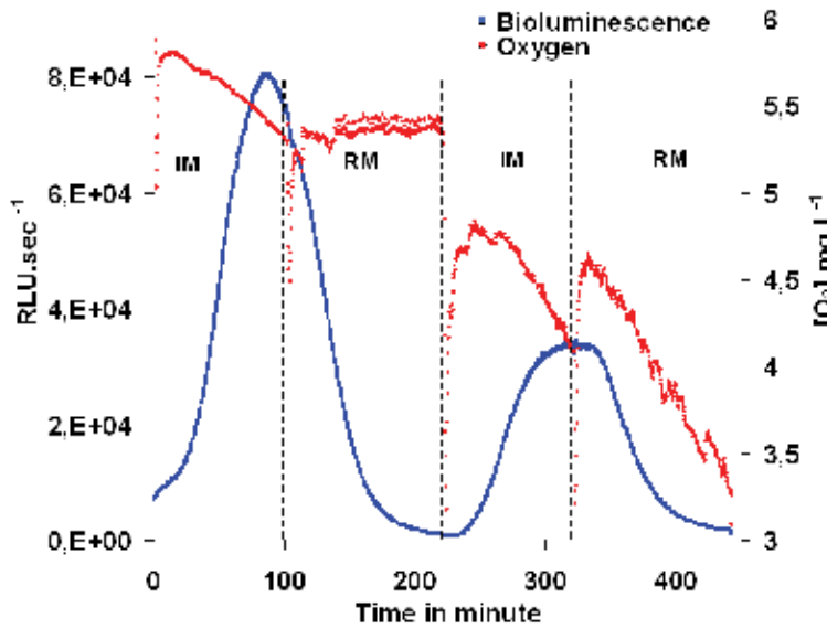
Fig. 10. Evolution of oxygen concentration at the exit of the Lumisens2 biosensor measurement cell.
