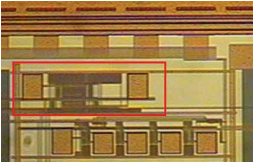
Fig. 8. Die micrograph of the ULCA circuit.
