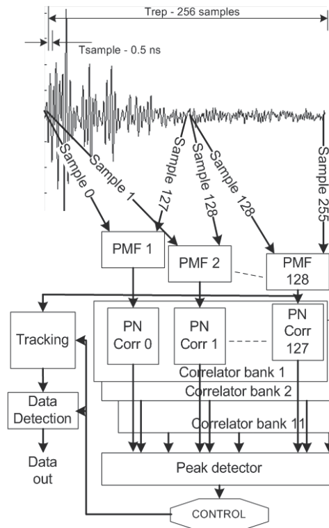
Fig. 5. UWB receiver digital backend (O'Donnell & Brodersen, 2005)
