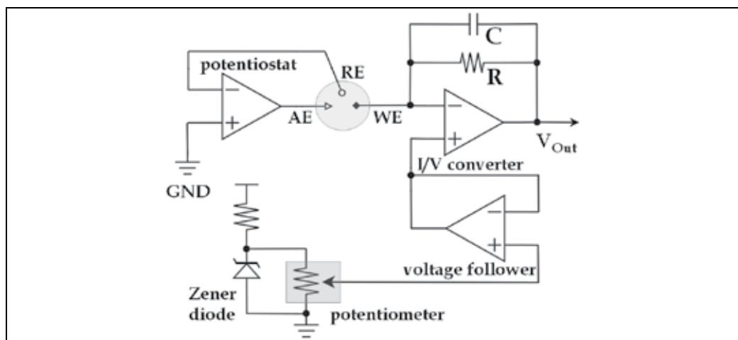
Fig. 3. Schematic of the amperometric module of the biotelemetric device working in "oxidation mode".
