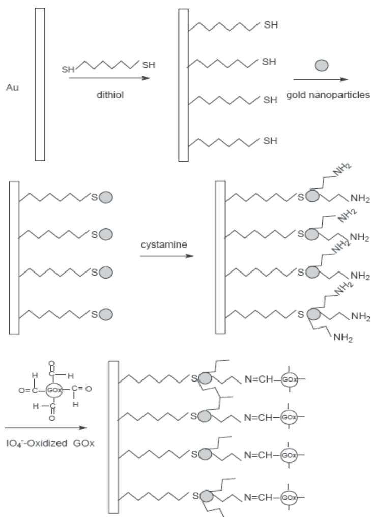
Fig. 2. Stepwise assembly of dithiol, gold, cystamine, IO 4 - oxidized GOD on a gold electrode, from paper (Zhang et al., 2005)
