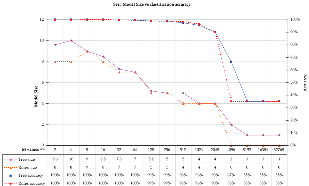
Fig. 14. Symbolic Model size and accuracy variations as measured by 10-fold cross validation for four motion classes (walk, run, golfswing, and golfputt).
