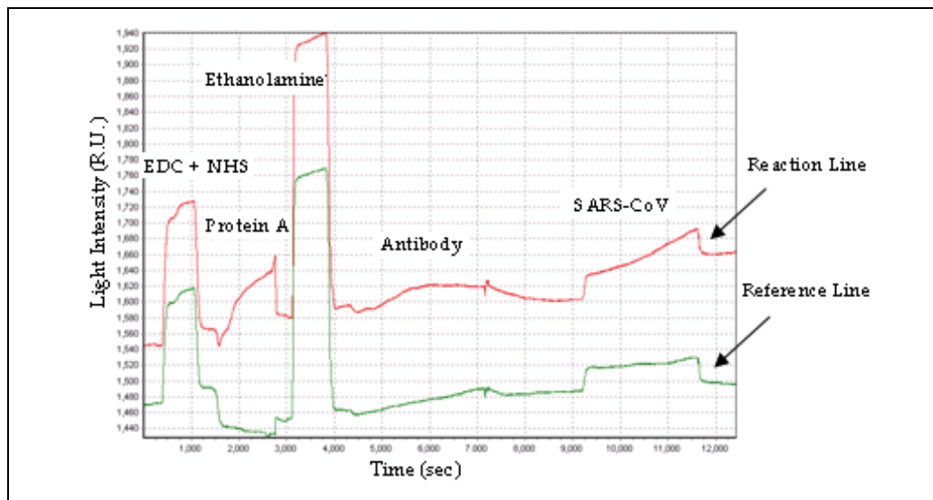
Fig. 6. Detection of sterilized SARS-CoV using Protein A The green line is a reference curve. The red line is a reaction curve.
