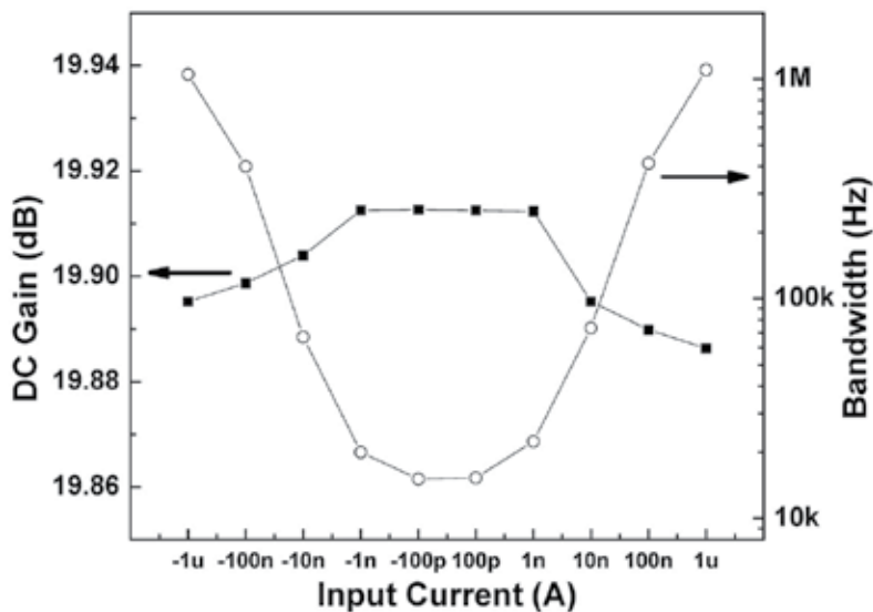
Fig. 9. DC gain and bandwidth as functions of input currents ranging from -1 to 1 \mu\text{A} . The black squares represent the dc gain, whereas the circles illustrate the bandwidth.
