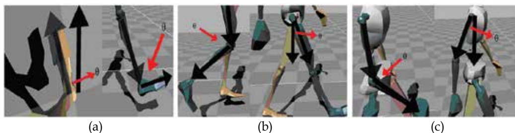
Fig. 4. Selected features annotated of the Moven avatar; (a) Foot Orientation Angle and Foot Angle, (b) Knee Angle and Thigh Angle (c) Elbow Angle and Arm Angle.
