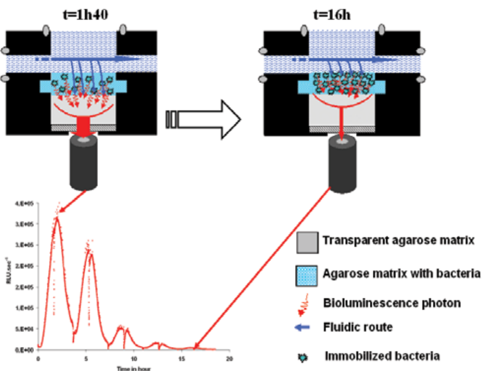
Fig. 17. Possible effects on cadmium detection of the bacterial growth in Lumisens2 Biosensor chip.
