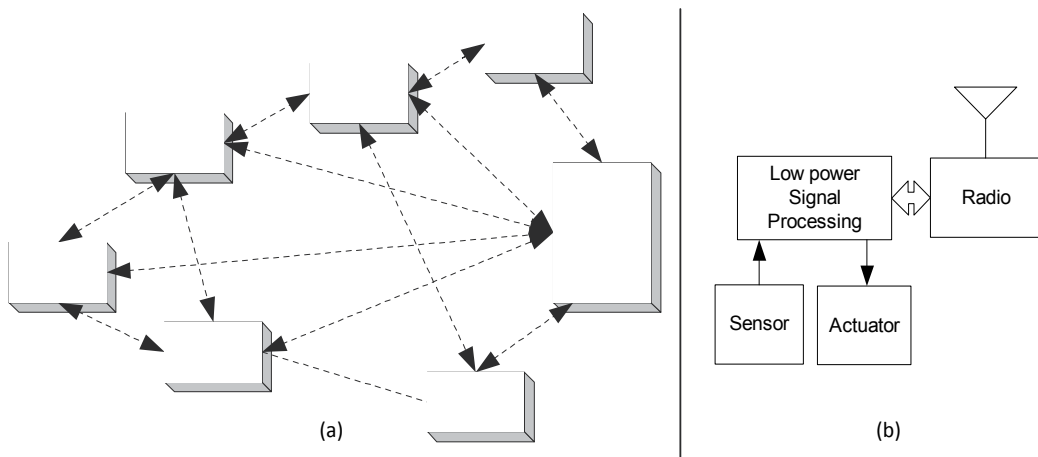
Fig. 1. (a) Typical wireless sensor network scenario (b) Sensor node block diagram
