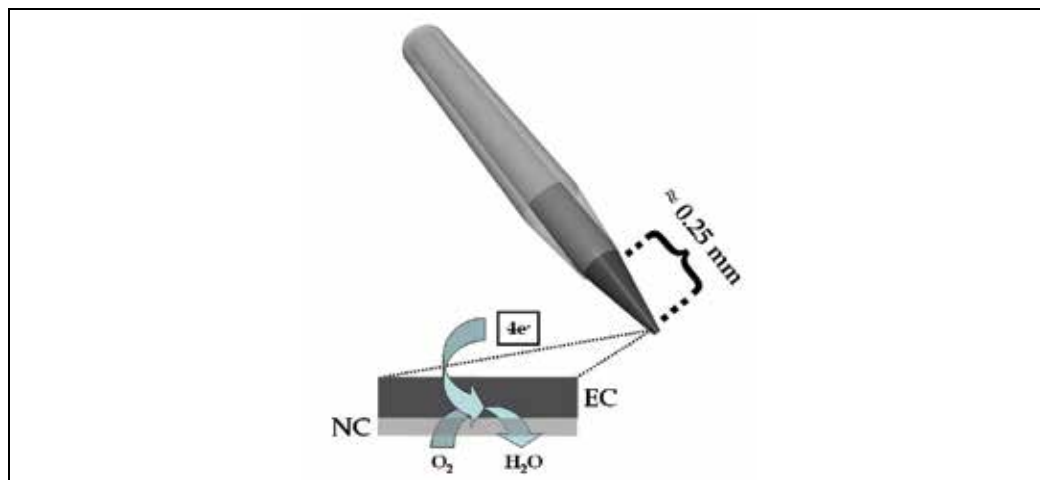
Fig. 8. Schematic representation of the oxygen microsensor used in this study.
