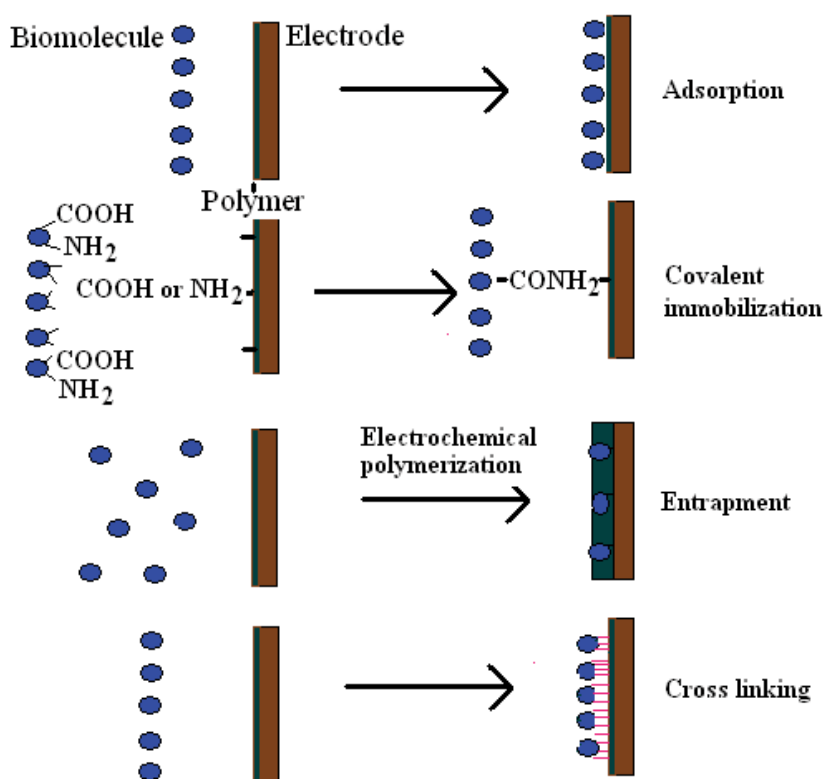
Scheme 2. Schematic representation of process in different immobilization methods.
