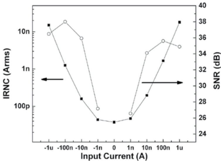
Fig. 10. IRNC and SNR as functions of input currents ranging from -1 to 1 \mu A. The black squares represent the IRNC, whereas the circles illustrate the SNR.
