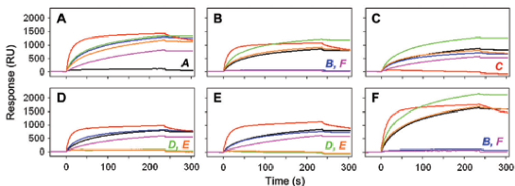
Fig. 10. Classical sandwich binning. Panels are grouped and labeled by the coupled Ab (A-F) and colored by the sandwiching Ab (A-black, B-blue, C-red, D-green, E-orange, and F-pink).
