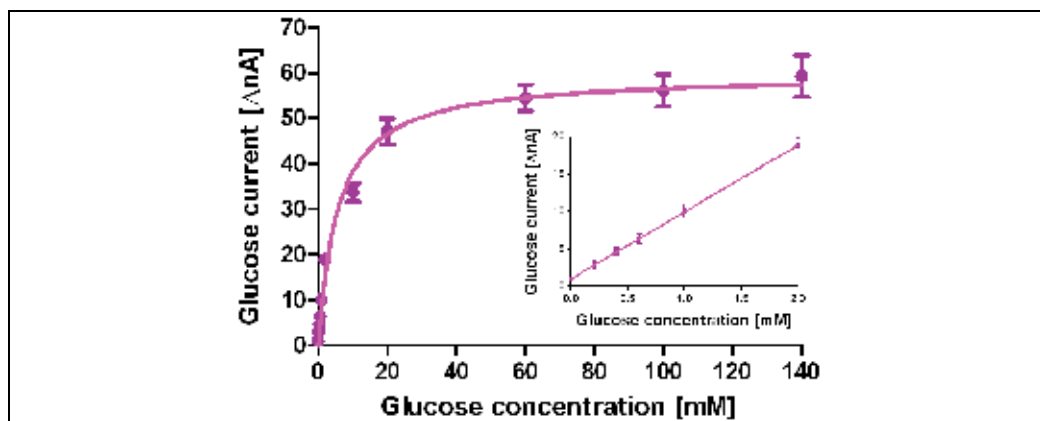
Fig. 13. In-vitro calibration of glucose biosensor (see text).
