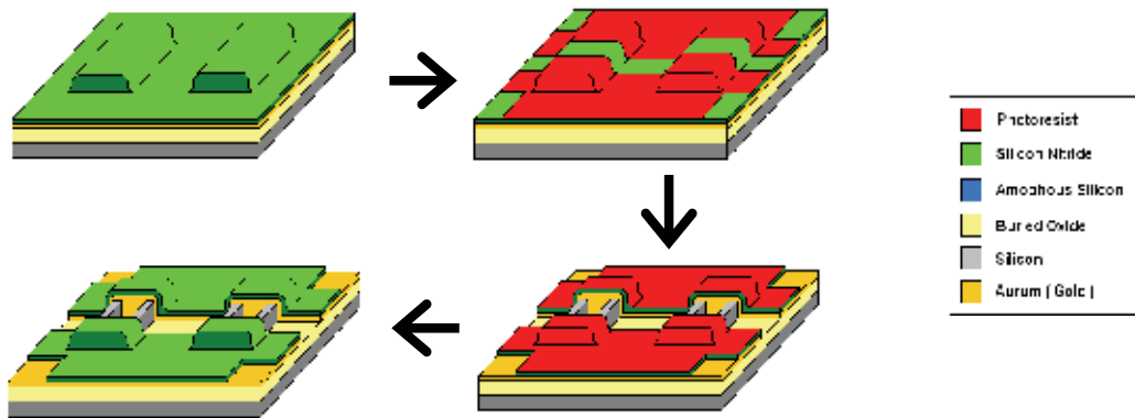
Fig. 7. Si 3 N 4 passivation layer process flow
