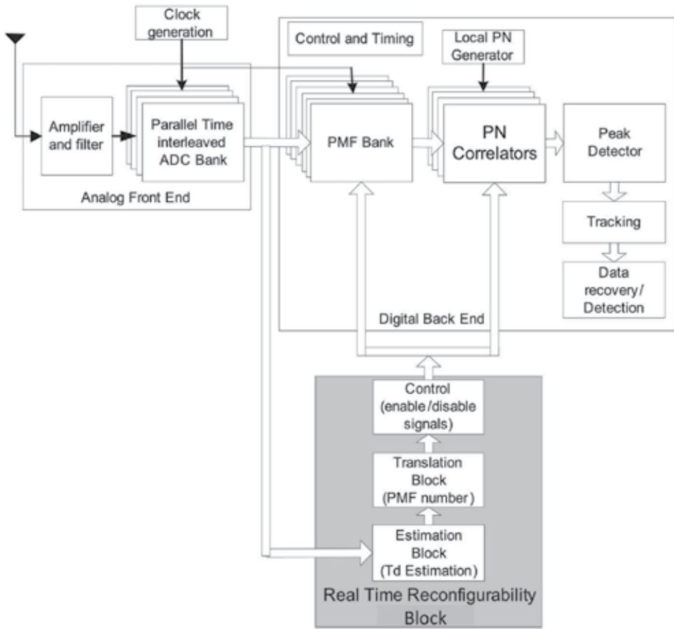
Fig. 6. Real time reconfigurability algorithm architecture
