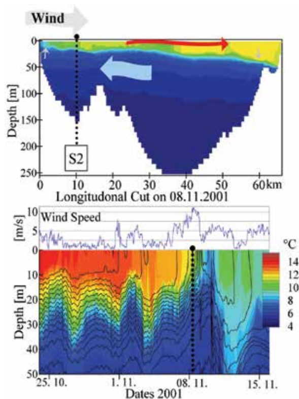
Fig. 8. Upper part: calculated temperature distribution along the longitudinal cut during a strong westerly wind: arrows show flow direction in the epilimnion- and hypolimnion. Lower part: measured (colours) and calculated (lines) temperature profile over time at point S2.
