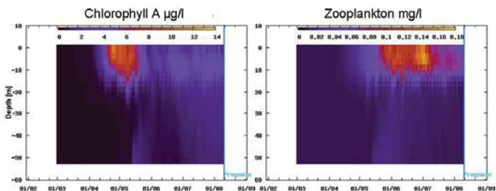
Fig. 6. Calculated profiles of chlorophyll A concentration and zooplankton concentration in BodenseeOnline in spring 2009
