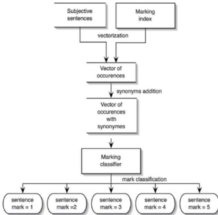
Fig. 5. Subjectivity classification - the classification steps
