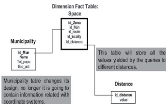
Fig. 8. Changes to the Schema of County and Distances
