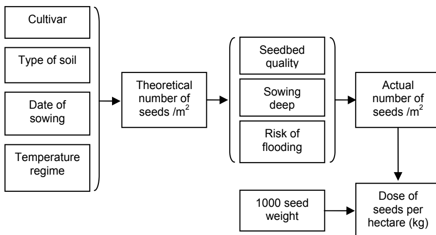
Fig. 13. Flow chart of the step-by-step problem-solving procedure used by the DSS for calculating the optimum seeding rate per hectare.
