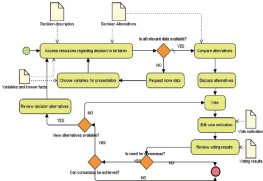
Fig. 8. The collaborative discussion implemented in VCDE
