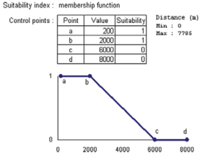
Fig. 4. Membership function used to convert a suitability criterion (in this example, the distance to the nearest high voltage power line is given in meters) into a suitability index.
