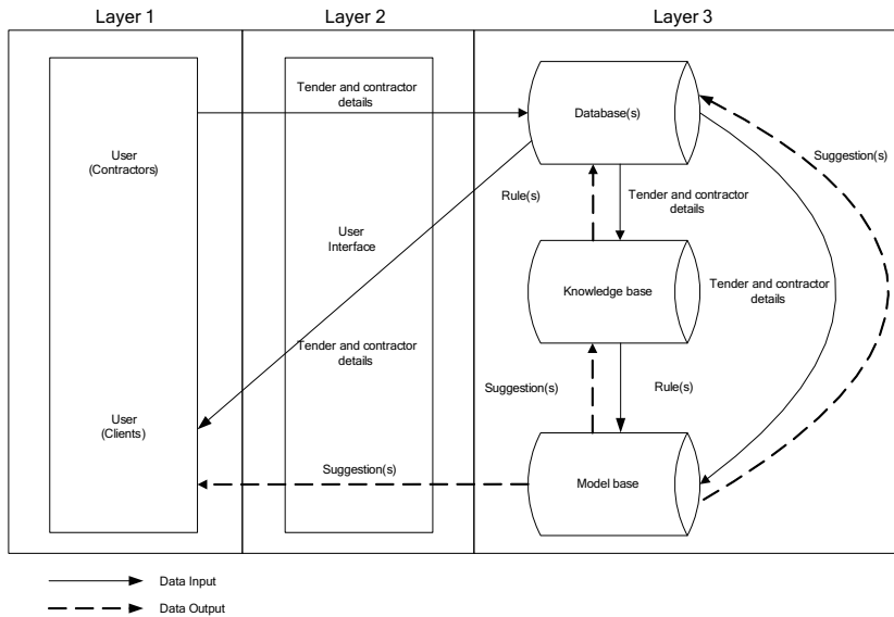
Fig. 5. iWDSS-Tender Detailed Framework
