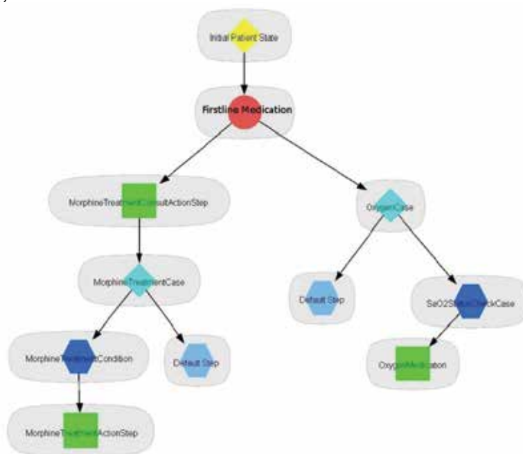
Fig. 2. Flowchart representation of a GLIF-encoded guideline
