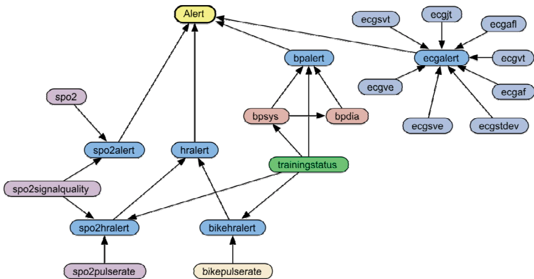
Fig. 10. Bayesian network for alert generation
