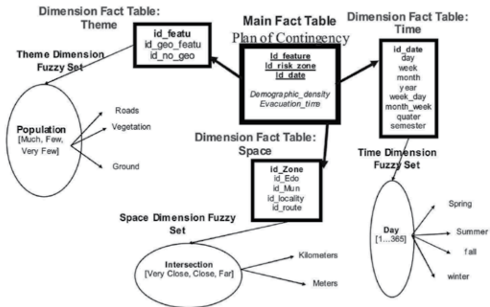
Fig. 5. Fuzzy Sets related to Data Warehouse Dimensions
