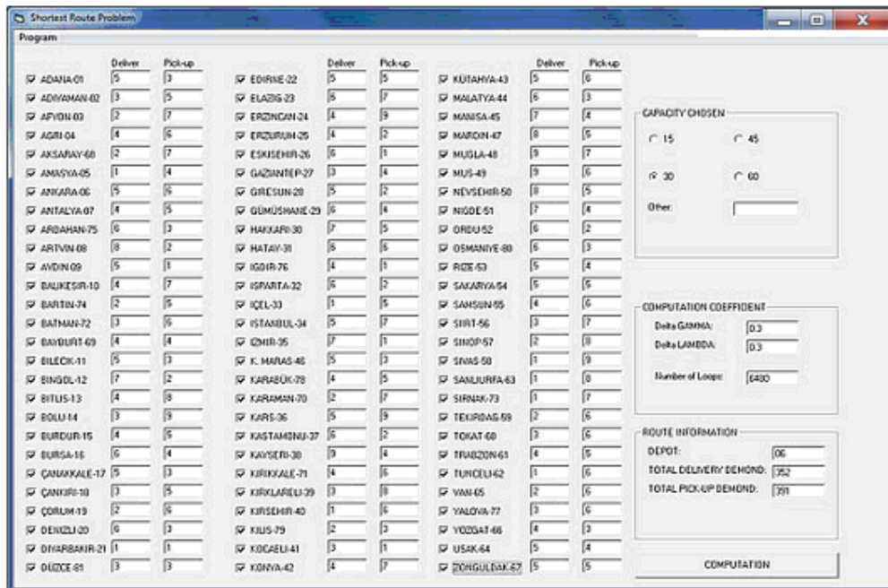
Fig. 3. Computation Interface of the VRP 2.0 Program
