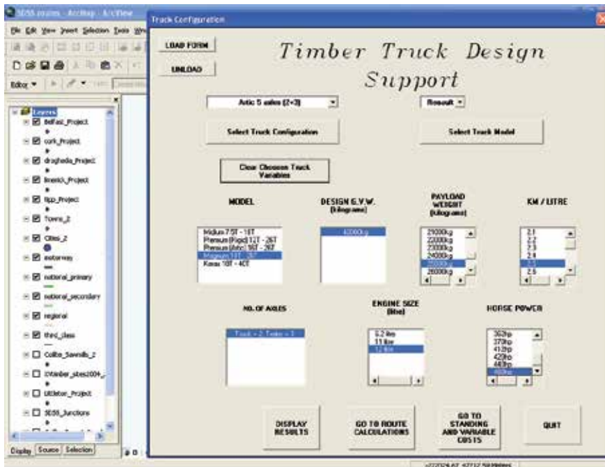
Fig. 2. Screenshot of the Truck Configuration userform.
