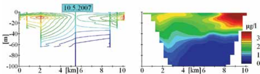
Fig. 13. Measured (left) and calculated (right) concentration of chlorophyll A in a vertical cross section (location see Fig. 12)
