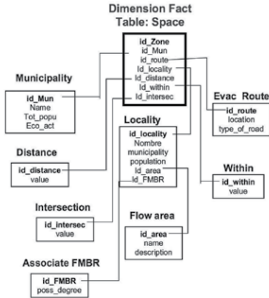
Fig. 9. Modified Schema for Spatial Dimension
