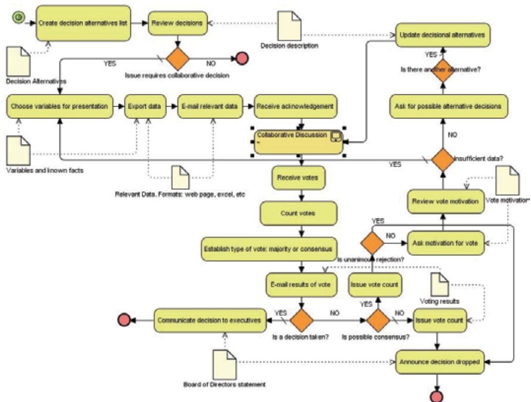
Fig. 7. The collaborative decision process in VCDE
