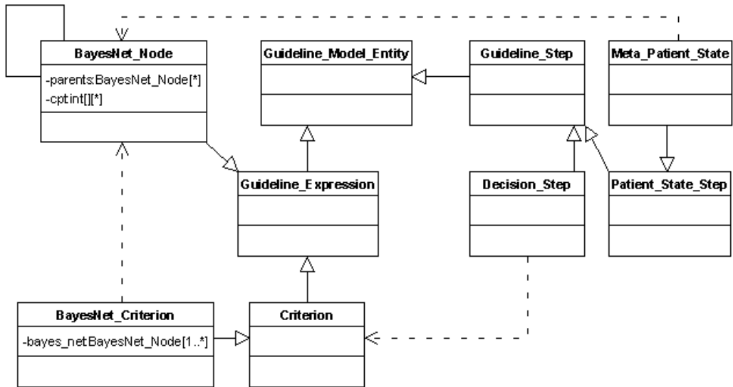
Fig. 9. Extended Guideline Interchange Format
