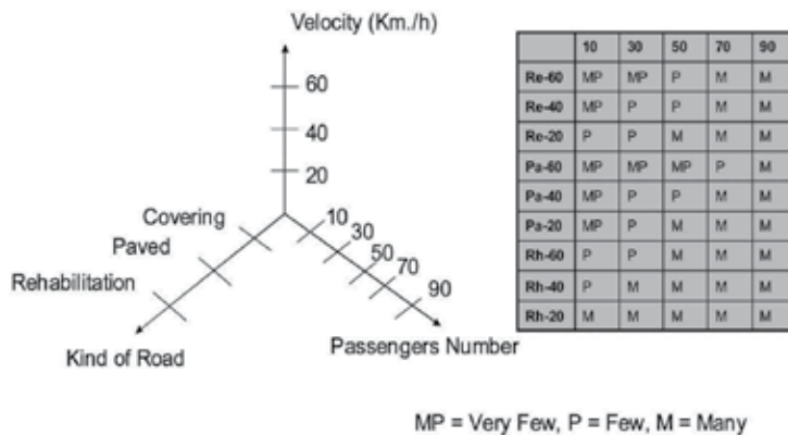
Fig. 11. Empirical Estimation of the Linguistic Variables
