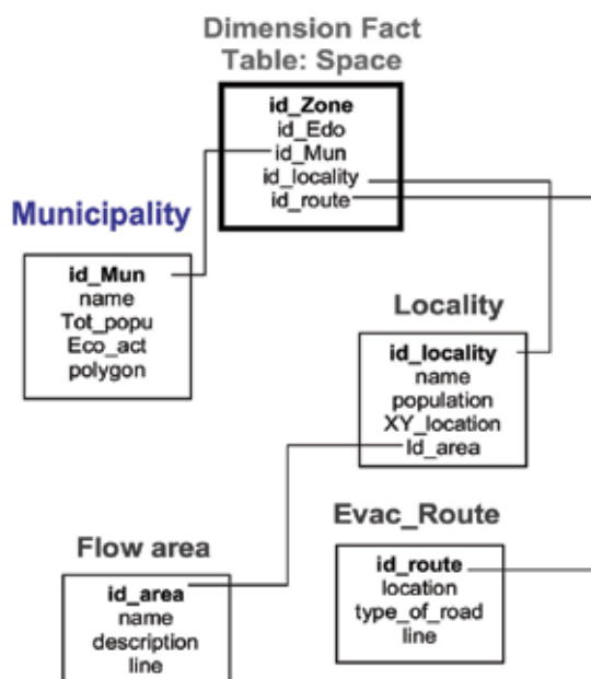
Fig. 6. Space Dimension from the Snow Flake Schema
