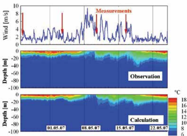
Fig. 11. Observed wind speed, observed and calculated temperature profile in Überlinger See during field campaign 2007
