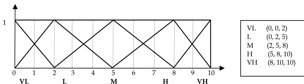
Fig. 5. A linguistic scale for triangular fuzzy numbers
