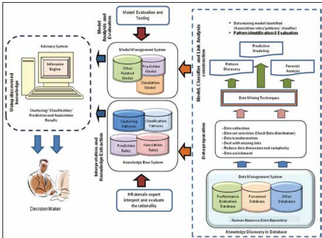
Fig. 2. Suggested HR IDSS Framework
