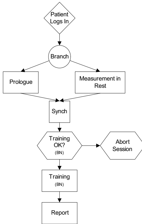
Fig. 8. Training control with a GLIF guideline
