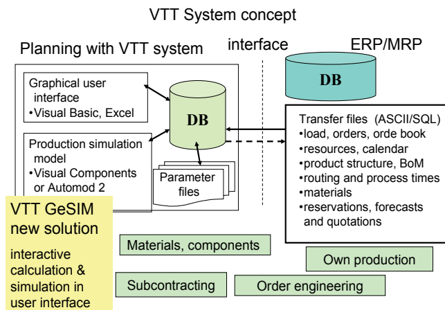
Fig. 8. Current VTT system concept for manufacturing operations planning
