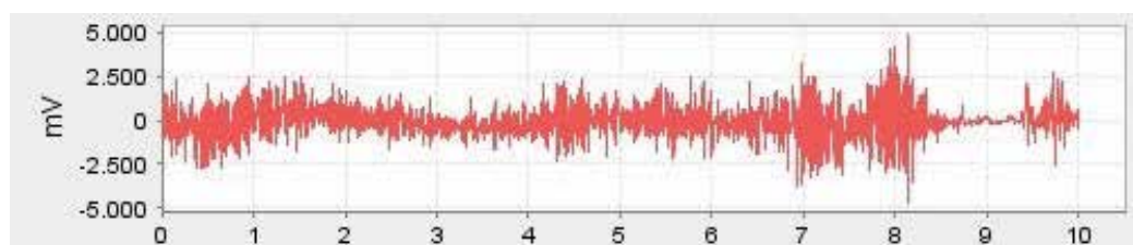
Fig. 7. ECG signal with motion artifacts
