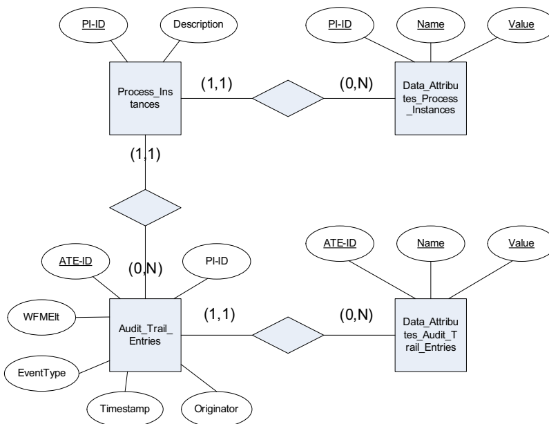
Fig. 9. ERD of tables required for user activity logging in VCDE
