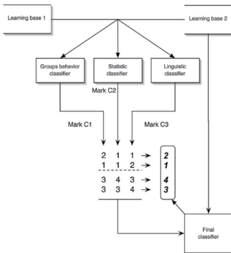
Fig. 6. Final classification- the marks behavior shows the presence of a determinant classifier in some situations
