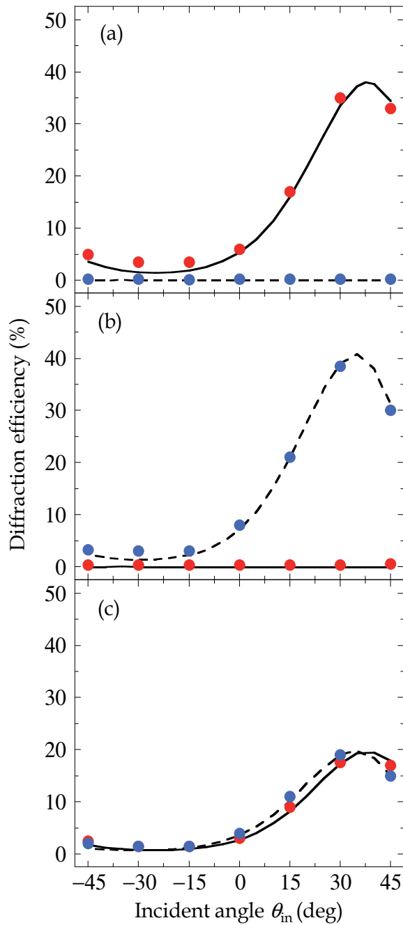
Fig. 7. Angular dispersion of the diffraction efficiency for (a) p -, (b) s -, and (c) q_+ -polarized probe beam. Red and blue plots represent the measured positive and negative first-order diffraction efficiencies. Solid and dashed lines represent the calculated positive and negative first-order diffraction efficiencies
