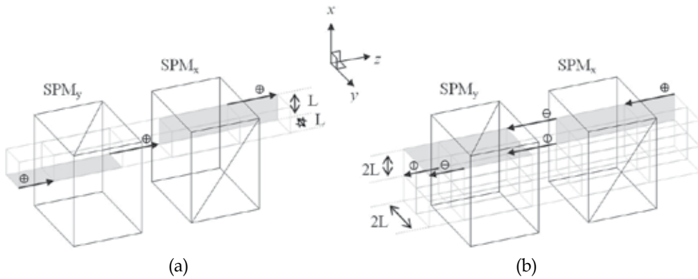
Fig. 11. Structure and operation characteristic of the connected SPM_y and SPM_x for (a) forward and (b) backward transmissions.
