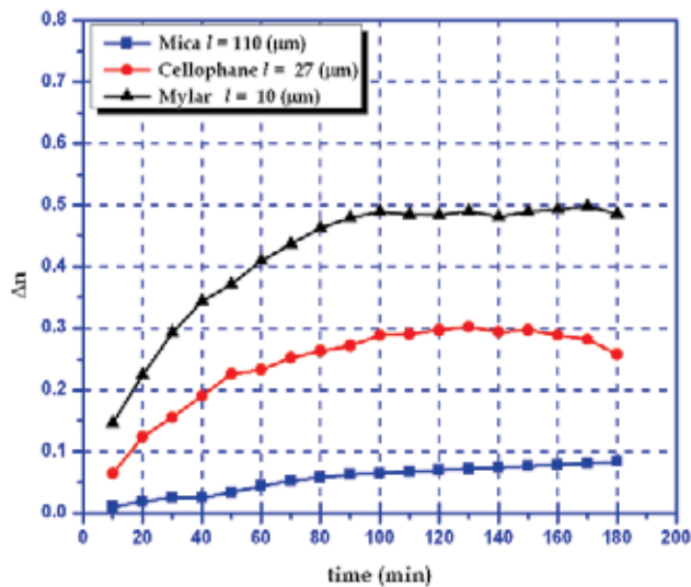
Fig. 14. Modulation amplitude for the refraction index for all thicknesses.
