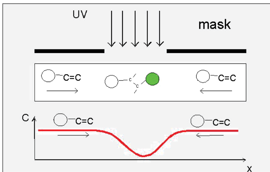
Fig. 10. Illustration of the lithographic writing process.
