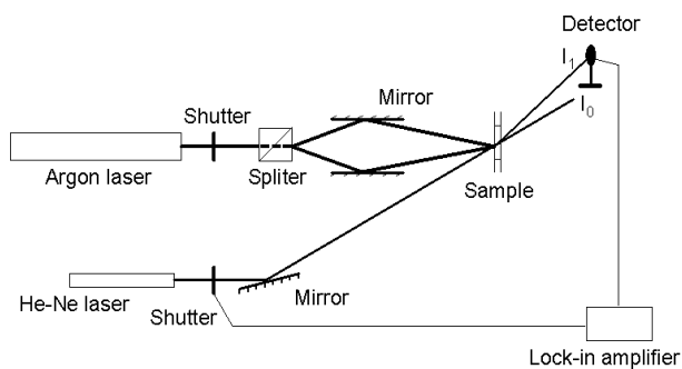
Fig. 2. The optic set-up for the hologram recording.
