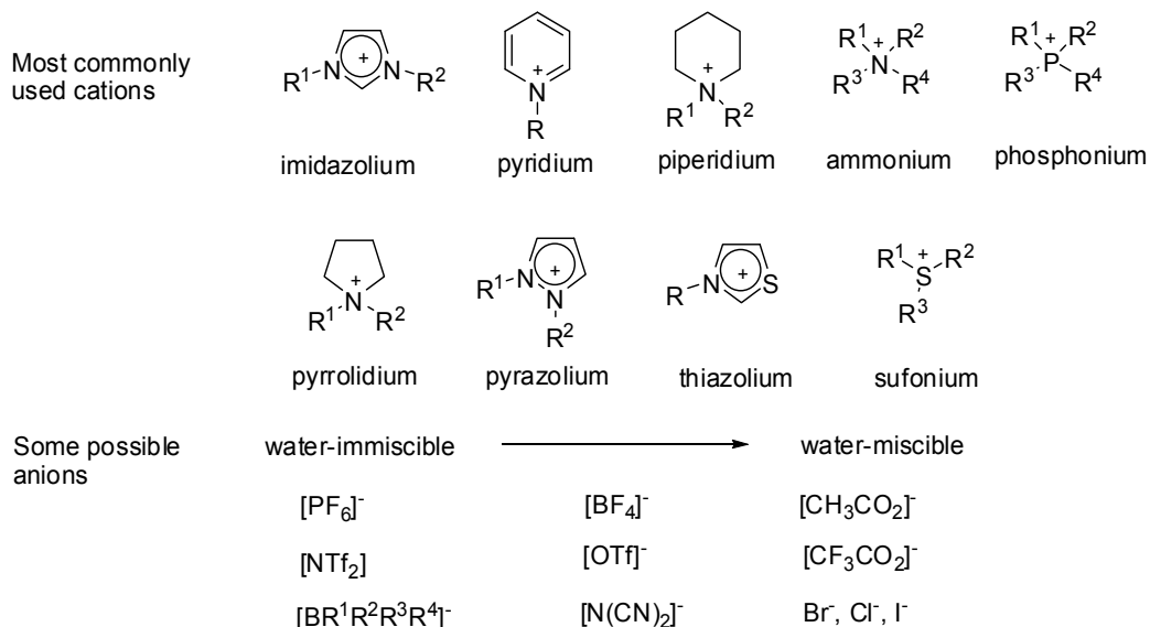
Fig. 1. Chemical structures of typical ionic liquids.
