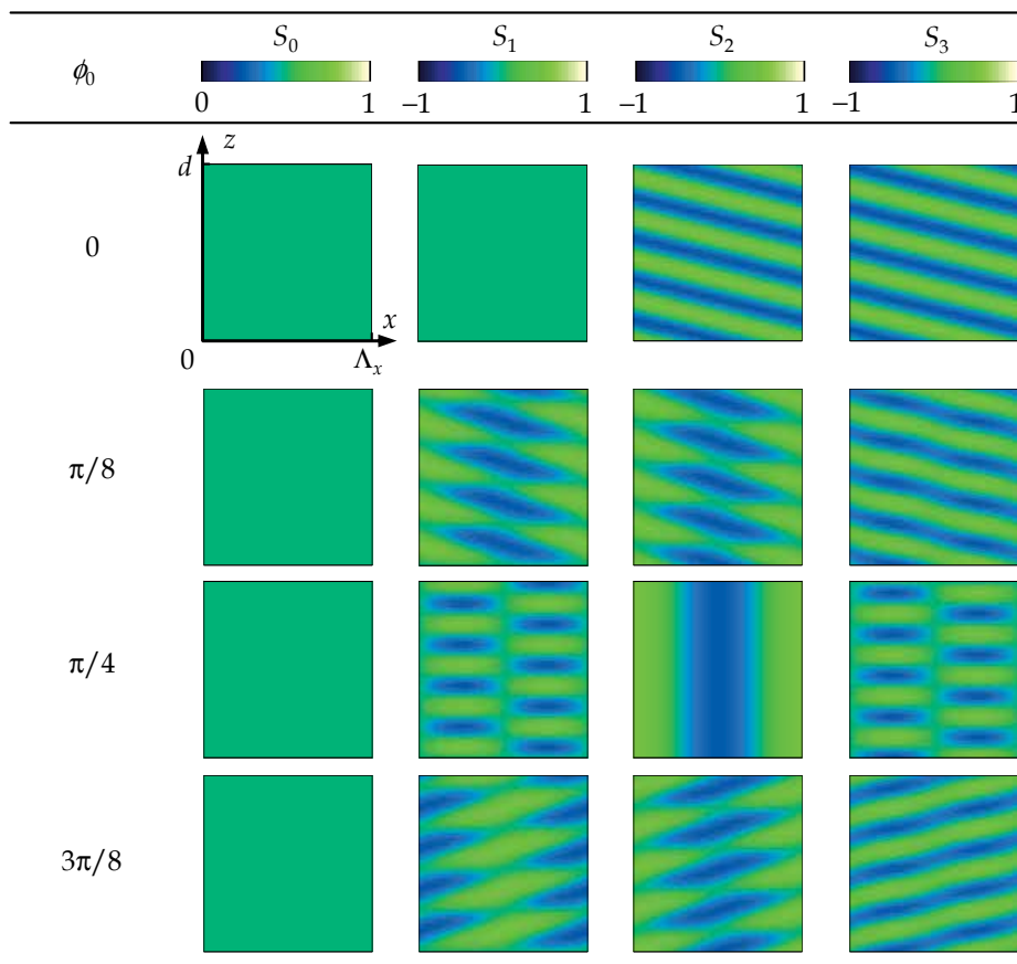
Fig. 4. Spatial distribution of the Stokes parameters in interference light calculated by varying the direction of the optical axis
