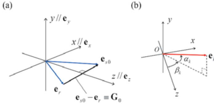
Fig. 5. Definition of (a) the Cartesian coordinate system and (b) the elevation angle \alpha_k and the azimuthal angle \beta_k of the unit direction vector \mathbf{e}_k .
