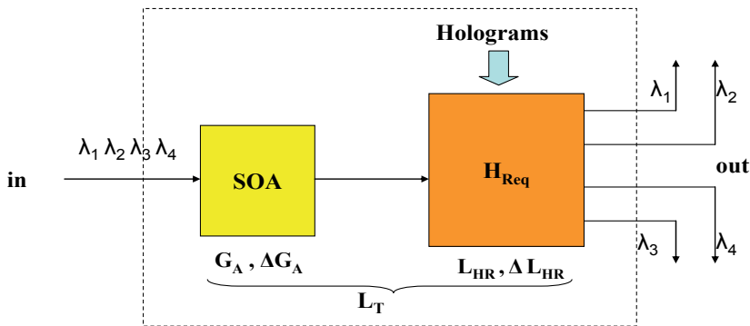
Fig. 14. Equalized Holographic ROADM 1x4
