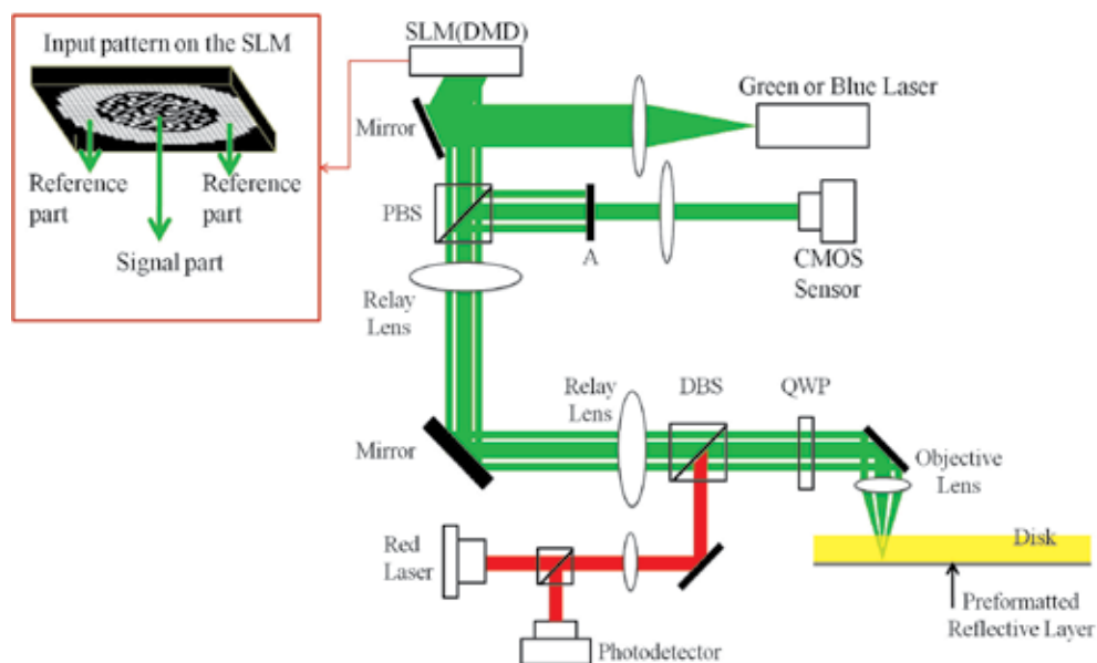
Fig. 1-1. The collinear holographic storage system proposed by Optware [2].
