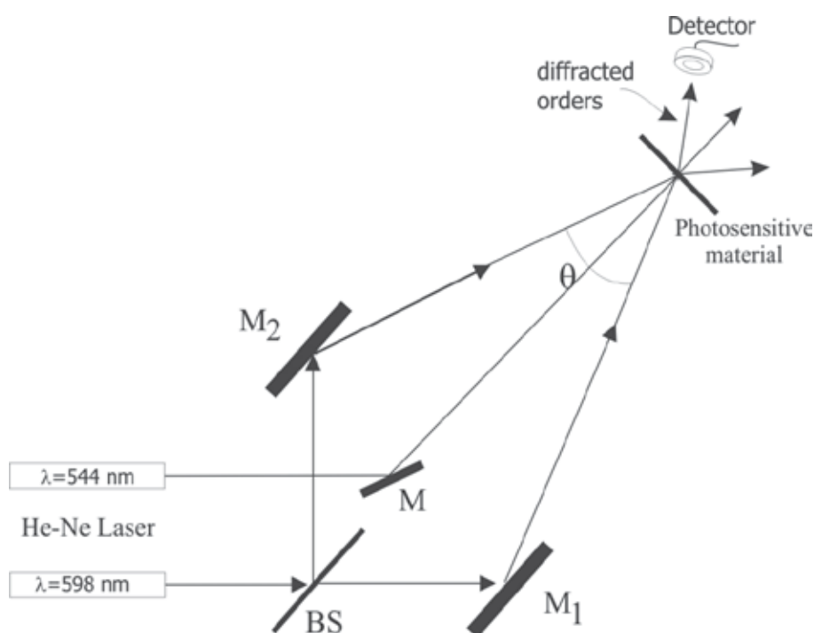
Fig. 7. Setup to make diffraction grating in real time.
