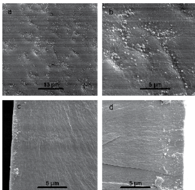
Fig. 14. The SEM images of the diffuser based on sample 2. (a) The surface image in 2000 \times magnification. (b) The surface image in 6000 \times magnification. (c) The cross section near the mask region. (d) The cross section near the substrate.
