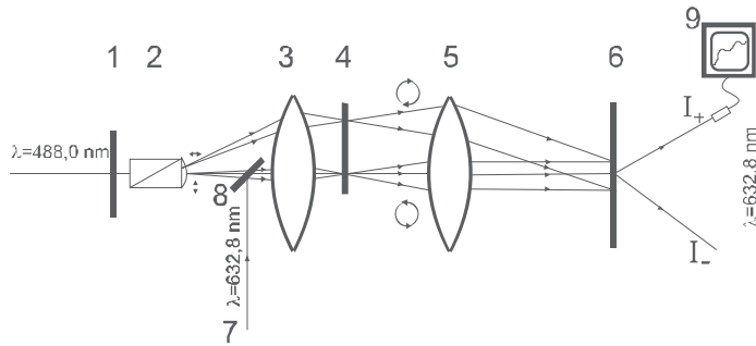
Fig. 20. The scheme of the dynamic holographic recording
