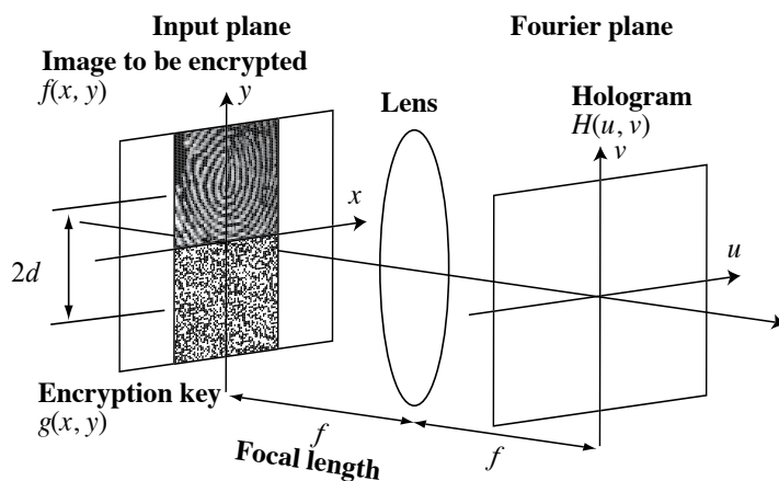
Fig. 2. Optical encryption system using joint Fourier transform
