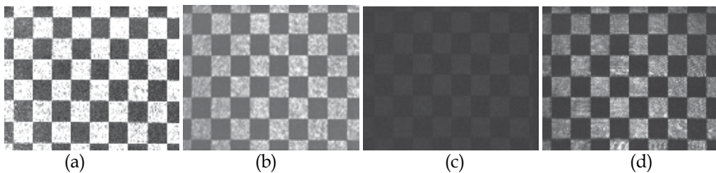
Fig. 29. Results of holographic storage experiments with different polarization recording waves on Fulgide film: (a) parallel linear polarization recording; (b) parallel circular polarization recording; (c) orthogonal linear polarization recording; (d) orthogonal circular polarization recording
