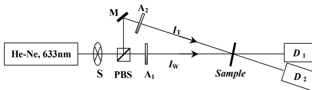
Fig. 12. Schematic of the experimental setup for measuring transmission kinetics.
