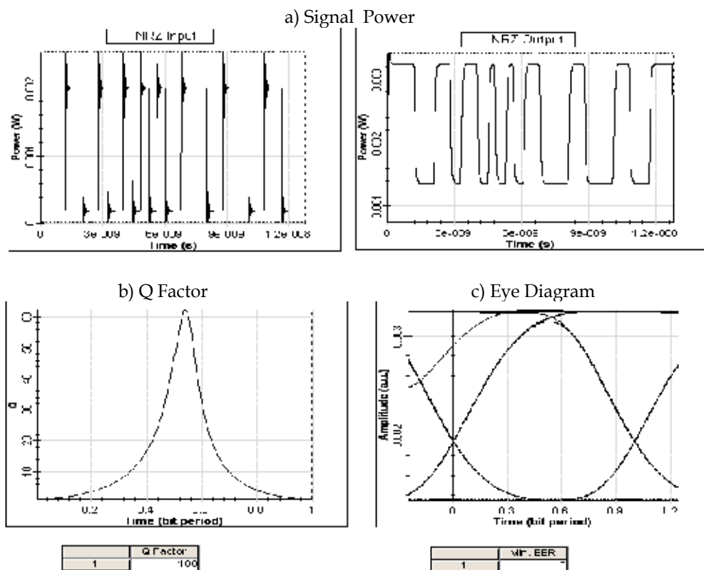
Fig. 20. WCR-HD response for a 2.5 Gbit/s input signal: a) \lambda_i = 1540 nm, with wavelength conversion \lambda_o = 1520 nm, and losses compensation, b) Q factor \approx 100 and c) BER \approx 0 .
