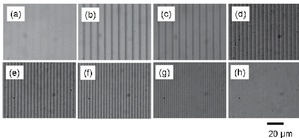
Fig. 6. Comparison of the optic microscopy images of the gratings. (a) Sample 1 (PEGDMA, 4.0g; Irg184, 0.2 g), \eta = 1\% , \Lambda = 10.0 \mu\text{m} , \theta = 1.0^\circ . (b) Sample 2 (PEGDMA, 4.0g; BMIMBF 4 , 1.0g; Irg184, 0.2 g), \eta = 16\% , \Lambda = 10.0 \mu\text{m} , \theta = 1.0^\circ . (c) Sample 22 (PEGDMA/PVAC, 4.0 g, w/w = 10: 1; BMIMBF 4 , 1.0 g; Irg184, 0.08 g), \eta = 34\% , \Lambda = 10.0 \mu\text{m} , \theta = 1.0^\circ . (d) Sample 22, \eta = 14\% , \Lambda = 5.6 \mu\text{m} , \theta = 1.8^\circ . (e) Sample 22, \eta = 11\% , \Lambda = 4.7 \mu\text{m} , \theta = 2.1^\circ . (f) Sample 22, \eta = 8\% , \Lambda = 4.0 \mu\text{m} , \theta = 2.5^\circ . (g) Sample 22, \eta = 3\% , \Lambda = 2.9 \mu\text{m} , \theta = 3.5^\circ . (h) Sample 22, \eta = 1\% , \Lambda = 2.2 \mu\text{m} , \theta = 4.6^\circ .
