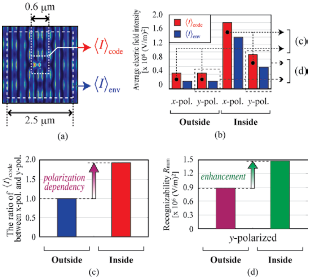
Fig. 9. (a) Schematic diagram explaining definition of average electric field intensities \langle I \rangle_{\text{code}} and \langle I \rangle_{\text{env}} , and (b) their graphical representations in each calculation model. Evident polarization dependency was exhibited in the case of the nanometric code embedded in environmental structures. (c) The ratio of \langle I \rangle_{\text{code}} with x -polarized input light to that with y -polarized input light for the embedded and isolated structures. (d) Numerical visibility R_{\text{num}} in two types of models with y -polarized input light. The result indicates that the visibility of the nanophotonic code was greatly enhanced by embedding it in the environmental structure.
