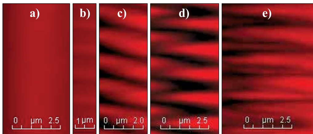
Fig. 22. Image of optical absorption in volume of \text{As}_2\text{S}_3 -Al films after dot-matrix hologram recording ( \lambda=532 \text{ nm} , N=800 \text{ mm}^{-1} , E=10 \text{ J/cm}^2 ). The pictures were obtained while performing Z-scanning ( \lambda=632 \text{ nm} ) by the confocal microscope LEICA TCS SP5. The left part of each picture corresponds to the layer Al, the right one to the film-air surface; a) without recording, b) film 1.2 \mu\text{m} , c) film 2.4 \mu\text{m} , d) film 3.6 \mu\text{m} , e) film 4.8 \mu\text{m} .
