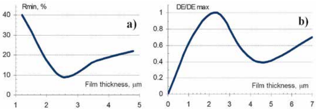
Fig. 20. a) Dependence of minimum reflection R_{\min} of the system \text{As}_2\text{S}_3 -Al on the film thickness ( \lambda=532 \text{ nm} ). b) Dependence of the maximum diffraction efficiency of dot-matrix holograms on the thickness of films \text{As}_2\text{S}_3 -Al
