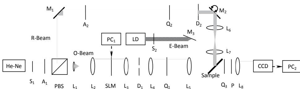
Fig. 28. Fourier transform angular multiplexing holographic storage experimental setup
