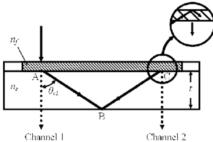
Fig. 4. Schematic representation of the proposed polarization-selective substrate-mode volume hologram (II).
