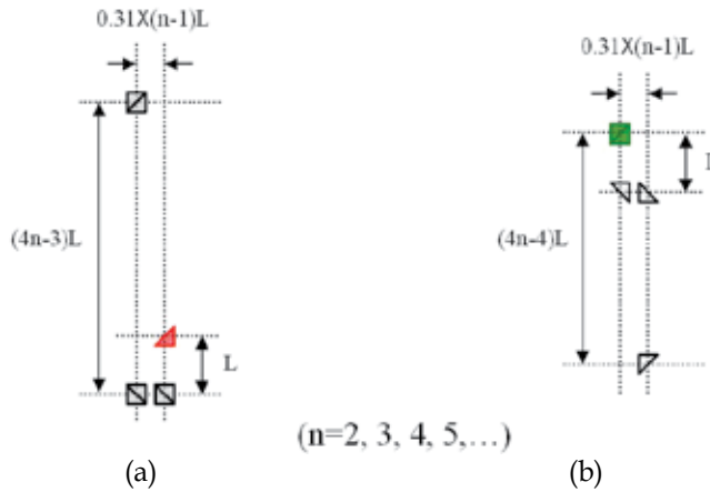
Fig. 17. PBSs and RPs guiding modules for (a) the odd ports; (b) the even ports.
