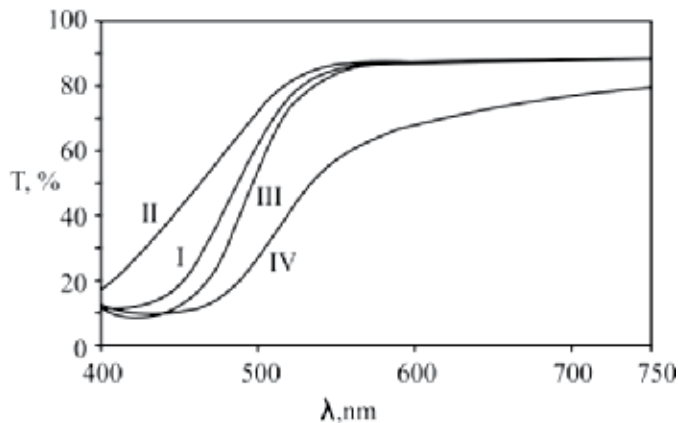
Fig. 2. Polarization spectral transmittance characteristics of azo-dye Mordant Pure Yellow
