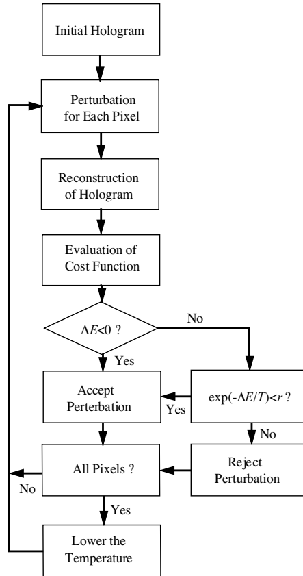
Fig. 6. Algorithm for optimizing hologram by simulated annealing method.
