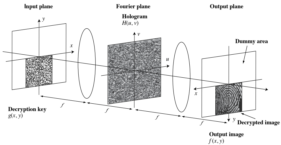
Fig. 4. Optical decryption system
