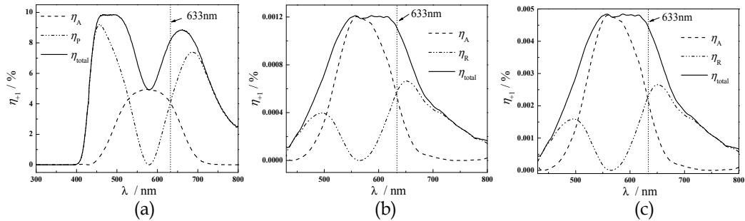
Fig. 17. Diffraction efficiency spectra of the (a) Ordinary holography; (b) Orthogonal linearly polarization holography; (c) Orthogonal circularly polarization holography
