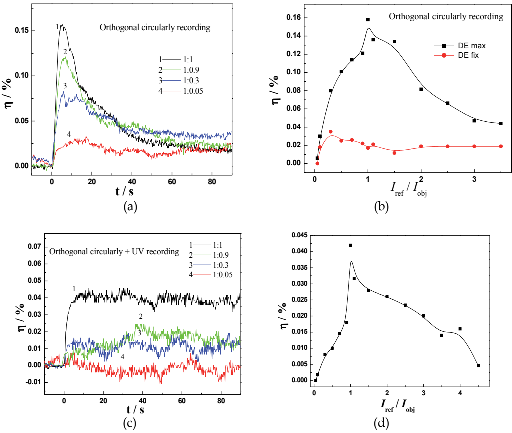
Fig. 20. The diffraction efficiency of orthogonal circularly polarization holograph recording at different ORR: (a) Kinetic curves (without auxiliary light); (b) maximum values and stable values compare (without auxiliary light); (c) Kinetic curves (with auxiliary light); (b) stable values compare (maximum value basically same with the stable values, with auxiliary light)
