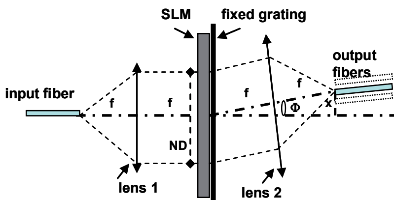
Fig. 6. "4f" dynamic holographic device with a transmissive SLM and fixed grating.
