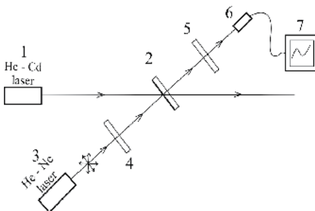
Fig. 4. The scheme of multiple recording and erasure of Weigert's effect
