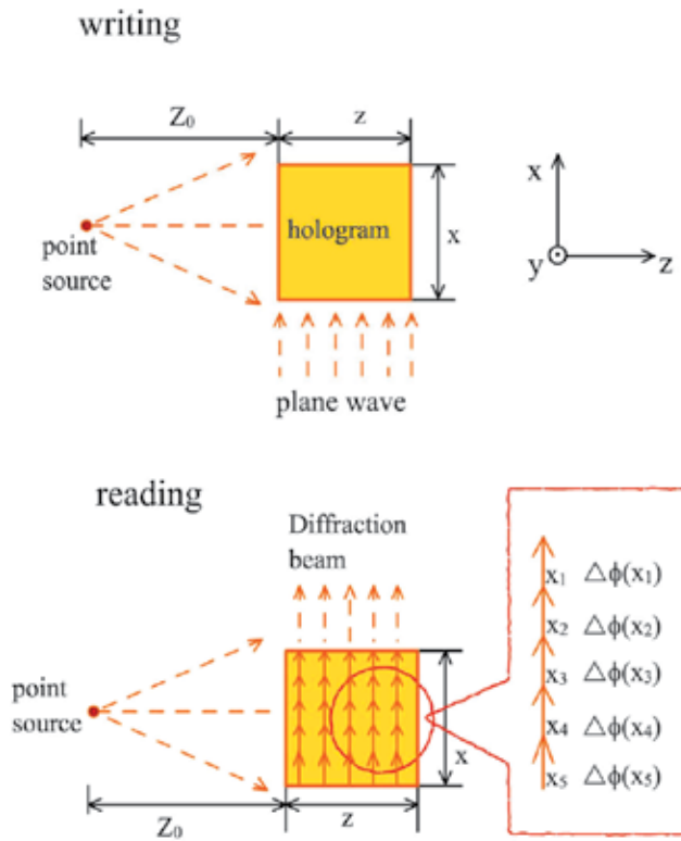
Fig. 1-4. The diagram of VOHIL
