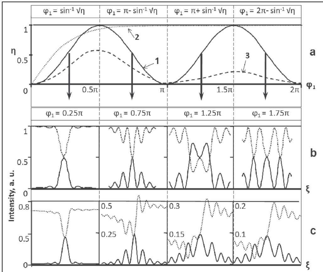
Fig. 1. a - dependence of diffraction efficiency ( \eta ) on phase modulation amplitude ( \varphi_1 ) for volume phase transmission (curve 1) and reflection (curve 2) holograms; amplitude-phase transmission hologram with absorption index \gamma_0 = \gamma_1 = 0.1 (curve 3). b, c - intensity distribution in diffracted (solid lines) and zero (dotted lines) beams at deviation from Bragg conditions ( \xi ) at reconstruction of transmission phase hologram (b) and transmission amplitude-phase hologram (c) at \gamma_1 = \gamma_0 = 0.1 with phase modulation: 1 - \varphi_1 = 0.25\pi , 2 - \varphi_1 = 0.75\pi , 3 - \varphi_1 = 1.25\pi , 4 - \varphi_1 = 1.75\pi .
