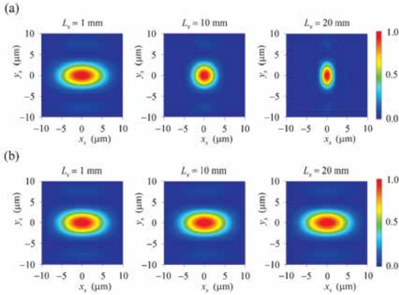
Fig. 15. The input image area suffering from intra-page crosstalk noise in (a) the conventional monochromatic case ( \lambda_w = \lambda_{p0} = 532 nm, \Delta\lambda_p = 0 nm) and (b) the PCR method ( \lambda_w = 532 nm, \lambda_{p0} = 815 nm, \Delta\lambda_p = 50 nm). The calculation parameters are as follows: \beta_{s0} = 30^\circ ; n_w = 1 ; f_s = 100 mm; and L_y = L_z = 10 mm.
