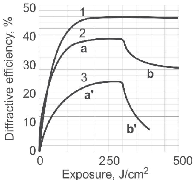
Fig. 21. The dynamic of the holographic recording and reconstruction
