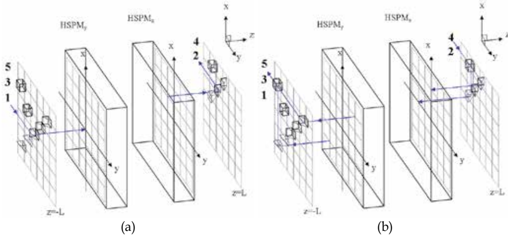
Fig. 18. Structure and operation principles of the proposed 5-port polarization-independent optical quasi-circulator.
