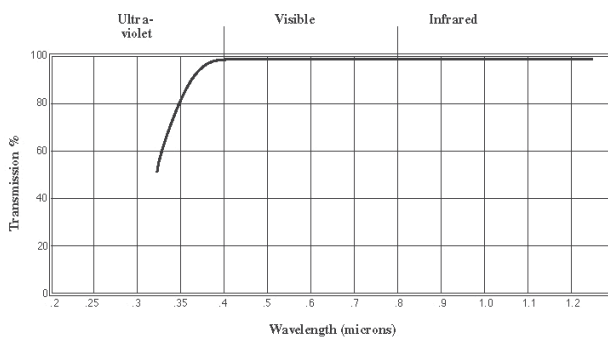
Fig. 2. Transmission spectra for NOA 65.
