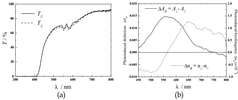
Fig. 11. Spectra of photo-induced anisotropic properties of Indolyfulgimide / PMMA film excited by linearly polarized light: (a) Transmission spectra on directions parallel and perpendicular to exciting beam polarization; (b) Dichroism and birefringence spectra
