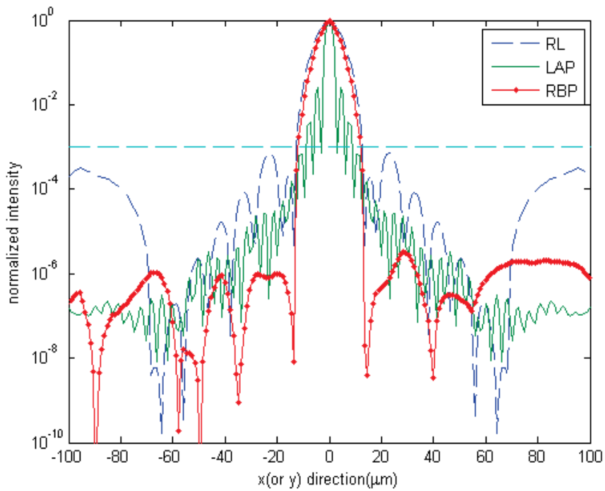
Fig. 1-9. PSF for different reference patterns [19].
