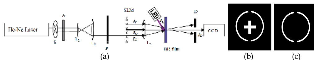
Fig. 33. Optical setup and the patterns displayed on the SLM in rewritable collinear holographic image storage; (a) Optical setup; (b) Recording process pattern; (c) Reading process pattern
