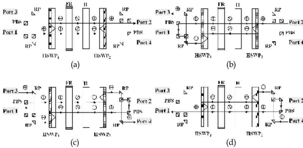
Fig. 13. Structure and operation principles of the 4-port polarization independent optical circulator.
