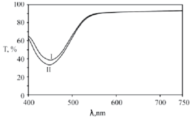
Fig. 1. Spectral transmittance characteristics of azobenzene
