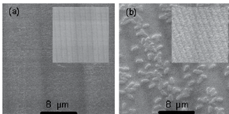
Fig. 9. SEM micrographs of the gratings. (a) sample 2 (PEGDMA, 4.0g; BMIMBF 4 , 1.0g; Irg184, 0.2 g), (b) sample 35 (PEGDMA, 3.4 g; Epoxy L20/Hardener EPH161, 0.5 g, w/w = 4; Irg184, 0.1 g, BMIMBF 4 , 1.0g).
