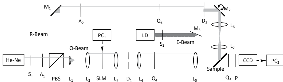
Fig. 27. Fraunhofer angular multiplexing holographic storage experimental setup
