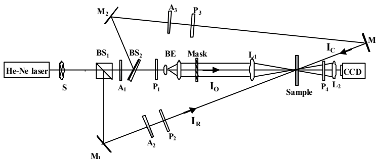
Fig. 23. Experimental setup of reference beam reconstruction holography
