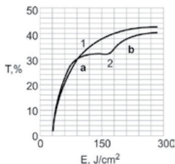
Fig. 24. The dynamic of the Weigert's effect
