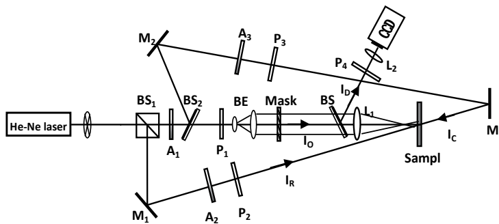
Fig. 24. Experimental setup of conjugated beam reconstruction holography
