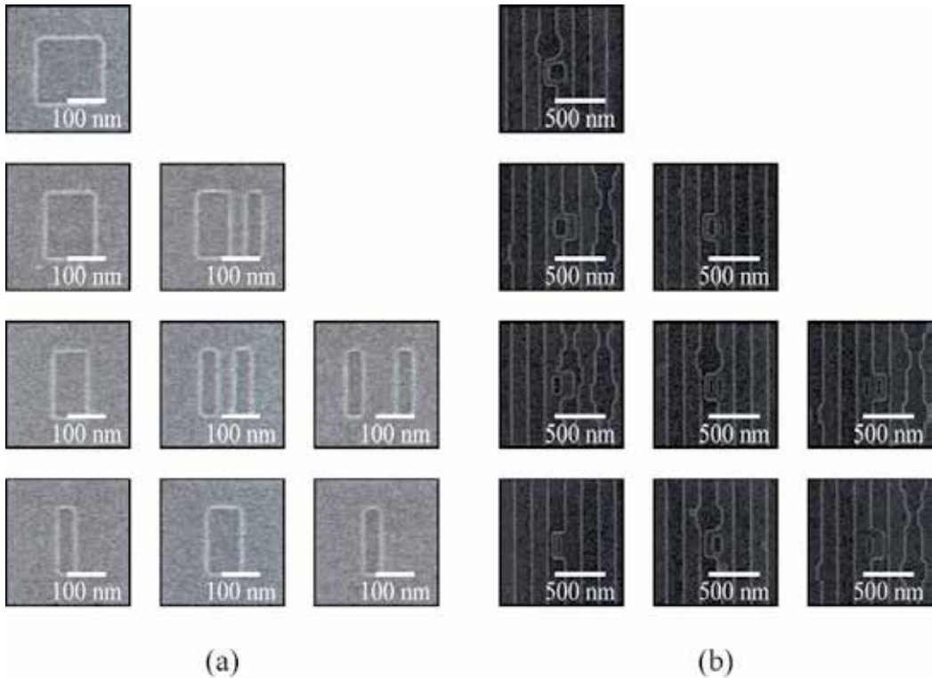
Fig. 6. SEM images of embedded nanometric structures (a) outside and (b) inside the grid structures of the original hologram.
