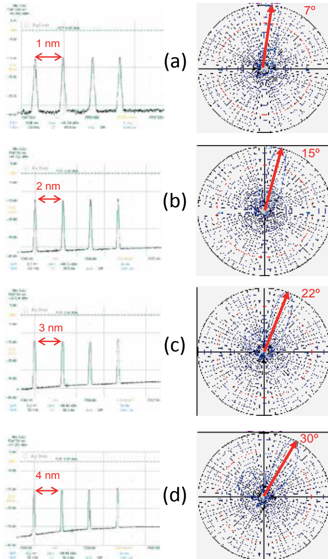
Fig. 12. Opto-VLSI-based tunable laser generations (left), and the corresponding RF beam steering profile measured in the experiments (right).
