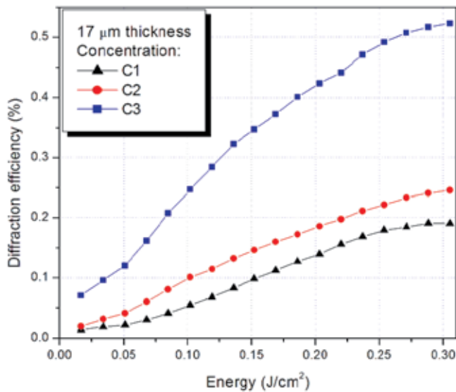
Fig. 9. Diffraction efficiency vs. energy of the three concentrations.
