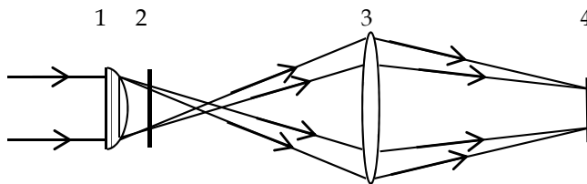
Fig. 10. The scheme of holographic recording of the zone plate
