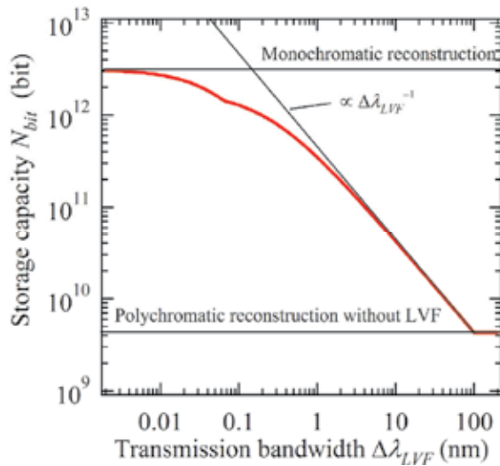
Fig. 18. Storage capacity as a function of transmission bandwidth \Delta\lambda_{LVF} . The calculation parameters are as follows: \lambda_w = 532 nm, \lambda_{p0} = 815 nm, \Delta\lambda_p = 50 nm, \beta_{s0} = 30^\circ , n_w = 1 , and L_x = L_y = L_z = 10 mm.
