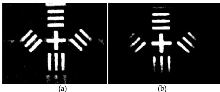
Fig. 25. The reconstructed images of parallel linear polarized transmission hologram and reflection hologram: (a) reconstructed image of transmission recording hologram; (b) reconstructed image of reflection recording hologram
