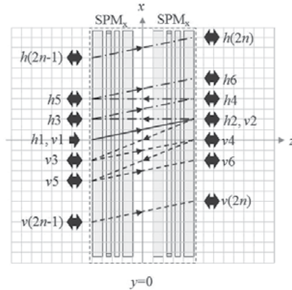
Fig. 10. Operation characteristic for an unpolarized light shuttled between the two sides of two connected SPM x s.
