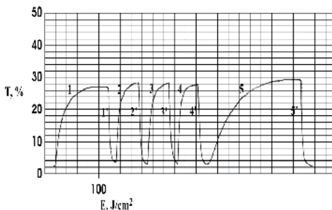
Fig. 5. The dynamics of 5 series of recording and erasure of Weigert's effect
