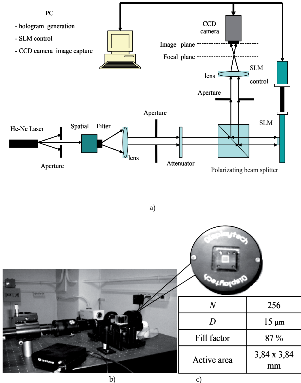
Fig. 8. (a) Optical bench diagram; (b) experimental optical bench and (c) binary phase SLM characteristics
