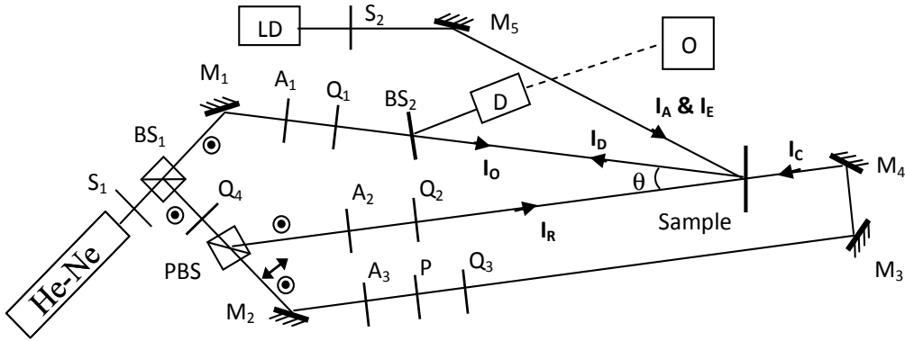
Fig. 14. Schematic of the experimental setup for measuring real-time polarization hologram diffraction kinetics.
