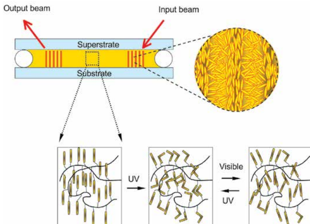
Fig. 9. Periodically flat-structured grating waveguide couplers and photo-switching behaviors.
