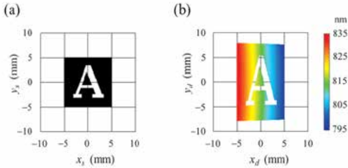
Fig. 4. Simulated results of image reconstruction by PCR. (a) Input image and (b) the reconstructed image. The color in (b) represents the Bragg-matched wavelength of each diffracted wave. The calculation parameters are as follows: \lambda_w = 532\text{ nm} ; \theta_w = 30^\circ ; \theta_p = 50^\circ ; n = 1 ; and f_s = f_d = 100\text{ mm} .
