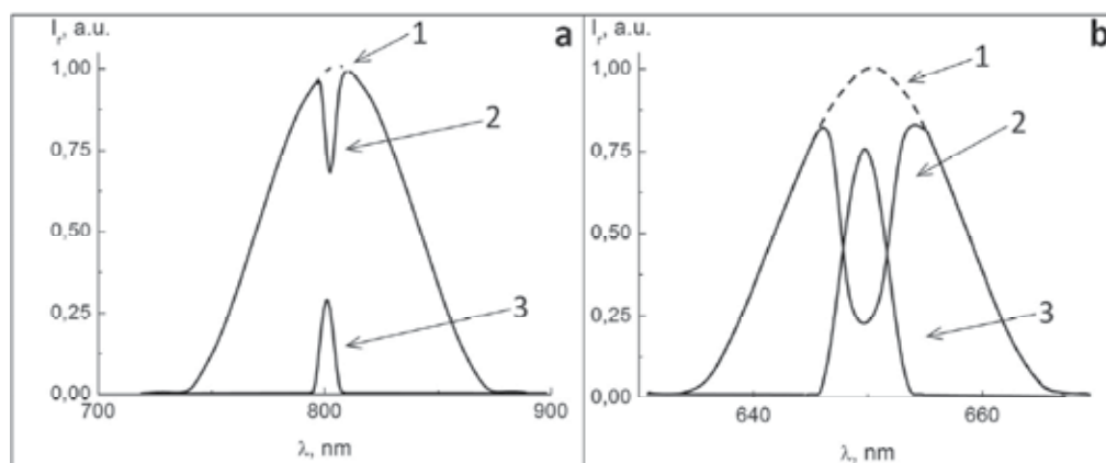
Fig. 14. Spectral distribution of intensity of laser radiation, passed the hologram outside Bragg conditions (curves 1) and under Bragg conditions of hologram reading (curves 2); spectral selectivity contour of a hologram (curves 3): a – femtosecond laser ( \lambda_{\max} = 808 nm); b – semiconductor radiation source ( \lambda_{\max} = 654 nm).
