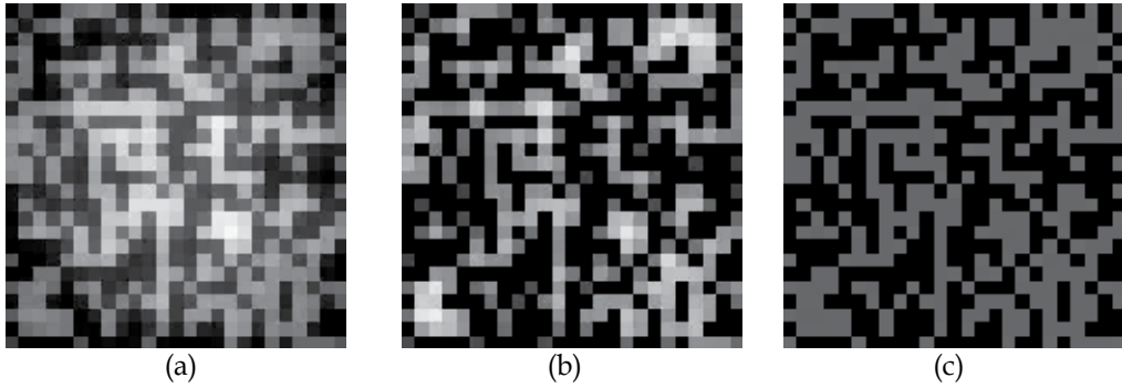
Fig. 1-10. Simulation result of signal detected by the CCD for (a) RL amplitude modulation, (b) RBP modulation and (c) LAP modulation [19].
