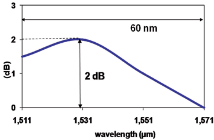
Fig. 13. Incremental gain ( \Delta G_A ) of a typical CWDM SOA
