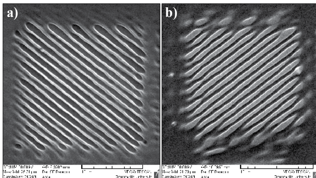
Fig. 12. SEM image of pixel with diffraction grating recorded by image-matrix technology a) positive organic photoresist of the AZ1800 series b) inorganic negative As_{40}S_{20}Se_{40} photoresist.
