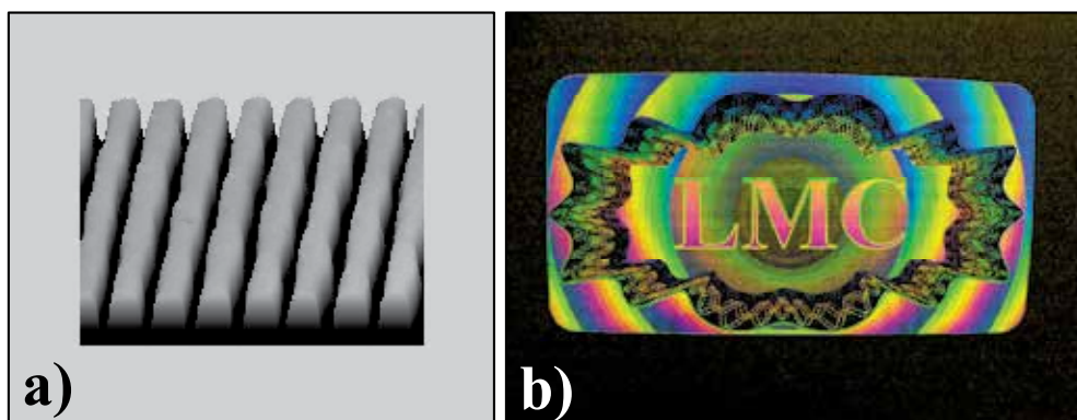
Fig. 11. a) 3D model of the gratings profile based on a SEM image. b) Photo of a protective image-matrix hologram recorded on As_{40}S_{20}Se_{40} photoresist with the help of the created device.
