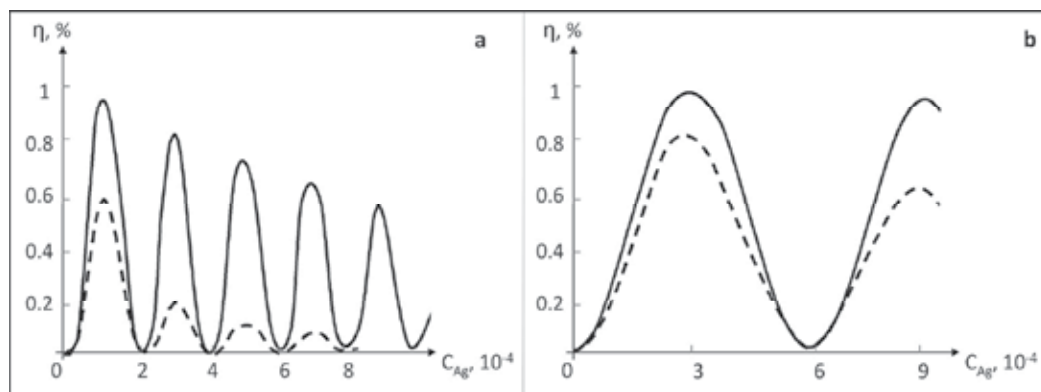
Fig. 6. Theoretically calculated dependences of DE of transmission Ag-PG holograms on developed silver concentration C_{\text{Ag}} for porous medium 1 mm thick with ideal ( l = 8 \text{ nm} , solid curves) and real ( l \approx 2 \text{ nm} , dashed curves) particles: \lambda = 0.63 \mu\text{m} (a) and \lambda = 1.5 \mu\text{m} (b).
