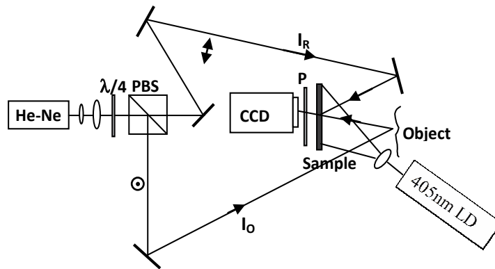
Fig. 31. Diffuse reflection object orthogonal linearly polarization transformation type holographic storage experiment setup
