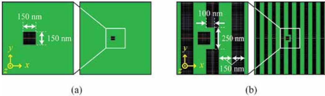
Fig. 7. Calculation model of embedded nanometric structure (a) without and (b) with environmental grid structure.
