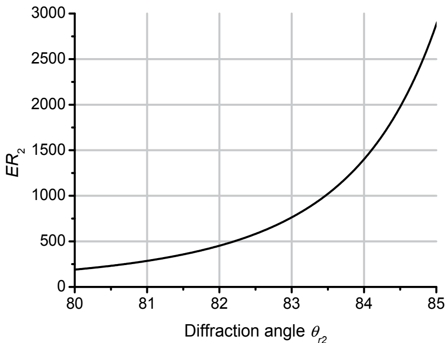
Fig. 7. The theoretical relation of ER_2 v.s. \theta_{r2} .
