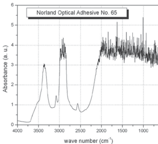
Fig. 3. Absorbance spectra in IR region
