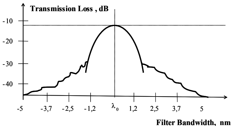
Fig. 7. Holographic filter shape. For wavelengths close to the central value, \lambda < \lambda_0 \pm 1.5 nm, the shape is Gaussian and like a Bessel function for wavelengths \lambda > \lambda_0 \pm 1.5 nm
