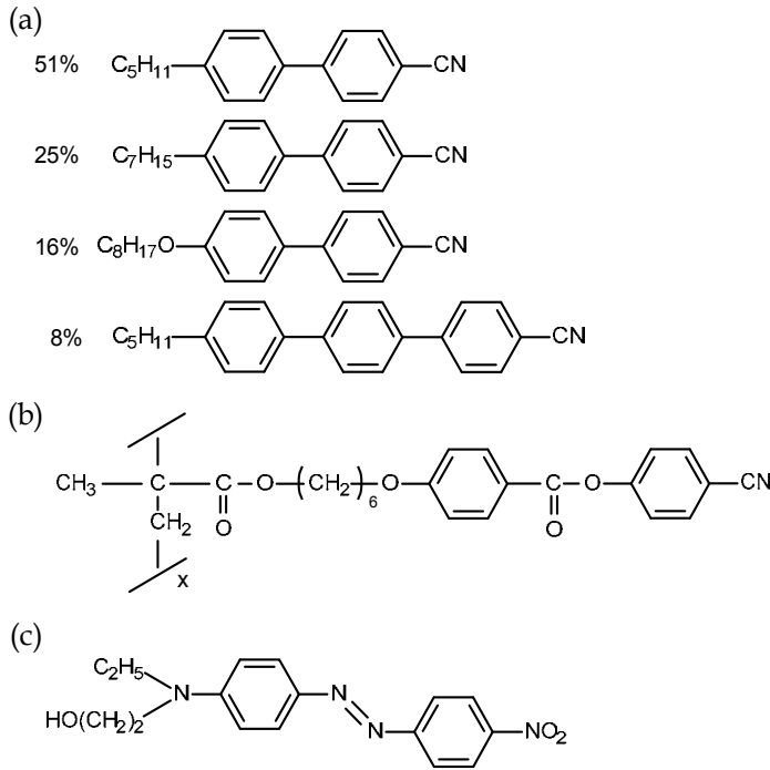
Fig. 5. Chemical structures of (a) E7, (b) SLCP, and (c) DR1
