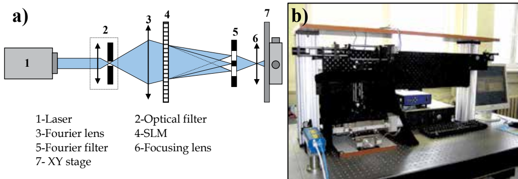
Fig. 8. a) Optical scheme of the image-matrix holographic recording device. b) Photo of the device.
