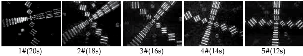
Fig. 36. The experimental results of angular multiplexing holograms
