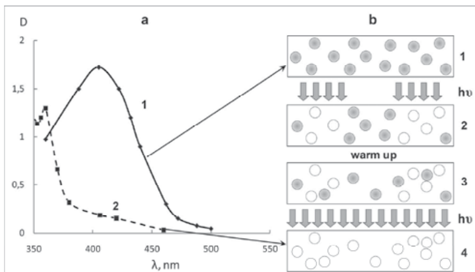
Fig. 7. a – absorption spectra of PQ (curve 1) and photoproduct (curve 2) in polymeric matrix. b – diagram to explain hologram construction process in polymeric medium with diffusion enhancement: distribution of molecules of PQ (○) and photoproduct (●) across the sample bulk in the initial state (1), after recording of hologram-grating (2), after warm-up (3), after fixation (4).
