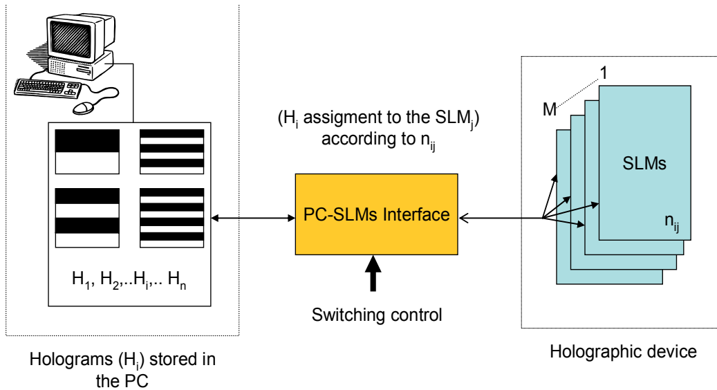
Fig. 5. Tunable holographic device: switching operation
