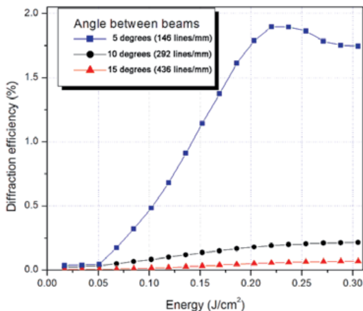
Fig. 12. Diffraction efficiencies for different frequencies.
