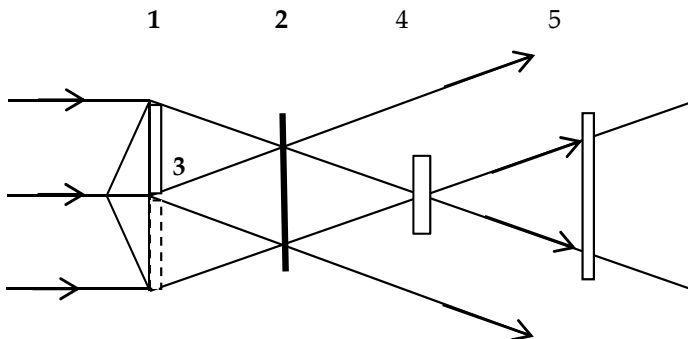
Fig. 25. The scheme of the holographic recording.
