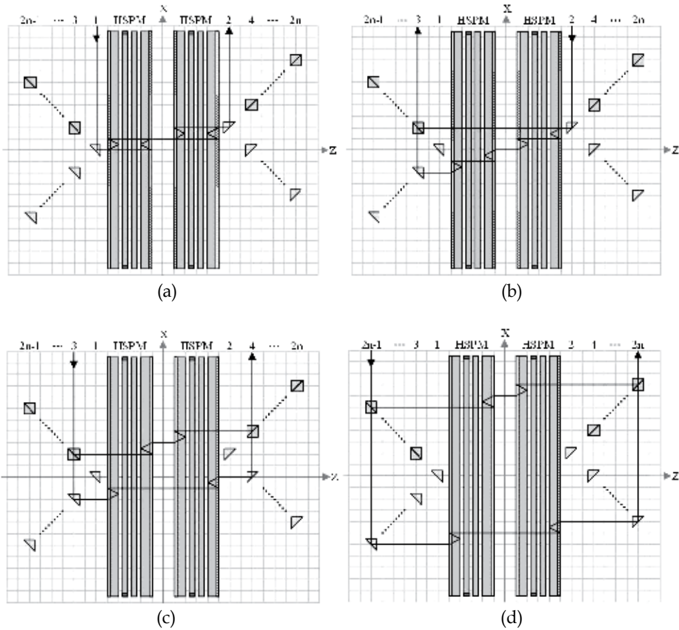
Fig. 15. Structure and operation principles of the proposed multi-port optical quasi-circulator.
