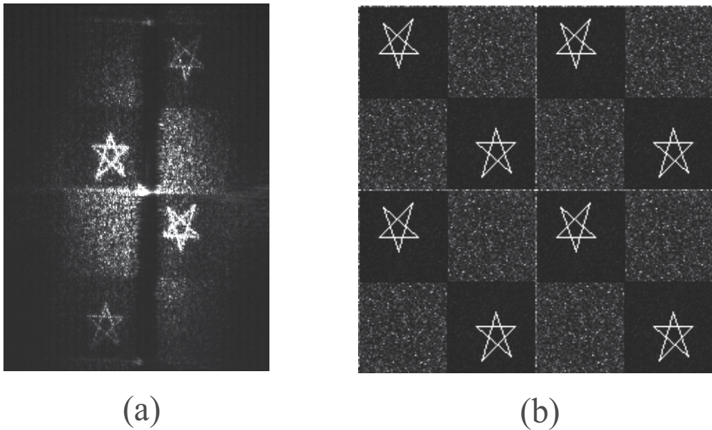
Fig. 20. Experimental result of optical phase-coding method. (a) Optical and (b) simulation results.
