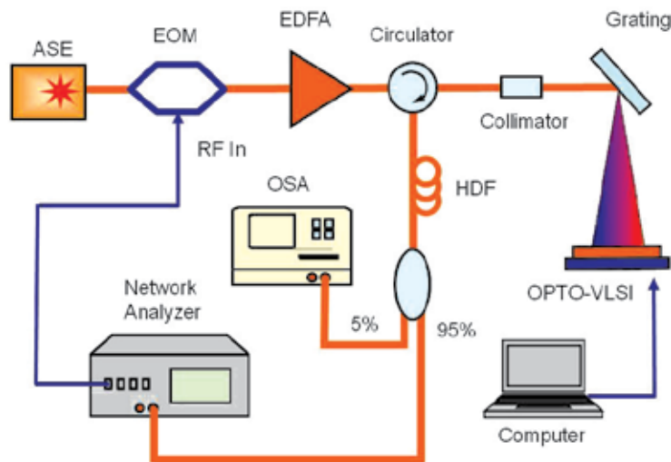
Fig. 4. Experimental setup for the tunable photonic microwave filter structure.
