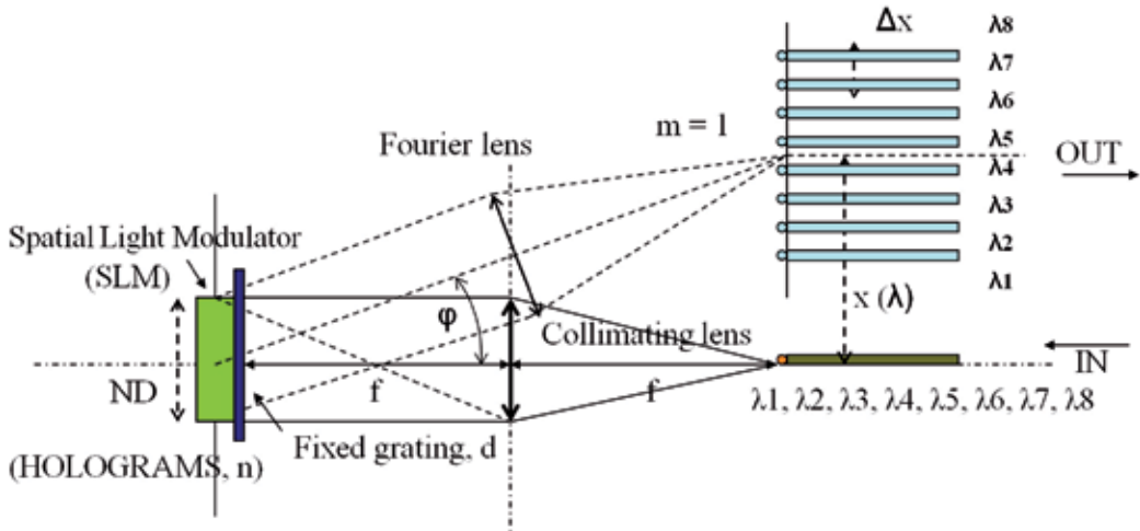
Fig. 11. Reflective holographic router
