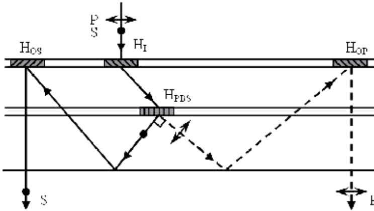
Fig. 1. Schematic representation of the conventional polarization-selective substrate-mode volume hologram.
