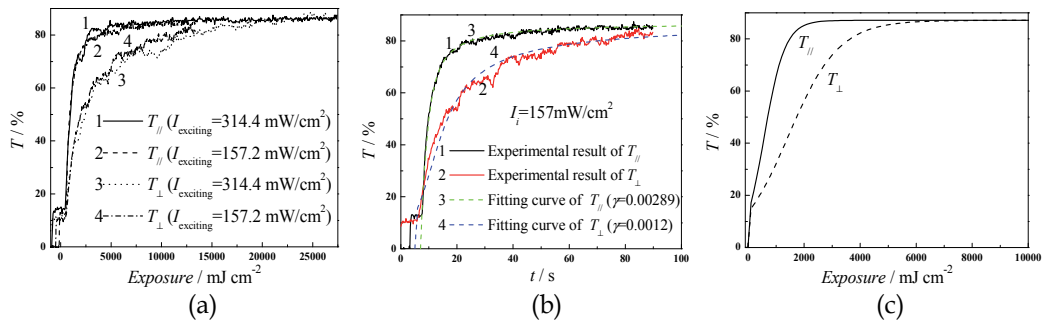
Fig. 13. Photo-induced anisotropic transmission curves of Indolyfulgimide/PMMA film on the directions parallel or perpendicular to exciting beam polarization depending on the exposure or erasing time: (a) Experiment curves measured at different exciting beam intensity; (b) Simulation of experimental results; (c) Calculated curves of uniformity light
