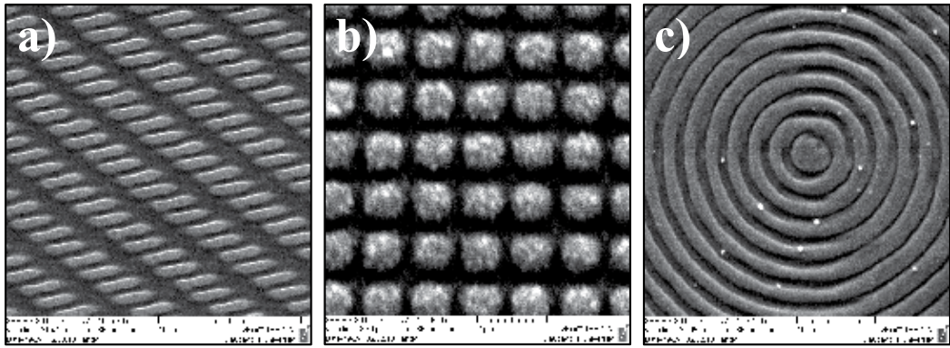
Fig. 15. Samples of microstructure that were recorded on As-S-Se photoresist with the help of image-matrix technology: a) complex grating, b) 2D diffraction grating, c) axicon.
