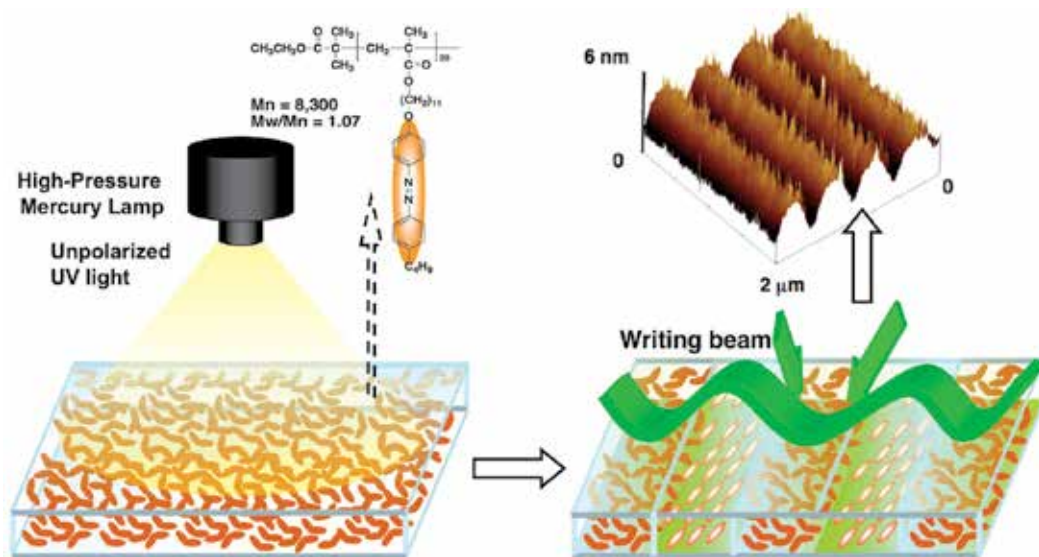
Fig. 10. Subwavelength modulation of surface relief and refractive index in LC polymer films.
