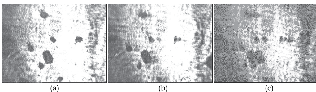
Fig. 41. The double exposure experimental results to record movement track of the particles at different times (a) 1 st image recorded as parallel linearly polarization hologram; (b) 2 nd image recorded as orthogonal linearly polarization hologram; (c) reconstructed image obtained when the polarization P is rotated to 30°
