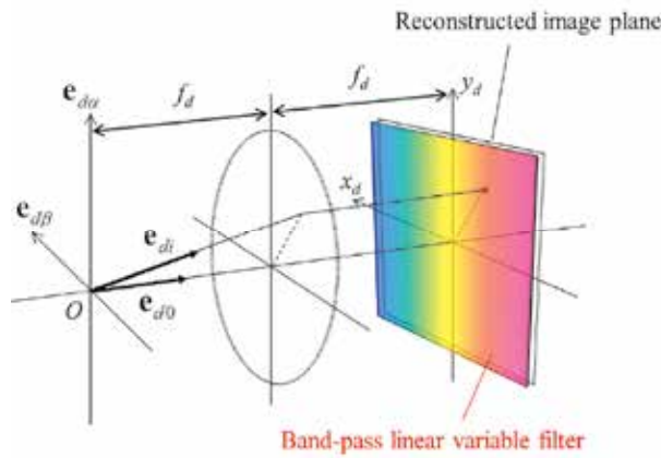
Fig. 16. Configuration for the selective detection method. A special wavelength filter, like a band-pass linear variable filter, is inserted at the reconstructed image plane.
