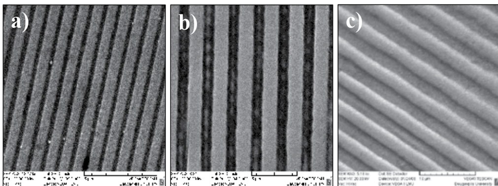
Fig. 18. SEM images of diffraction gratings recorded in different modes of operation on A_{40}S_{20}Se_{40} thin films: a) phase modulation regime with Fourier filtration (period 1\ \mu\text{m} ), b) amplitude modulation regime (period 2.5\ \mu\text{m} ), and c) phase contrast method (period 5\ \mu\text{m} ).
