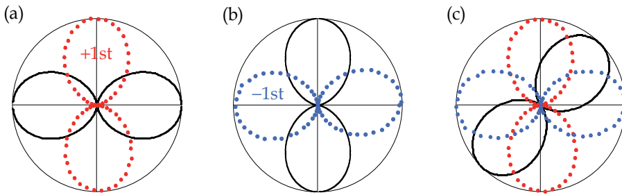
Fig. 8. Polar plots of polarization states for incident and diffraction beams. The incident beam, indicated as solid lines, is (a) p -, (b) s -, and (c) q_+ -polarized. Red and blue plots represent measured data for positive and negative first-order diffraction beams
