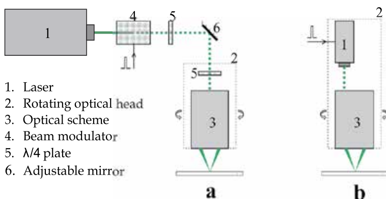
Fig. 6. Entering of the laser beam into a rotating optical part of the dot-matrix recording device. a) The laser is located outside of optical scheme. b) Laser is integrated into the optical scheme.
