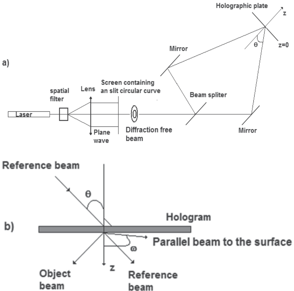
Fig. 2. In a) Experimental Set up for generate the hologram, the radius of the circular slit is 2 mm. approximately and the recording angle \theta is in the range [15^\circ-20^\circ] . In b), The arrows represent the direction of propagation for the set of diffraction free beams generated during the reconstruction process.
