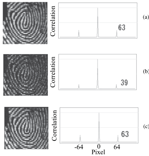
Fig. 8. Reconstructed images (left) and correlations with original image (right). (a) Original fingerprint image, (b) reconstructed image without optimization, and (c) reconstructed image with optimization.
