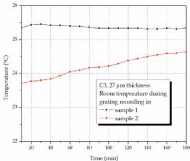
Fig. 16. (b). Temperature behavior during the recording process in the 27 \mu\text{m} thickness cell of two holographic gratings. The red and black line in both plots corresponds to same experiment.
