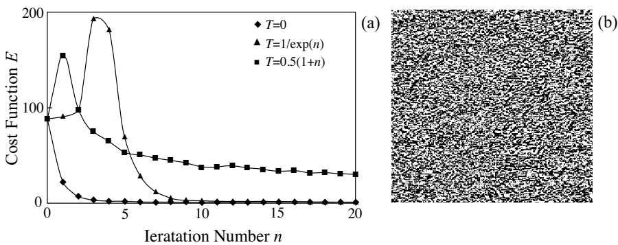
Fig. 7. (a) Variations of cost functions for each cooling schedule and (b) optimized binary hologram at T=0 .
