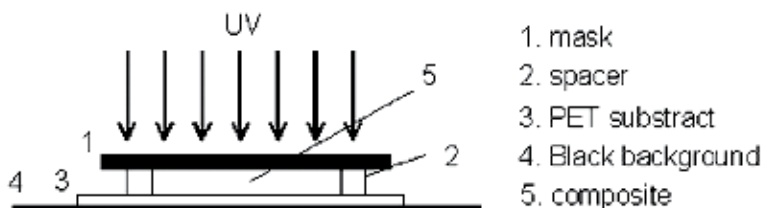
Fig. 3. The optic set-up for fabricating optic diffuser.
