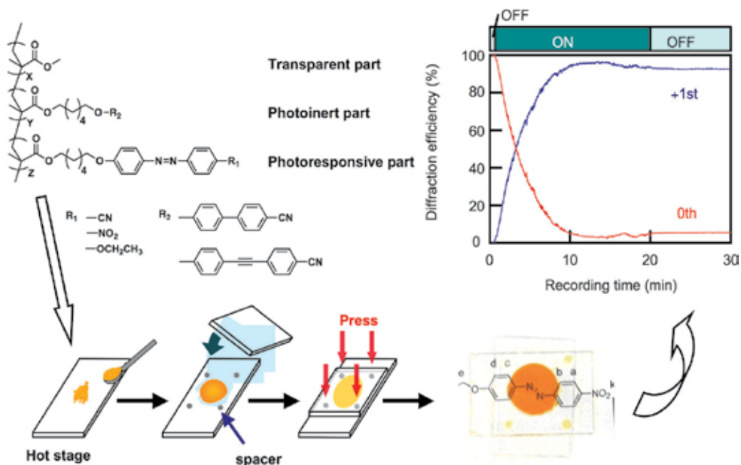
Fig. 14. Transparent and thick films of AZ-containing copolymers for Bragg gratings.
