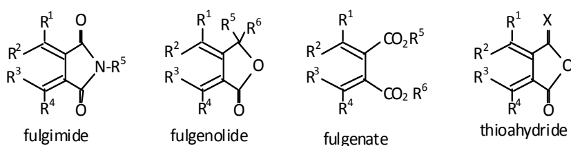
Fig. 6. Chemical molecular formula of the fulgide derivatives
