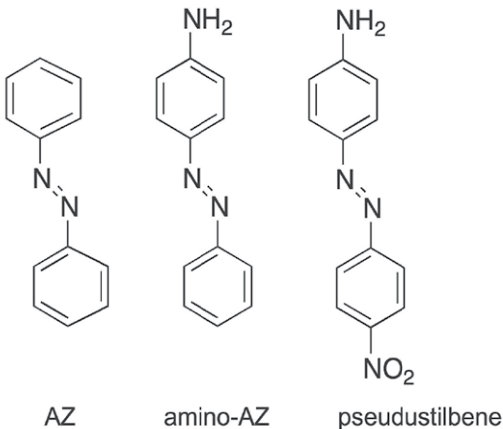
Fig. 3. Examples of three kinds of AZs classified by Natansohn and Kumar.
