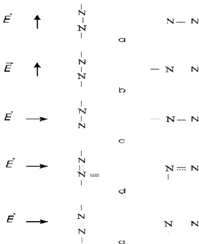
Fig. 6. The scheme of transformation of absorbing oscillators of azo-dye
