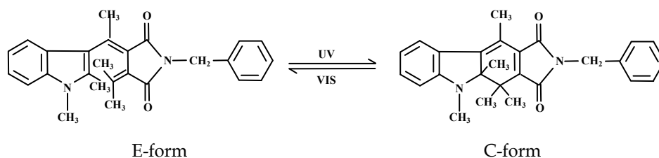
Fig. 9. Molecular formula of the Indolyfulgimide and the photochromic reaction. Left, E-form; right, C-form
