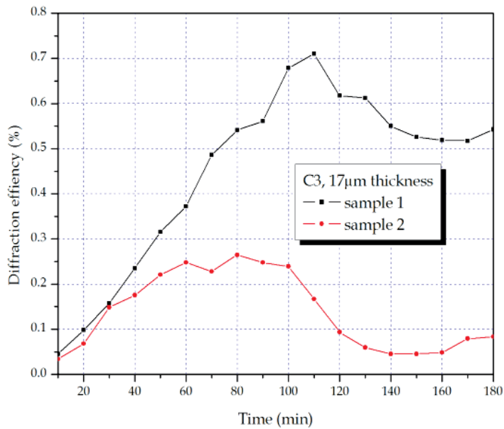
Fig. 17. (a). Plot of the Diffraction efficiency to certain temperature during the recording process.
