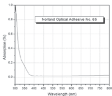
Fig. 1. Absorption spectra of NOA 65 in region UV-Vis.
