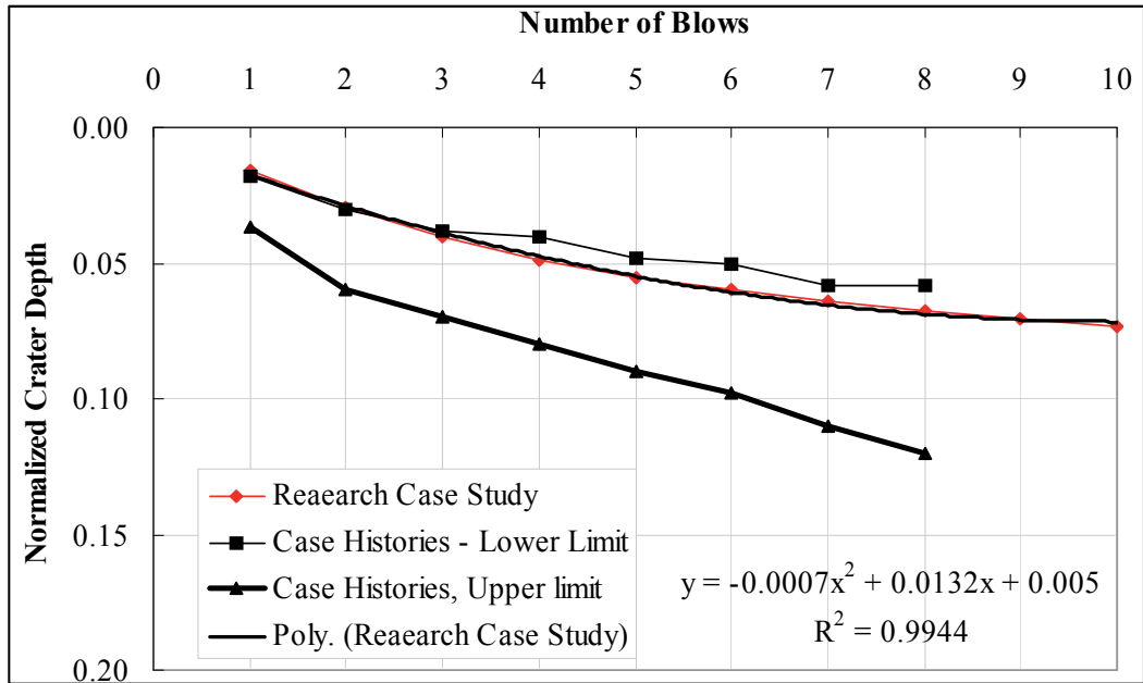
Fig. 18. Comparison of Normalized Crater Depths Vs No. of Drops with the Range proposed by Mayne et al., (1984)
