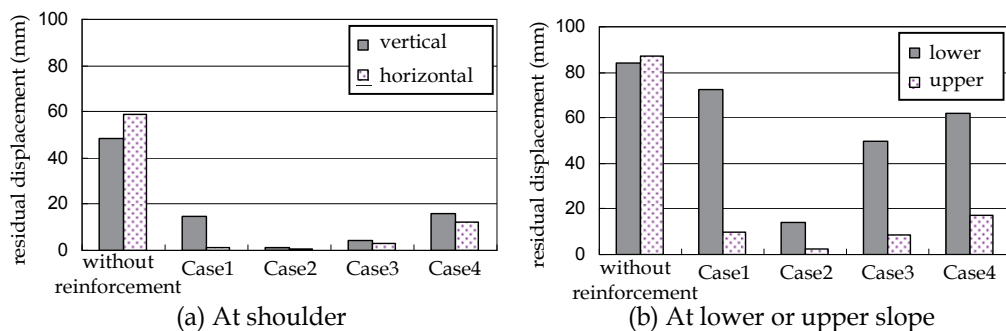
Fig. 15. Comparison of Residual Displacement
