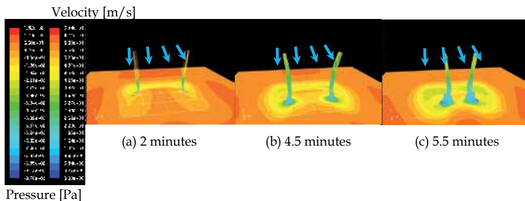
Fig. 21. Pressure field at the bottom surface and streamline distributions since the introduction of horizontal wind in Model 3
