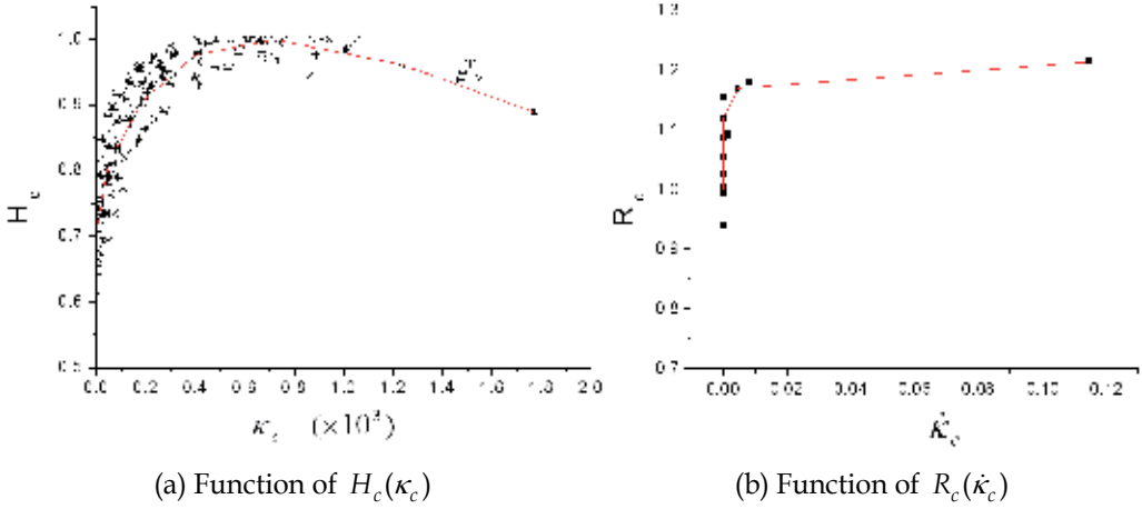
Fig. 10. Function of H_c(\kappa_c) and R_c(\dot{\kappa}_c)
