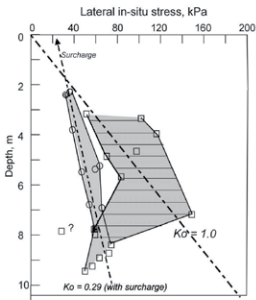
Fig. 9. Tests in loose sand at the San Francisco Naval Shipyard the slope of the lateral stress line gives K_o = 0.29 prior to pile driving, indicating a potential for liquefaction. As in the case of DDC, pile driving increased the average K_o to 1.0, indicating temporary liquefaction down to the bottoms of the piles. Data are from Handy et al. (1990)
