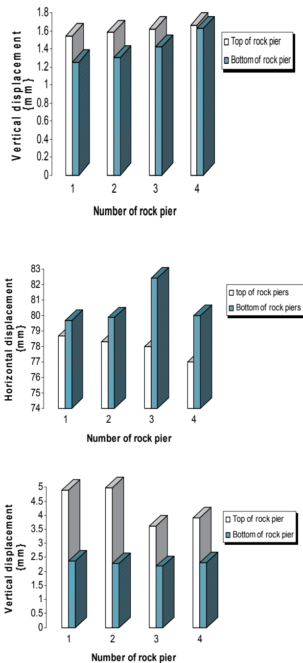
Fig. 10. Differential horizontal and vertical displacements on the top and base of the rock piers in the catacomb complex (a) Kalamata at time (t) = 4.60 sec, (b) Erzincan at (t) = 7.09 sec, (c) Aqaba at time (t) = 23.22 sec. PGA = 0.24g.
