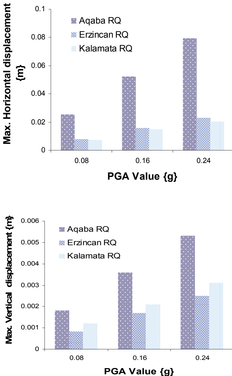
Fig. 12. (a) Maximum horizontal displacements, (b) Maximum vertical displacements on the top of Catacombs, for Aqaba, Erzincan, and Kalamata earthquakes, scaled to several values of PGA.
