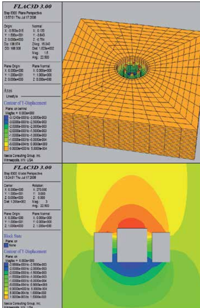
Fig. 5. Results from the 3D analysis indicating that the maximum ground displacements above the rotunda are relatively small (of the order of 2.6 mm), and the maximum horizontal displacement is about 1 mm.
