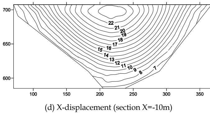
Fig. 9. Distribution of maximum displacement response (mm)
