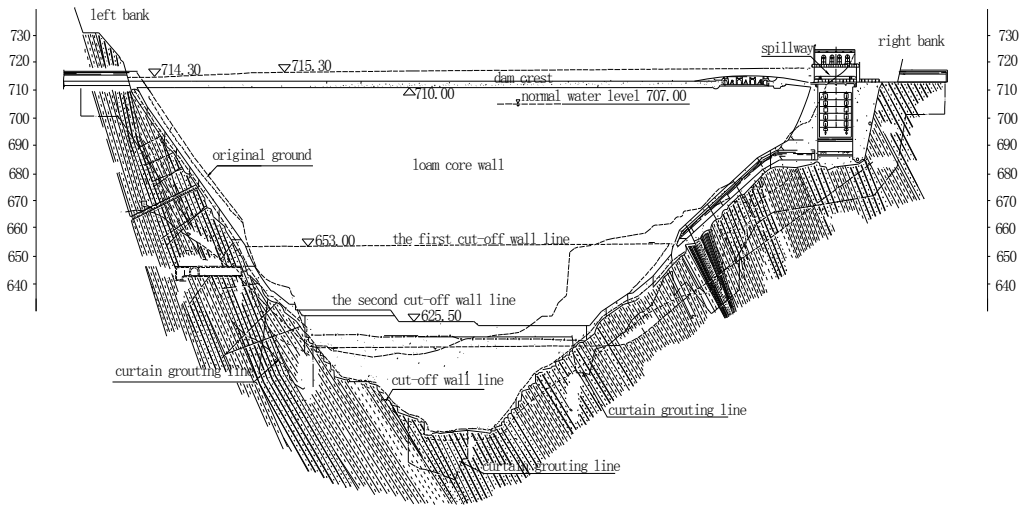
Fig. 2. Section of the dam along the dam axis
