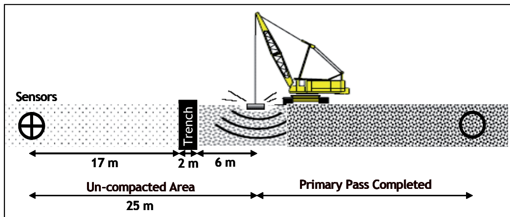
Fig. 22. Layout of Vibration Measurement Points at 25 m Distance
