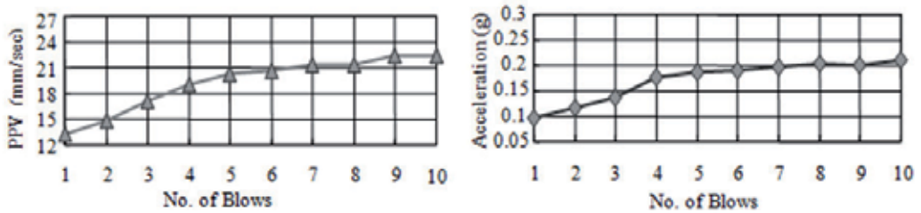
Fig. 26. Accelerograms for successive blows
