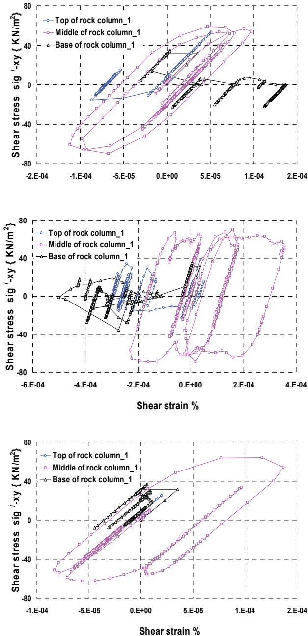
Fig. 11. Deformed meshes, vertical displacement-time history, shear stresses-shear strain, (a) Kalamata , (b) Erzincan , and (c) Aqaba earthquakes. Input motion PGA = 0.24g. Catacombs of Kom El-Shoqafa, a typical cross section 2, second floor, the royal tomb.
