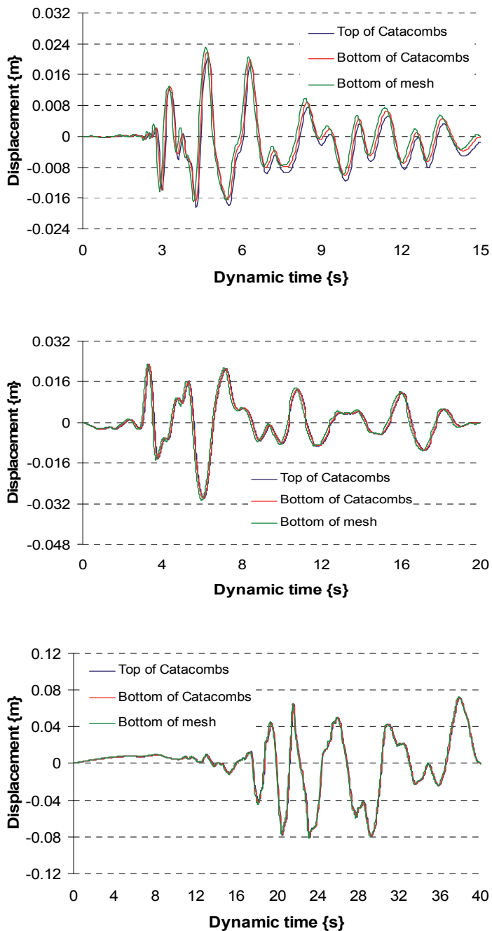
Fig. 7. Deformed meshes and peak total displacement, and acceleration, horizontal displacements-time histories, (a) Kalamata , (b) Erzincan , and (c) Aqaba earthquakes. Input motion PGA = 0.24g. Catacombs of Kom EL-Shoqafa, a typical cross section 1, first floor.
