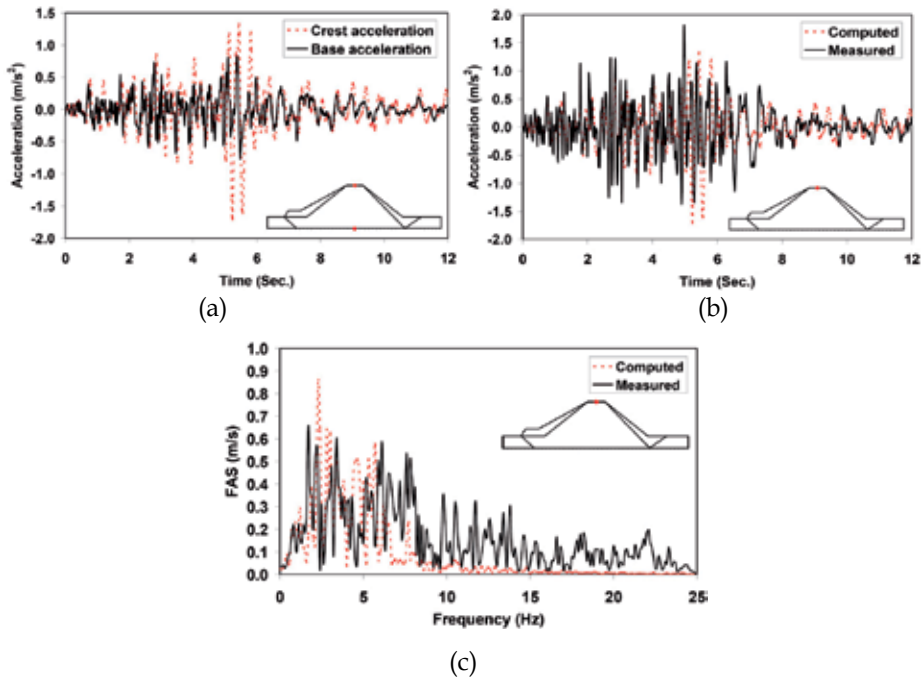
Fig. 14. Comparing computed and measured time histories in vertical direction: (a) crest and base acceleration, (b) crest acceleration, and (c) Fourier amplitude spectrum
