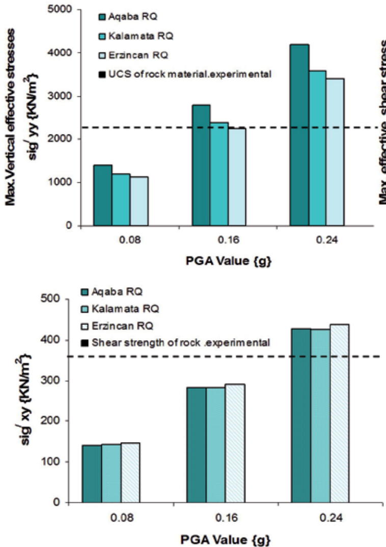
Fig. 13. (a) Maximum vertical effective compressive stresses \sigma_{yy} , (b) Maximum effective shear stresses \sigma_{xy} on the base of rock pier_1, for Aqaba, Erzincan, and Kalamata earthquakes, scaled to several values of PGA.
