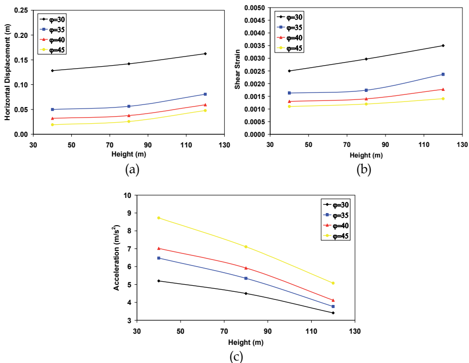
Fig. 18. Computed values of: (a) permanent horizontal displacements, (b) permanent shear strains, and (c) induced maximum accelerations at dam crest versus dam height for different friction angles of shell materials
