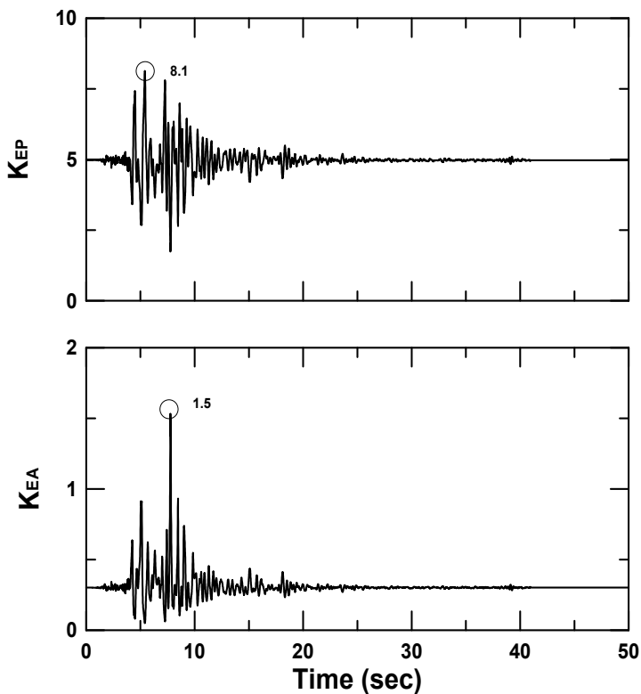
Fig. 16. Dynamic coefficients of earth pressure
