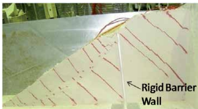
Photo 14. Centrifuge test on the Barrier Reinforcement Structure
