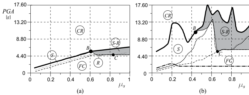
Fig. 15. Seismic analysis under Brienza earthquake, PGA vs static friction coefficient \mu_s : (a) no security stops; (b) base and sliding stops; ( \lambda = 1 , \varepsilon = 0.35 , T = 2s ).
