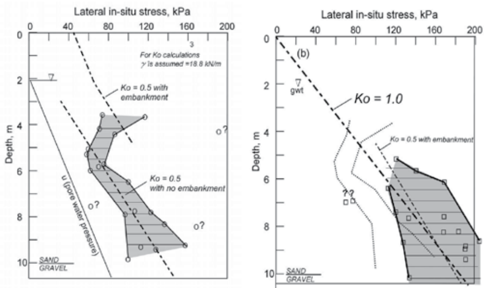
Fig. 8. Lateral stresses measured in foundation sand at the Jackson Lake dam site, (left) before and (right) after compaction. At the left, the soil was normally consolidated until after the embankment was built, when the weight of the dam compacted the upper part but left the lower soil underconsolidated and potentially liquefiable. At the right, compaction increased the average K_0 to 1.0, indicating a history of induced liquefaction, and K_0 = 0.5 after the dam was replaced. From Handy (2012), modified from Handy et al. (1990).
