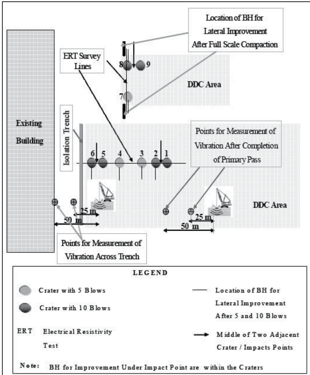
Fig. 5. Layout of Compaction Site, Test Craters, Vibration Measurement Points and Location of ERT Survey
