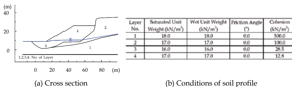
Fig. 18. Analytical model of in-situ field shown in Fig. 16
