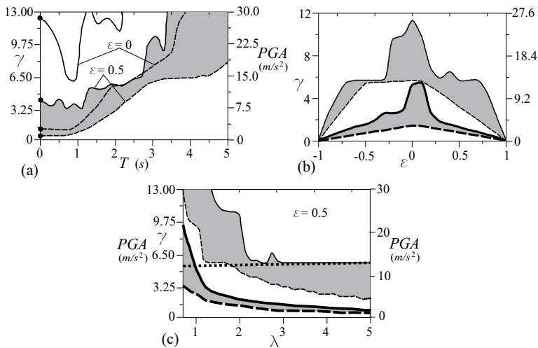
Fig. 9. Seismic analysis under Buia earthquake: (a) Seismic scale factor versus period T ( \lambda = 3 ); (b) Seismic scale factor versus eccentricity \varepsilon ( \lambda = 3 , T = 2s ); (c) Seismic scale factor versus slenderness \lambda ( T = 2s ); ( b = 0.3m , \rho = 2000kg / m^3 , \xi = 0.20 ).
