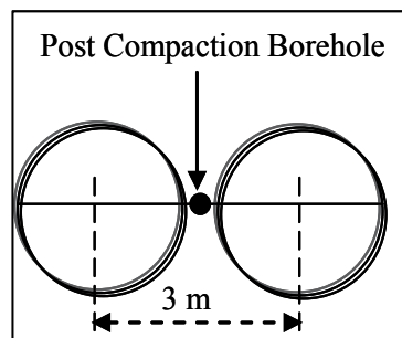
Fig. 8. Location of boreholes for evaluation of improvement at the middle of adjacent craters
