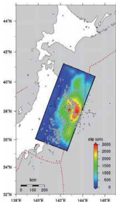
Fig. 31. Fault Plane Slip Distribution Tohoku-Oki, Japan. http://tectonics.caltech.edu/slip_history/2011_taiheiyo-oki/index.html
