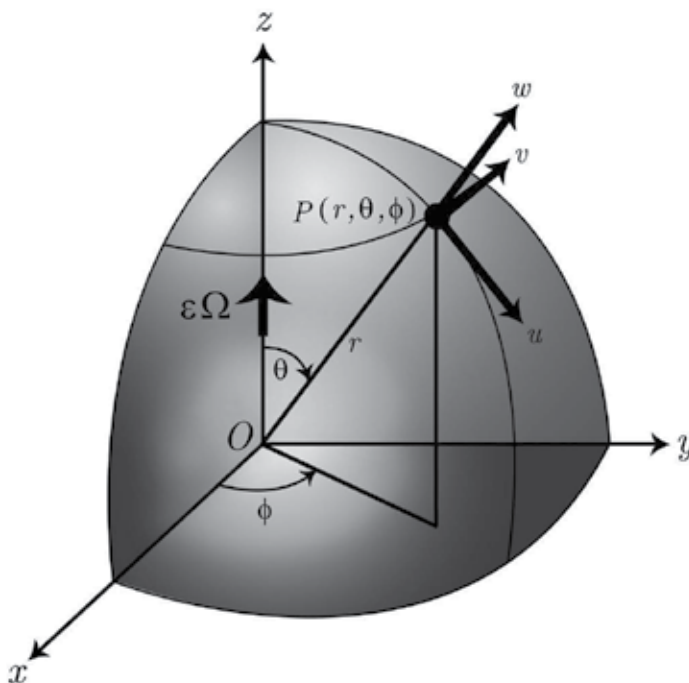
Fig. 1. The spherical coordinate system Or\theta\phi and its relation to the reference frame Oxyz that is rotating slowly about the z -axis at rate \epsilon\Omega , showing a particle in the i^{th} layer with position of rest P(r, \theta, \phi) and displacement from the position of rest u in the direction of increasing angle \theta , v in the direction of increasing angle \phi and w in the radial direction.
