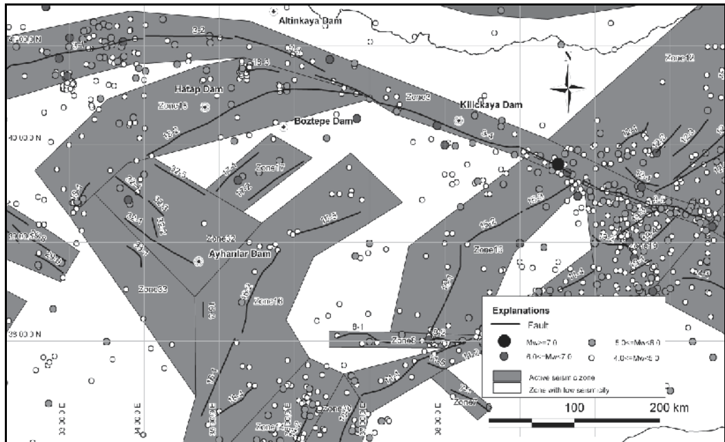
Fig. 4. Locations of dams on seismo-tectonic map
