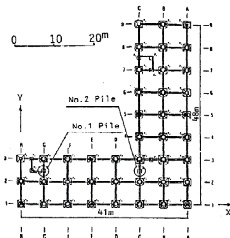
Fig. 8. Footing and foundation beams of Niigata Family Court House (from Hamada, 1992)
