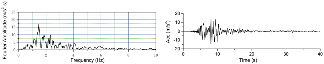
Fig. 5. Fourier amplitude and time history of the foundation input motion.
