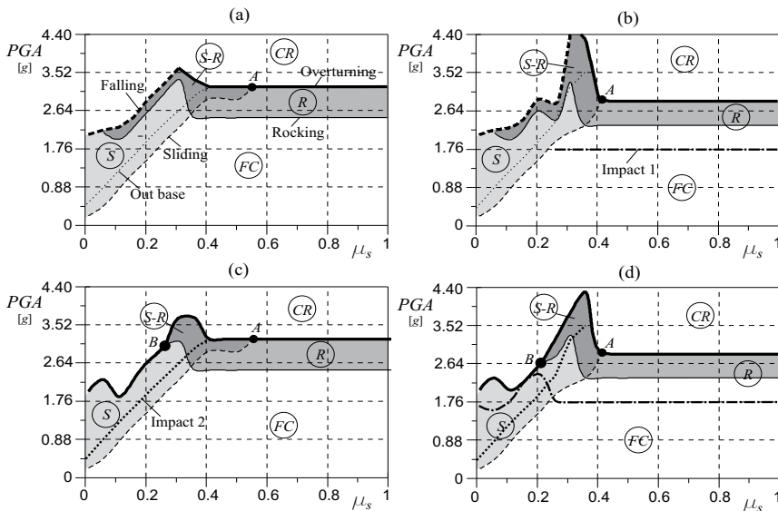
Fig. 12. Seismic analysis under Brienza earthquake: (a) PGA versus static friction coefficient \mu_s - no security stops; (b) PGA versus static friction coefficient \mu_s - only base stops; (c) PGA versus static friction coefficient \mu_s - only sliding stops; (d) PGA versus static friction coefficient \mu_s - both base and sliding stops; ( \lambda = 3 , \varepsilon = 0 , T = 2s ).
