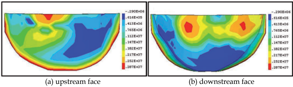
Fig. 22. Distribution of the first principle stresses (model III), MPa
