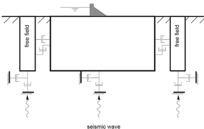
Fig. 3. Free field boundaries in dynamic analysis (Itasca, 2004)
