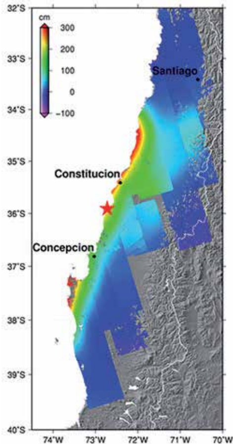
Fig. 21. Fault Plan Slip Distribution over land area - Maule, Chile. http://tectonics.caltech.edu/sliphistory/2010_chile/index.html
