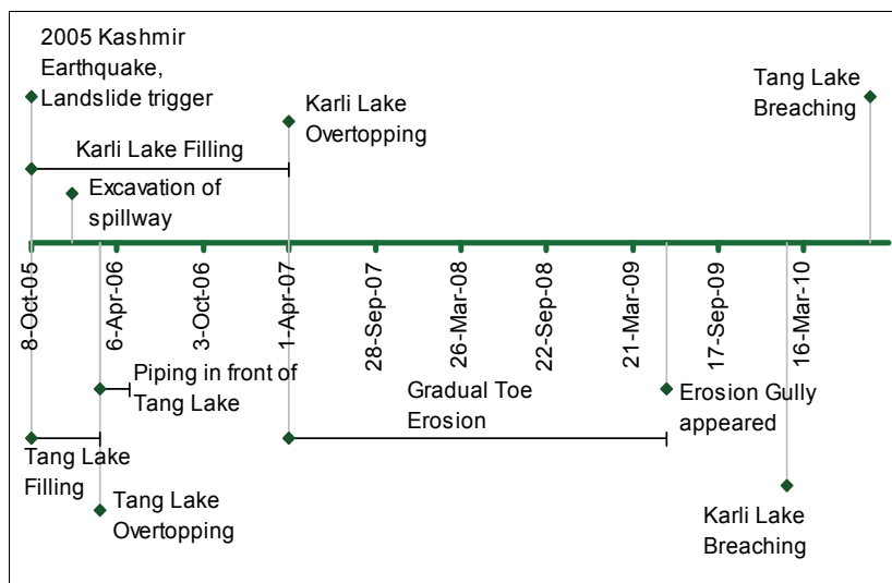
Fig. 8. Timeline of post formation features and major events at Hattian Bala landslide dam
