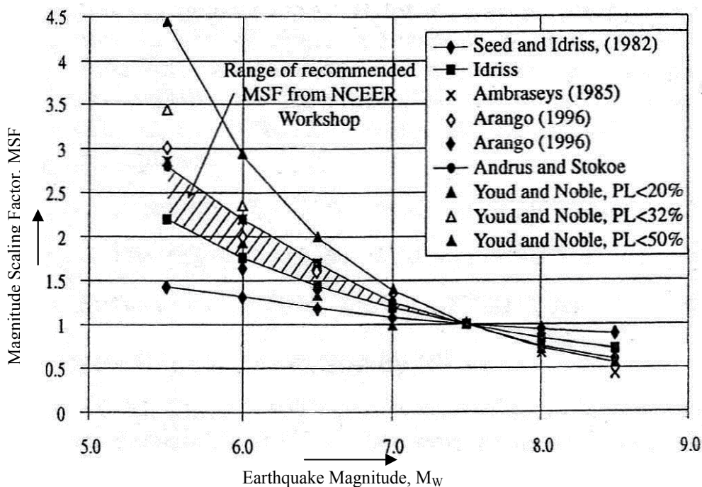
Fig. 4. Magnitude Scaling Factor Derived by Various Investigations (Youd et al., 2001)
