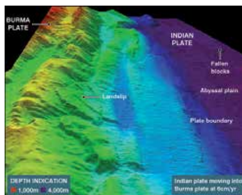
Fig. 2. Three-Dimensional Sonar Imagery of Seabed off the coast of Sumatra Island. (BBC 2005)
