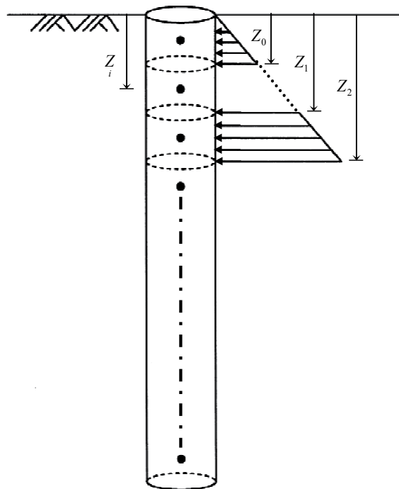
Fig. 6. Distribution of earth pressure along a pile
