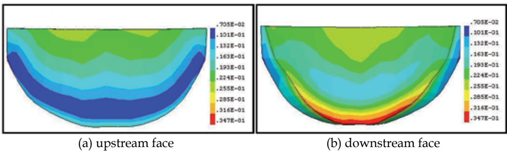
Fig. 24. Distribution of the equivalent strain rate (model I, II, and III), s^{-1}
