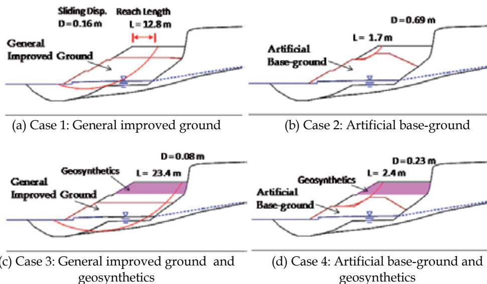
Fig. 19. Sliding characteristics according to reinforcement structures
