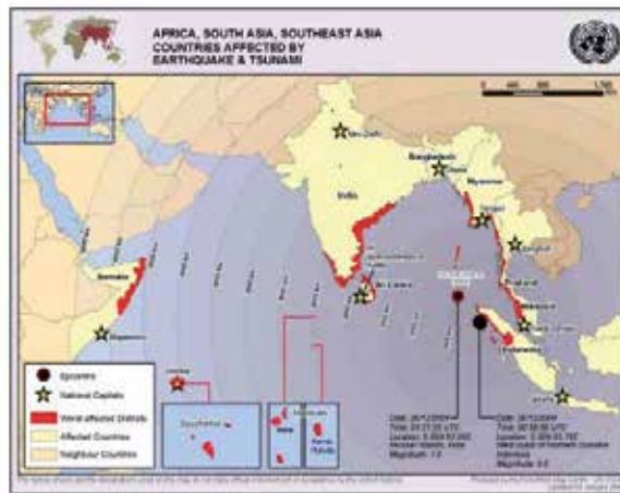
Fig. 4. Tsunami-Damaged Countries Around Indian Ocean, 2004. (UN OCHA 2005)
