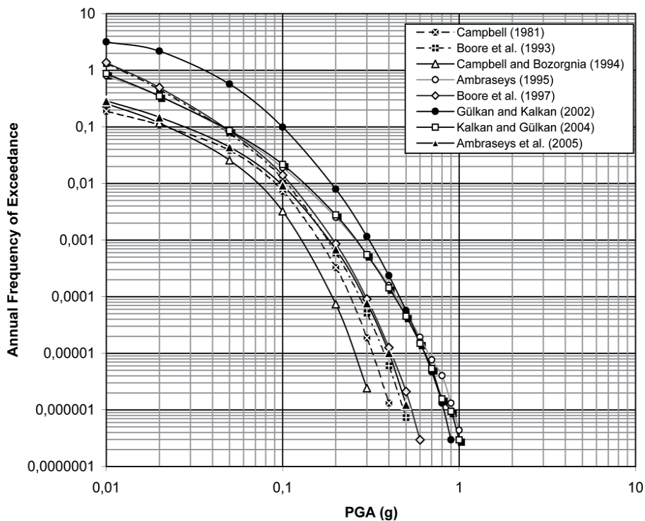
Fig. 6. Seismic hazard curve for Altinkaya dam site
