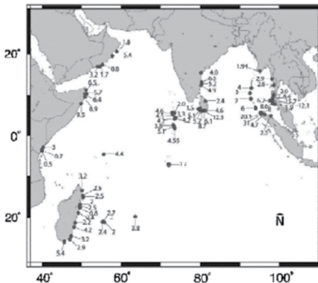
Fig. 5. Representative Tsunami Runup Heights along Shores of Indian Ocean, 2004. (EERI 2006)
