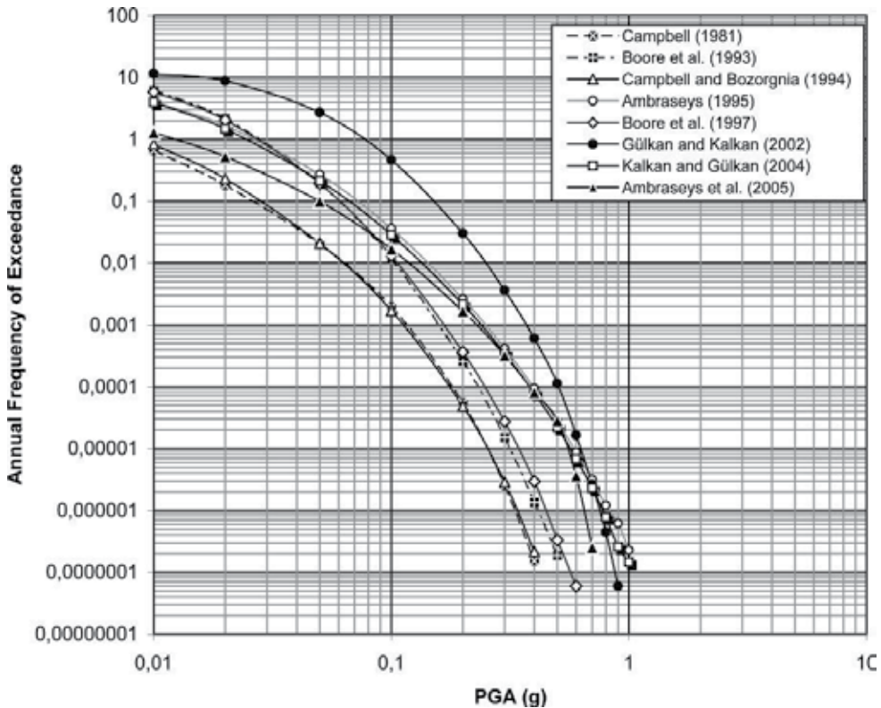
Fig. 14. Seismic hazard curve for Boztepe dam site
