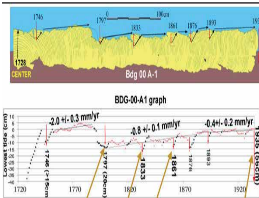
Fig. 35. Sea Level Changes Inferred from Truncated Coral Growth Rings. (Caltech 2011) http://www.tectonics.caltech.edu/images/sumatra/coral_record_web.jpg
