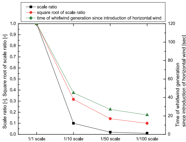
Fig. 17. Relation among scale ratio, square root of scale ratio, and time of whirlwind generation since introduction of horizontal wind in Model 1
