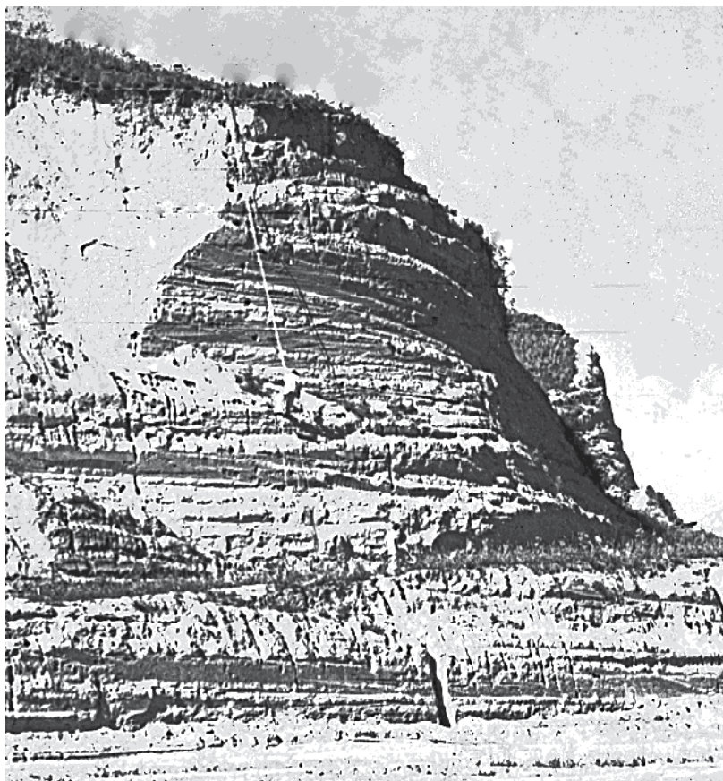
Fig. 12. Western Iowa loess deposits are thick close to the Missouri River floodplain, where glacial outwash was the major source of wind-blown silt. The author in his younger days is sampling about half-way down the cut slope.
