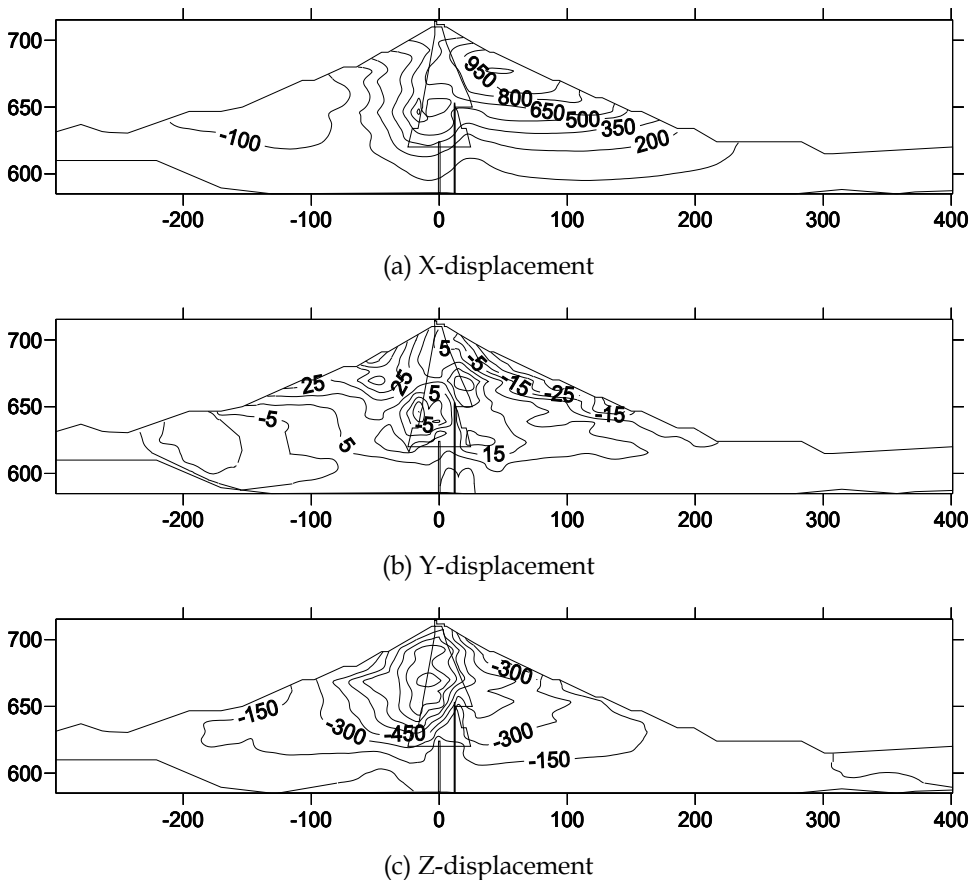
Fig. 4. Displacement distribution on section Y=210m (unit: mm)
