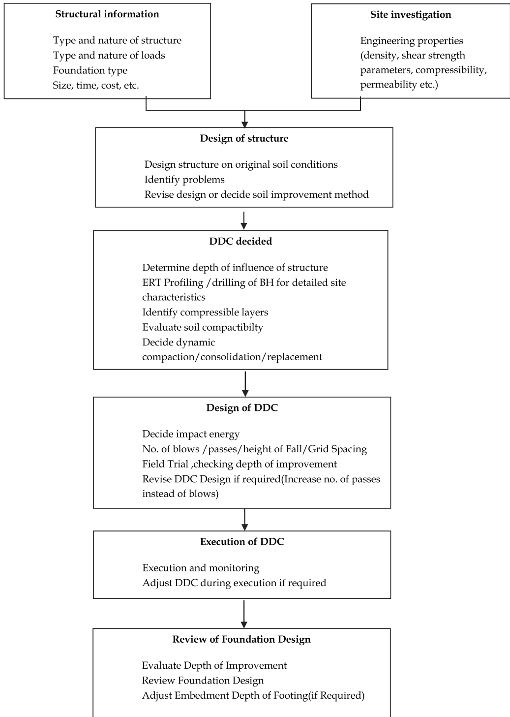
Fig. 28. Suggested Procedures for DDC Project
