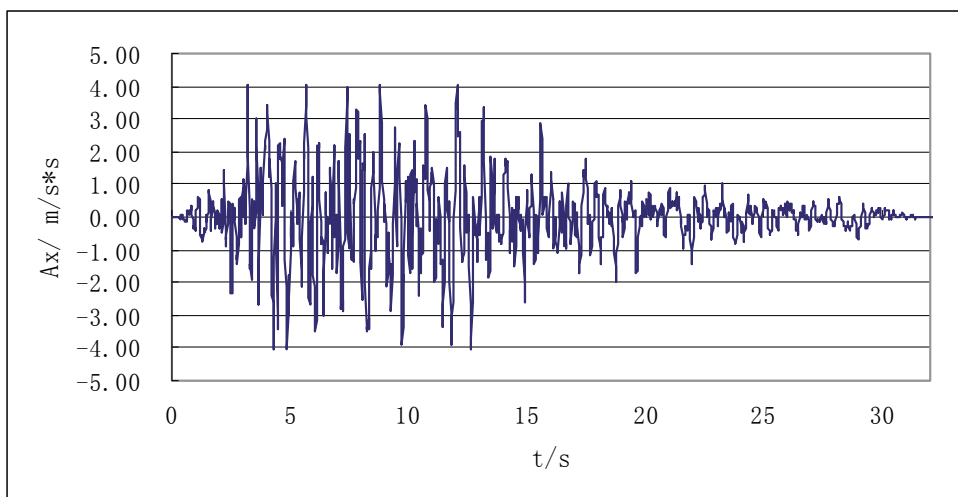
Fig. 7. The input curve of earthquake acceleration of bedrock in horizontal direction
