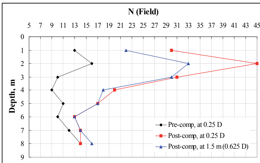
Fig. 12. Pre-to-post Compaction N (Field) Comparison of Improvement at Crater # 5 (Upper Half) and Middle of Crater # 5 and Crater # 6
