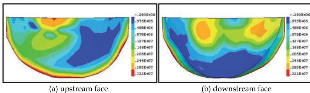
Fig. 21. Distribution of the first principle stresses (model II), Mpa
