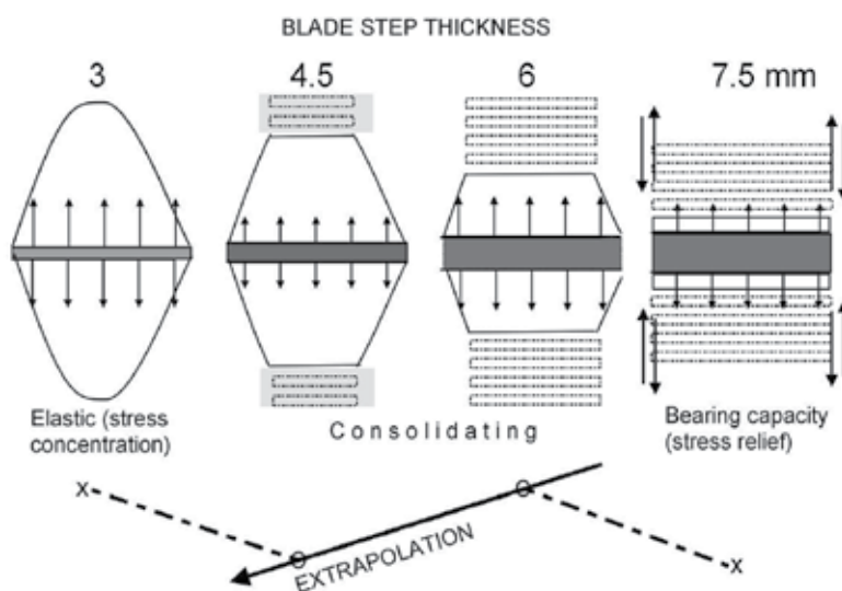
Fig. 3. Stress diagrams inferred from pressure measurements on different thickness steps, showing the critical role of consolidation and reasons for rejecting specific data points.
