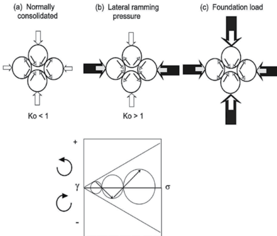
Fig. 11. Model illustrating how a high imposed lateral stress can reverse friction directions at grain contacts and increase the preconsolidation pressure without actually consolidating the soil. Modified from Handy (2001).
