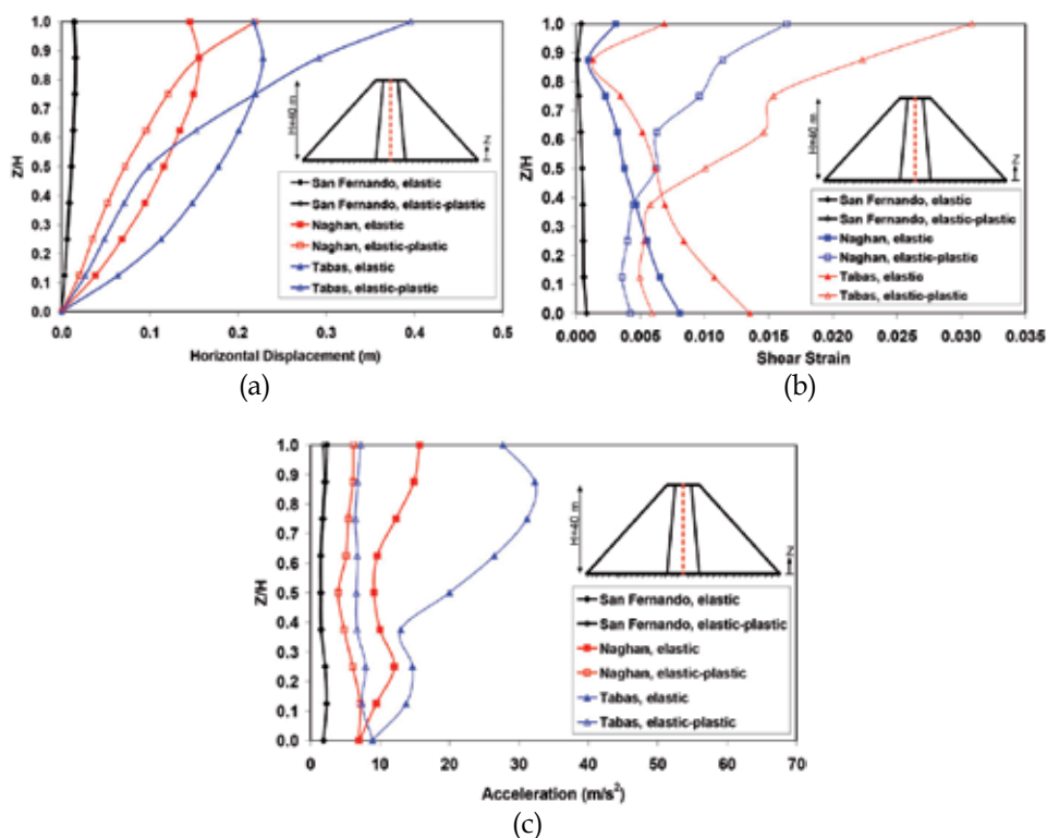
Fig. 17. Computed values of: (a) permanent horizontal displacements, (b) permanent shear strains, and (c) induced maximum accelerations along the dam height for elastic and elastic-plastic behaviours subjected to different earthquakes
