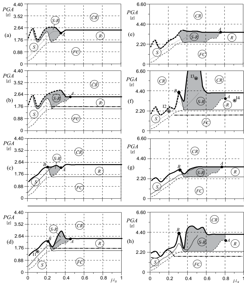
Fig. 13. Seismic analysis under Brienza earthquake: (a)-(d) PGA versus static friction coefficient \mu_s ( \lambda = 3 ); (a) no security stops; (b) only base stops; (c) only sliding stops; (d) both base and sliding stops. (e)-(h) PGA versus static friction coefficient \mu_s ( \lambda = 2 ); (e) no security stops; (f) only base stops; (g) only sliding stops; (h) both base and sliding stops; ( \varepsilon = 0.35 , T = 2s ).
