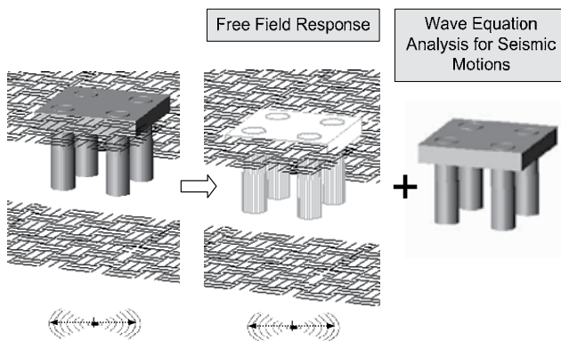
Fig. 2. Superposition of the free-field analysis and WEA
