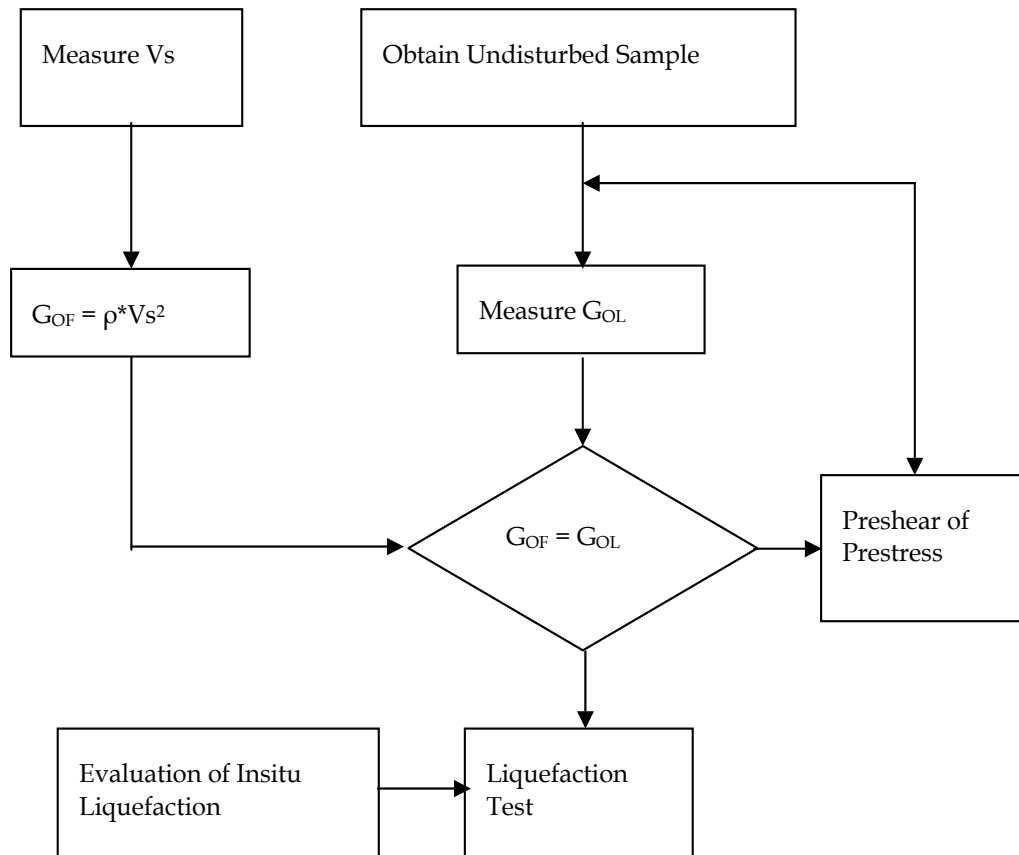
Fig. 3. Outline of Method (Tokimatsu et al., 1986)
