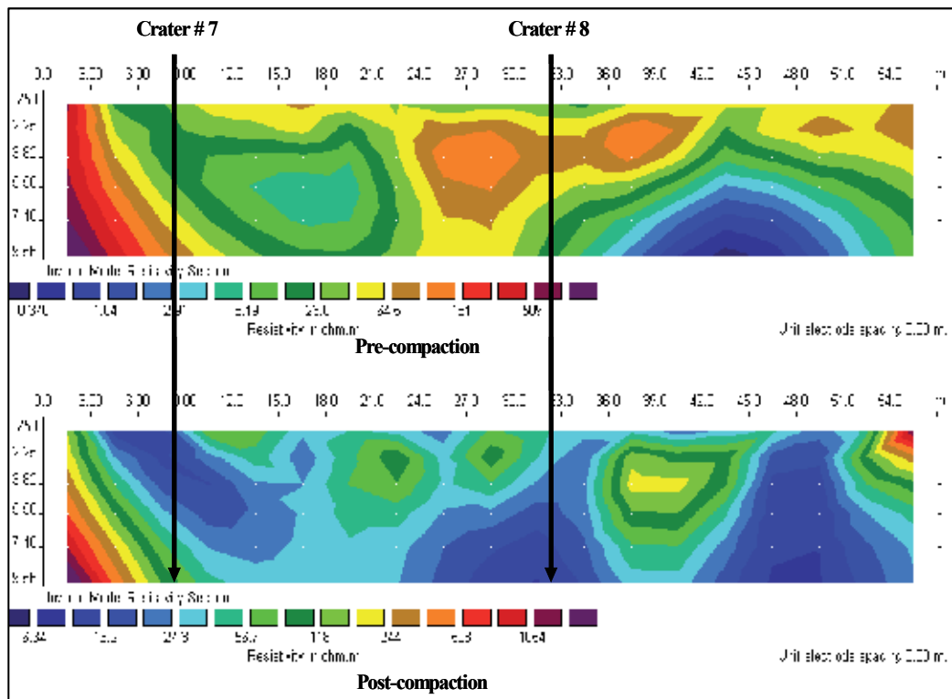
Fig. 21. ERT Profiles, Crater # 7 to Crater # 8
