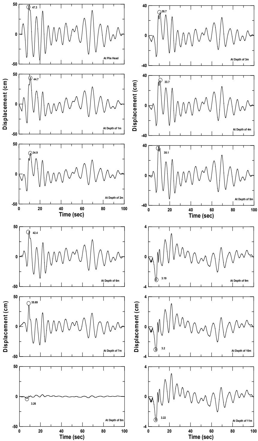
Fig. 12. Time histories of ground motions at different depths
