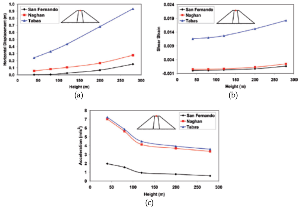
Fig. 15. Computed values of: (a) permanent horizontal displacements, (b) permanent shear strains, and (c) induced maximum accelerations at dam crest versus dam height for different earthquakes
