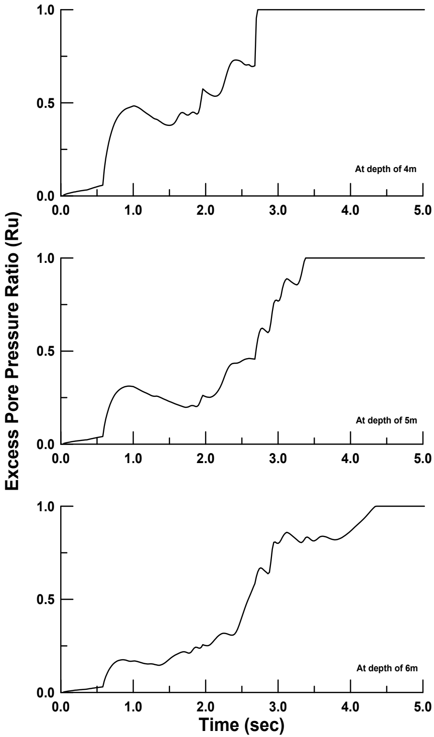
Fig. 11. The time history of excess pore pressure ratios at different depths
