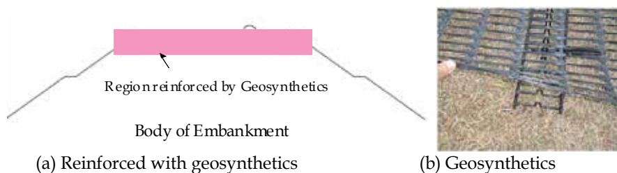
Fig. 8. Example of crest reinforcement structure
