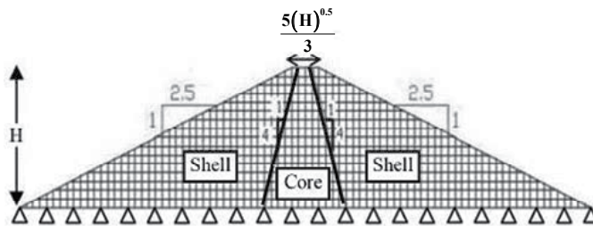
Fig. 2. Geometry of dam
