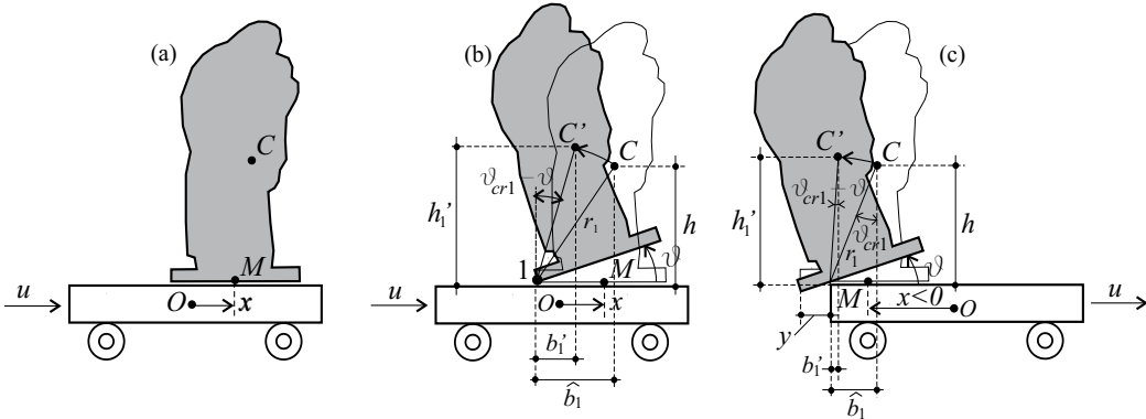
Fig. 3. Geometrical description of the different phases of motion: (a) sliding; (b) (slide-) rocking around corner 1; (c) (slide-)rocking where the left corner of the body is outside the oscillating base.
