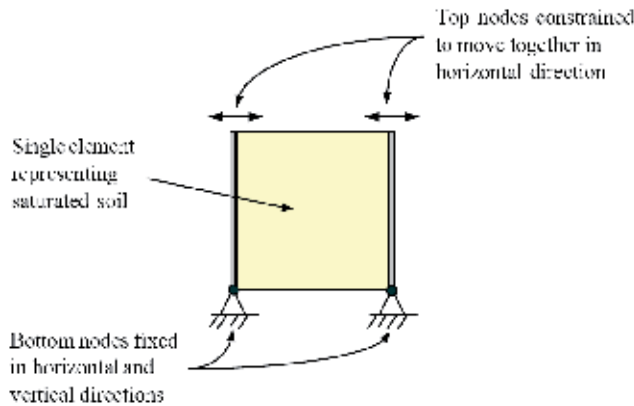
Fig. 8. One-zone model in FLAC for simulating cyclic simple shear test
