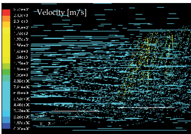
Fig. 8. Side view of streamlines after 26.6 minutes for the wind of 4m/s in Model 1
