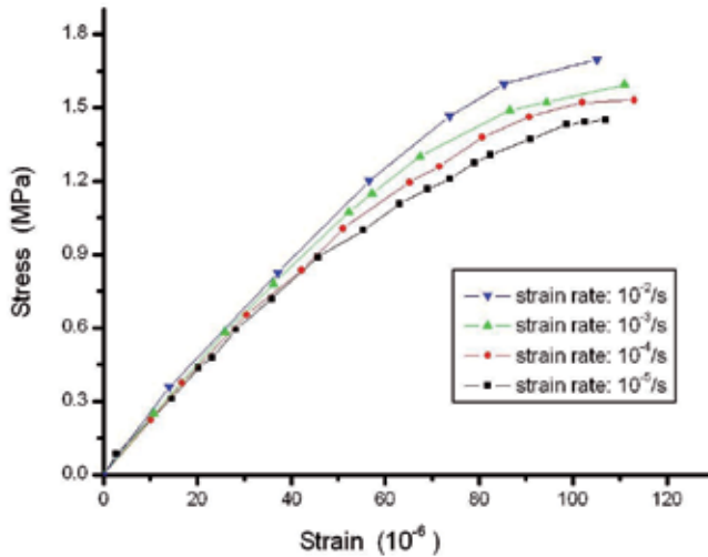
Fig. 4. The stress-strain curves of concrete in tension
