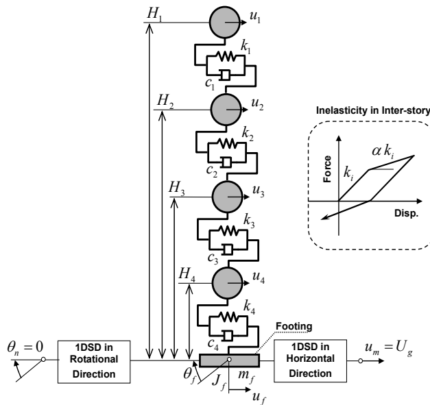
Fig. 7. Numerical model representing complete structural system.
