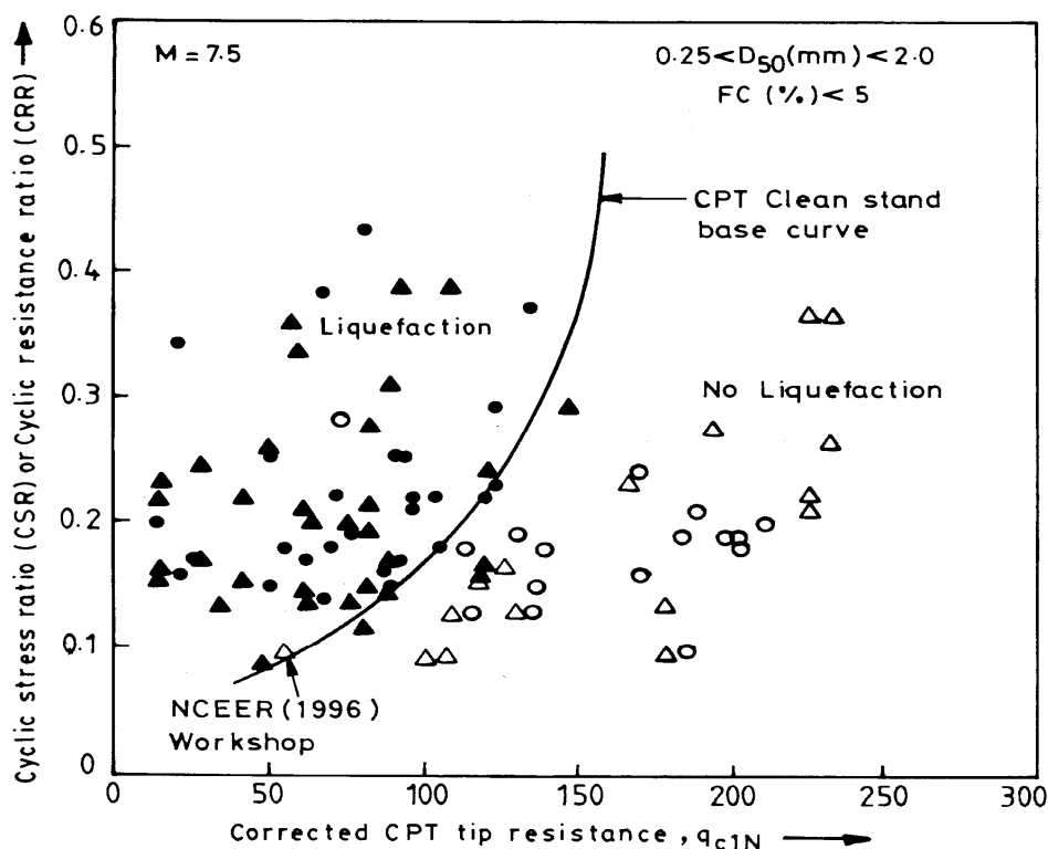
Fig. 2. Calculation of CRR from CPT q_{c1N} (Youd et al., 2001)
