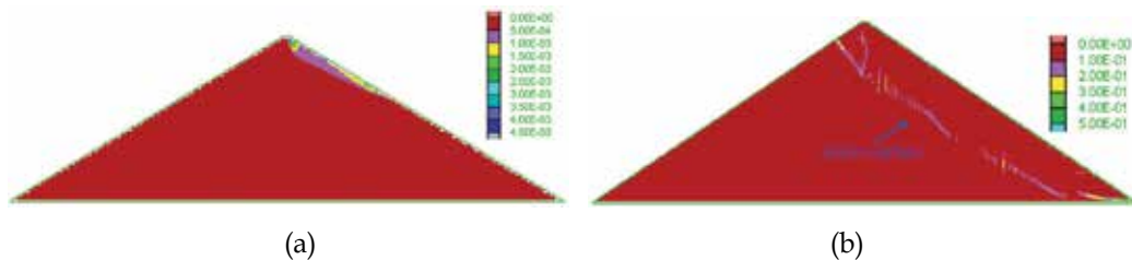
Fig. 16. Failure surface with shear strain contour in dam body at the end of Naghan earthquake: (a) dam height=120 m, and (b) dam height=280 m
