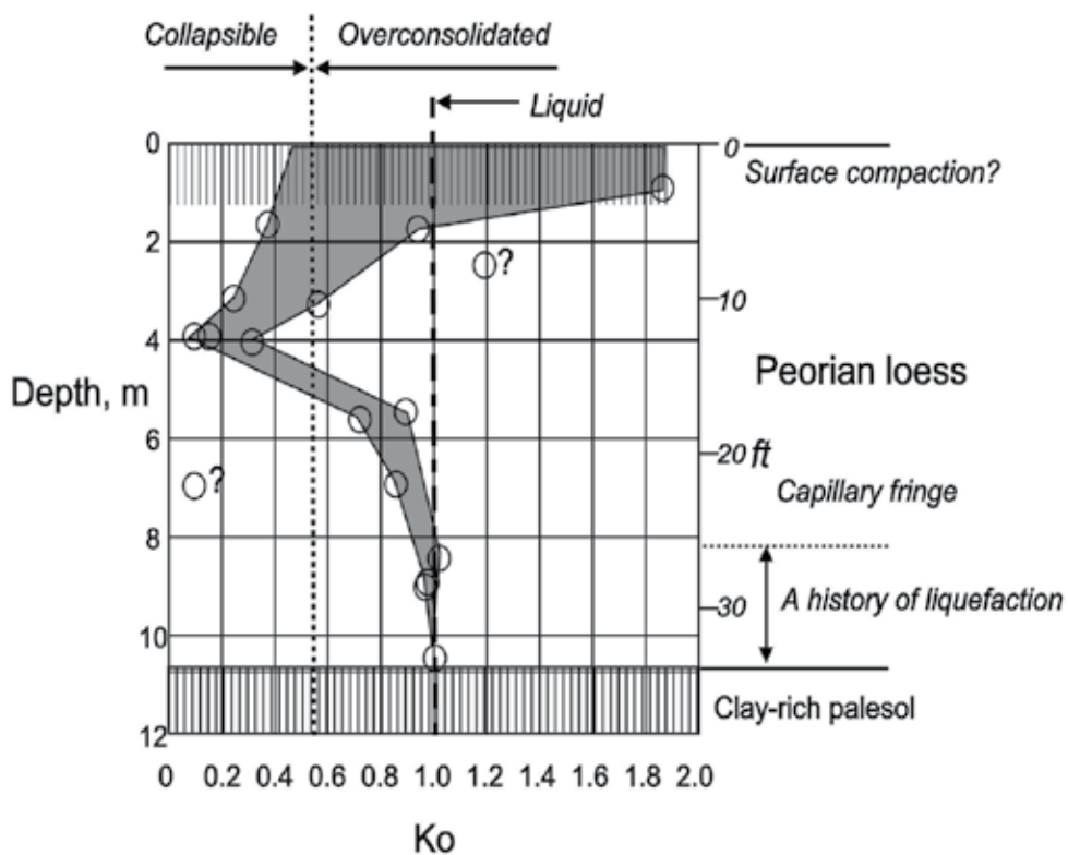
Fig. 13. K_0 Stepped Blade data from Nebraska loess about 17 km (11 miles) from the Missouri River floodplain source. From Handy (1994).
