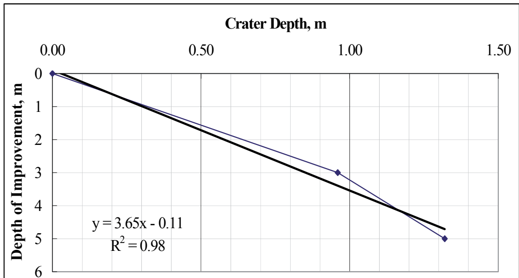
Fig. 19. Plot of Crater Depths vs. Depth of Improvement
