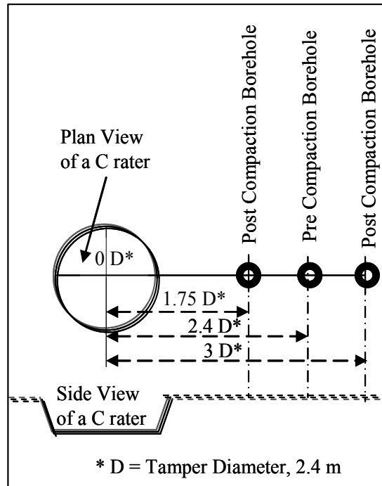
Fig. 7. Location of boreholes for evaluation of improvement in lateral direction
