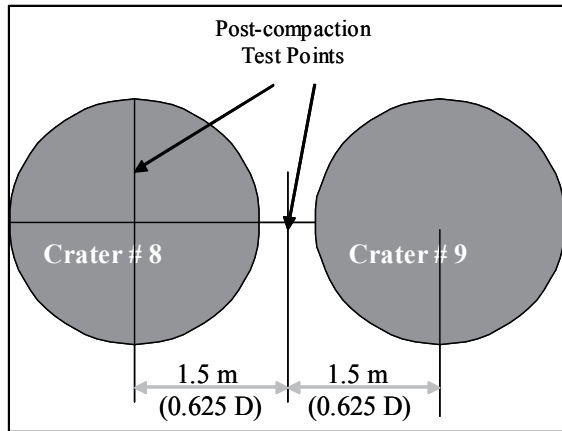
Fig. 13. Layout of BH for Evaluation of Improvement after Full scale Compaction at Crater # 8 (Upper Half) and Middle of Crater # 8 and Crater # 9
