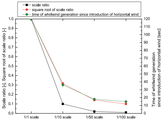
Fig. 24. Relation among scale ratio, square root of scale ratio, and time of whirlwind generation since introduction of horizontal wind in Model 3
