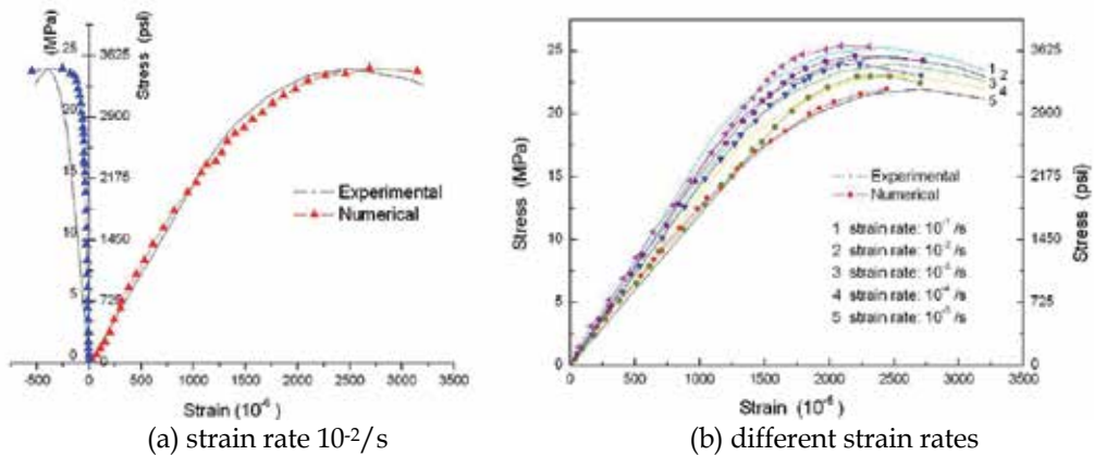
Fig. 12. Model and compressive test results
