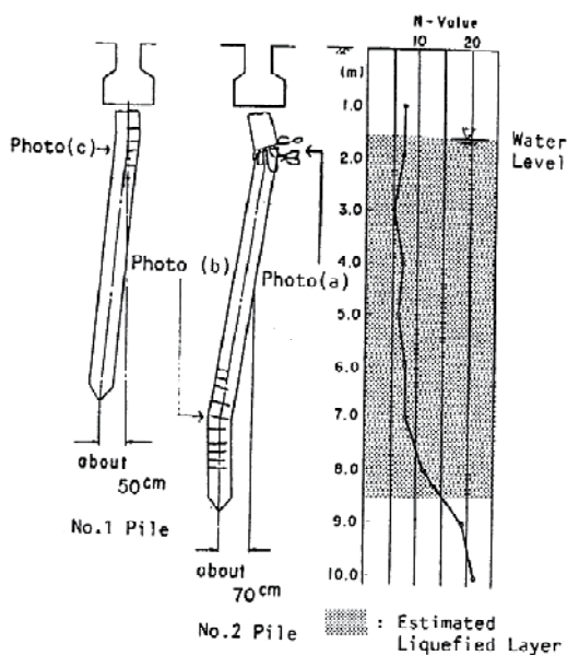
Fig. 9. Damage to piles and SPT-N values in situ (from Hamada, 1992)
