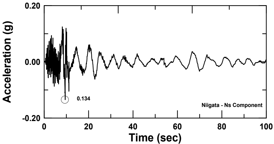
Fig. 10. Time history of Niigata Earthquake (NS Component)
