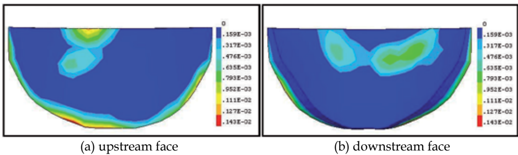
Fig. 28. Distribution of the equivalent viscoplastic strain
