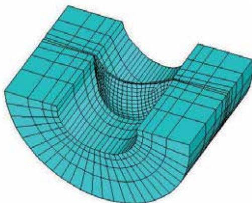
Fig. 17. Geometry and mesh of arch dam
