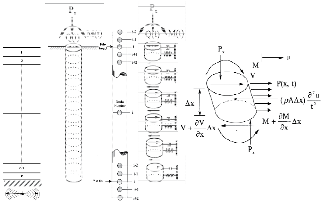
Fig. 1. Discrete system of the single pile
