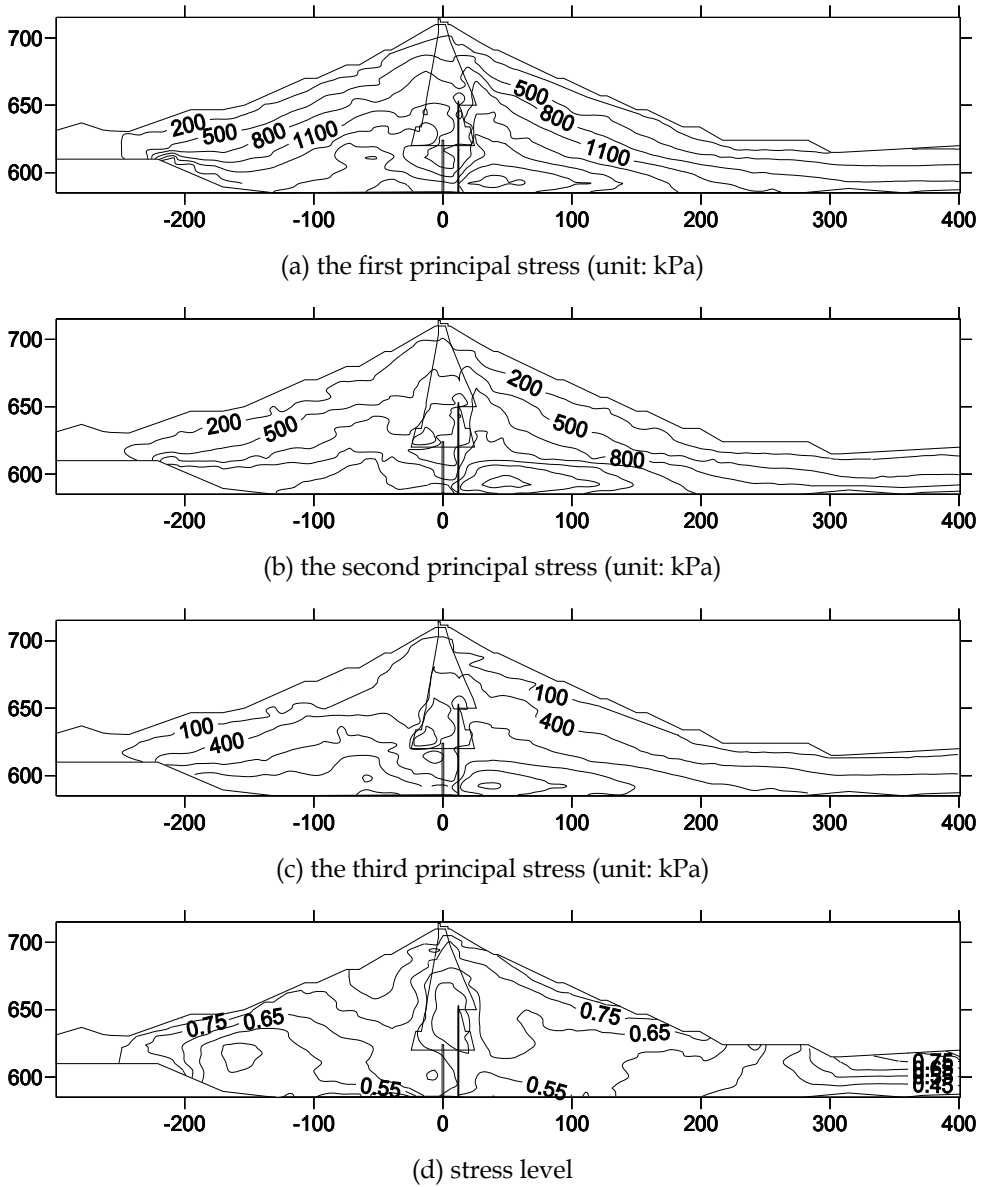
Fig. 5. Stress distribution on section Y=210m
