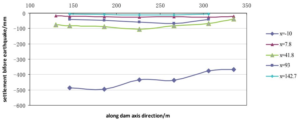
Fig. 17. Distribution of settlement measured value before the earthquake
