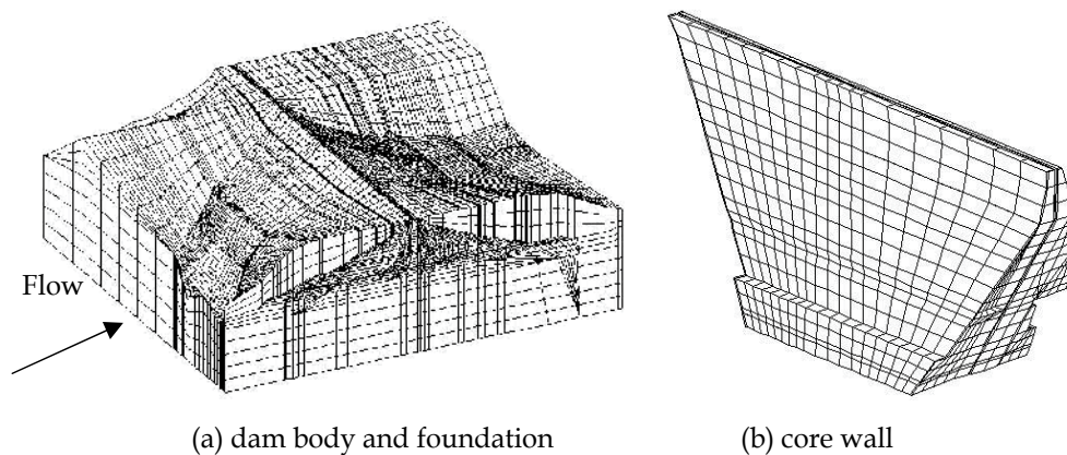
Fig. 3. Finite element grid
