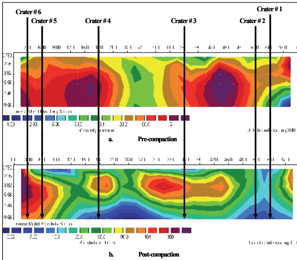
Fig. 20. ERT Profiles, Crater # 1 to Crater # 6
