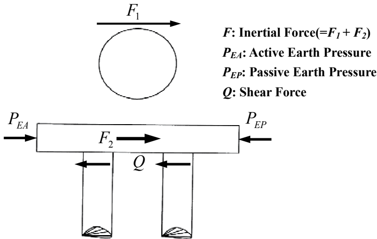
Fig. 5. Schematic layout of forces acting on Foundation (from Uchida and Tokimatsu, 2005)
