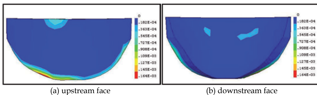
Fig. 25. Distribution of the equivalent viscoplastic strain (model II)
