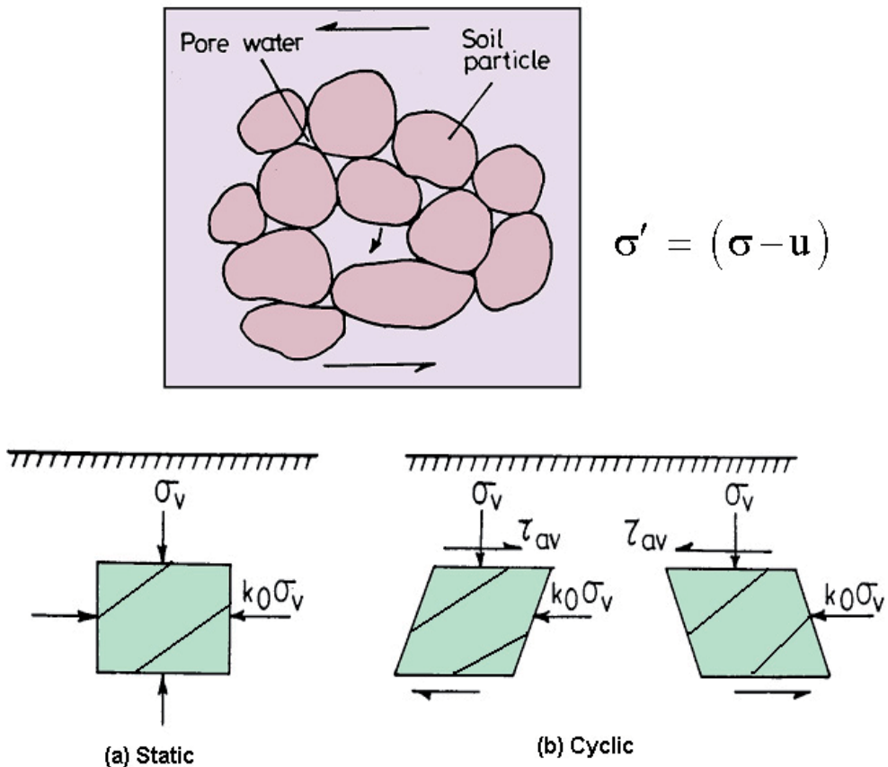
Fig. 1. Mechanism of Soil Liquefaction
