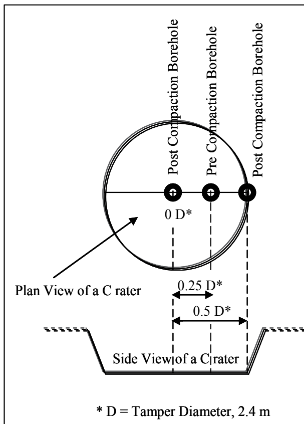
Fig. 6. Location of boreholes for evaluation of improvement under impact point
