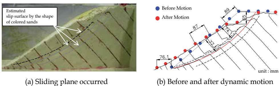
Fig. 12. Sliding failure in case of non-reinforced model
