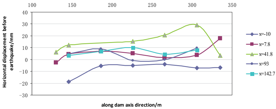
Fig. 16. Distribution of horizontal displacement measured value before the earthquake
