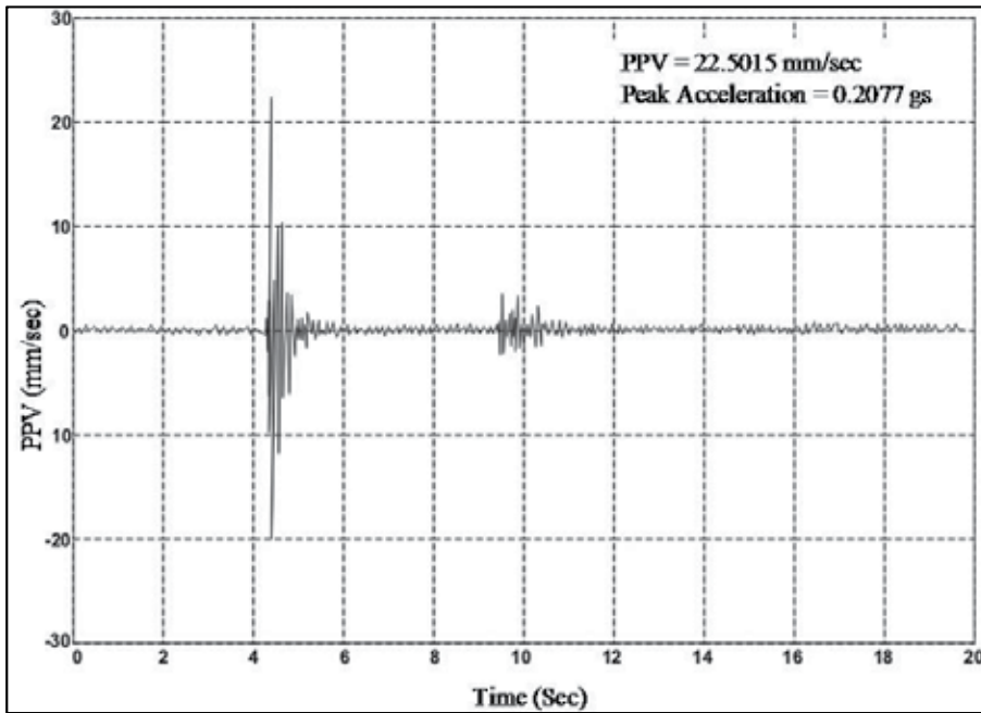
Fig. 27. Accelrogram of PPV at 10th blow
