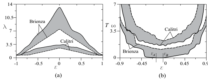
Fig. 10. Comparison between normalized Brienza and Calitri earthquakes (PGA=g): (a) slenderness \lambda versus eccentricity \varepsilon ( b = 0.3m , \lambda = 3 , T = 2s ) and (b) period T versus eccentricity \varepsilon ( b = 0.3m , \lambda = 3 , \rho = 2000kg/m^3 , \xi = 0.20 ).
