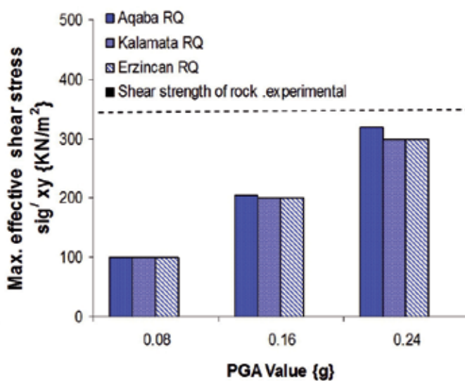
Fig. 16. Maximum effective shear stresses \sigma'_{xy} on the base of rock pier_1, (a) Initial model (b) After the installation of polymer anti-seismic piling. For Aqaba, Erzincan, and Kalamata earthquakes, scaled to several values of PGA.
