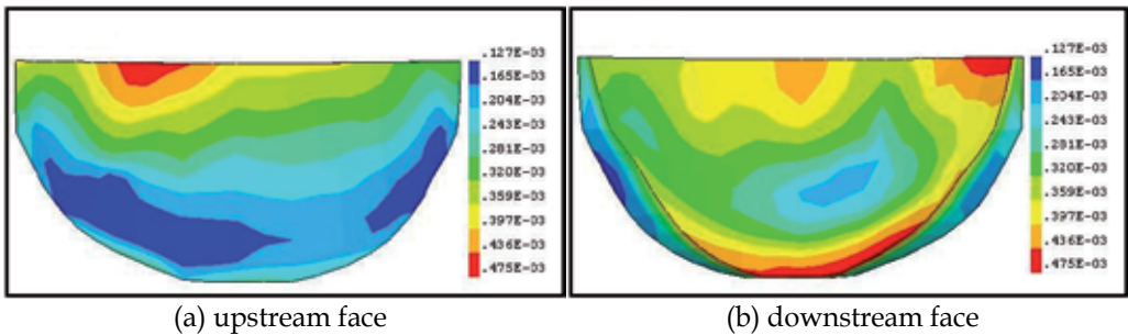
Fig. 23. Distribution of the equivalent strain (model I, II, and III)
