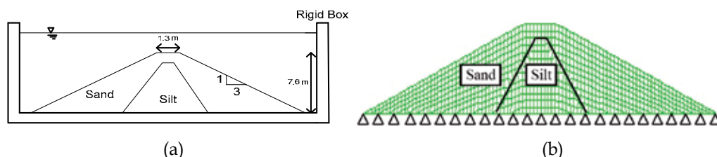
Fig. 10. Model configuration: (a) schematic sketch of dam in centrifuge container box, and (b) numerical grid constructed in FLAC
