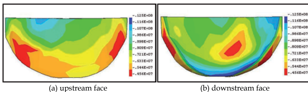
Fig. 19. Distribution of the third principle stress (model I, II, and III), Mpa
