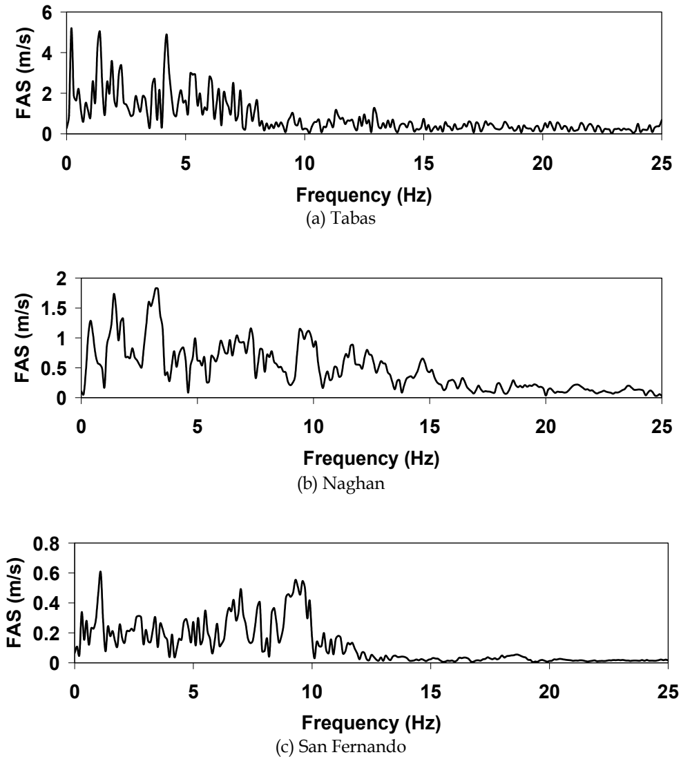
Fig. 6. Fourier amplitude spectra
