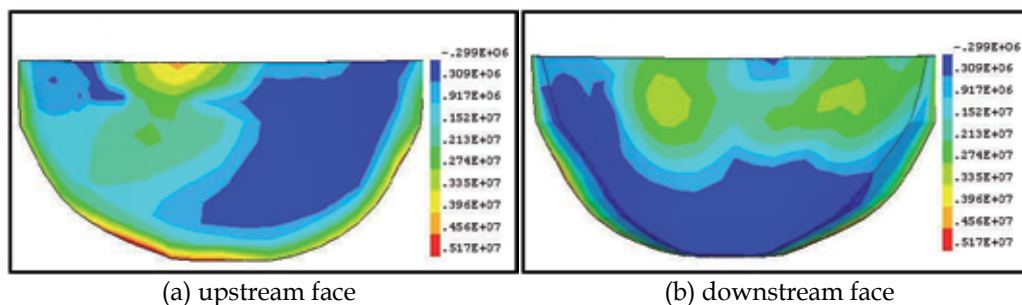
Fig. 20. Distribution of the first principle stress (model I), Mpa
