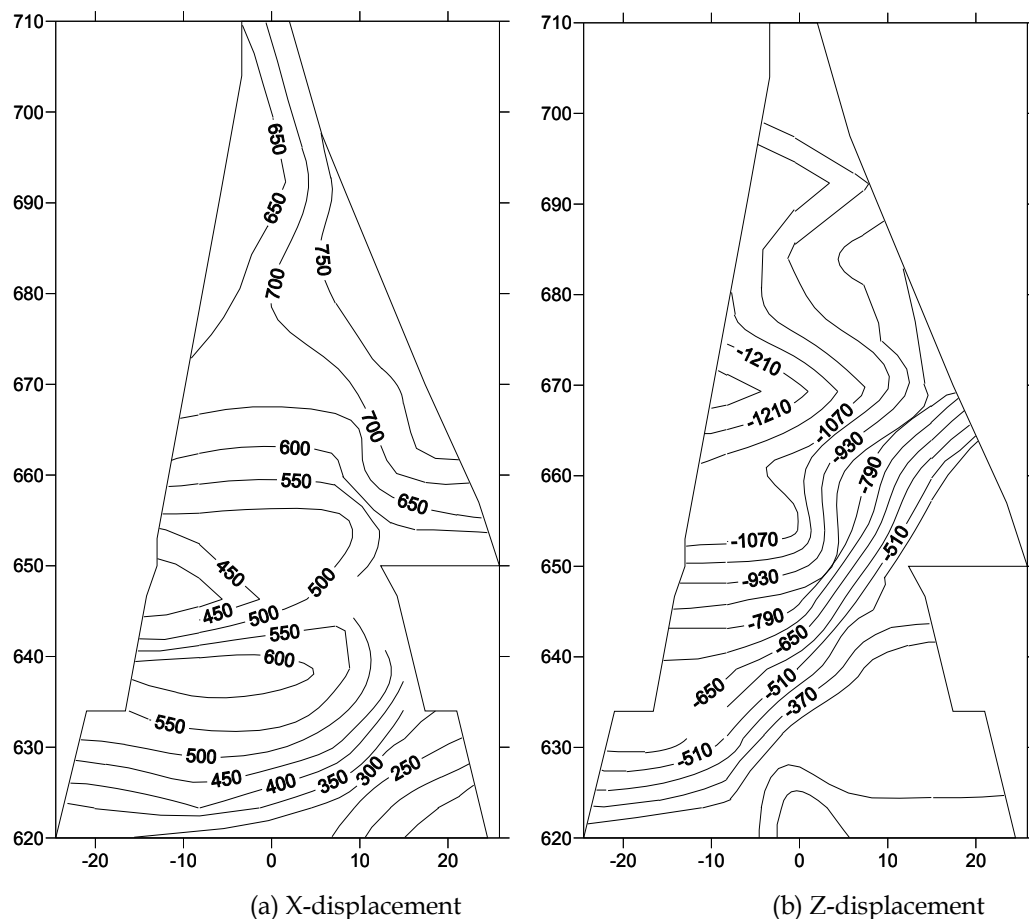
Fig. 6. Displacement distribution of core wall on section Y=210m (unit: mm)
