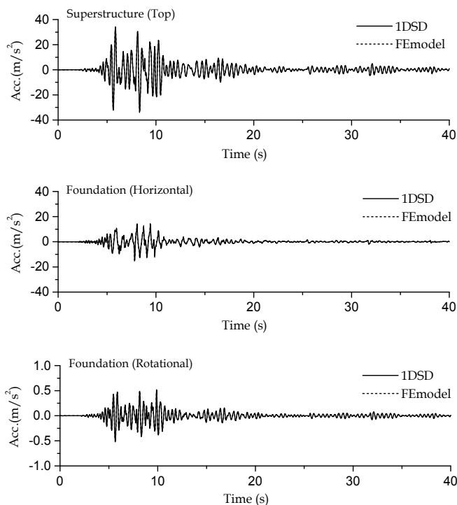
Fig. 9. Time-history response accelerations of superstructure and footing in the horizontal and rotational directions when subjected to ground motion associated with 2004 Ojia EW by using 1DSDs and the original FE model.
