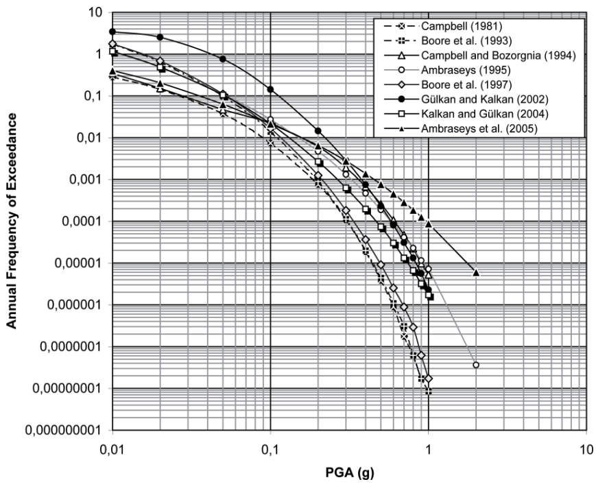
Fig. 10. Seismic hazard curve for Hatap dam site
