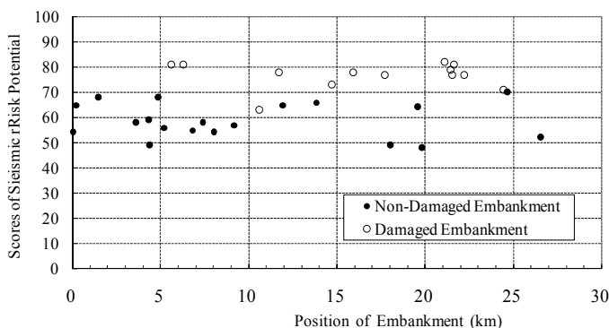
Fig. 4. Scores of seismic risk potential between non-damaged and damaged embankments in the 2007 Noto Peninsula Earthquake
