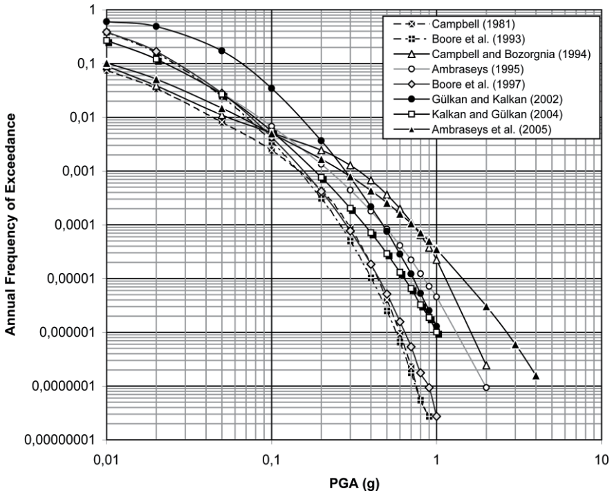
Fig. 12. Seismic hazard curve for Ayhanlar dam site
