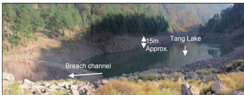
Fig. 12. Tang Lake after breaching (Photo taken on 6 th Dec-2010). From Konagai et al., 2011
