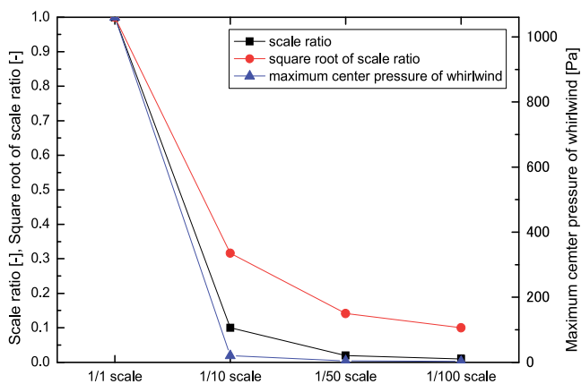
Fig. 16. Relation among scale ratio, square root of scale ratio, and maximum center pressure of whirlwind in Model 1
