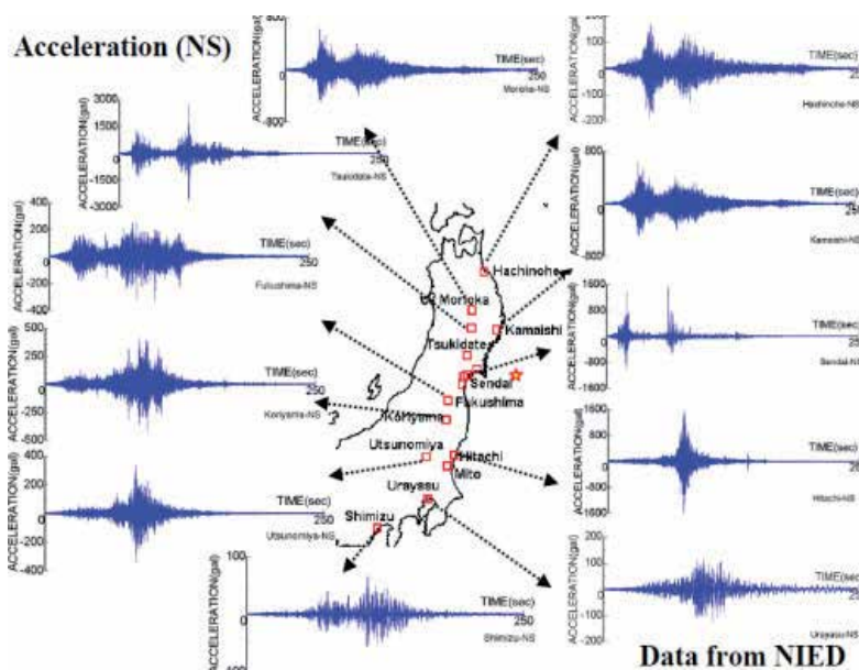
Fig. 32. Ground Acceleration Time histories Recorded in Earthquake Region. (NIED 2011)
