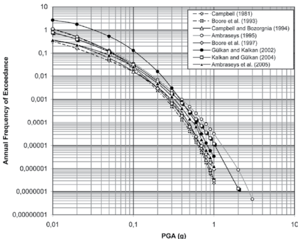
Fig. 8. Seismic hazard curve for Kilickaya dam site
