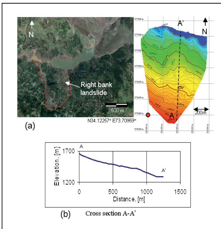
Fig. 11. (a) Satellite image of the Hattian landslide dam, Karli lake and the right bank landslide after the breaching event, along with the contour map of the landslide, (b) the longitudinal profile of the right bank slide. Modified from Konagai et al., 2011
