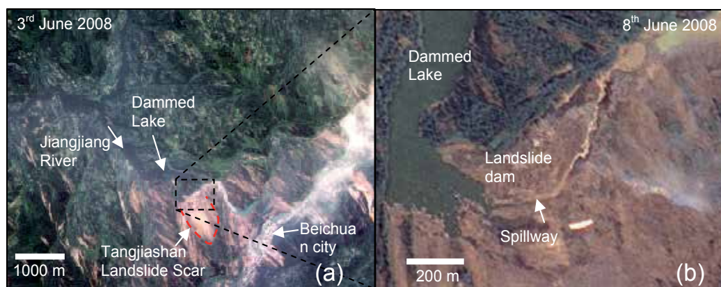
Fig. 1. True-color image of Tangjiashan landslide dam and dammed lake captured by NASA's Earth Observing-1 (EO-1) (a) on 3 rd June 2008 prior to overtopping and (b) on 8 th June after overtopping but before the breaching of dam
