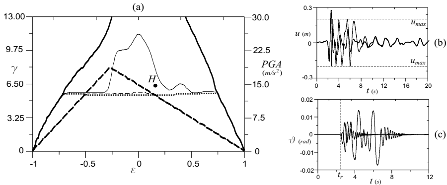
Fig. 8. Effects of the security stops under Buia earthquake: (a) Seismic scale factor versus eccentricity \varepsilon ( b = 0.3m , \lambda = 3 , \rho = 2000kg / m^3 , \xi = 0.20 , \eta = 0.70 , u_{max} = 0.20 , T = 2s ); (b) Time history of displacements u(t) for the case labelled with H in Fig.8a ( \varepsilon = 0.3 , \gamma = 6.5 ); (c) Time history of rotation \vartheta(t) for the case labelled with H .
