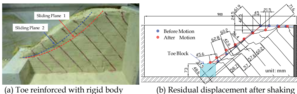
Fig. 17. Centrifuge test on toe reinforcement structure
