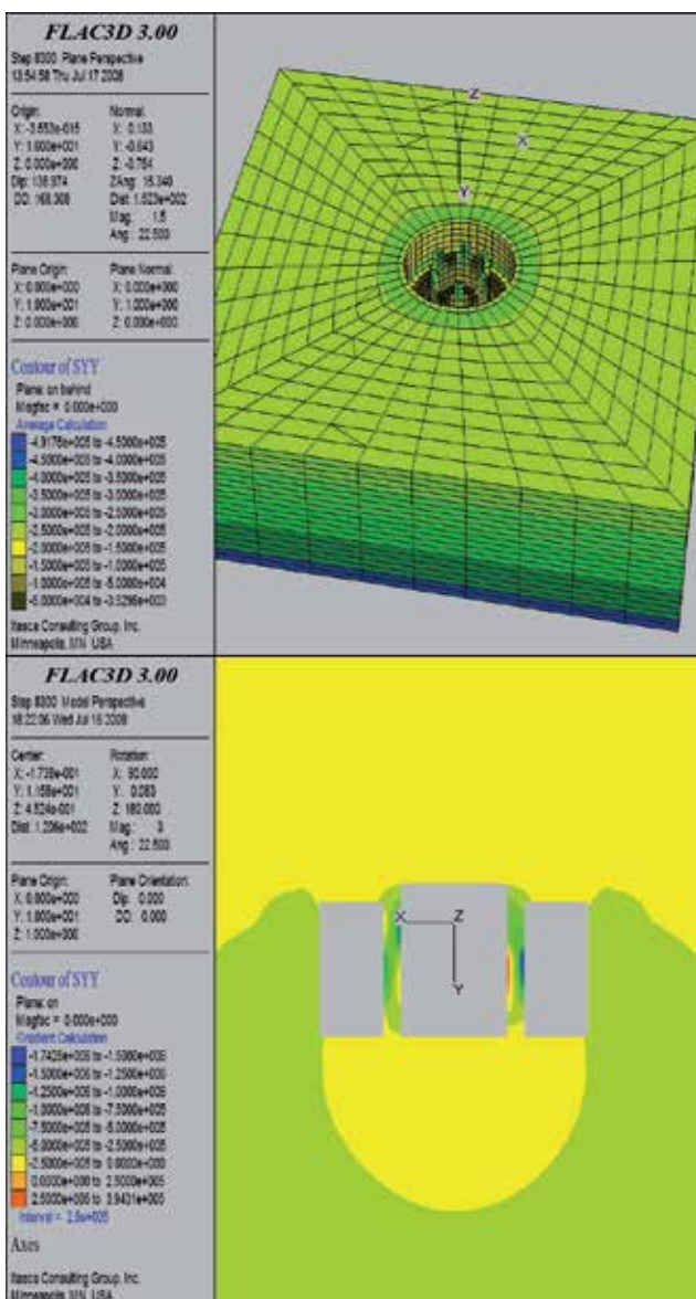
Fig. 4. Contour lines of vertical effective stresses \sigma_{yy} through the rotunda. The maximum effective compressive stresses on pillar_1 = -1.74 \times 10^5 (x) kN/m 2 .
