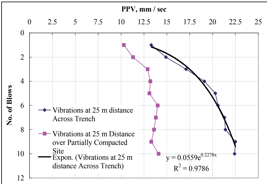
Fig. 25. Measured Ground Vibrations
