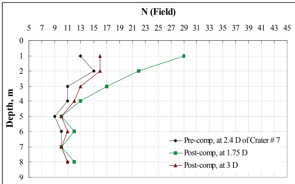
Fig. 15. Pre-to-post Compaction N (Field) Comparison of Lateral Improvement at Lower Side of Crater # 7
