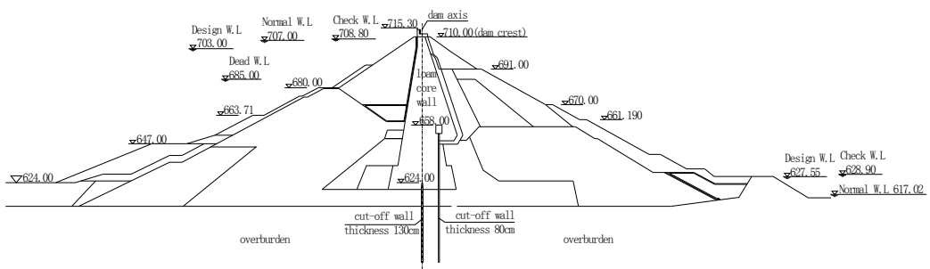
Fig. 1. Typical cross section of the dam
