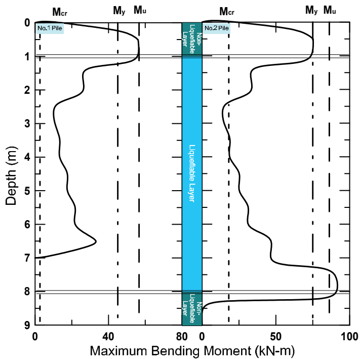
Fig. 14. Maximum pile bending moments for No.1 Pile and No.2 Pile
