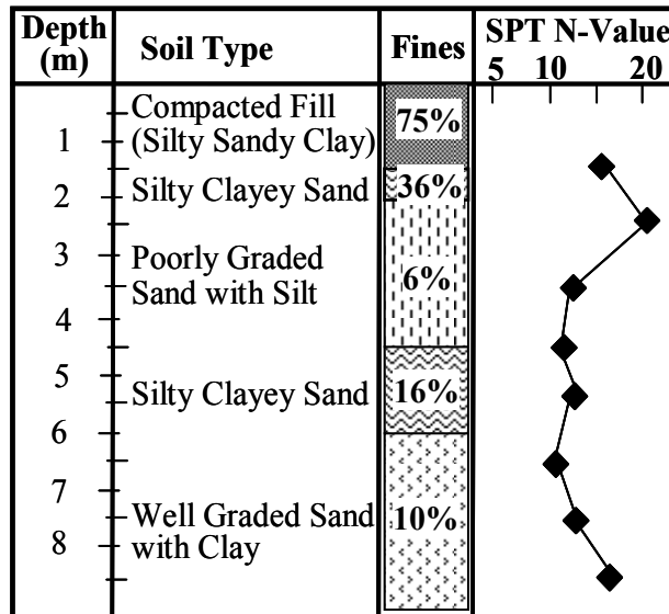
Fig. 2. Geotechnical Soil Profile
