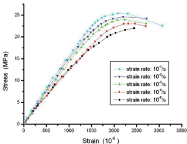
Fig. 8. The stress-strain curves of concrete in compression
