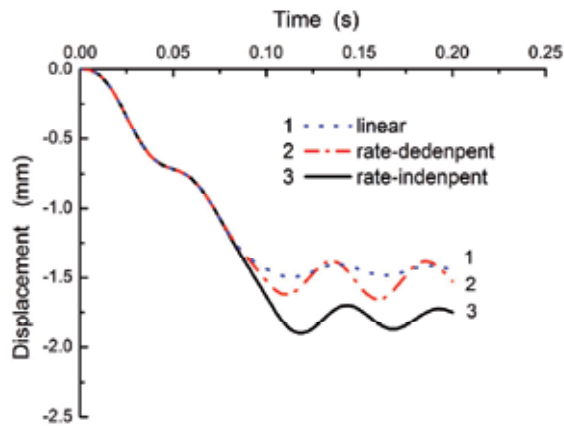
Fig. 15. Displacement of point A
