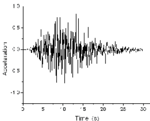
Fig. 18. Time history of earthquake input
