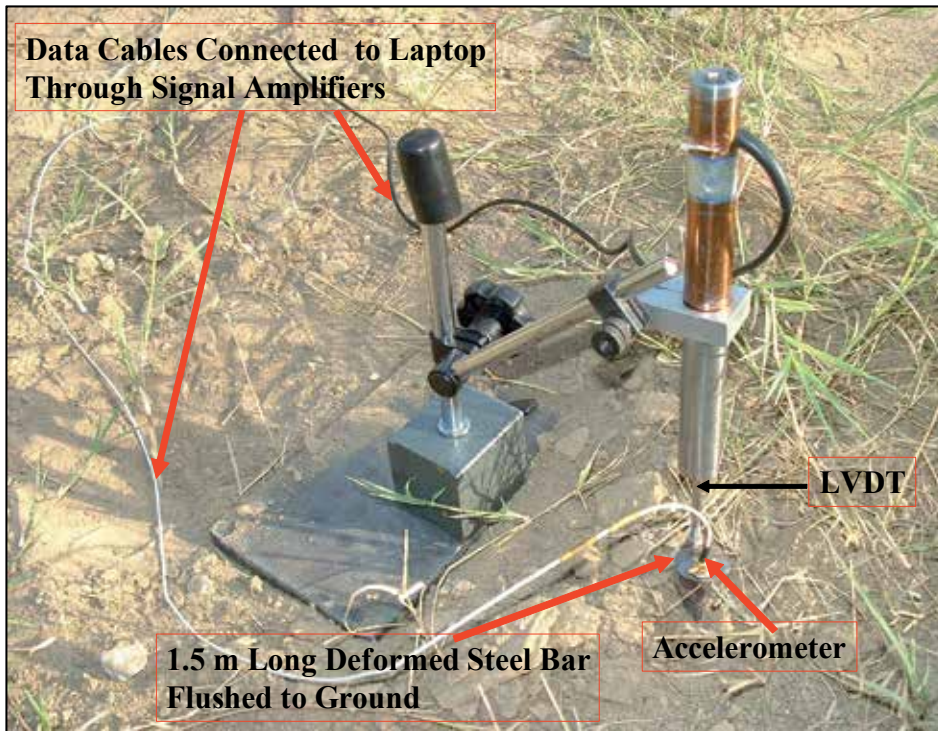
Fig. 23. Installation arrangement of LVDT and accelerometer
