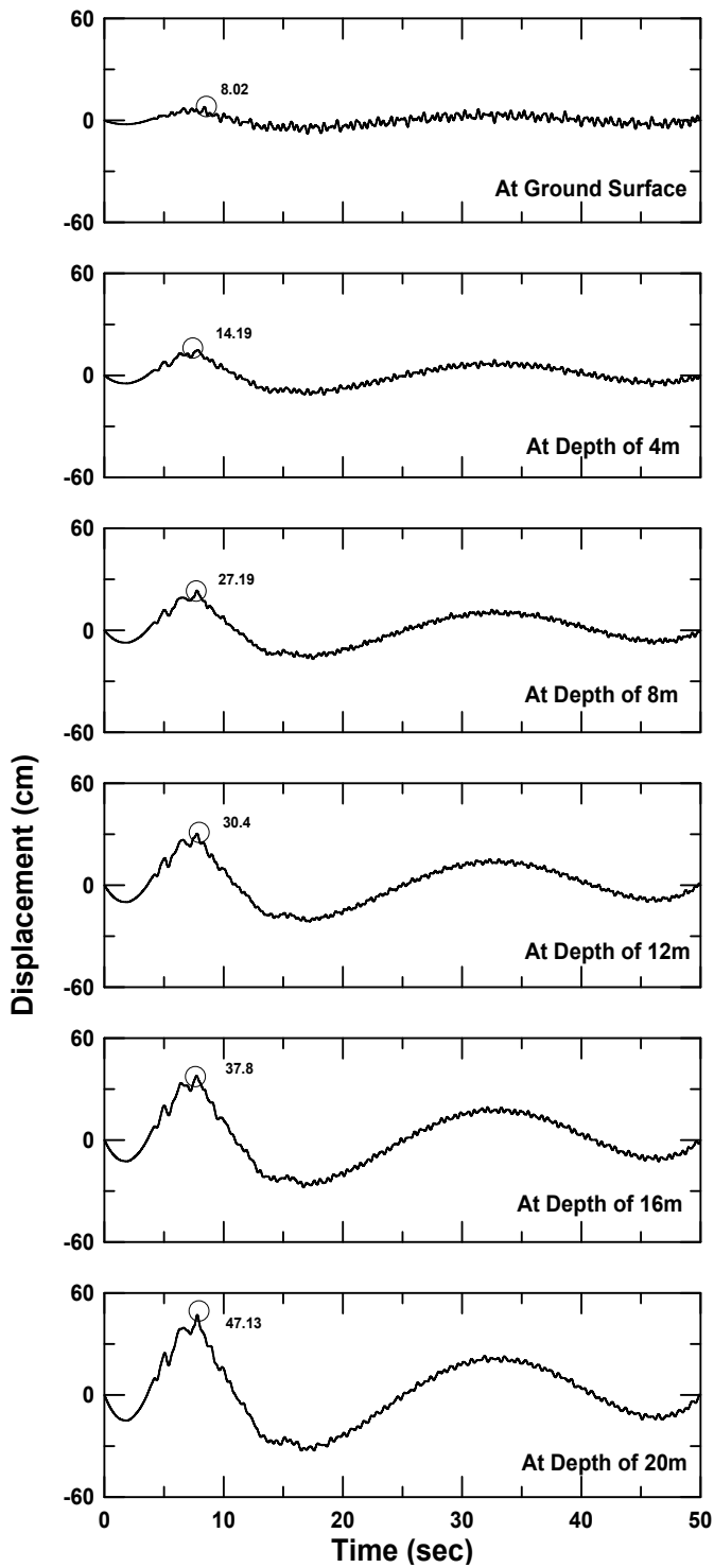
Fig. 17. Time histories of lateral displacement along the Tank TA72 No.2 pile
