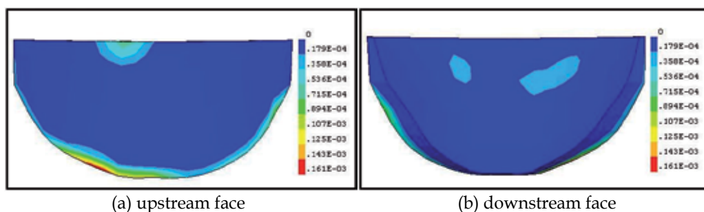
Fig. 26. Distribution of the equivalent viscoplastic strain (model III)
