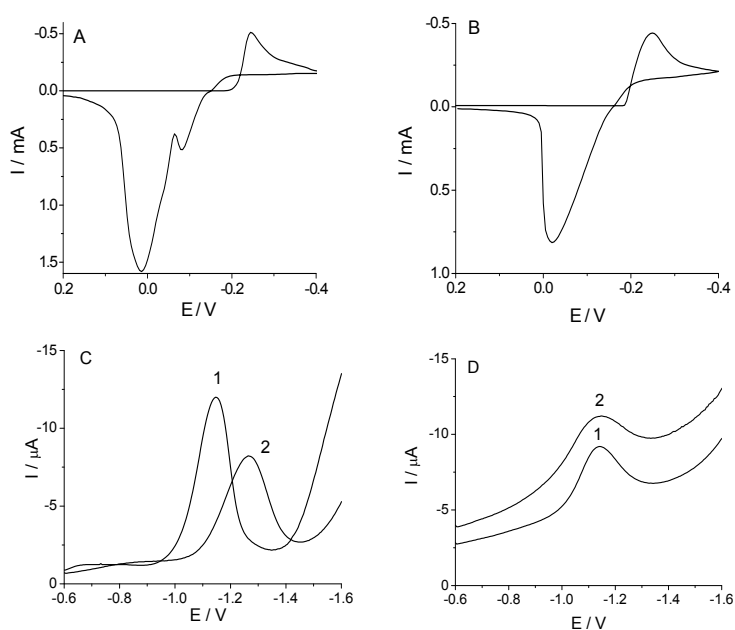
Fig. 12. Cyclic voltammogram recorded with two types of TCP in the solution consisting of 0.02 M \text{Bi}(\text{NO}_3)_3 , 1 M HCl and 0.5 M KBr, ( v = 25 \text{ mV s}^{-1} ): A) TCP-CPE and B) SO-CPE and comparison of DPV signals obtained at two different bare and surface modified substrate working electrodes: C) BiF/TCP-CPE (1) and TCP-CPE (2) and D) BiF/SO-CPE (1) and SO-CPE (2) in the same Imidacloprid solution while c = 33.34 \mu\text{g mL}^{-1} and pH 7.0.
