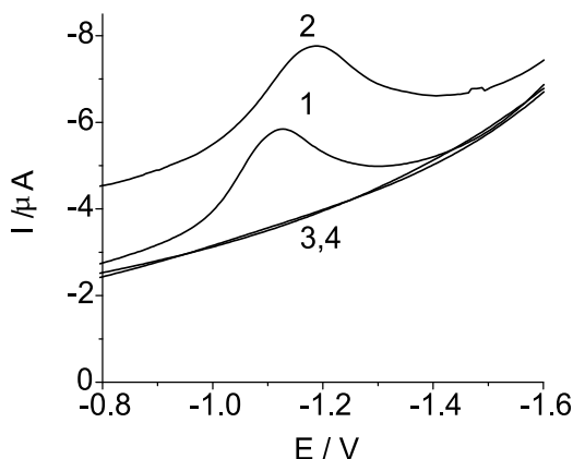
Fig. 6. An assay on potentially adsorptive behavior of Imidacloprid at the TCP-CPE: 1) DPV reduction, 2) DPV reduction after 20 min. of accumulating under open-circuit conditions, and 3,4) base-lines before and after 1 st measurement. Other experimental parameters: pH 8.0, c(\text{IMI}) = 33.3 \mu\text{g mL}^{-1} ; scan rate, 25 \text{ mV s}^{-1} , pulse amplitude, +50 \text{ mV} , pulse width 50 ms
