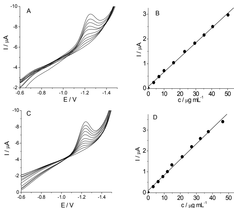
Fig. 15. Differential pulse voltammograms of Nitenpyram recorded at different concentrations of the compound at Bi 5 %/TCP-CPE (A) and TCP-CPE (C) with the corresponding calibration curves (B and D).
