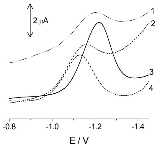
Fig. 1. Comparison of the DPV signals obtained at different working electrodes: SO-CPE (1), C14-CPE (2), TCP-CPE (3) and GCE (4) in the same solution of Imidacloprid . Experimental parameters: 25 mV s -1 , pulse amplitude 50 mV, pulse width 50 ms, c = 33.3 μg mL -1 , pH 7.0.
