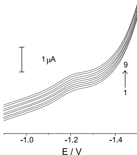
Fig. 7. The reproducibility of the analytical signal for Thiamethoxam at the TCP-CPE. Model concentration, c(\text{TH}) = 3.7 \mu\text{g mL}^{-1} measured in an time interval of 30 min (Papp, 2011).
