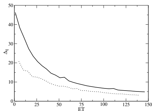
Fig. 7. Interval between pesticide application, \Delta_t , versus economic threshold, ET . The solid line corresponds to the non-spatial model, and the dotted line to the spatial model.
