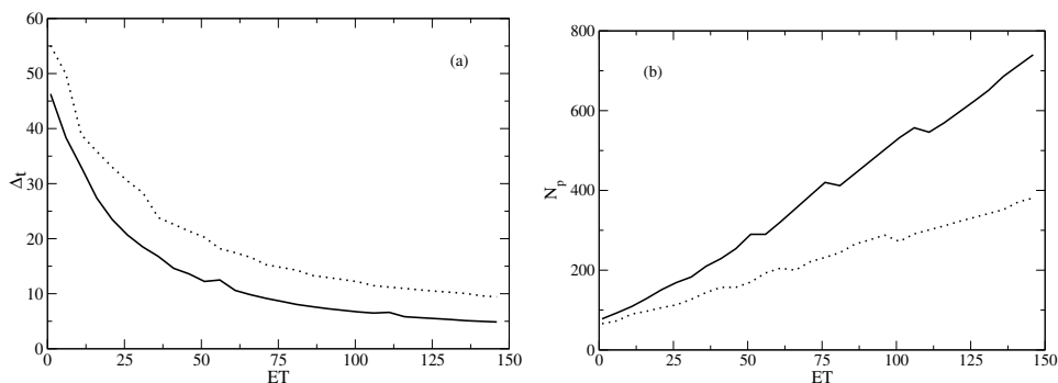
Fig. 5. In (a) interval between pesticide application, \Delta_t , versus economic threshold, ET . The lines divide the (\Delta_t - ET) parameter space into two regions, and are obtained for different \tau values. Below each line, the IMP technique succeeds, and above it the technique fails. In (b) the number of applications in 15 years versus ET . The solid line corresponds to \tau = 20 and the dotted line to \tau = 30 .
