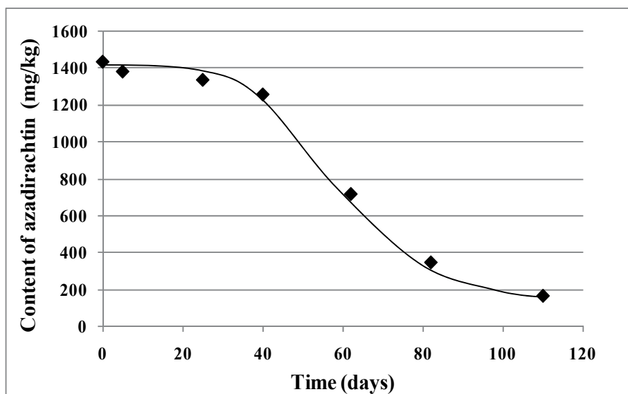
Fig. 3. Degradation curve of azadirachtin to commercial Neem oil in storage.
