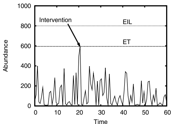
Fig. 1. Temporal evolution of the insect population, economic injury level (EIL) and economic threshold (ET).
