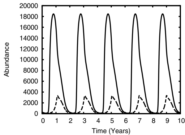
Fig. 3. Temporal evolution of the total prey (solid line) and natural enemy (dashed line) population for the non-spatial model without IPM strategy.
