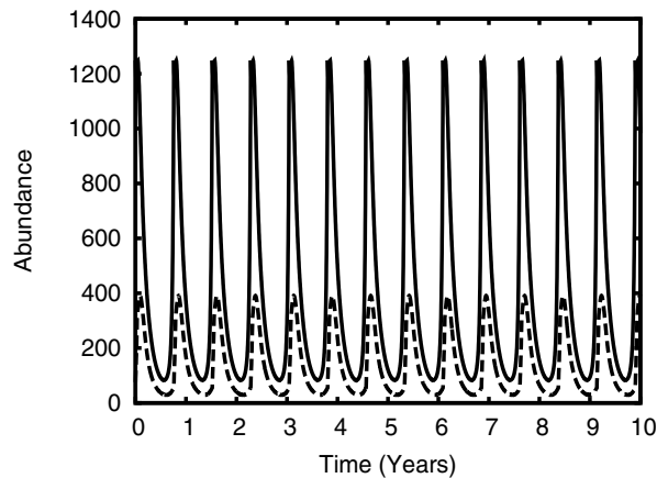
Fig. 4. Temporal evolution of the total pest (solid line) and natural enemy (dashed line) populations for the non-spatial model with IPM strategy
