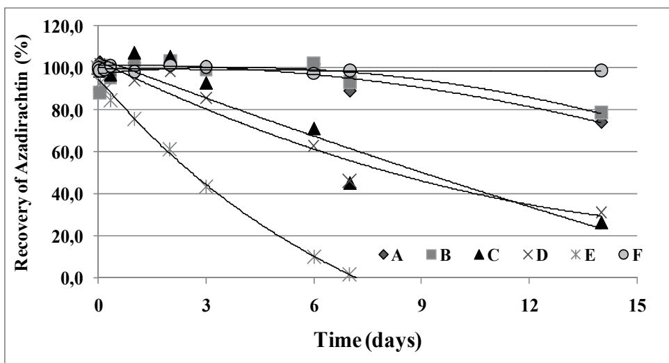
Fig. 8. Recovery of azadirachtin after UV radiation. A) Nanocapsules in powder without tensioactive; B) Nanocapsules in powder with tensioactive; C) Nanocapsules in colloidal suspension without tensioactive; D) Nanocapsules in colloidal suspension with tensioactive; E) Neem oil and F) Neem oil coated of UV radiation.
