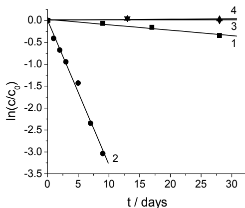
Fig. 11. Comparison of the kinetics of the photolytic (1) and photocatalytic (2) degradation of Thiamethoxam monitored by DPV with TCP-CPE. The lines for the monitoring of the stability of Thiamethoxam in dark in absence (3) and presence (4) of \text{TiO}_2 are also presented. The initial concentration of the insecticide was 116.7 \mu\text{g mL}^{-1} .
