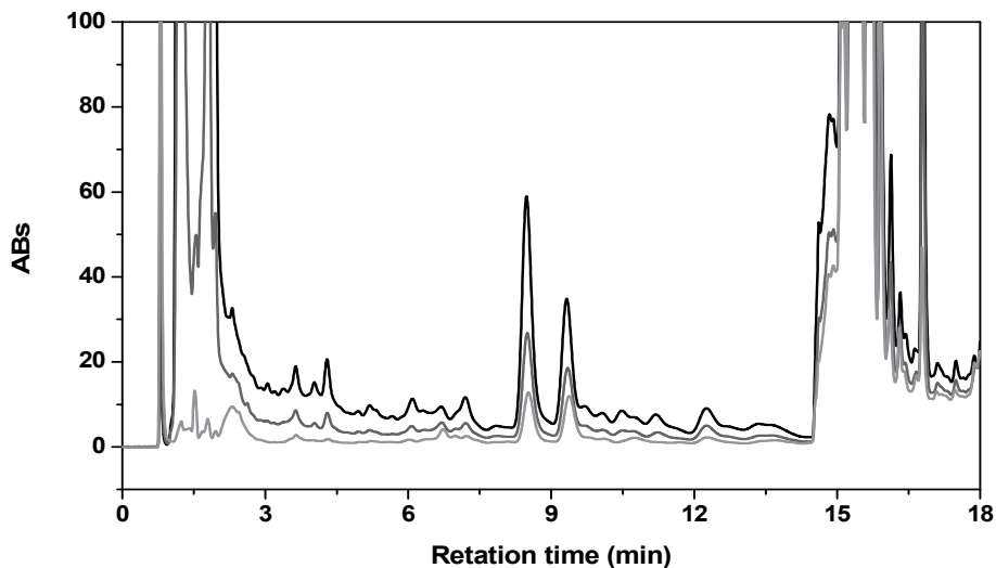
Fig. 6. Chromatograms of enriched Neem oil containing 1,000, 2,000 and 4,000 mg kg -1 of azadirachtin.
