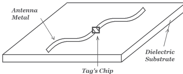
Fig. 2. The physical structure of a RFID tag.
