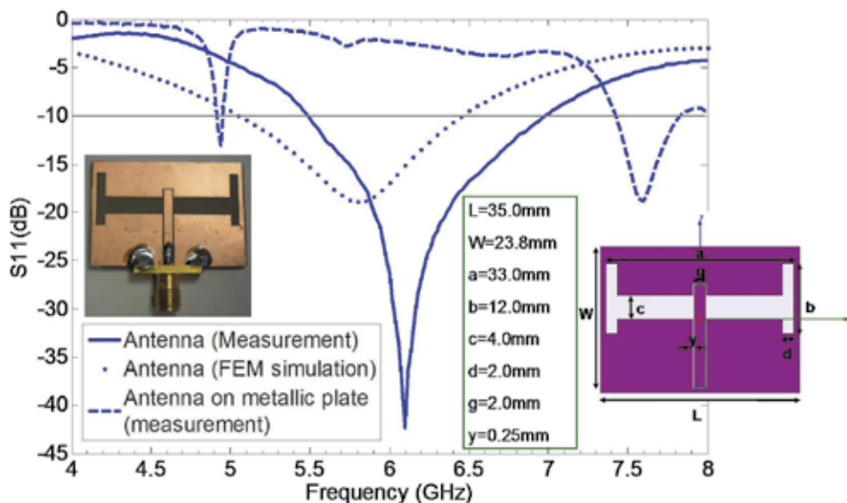
Fig. 4. Return loss of the antenna; Geometry and dimensions; Manufactured prototype.
