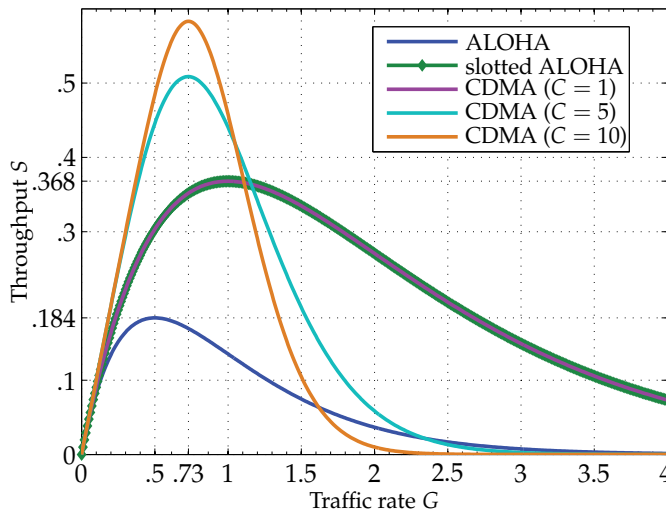
Fig. 2. Various throughputs S over traffic rate G for ALOHA, slotted ALOHA and CDMA
