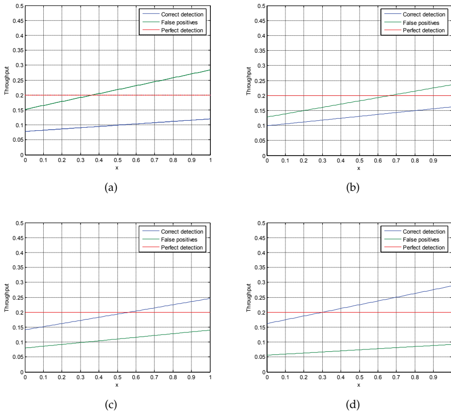
Fig. 4. Performance of ALOHA with context aware analysis
