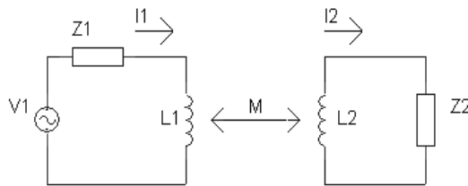
Fig. 3. Model of coupling reader-tag
