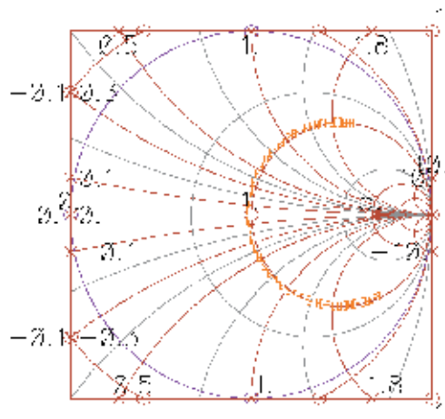
Fig. 10. S_{11} parameter of the circuit from Fig. 8, in a Smith chart.
