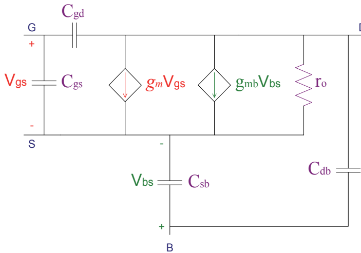
Fig. 14. Hybrid- \pi model including the parasitic capacitances.
