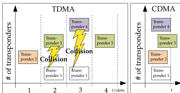
Fig. 1. Comparison of TDMA and CDMA communication channel access techniques for RFID
