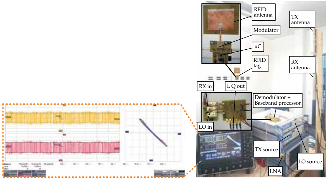
Fig. 6. Setup of CDMA-based UHF-RFID system with a magnification of the oscilloscope's screen
