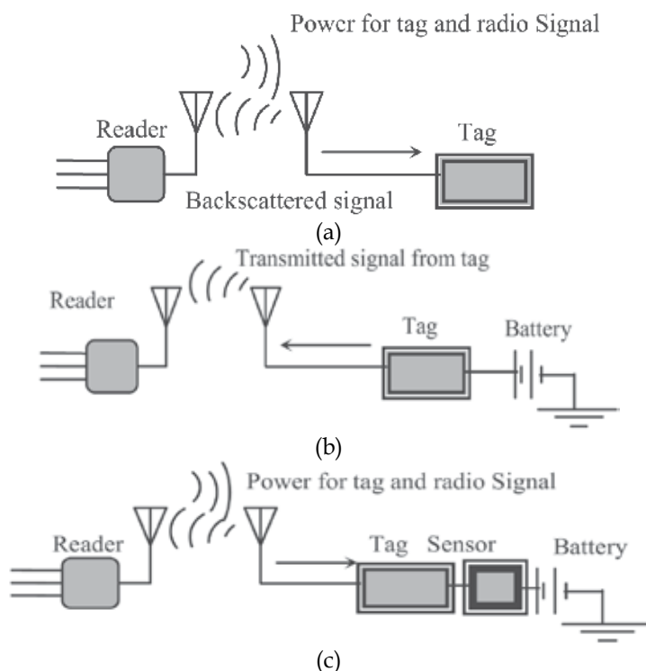
Fig. 2. Communication between (a) reader and passive tag, (b) reader and active tag, (c) reader and semi-passive tag (Khan et al. 2009)
