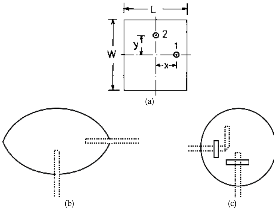
Fig. 13. (a) Rectangular microstrip antenna with two orthogonal feeds for dual-band operation, (b) Elliptical microstrip antenna with two orthogonal feeds, (c) Circular microstrip antenna with two orthogonal slots (Kumar & Ray 2003)
