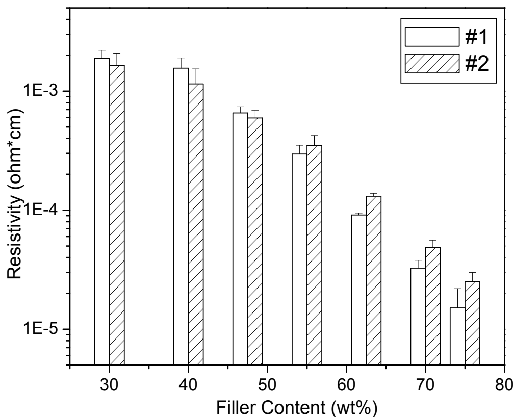
Fig. 8. Resistivity of the printed resistor of the ECAs (#1 and #2) with different silver filler contents. (Copyright © 2011 Springer Publishing House)
