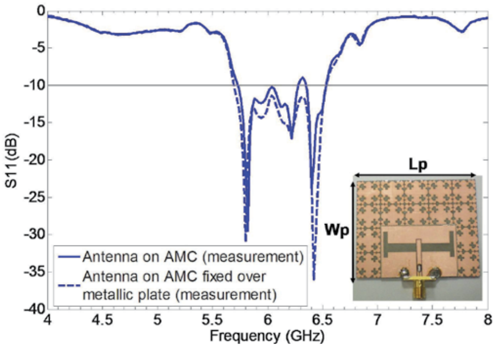
Fig. 7. Measured input return loss for the antenna and the antenna on AMC on a metallic plate; manufactured prototype.
