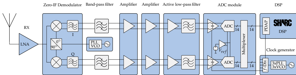
Fig. 16. Architecture of receiving system
