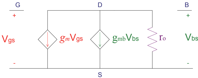
Fig. 11. Hybrid- \pi model.
