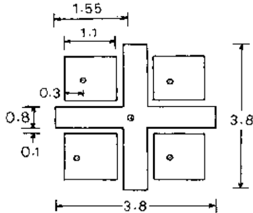
Fig. 17. Dual frequency sub-array microstrip antenna (Salvador et al. 1995)
