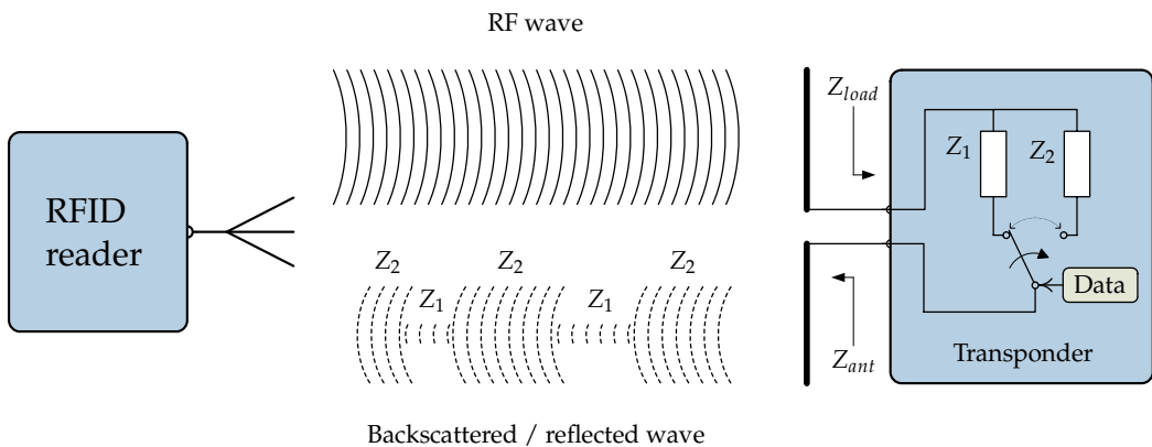
Fig. 7. Basic function of RFID transponder
