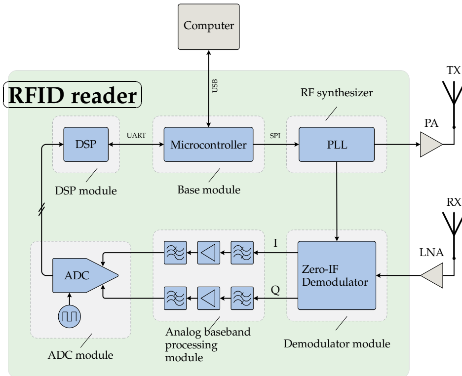
Fig. 4. Basic concept of RFID reader; depicted in bistatic antenna configuration
