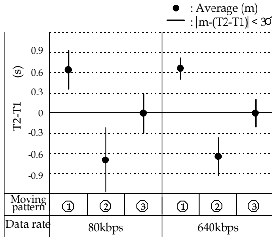
Fig. 12. Measurement results of (T2-T1)
