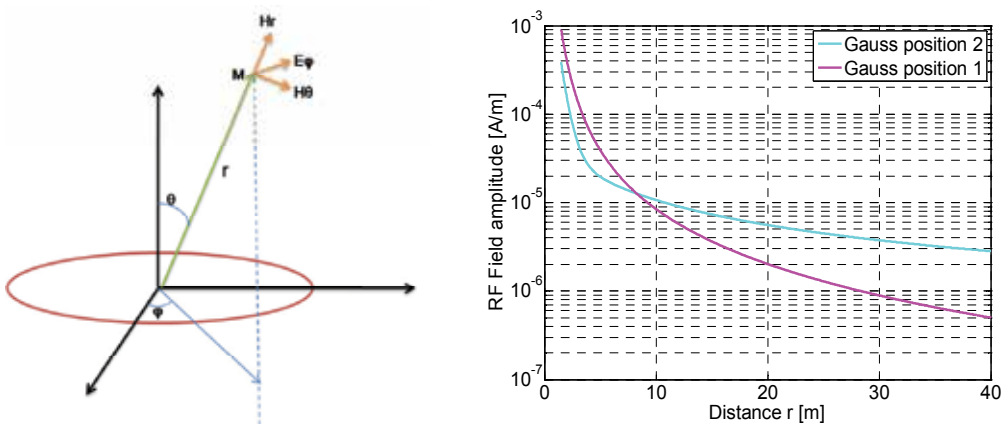
Fig. 2. a: Magnetic and electrical field seen as a distance r of the antenna; b: Results of the theoretical approach
