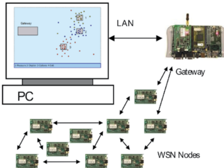
Fig. 6. WSN system overview
