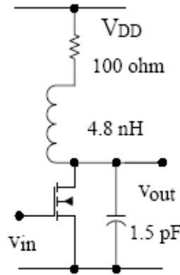
Fig. 6. Common-source stage with RLC-load.
