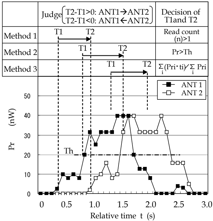
Fig. 6. Three methods in double antenna method
