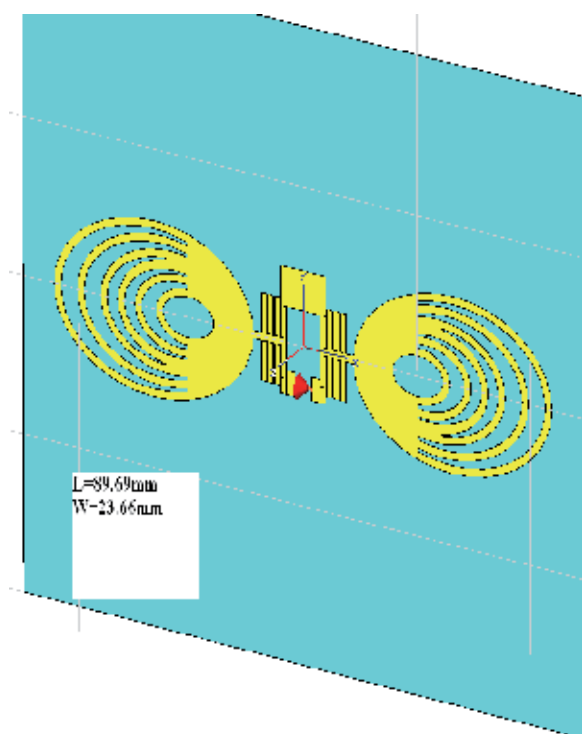
Fig. 14. A tag antenna using a company logo
