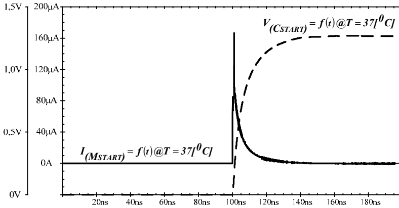
Fig. 13. The Start Up transient current.
