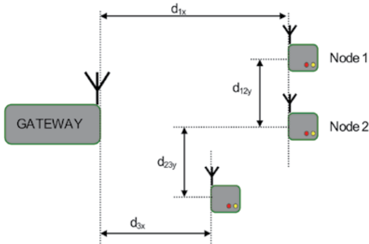
Fig. 7. Test setup with the Gateway and three WSN nodes ( d_{1x}=2.5\text{m} , d_{3x}=2.2\text{m} , d_{12y}=0.4\text{m} , d_{23y}=0.8\text{m} )
