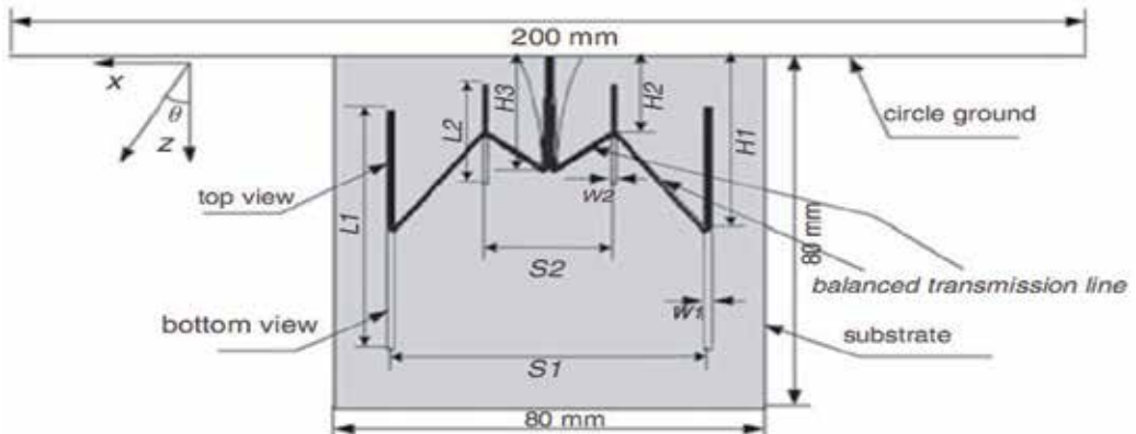
Fig. 22. Geometry of the dual-band bidirectional high gain antenna (Zhang et al. 2009)
