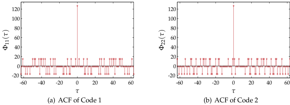
Fig. 13. ACF of original Gold codes
