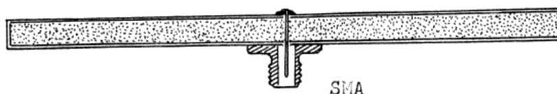
Fig. 12. Cavity method for measuring the PET's dielectric constant and loss tangent
