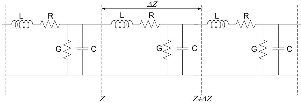
Fig. 1. Lumped component model of a transmission line.
