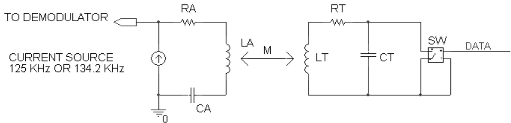
Fig. 2. Current-driven reader
