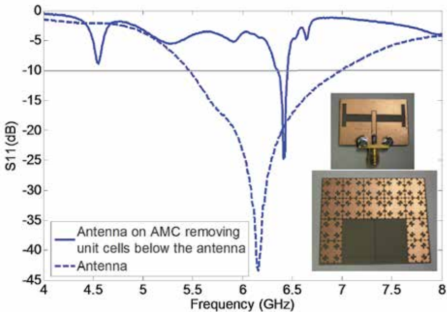
Fig. 11. Measured input return loss for the antenna and the antenna on AMC when the unit cells under the antenna are removed.
