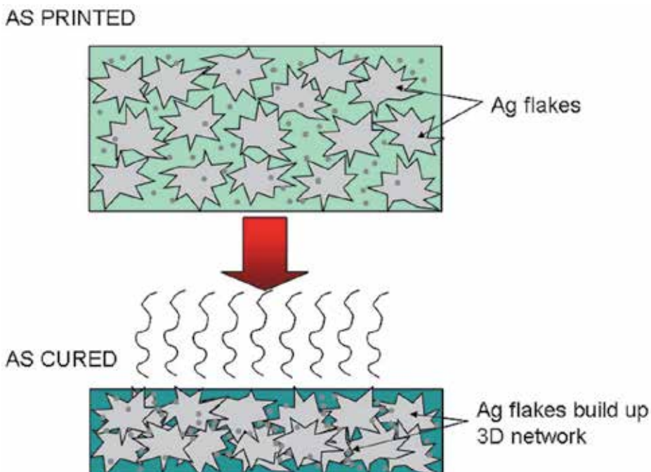
Fig. 3. A schematic showing the influence of the curing step of the ECAs, which is critical to the percolation of the fillers.
