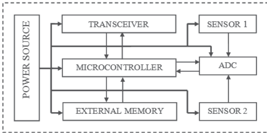
Fig. 2. WSN node architecture
