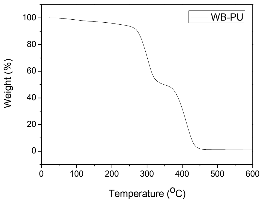
Fig. 14. TGA analysis of the PU dried film. The sample was ramped from 25 °C to 600 °C in the air.
