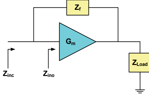
Fig. 13. Feedback system with effective transconductance.
