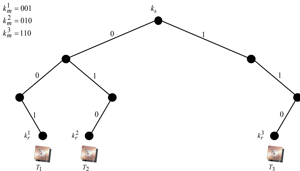
Fig. 23. A sparse binary tree of three levels
