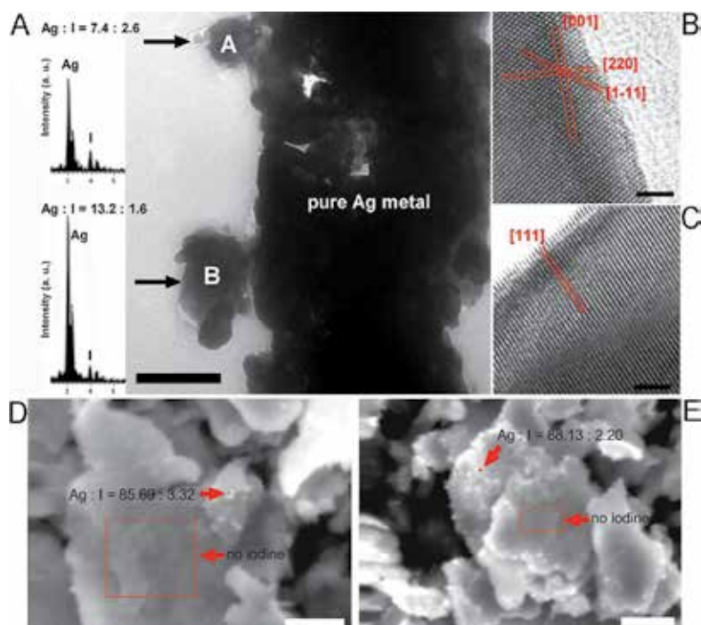
Fig. 4. A)-C): TEM-EDS analysis of the ECA cross sections. A) TEM-EDS of the nano-islands on a sectioned ECA sample (filled with A9). (Scale bar = 200 nm) EDS spectra are accompanied on the left. B) HRTEM image of bare silver micro-flake surface. (scale bar = 2 nm) C) HRTEM image of A9 filled ECA surface, except for the nanocluster parts. (scale bar = 2 nm) The crystal lattice of silver metal is marked in both the images of (b) and (c). (All samples are embedded in a resin filled with 75 wt% of the filler.) D)-E): SEM-EDS analysis of the iodinated silver flakes. D) Sample A3, the elemental ratios between silver and iodine are listed in this image; (scale bar = 2.5 \mu\text{m} ) E) Sample A9, the elemental ratios between silver and iodine are listed in this image. (scale bar = 2.5 \mu\text{m} ) (Copyright © 2010 WILEY-VCH)
