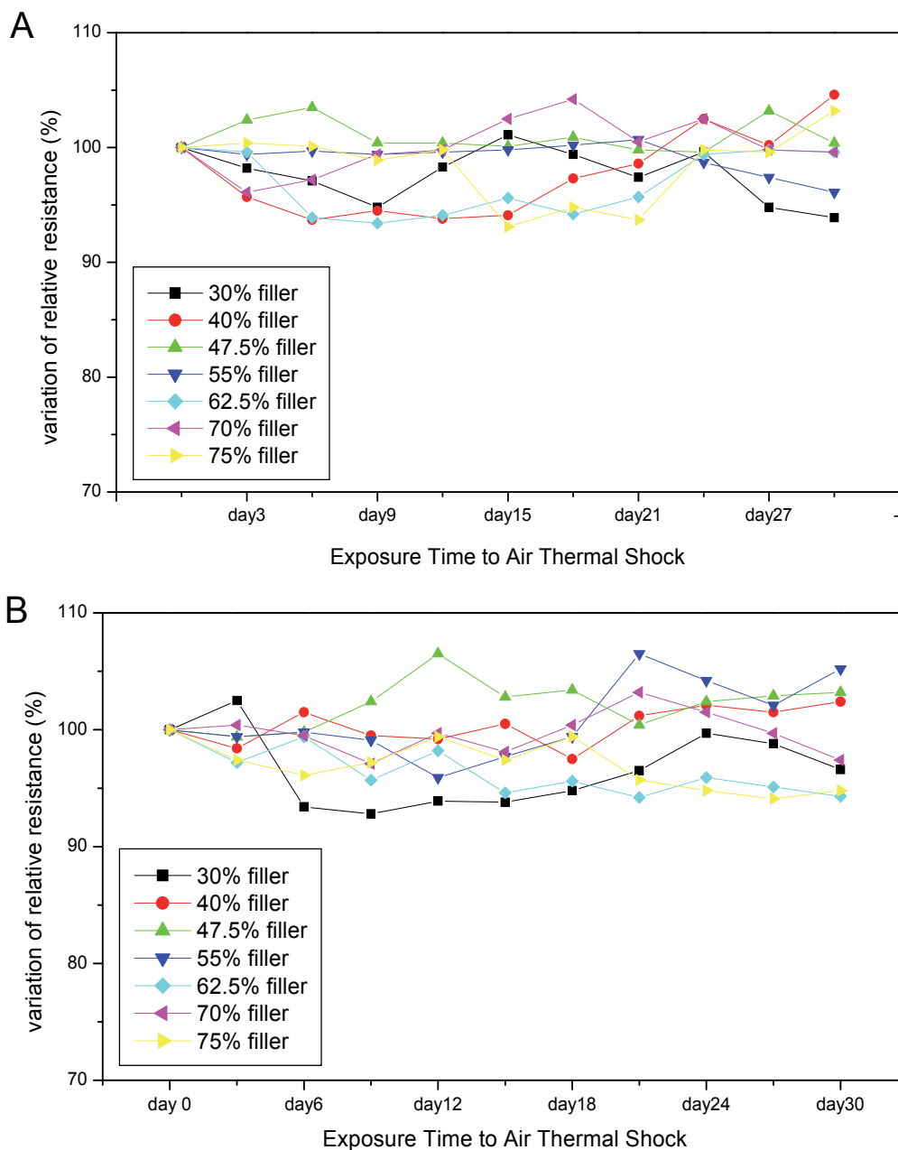
Fig. 10. Thermal cycling analysis of the ECAs. A) Variation of the relative resistance of the printed resistors of the ECA #1; B) Variation of the relative resistance of the printed resistors of the ECA #2. (Copyright © 2011 Springer Publishing House)
