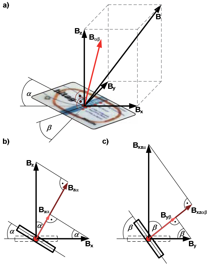
Fig. 7. Orientation of a tag, which is deviated of \alpha and \beta angles from components of magnetic induction vector: a) deviation in 3D coordinate, b) deviation of \alpha angle on z - x plane, c) deviation of \beta angle on \alpha - y plane
