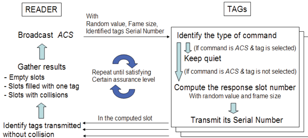
Fig. 6. Tag Identification Procedure of the I-Code System
