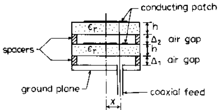
Fig. 14. A dual-frequency stacked circular-disc antenna (Long & Walton 1979)
