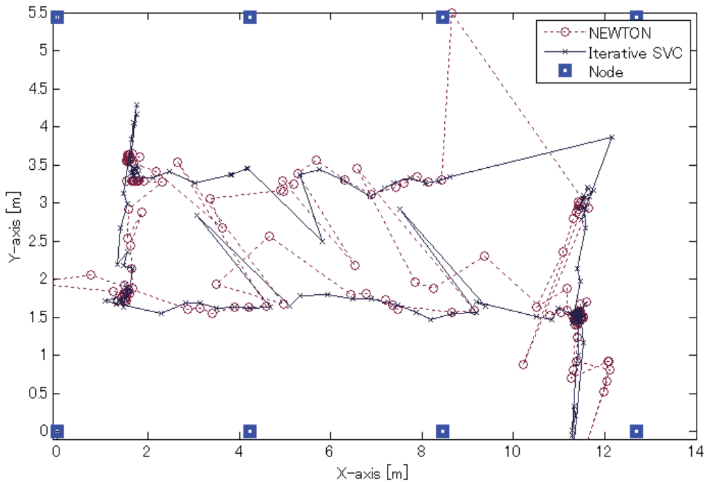
Fig. 15. Tracking result in serious NLOS environment
