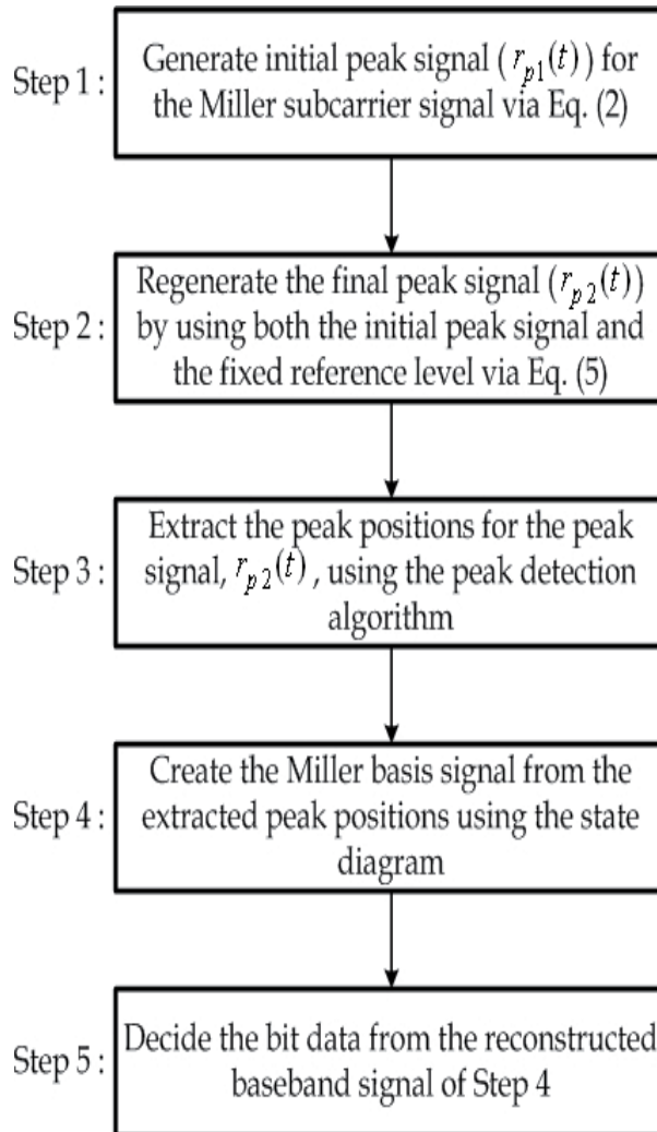
Fig. 5. Flowchart illustrating the Miller subcarrier demodulation method
