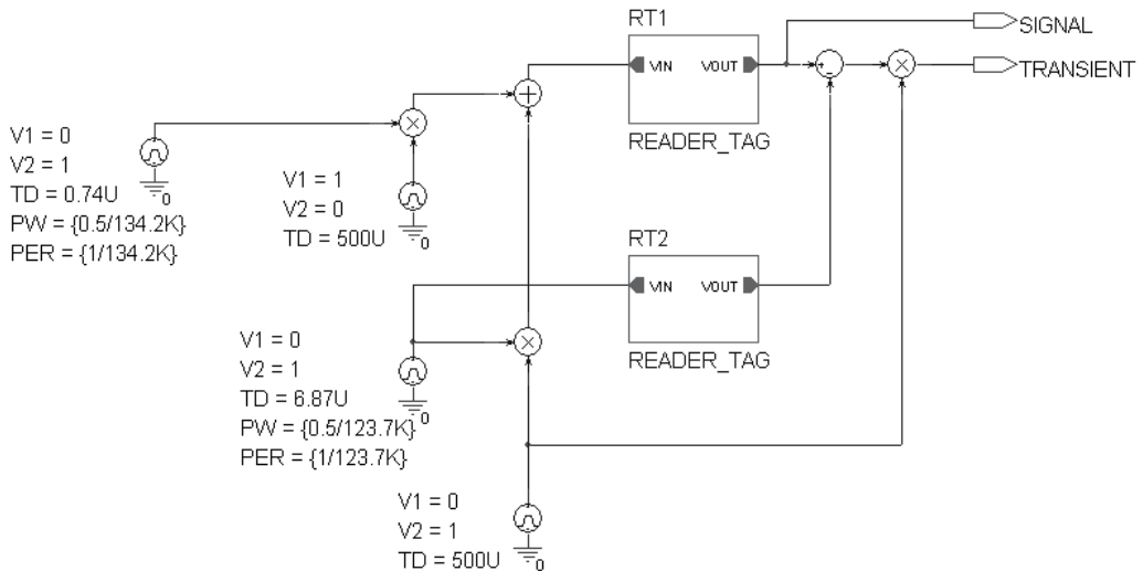
Fig. 19. Simulation of transients in the composite system
