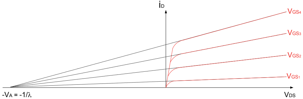
Fig. 10. Effect of channel modulation on saturation current.
