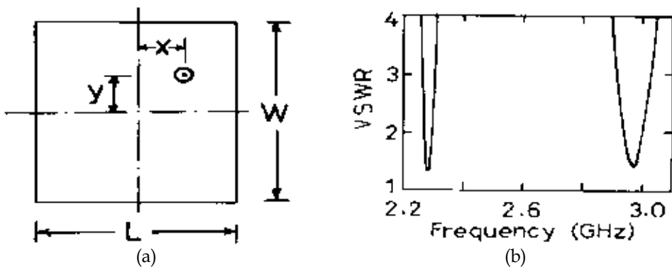
Fig. 11. (a) Rectangular microstrip antenna with a single feed for orthogonal dual-band operation and its (b) VSWR plots (Chen & Wong 1996)
