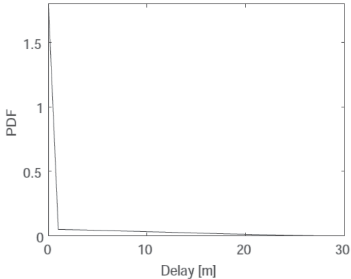
Fig. 4. IEEE.802.15.4a propagation PDF CM1(LOS)
