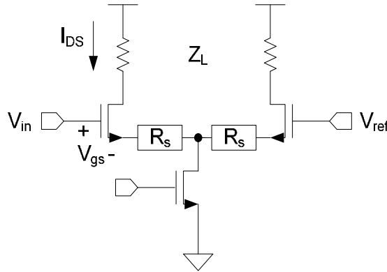
Fig. 15. Setup for transfer characteristic simulation.
