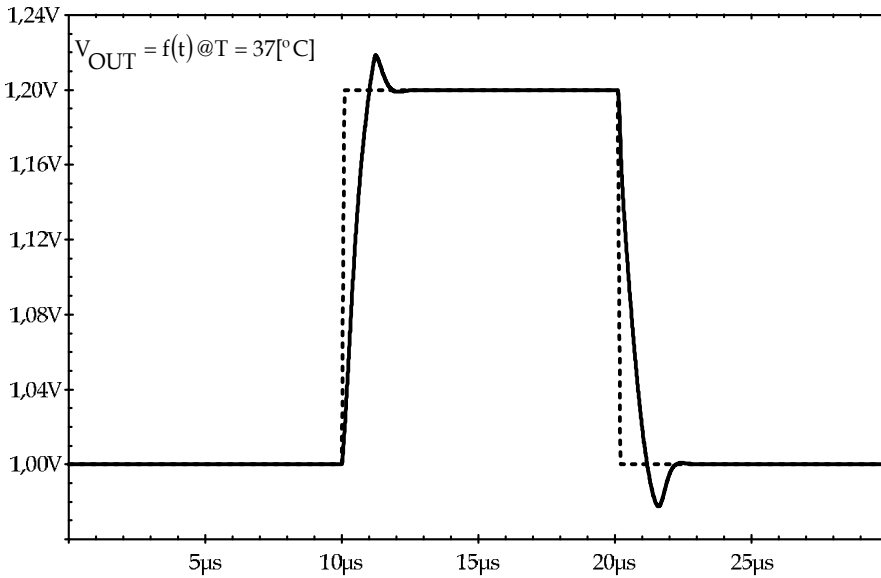
Fig. 23. OTA transient response.
