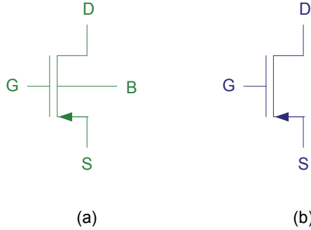
Fig. 13. Symbols for p MOS transistor; (a) four terminals and (b) three terminals.
