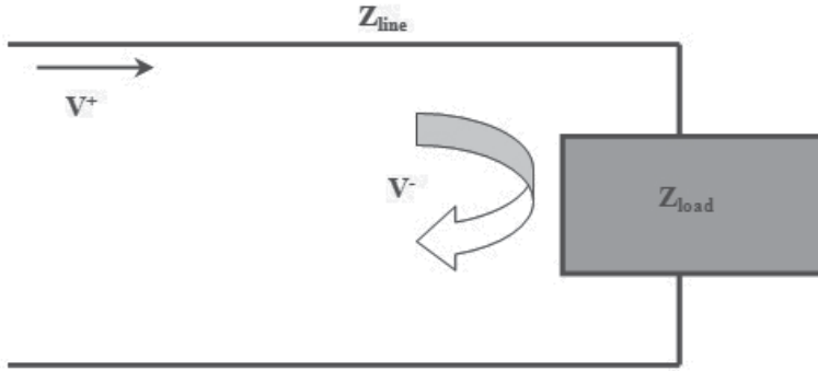
Fig. 8. Transmission line model
