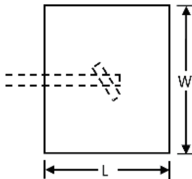
Fig. 12. Aperture coupled RMSA with an inclined slot
