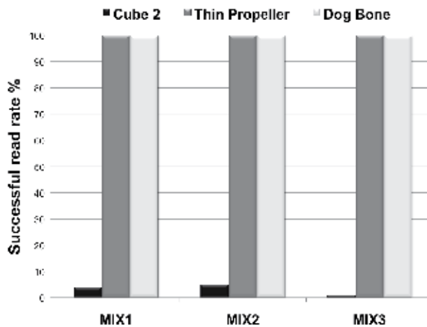
Fig. 9. A performance comparison on the border gate by varying the tag type and the composition of the plastic bag containing heterogeneous drugs.
