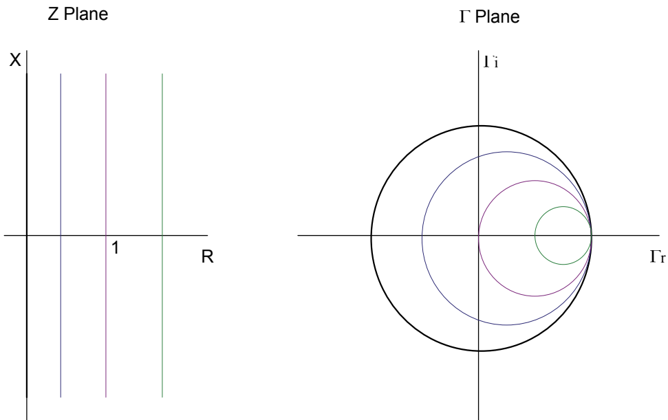
Fig. 2. Mapping of Z-plane into \Gamma -plane for constant resistances.
