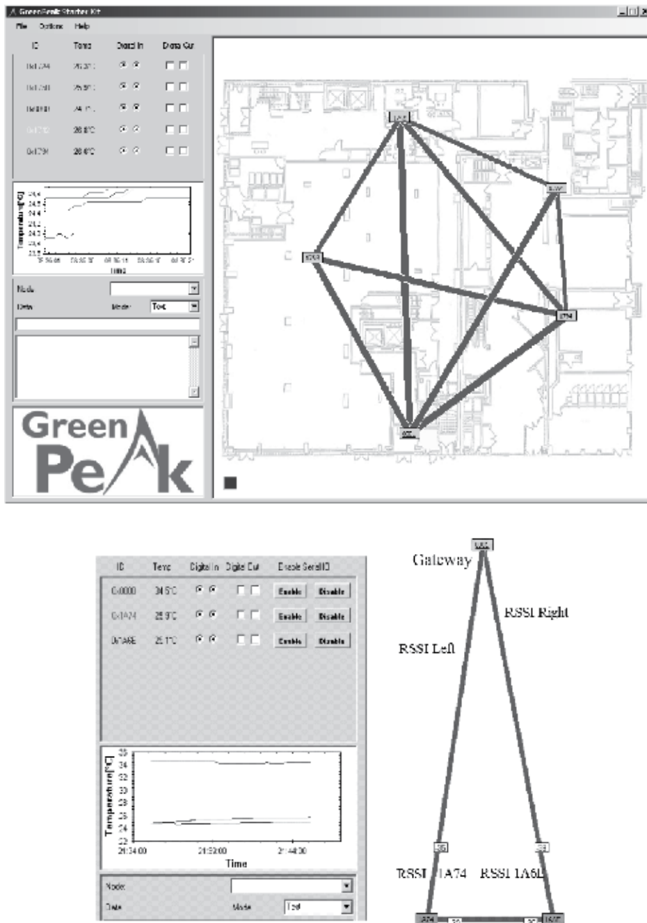
Fig. 6. Green Peak Development Software interface with RSSI measurements
