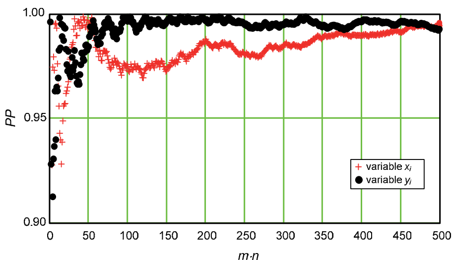
Fig. 3. Example result of probability PP of sampling of independent random variables x_i and y_i in function of numbers product: multiple sampling of m and n -tags location
