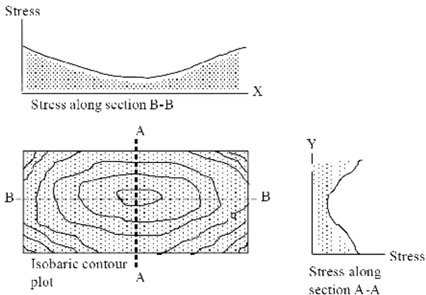
Fig. 24. Example of isobaric lines.
