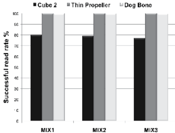
Fig. 8. A performance comparison on the cases line by varying the tag type and the composition of the case containing heterogeneous drugs.
