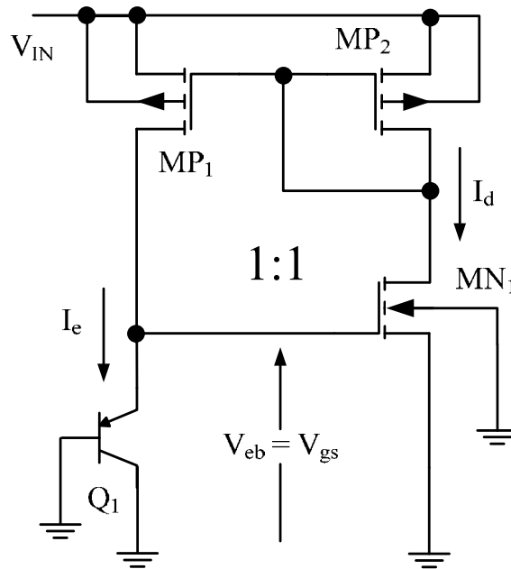
Fig. 10. Self biased current mirror.
