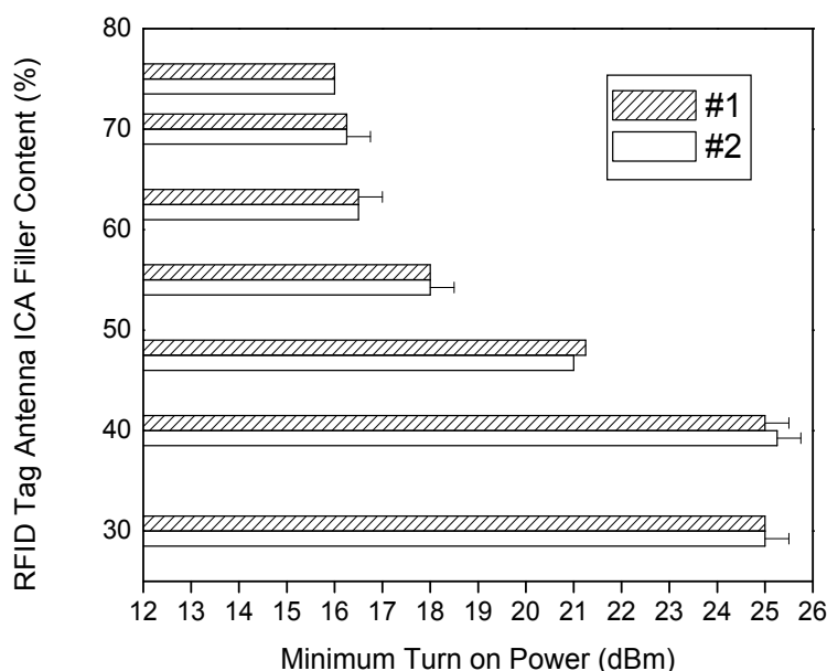
Fig. 12. Minimum turn-on power of the reader in detecting the RFID tags with the antenna printed using the ECAs. (Copyright @ 2011 Springer Publishing House)
