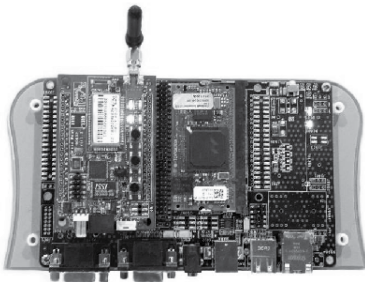
Fig. 4. Gateway/Coordinator node built around a RISC microcontroller
