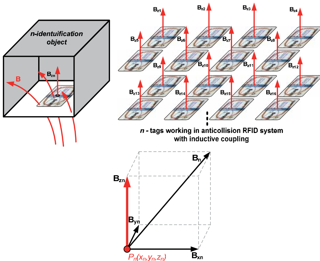
Fig. 6. Typical orientation of tags working in anticollision RFID system in relation to components of magnetic induction vector
