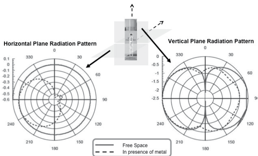
Fig. 10. Horizontal radiation pattern in free space condition (continuous line) and in presence of metal (dot line) of the Alien Squiggle Tag.
