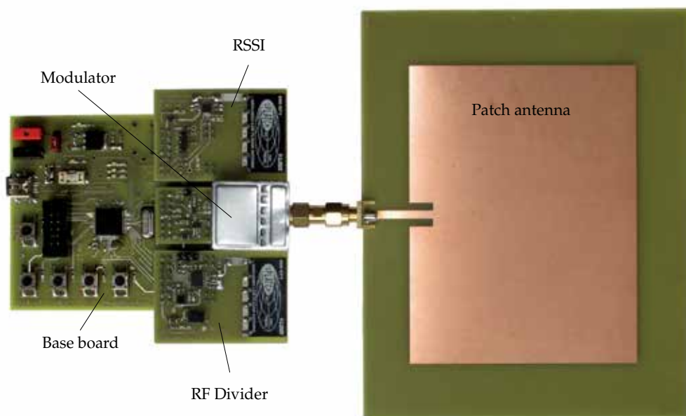
Fig. 10. Prototype of semi-passive UHF RFID transponder
