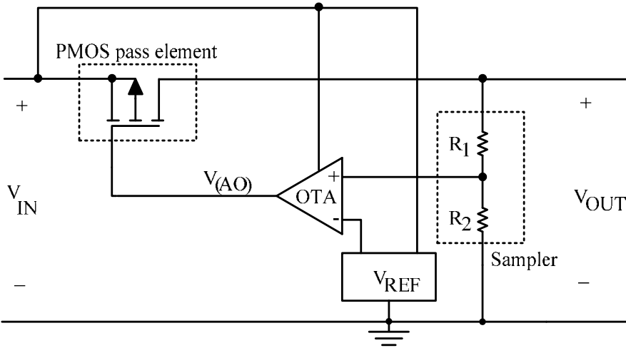
Fig. 3. PMOS based LDO.
