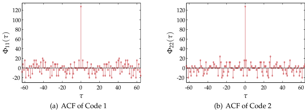
Fig. 14. ACF of adjusted Gold codes
