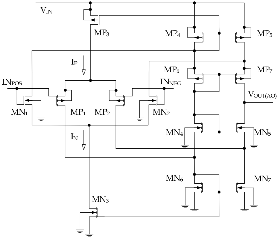
Fig. 18. Operational Transconductance Amplifier (OTA).
