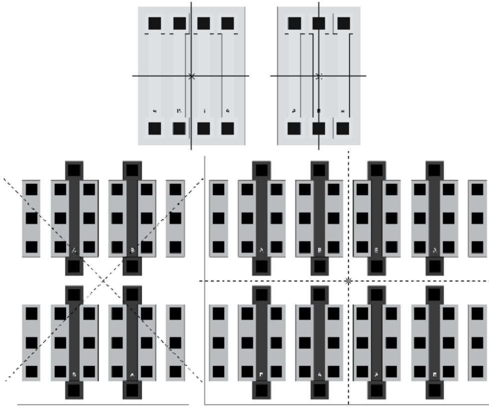
Fig. 25. Examples of centroid layout configurations.
