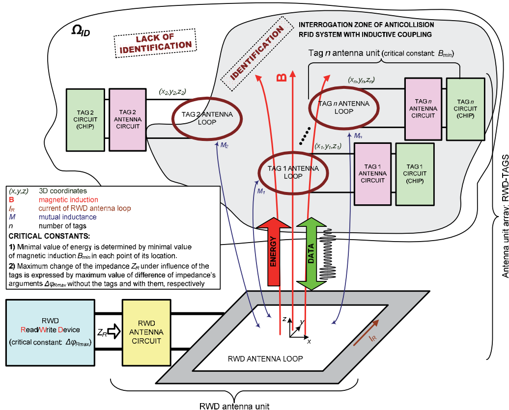
Fig. 4. Block diagram of anticollision RFID system with inductive coupling
