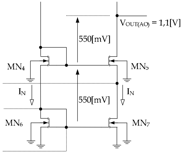
Fig. 19. Lower half used to evaluate the geometric aspect ratios.
