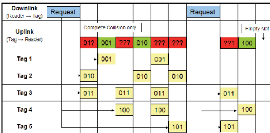
(b) Slotted ALOHA
