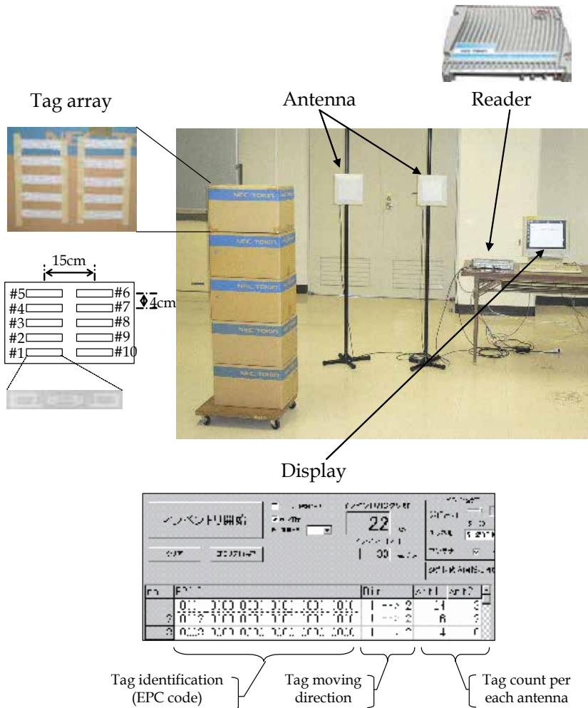
Fig. 9. Photograph of experimental environment
