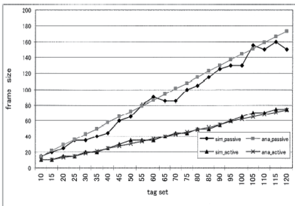
Fig. 8. Example of Optimal Frame Size For Minimum Census Delay [Bin05]
