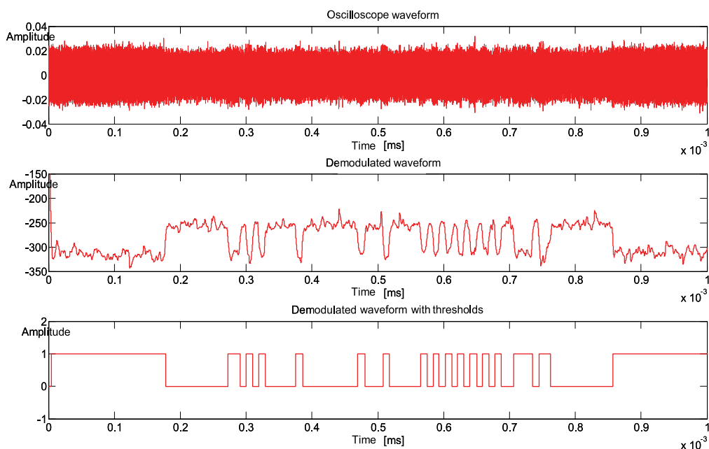
Fig. 7. Measured signals with an electric dipole at 4 metres from the emission
