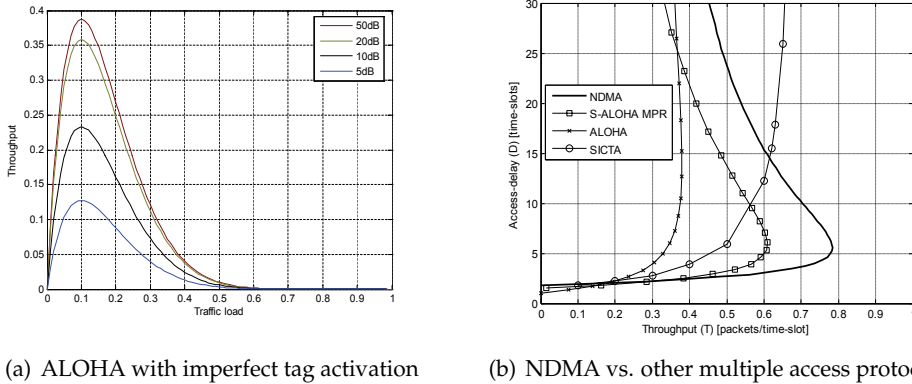
Fig. 3. Performance of MAC algorithms with cross-layer optimization
