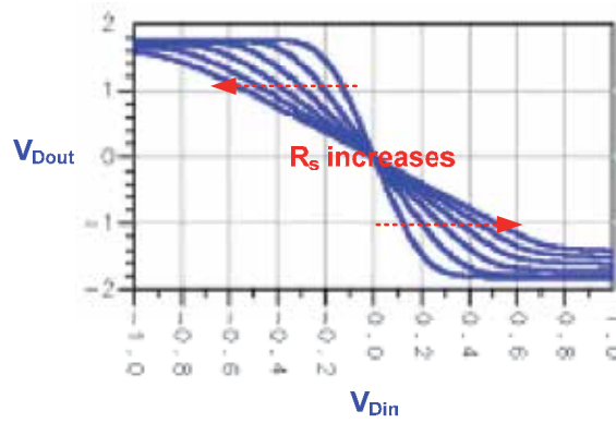
Fig. 16. DC input voltage sweeping for linearity simulation.
