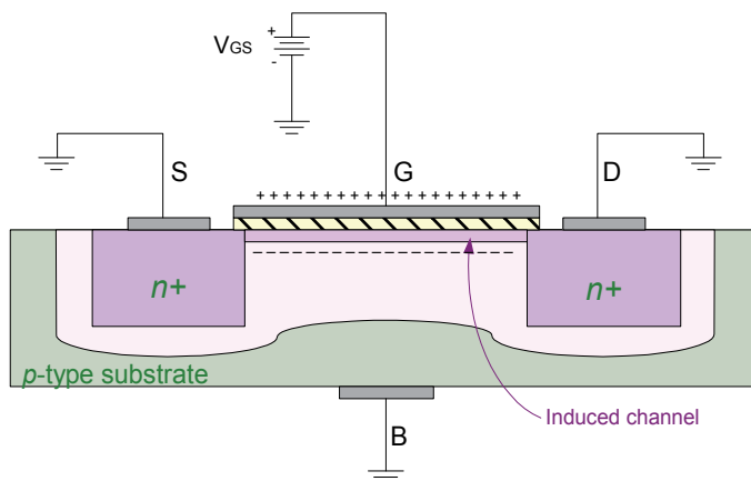
Fig. 2. n MOS with an induced channel.
