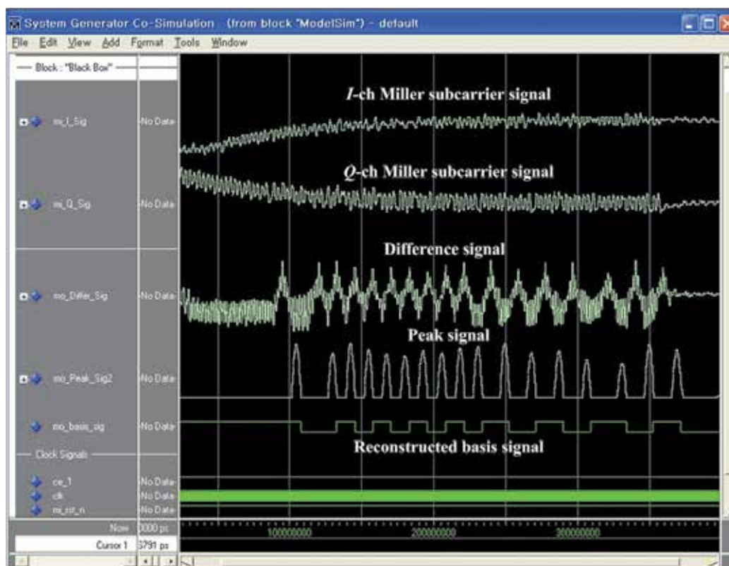
Fig. 13. Simulation result showing Black Box output through ModelSim for the proposed demodulation structure
