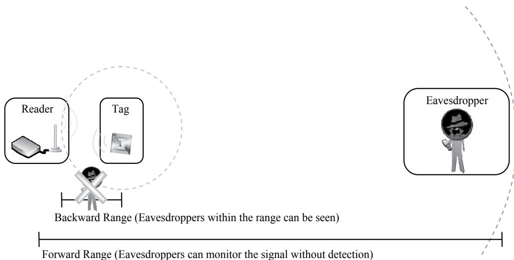
Fig. 10. Forward vs. backward channels
