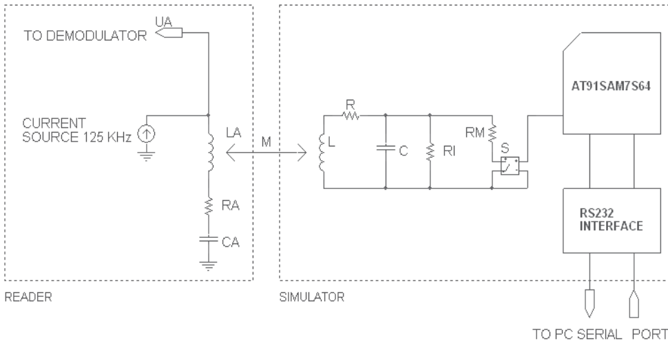
Fig. 15. Interaction between current-driven reader and simulator
