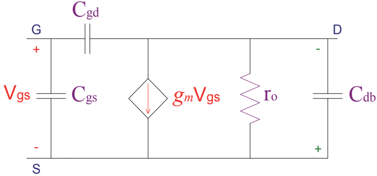
Fig. 15. Simplified high frequency model for source and substrate shorted.
