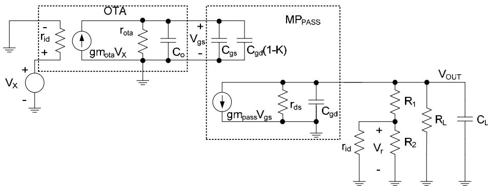
Fig. 8. Small signal equivalent circuit of the LVR
