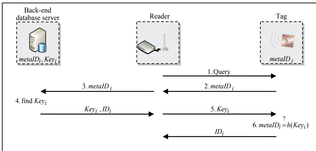
Fig. 13. Weis's hash-based access control scheme
