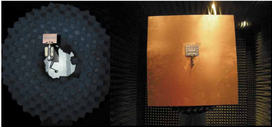
Fig. 8. Measurement set-up in anechoic chamber. Antenna measurement (left) and antenna on AMC over metallic plate measurement (right).
