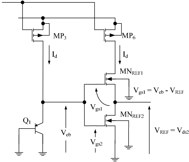
Fig. 14. The topology used to generate de voltage reference V_{REF}
