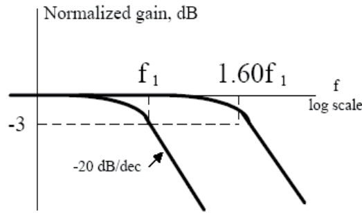
Fig. 8. Maximally flat frequency response.
