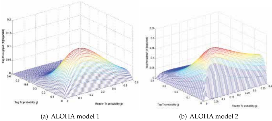
Fig. 2. Joint evaluation of ALOHA reader and tag anti-collision algorithms optimization
