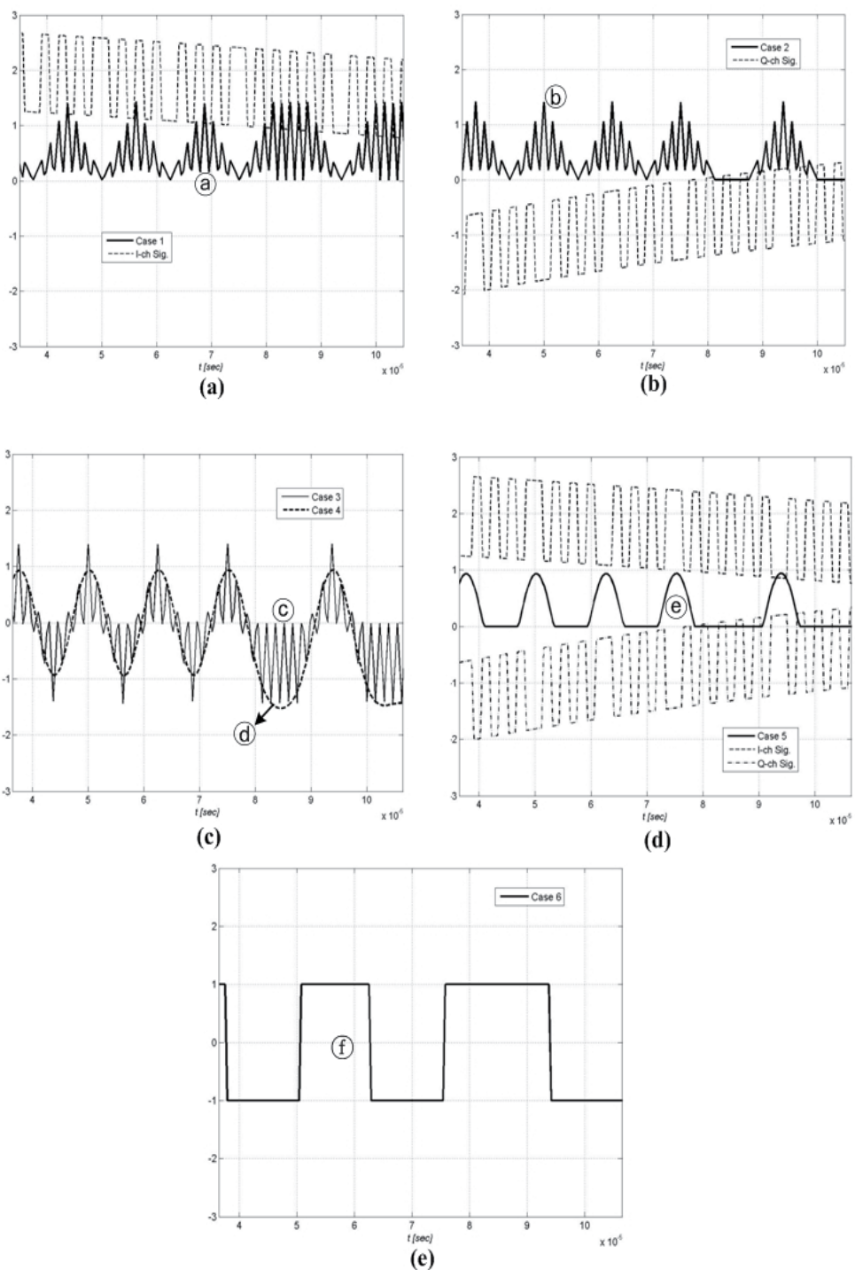
Fig. 11. Operation results of the proposed demodulation structure shown in Figure 3 (320kHz-Miller subcarrier signal with M = 4 )
