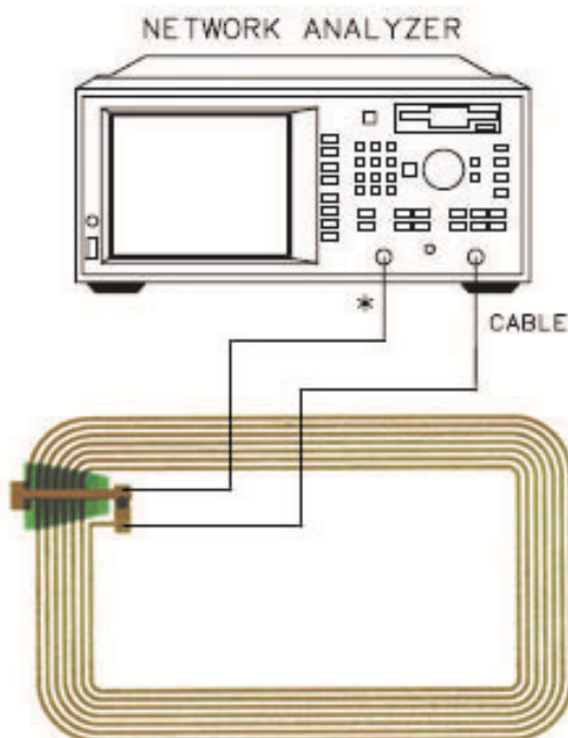
Fig. 3. The diagram of antenna impedance measurement
