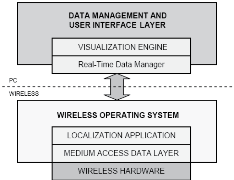
Fig. 7. Development software architecture
