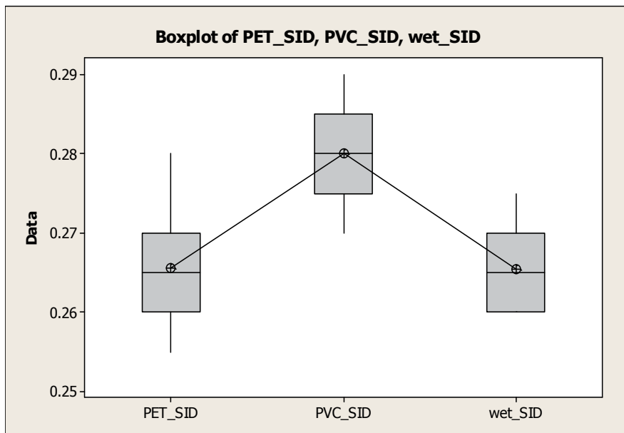
Fig. 4. Box plot of SID readings for the three substrates
