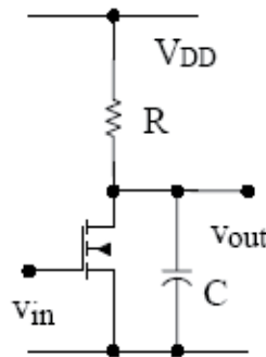
Fig. 4. Common-source stage with RC-load.
