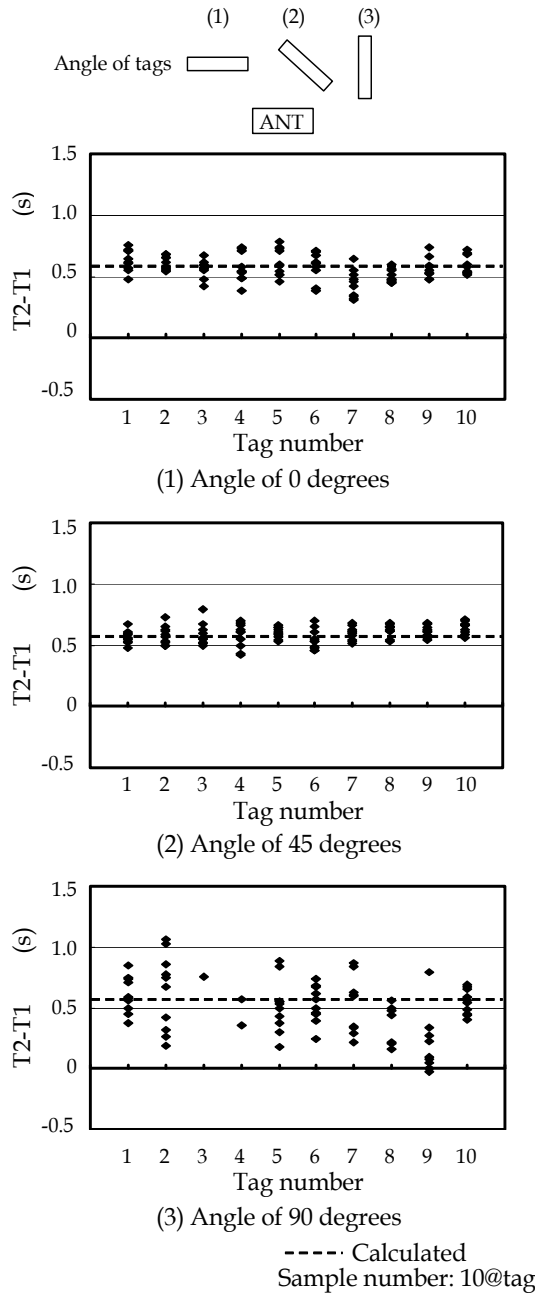
Fig. 14. Different time between two antennas
