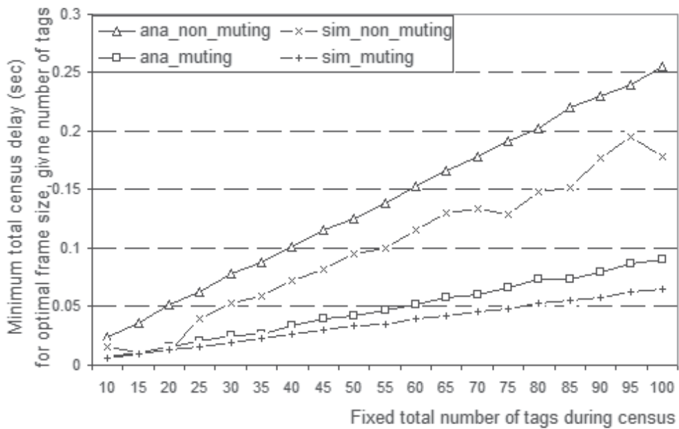
Fig. 19. Minimum Total Census Delay for Given Number of Tags
