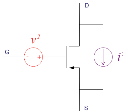
Fig. 17. Noise model of an n MOS transistor.
