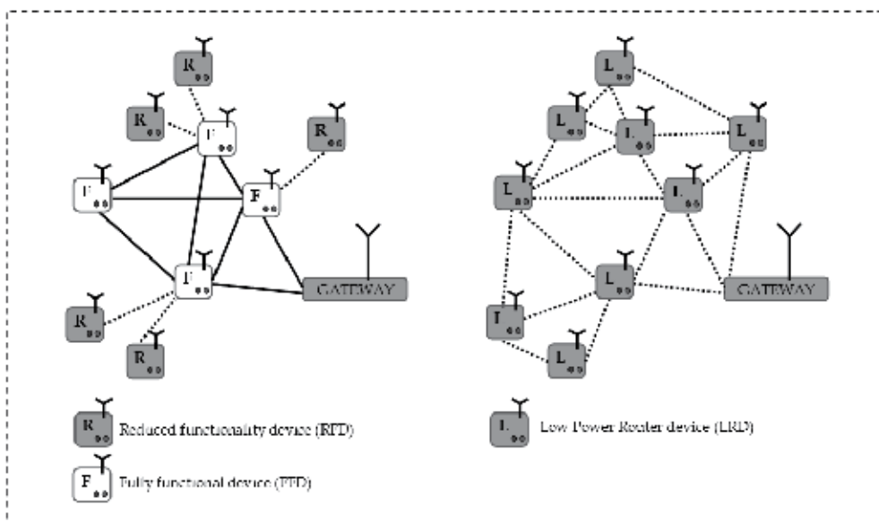
Fig. 5. The 2 types of network stacks PEAKNET™ Z (left) and PEAKNET™ LPR (right) (GreenPeak, 2010)
