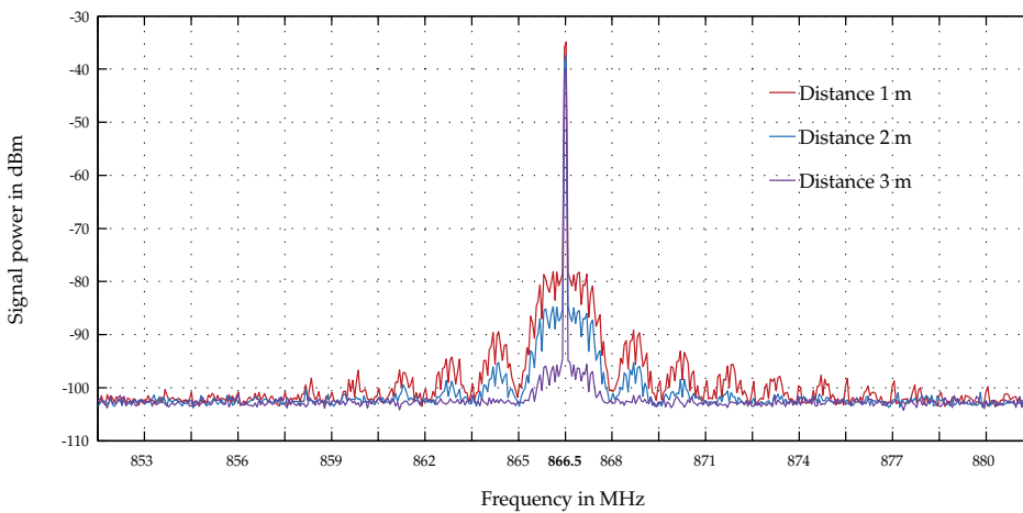
Fig. 17. Spectrum of backscattered signal from transponder
