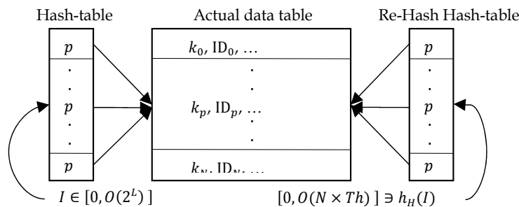
Fig. 1. The traditional Hash-table vs. basic Re-Hash hash-table
