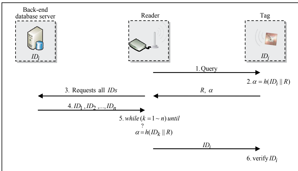
Fig. 11. Weis's randomized access control scheme
