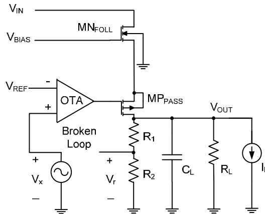
Fig. 7. Feedback broken to analyze the open loop gain.
