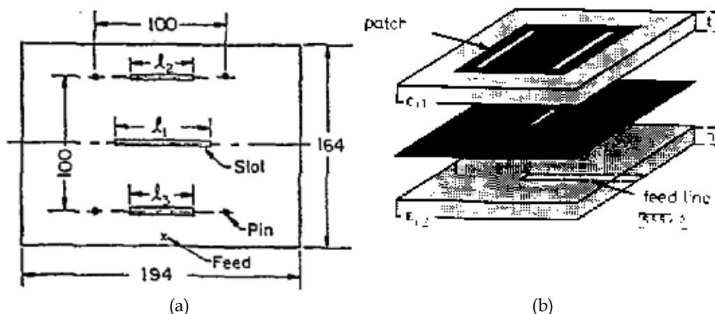
Fig. 21. (a) The microstrip antenna with shorting pins and slot, (b) Aperture coupled microstrip antenna for dual frequency operation (Wang & Lo 1984; Yazidi et al. 1993)
