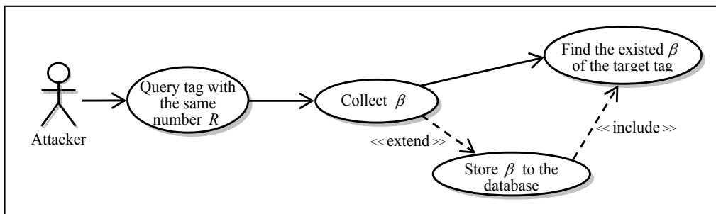
Fig. 20. The attack on LCAP
