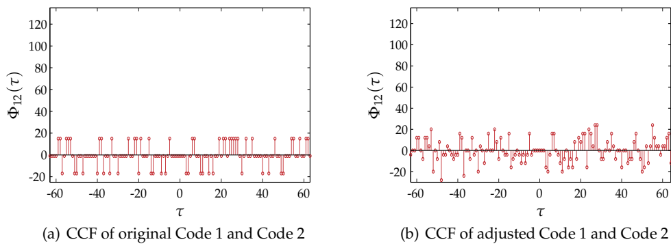
Fig. 15. CCF of both, original and adjusted Gold codes
