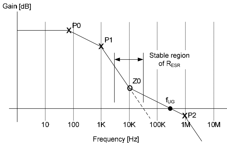
Fig. 5. Frequency response of a PMOS LDO regulator with external compensation capacitor PMOS based LDO.
