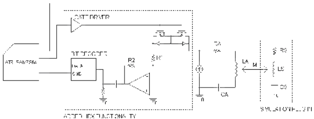
Fig. 23. Simulation plug-in added for test purposes to the current-driven reader
