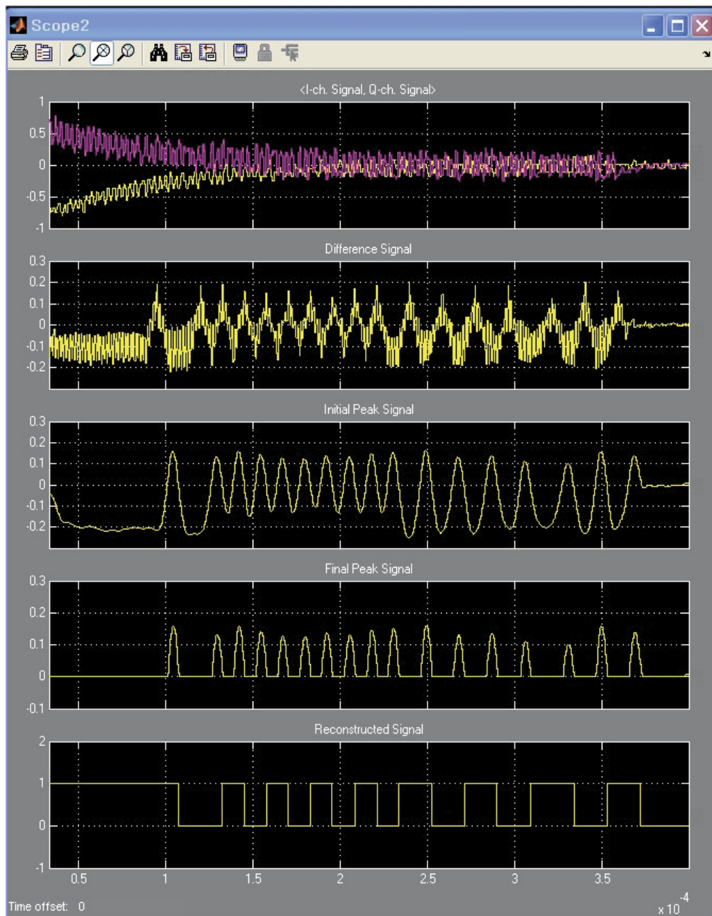
Fig. 14. Simulation result showing Black Box output through ISE simulator for the proposed demodulation structure
