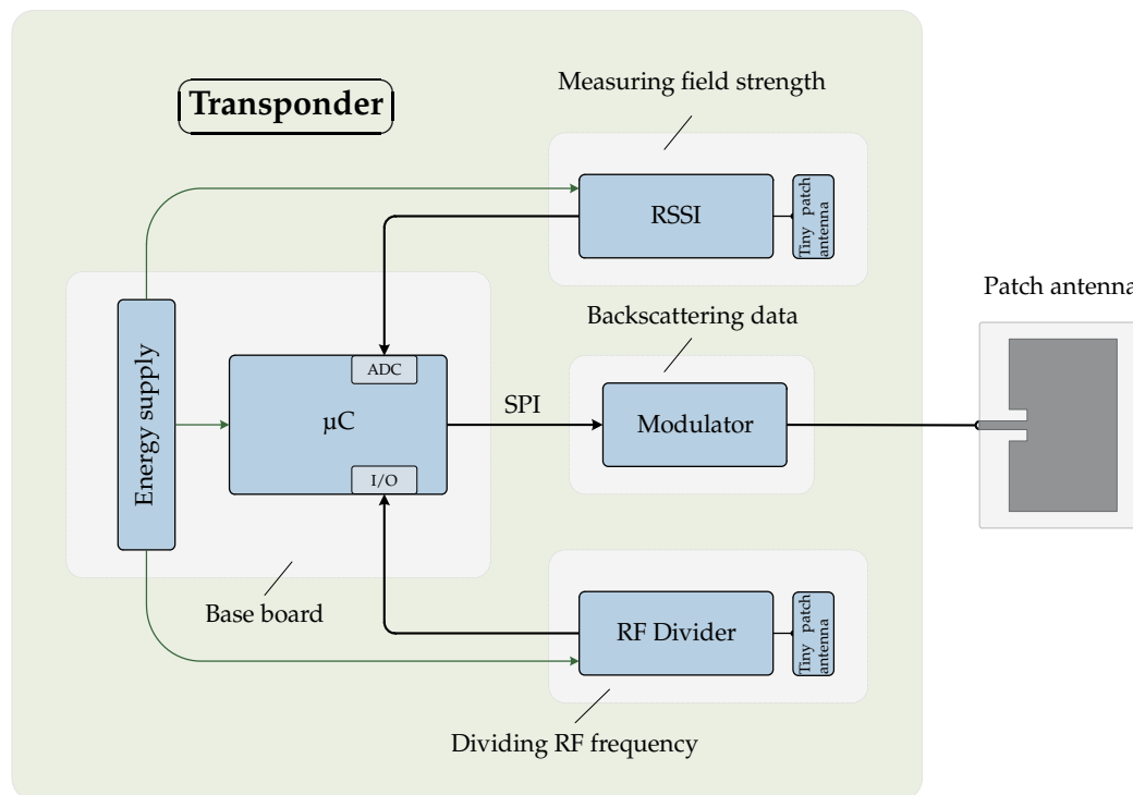
Fig. 9. Block diagram of semi-passive UHF RFID transponder with limited downlink capabilities
