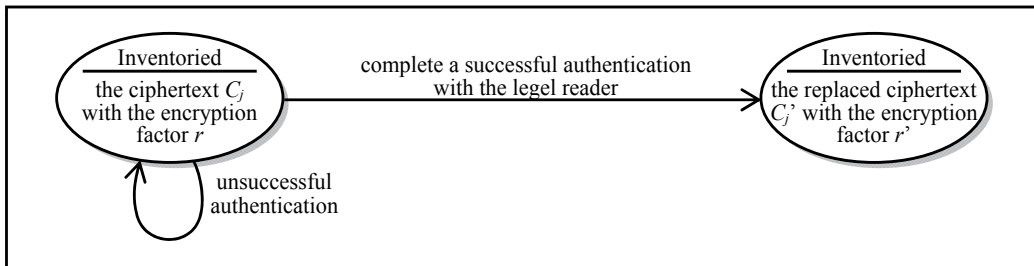
Fig. 7. Juels & Pappu’s re-encryption approach
