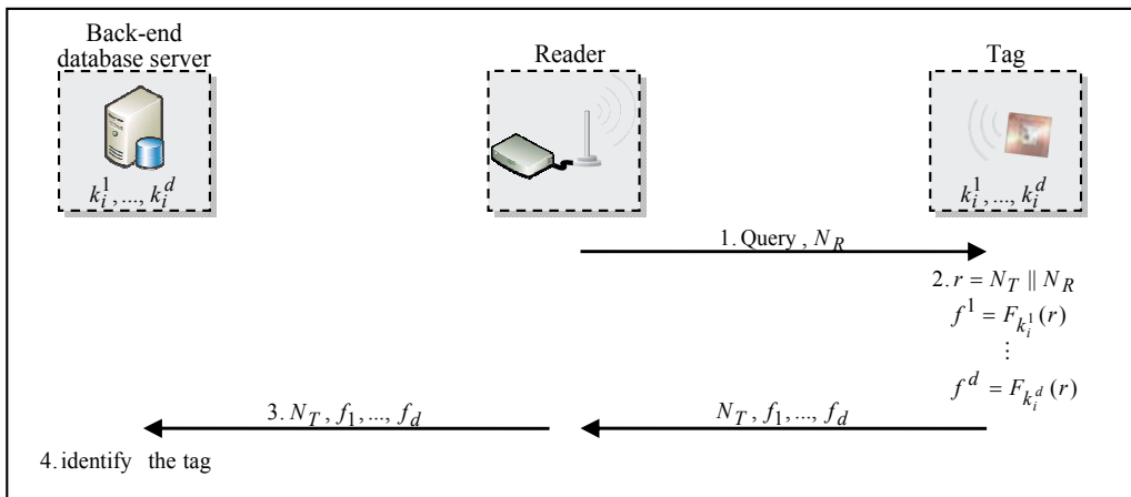
Fig. 22. Dimitriou's tree-based tag identification scheme
