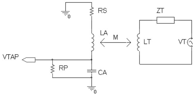
Fig. 6. Model for studying the effect of transients
