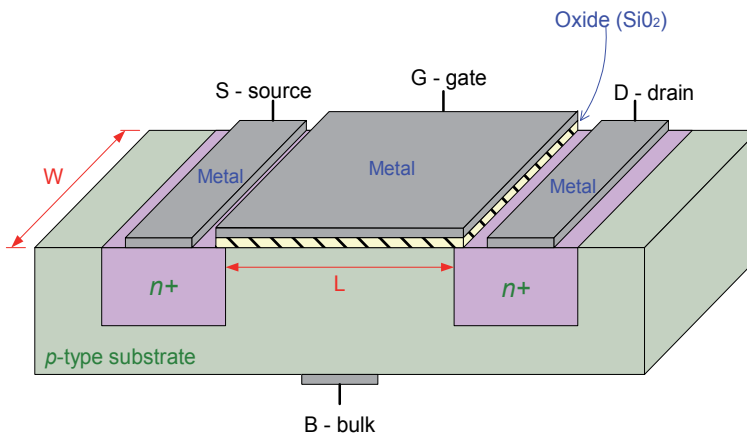
Fig. 1. Physical structure of an n MOS transistor.
