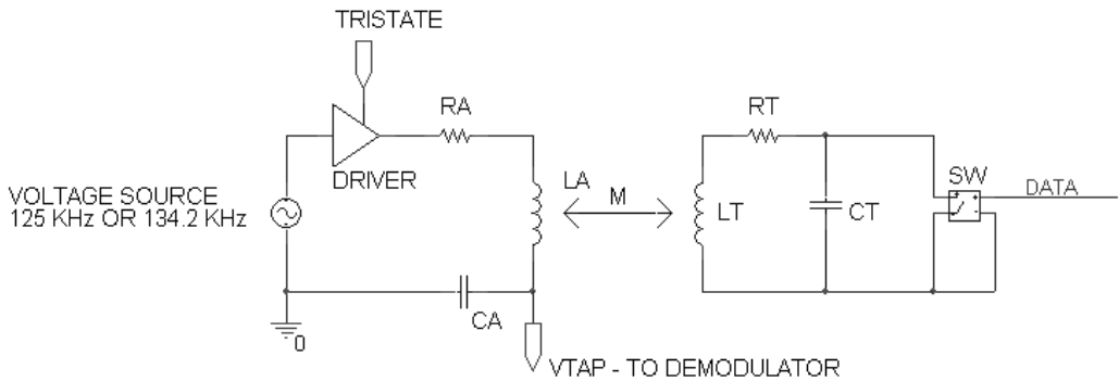
Fig. 1. Voltage-driven reader
