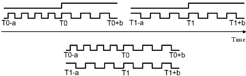
Fig. 20. Upper: input signals VIN_{12} and VIN_2 fed one after the other to the same system. The traces above the signals show the trigger provided by the simulator. Lower: signals superimposed for displaying overlap condition
