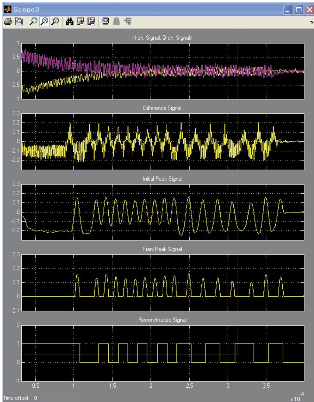
Fig. 15. Simulation result showing JTAG Co-Sim block output for the proposed demodulation structure
