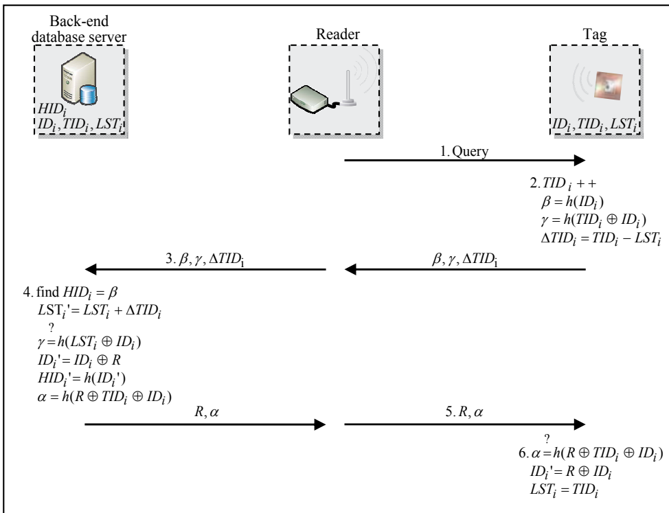
Fig. 17. Henrici & Muller's hash-based ID variation scheme
