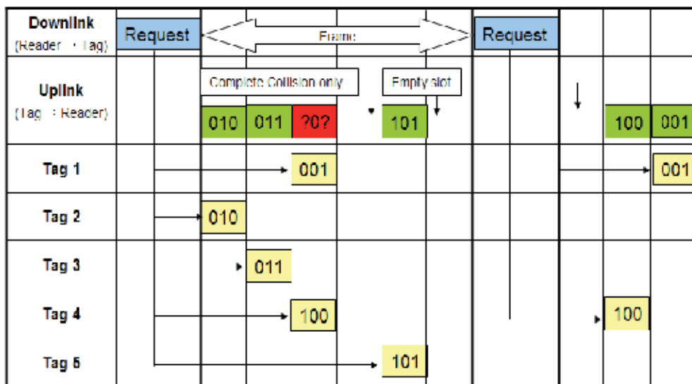
Fig. 3. Framed Slotted ALOHA Algorithms
