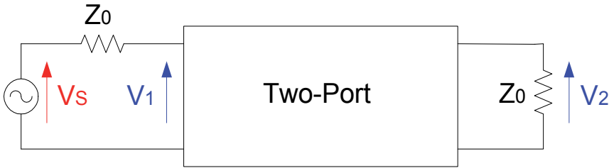
Fig. 8. Circuit topology used to measure S-Parameters.
