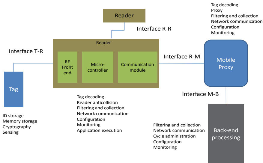
Fig. 1. Reference RFID system architecture
