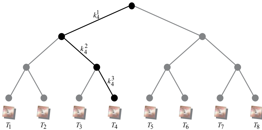
Fig. 21. A binary key tree with eight tags
