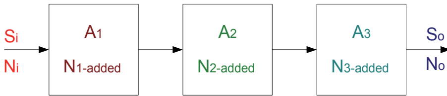
Fig. 13. Cascade amplifying system.
