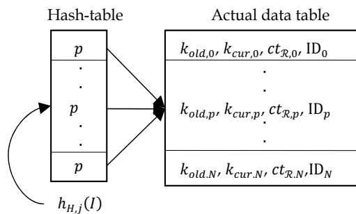
Fig. 2. The 2-level Database Structure with a Re-Hash Hash-table
