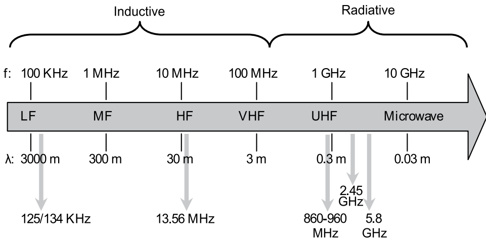
Fig. 4. Frequency-ranges used for RFID-systems
