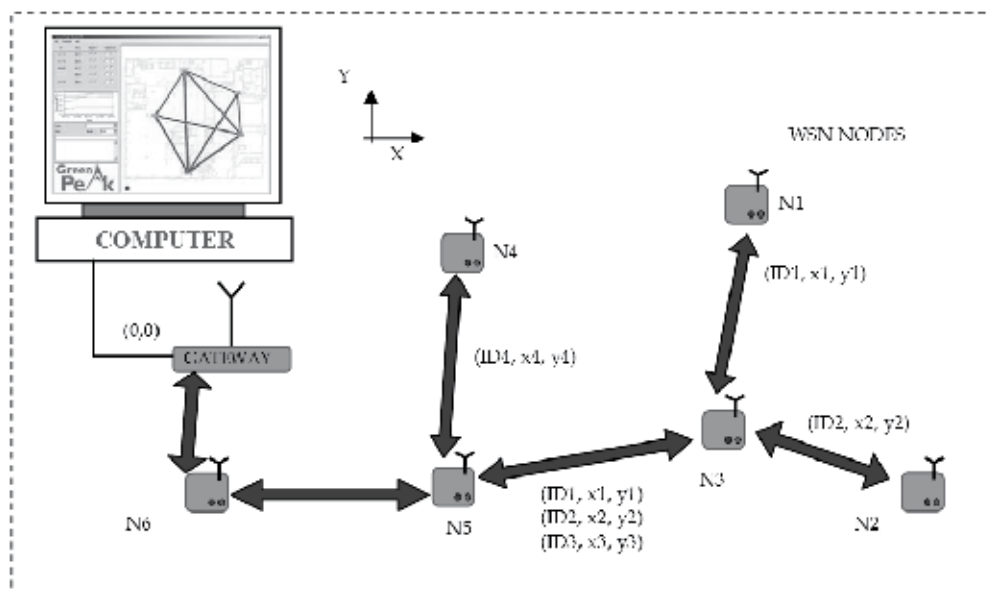
Fig. 1. Typical third generation RFID locating network overview
