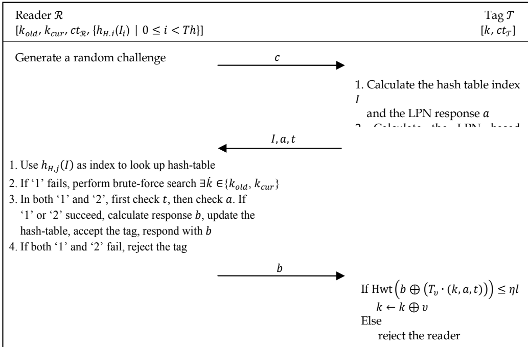
Fig. 3. The Proposed F-HB + Protocol
