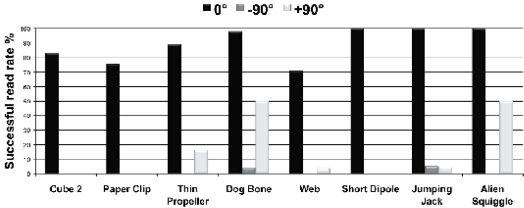
Fig. 11. A performance comparison on the items line by varying tag type and the tag-reader antenna misalignment in presence of liquids and metals (ophthalmic solution).
