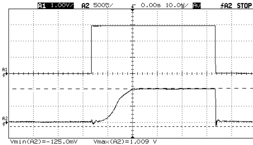
Fig. 28. LVR step response indicating a BIBO system.
