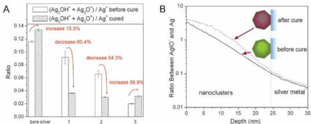
Fig. 5. TOF-SIMS analyses of the silver sputtered silicon wafer samples. A) Silver sputtered silicon wafers after treatment of different concentration of iodine solutions. (The cured samples refer to those experienced a curing and post-washing process prior to this analysis.) Conditions: 1. Ag : I = 100 : 0.2; 2. Ag : I = 100 : 0.4; 3. Ag : I = 100 : 20. B) Depth profile of the surface-modified sputtered wafer sample (treatment condition: Ag : I = 100 : 20; y -axis in logarithmic scale). (Copyright © 2010 WILEY-VCH)
