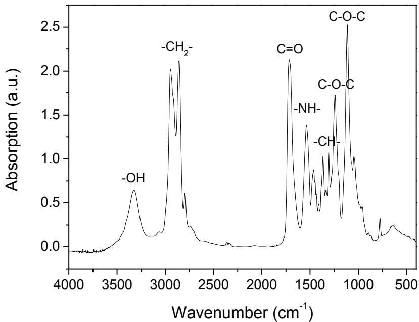
Fig. 13. FT-IR spectrum of the dried film of the water-borne PU.
