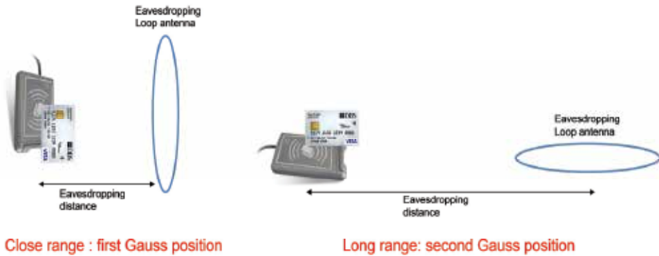
Fig. 3. Antennas positions for the two Gauss positions
