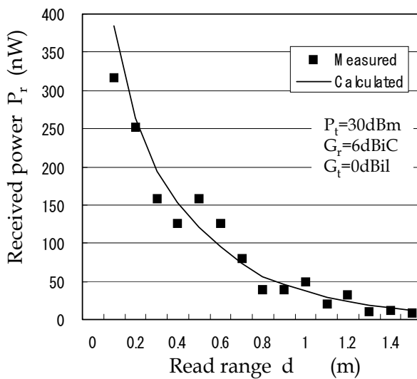
Fig. 4. Read range vs Received power
