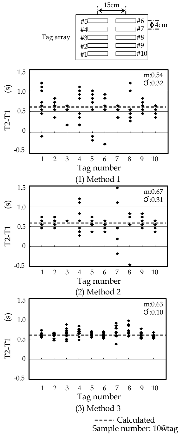
Fig. 8. Different time between two antennas
