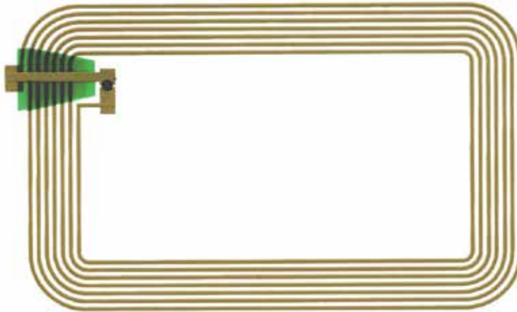
Fig. 2. Antenna design (13.56MHz, 45mm x 76mm) for the study
