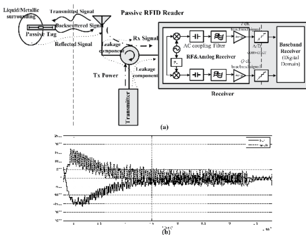
Fig. 1. Description of leakage components (a) and the corresponding DC-offset phenomenon (b) in a passive RFID communication environment
