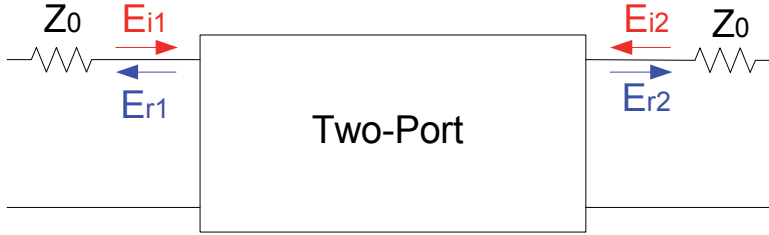
Fig. 7. Two port circuit representation for S-parameters.
