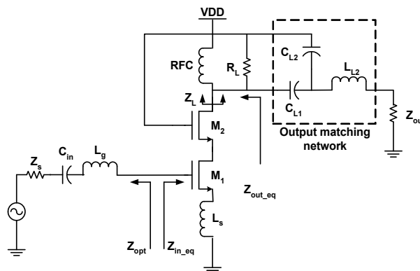
Fig. 9. Overall LNA architecture.
