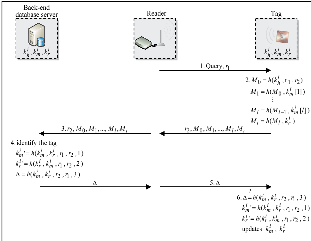
Fig. 24. Wang et al.'s tree-based authentication scheme
