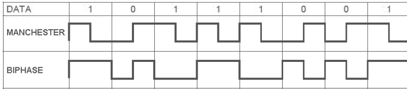
Fig. 14. Methods of bit encoding. Traces show the digital signal on the LOADMOD line.
