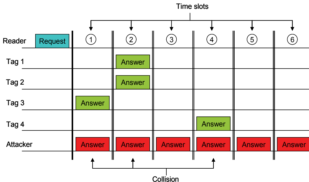
Fig. 17. Blocking protocol for Aloha method
