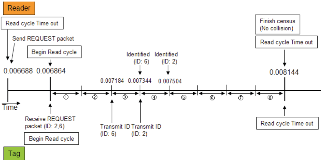
(e) Fifth Read Cycle of the Simulation
