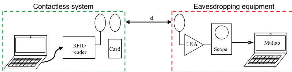
Fig. 4. Eavesdropping bench test
