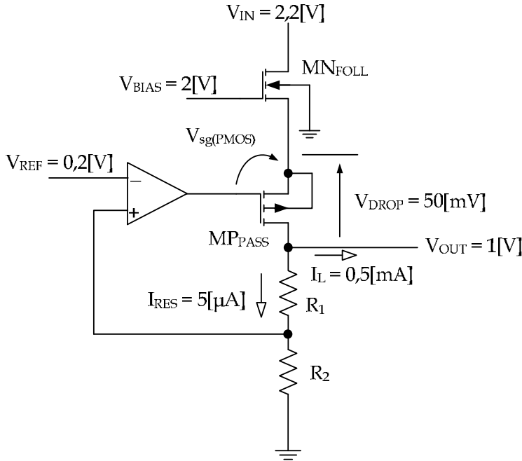
Fig. 17. Circuit used to optimize the MN_{FOLL} geometric aspect ratio.
