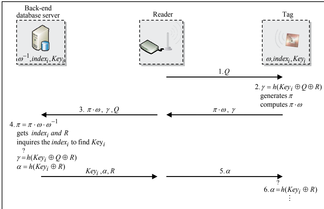
Fig. 25. Chen’s indefinite-indexed access control scheme
