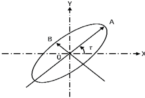
Fig. 9. Elliptically polarized wave
