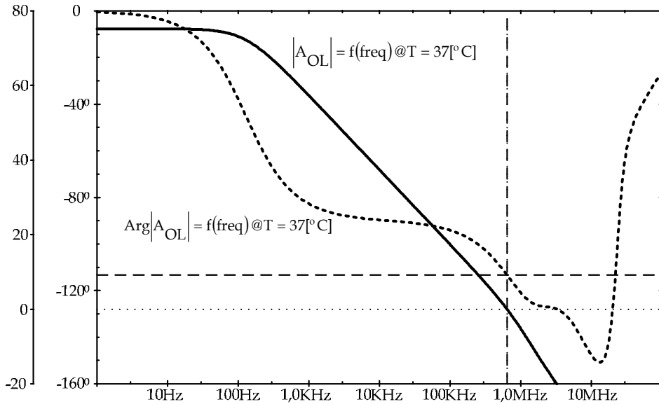
Fig. 22. OTA Frequency response.
