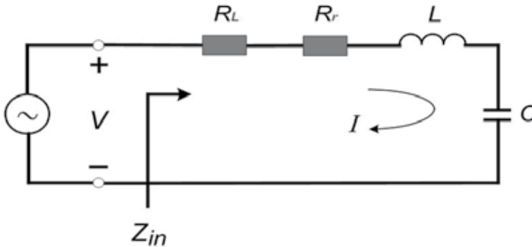
Fig. 10. Equivalent circuit of antenna
