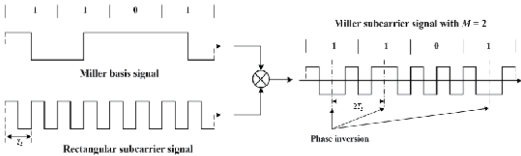
Fig. 2. Configuration of the Miller subcarrier signal with M = 2
