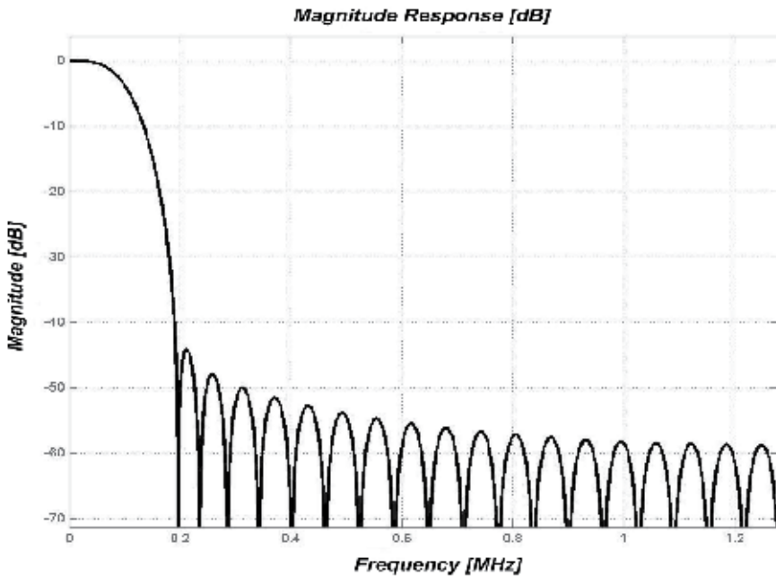
Fig. 8. The magnitude response of the designed 39th order low-pass filter for the generation of the initial peak signal
