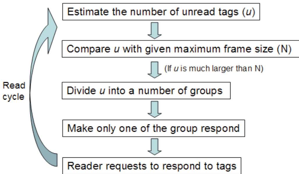
Fig. 12. Read Cycle of EDFSA Algorithm
