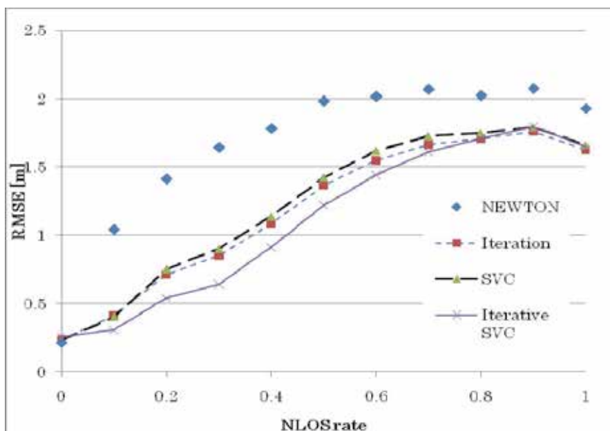
Fig. 10. RMSE evaluation changing NLOS rate
