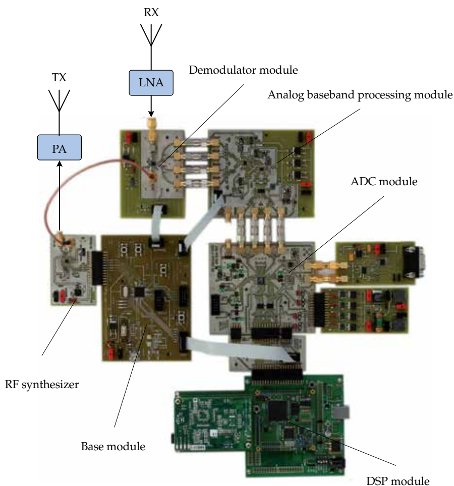
Fig. 5. Architecture of CDMA-based RFID reader
