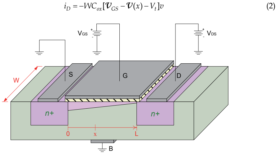
Fig. 9. Biasing of an nMOS.
