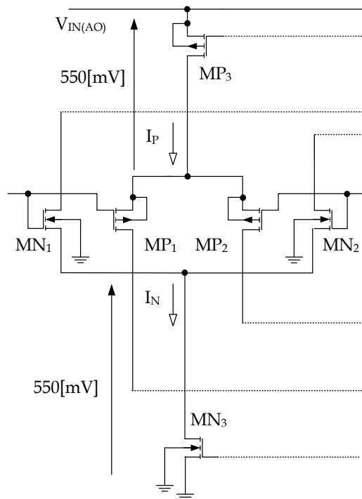
Fig. 20. NMOS and PMOS differential input pairs.
