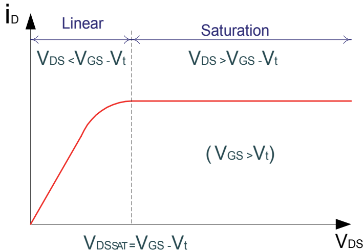
Fig. 8. Operation condition of an n MOS transistor.
