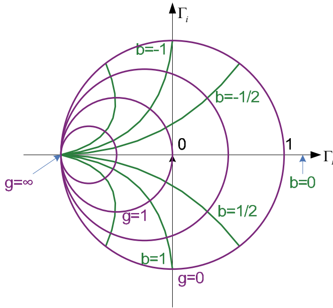
Fig. 5. Admittance Smithchart.
