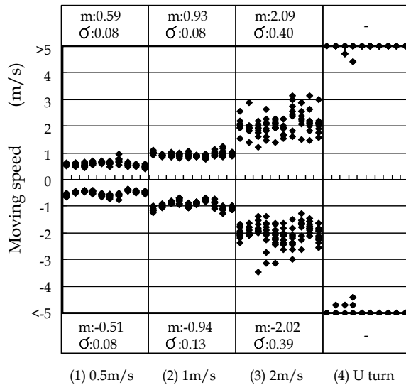
Fig. 13. Measurement results of moving speed
