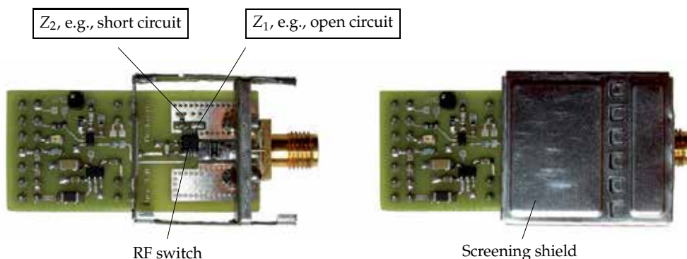
Fig. 11. Backscatter modulator
