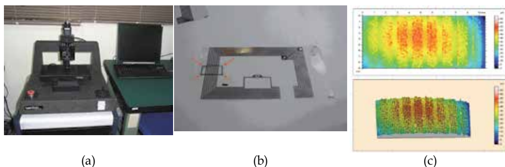
Fig. 9. (a) A confocal laser scanning microscope (b) Antenna film under measurement (c) measured thickness distribution
