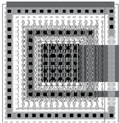
Fig. 26. PNP vertical bipolar transistor example.
