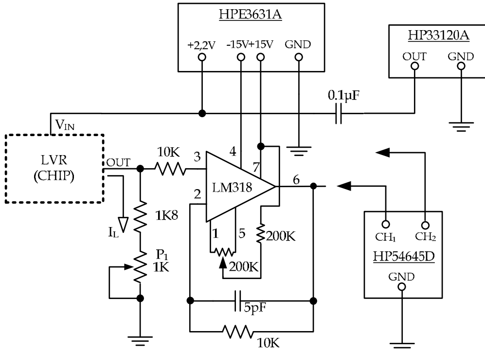
Fig. 27. The test structure to measure the LVR parameters.
