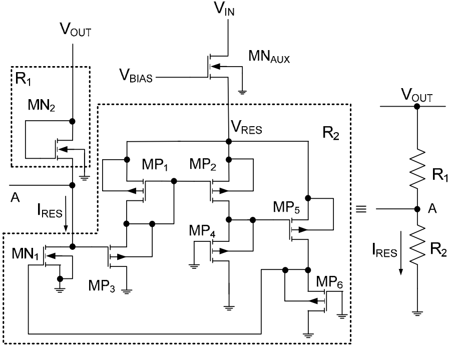
Fig. 9. Sampler Circuit for the LVR.
