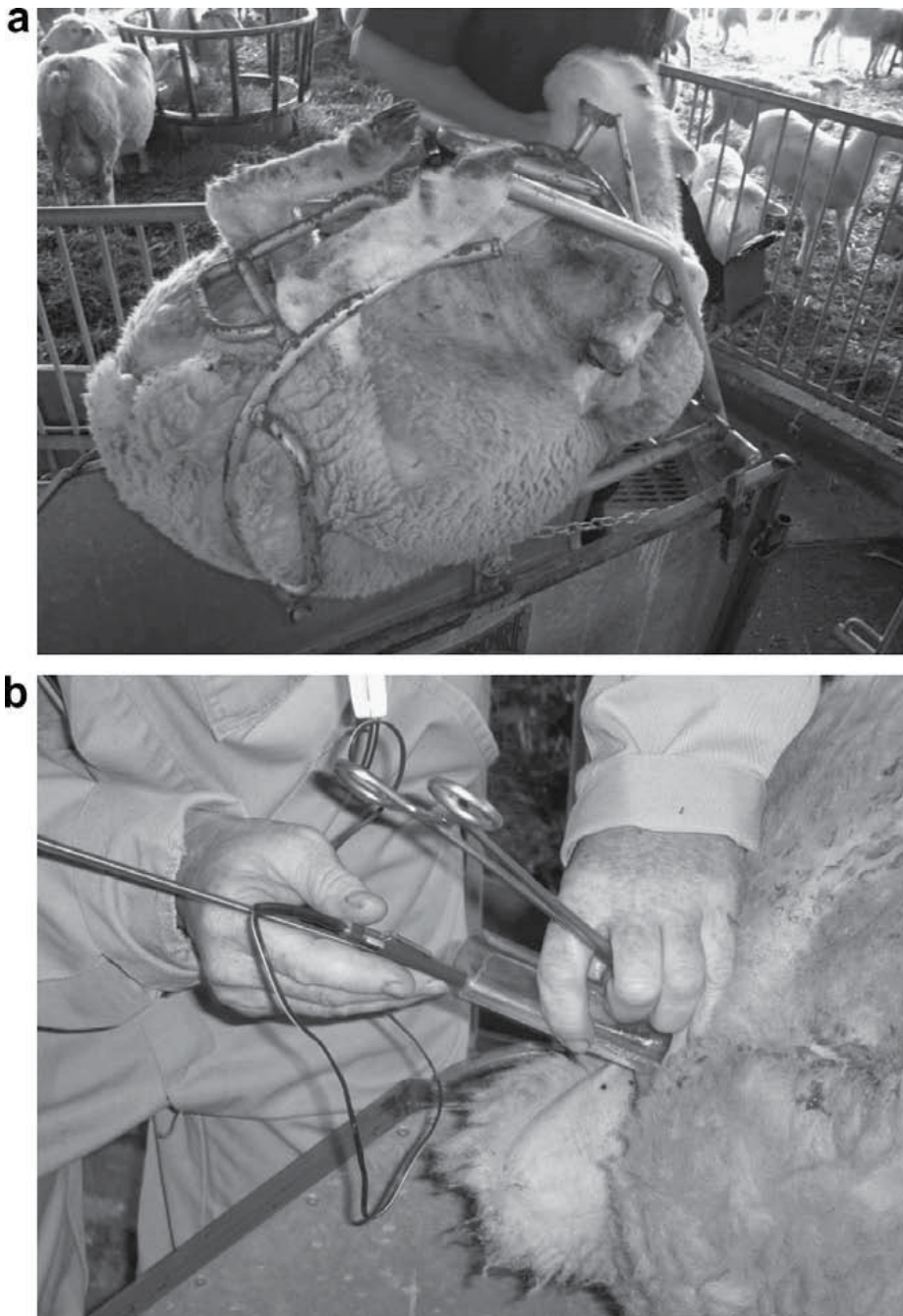
Fig. 2. The Guelph TCAI System: (a) fetal-like positioning of ewes in dorsal recumbency; (b) a plexiglass speculum with light source is inserted into the vagina and forceps are used to grab the cervix near the os and retract it. Subsequently, a bent-tipped and preloaded insemination gun is introduced and manipulated through the cervix to deposit semen. From Candappa et al., 2009.
