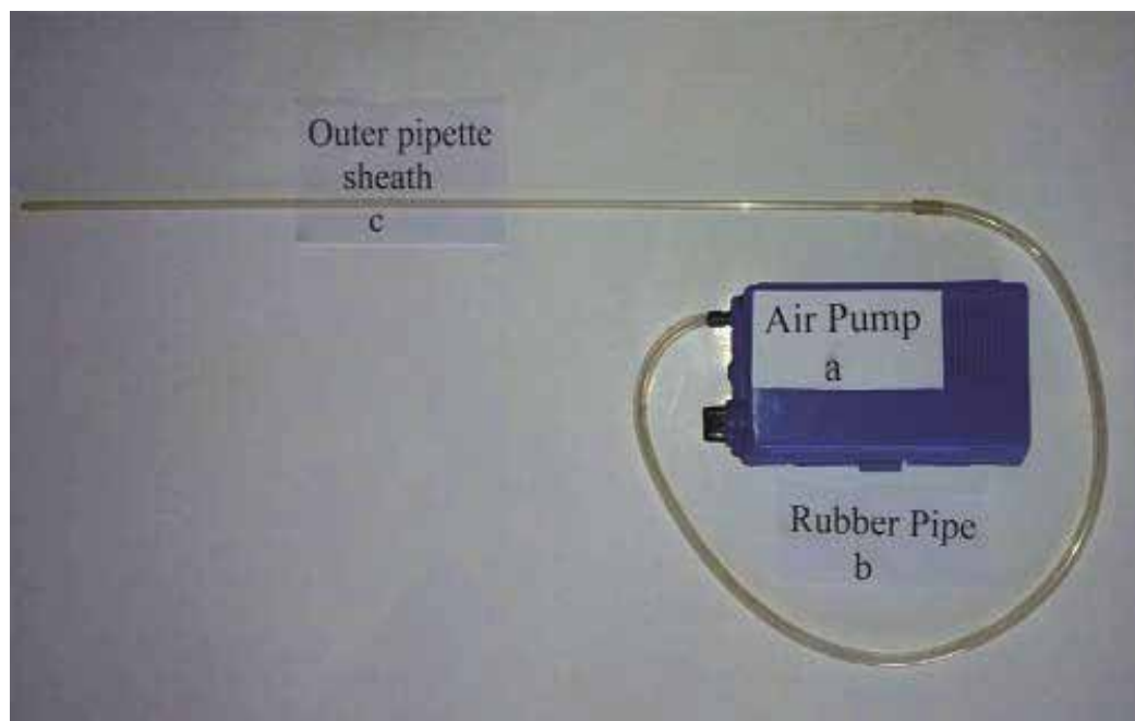
Fig. 4. Artificial insemination equipment of APCA method; (A) Air pump, (B) Rubber pipe, (C) a stainless steel outer pipette sheath used in cattle AI. From Aral et al., 2010.
