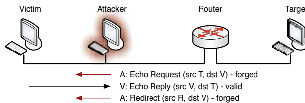
Fig. 11. ICMP Redirect attack
