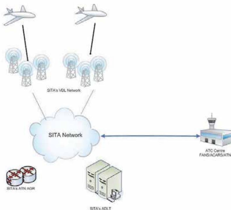
Fig. 3. Overview of SITA ATN architecture.
