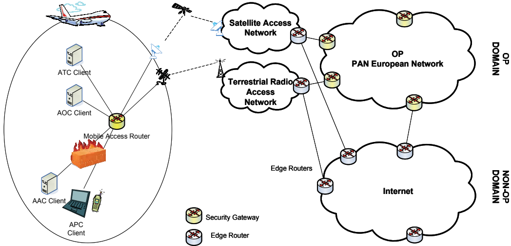
Fig. 8. Full integration of services, links and networks.
