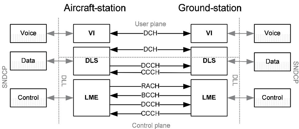
Fig. 2. L- DACS 1 logical channel structure.
