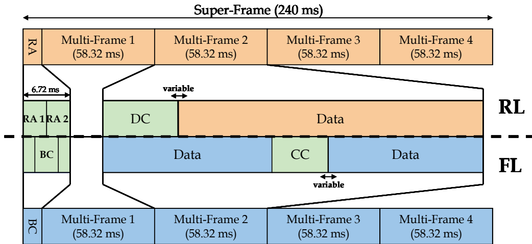
Fig. 11. Super-Frame Structure.
