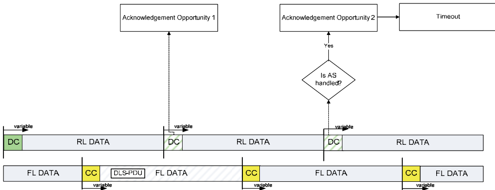
Fig. 11. LDACS1 FL DLS retransmission timer.
