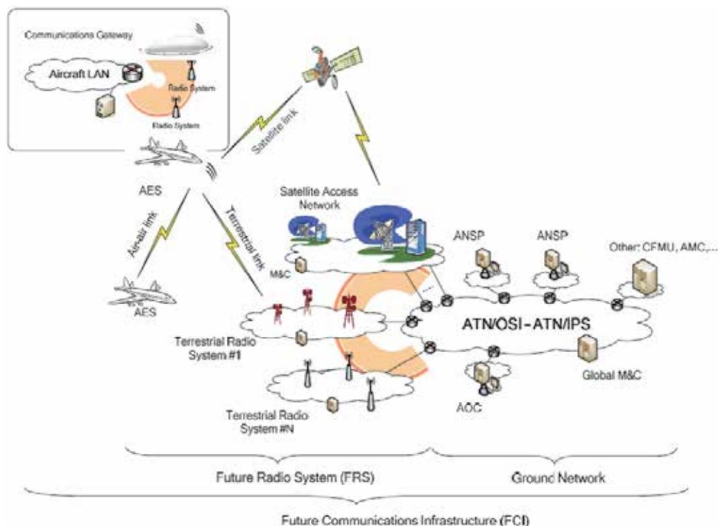
Fig. 12. Future ATM network architecture integrating the satellite access network as presented in the ICOS ESA project.
