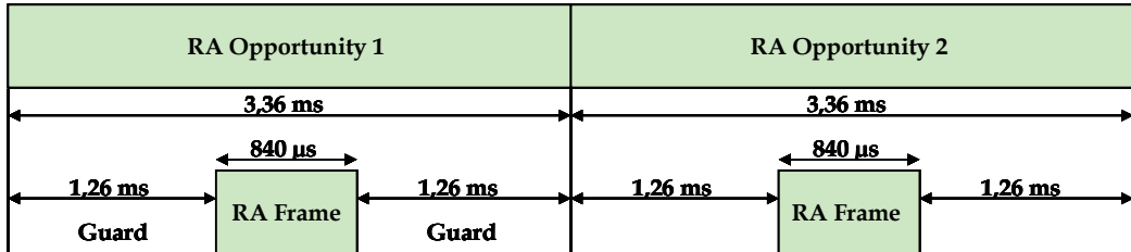
Fig. 8. Random access opportunities.
