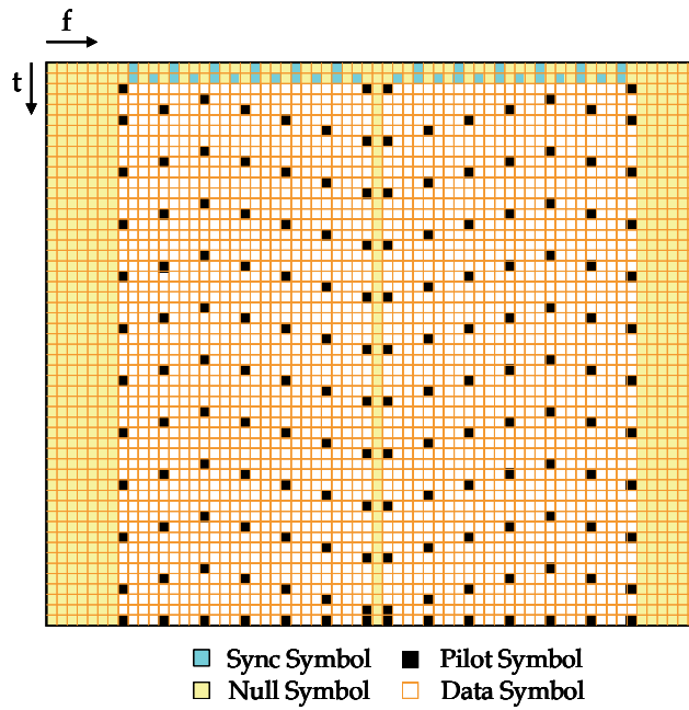
Fig. 3. Structure of a FL Data/CC frame.
