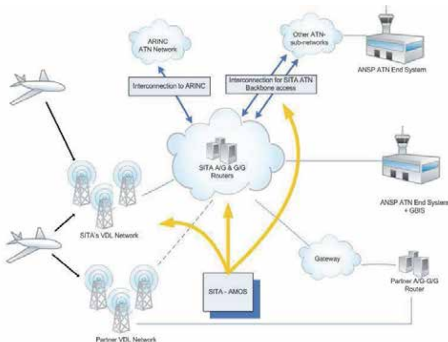
Fig. 4. Overview of SITA ATN architecture – interface with other parties.
