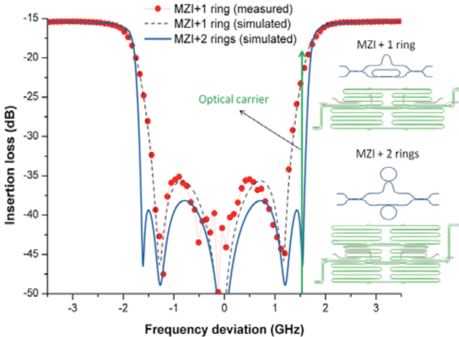
Fig. 17. Optical sideband filters measured and simulated responses. In the fitting a waveguide propagation loss of 0.2 dB/cm is used.
