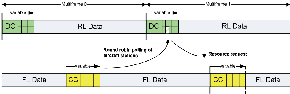
Fig. 5. RL resource request over the DCCH.
