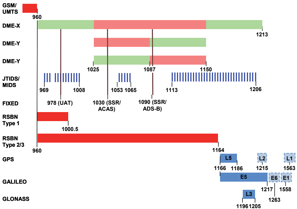
Fig. 1. Current L-band usage (SESAR JU, 2011).
