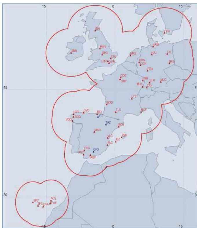
Fig. 2. SITA VDL2 network in Europe.
