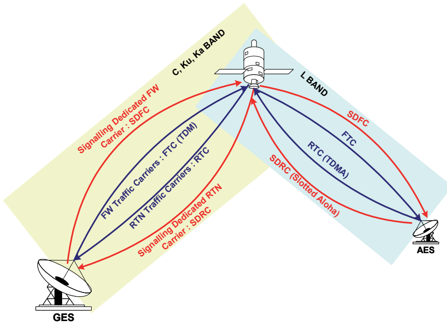
Fig. 6. Typical channel allocation.
