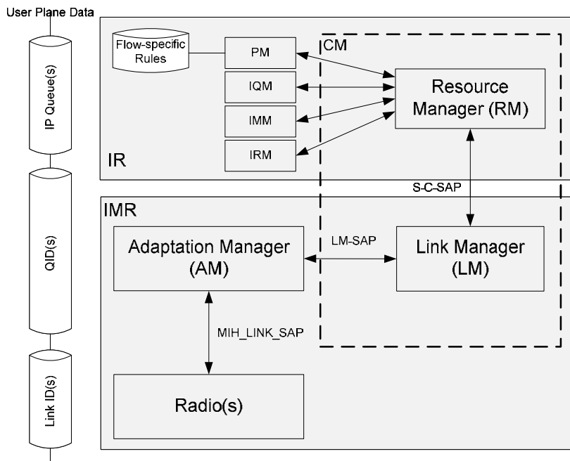
Fig. 7. Cross-layer collaborative connection management.
