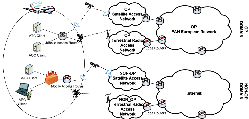
Fig. 6. Service domain separation for near future.
