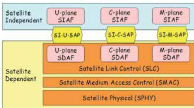
Fig. 2. SI-SAP expanded reference model (ETSI, 2007).
