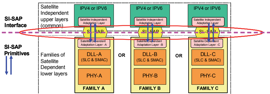
Fig. 3. ETSI BSM protocol architecture and SI-SAP interface definition.
