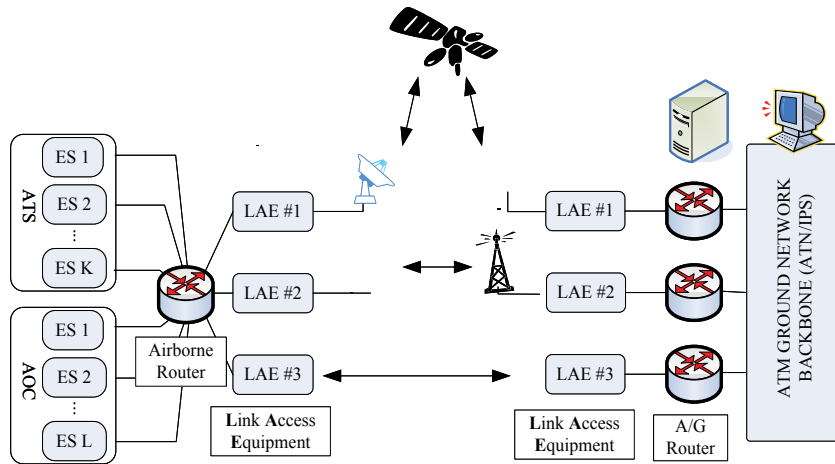
Fig. 2. System architecture
