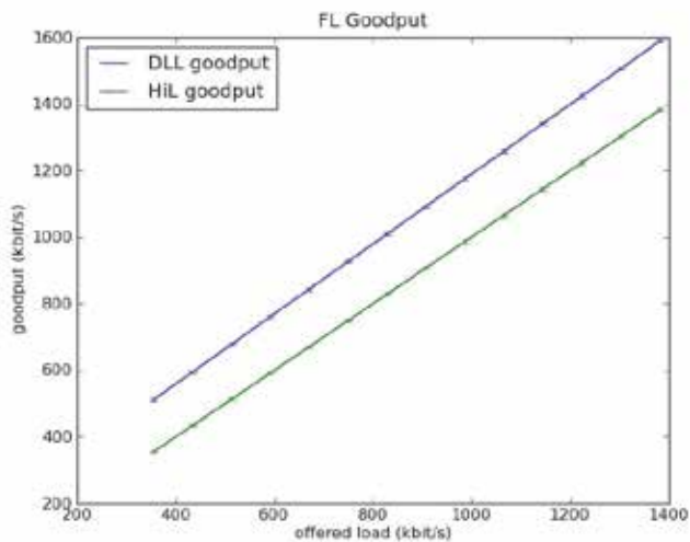
Fig. 22. FL goodput - scenario LOAD.
