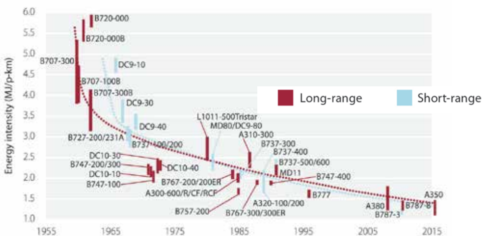
Fig. 3. Energy intensity of aircraft. The range of points for each aircraft reflects varying configurations; connected dots show estimated trends for short and long-range aircraft. (Source: IEA).
