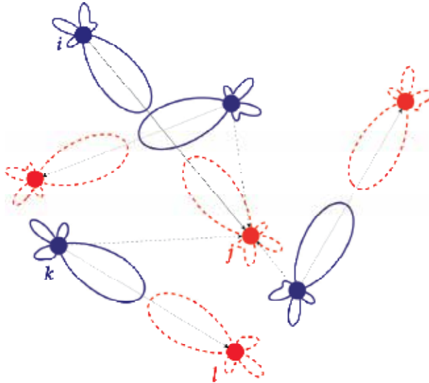
Fig. 9. Example network illustrating our SIR-based interference model (solid lines represent communication links, dotted lines represent interference links).
