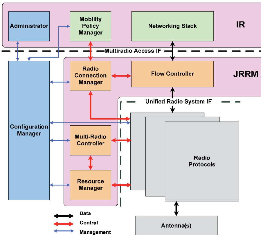
Fig. 5. The SDR-enabled RRM Functional Architecture for the SANDRA Terminal.
