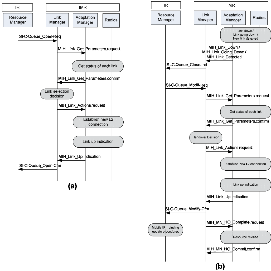
Fig. 8. (a) General session establishment and (b) mobile controlled handover.
