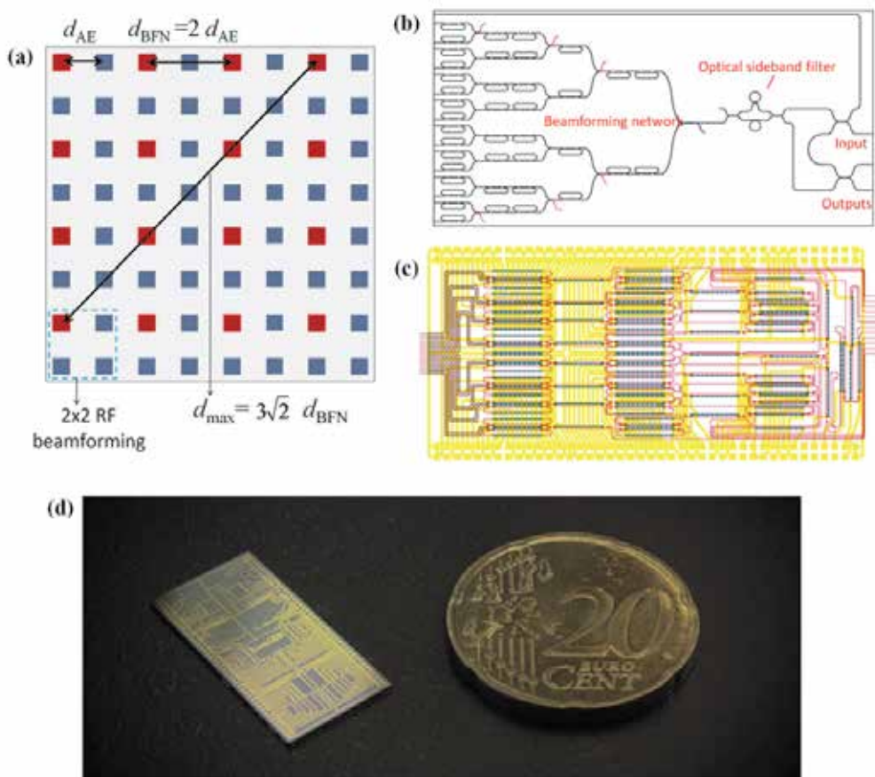
Fig. 16. (a) An antenna tile consisting of 64 AEs. (b) Functional design of the 16x1 photonic BFN showing the ORR delay elements and the sideband filter. (c) Chip layout of the BFN showing the optical waveguides, the heaters layout and the electrical wiring. The chip dimension is 0.7 cm x 2.2 cm. (d) The 16x1 photonic BFN chip pictured with a 20 cent Euro coin for size comparison.
