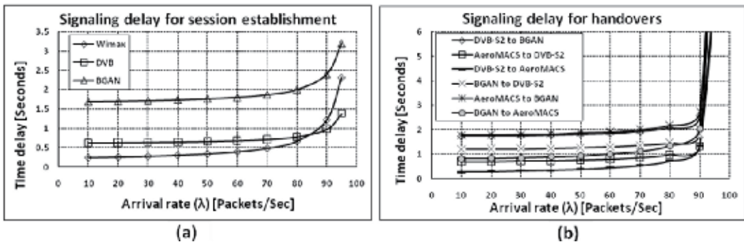
Fig. 9. (a) Signalling delay for new session establishment on different technologies and (b) Signalling delay to handover to different technologies.
