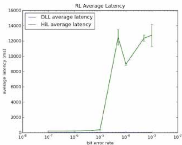
Fig. 21. RL avg. latency - scenario BER.
