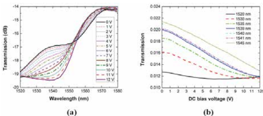
Fig. 13. DC characterisation results on a single pass (transmissive) EAM with an aperture of 100\ \mu\text{m} . The input optical power to the modulator is set at 0 dBm. (a) The transmission through the modulator (in decibels) as a function of the optical wavelength for different reverse bias voltages. (b) Transmission (in linear scale) as a function of the reverse bias voltage, for various optical wavelengths from 1520 nm to 1545 nm
