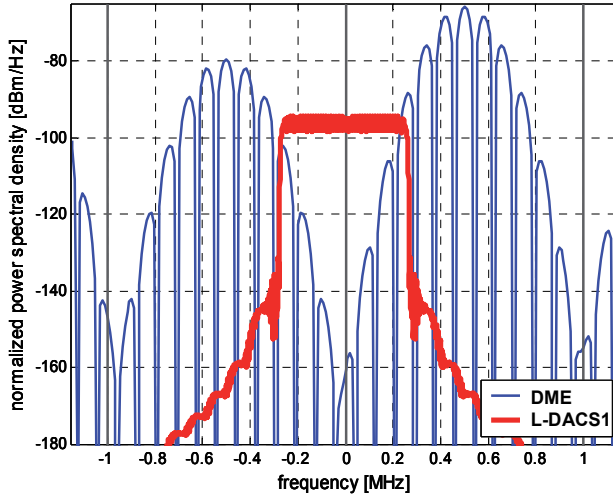
Fig. 2. An example of LDACS1 spectrum and DME interference in the inlay deployment scenario.
