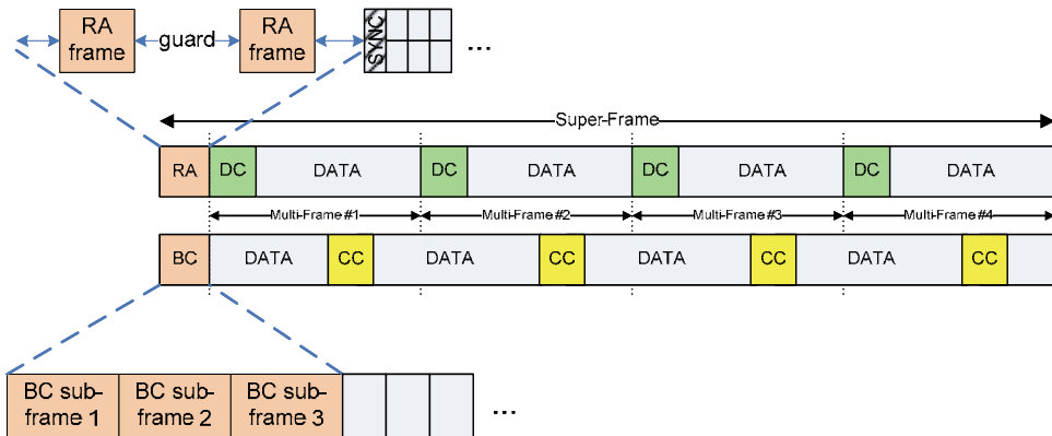
Fig. 3. LDACS1 super-frame structure.
