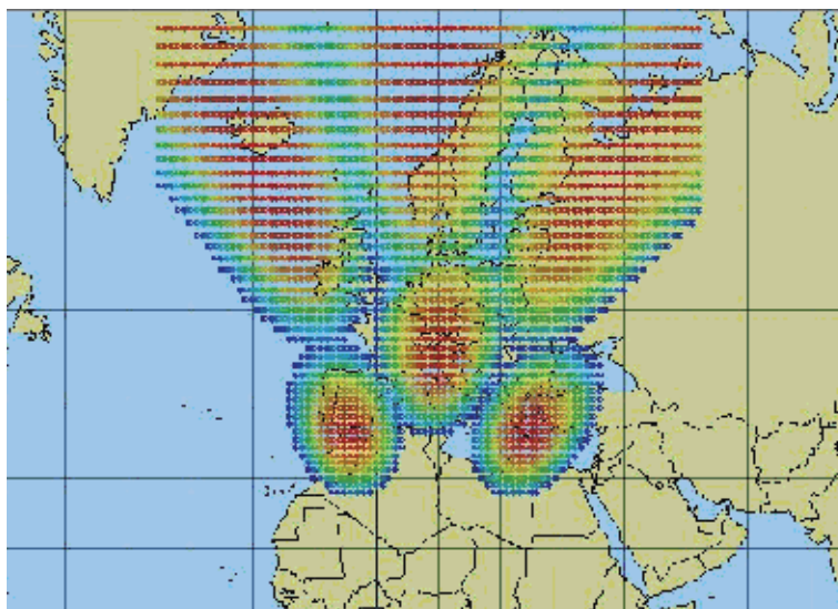
Fig. 7. Illustration of the interest of using spot beams in satellite system. In this example, when the overall available spectrum is limited, the gain provided by frequency reuse between non-adjacent spots can be visually verified.
