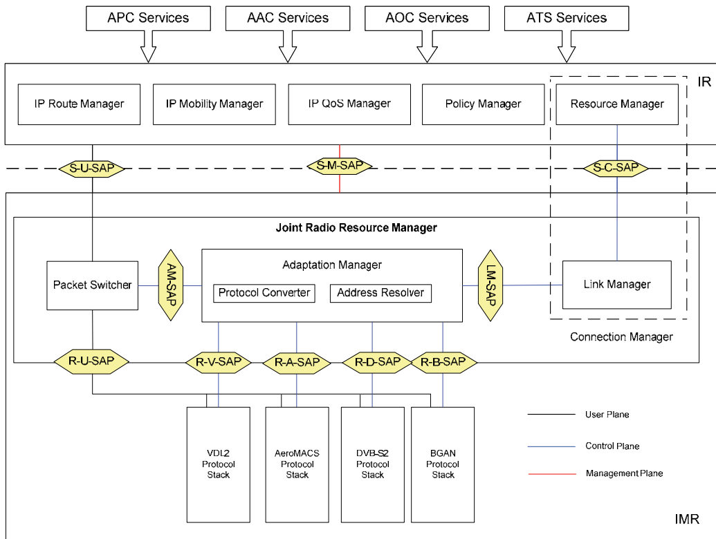
Fig. 6. CRRM architecture.
