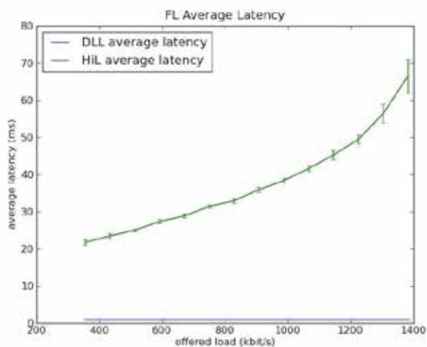
Fig. 24. FL avg. latency - scenario LOAD.
