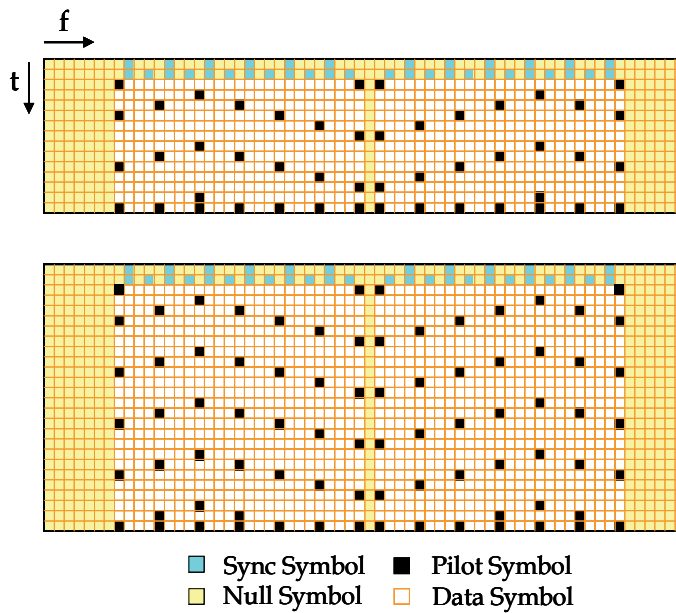
Fig. 4. Structure of BC1 and BC3 sub-frames (above) and BC2 sub-frame (below).
