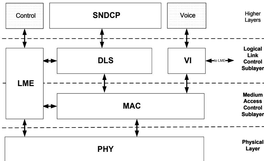
Fig. 1. LDACS1 protocol stack.
