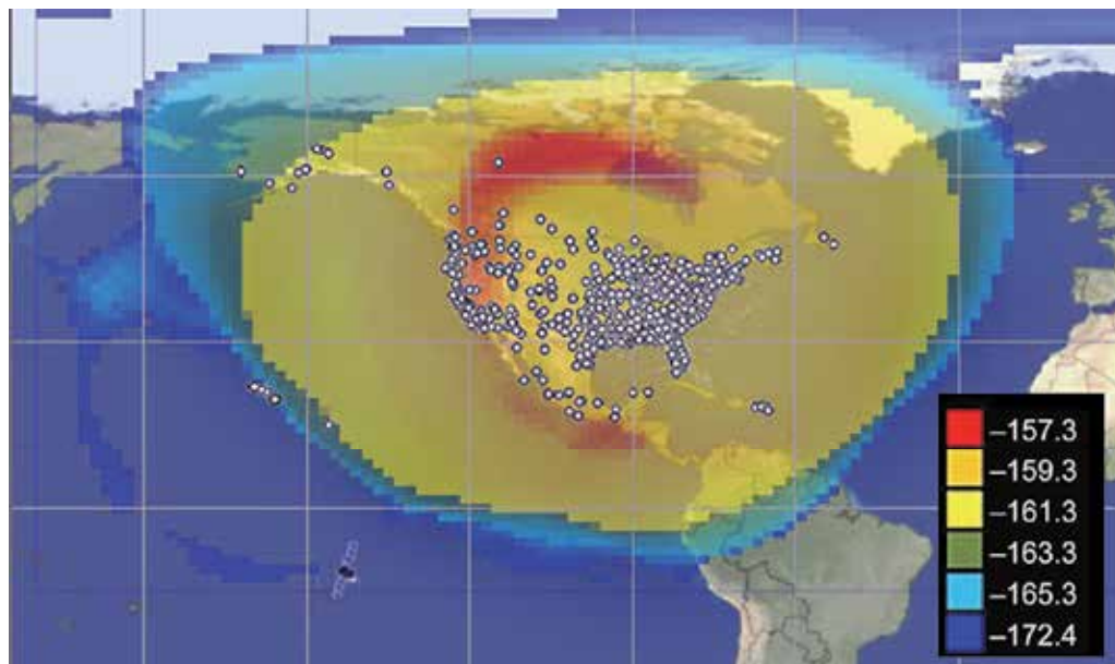
Fig. 6. Modeled interference power distribution from 757 AeroMACS-equipped airports in North America as seen at a Globalstar receiver orbiting 1414 m above the Earth's surface.
