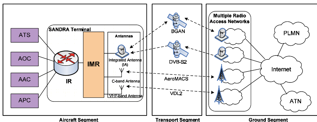
Fig. 4. SANDRA network architecture.
