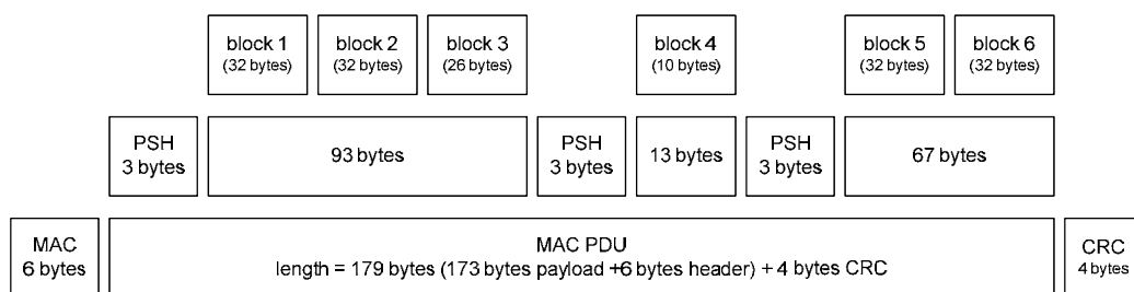
Fig. 6. Example MAC PDU - MAC packing.
