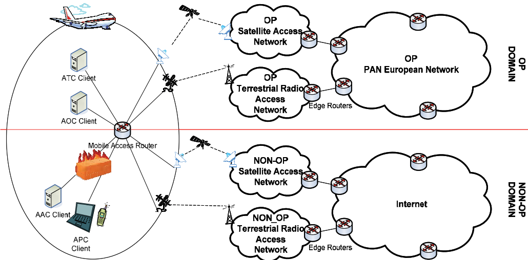
Fig. 7. Service integration in Mobile Access Router, separation at network domain level.
