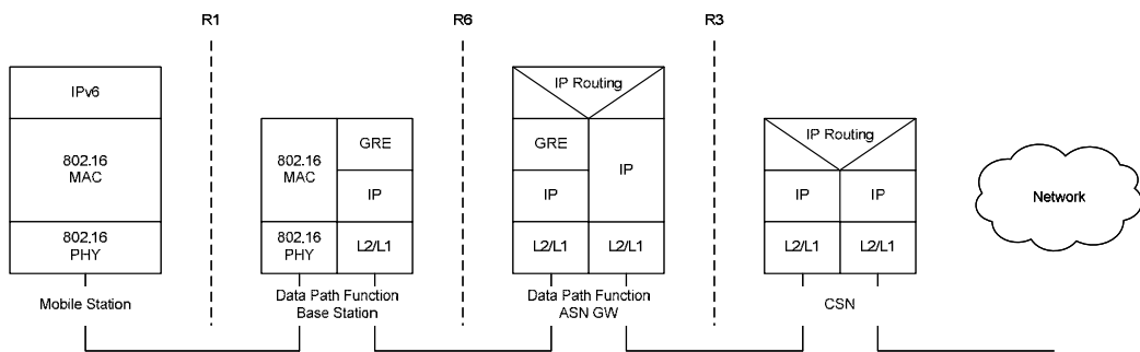
Fig. 13. Protocol stacks of different entities, considering an IP point to point link model.
