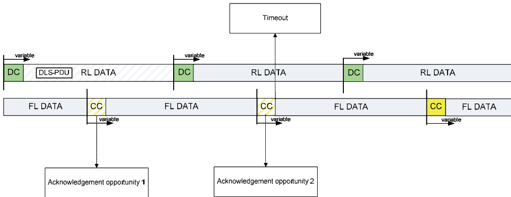
Fig. 10. LDACS1 RL DLS retransmission timer.
