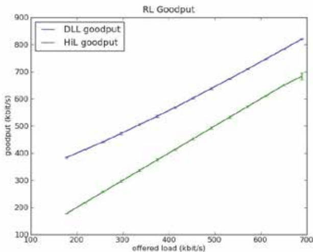
Fig. 23. RL goodput - scenario LOAD.
