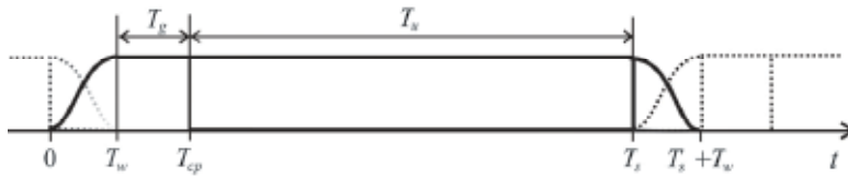
Fig. 13. Tx windowing principle.
