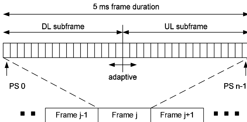
Fig. 2. AeroMACS frame with an adaptive DL/UL subframe width.
