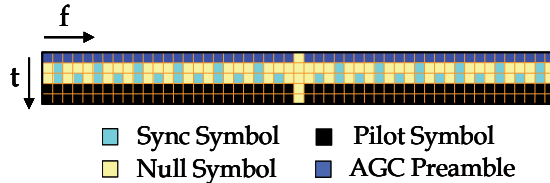
Fig. 6. Structure of one synchronization tile.
