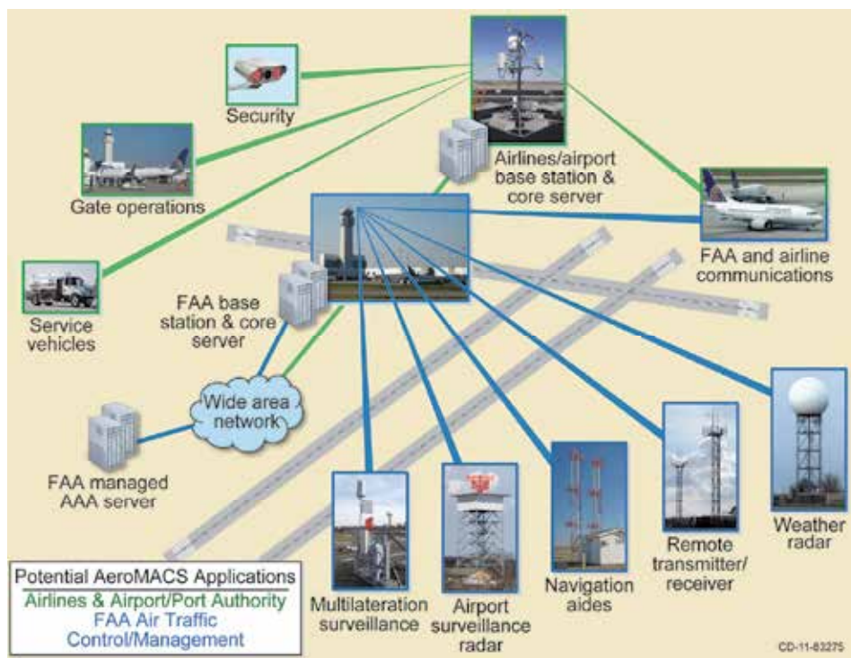
Fig. 4. Notional AeroMACS network configuration and potential applications.
