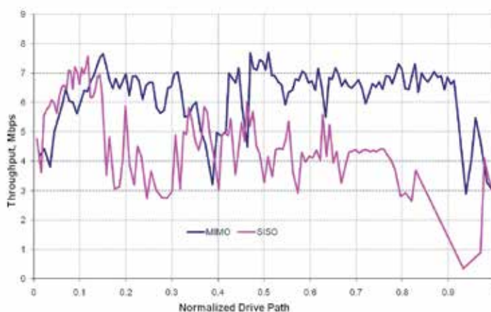
Fig. 14. Comparison of downlink throughput in MIMO and SISO antenna modes.
