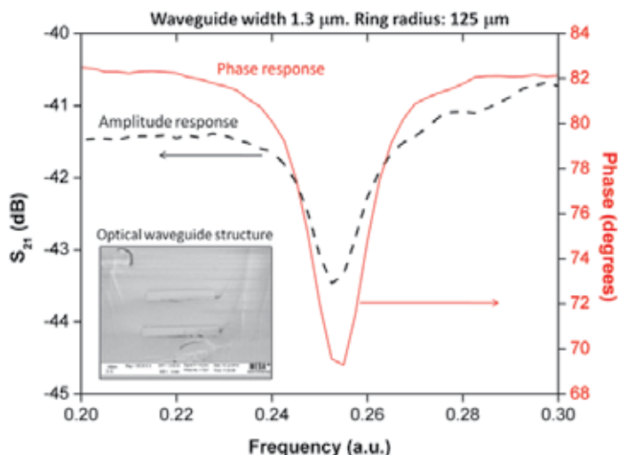
Fig. 15. Result of the propagation loss characterization of an optical ring resonator using the phase shift method. A loss of 0.2 dB/cm has been achieved. Inset: A scanning electron microscope (SEM) image of the waveguide cross-section.
