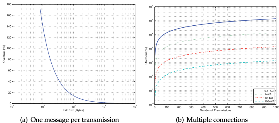
Fig. 6. Overhead estimation of a TCP connection establishment and shutdown
