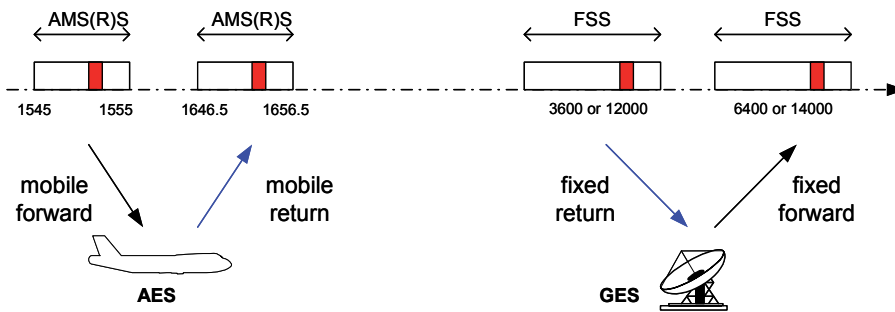
Fig. 3. Typical frequency bands used for safety aeronautical communications via satellite. These band allocations are managed by the ITU.
