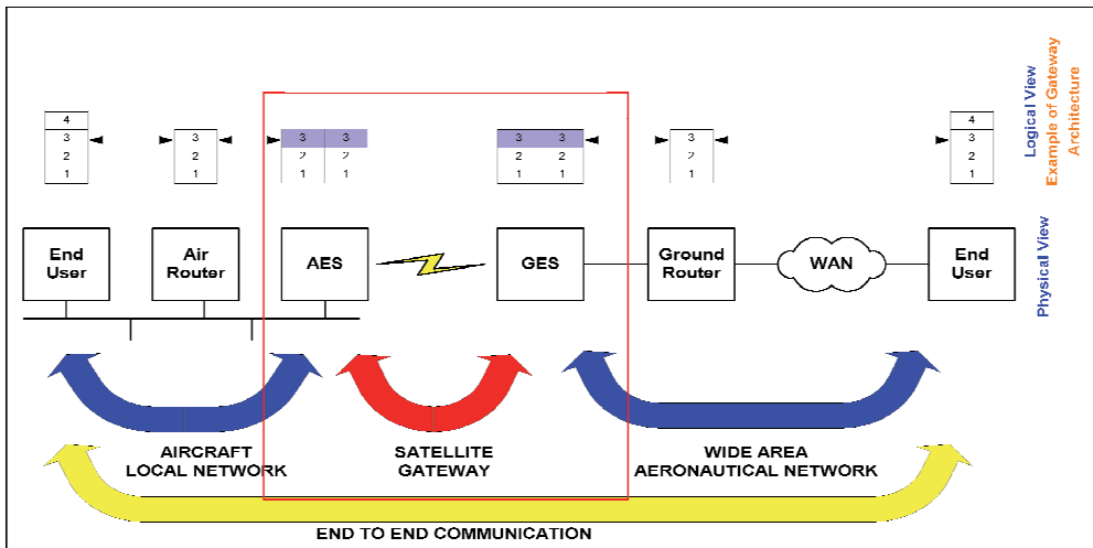
Fig. 2. SATCOM system integration in the ATN network.
