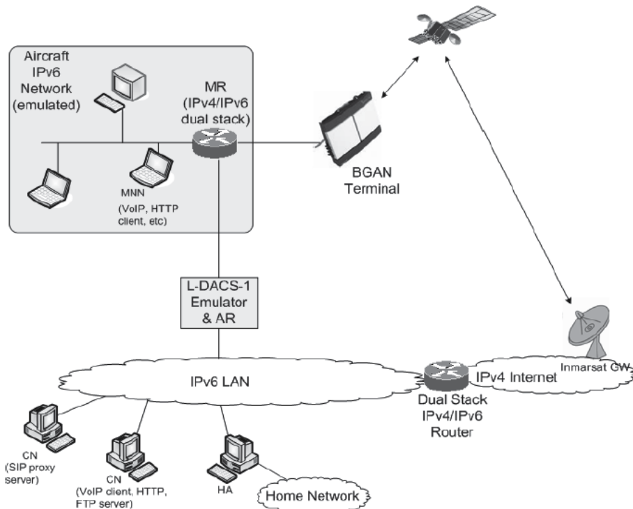
Fig. 1. NEWSKY laboratory testbed network architecture.
