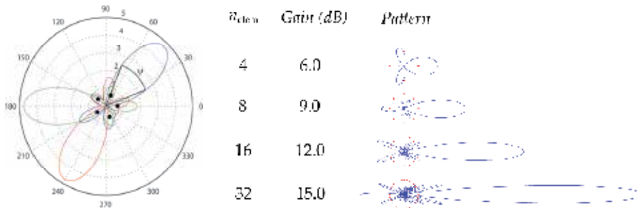
Fig. 8. Multibeam uniform circular array antenna azimuthal radiation patterns.
