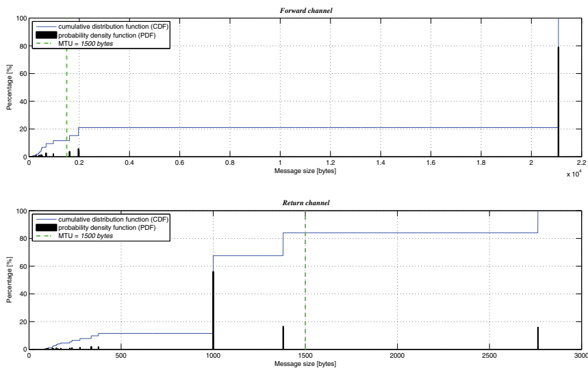
Fig. 11. Amount of data traffic generated by different ATM messages on the FW and RT channels, respectively
