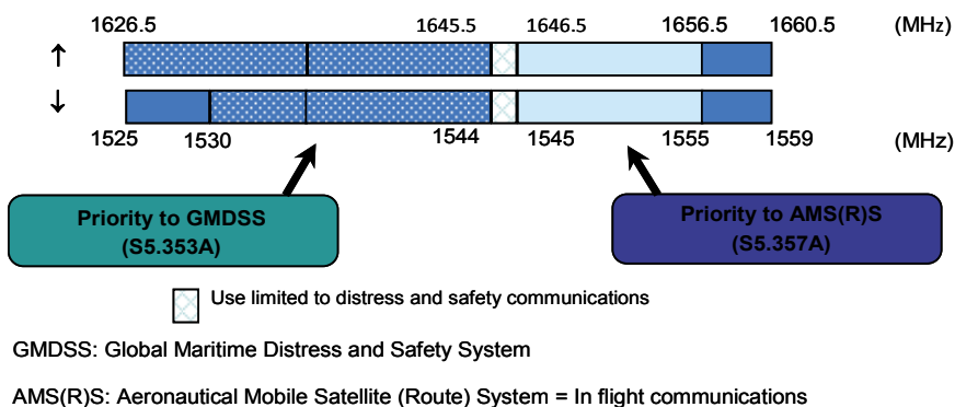
Fig. 4. AMS(R)S L band allocation for SATCOM.
