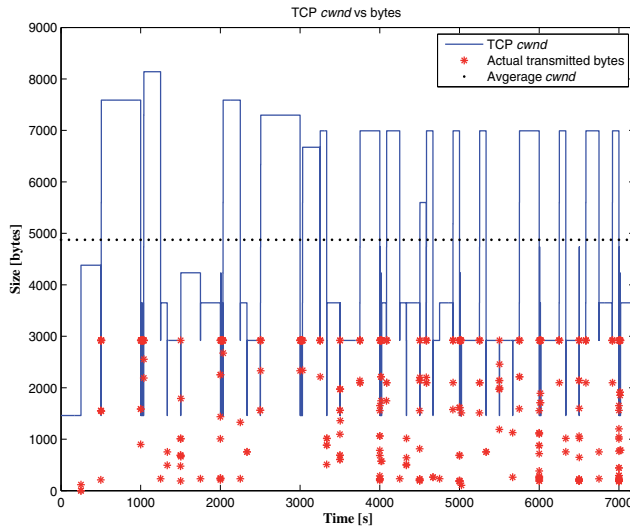
Fig. 7. cwnd of TCP vs the actual transmitted bytes from the aeronautical services
