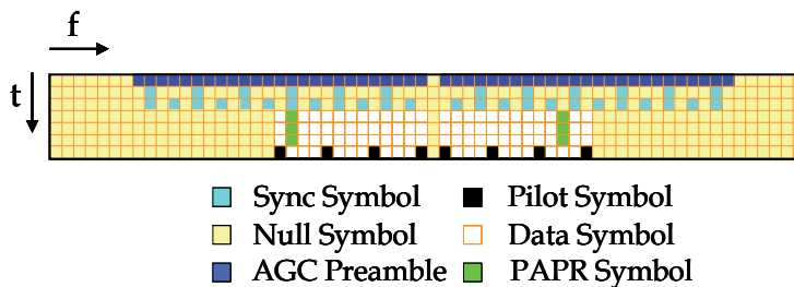
Fig. 9. Structure of random access frame.
