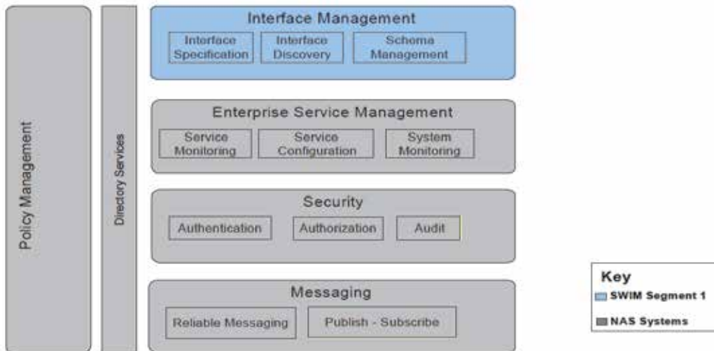
Fig. 8. SWIM Segment 1 Core Capabilities.
