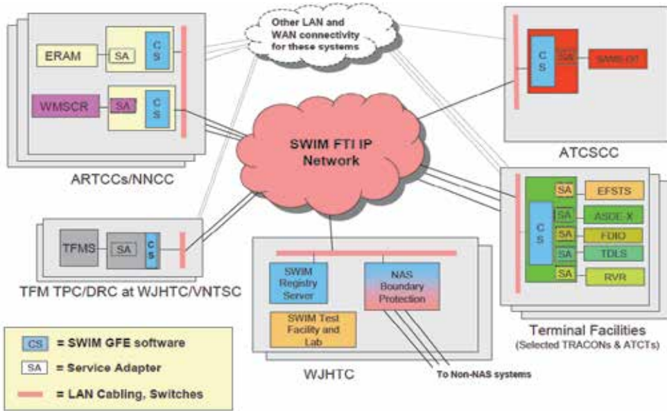
Fig. 7. FAA SWIM architecture with core services.
