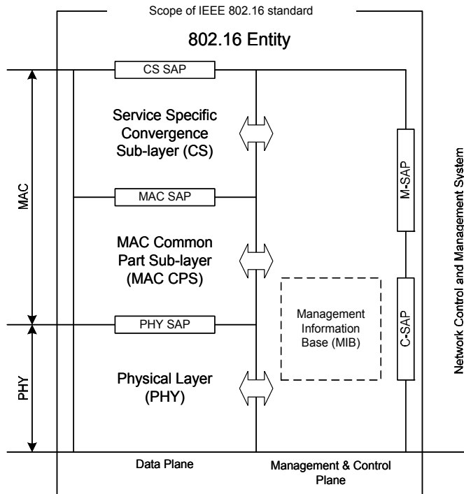
Fig. 1. The IEEE 802.16 protocol reference model.
