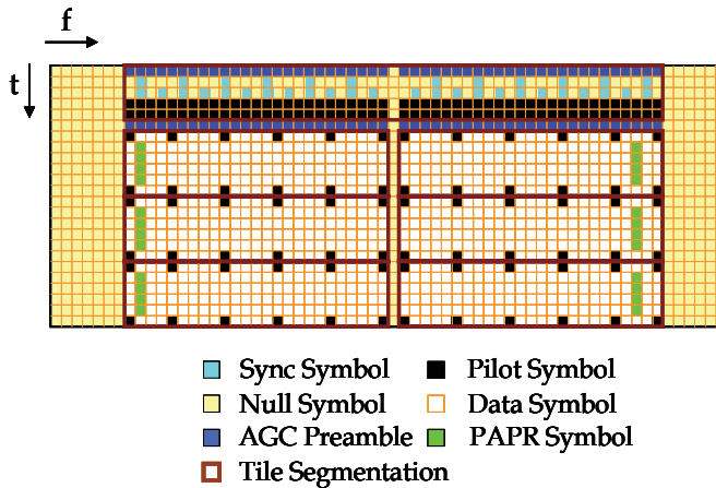
Fig. 7. Structure of one DC segment.
