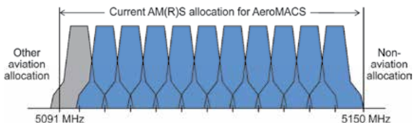
Fig. 7. Proposed AeroMACS channel plan for 5091-5150 MHz allocation.
