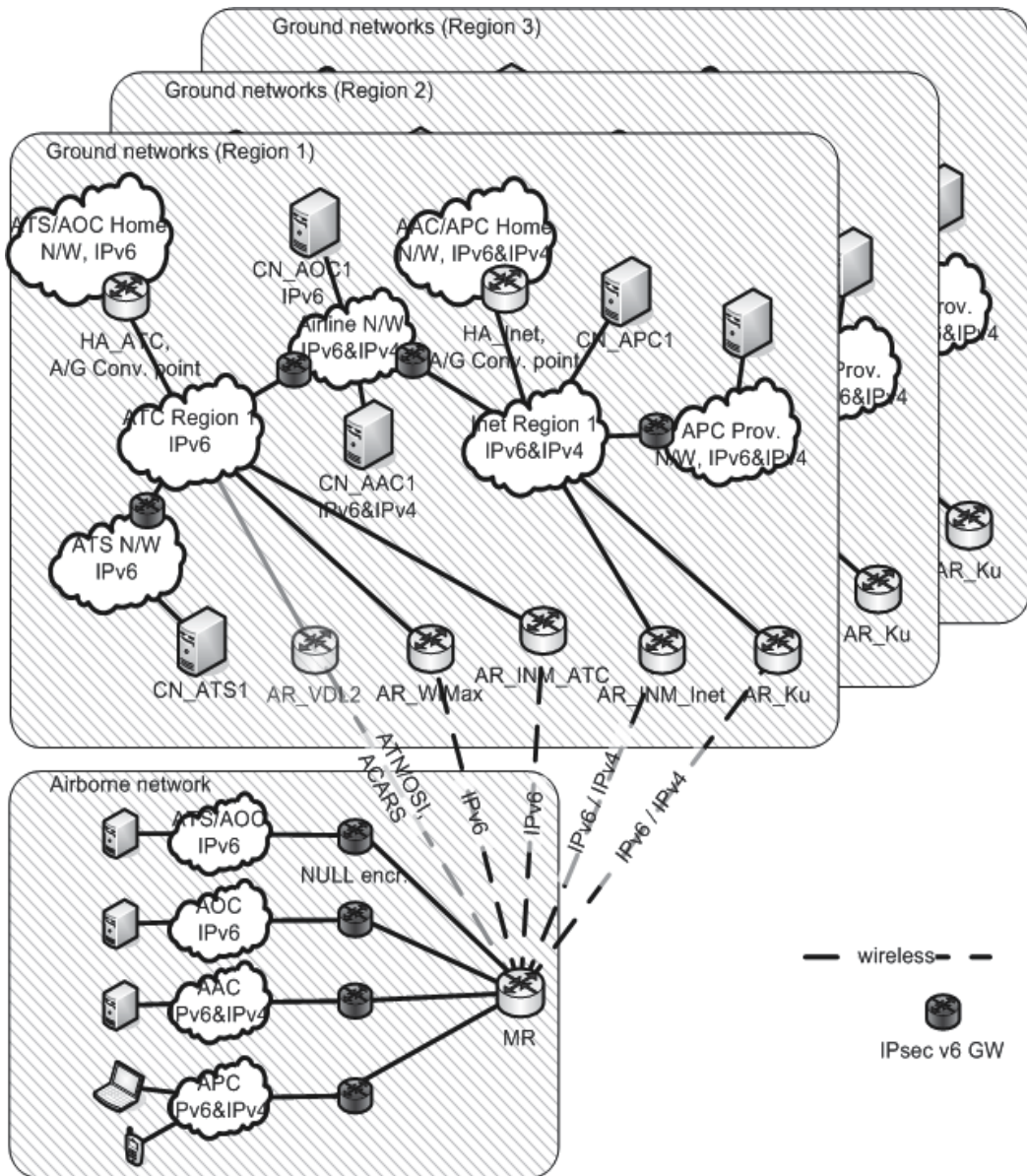
Fig. 2. SANDRA reference network architecture.
