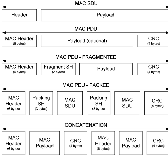
Fig. 4. Overview of different MAC PDU options.
