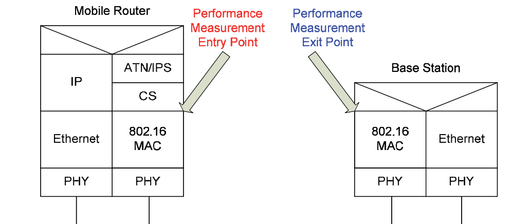
Fig. 16. Protocol stack of involved entities.
