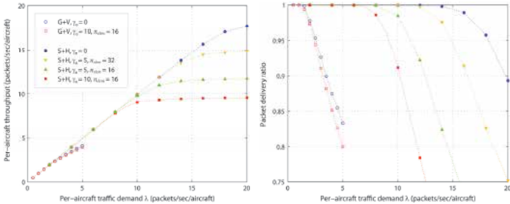
Fig. 17. Per-aircraft throughput and packet delivery ratio as a function of traffic load.
