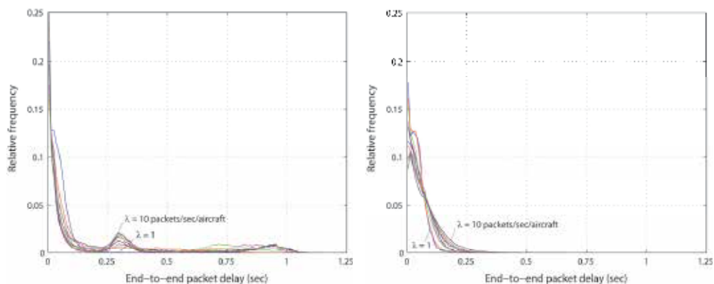
Fig. 18. Delay histograms for G+V (left) and S+H (right) routing schemes at 1200 UTC ( \gamma_0=0 ).
