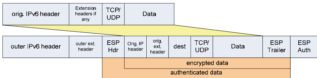
Fig. 9. IPv6 IPsec in ESP-tunnel mode.
