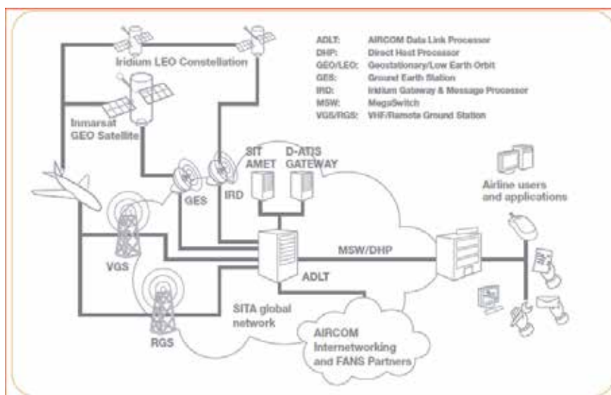
Fig. 1. Overview of SITA ACARS service architecture.
