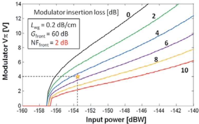
Fig. 10. Simulation results used to determine modulator parameters, V_\pi and L_m to achieve a minimum CNR of 8 dB. Preliminary target values of L_m = 5 dB and V_\pi = 4 V have been set, as indicated by a star symbol.
