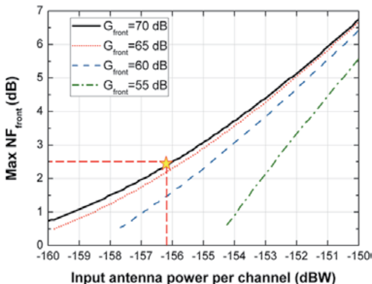
Fig. 9. Simulation results used to determine the maximum allowed NF_{\text{front}} as a function of the received signal power. The parameter values used are: V_{\pi} = 4 V, L_m = 2 dB and L_{\text{wg}} = 0.2 dB/cm. A target value of 2.5 dB front-end NF has been set, as indicated by a star symbol.
