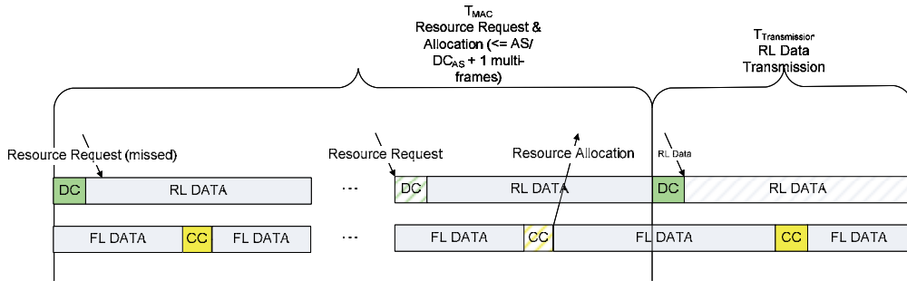
Fig. 7. Maximum length of RL packet transmission.
