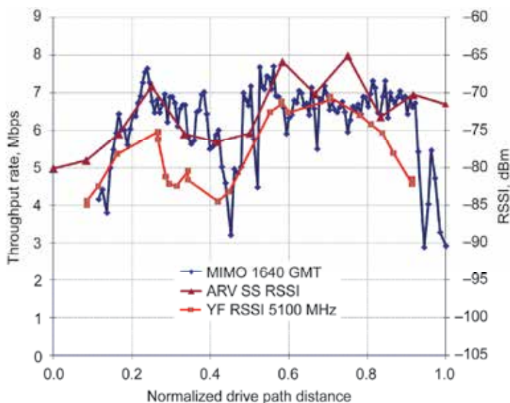
Fig. 15. Runway 24L drive test RSSI and throughput.
