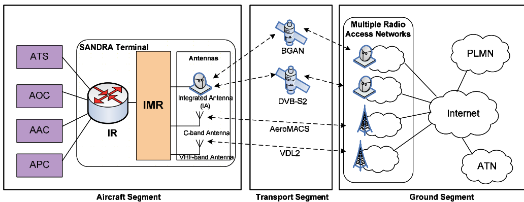
Fig. 1. SANDRA Network Architecture (Ali, 2011).
