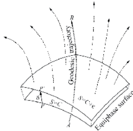
Fig. 1. Particle, at passing from A to B, moves along geodesic trajectory - the trajectory satisfying the principle of least action. All geodesic trajectories intersect equiphasic surfaces, S=C , S = C+\epsilon , perpendicularly (Lanczos, 1970).
