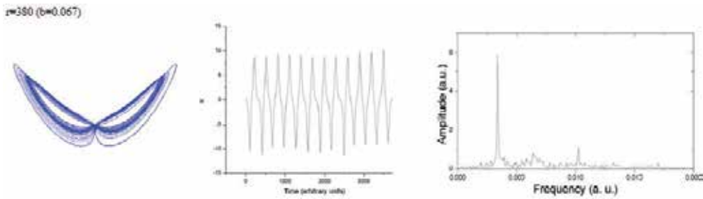
Fig. 8. a) Time evolution b) phase portrait c) the Fourier transform for r=380 , b=0.067
