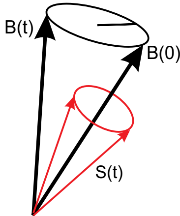
Fig. 1. A spin-1/2 subjected to a variable magnetic field \mathbf{B}(t) that describes a closed trajectory. When the field changes slowly in the time scale of the spin dynamics, then the spin \mathbf{S} can follow the field adiabatically. After a period, the spin state has accumulated a geometric phase in addition to the dynamical one.
