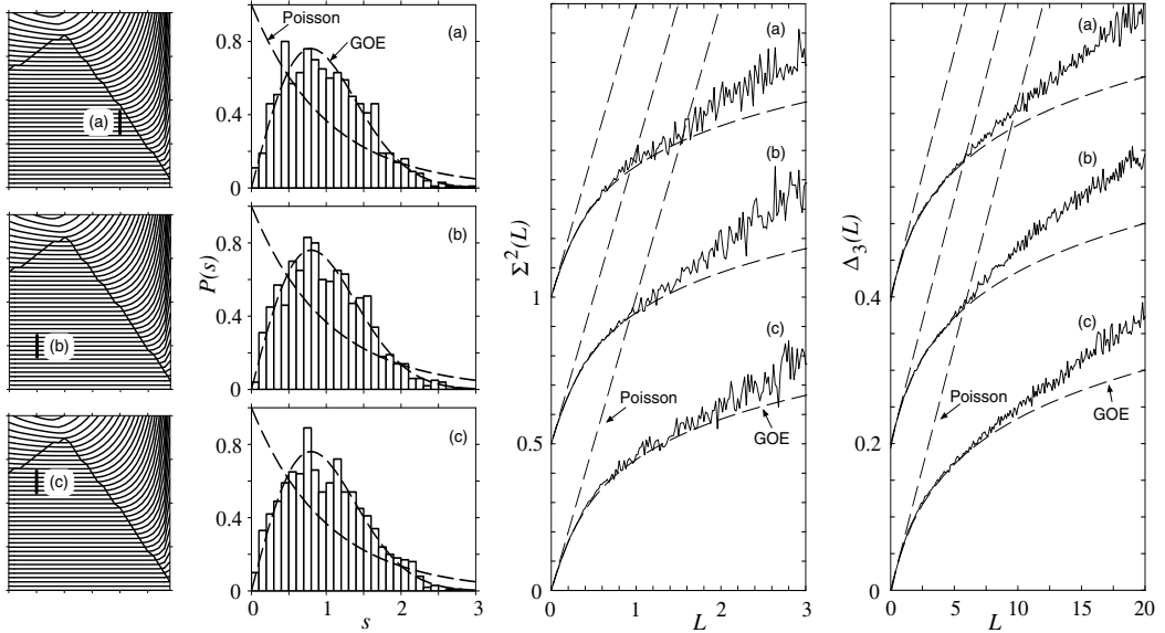
Fig. 2. Comparison of the level statistics P(s) , \Sigma^2(L) , \Delta_3(L) sampled at regions (a), (b), (c). Note that graphs for the latter two statistics are properly shifted to avoid their overlap. The vertical axis is for (c).
