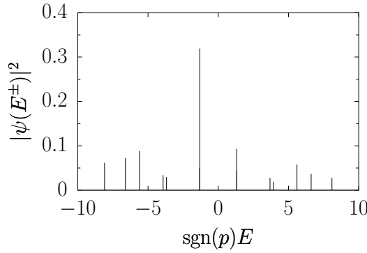
Fig. 7. Quantum energy representation of the Gaussian state
