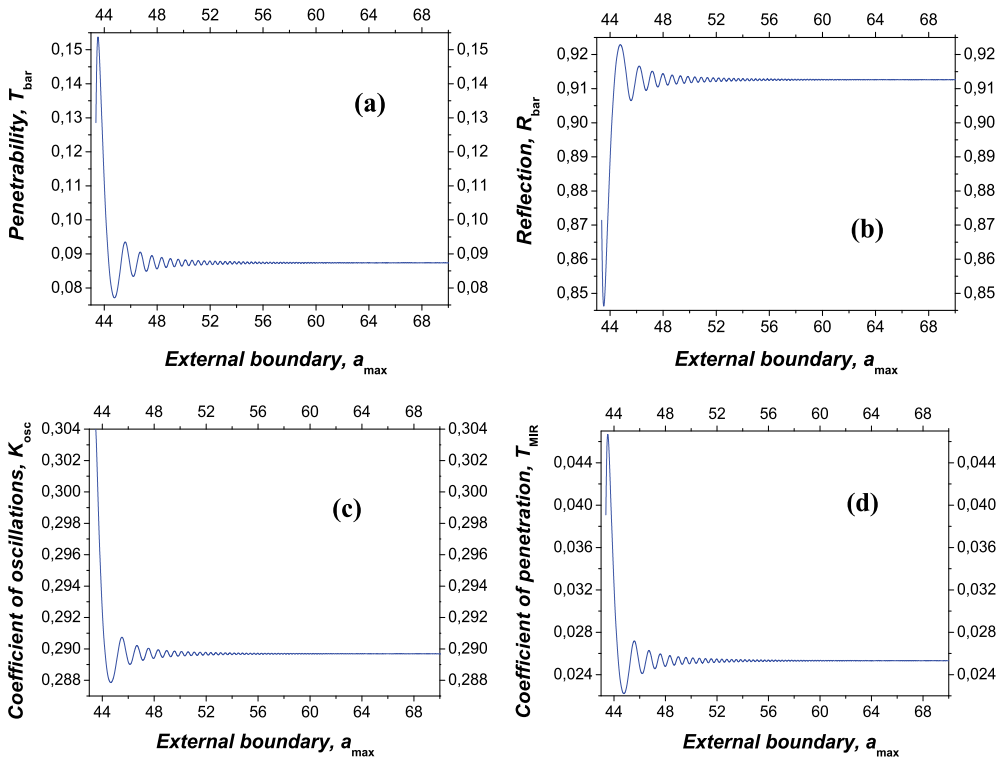
Fig. 10. Dependencies of the coefficients of penetrability (a), reflection (b), oscillations (c) and penetration (d) on the position of the external region, a_{\max} for the energy E = 223 ( A = 0.001, B = 0.001 ). For all presented values we have achieved accuracy |T_{\text{bar}} + R_{\text{bar}} - 1| < 1 \cdot 10^{-15} (the maximum number of intervals is 2000).
