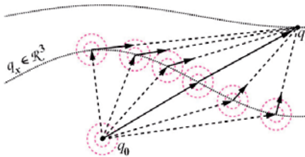
Fig. 11. Computation of all possible paths that pass from point q_0 to point q_1 through possible intermediate points q_x \in \mathcal{R}^3 represents a core of the path integral method. Pink circles conditionally represent radiation of Huygens waves.
