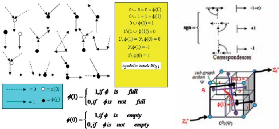
Fig. 5. a) String diagrams of corrective action using direct encoding by path integral. b) Euclidean portion of the space time \Omega(\Gamma) .
