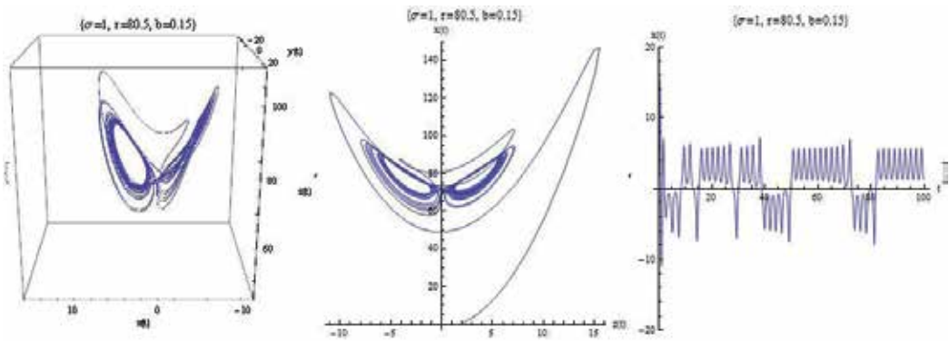
Fig. 2. a) Trajectory b) time evolution c) phase pattern for r=80, b=0.15
