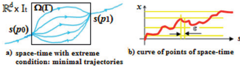
Fig. 1. a). The extreme condition in paths of the space \Omega(\Gamma) . b). Curve of the space-time in the \mathbb{R}^3 \times I_t .
