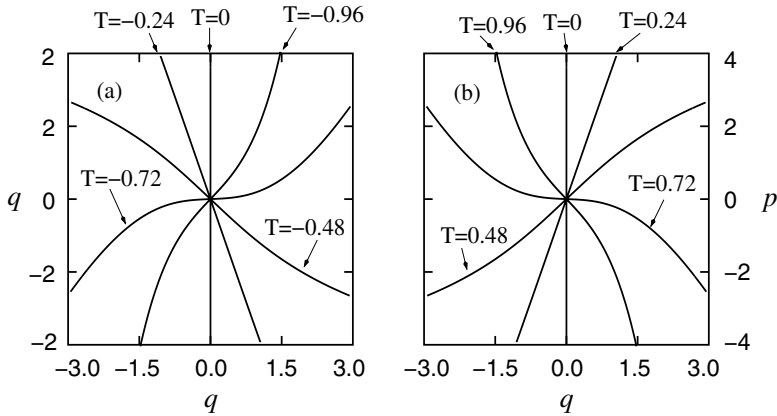
Fig. 2. Time surfaces for the nonlinear oscillator with a = 1 , l = 2 , and k = 9.8 . (a) Negative times and (b) positive times. The initial curve is q = 0 . Dimensionless units.
