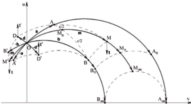
Fig. 3. The Poincare map. Geodesic lines are semicircles with centers on v-axis.
