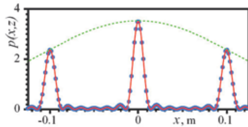
Fig. 6. Diffraction of thermal neutrons ( \lambda_{dB}=0.5 nm) in the far-field zone from grating having N=7 slits. Distance to observation screen is z=1 m. Blue circles relate to the probability density calculated by Eqs. (24)–(25). Intensity (27) is drawn by red solid curve. Dotted green curve draws envelope I_0(x,z) N^2 .
