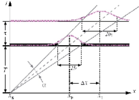
Fig. 4. Trajectories of particles passing through the Gaussian slit (Feynman & Hibbs, 1965), form a ray with an angle \alpha of the divergent particle beam emanating from the source x_s .
