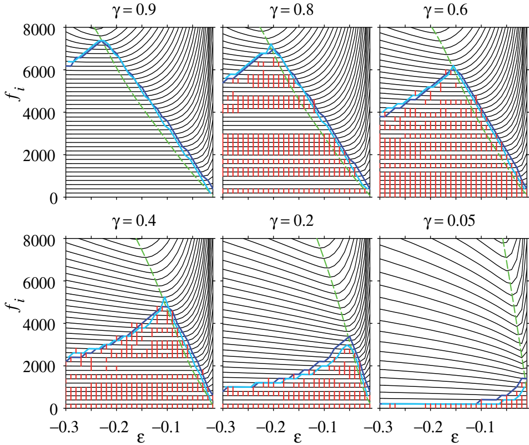
Fig. 1. Stretched level curves f_i at every 200 level along with the good domain on the f_i - \epsilon plane. N_p = 177 , N = 7921 , \ell = \text{even} , m = 0 . Sky- and dark-blue mountain-like curves account for necessary conditions 1 and 2 respectively and the bulk under the curves satisfies sampling test (e.g. Fig. 2). In order to make curves, diagonalization is performed for each \gamma and for thirty values of scaling parameter \epsilon ranging from -0.3 to -0.01 with increment 0.01 . The green dashed curve connects the minimum point of f_i and hits naturally the peak of the mountain. The level group with level-repulsion property is marked by red; these groups together remarkably overlap the domain for any \gamma (except the one \gamma = 0.9 > 8/9 ). For discussion on this, see subsection 3.1.
