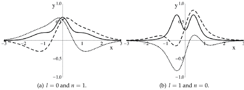
Fig. 3. Eigenfunction (86) with \zeta_1 = 0.2, \zeta_2 = 1 .
