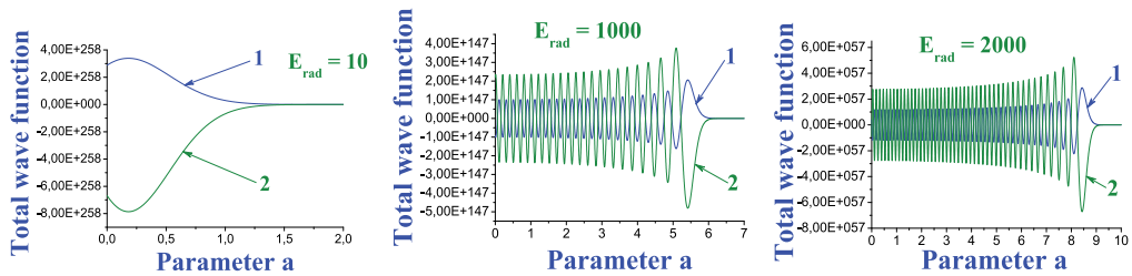
Fig. 4. The wave function at selected values of the energy of radiation E_{\text{rad}} (the blue line, represents the real part of the wave function; the green line the imaginary part of the wave function): (a) E_{\text{rad}} = 10 ; (b) E_{\text{rad}} = 1000 ; (c) E_{\text{rad}} = 2000
