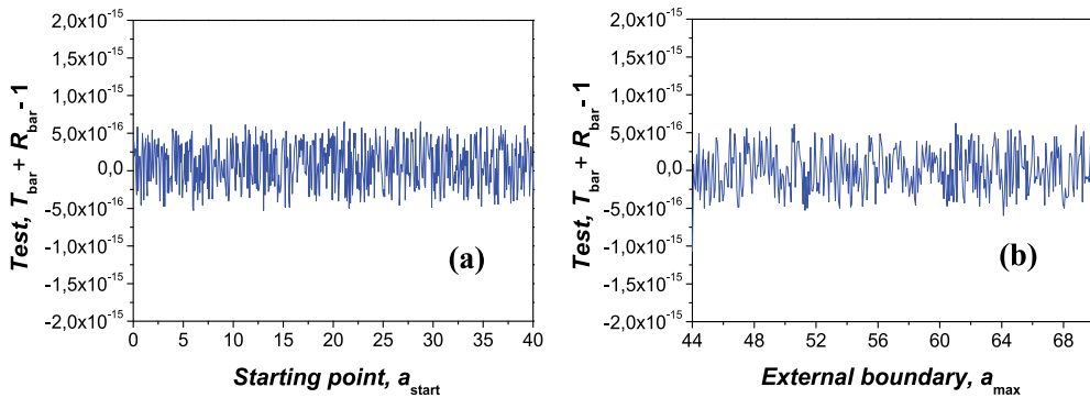
Fig. 12. Accuracy of the obtained penetrability T_{\text{bar}} and reflection R_{\text{bar}} for the energy E = 220 used in previous figs. 9 and 10. As a test, we calculate T_{\text{bar}} + R_{\text{bar}} - 1 in dependence on the position of the starting point a_{\text{start}} (a) and the external boundary a_{\text{max}} (b) ( A = 0.001, B = 0.001 , total number of intervals is 2000).
