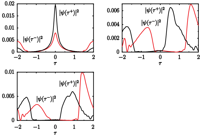
Fig. 9. Quantum time representation of the Gaussian state e^{-(q-q_0)^2/4\sigma^2 - ip_0(q-q_0/2)} / \sqrt{\sigma\sqrt{2\pi}} centred at (q, p) = (0, -1) , with \sigma = 0.2 , and for the nonlinear oscillator. The zero-time reference state is located at (a) X = 0 , (b) X the location of the right fixed point, and (c) X = 2 . Dimensionless units.
