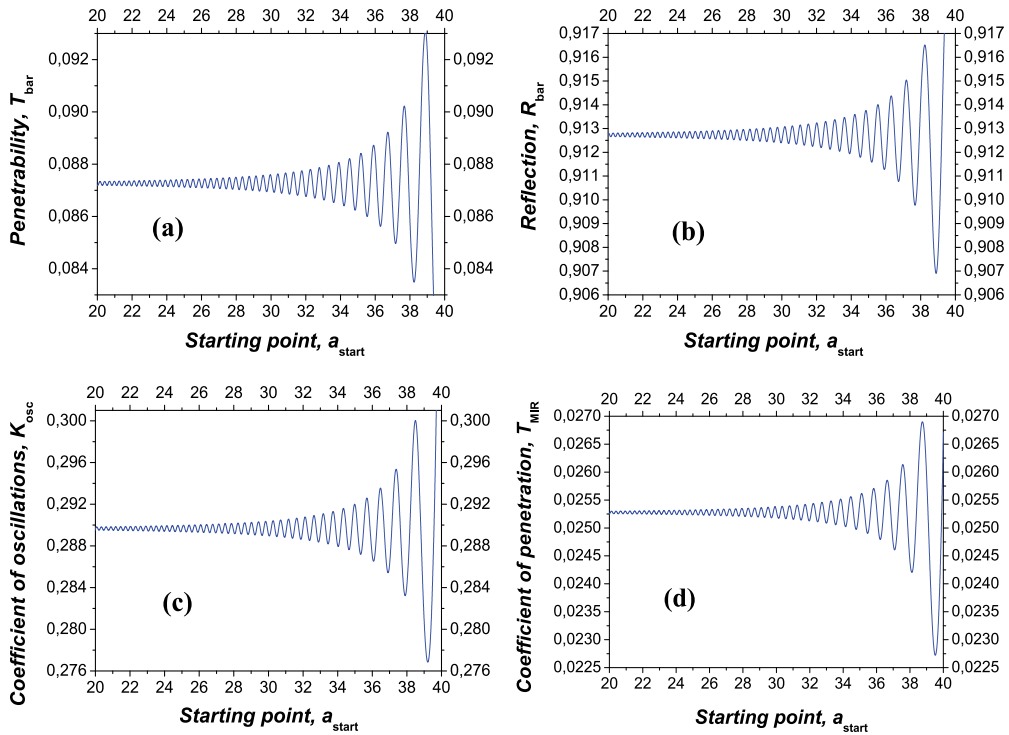
Fig. 9. Dependencies of the coefficients of the penetrability T_{\text{bar}} (a), reflection R_{\text{bar}} (b), coefficient of oscillations K_{\text{osc}} (c) and coefficient of penetration T_{\text{MIR}} (d) in terms of the position of the starting point a_{\text{start}} for the energy E = 220 ( A = 0.001 , B = 0.001 , a_{\text{max}} = 70 ). The total number of intervals is 2000, for all presented cases the achieved accuracy is |T_{\text{bar}} + R_{\text{bar}} - 1| < 10^{-15} . These figures clearly demonstrate oscillating ( i.e. not constant) behavior of all considered coefficients on a_{\text{start}} .
