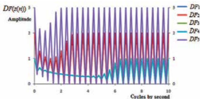
Fig. 7. Electronic propagators measuring corrective and restorer actions.
