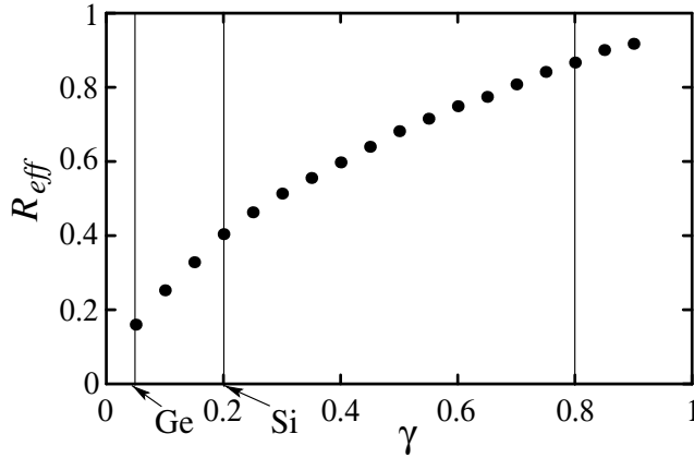
Fig. 4. Ratio of reliable levels vs. \gamma .
