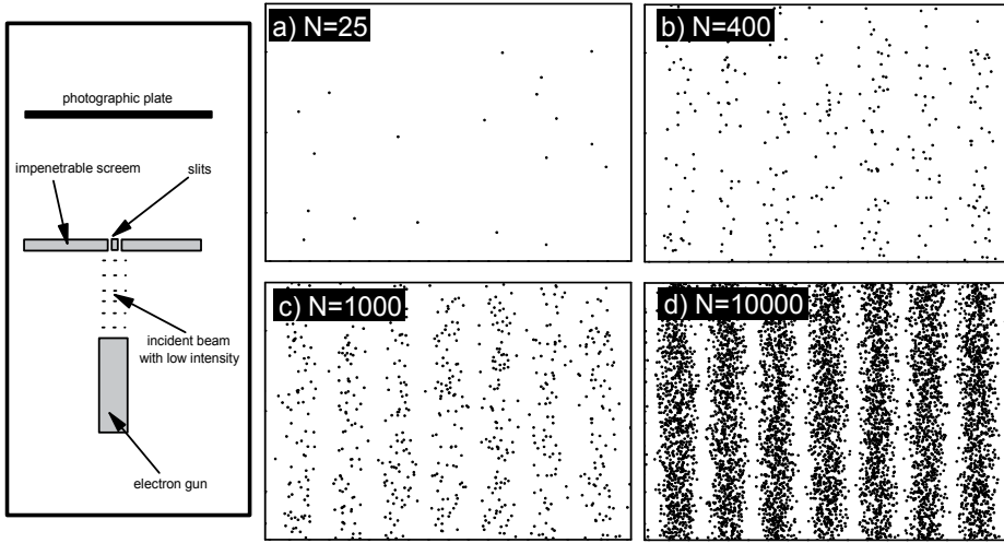
Fig. 1. Schematic representation of electron interference by double-slit apparatus using an incident beam with low intensity. Sending electrons through a double-slit apparatus one at a time results in single spot appearing on the photographic plate. However, an interference pattern progressively emerges when the number N of electrons impacted on the plate is increased. The emergence of an interference pattern suggested that each electron was interfering with itself , and therefore in some sense the electron had to be going through both slits at once. Clearly, this interpretation contradicts the classical notion of particles trajectory.
