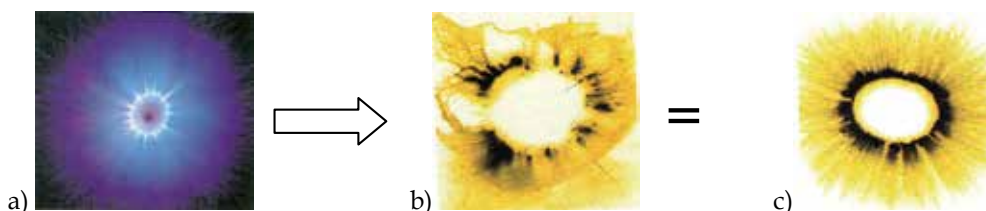
Fig. 8. The field in a) is the radiation electromagnetic spectra to re-compose and restore the field X , given in b). The corresponding image in c), is the field restored and corrected after the application a) in b).
