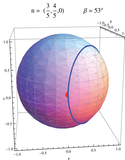
Fig. 4. The trajectory described on the Poincaré sphere. The dynamical phase is simultaneously cancelled by means of a QHQ gadget.
