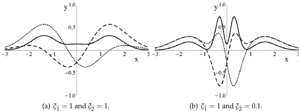
Fig. 4. Eigenfunction (86) with l = 2, n = 1 .
