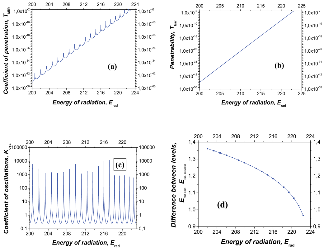
Fig. 11. Dependencies of the coefficient of the coefficient of penetration T_{MIR} (a), the coefficient of the penetrability T_{\text{bar}} (b), coefficient of oscillations K_{\text{osc}} (c) and difference E_{\text{res,next}} - E_{\text{res,previous}} between two closest energy peaks (d) on the E_{\text{rad}} energy (we have choose: A = 0.001 and B = 0.001 , a_{\text{start}} = 10 , a_{\text{max}} = 70 , number of intervals inside the scale axis a 1000, number of intervals of energy 100000). Inside the energy region E_{\text{rad}} = 200 - 223 we observe 19 resonant peaks in the dependencies of coefficients T_{MIR} and K_{\text{osc}} while the penetrability increases monotonously with increasing the E_{\text{rad}} energy.
