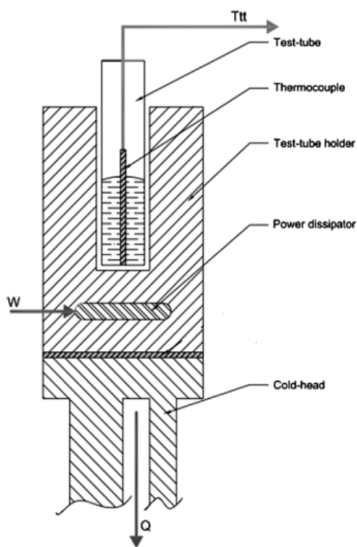
Fig. 2. Representation of the experimental apparatus. T_{tt} represents the temperature inside the test tube, measured by a thermocouple, Q is the heat absorbed by the refrigerating fluid and W is the dissipated power.
