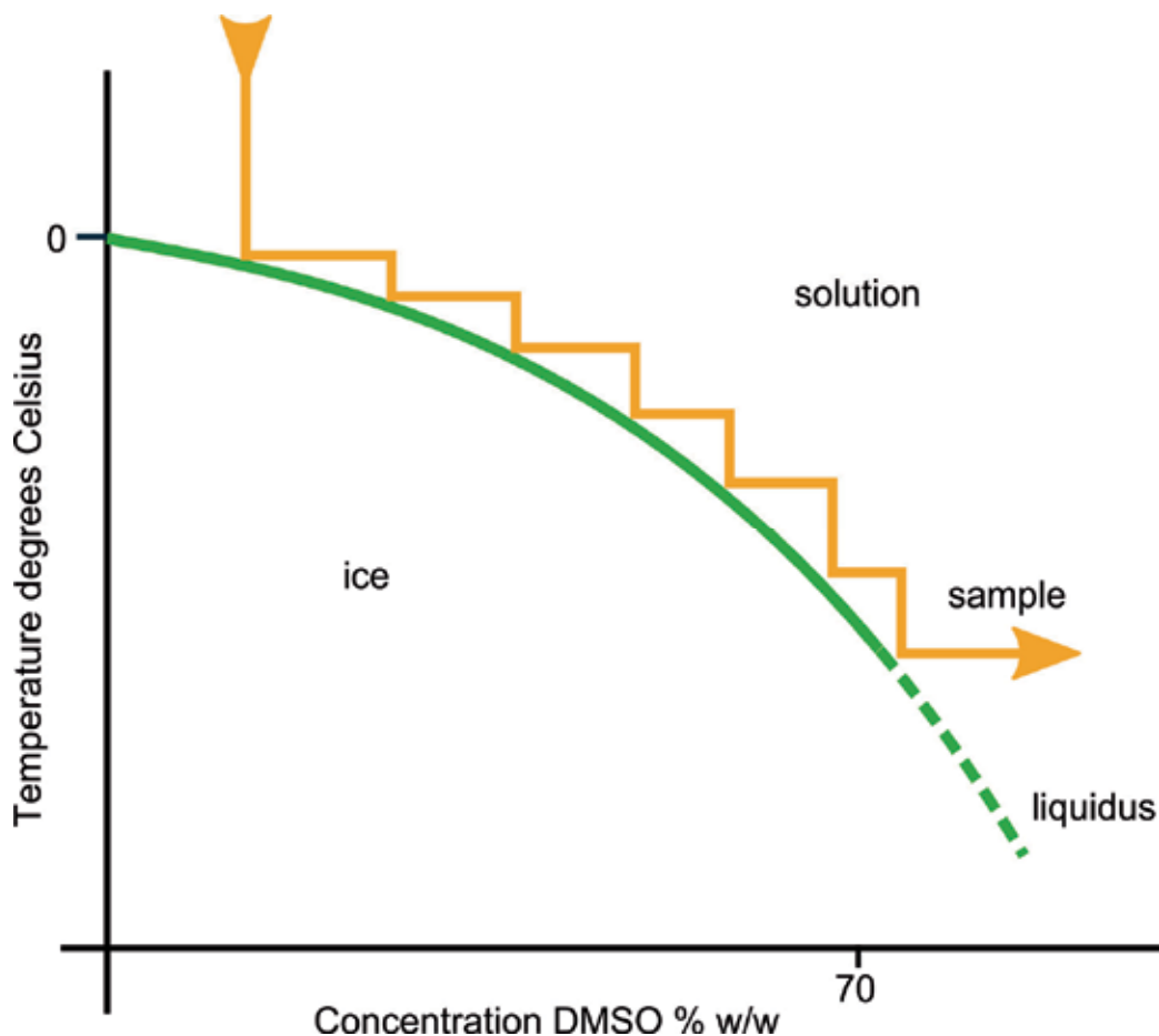
Fig. 1. Concentration of sample tracking liquidus
