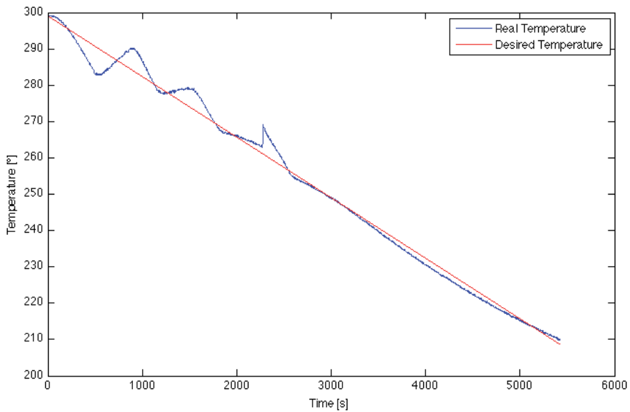
Fig. 6. Predictive model regulation - Temperature inside the test tube vs time. A desired cooling rate of -1^{\circ}/\text{min} was selected.
