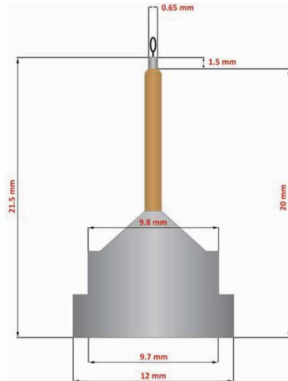
Fig. 7. CryoLoop Properly Installed in a CrystalCap Copper Magnetic - Hampton Research Corporation
