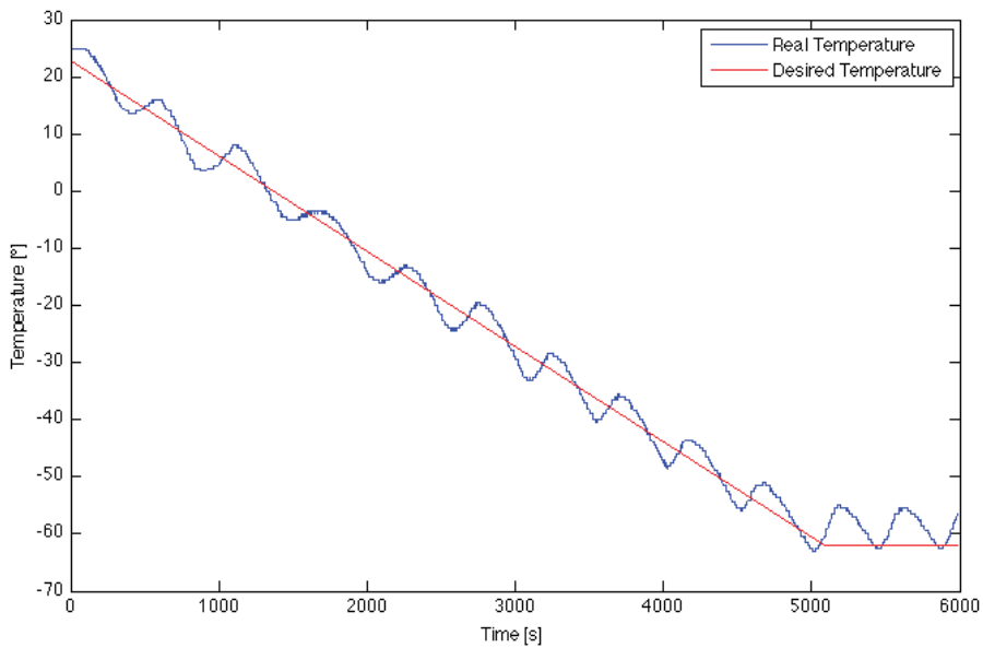
Fig. 4. On-Off regulation - Temperature inside the test tube vs time. A desired cooling rate of -1^{\circ}/\text{min} was selected.
