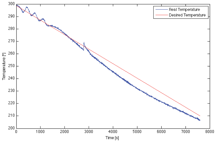
Fig. 5. Predictive model regulation - Temperature inside the test tube vs time. A desired cooling rate of -0.7^{\circ}/\text{min} was selected.
