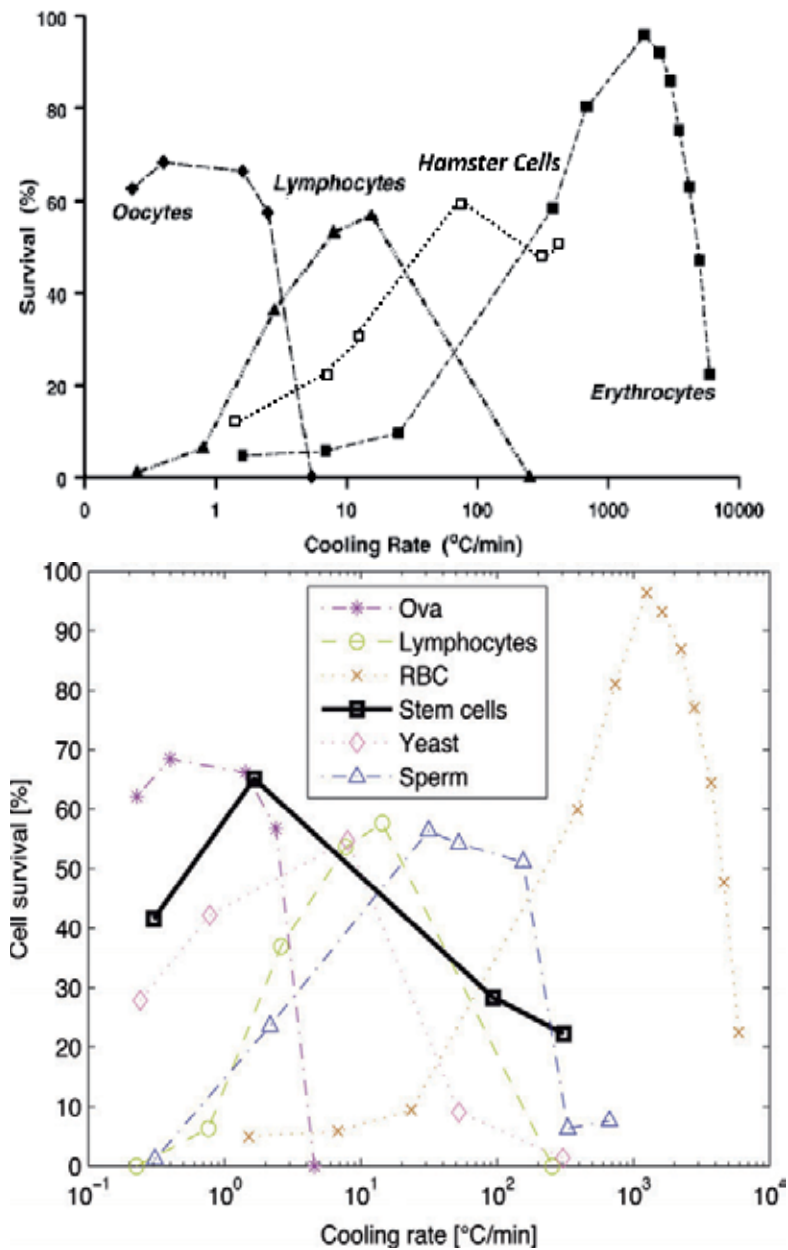
Fig. 2. The two-factor hypothesis of the cryoinjury by Peter Mazur: survival of cells of different size (oocytes \gg lymphocytes > hamster cells \gg erythrocytes) as function of the cooling rate. Top: Mazur's original graph, adapted from [Mazur et al. , 1972; Mazur et al. , 2008]. Bottom: Updated for stem cells (large size), yeast moderate) and sperm (slow) in [Cipri et al. , 2010]. Note that "slow (sub-optimal) and "fast" (supra-optimal) freezing in this case largely depends on the cells size: e.g., the rate of cooling 10 °C/min is very fast for oocytes (lethal IIF), very slow for erythrocytes ('damage due to the "solute effects") and close to the optimal for lymphocytes.
