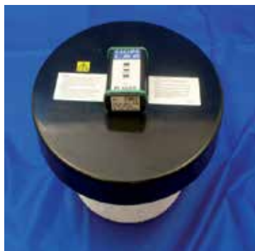
ShipsLog datalogger for vapour shippers
