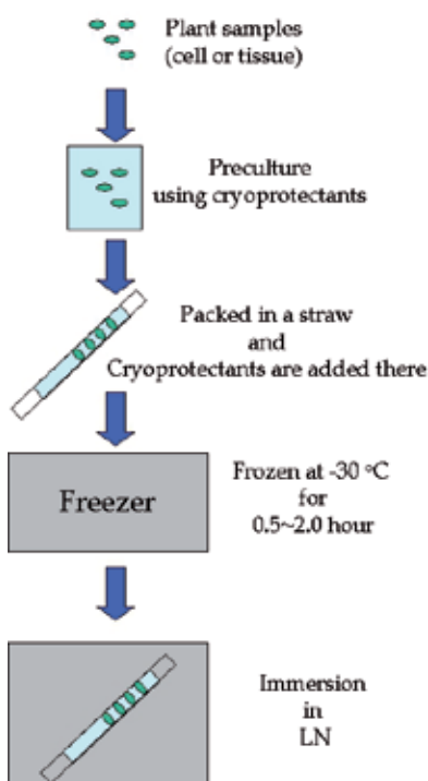
Fig. 2. The protocol of slow unprogrammed freezing (from Sakai et al., 1991).
