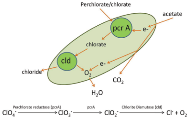
Fig. 1. Perchlorate reduction pathway. The reactions are catalyzed by perchlorate reductase (pcrA) that reduces perchlorate to chlorite and chlorite dismutase (cld) that converts toxic chlorite to chloride and oxygen (Adapted from Ederer et al., 2011).
