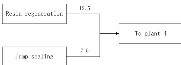
Fig. 14. Cross plant water reuse scheme
