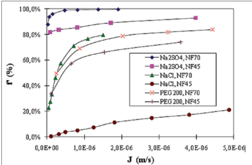
Fig. 4. Experimental data for nanofiltration (NF70 and NF45) for solutions of PEG, Na 2 SO 4 , NaCl: Modeling maximum and minimum separation factors based on permeation flux.
