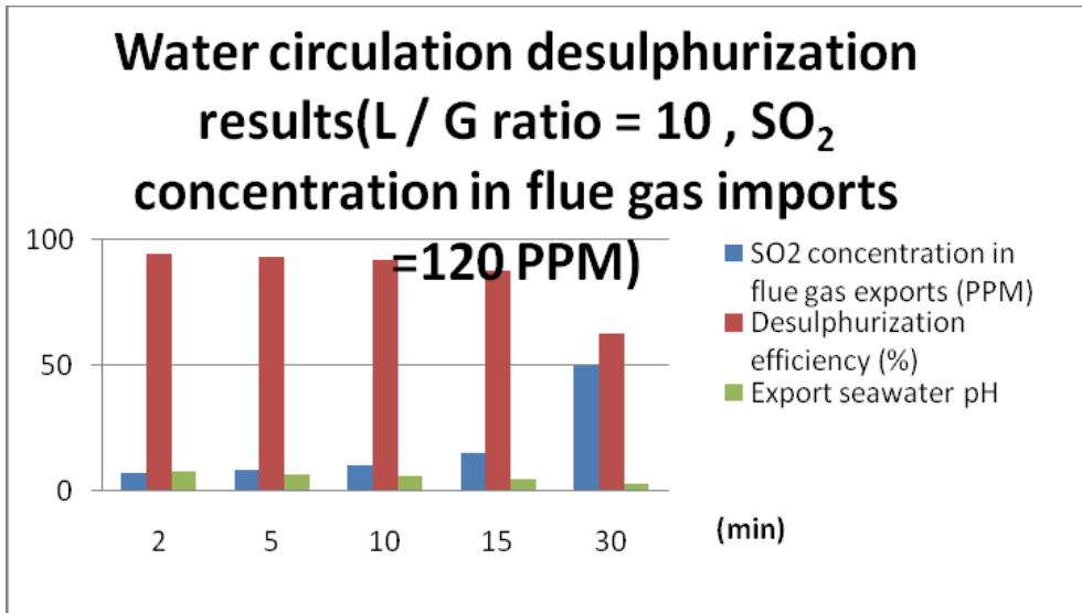
Fig. 4. The seawater circulation desulphurization test results
