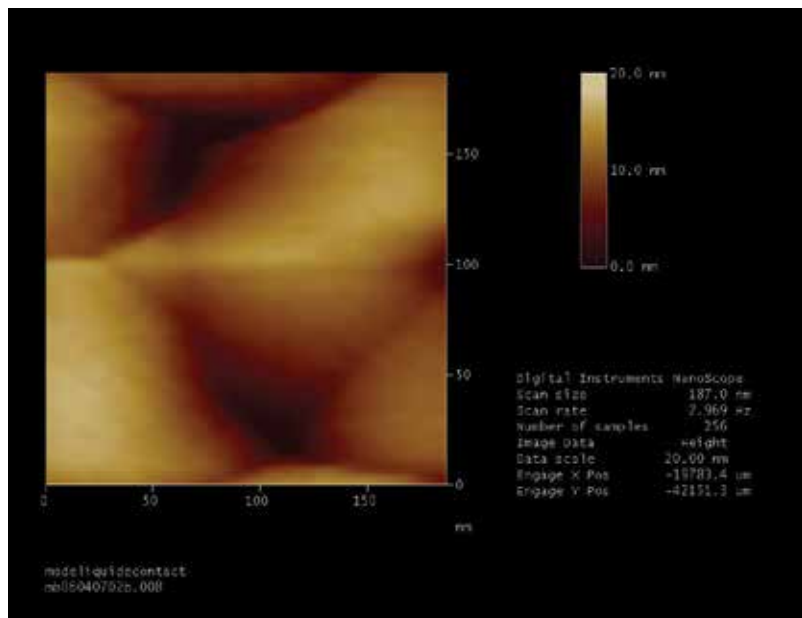
Fig. 7. Ceramic membrane D_p = 20 nm. Image Scanning Probe Microscope 200x200 nm, contact mode, ambient air.
