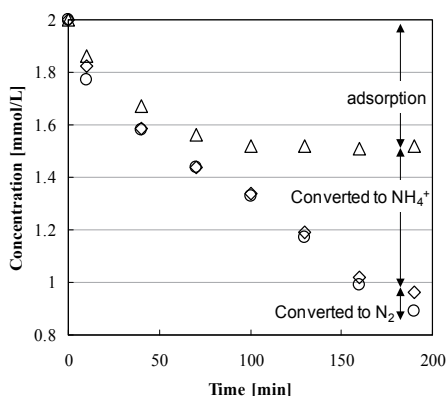
Fig. 11. 2 mmol/L NaNO_2 was reduced by H_2 gas on 0.1 wt% Pt/ Al_2O_3 catalyst. The decrease of NO_2^- (○) was found to be caused by catalytic conversion to N_2 or NH_4^+ , and by adsorption onto alumina (Δ).
