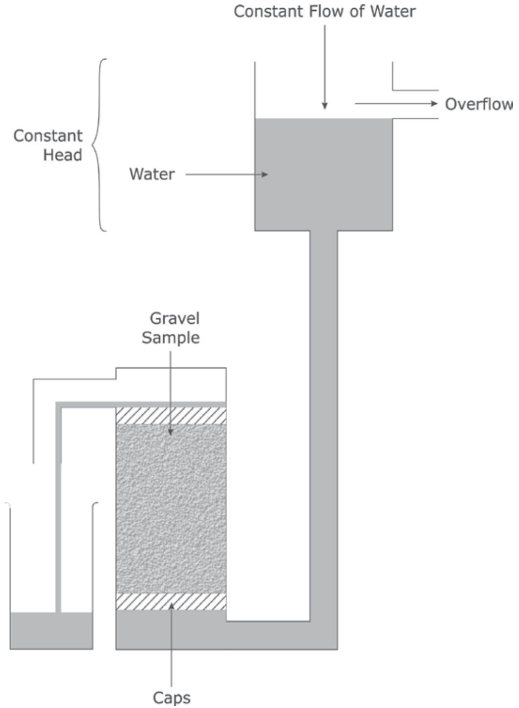
Fig. 5. Schematic representation of laboratory permeameter setup.
