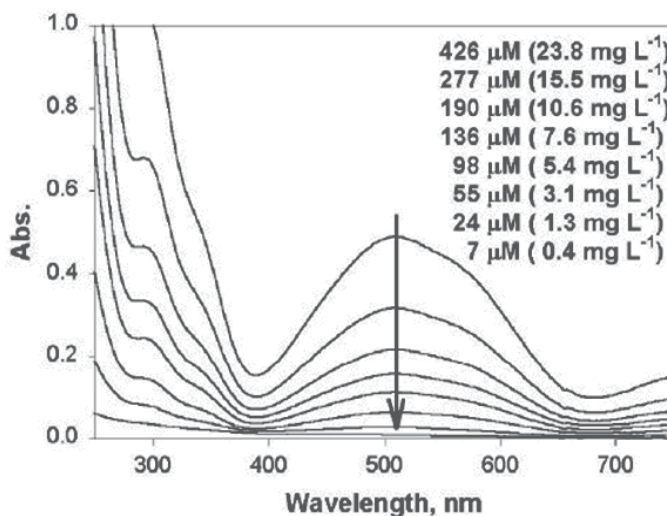
Fig. 6. UV-Vis absorption spectrum of Fe(VI) in aqueous solution as a function of its concentration, pH = 9.2, 25 mM phosphate buffer [27].
