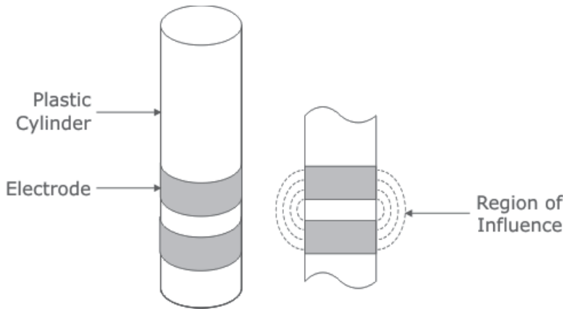
Fig. 6. Schematic of capacitance sensor. Right hand figure is front view of left hand figure showing the area in which measurements are made.
