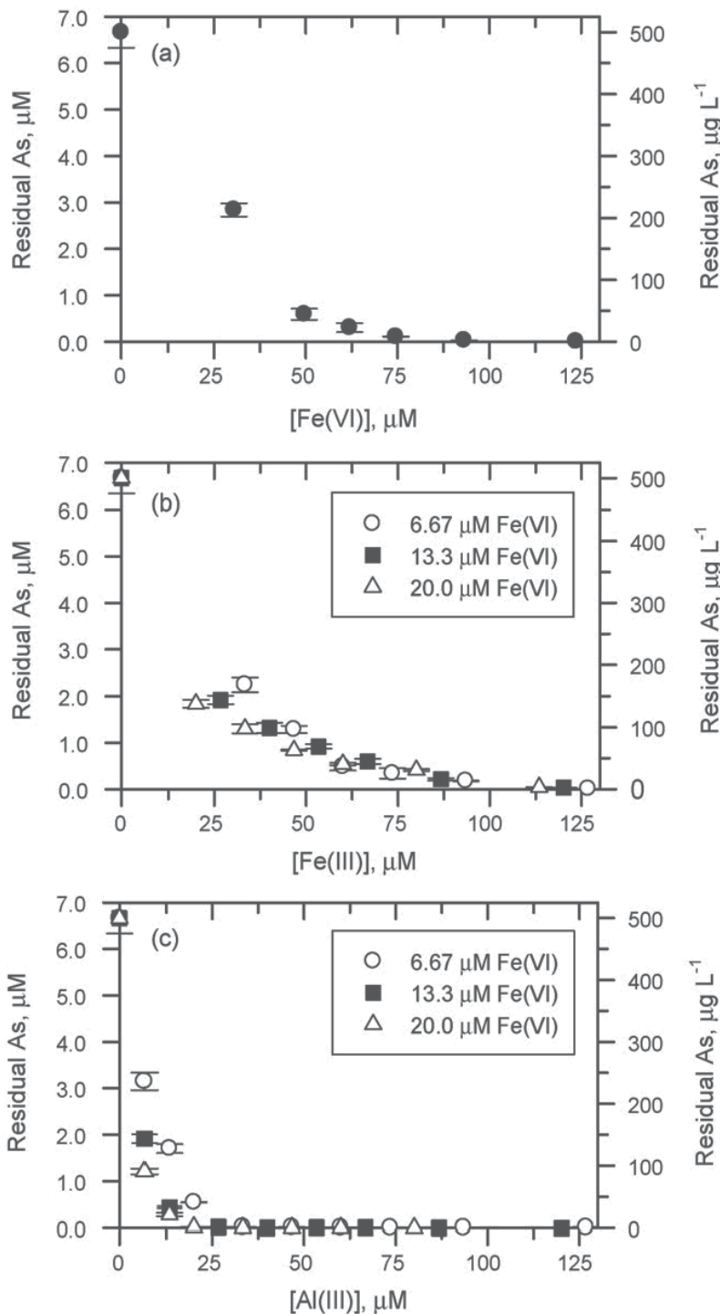
Fig. 17. Removal of arsenite by \text{Fe(VI)} (a), \text{Fe(VI)/Fe(III)} salts (b), and \text{Fe(VI)/Al(III)} salts (c) at pH 6.5. Initial concentration = 500 \mu\text{g As(III)/L} [81].
