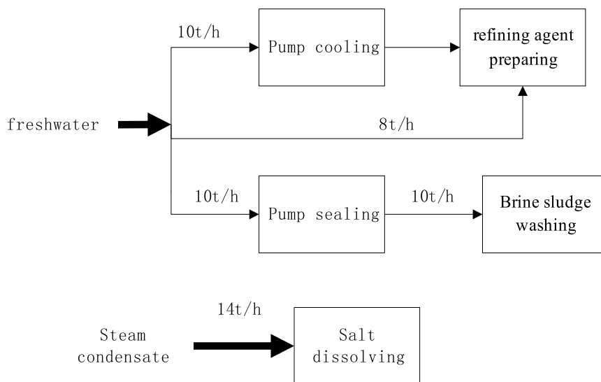
Fig. 12. Water reuse schemes in plant 1
