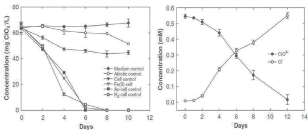
Fig. 5. A. Perchlorate removals in the iron-mediated microbial culture. Fe(0)-cell batch reactor contained 2 g of Master Builder's cast iron. B. Chloride balance in microbial perchlorate reduction by pure iron granules. Initial concentration of perchlorate was 55mg/L. Batch reactor contained 2 g of Alfa Aesar high purity iron granules. (Adopted from Son et al., 2006).
