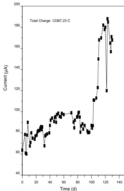
Fig. 8. Total charge calculated from the integration of current over time for substrate consumption.
