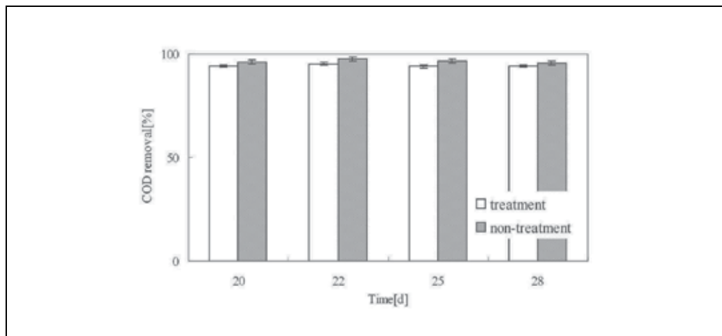
Fig. 7. COD removal efficiency during test tube treatment plant (CAS)
