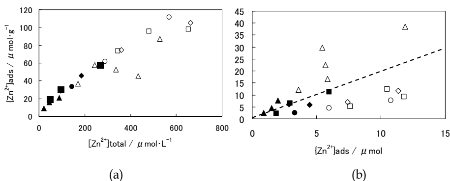
Fig. 2. Adsorption of Zn 2+ ions onto alumina. (a) Relationship between total concentration of Zn 2+ and adsorbed amount of Zn by 1g of Al 2 O 3 . The results obtained by using several concentration of Zn stock solutions are depicted with different symbols. The closed symbols are used for the results which seems to fit a line, while open symbols are used for the other. (b) Relationship between absolute amount of adsorbed Zn 2+ and released H + , which are calculated for the same experimental data shown in Fig. 2(a). The type of symbols is followed Fig. 2 (a). The line represents a slope 2.
