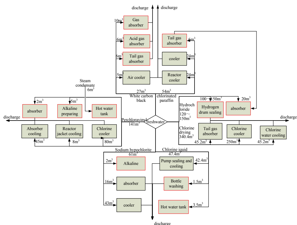
Fig. 3. Balanced water system of plant 2
