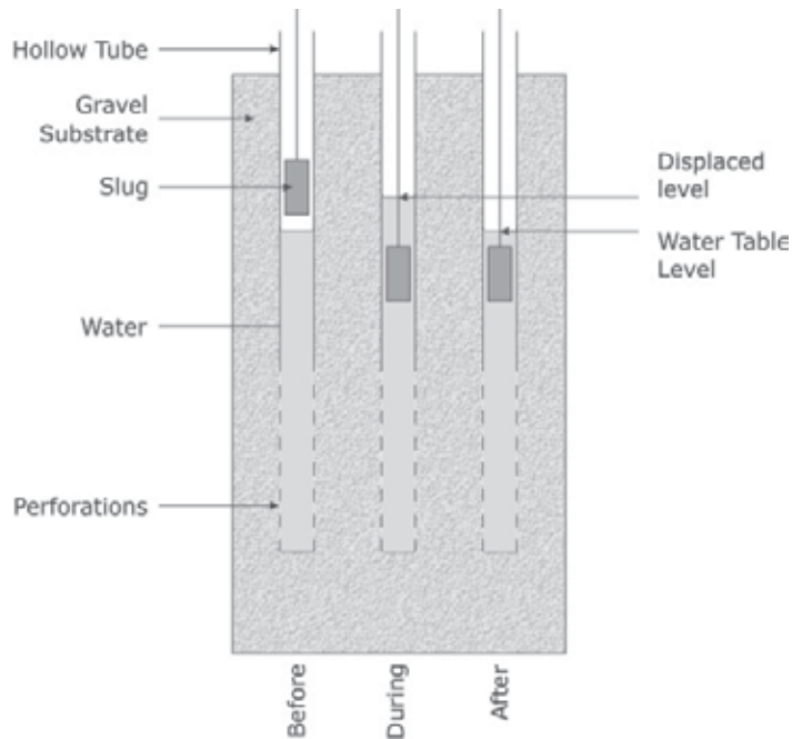
Fig. 2. Schematic representation of the measurement phases in the slug test used in a gravel substrate.
