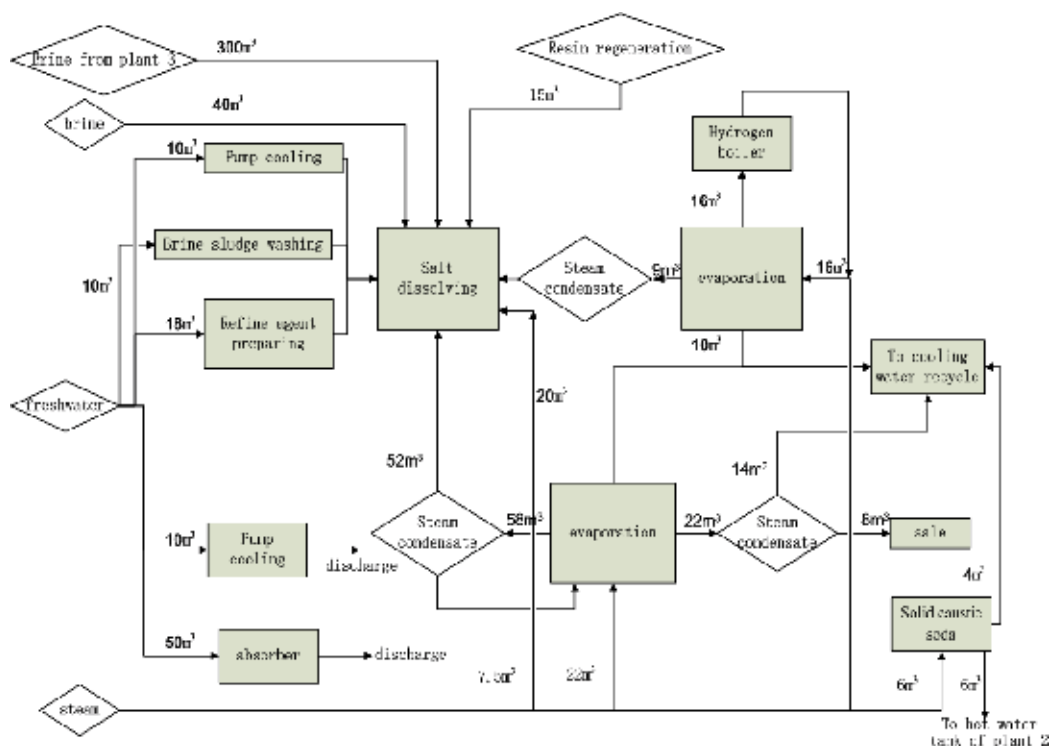
Fig. 2. Balanced water system of plant 1
