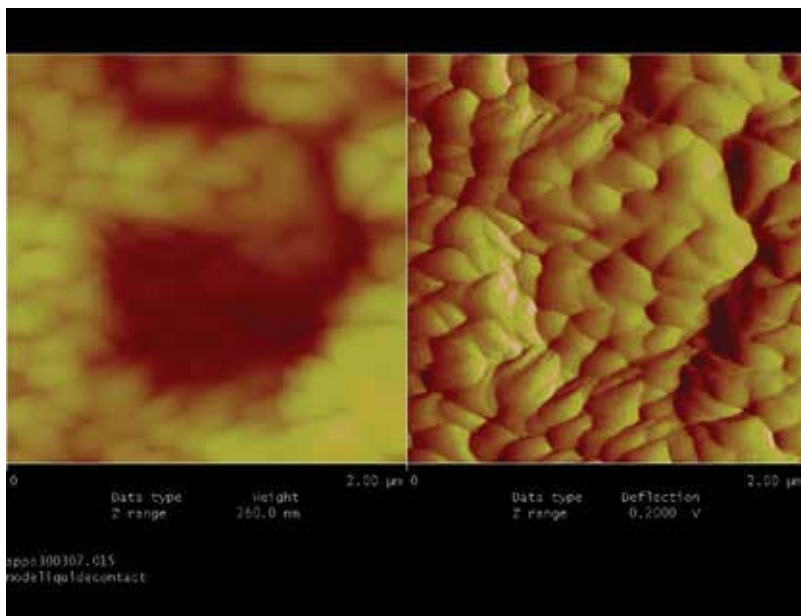
Fig. 9. Surface modification of ceramic membrane D_p = 20 nm with sulfonated oxide of polyphenyl. Image Scanning Probe Microscope 2 \times 2 \mu\text{m} , contact mode, aqueous medium, ambient temperature and pressure.
