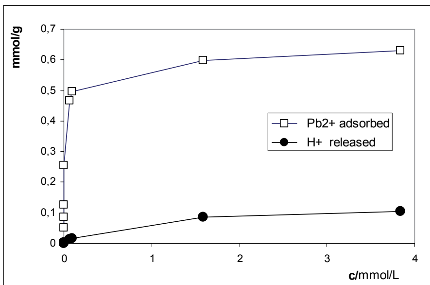
Fig. 6. Comparison between amounts of adsorbed lead(II) and H + released from OC coal, 30°C, initial pH = 4.2
