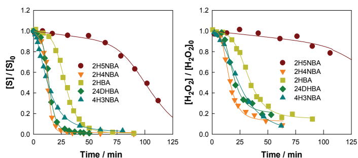
Fig. 7. Normalized concentration profiles of model substrates obtained in dark Fenton-like process.
