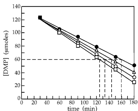
Fig. 10. DMP in function of reaction time. ●: \Delta T=0^\circ\text{C} ; Δ: \Delta T=10^\circ\text{C} ; ○: \Delta T=20^\circ\text{C} ; □: \Delta T=30^\circ\text{C} .
