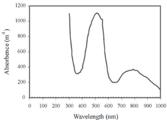
Fig. 5. UV-Vis spectrum of potassium ferrate(VI) [25].
