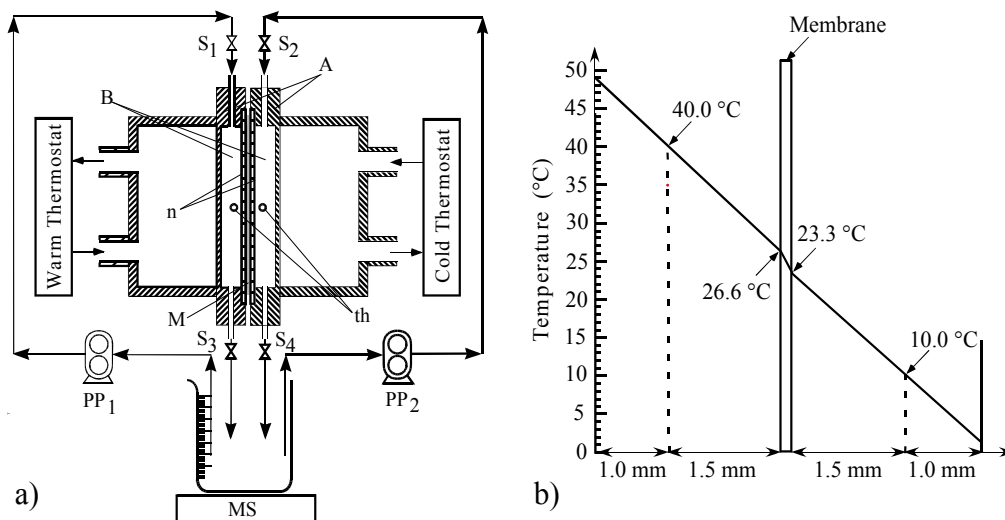
Fig. 2. a) Schematic representation of the planar bioreactor. Half-cells (A); internal working volumes (B); membrane (M); supporting nets (n); thermocouples (th); stopcocks (Si); thermostatic magnetic stirrer (MS); peristaltic pumps (PPi); b) Temperature profile in a non-isothermal bioreactor under the following experimental conditions: \Delta T=30^{\circ}\text{C} , T_{\text{av}}=25^{\circ}\text{C} .
