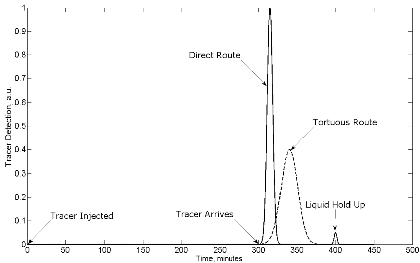
Fig. 7. Breakthrough curves from a direct (solid line) and tortuous (dashed line) system.
