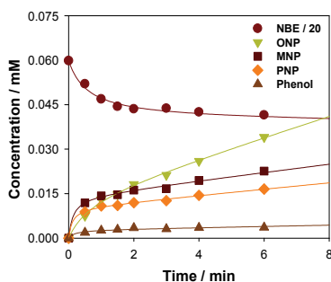
Fig. 4. Kinetic profiles of NBE and its primary phenolic products obtained in Fenton treatment.
