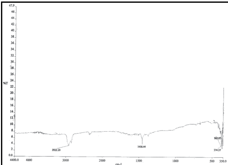
Fig. 3c. FTIR spectrum of the mixture of seed and sponge of L. cylindrica biosorbent after biosorption of \text{Cu}^{2+} ions.
