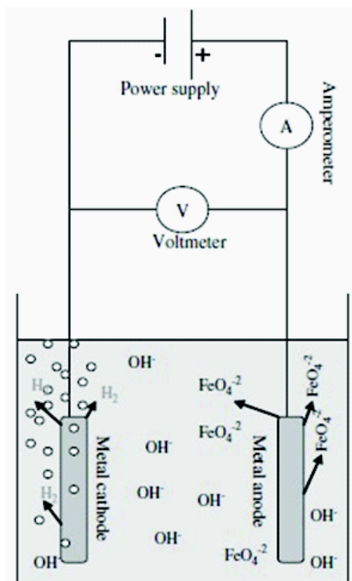
Fig. 1. Electrochemical cell used for Ferrate synthesis [4].
