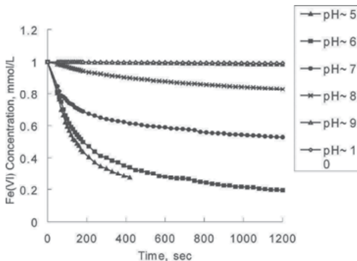
Fig. 7. The change of the Fe(VI) concentration as a function of time at various pH values [Initial concentration of Fe(VI): 1 mM] [34].
