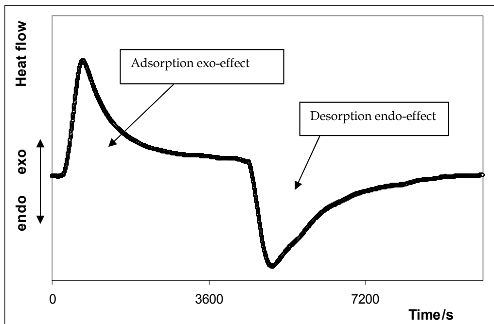
Fig. 4. Calorimetric curve of Pb(II) ions adsorption/desorption cycle ascertained for sample SC, grain size = 0.06 –0.25 mm, temperature = 30°C, Pb(II) ions concentration = 20 mmol/L, flow rate = 0.4 ml/min
