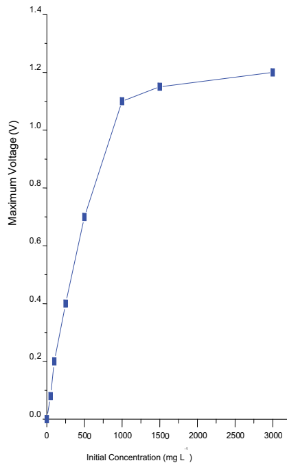
Fig. 7. Maximum voltage generation as a function of glucose concentration.
