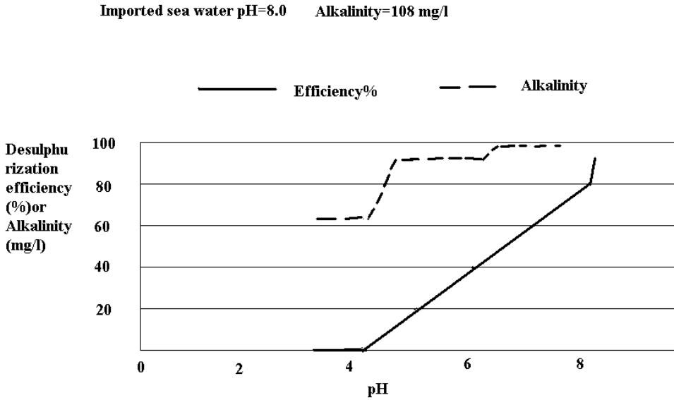
Fig. 3. The pH and alkalinity of exit seawater and desulphurization efficiency diagram
