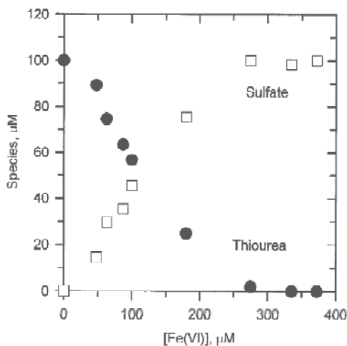
Fig. 10. A plot of thiourea consumption and sulfate formation versus [Fe(VI)] at pH 9.0 (Initial Thiourea: 100 \times 10^{-6} M; [Fe(VI)] = 50-375 \mu\text{M} ) [70].
