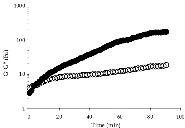
Fig. 1. Laccase induced gelation of FAXWB solutions at 5 % (w/v) ( G' ●, G'' ○). Rheological measurements made at 25°C, 0.25 Hz and 5% strain.
