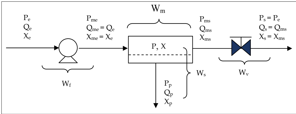
Fig. 5. Systemic diagram of a simple process.
