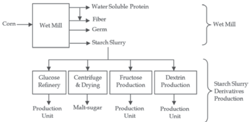
Fig. 3. Process flow diagram for a typical corn processing industry
