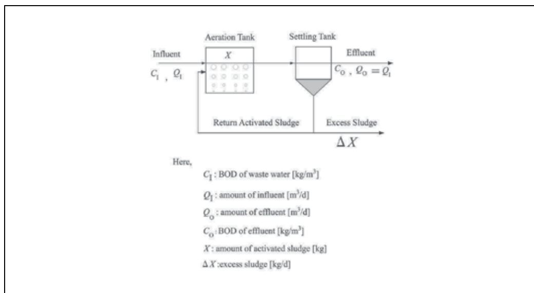
Fig. 2. Model diagram of a WWTP
