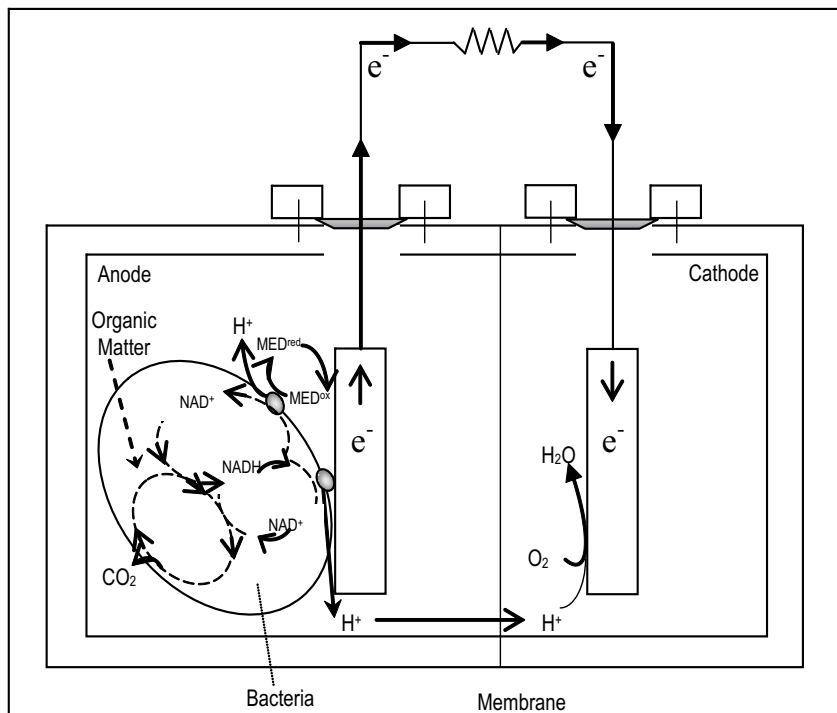
Fig. 3. Schematic of the basic components of a MFC. Bacteria grow on the anode, oxidising organic matter and releasing electrons. The cathode is sparged with air to provide dissolved oxygen for the reaction of electrons, protons and oxygen at the cathode, completing the circuit and producing power. (Logan, 2008)
