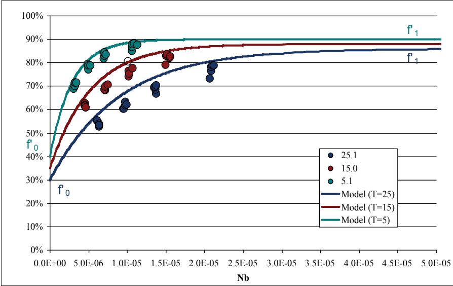
Fig. 3. Experimental data for nanofiltration of DEG in aqueous solution at different temperatures. Adequacy of the model of separation flow in a nanoscale pore.
