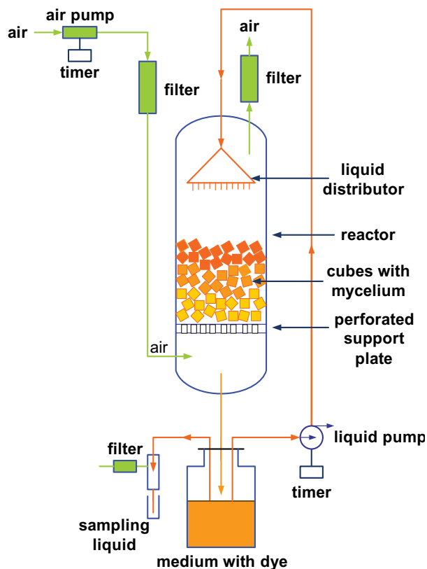
Fig. 4. Trickle bed reactor for decolourization of RO 16 with Irpex lacteus
