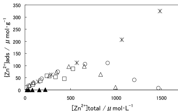
Fig. 1. Adsorption of Zn^{2+} ions onto Al_2O_3 . Relationship between the total concentration of Zn^{2+} and amount of Zn adsorbed by 1g of Al_2O_3 is shown. The experiments were performed at constant pH of 6.50 for Zn^{2+} concentrations ranging up to 600 \mu\text{mol/L} (□), 1000 \mu\text{mol/L} (Δ), 1500 \mu\text{mol/L} (○), and 3,000 \mu\text{mol/L} (*). Blank experiment was carried out in the absence of solid (▲).
