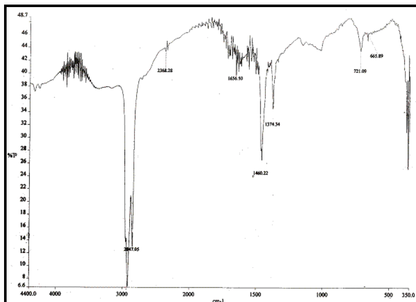
Fig. 3a. FTIR spectrum of the mixture of seed and sponge of L. cylindrica biosorbent before biosorption.
