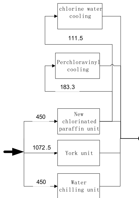
Fig. 11. Cooling water system retrofit solution 2
