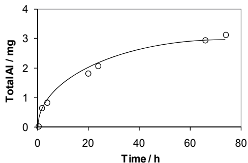
Fig. 6. Aluminum ion released in the solution outside the bag during \text{Cu}(\text{OH})_2 interaction with alumina.
