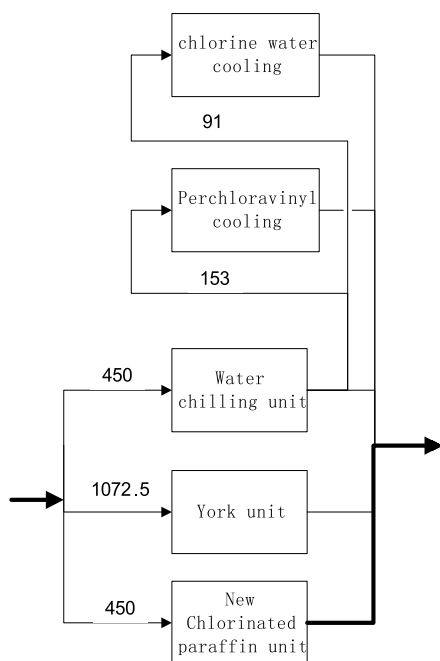
Fig. 10. Cooling water system retrofit solution 1
