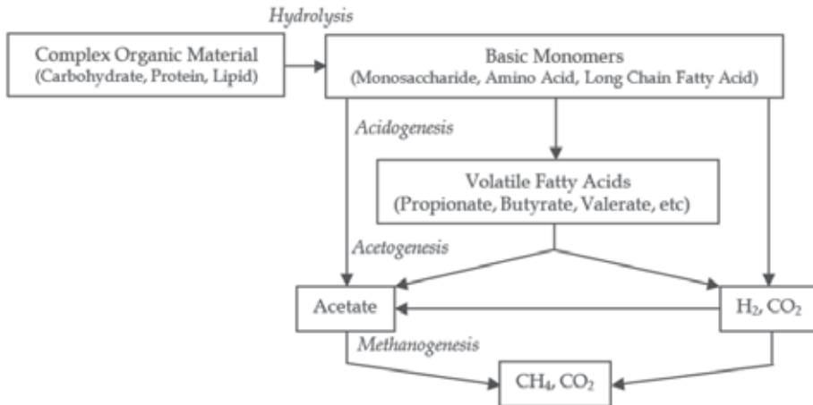
Fig. 1. Steps of anaerobic digestion process
