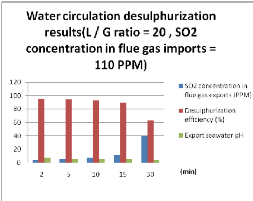
Fig. 5. The seawater circulation desulphurization test results
