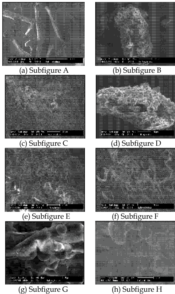
Fig. 1. Scanning electron microscopy of Luffa cylindrica seeds and sponge mixture biosorbent: (A) transversal view of the mixture of seed and sponge 33 \times ; (B, C, D, E) transversal view of the mixture of seed and sponge 1000 \times ; (G, H) transversal view of the mixture of seed and sponge 5000 \times .
