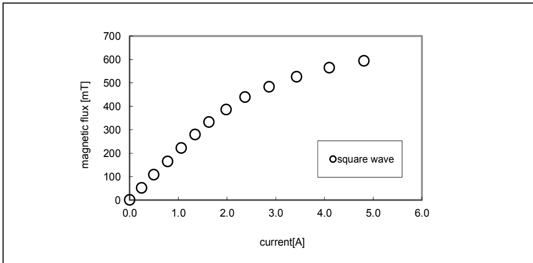
Fig. 14. B - I relationship of a coil
