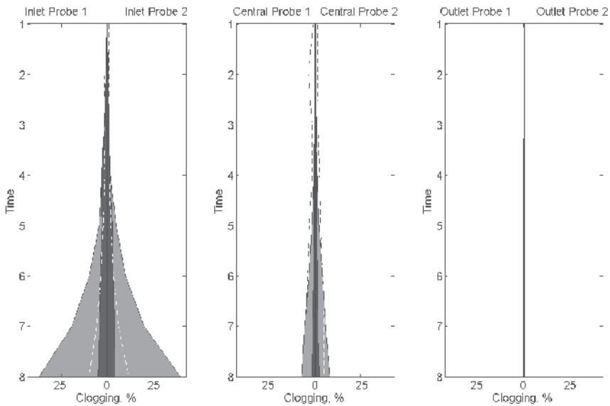
Fig. 12. Simulated results of typical monitored output for six probe system. Grey is biological clogging whilst black represents particulate clogging. The dashed line is 10 times the ratio between them.
