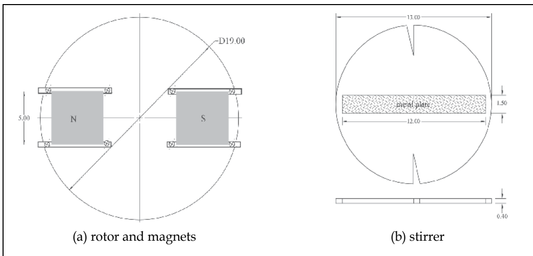
Fig. 11. Diagrams of the rotor and stirrer
