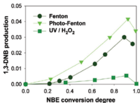
Fig. 10. Relative production of 1,3-dinitrobenzene against the conversion degree of nitrobenzene.
