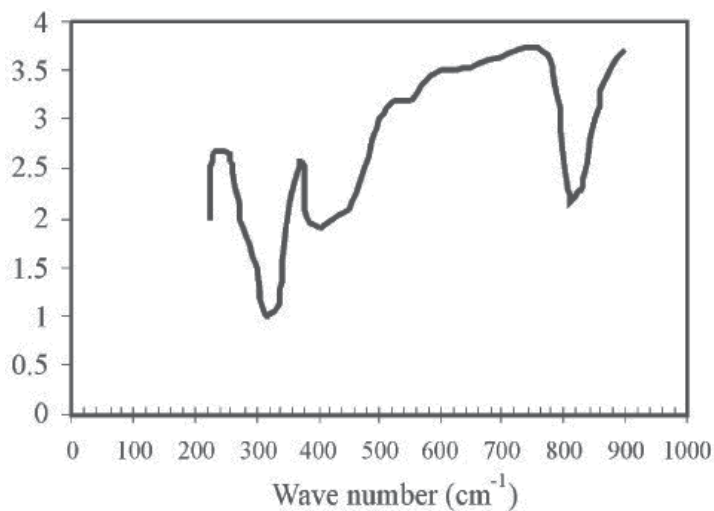
Fig. 3. IR spectrum of potassium ferrate [17].
