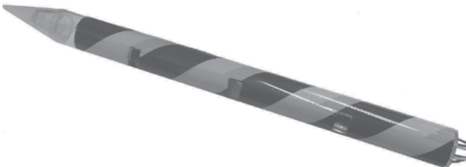
Fig. 9. Magnetic resonance probe used to determine the ratios of particulate and biological clogging. This version has three sensors spaced along its length.
