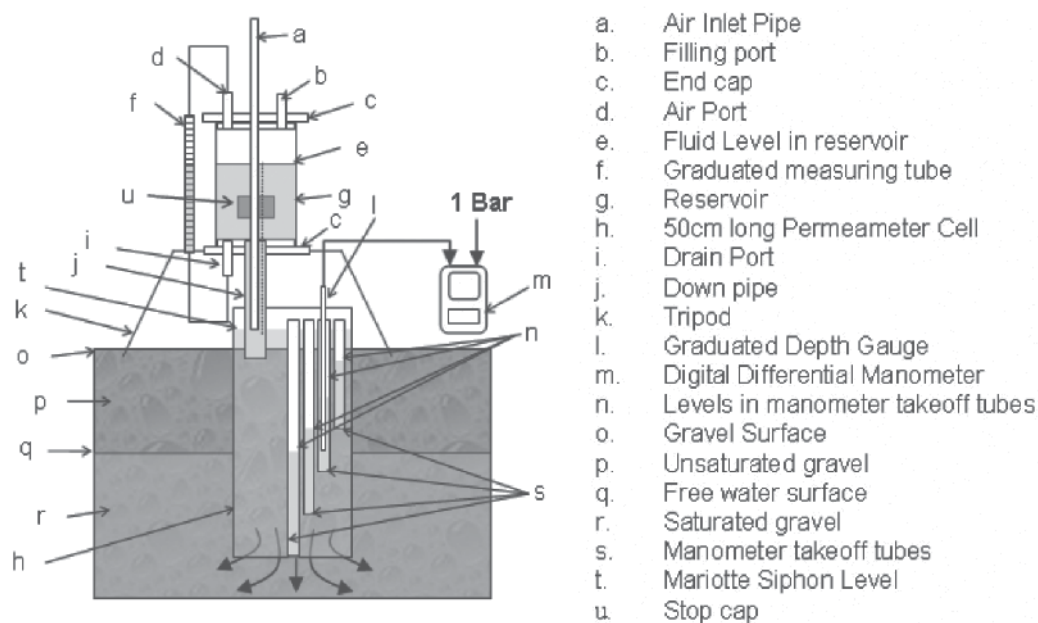
Fig. 9. Experimental set-up for the in situ determination of the vertical hydraulic conductivity profile of high porous media (not to scale). Reproduced from Knowles and Davies (2009b).
