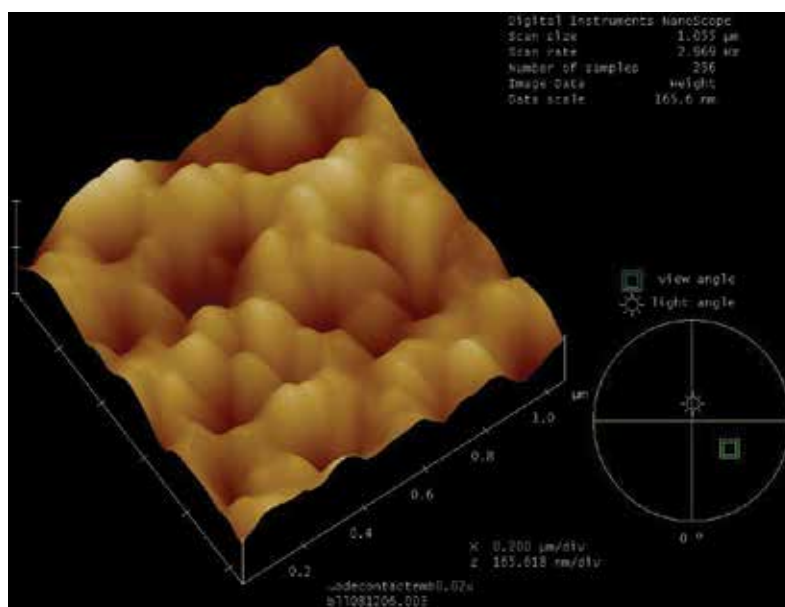
Fig. 6. Ceramic membrane D_p = 20\ \text{nm} . Image Scanning Probe Microscope 1 \times 1\ \mu\text{m} , contact mode, ambient air.
