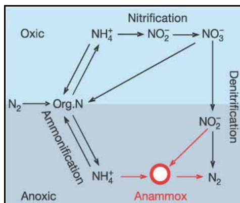
Fig. 1. Anammox in the context of nitrogen cycle (Modified from Kuyper, et al., 2003).
