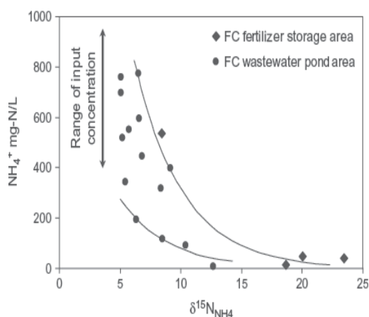
Fig 5. Evolution of \delta^{15}\text{N}_{\text{NH}_4} during anammox reaction for the high \text{NH}_4^+ - \text{NO}_3^- fertilizer company ground water. Trend lines calculated from a Rayleigh distillation with a reaction enrichment factor of 4%.
