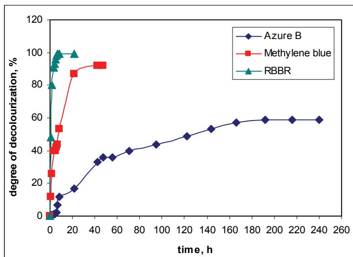
Fig. 6. Decolourization of various dyes in rotating discs reactor
