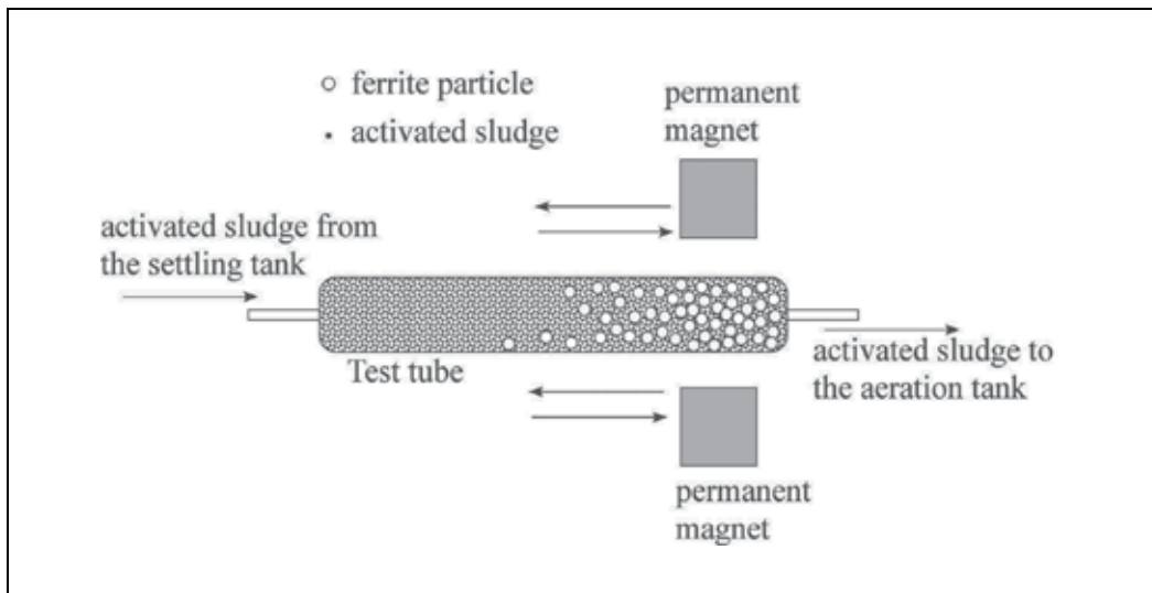
Fig. 4. Model diagram of test tube treatment plant
