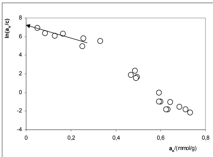
Fig. 3. Dependence of a_e/c versus a_e as obtained for lead(II) adsorption on sample OC at 30°C
