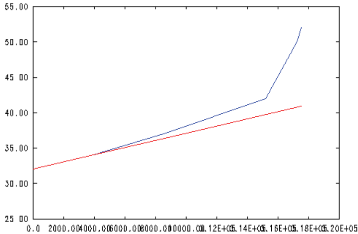
Fig. 7. Cooling water composite curve
