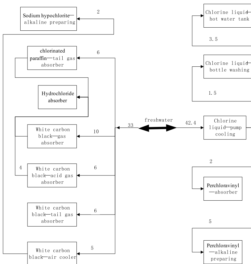
Fig. 13. Water reuse scheme in plant 2
