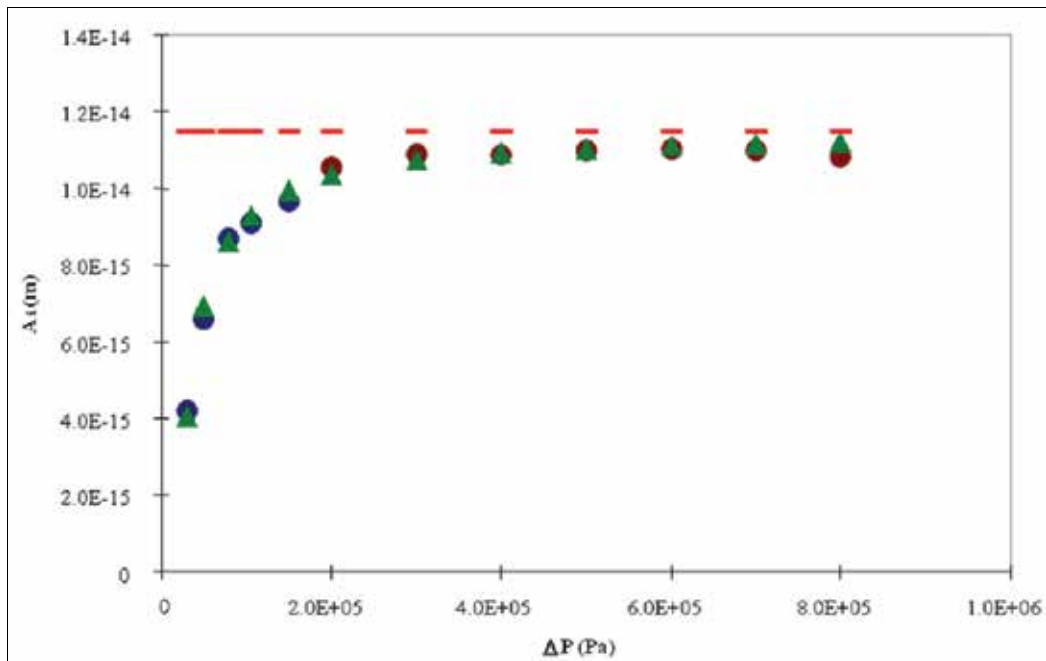
Fig. 2. Permeability of pure water at 25°C: comparison of Bingham and Poiseuille models with experimental data in hyperfiltration.
