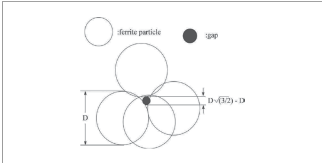
Fig. 3. Estimated gap made by ferrite particles
