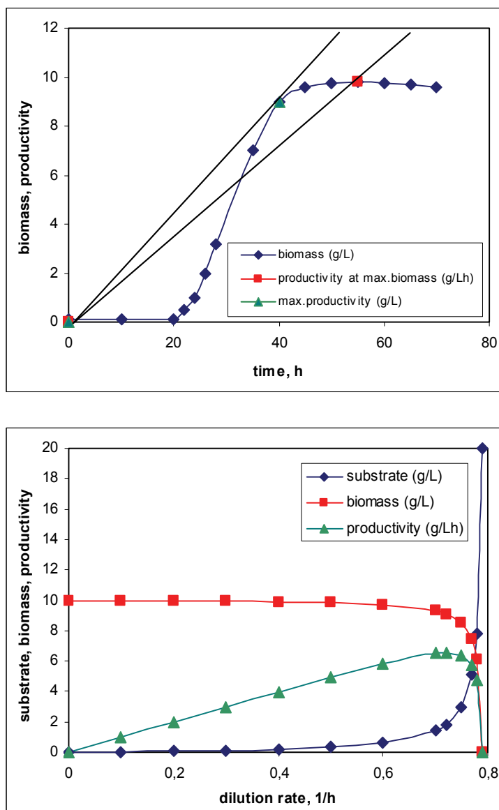
Fig. 3. Biomass productivity during batch (above) and continuous operation (below) of stirred tank reactor
