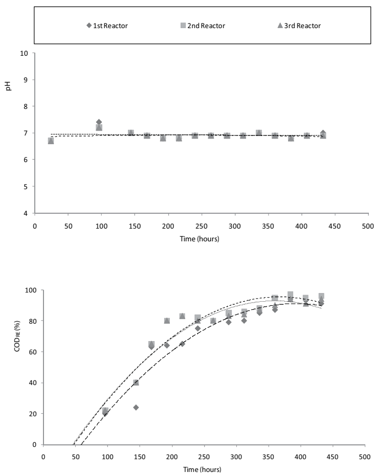
Fig. 2. Variation of pH and COD_{RE} (%) during the start-up period (HRT=9 days).
