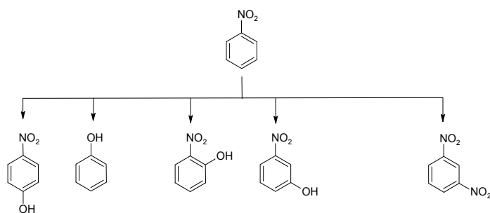
Scheme 1. Nitrobenzene primary hydroxylation and nitration pathways
