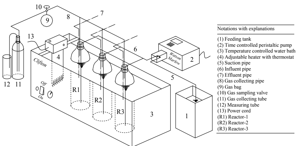
Fig. 1. Detailed schematic of the experimental set-up
