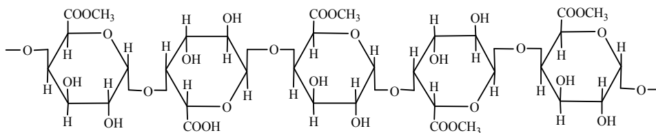
Fig. 1. Structural formula of the polygalacturonic acid.
