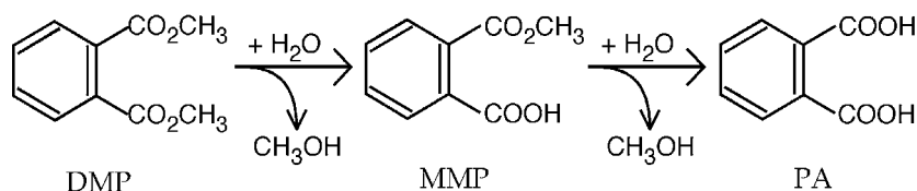
Scheme 1. Possible mechanism of DMP oxidation.
