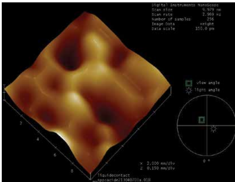
Fig. 10. Surface modification of ceramic membrane D_p = 20 nm with sulfonated oxide of polyphenyl. Image Scanning Probe Microscope 10 \times 10 nm, contact mode, aqueous medium, ambient temperature and pressure.
