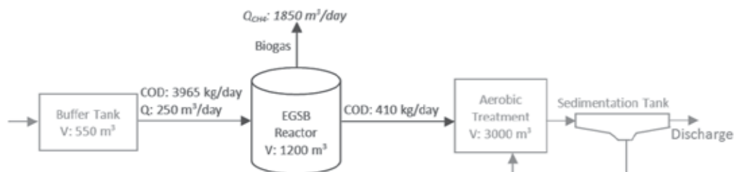
Fig. 8. Mass balance study for a wastewater treatment plant of the confectionery industry
