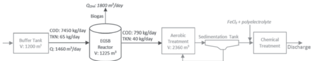
Fig. 4. Mass balance study for a wastewater treatment plant of the corn processing industry
