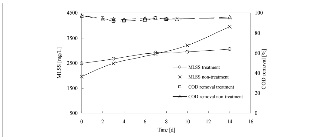
Fig. 12. Sludge reduction rotary treatment plant
