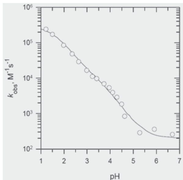
Fig. 9. The second-order rate constants for the decay of ferrate(VI) to iron(II) in 5 mM (phosphate/acetate) buffers [36].
