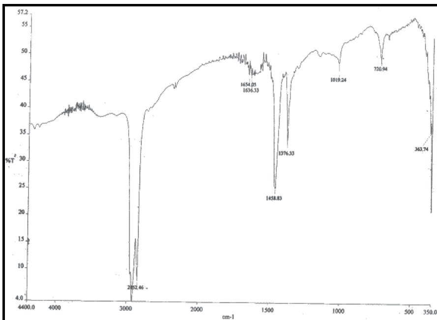
Fig. 3d. FTIR spectrum of the mixture of seed and sponge of L. cylindrica biosorbent after biosorption of Pb^{2+} ions.
