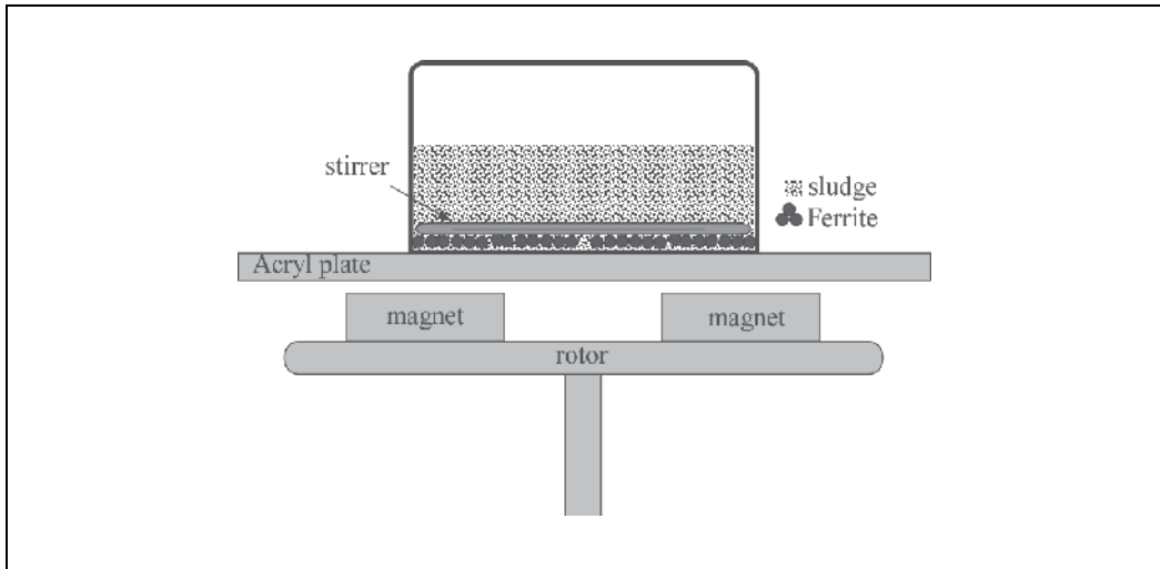
Fig. 10. Model diagram for rotary treatment plant
