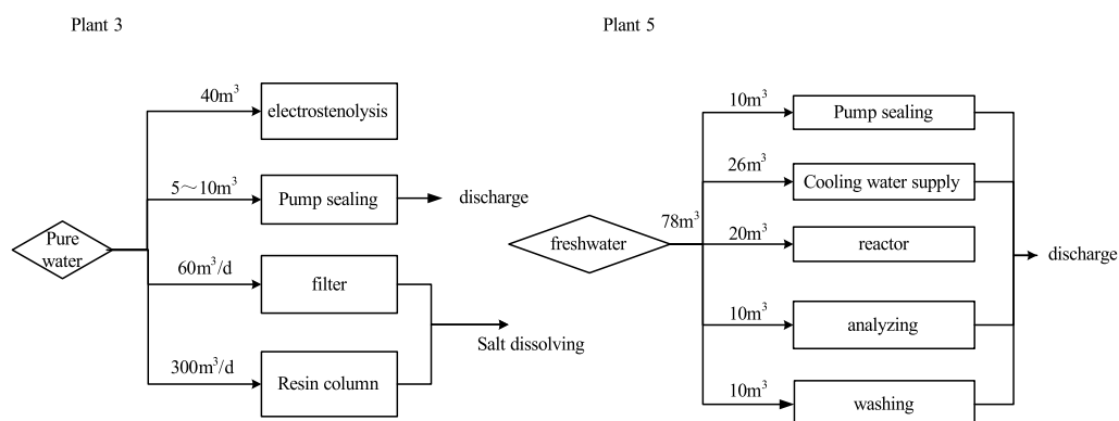
Fig. 4. Balanced water system of plant 3 and 5
