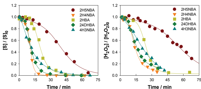
Fig. 9. Normalized concentration profiles of model substrates obtained in the photo-Fenton process.
