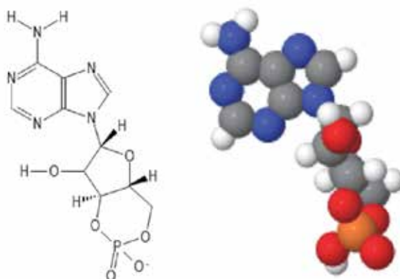
Fig. 1. Chemical and 3D structures of cAMP (Molecular formula: C_{10}H_{12}N_5O_6P )
