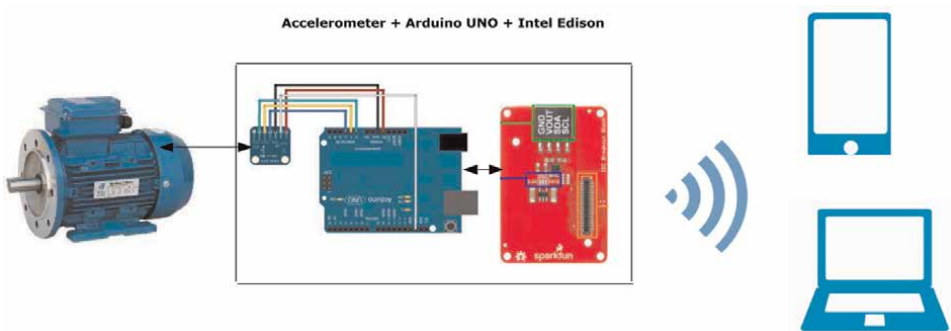
Figure 5. Experimental setup.
