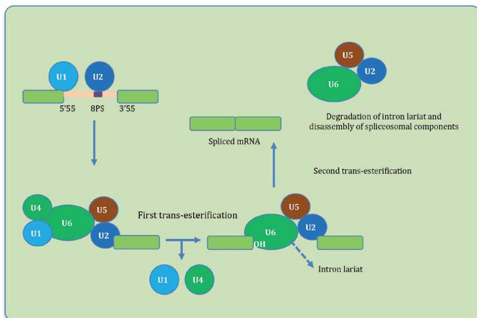
Figure 1. Two-step splicing reaction. Splicing occurs by a 2-step trans-esterification reaction to remove introns and join exons together. The first step, U1 small nuclear ribonucleoprotein (snRNP) assembles at the 5' splice site of an exon and U2 snRNP at the branch point sequence (BPS), just upstream of the 3' splice site of the adjacent/downstream exon. This configuration is known as the pre-spliceosome. Hereafter, U1 and U2 are joined by the snRNPs U5 and U4–U6 complexes to form the pre catalytic spliceosome. Next, U4–U6 complexes unwind, releasing U4 and U1 from the pre-spliceosomal complex. This allows U6 to base pair with the 5' splice site and the BPS. The 5' splice site gets cleaved, which leads to a free 3' OH-group at the upstream exon, and a branched intronic region at the downstream exon called the intron lariat.
