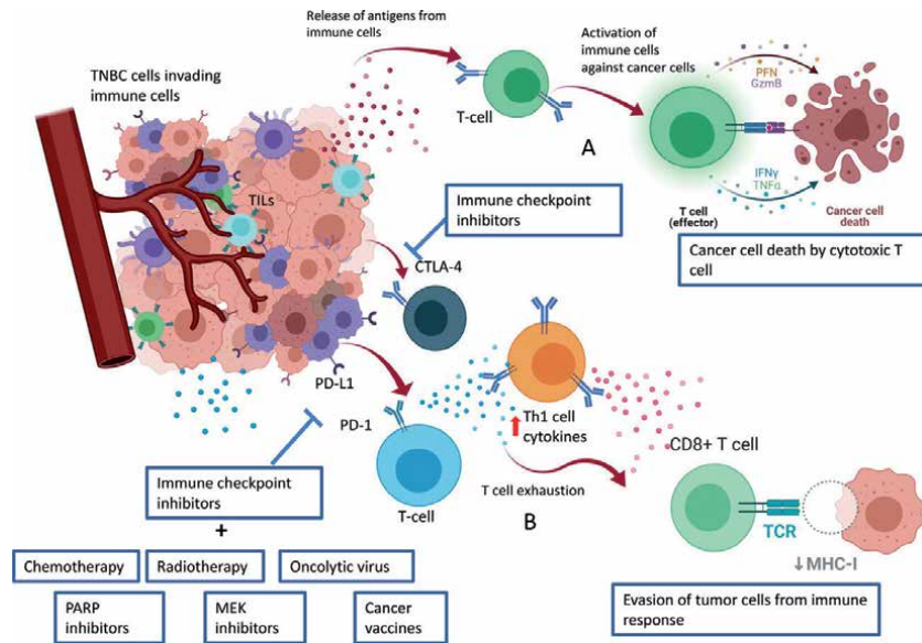
Figure 2. Overview of involvement of immune system in TNBC with combination treatment options; A. Represents on recognition of the antigen from the tumor cell the immune cell destroying the tumor cell B. Shows that how PD-L1 from the tumor cell interacts with PD-1 and this binding causes T cell exhaustion and helps the tumor cell evading the immune response.
